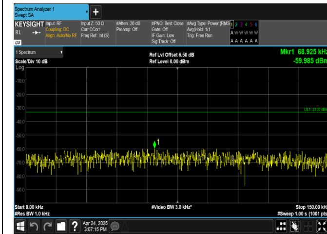
Band26(824-849)-15MHz-16QAM-26965-1RB#74-0.009-0.15-PASS
