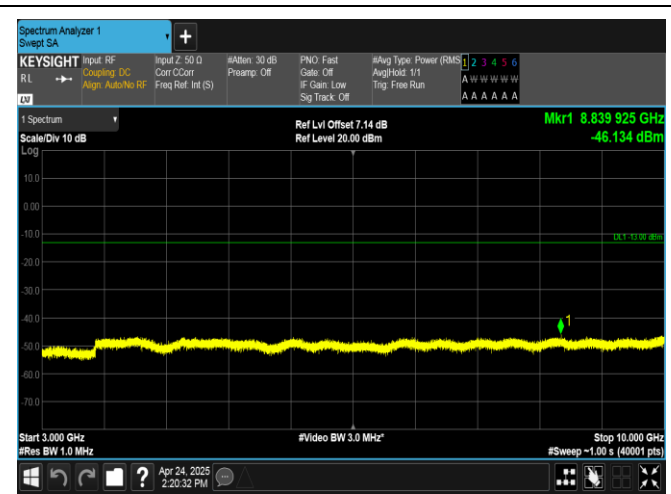
Band26(824-849)-15MHz-16QAM-26865-1RB#0-3000-10000-PASS
