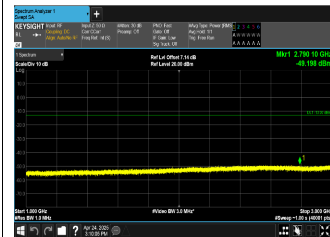
Band26(824-849)-15MHz-16QAM-26965-75RB#0-1000~3000-PASS
