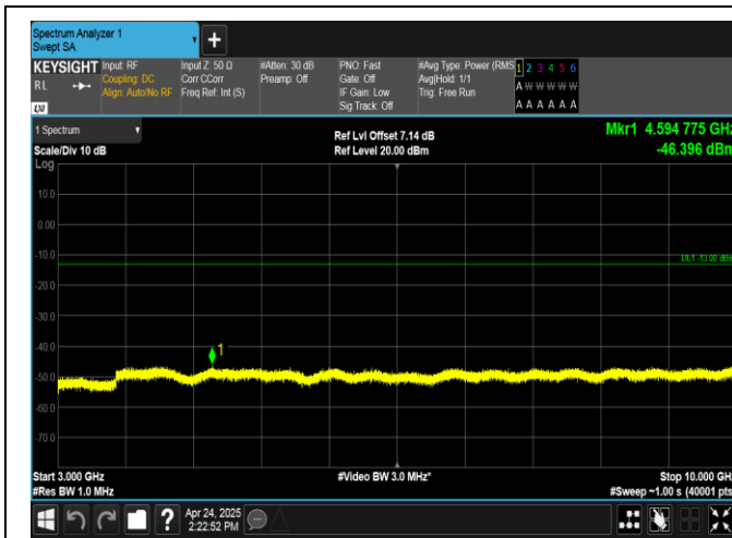
Band26(824-849)-15MHz-16QAM-26865-1RB#74-3000~10000-PASS
