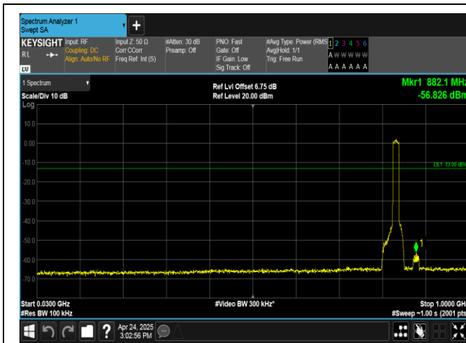
Band26(824-849)-15MHz-16QAM-26915-75RB#0-30~1000-PASS
