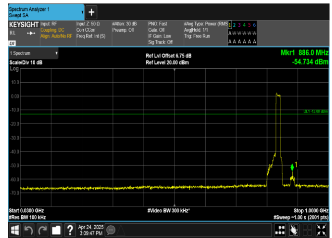
Band26(824-849)-15MHz-16QAM-26965-75RB#0-30~1000-PASS
