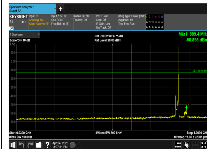
Band26(824-849)-15MHz-16QAM-26965-1RB#74-30-1000-PASS
