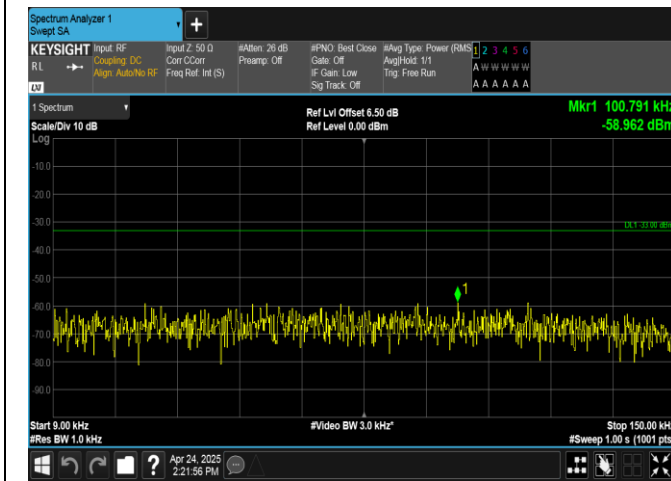
Band26(824-849)-15MHz-16QAM-26865-1RB#74-0.009-0.15-PASS
