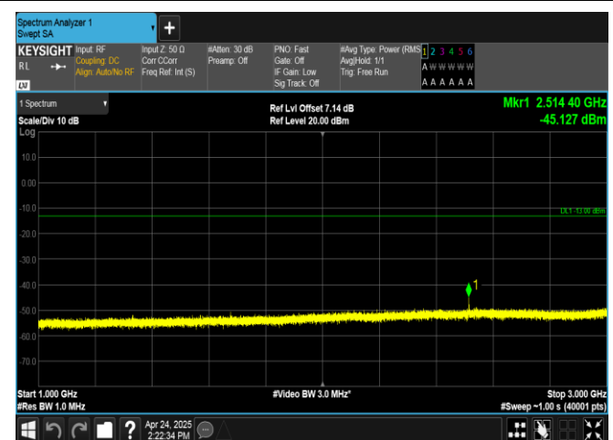
Band26(824-849)-15MHz-16QAM-26865-1RB#74-1000-3000-PASS
