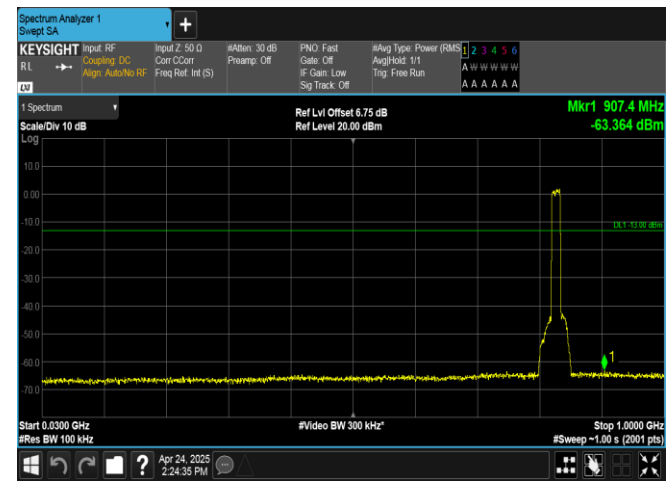
Band26(824-849)-15MHz-16QAM-26865-75RB#0-30~1000-PASS
