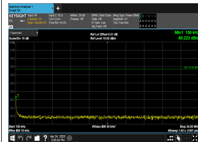
Band26(824-849)-15MHz-16QAM-26965-1RB#0-0.15~30-PASS
