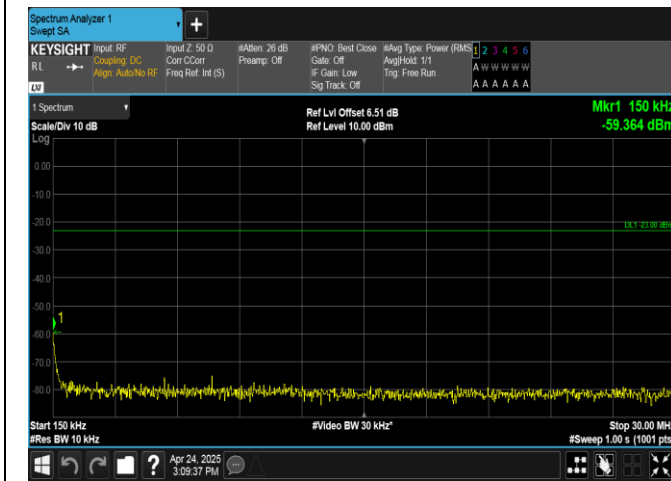
Band26(824-849)-15MHz-16QAM-26965-75RB#0-0.15~30-PASS
