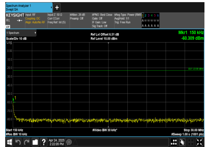
Band26(824-849)-15MHz-16QAM-26865-1RB#74-0.15-30-PASS
