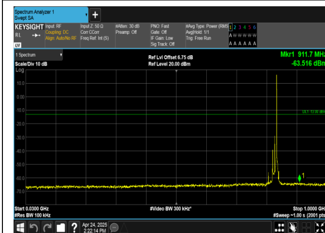
Band26(824-849)-15MHz-16QAM-26865-1RB#74-30-1000-PASS
