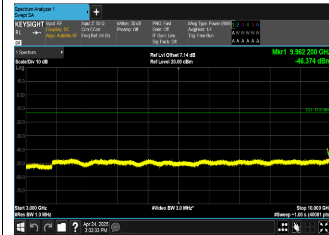
Band26(824-849)-15MHz-16QAM-26915-75RB#0-3000~10000-PASS
