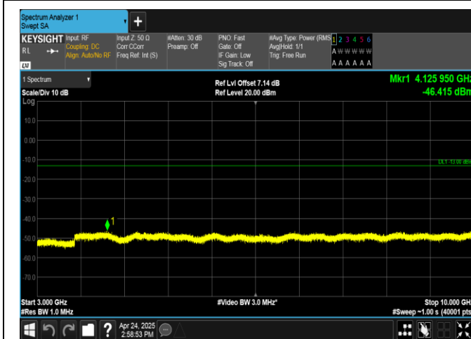
Band26(824-849)-15MHz-16QAM-26915-1RB#0-3000~10000-PASS
