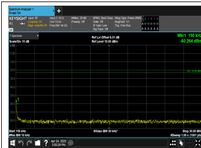
Band26(824-849)-15MHz-16QAM-26915-1RB#74-0.15~30-PASS
