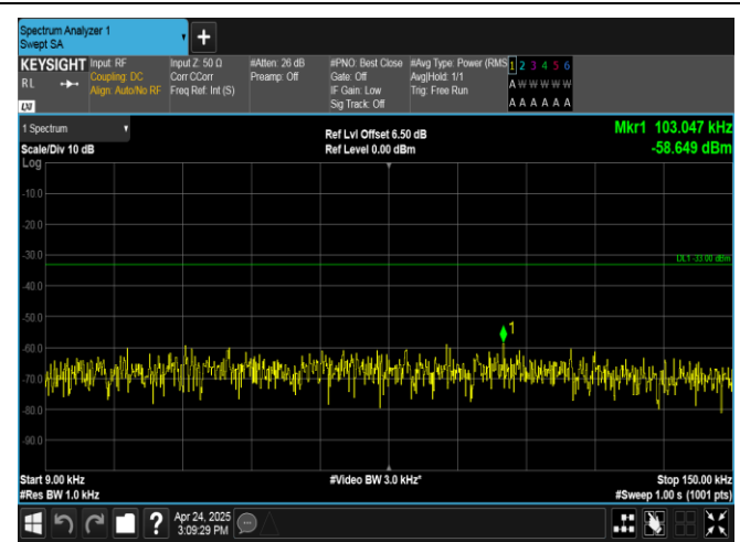
Band26(824-849)-15MHz-16QAM-26965-75RB#0-0.009~0.15-PASS
