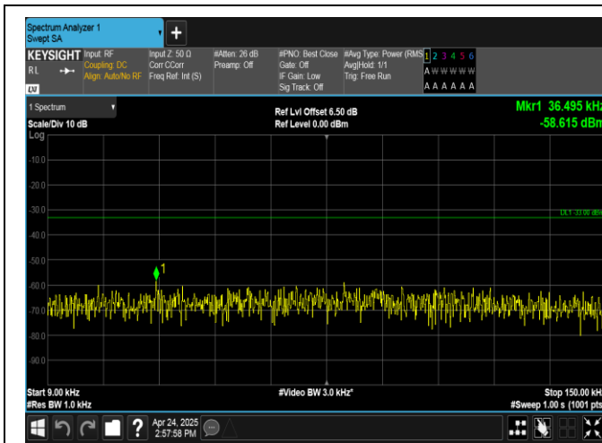
Band26(824-849)-15MHz-16QAM-26915-1RB#0-0.009~0.15-PASS
