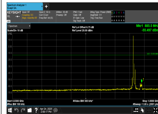
Band26(824-849)-15MHz-16QAM-26915-1RB#0-30~1000-PASS
