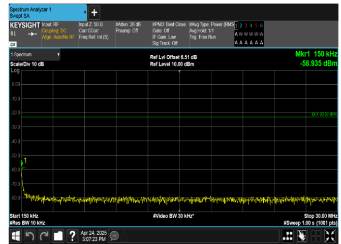
Band26(824-849)-15MHz-16QAM-26965-1RB#74-0.15-30-PASS
