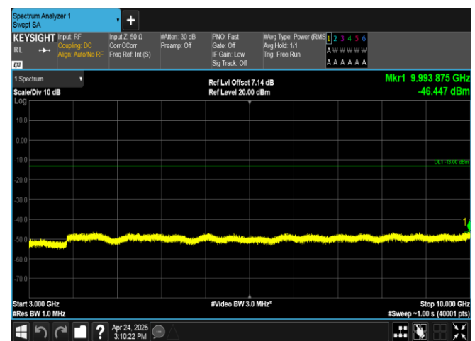
Band26(824-849)-15MHz-16QAM-26965-75RB#0-3000~10000-PASS
