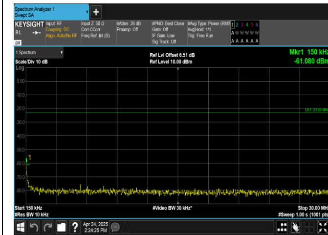
Band26(824-849)-15MHz-16QAM-26865-75RB#0-0.15~30-PASS
