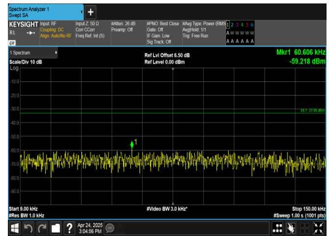
Band26(824-849)-15MHz-16QAM-26965-1RB#0-0.009~0.15-PASS
