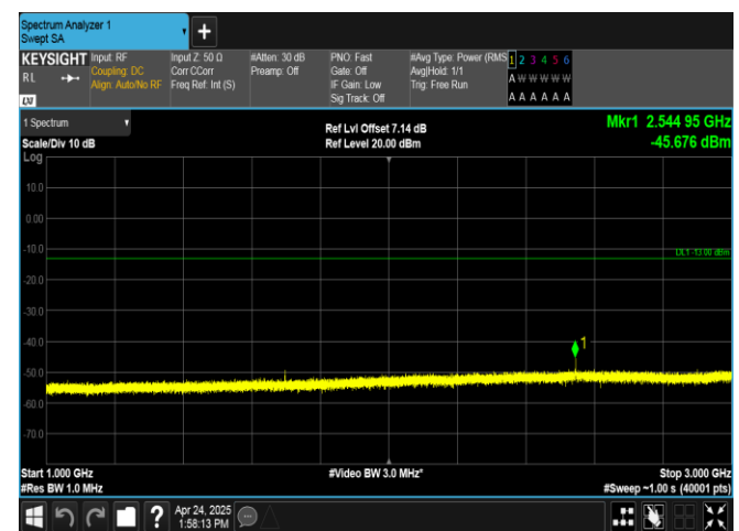
Band26(824-849)-10MHz-16QAM-26990-1RB#49-1000-3000-PASS
