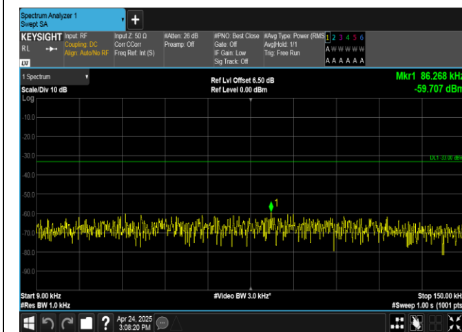
Band26(824-849)-15MHz-QPSK-26965-75RB#0-0.009~0.15-PASS
