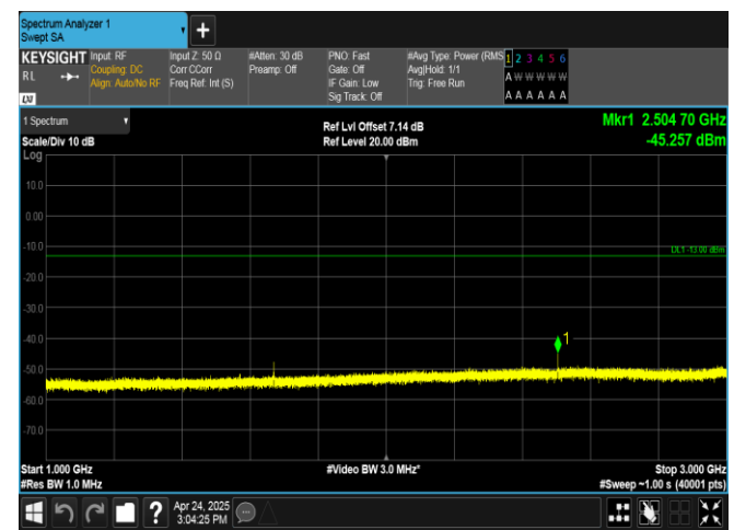
Band26(824-849)-15MHz-QPSK-26965-1RB#0-1000~3000-PASS
