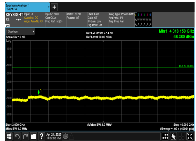
Band26(824-849)-15MHz-QPSK-26965-1RB#74-3000~10000-PASS
