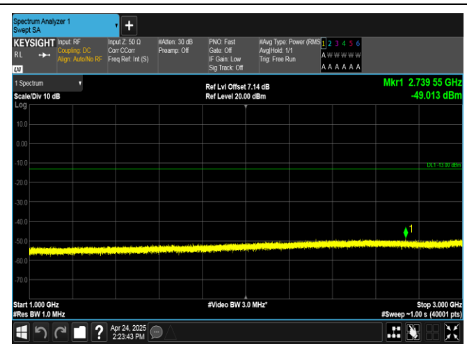
Band26(824-849)-15MHz-QPSK-26865-75RB#0-1000~3000-PASS
