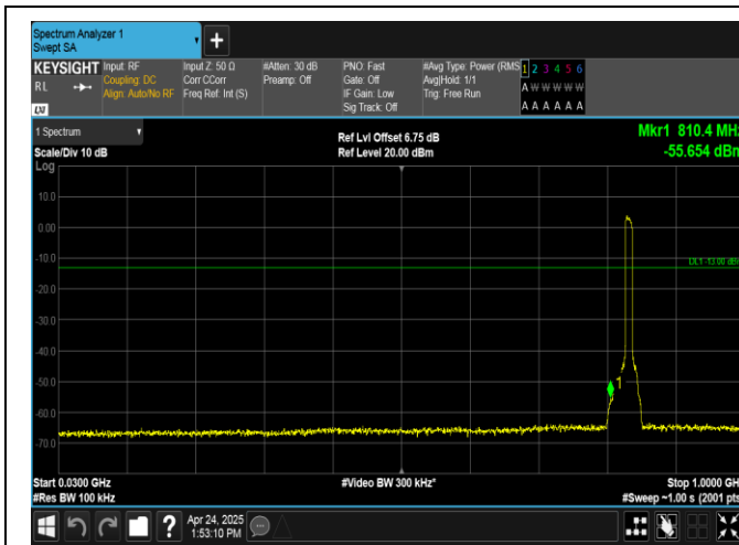
Band26(824-849)-10MHz-16QAM-26915-50RB#0-30~1000-PASS
