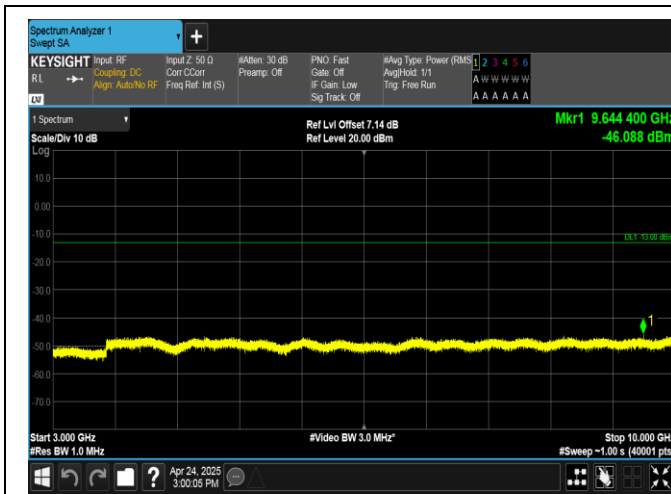
Band26(824-849)-15MHz-QPSK-26915-1RB#74-3000~10000-PASS
