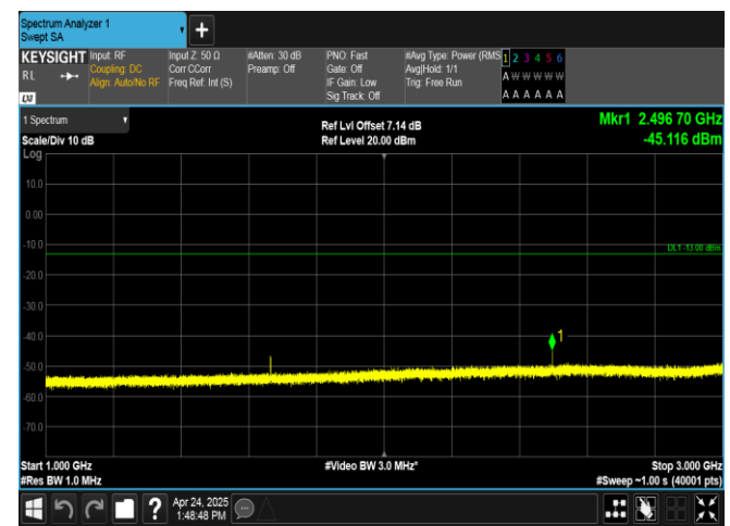
Band26(824-849)-10MHz-16QAM-26915-1RB#0-1000~3000-PASS
