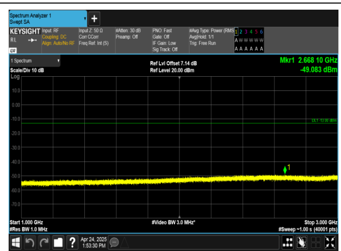
Band26(824-849)-10MHz-16QAM-26915-50RB#0-1000~3000-PASS
