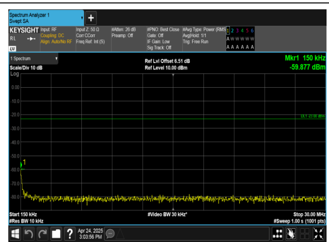
Band26(824-849)-15MHz-QPSK-26965-1RB#0-0.15~30-PASS
