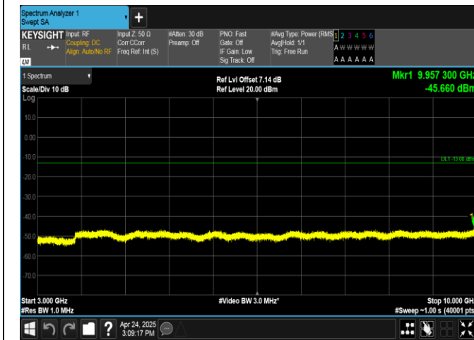
Band26(824-849)-15MHz-QPSK-26965-75RB#0-3000~10000-PASS
