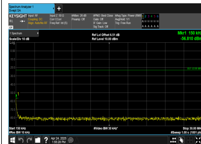
Band26(824-849)-10MHz-16QAM-26990-1RB#0-0.15~30-PASS
