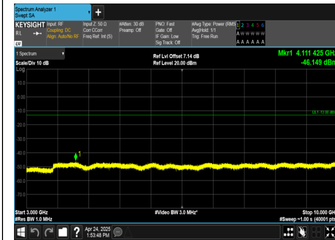
Band26(824-849)-10MHz-16QAM-26915-50RB#0-3000~10000-PASS
