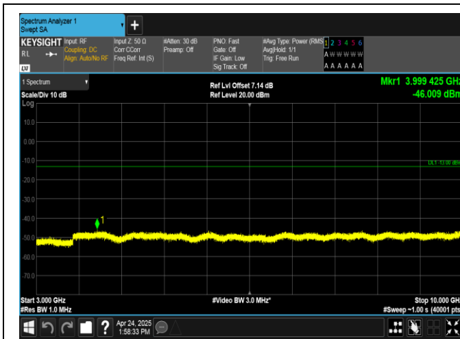
Band26(824-849)-10MHz-16QAM-26990-1RB#49-3000~10000-PASS
