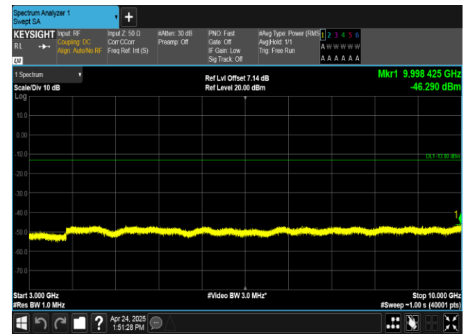
Band26(824-849)-10MHz-16QAM-26915-1RB#49-3000~10000-PASS
