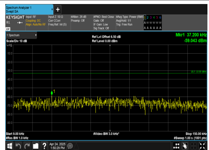
Band26(824-849)-10MHz-16QAM-26915-1RB#49-0.009~0.15-PASS
