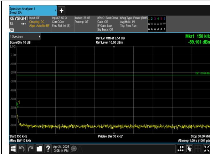
Band26(824-849)-15MHz-QPSK-26965-1RB#74-0.15~30-PASS
