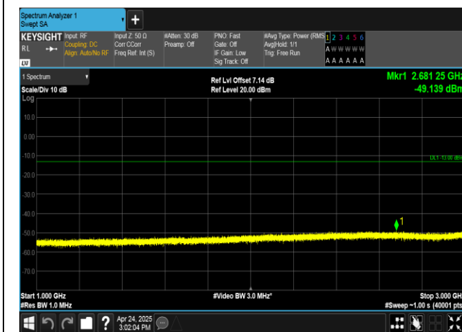
Band26(824-849)-15MHz-QPSK-26915-75RB#0-1000~3000-PASS
