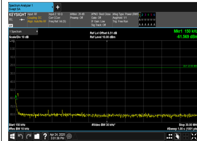
Band26(824-849)-15MHz-QPSK-26915-75RB#0-0.15~30-PASS
