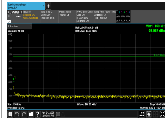
Band26(824-849)-10MHz-16QAM-26990-50RB#0-0.15~30-PASS
