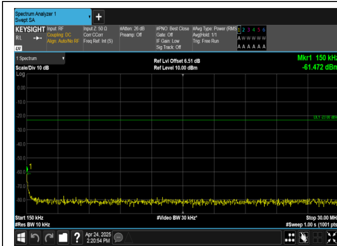
Band26(824-849)-15MHz-QPSK-26865-1RB#74-0.15~30-PASS
