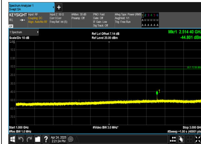
Band26(824-849)-15MHz-QPSK-26865-1RB#74-1000~3000-PASS
