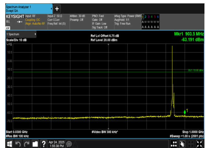
Band26(824-849)-10MHz-16QAM-26990-1RB#0-30~1000-PASS
