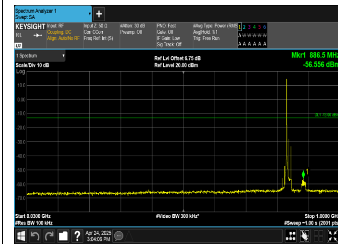
Band26(824-849)-15MHz-QPSK-26965-1RB#0-30~1000-PASS
