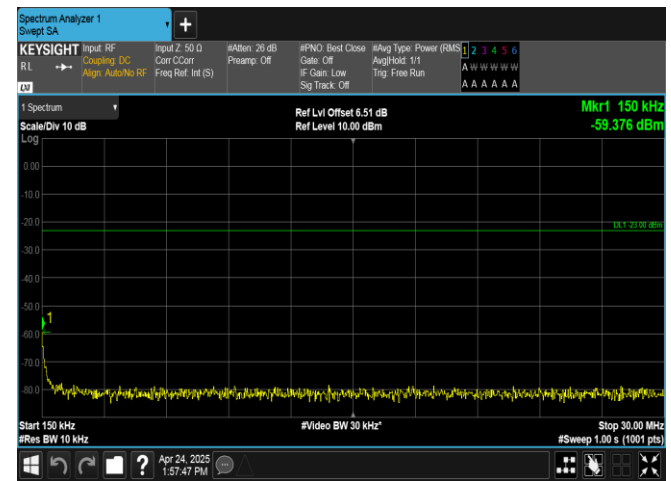
Band26(824-849)-10MHz-16QAM-26990-1RB#49-0.15-30-PASS
