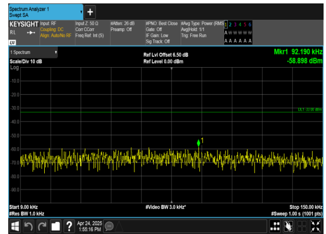
Band26(824-849)-10MHz-16QAM-26990-1RB#0-0.009~0.15-PASS
