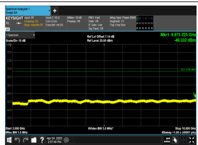
Band26(824-849)-15MHz-QPSK-26915-1RB#0-3000~10000-PASS
