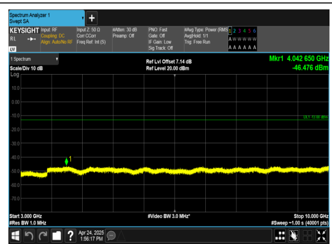
Band26(824-849)-10MHz-16QAM-26990-1RB#0-3000-10000-PASS
