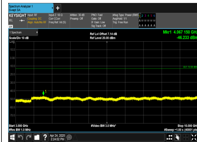
Band26(824-849)-15MHz-QPSK-26865-75RB#0-3000~10000-PASS
