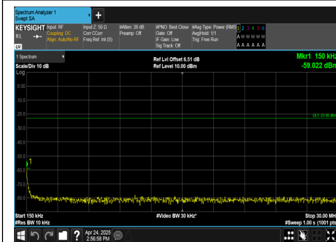
Band26(824-849)-15MHz-QPSK-26915-1RB#0-0.15~30-PASS
