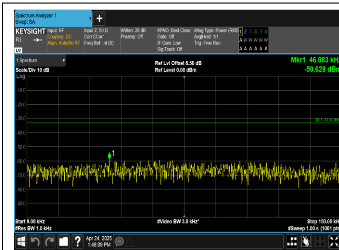
Band26(824-849)-10MHz-16QAM-26915-1RB#0-0.009~0.15-PASS
