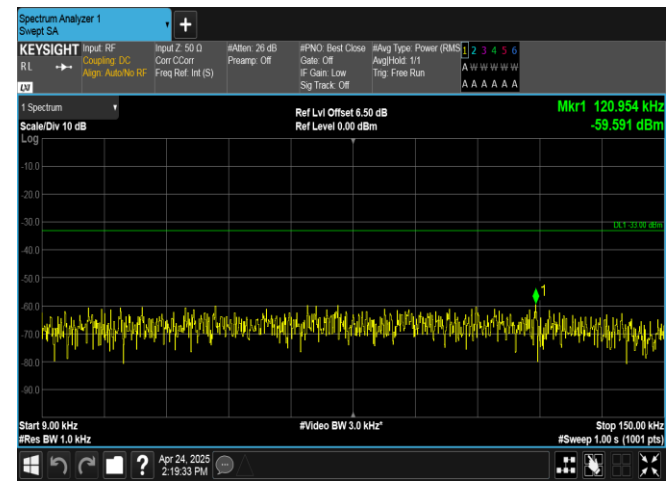
Band26(824-849)-15MHz-16QAM-26865-1RB#0-0.009~0.15-PASS
