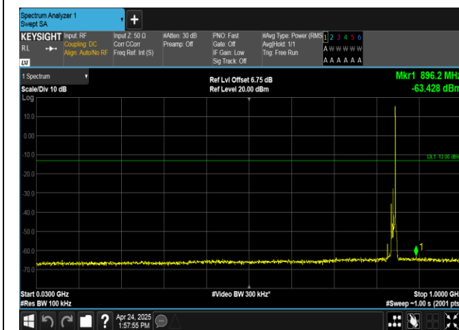
Band26(824-849)-10MHz-16QAM-26990-1RB#49-30-1000-PASS
