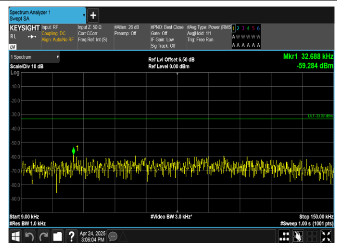
Band26(824-849)-15MHz-QPSK-26965-1RB#74-0.009~0.15-PASS
