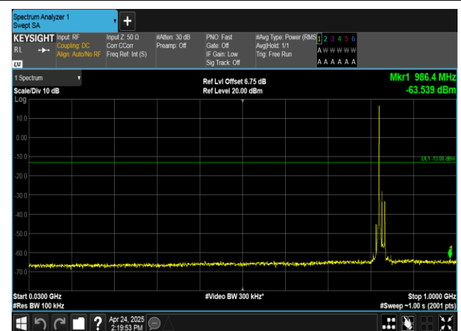
Band26(824-849)-15MHz-16QAM-26865-1RB#0-30~1000-PASS
