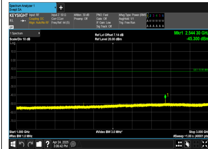
Band26(824-849)-15MHz-QPSK-26965-1RB#74-1000~3000-PASS
