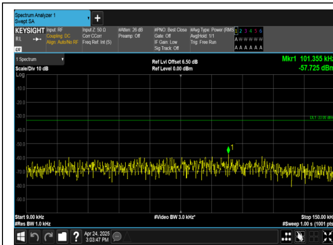
Band26(824-849)-15MHz-QPSK-26965-1RB#0-0.009~0.15-PASS
