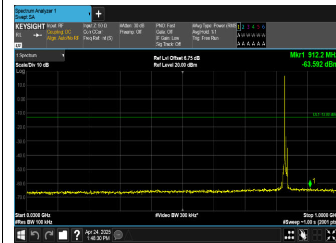
Band26(824-849)-10MHz-16QAM-26915-1RB#0-30~1000-PASS
