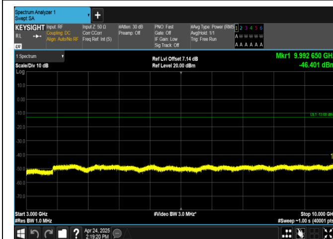
Band26(824-849)-15MHz-QPSK-26865-1RB#0-3000~10000-PASS
