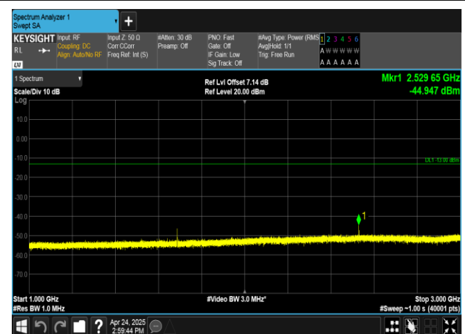
Band26(824-849)-15MHz-QPSK-26915-1RB#74-1000~3000-PASS
