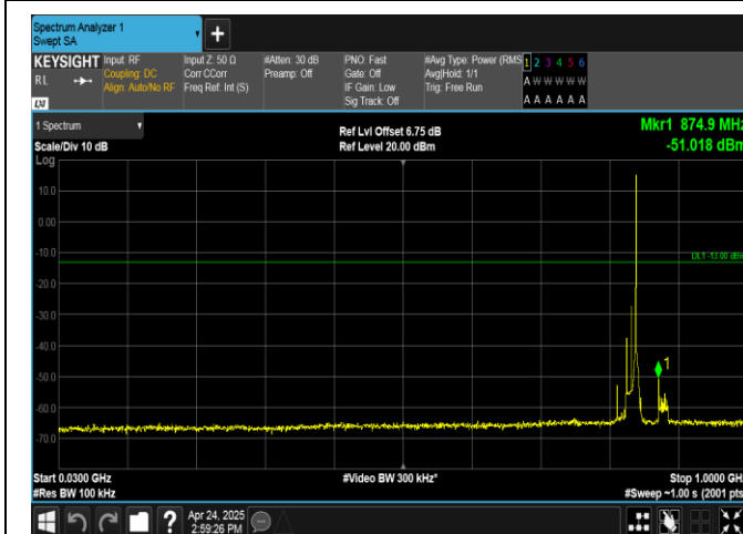
Band26(824-849)-15MHz-QPSK-26915-1RB#74-30~1000-PASS
