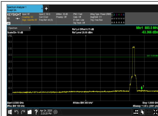
Band26(824-849)-15MHz-QPSK-26865-75RB#0-30~1000-PASS
