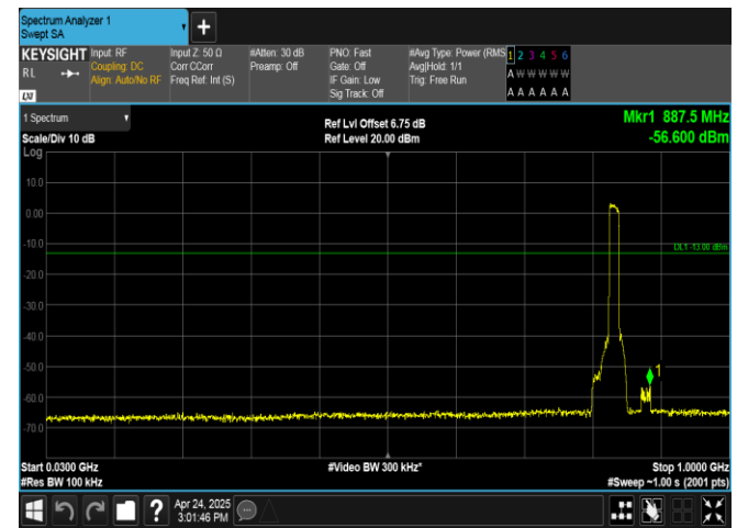
Band26(824-849)-15MHz-QPSK-26915-75RB#0-30~1000-PASS
