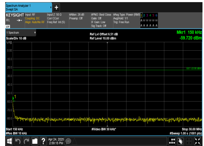
Band26(824-849)-15MHz-QPSK-26915-1RB#74-0.15~30-PASS
