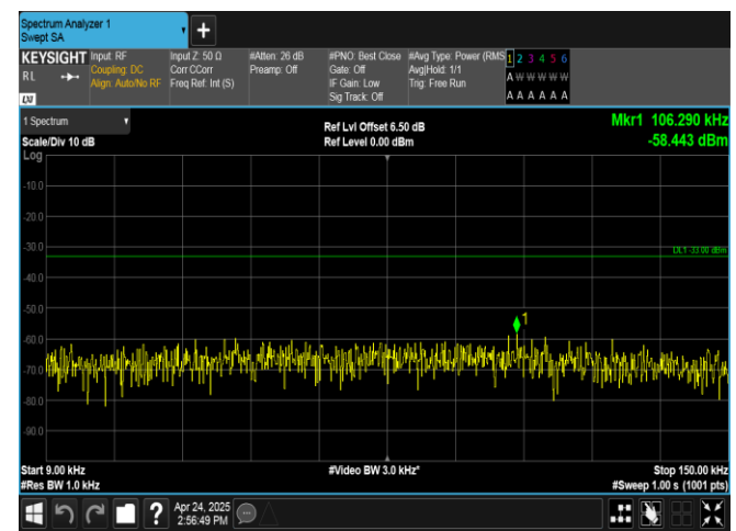
Band26(824-849)-15MHz-QPSK-26915-1RB#0-0.009~0.15-PASS
