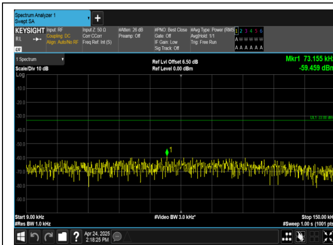
Band26(824-849)-15MHz-QPSK-26865-1RB#0-0.009~0.15-PASS
