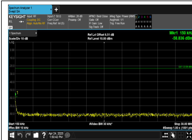
Band26(824-849)-10MHz-16QAM-26915-1RB#49-0.15~30-PASS
