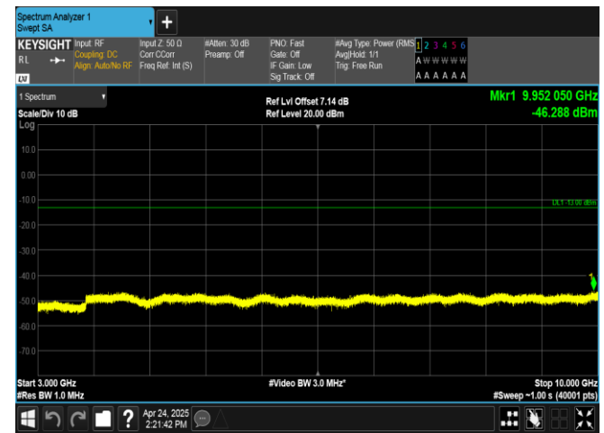
Band26(824-849)-15MHz-QPSK-26865-1RB#74-3000~10000-PASS
