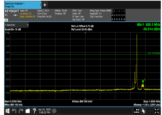
Band26(824-849)-15MHz-QPSK-26965-1RB#74-30~1000-PASS
