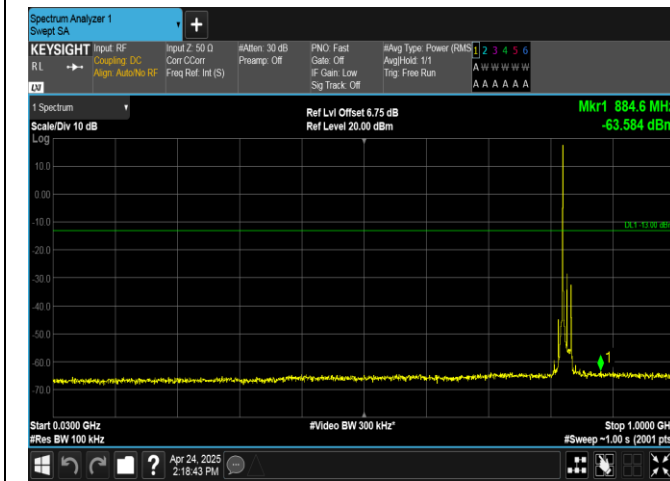
Band26(824-849)-15MHz-QPSK-26865-1RB#0-30~1000-PASS
