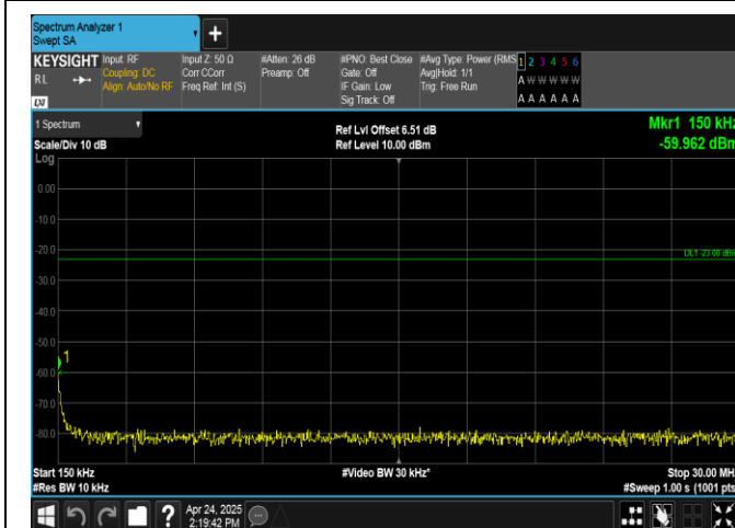
Band26(824-849)-15MHz-16QAM-26865-1RB#0-0.15~30-PASS
