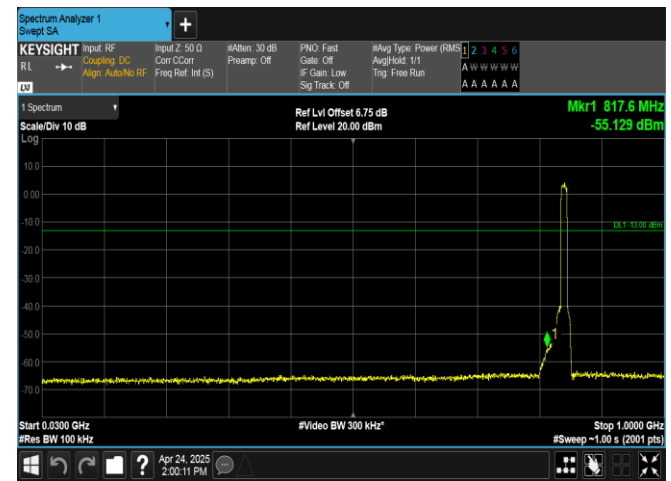
Band26(824-849)-10MHz-16QAM-26990-50RB#0-30~1000-PASS
