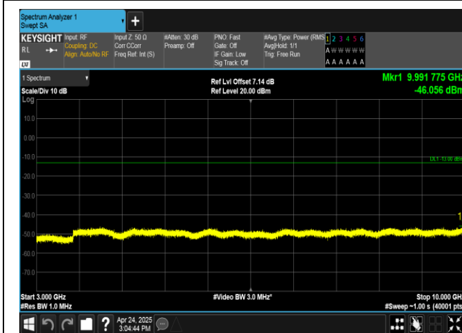
Band26(824-849)-15MHz-QPSK-26965-1RB#0-3000~10000-PASS
