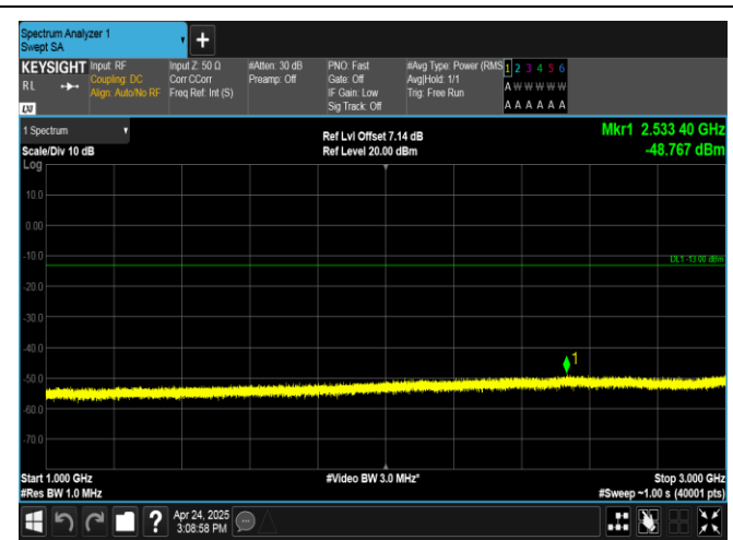
Band26(824-849)-15MHz-QPSK-26965-75RB#0-1000~3000-PASS
