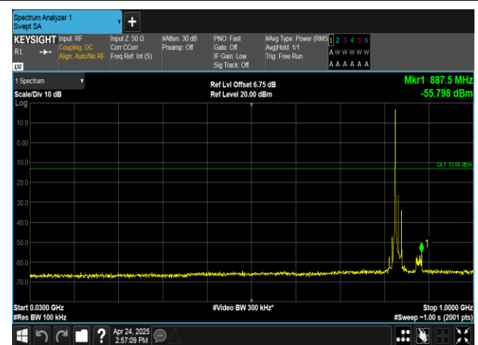
Band26(824-849)-15MHz-QPSK-26915-1RB#0-30~1000-PASS
