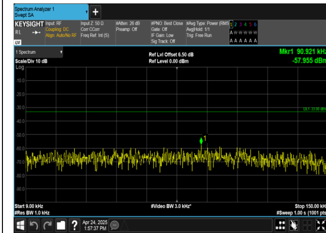
Band26(824-849)-10MHz-16QAM-26990-1RB#49-0.009-0.15-PASS
