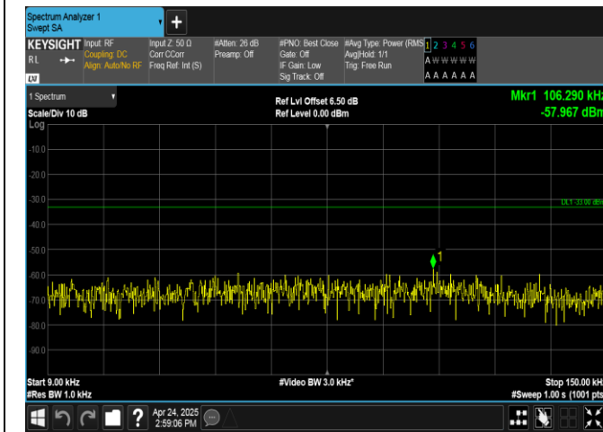
Band26(824-849)-15MHz-QPSK-26915-1RB#74-0.009~0.15-PASS
