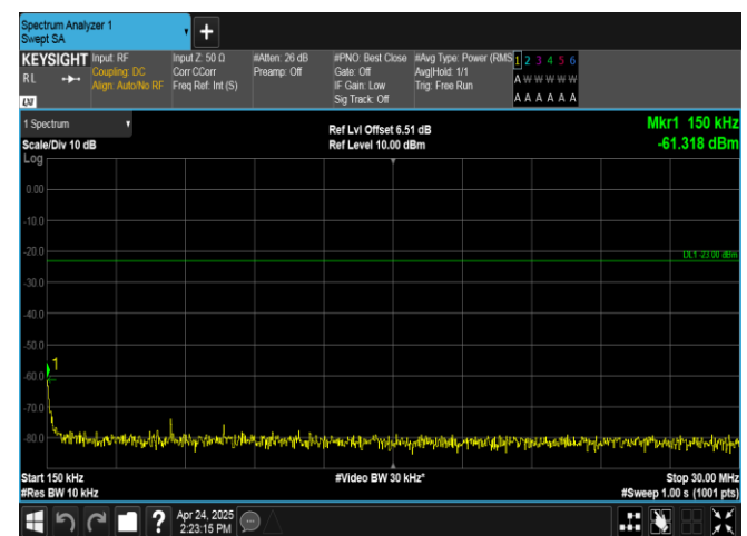
Band26(824-849)-15MHz-QPSK-26865-75RB#0-0.15~30-PASS
