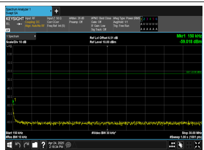
Band26(824-849)-15MHz-QPSK-26865-1RB#0-0.15~30-PASS
