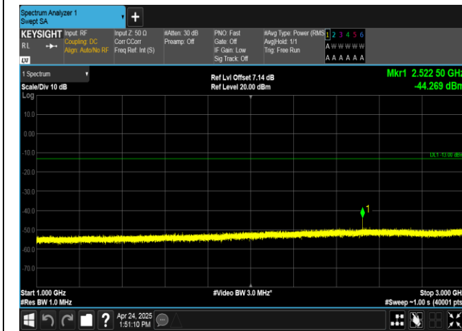
Band26(824-849)-10MHz-16QAM-26915-1RB#49-1000~3000-PASS
