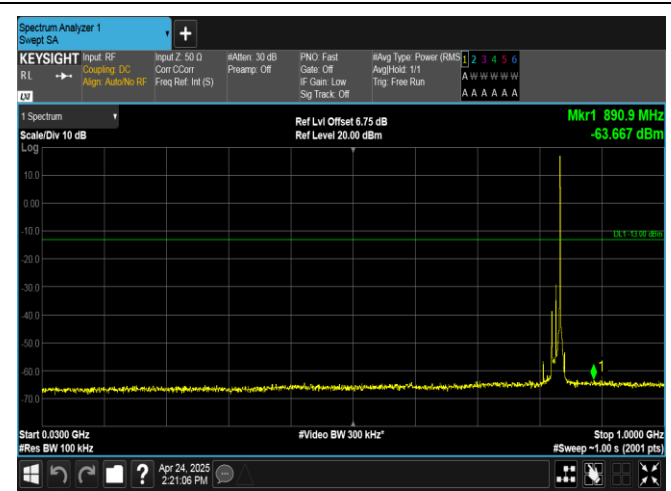
Band26(824-849)-15MHz-QPSK-26865-1RB#74-30~1000-PASS
