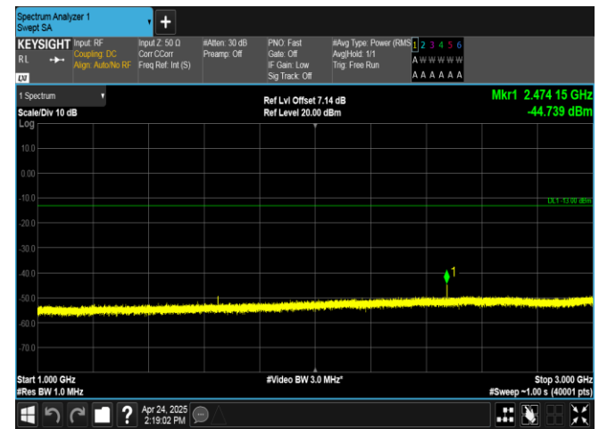
Band26(824-849)-15MHz-QPSK-26865-1RB#0-1000~3000-PASS
