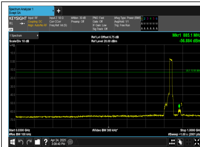
Band26(824-849)-15MHz-QPSK-26965-75RB#0-30~1000-PASS
