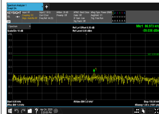
Band26(824-849)-15MHz-QPSK-26865-75RB#0-0.009~0.15-PASS
