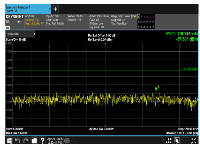
Band26(824-849)-15MHz-QPSK-26865-1RB#74-0.009~0.15-PASS
