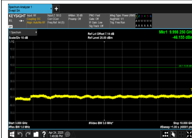
Band26(824-849)-10MHz-16QAM-26915-1RB#0-3000~10000-PASS
