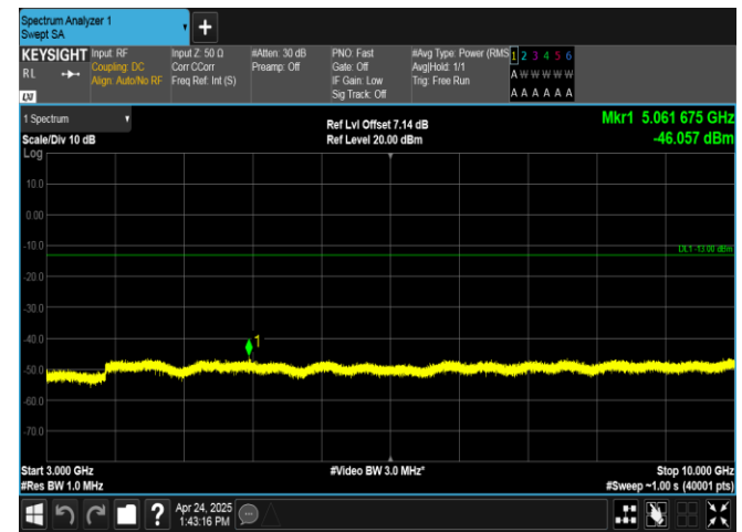
Band26(824-849)-10MHz-QPSK-26840-1RB#49-3000~10000-PASS
