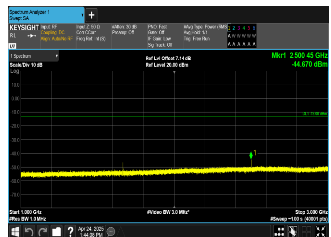
Band26(824-849)-10MHz-16QAM-26840-1RB#49-1000~3000-PASS
