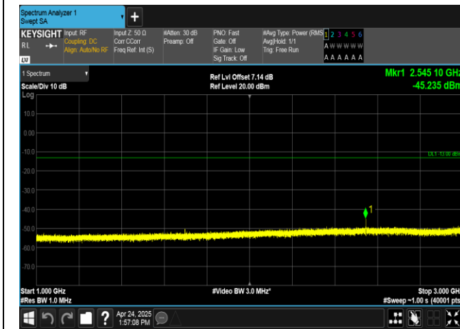
Band26(824-849)-10MHz-QPSK-26990-1RB#49-1000~3000-PASS
