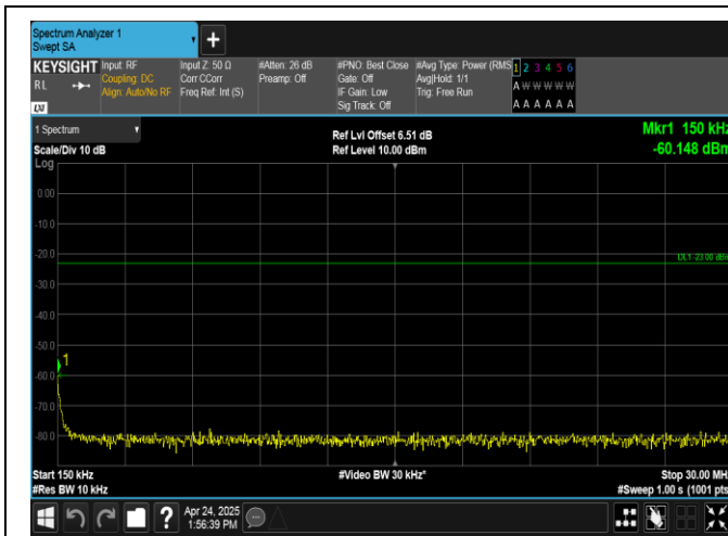
Band26(824-849)-10MHz-QPSK-26990-1RB#49-0.15~30-PASS
