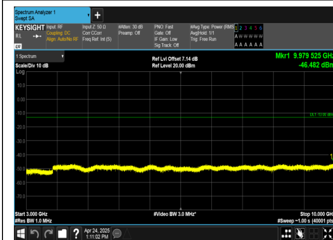
Band26(824-849)-5MHz-16QAM-26915-1RB#0-3000~10000-PASS
