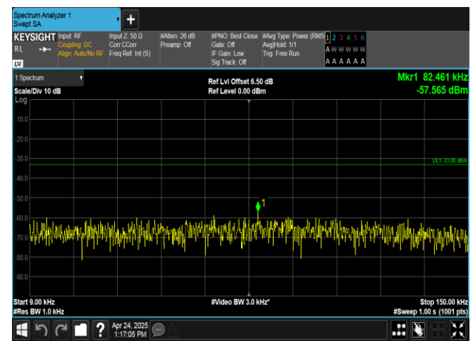
Band26(824-849)-5MHz-16QAM-27015-1RB#0-0.009~0.15-PASS
