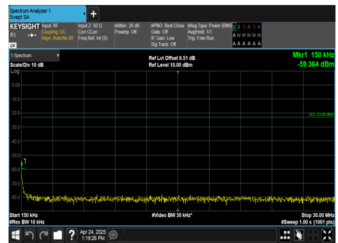
Band26(824-849)-5MHz-16QAM-27015-1RB#24-0.15~30-PASS
