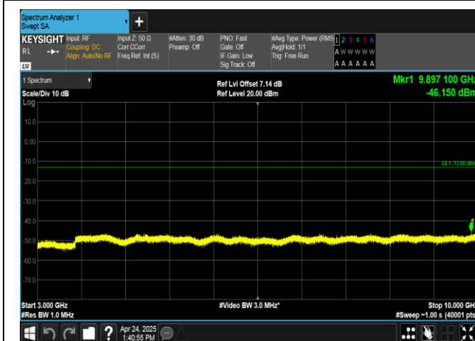
Band26(824-849)-10MHz-QPSK-26840-1RB#0-3000~10000-PASS
