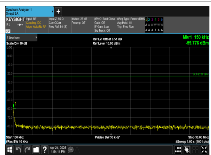
Band26(824-849)-10MHz-QPSK-26990-1RB#0-0.15~30-PASS
