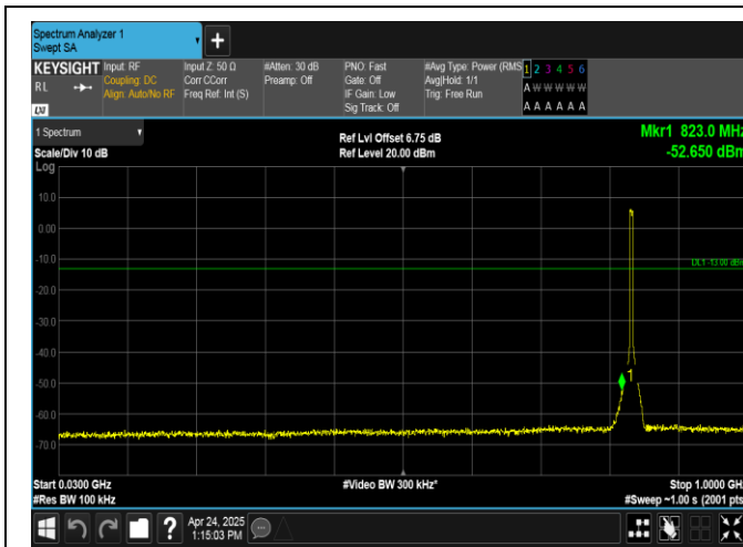
Band26(824-849)-5MHz-16QAM-26915-25RB#0-30~1000-PASS
