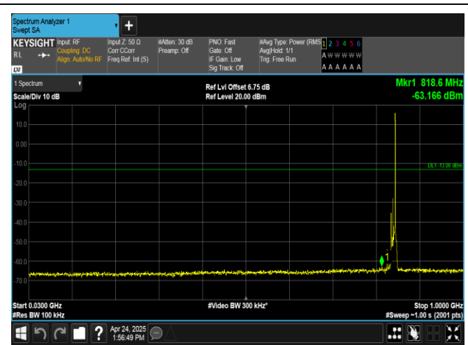
Band26(824-849)-10MHz-QPSK-26990-1RB#49-30~1000-PASS
