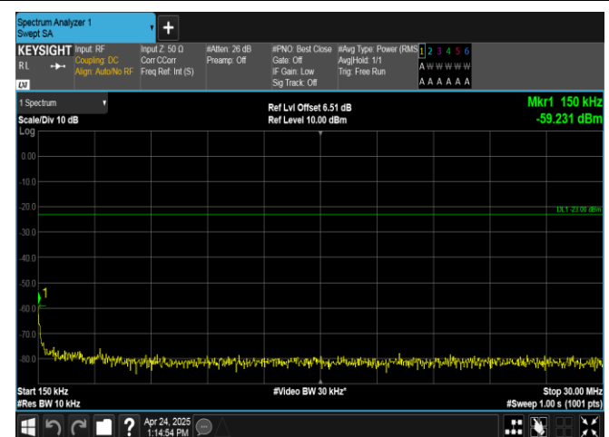
Band26(824-849)-5MHz-16QAM-26915-25RB#0-0.15~30-PASS
