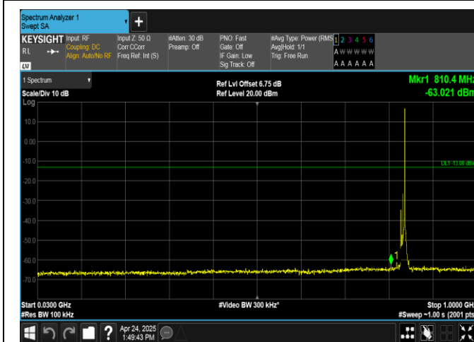
Band26(824-849)-10MHz-QPSK-26915-1RB#49-30~1000-PASS
