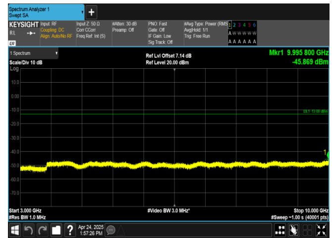
Band26(824-849)-10MHz-QPSK-26990-1RB#49-3000~10000-PASS
