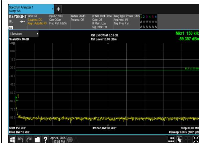
Band26(824-849)-10MHz-QPSK-26915-1RB#0-0.15~30-PASS
