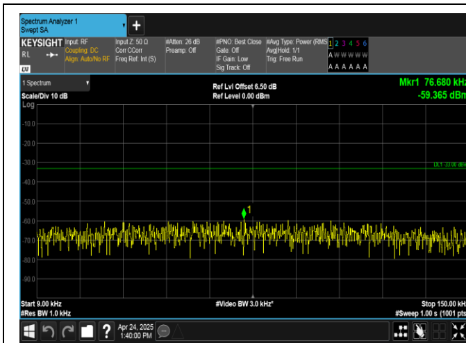
Band26(824-849)-10MHz-QPSK-26840-1RB#0-0.009~0.15-PASS
