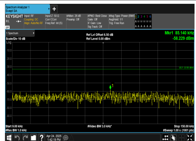
Band26(824-849)-10MHz-QPSK-26840-1RB#49-0.009~0.15-PASS
