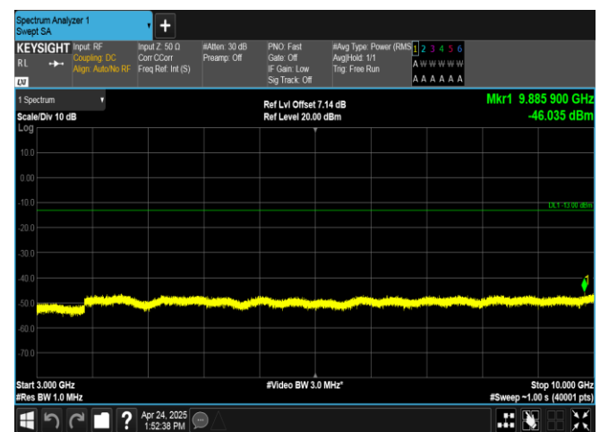
Band26(824-849)-10MHz-QPSK-26915-50RB#0-3000~10000-PASS
