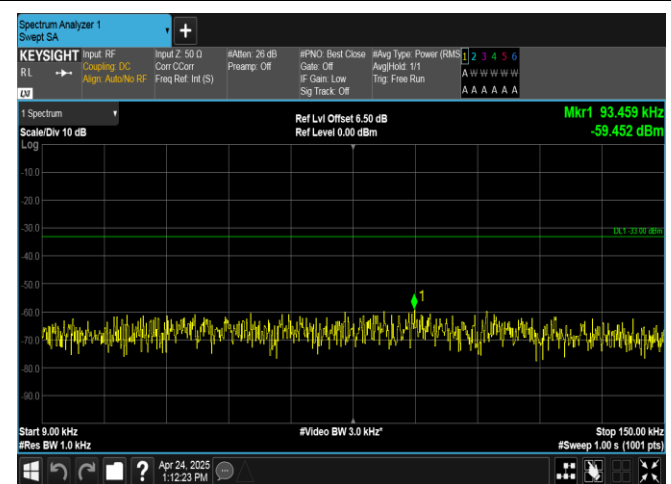
Band26(824-849)-5MHz-16QAM-26915-1RB#24-0.009~0.15-PASS
