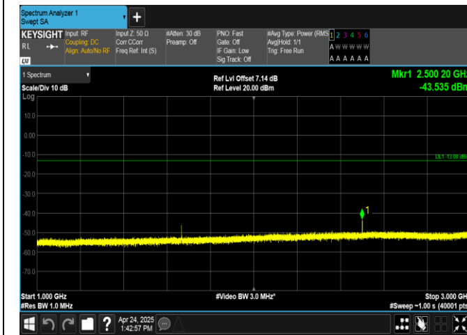
Band26(824-849)-10MHz-QPSK-26840-1RB#49-1000~3000-PASS
