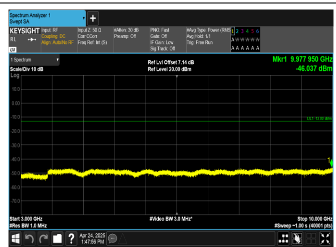
Band26(824-849)-10MHz-QPSK-26915-1RB#0-3000~10000-PASS
