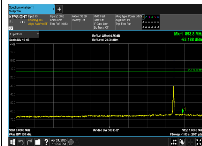
Band26(824-849)-5MHz-16QAM-27015-1RB#24-30~1000-PASS
