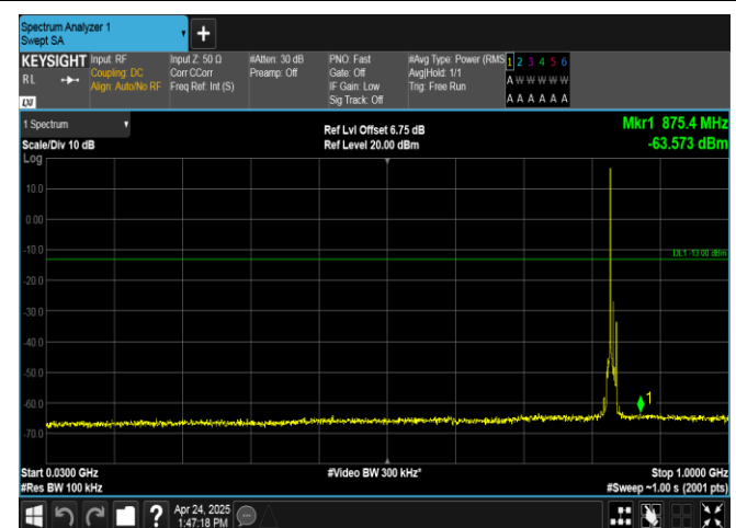
Band26(824-849)-10MHz-QPSK-26915-1RB#0-30~1000-PASS
