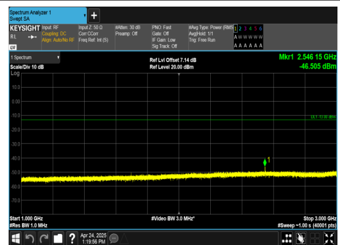
Band26(824-849)-5MHz-16QAM-27015-1RB#24-1000~3000-PASS
