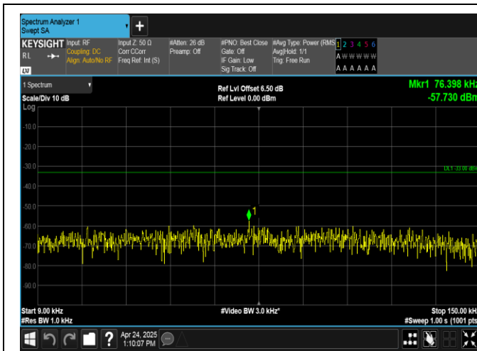
Band26(824-849)-5MHz-16QAM-26915-1RB#0-0.009~0.15-PASS
