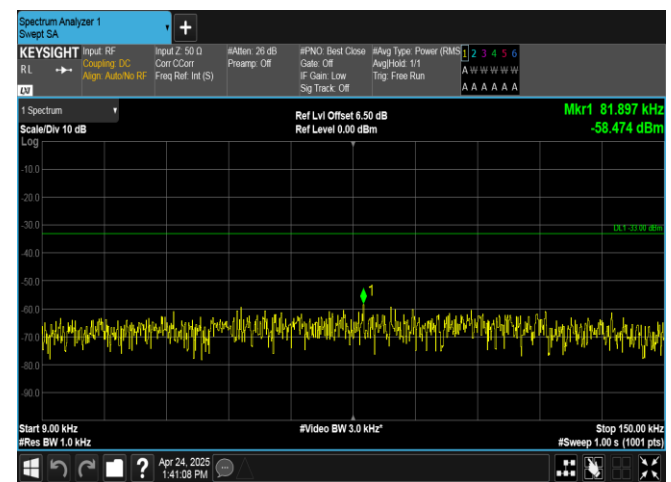
Band26(824-849)-10MHz-16QAM-26840-1RB#0-0.009~0.15-PASS
