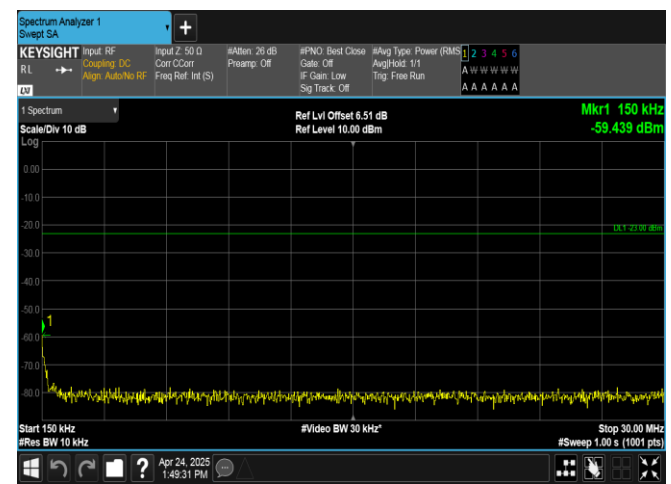
Band26(824-849)-10MHz-QPSK-26915-1RB#49-0.15~30-PASS
