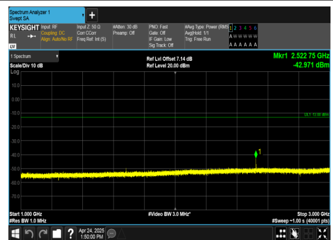
Band26(824-849)-10MHz-QPSK-26915-1RB#49-1000~3000-PASS
