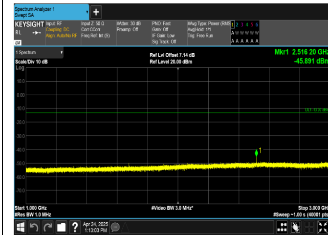
Band26(824-849)-5MHz-16QAM-26915-1RB#24-1000~3000-PASS
