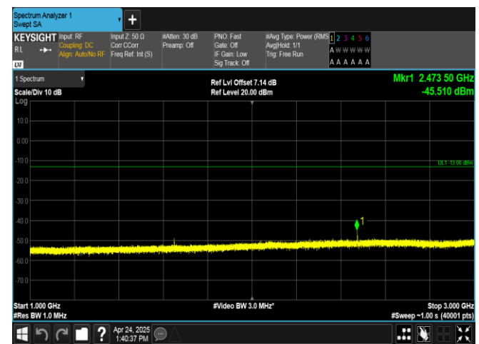
Band26(824-849)-10MHz-QPSK-26840-1RB#0-1000~3000-PASS
