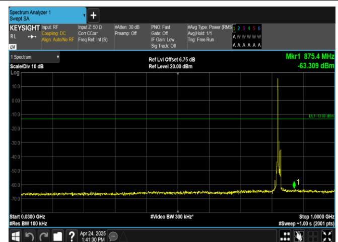
Band26(824-849)-10MHz-16QAM-26840-1RB#0-30~1000-PASS
