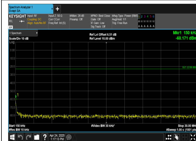
Band26(824-849)-5MHz-16QAM-27015-1RB#0-0.15~30-PASS
