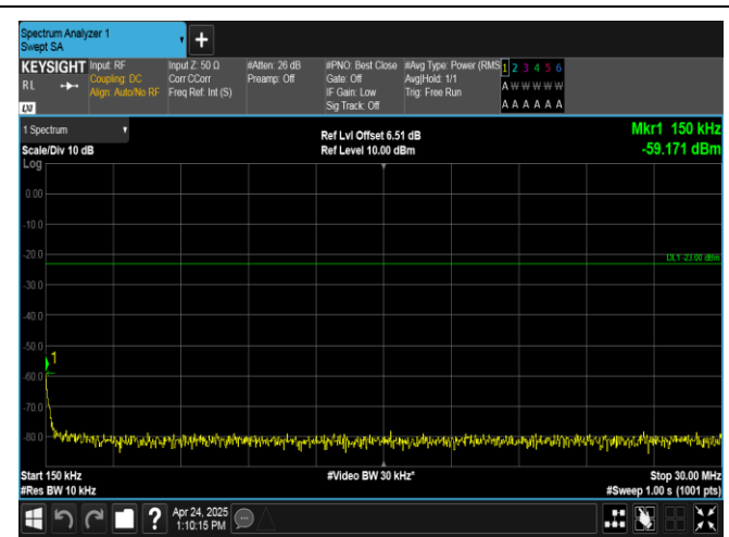
Band26(824-849)-5MHz-16QAM-26915-1RB#0-0.15~30-PASS
