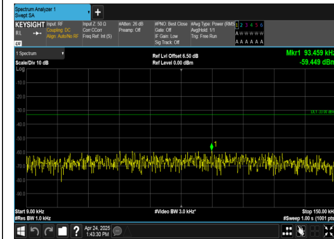
Band26(824-849)-10MHz-16QAM-26840-1RB#49-0.009~0.15-PASS
