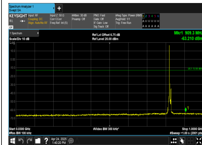
Band26(824-849)-10MHz-QPSK-26840-1RB#0-30~1000-PASS
