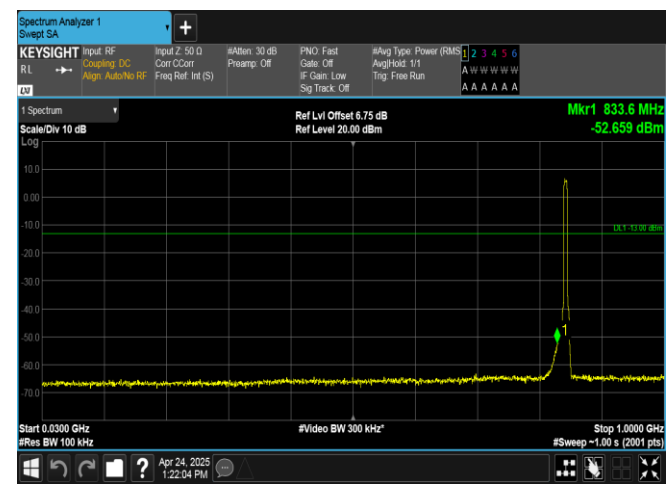
Band26(824-849)-5MHz-16QAM-27015-25RB#0-30~1000-PASS
