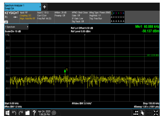
Band26(824-849)-10MHz-QPSK-26990-1RB#49-0.009~0.15-PASS
