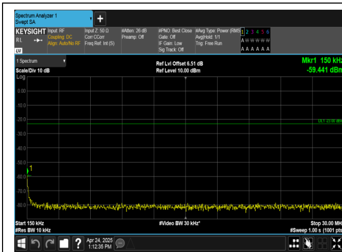
Band26(824-849)-5MHz-16QAM-26915-1RB#24-0.15~30-PASS
