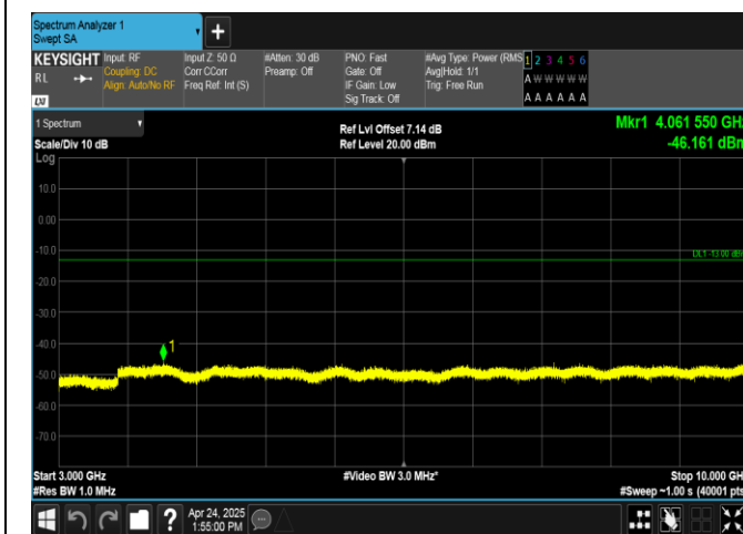
Band26(824-849)-10MHz-QPSK-26990-1RB#0-3000~10000-PASS
