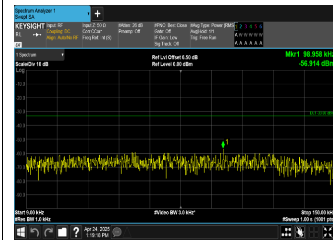
Band26(824-849)-5MHz-16QAM-27015-1RB#24-0.009~0.15-PASS
