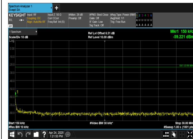
Band26(824-849)-5MHz-16QAM-27015-25RB#0-0.15~30-PASS
