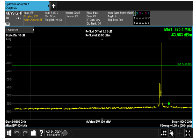
Band26(824-849)-10MHz-QPSK-26840-1RB#49-30~1000-PASS
