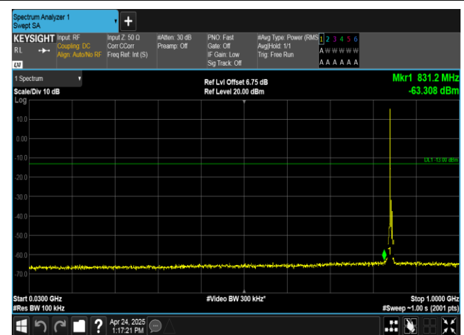
Band26(824-849)-5MHz-16QAM-27015-1RB#0-30~1000-PASS
