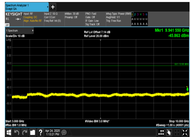
Band26(824-849)-5MHz-16QAM-26915-1RB#24-3000~10000-PASS
