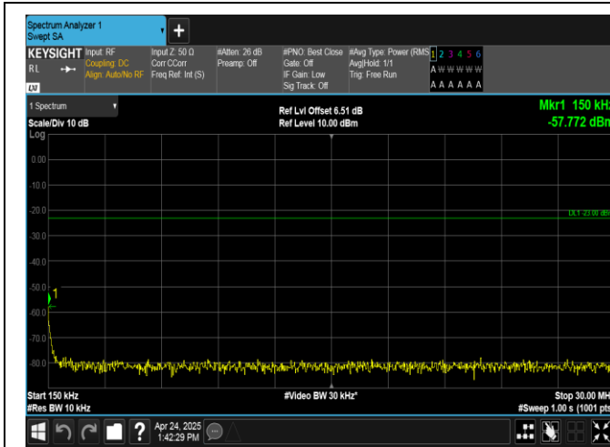
Band26(824-849)-10MHz-QPSK-26840-1RB#49-0.15~30-PASS
