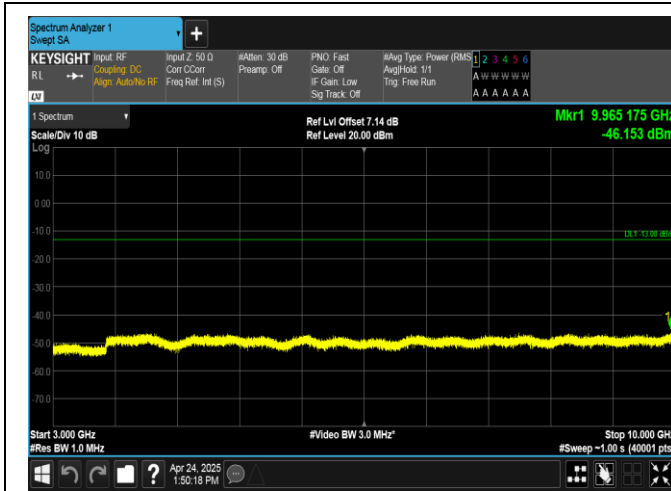
Band26(824-849)-10MHz-QPSK-26915-1RB#49-3000~10000-PASS
