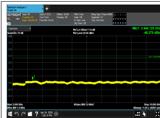
Band26(824-849)-5MHz-16QAM-27015-1RB#24-3000~10000-PASS
