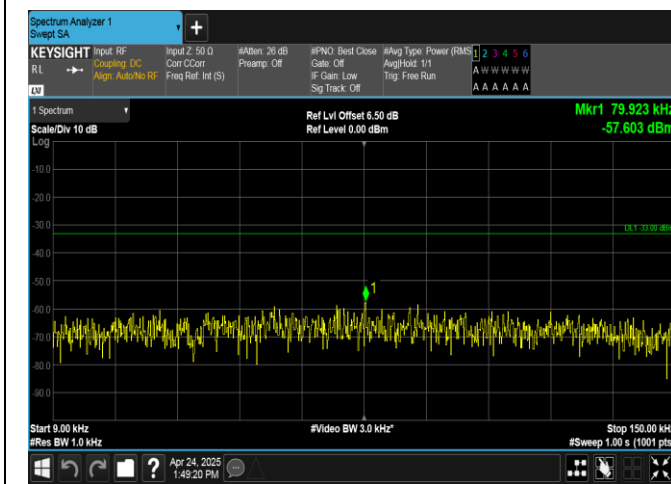
Band26(824-849)-10MHz-QPSK-26915-1RB#49-0.009~0.15-PASS
