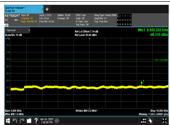
Band26(824-849)-10MHz-16QAM-26840-1RB#0-3000~10000-PASS
