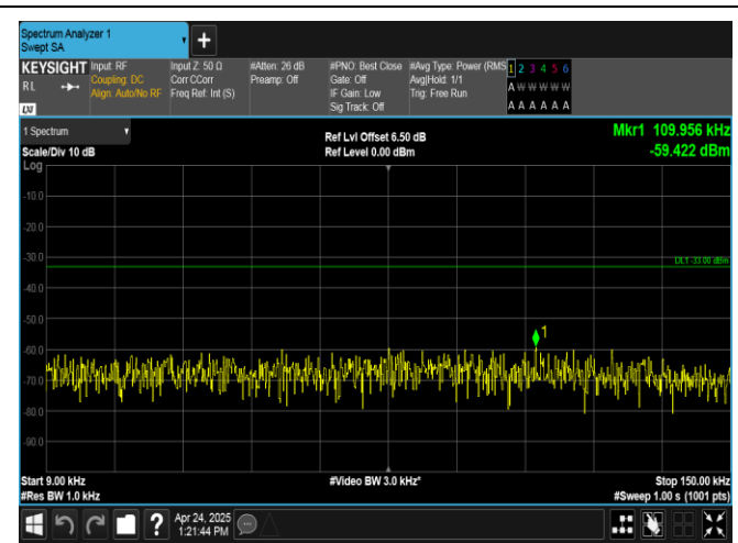
Band26(824-849)-5MHz-16QAM-27015-25RB#0-0.009~0.15-PASS
