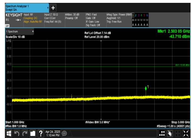
Band26(824-849)-5MHz-16QAM-26915-1RB#0-1000~3000-PASS
