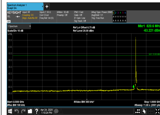
Band26(824-849)-5MHz-16QAM-26915-1RB#0-30~1000-PASS
