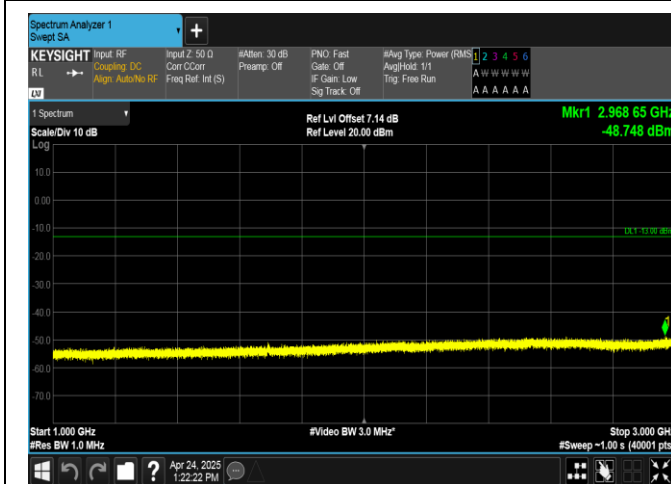
Band26(824-849)-5MHz-16QAM-27015-25RB#0-1000~3000-PASS
