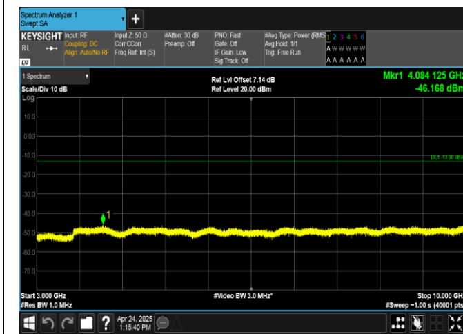
Band26(824-849)-5MHz-16QAM-26915-25RB#0-3000~10000-PASS
