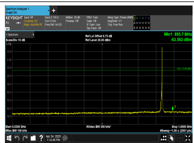
Band26(824-849)-5MHz-16QAM-26915-1RB#24-30~1000-PASS
