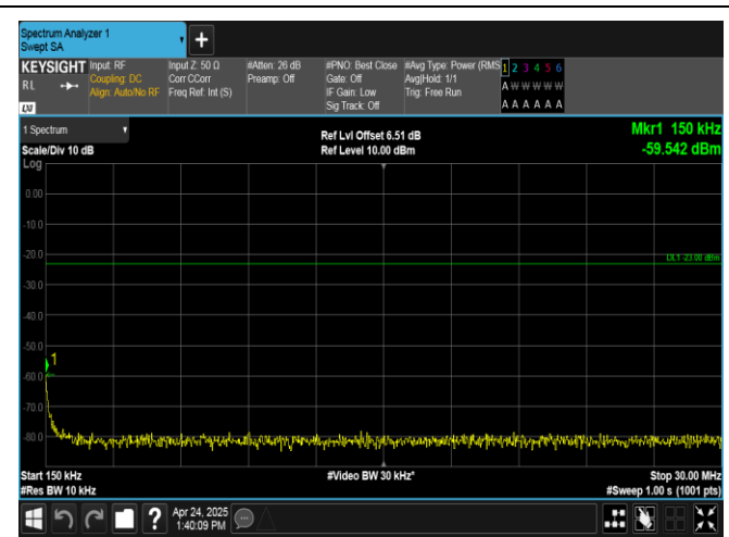
Band26(824-849)-10MHz-QPSK-26840-1RB#0-0.15~30-PASS
