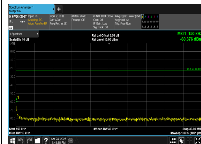
Band26(824-849)-10MHz-16QAM-26840-1RB#0-0.15~30-PASS
