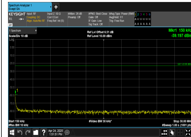
Band26(824-849)-10MHz-QPSK-26915-50RB#0-0.15~30-PASS
