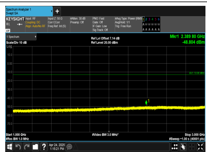
Band26(824-849)-5MHz-16QAM-26915-25RB#0-1000~3000-PASS
