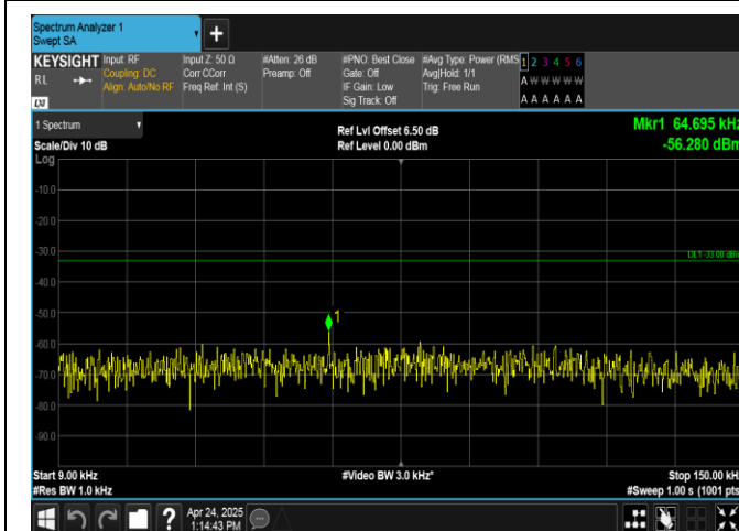
Band26(824-849)-5MHz-16QAM-26915-25RB#0-0.009~0.15-PASS
