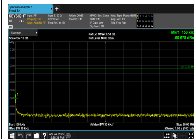
Band26(824-849)-3MHz-16QAM-27025-1RB#0-0.15~30-PASS
