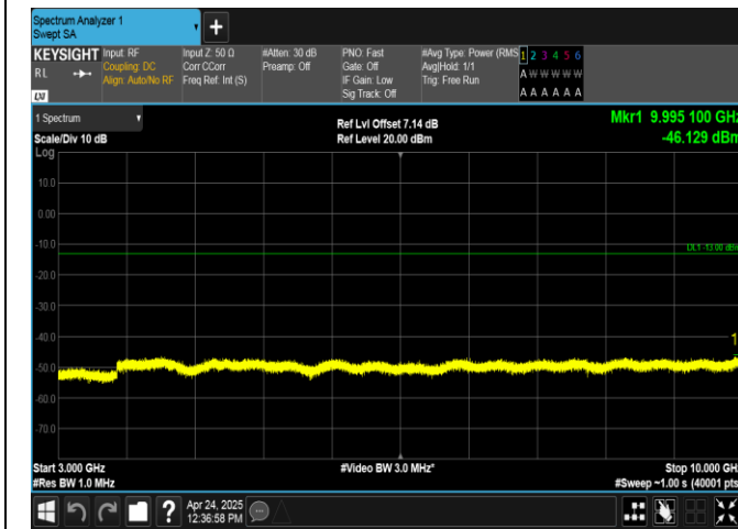
Band26(824-849)-3MHz-16QAM-26915-15RB#0-3000~10000-PASS
