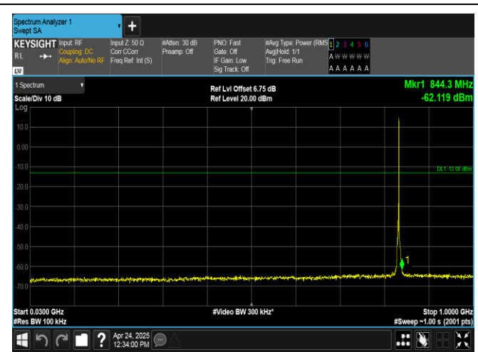
Band26(824-849)-3MHz-16QAM-26915-1RB#14-30~1000-PASS
