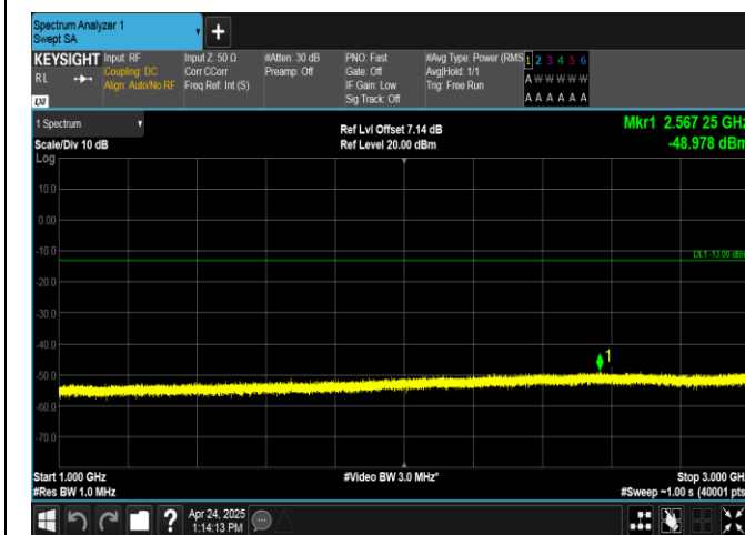
Band26(824-849)-5MHz-QPSK-26915-25RB#0-1000~3000-PASS
