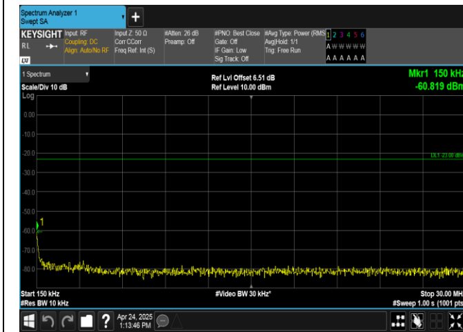
Band26(824-849)-5MHz-QPSK-26915-25RB#0-0.15~30-PASS
