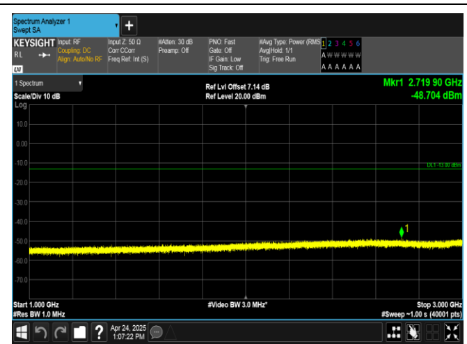
Band26(824-849)-5MHz-QPSK-26815-25RB#0-1000~3000-PASS
