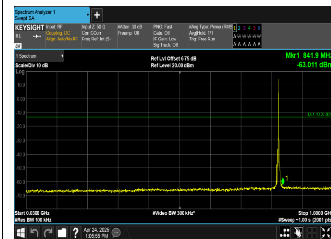
Band26(824-849)-5MHz-16QAM-26815-1RB#24-30~1000-PASS
