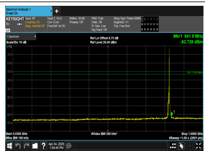
Band26(824-849)-5MHz-QPSK-26815-1RB#24-30~1000-PASS
