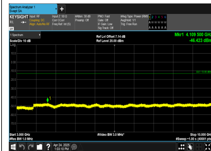
Band26(824-849)-5MHz-QPSK-26815-1RB#0-3000~10000-PASS
