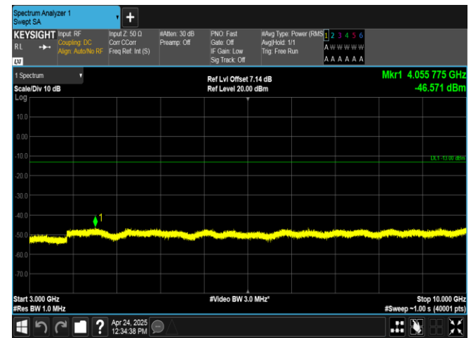
Band26(824-849)-3MHz-16QAM-26915-1RB#14-3000~10000-PASS
