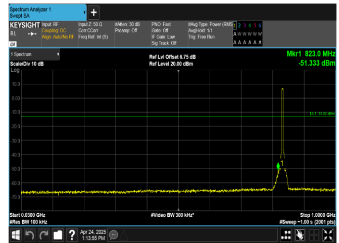
Band26(824-849)-5MHz-QPSK-26915-25RB#0-30~1000-PASS
