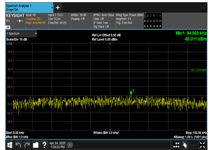
Band26(824-849)-5MHz-16QAM-26815-1RB#0-0.009~0.15-PASS
