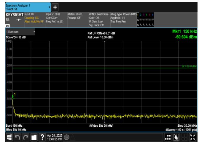
Band26(824-849)-3MHz-16QAM-27025-1RB#14-0.15~30-PASS
