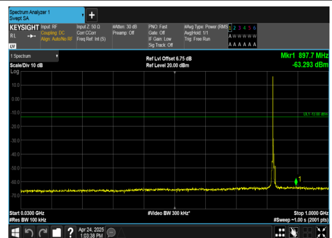
Band26(824-849)-5MHz-16QAM-26815-1RB#0-30~1000-PASS
