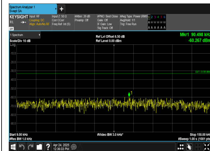
Band26(824-849)-3MHz-16QAM-26915-15RB#0-0.009~0.15-PASS
