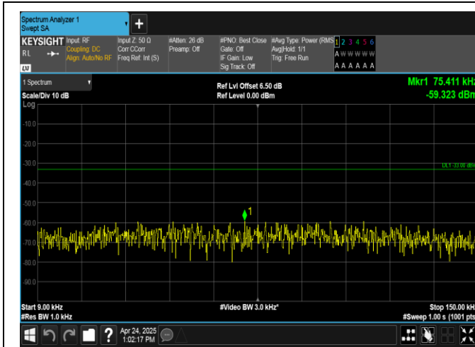
Band26(824-849)-5MHz-QPSK-26815-1RB#0-0.009~0.15-PASS
