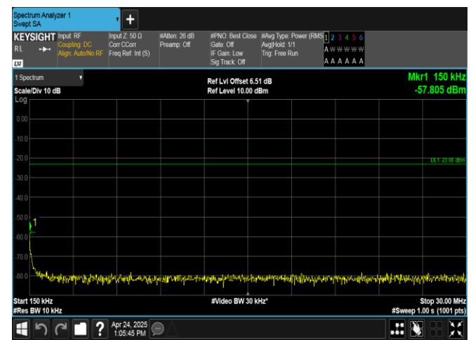
Band26(824-849)-5MHz-16QAM-26815-1RB#24-0.15~30-PASS
