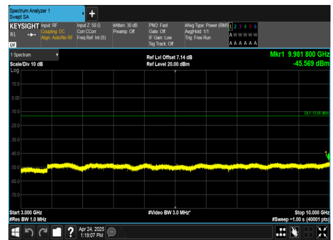
Band26(824-849)-5MHz-QPSK-27015-1RB#24-3000~10000-PASS
