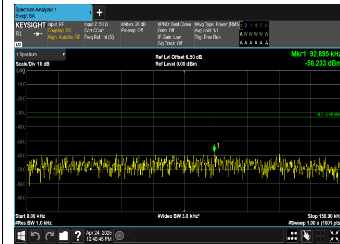
Band26(824-849)-3MHz-16QAM-27025-1RB#14-0.009~0.15-PASS
