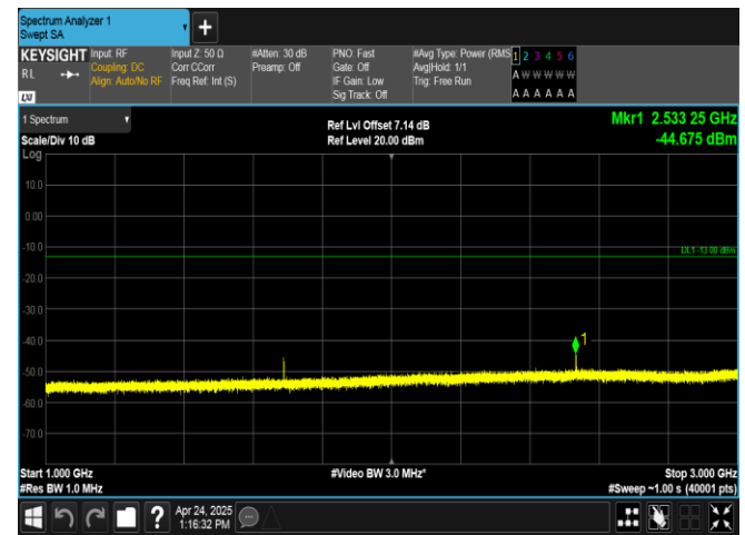
Band26(824-849)-5MHz-QPSK-27015-1RB#0-1000~3000-PASS
