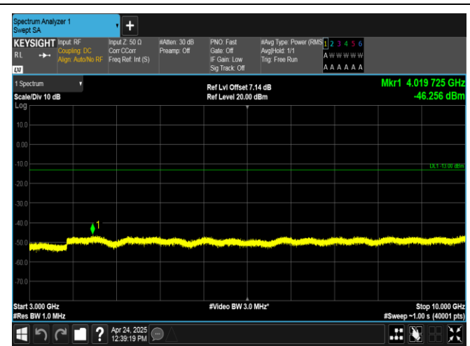
Band26(824-849)-3MHz-16QAM-27025-1RB#0-3000~10000-PASS
