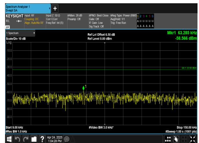
Band26(824-849)-5MHz-QPSK-26815-1RB#24-0.009~0.15-PASS
