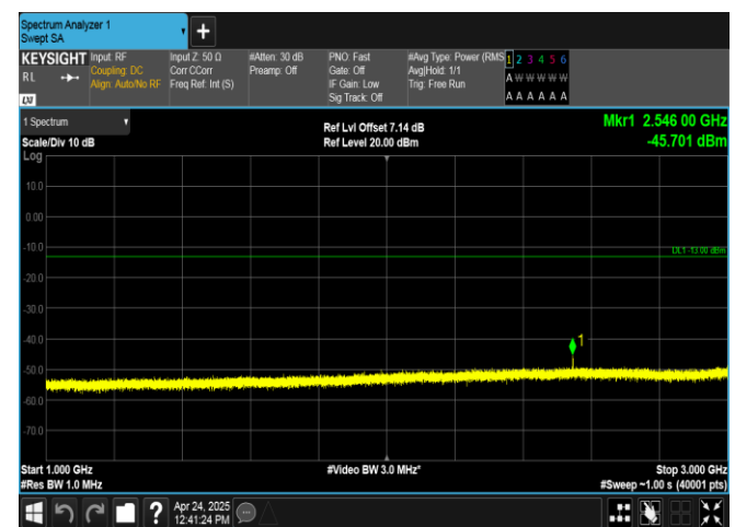
Band26(824-849)-3MHz-16QAM-27025-1RB#14-1000~3000-PASS
