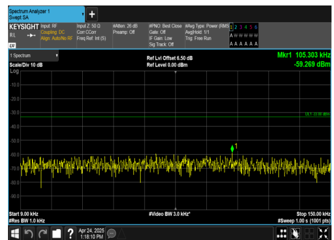
Band26(824-849)-5MHz-QPSK-27015-1RB#24-0.009~0.15-PASS
