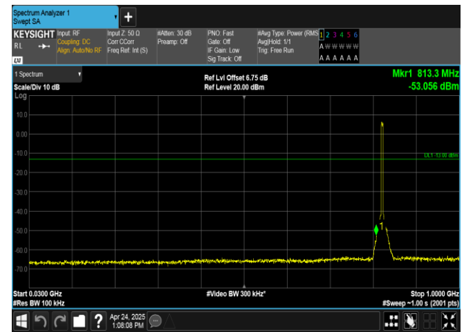
Band26(824-849)-5MHz-16QAM-26815-25RB#0-30~1000-PASS
