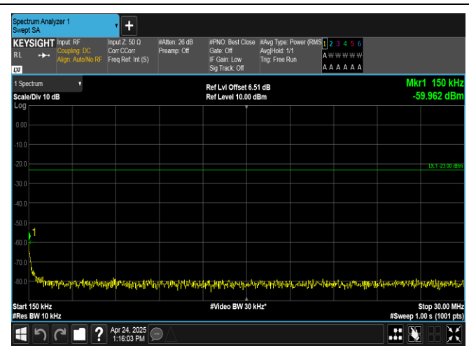
Band26(824-849)-5MHz-QPSK-27015-1RB#0-0.15~30-PASS
