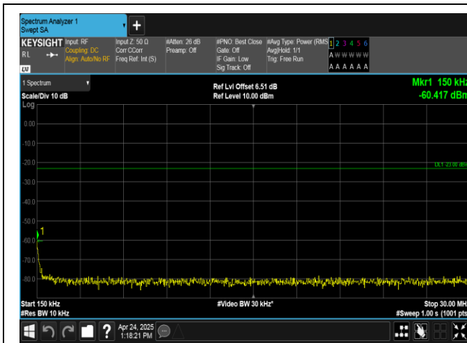
Band26(824-849)-5MHz-QPSK-27015-1RB#24-0.15~30-PASS
