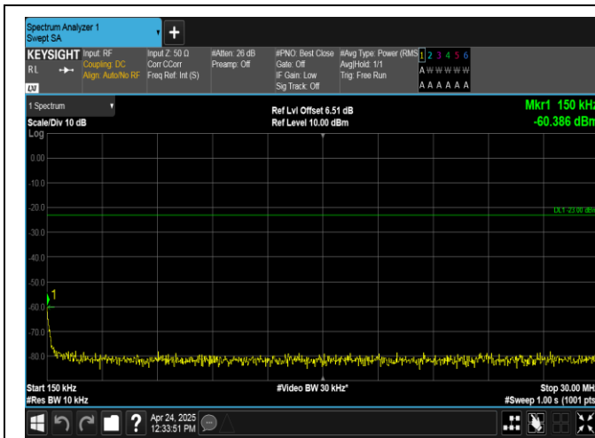
Band26(824-849)-3MHz-16QAM-26915-1RB#14-0.15~30-PASS
