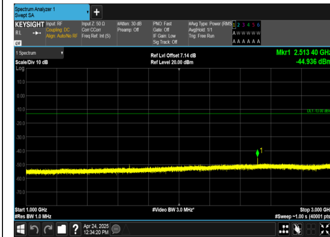
Band26(824-849)-3MHz-16QAM-26915-1RB#14-1000~3000-PASS
