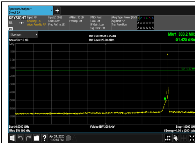
Band26(824-849)-5MHz-QPSK-27015-25RB#0-30~1000-PASS
