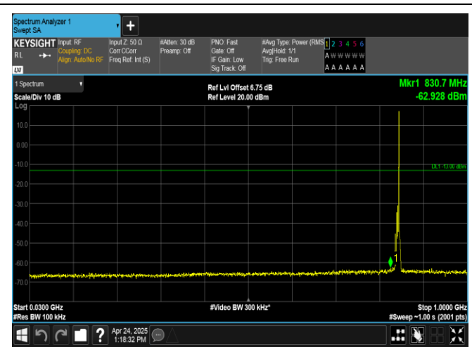
Band26(824-849)-5MHz-QPSK-27015-1RB#24-30~1000-PASS
