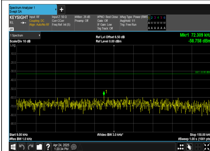
Band26(824-849)-5MHz-QPSK-27015-25RB#0-0.009~0.15-PASS
