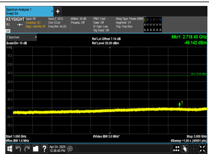
Band26(824-849)-3MHz-16QAM-26915-15RB#0-1000~3000-PASS
