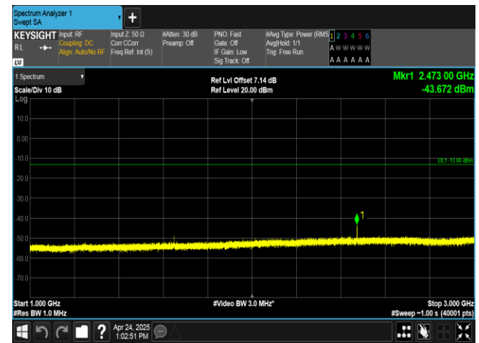
Band26(824-849)-5MHz-QPSK-26815-1RB#0-1000~3000-PASS
