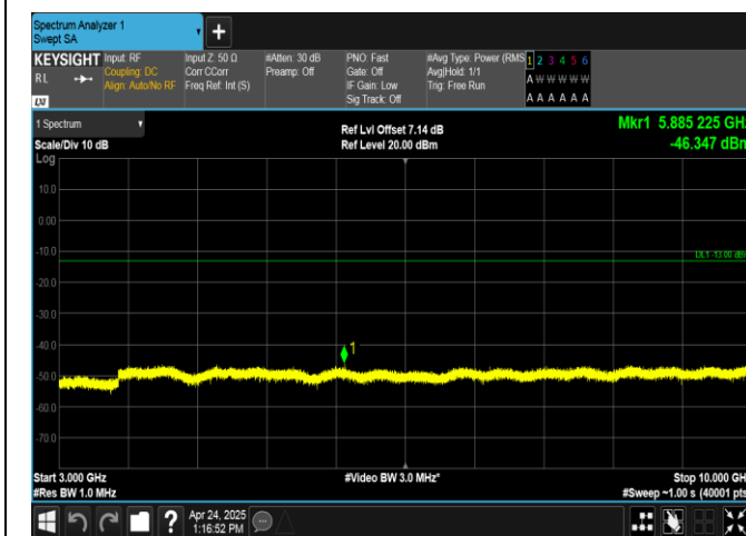
Band26(824-849)-5MHz-QPSK-27015-1RB#0-3000~10000-PASS
