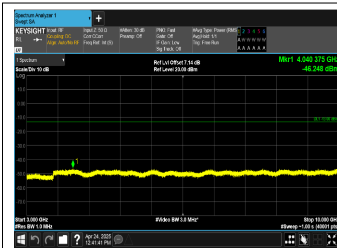
Band26(824-849)-3MHz-16QAM-27025-1RB#14-3000~10000-PASS
