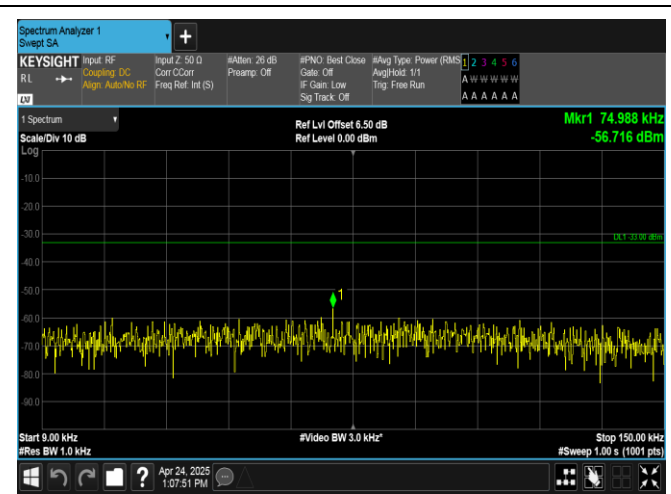
Band26(824-849)-5MHz-16QAM-26815-25RB#0-0.009~0.15-PASS
