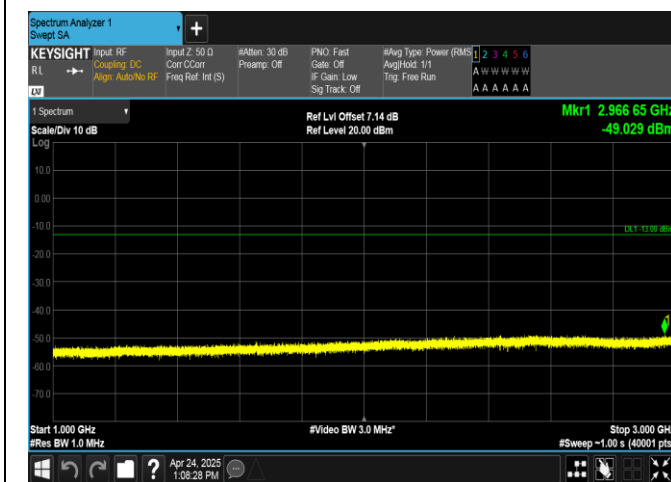
Band26(824-849)-5MHz-16QAM-26815-25RB#0-1000~3000-PASS
