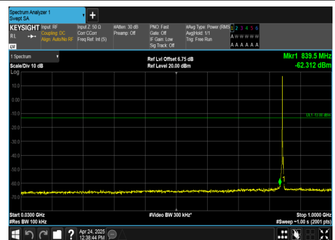
Band26(824-849)-3MHz-16QAM-27025-1RB#0-30~1000-PASS
