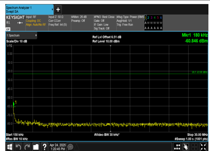
Band26(824-849)-5MHz-QPSK-27015-25RB#0-0.15~30-PASS
