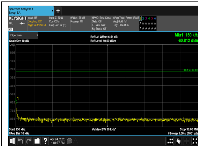
Band26(824-849)-5MHz-QPSK-26815-1RB#24-0.15~30-PASS
