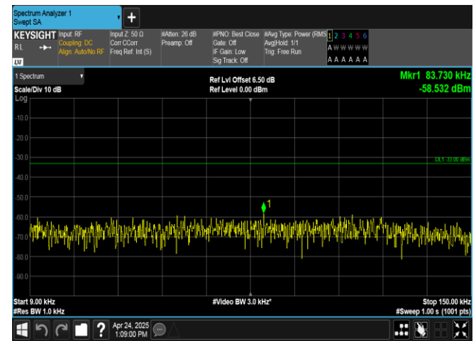
Band26(824-849)-5MHz-QPSK-26915-1RB#0-0.009~0.15-PASS
