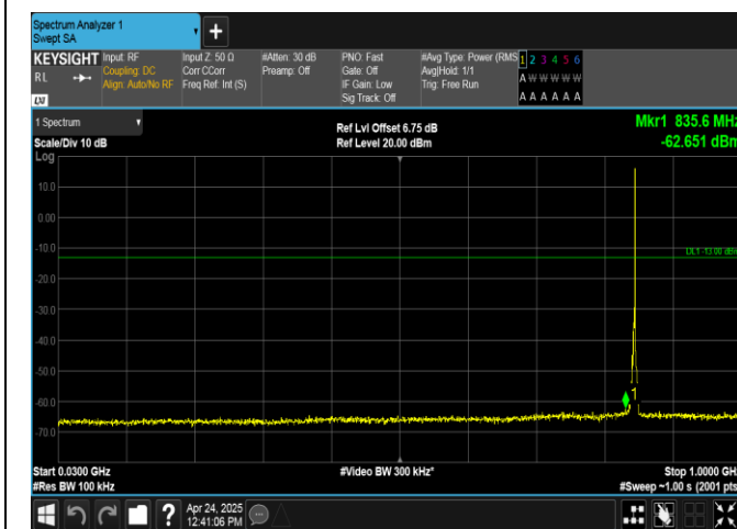
Band26(824-849)-3MHz-16QAM-27025-1RB#14-30~1000-PASS
