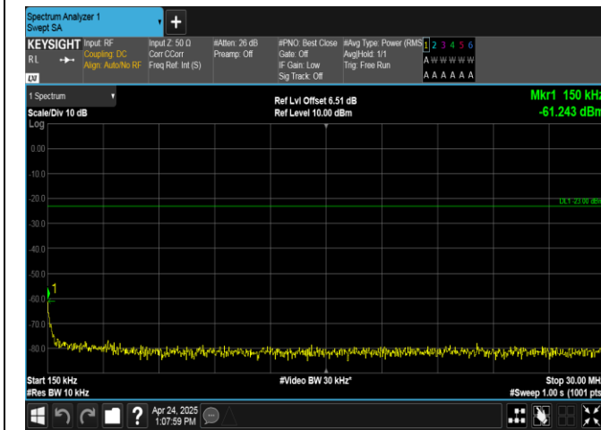
Band26(824-849)-5MHz-16QAM-26815-25RB#0-0.15~30-PASS
