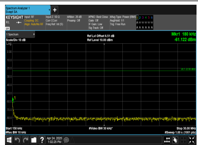
Band26(824-849)-5MHz-QPSK-26815-1RB#0-0.15~30-PASS
