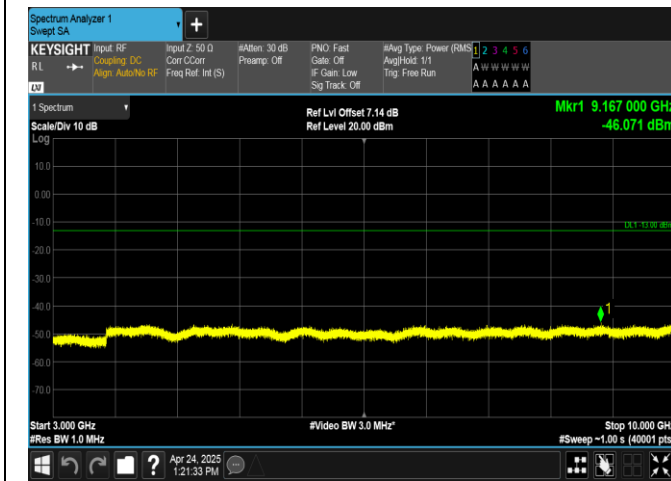
Band26(824-849)-5MHz-QPSK-27015-25RB#0-3000~10000-PASS
