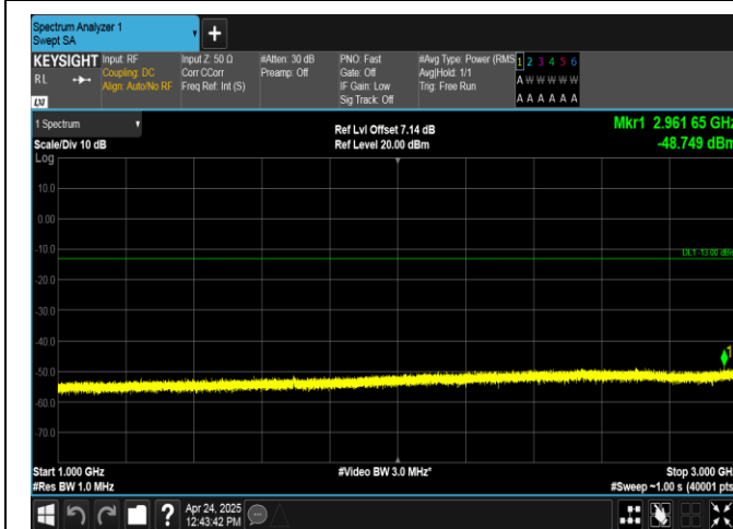
Band26(824-849)-3MHz-16QAM-27025-15RB#0-1000~3000-PASS
