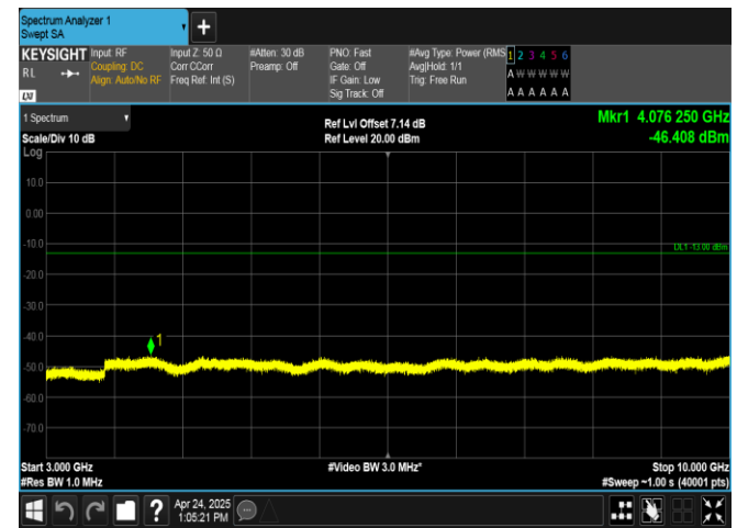
Band26(824-849)-5MHz-QPSK-26815-1RB#24-3000~10000-PASS
