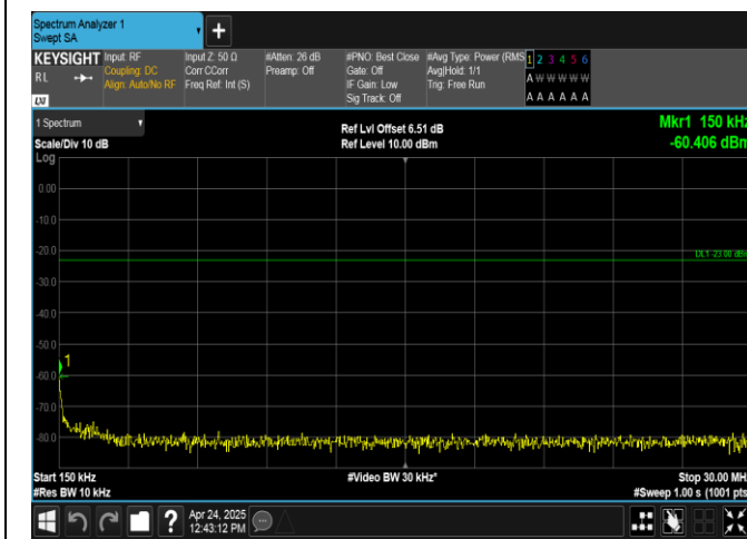
Band26(824-849)-3MHz-16QAM-27025-15RB#0-0.15~30-PASS
