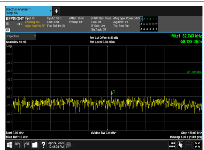
Band26(824-849)-3MHz-16QAM-27025-15RB#0-0.009~0.15-PASS
