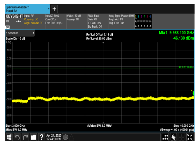
Band26(824-849)-3MHz-16QAM-27025-15RB#0-3000~10000-PASS
