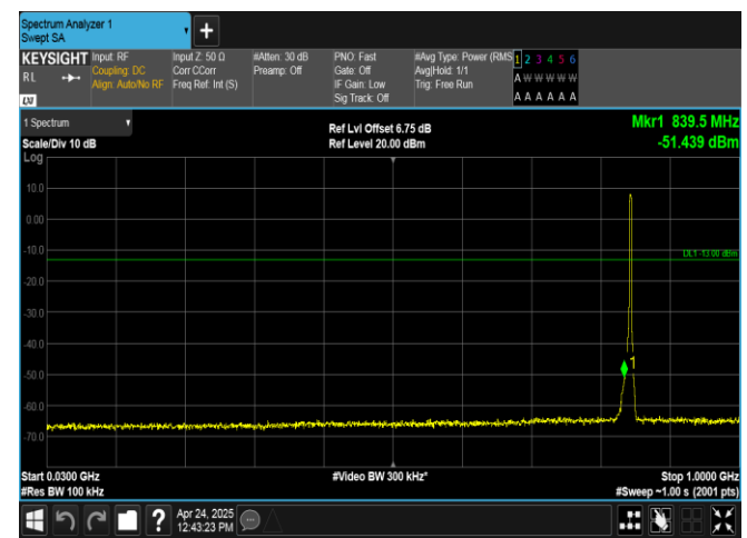
Band26(824-849)-3MHz-16QAM-27025-15RB#0-30~1000-PASS
