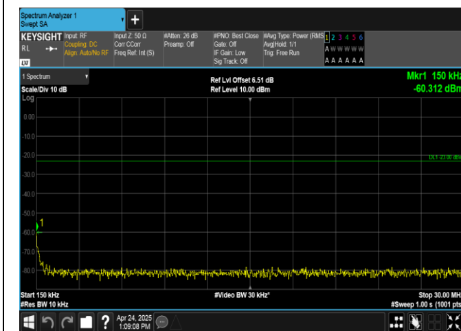
Band26(824-849)-5MHz-QPSK-26915-1RB#0-0.15~30-PASS
