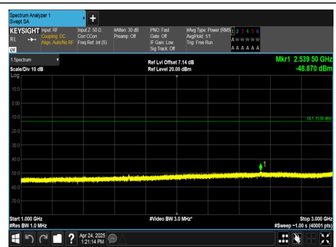
Band26(824-849)-5MHz-QPSK-27015-25RB#0-1000~3000-PASS
