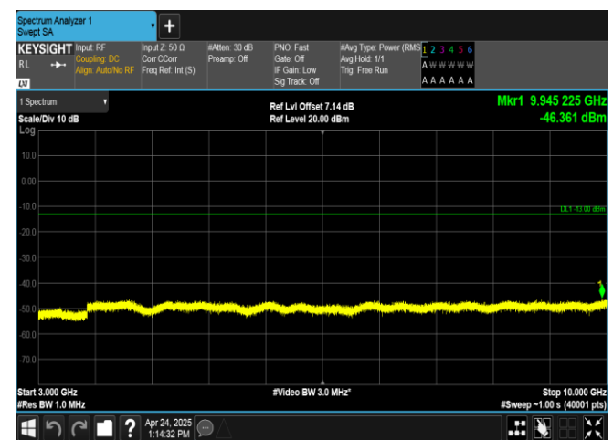
Band26(824-849)-5MHz-QPSK-26915-25RB#0-3000~10000-PASS
