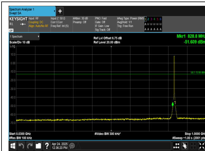
Band26(824-849)-3MHz-16QAM-26915-15RB#0-30~1000-PASS
