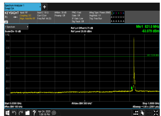
Band26(824-849)-5MHz-QPSK-26915-1RB#0-30~1000-PASS
