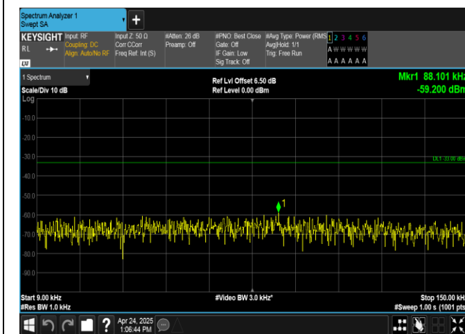
Band26(824-849)-5MHz-QPSK-26815-25RB#0-0.009~0.15-PASS
