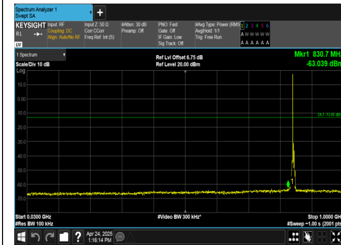
Band26(824-849)-5MHz-QPSK-27015-1RB#0-30~1000-PASS
