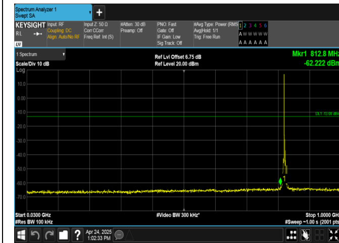
Band26(824-849)-5MHz-QPSK-26815-1RB#0-30~1000-PASS
