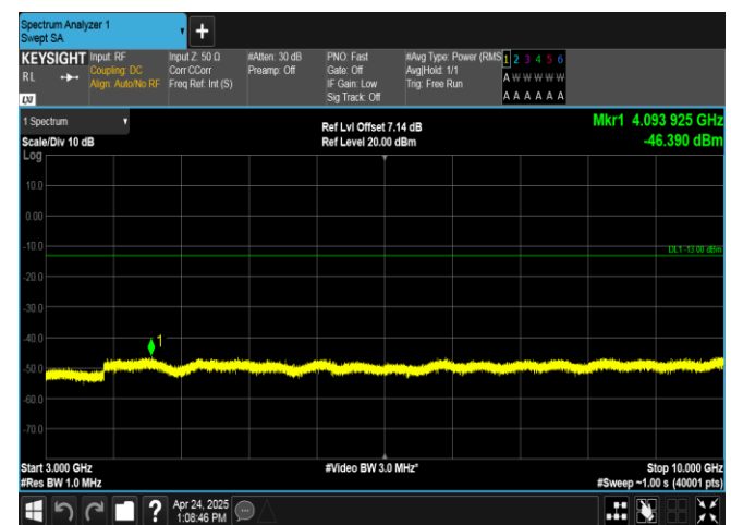
Band26(824-849)-5MHz-16QAM-26815-25RB#0-3000~10000-PASS
