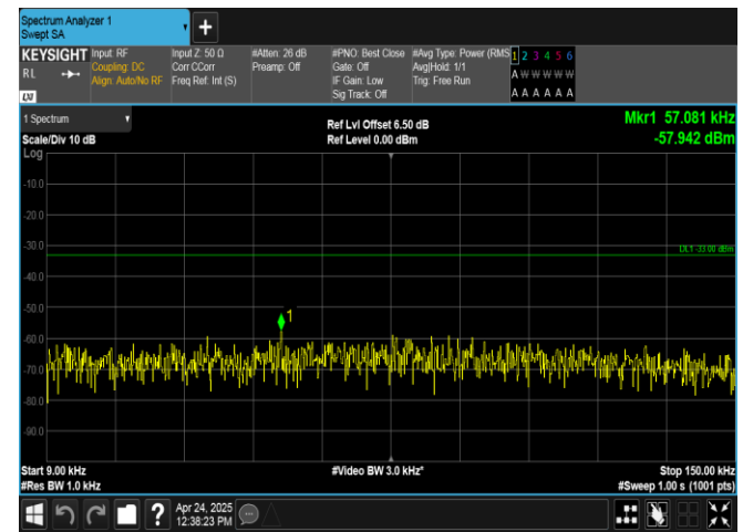
Band26(824-849)-3MHz-16QAM-27025-1RB#0-0.009~0.15-PASS
