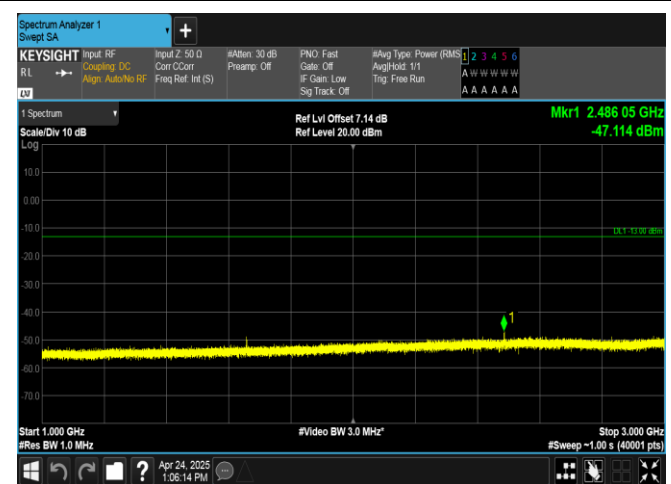
Band26(824-849)-5MHz-16QAM-26815-1RB#24-1000~3000-PASS
