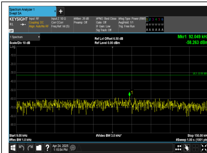
Band26(824-849)-5MHz-QPSK-27015-1RB#0-0.009~0.15-PASS
