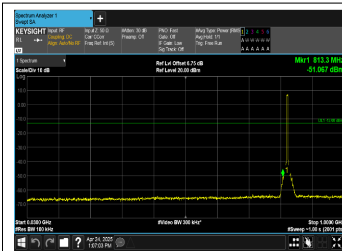
Band26(824-849)-5MHz-QPSK-26815-25RB#0-30~1000-PASS
