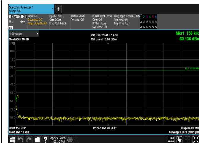
Band26(824-849)-5MHz-16QAM-26815-1RB#0-0.15~30-PASS
