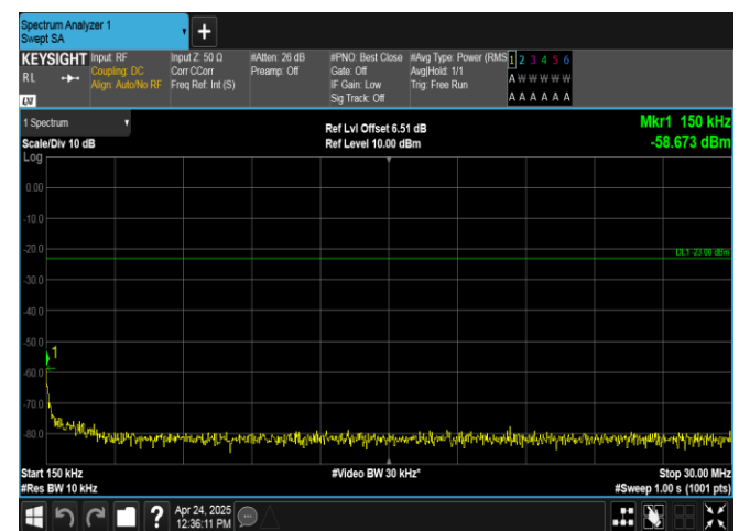
Band26(824-849)-3MHz-16QAM-26915-15RB#0-0.15~30-PASS
