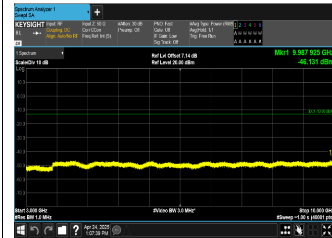
Band26(824-849)-5MHz-QPSK-26815-25RB#0-3000~10000-PASS
