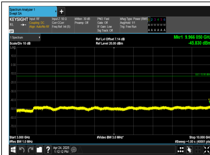
Band26(824-849)-5MHz-QPSK-26915-1RB#24-3000~10000-PASS
