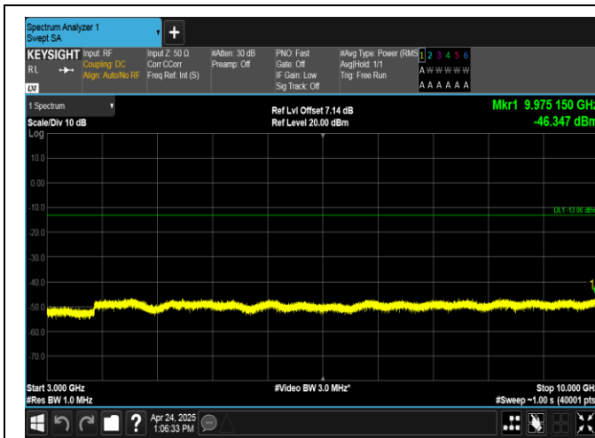
Band26(824-849)-5MHz-16QAM-26815-1RB#24-3000~10000-PASS
