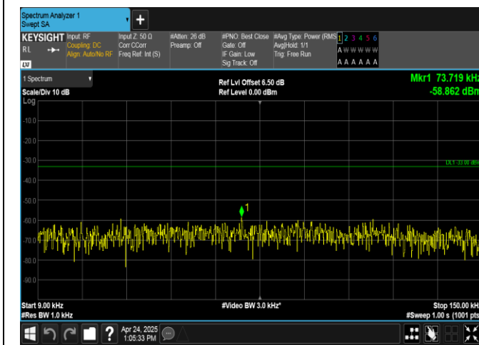
Band26(824-849)-5MHz-16QAM-26815-1RB#24-0.009~0.15-PASS
