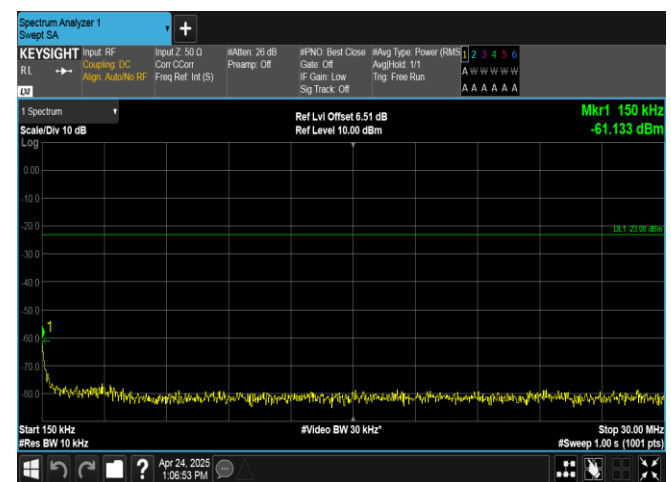
Band26(824-849)-5MHz-QPSK-26815-25RB#0-0.15~30-PASS
