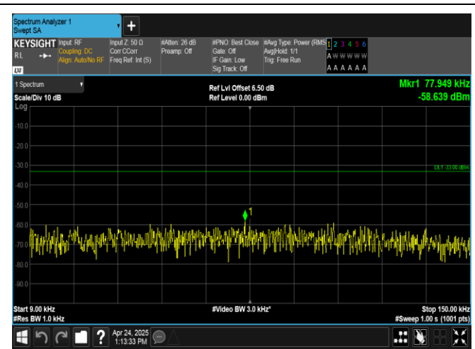
Band26(824-849)-5MHz-QPSK-26915-25RB#0-0.009~0.15-PASS
