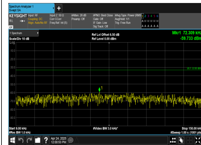
Band26(824-849)-1.4MHz-16QAM-27033-1RB#5-0.009~0.15-PASS
