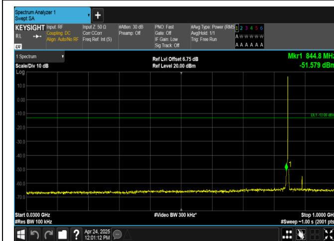
Band26(824-849)-1.4MHz-16QAM-27033-1RB#5-30~1000-PASS
