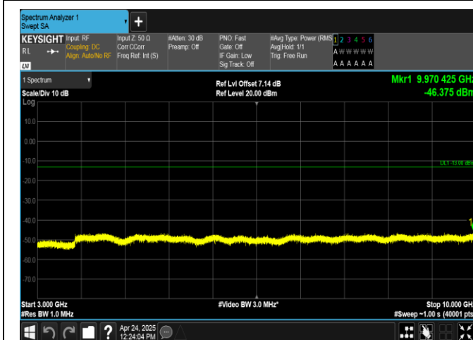
Band26(824-849)-3MHz-QPSK-26805-1RB#0-3000~10000-PASS
