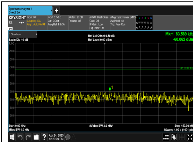
Band26(824-849)-3MHz-QPSK-26805-1RB#0-0.009~0.15-PASS
