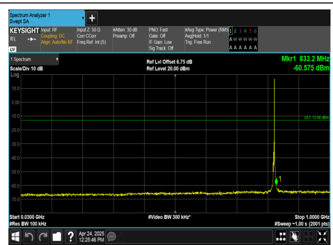
Band26(824-849)-3MHz-QPSK-26805-1RB#14-30~1000-PASS
