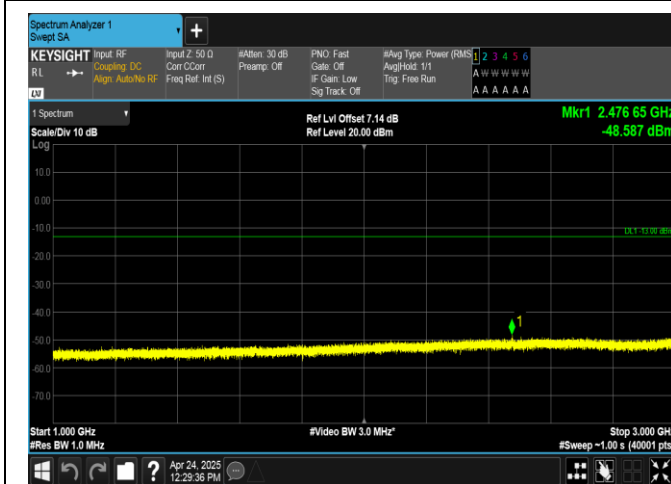
Band26(824-849)-3MHz-16QAM-26805-15RB#0-1000~3000-PASS
