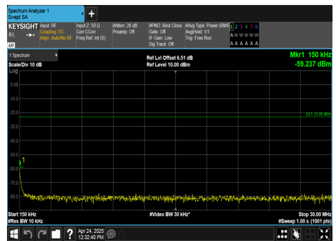
Band26(824-849)-3MHz-QPSK-26915-1RB#14-0.15~30-PASS
