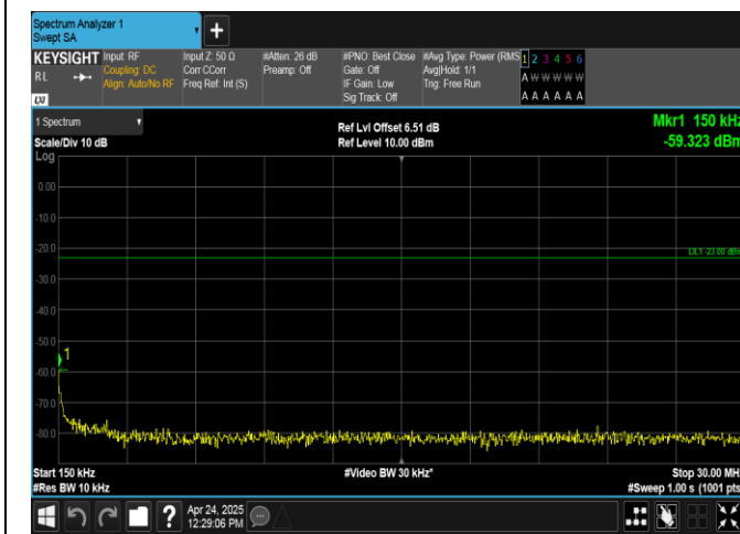
Band26(824-849)-3MHz-16QAM-26805-15RB#0-0.15~30-PASS
