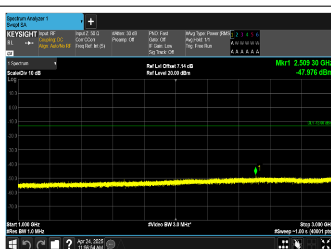
Band26(824-849)-1.4MHz-16OAM-26915-6RB#0-1000~3000-PASS
