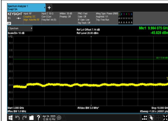
Band26(824-849)-3MHz-QPSK-27025-1RB#0-3000~10000-PASS
