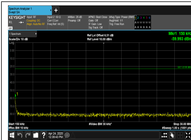
Band26(824-849)-3MHz-QPSK-27025-1RB#14-0.15~30-PASS
