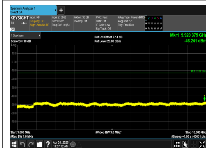
Band26(824-849)-1.4MHz-16OAM-26915-6RB#0-3000~10000-PASS
