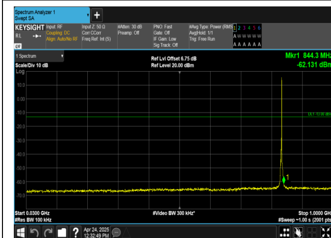
Band26(824-849)-3MHz-QPSK-26915-1RB#14-30~1000-PASS
