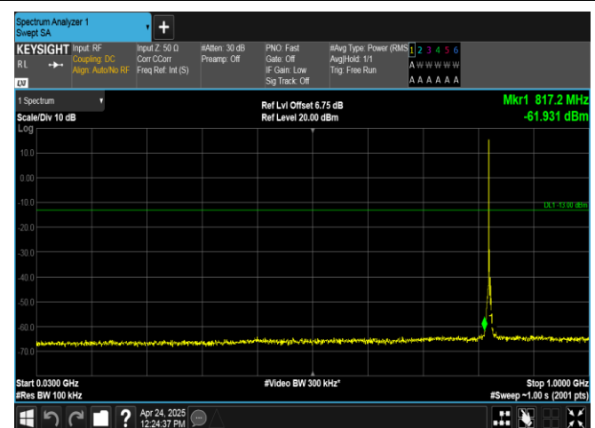
Band26(824-849)-3MHz-16QAM-26805-1RB#0-30~1000-PASS
