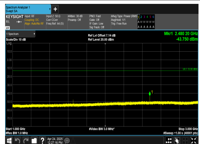
Band26(824-849)-3MHz-16QAM-26805-1RB#14-1000-3000-PASS
