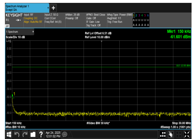
Band26(824-849)-1.4MHz-16QAM-27033-1RB#5-0.15~30-PASS
