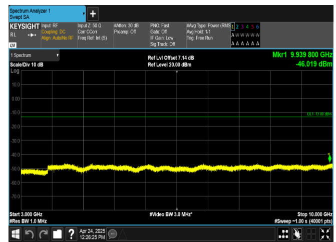
Band26(824-849)-3MHz-QPSK-26805-1RB#14-3000~10000-PASS
