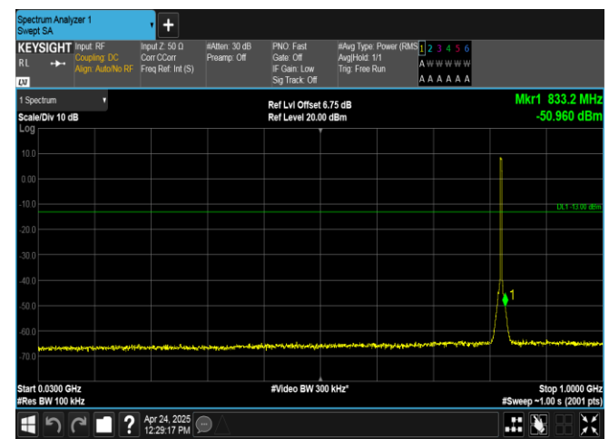
Band26(824-849)-3MHz-16QAM-26805-15RB#0-30~1000-PASS
