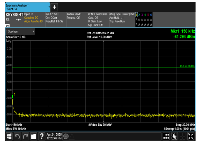
Band26(824-849)-3MHz-16QAM-26805-1RB#14-0.15-30-PASS
