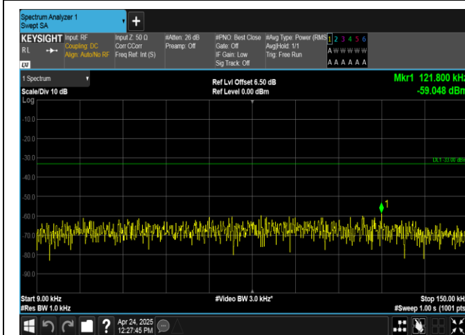
Band26(824-849)-3MHz-QPSK-26805-15RB#0-0.009~0.15-PASS
