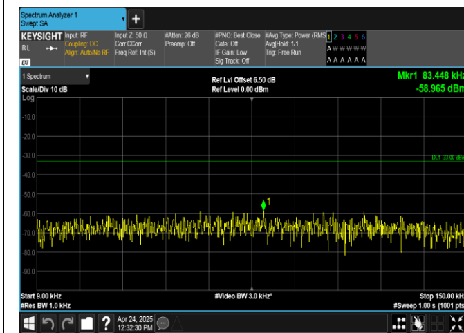
Band26(824-849)-3MHz-QPSK-26915-1RB#14-0.009~0.15-PASS
