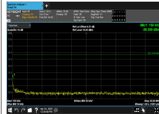
Band26(824-849)-3MHz-QPSK-26915-15RB#0-0.15~30-PASS
