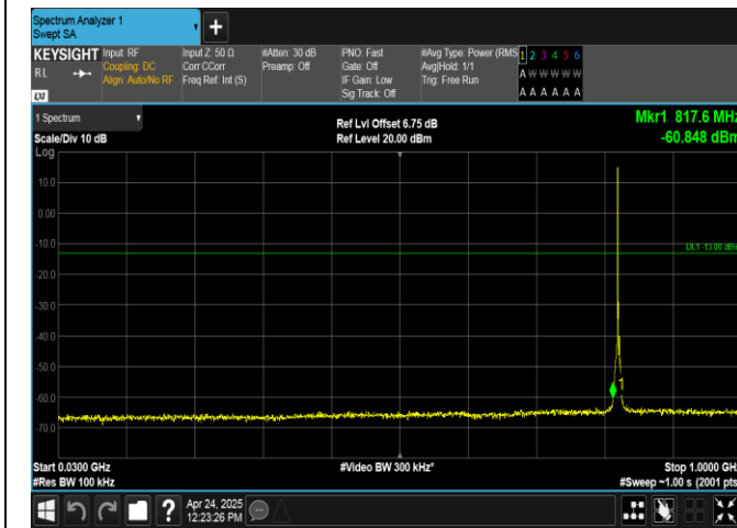
Band26(824-849)-3MHz-QPSK-26805-1RB#0-30~1000-PASS
