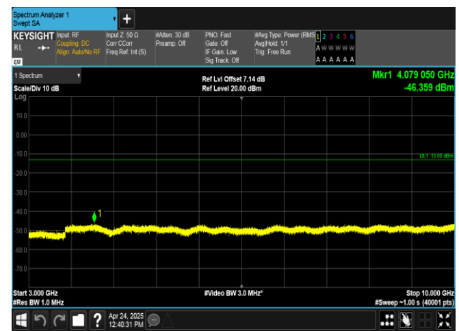
Band26(824-849)-3MHz-QPSK-27025-1RB#14-3000~10000-PASS
