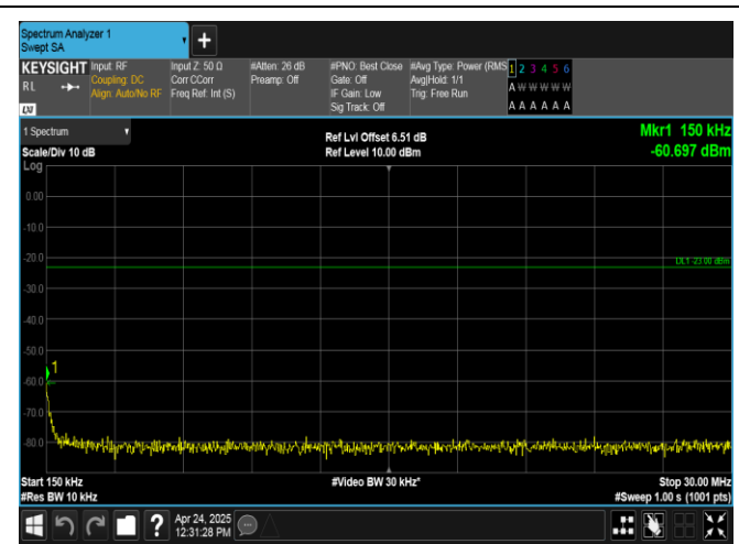
Band26(824-849)-3MHz-16QAM-26915-1RB#0-0.15-30-PASS
