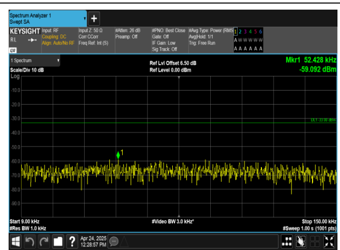
Band26(824-849)-3MHz-16QAM-26805-15RB#0-0.009~0.15-PASS
