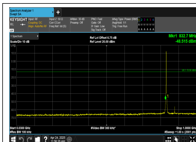
Band26(824-849)-1.4MHz-16OAM-26915-6RB#0-30~1000-PASS
