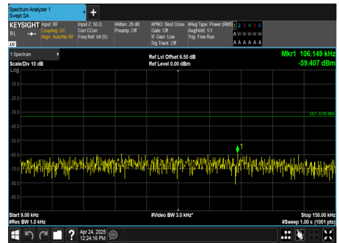
Band26(824-849)-3MHz-16QAM-26805-1RB#0-0.009~0.15-PASS
