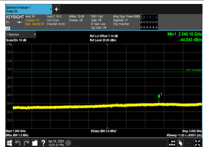
Band26(824-849)-1.4MHz-16QAM-27033-1RB#5-1000~3000-PASS
