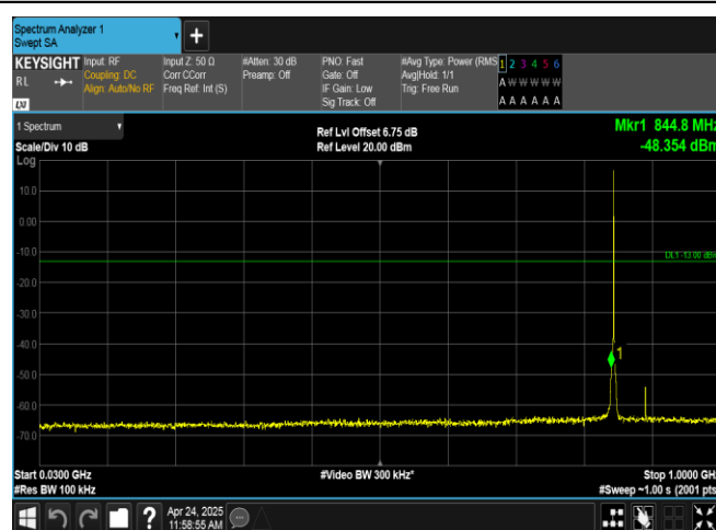
Band26(824-849)-1.4MHz-16QAM-27033-1RB#0-30~1000-PASS
