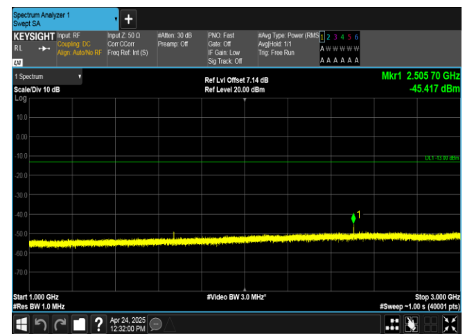
Band26(824-849)-3MHz-16QAM-26915-1RB#0-1000-3000-PASS
