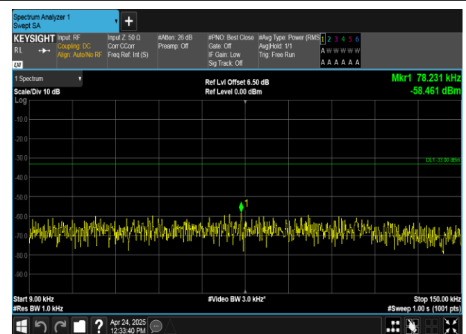
Band26(824-849)-3MHz-16QAM-26915-1RB#14-0.009-0.15-PASS
