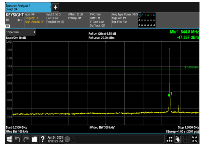
Band26(824-849)-1.4MHz-16QAM-27033-6RB#0-30~1000-PASS
