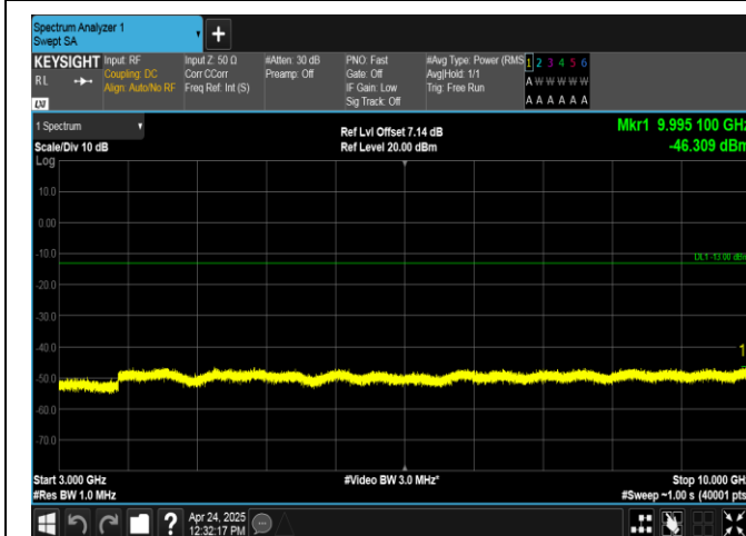
Band26(824-849)-3MHz-16QAM-26915-1RB#0-3000-10000-PASS
