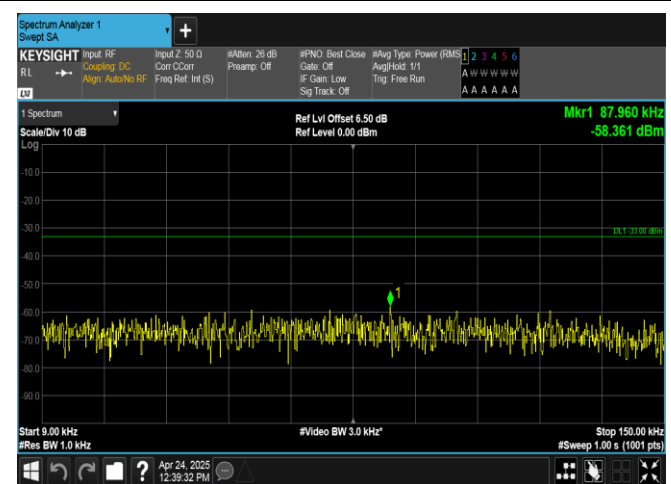
Band26(824-849)-3MHz-QPSK-27025-1RB#14-0.009~0.15-PASS
