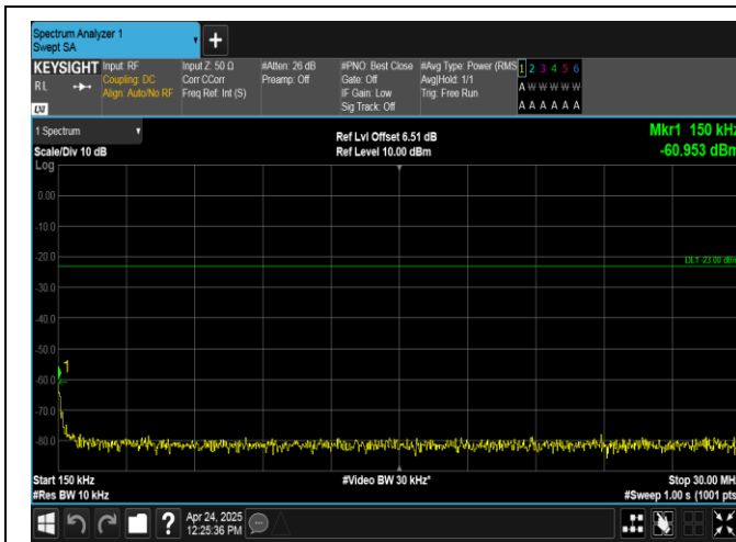
Band26(824-849)-3MHz-QPSK-26805-1RB#14-0.15~30-PASS
