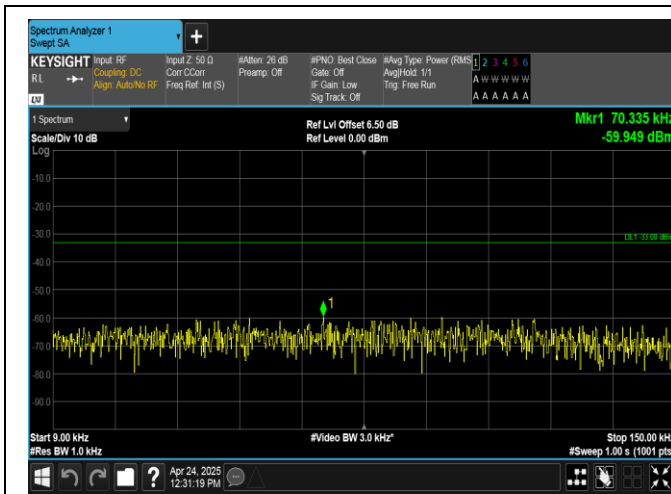
Band26(824-849)-3MHz-16QAM-26915-1RB#0-0.009-0.15-PASS
