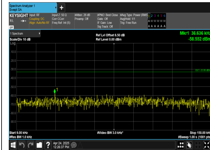
Band26(824-849)-3MHz-16QAM-26805-1RB#14-0.009-0.15-PASS
