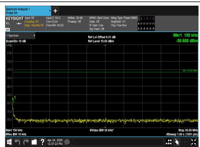
Band26(824-849)-3MHz-QPSK-27025-1RB#0-0.15~30-PASS
