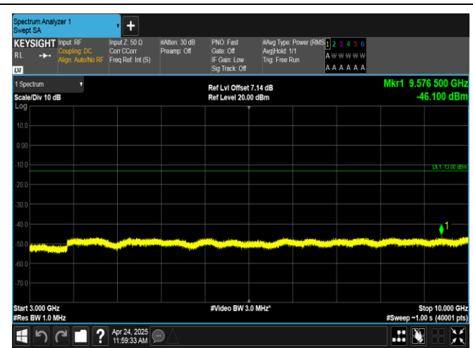
Band26(824-849)-1.4MHz-16QAM-27033-1RB#0-3000~10000-PASS
