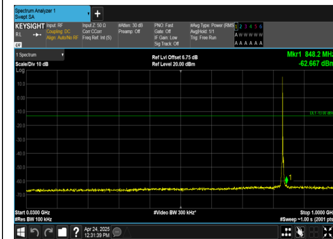
Band26(824-849)-3MHz-16QAM-26915-1RB#0-30-1000-PASS
