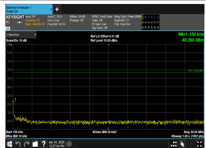
Band26(824-849)-3MHz-QPSK-26805-15RB#0-0.15~30-PASS
