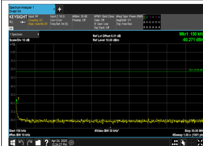
Band26(824-849)-3MHz-16QAM-26805-1RB#0-0.15~30-PASS
