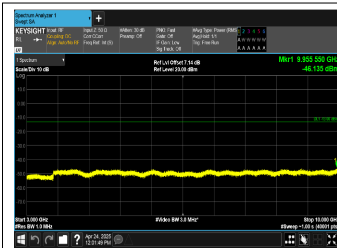
Band26(824-849)-1.4MHz-16QAM-27033-1RB#5-3000~10000-PASS
