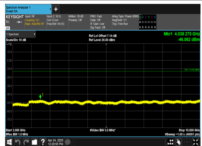
Band26(824-849)-3MHz-16QAM-26805-15RB#0-3000~10000-PASS
