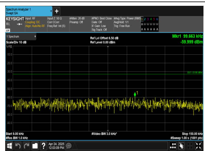
Band26(824-849)-1.4MHz-16QAM-27033-6RB#0-0.009~0.15-PASS
