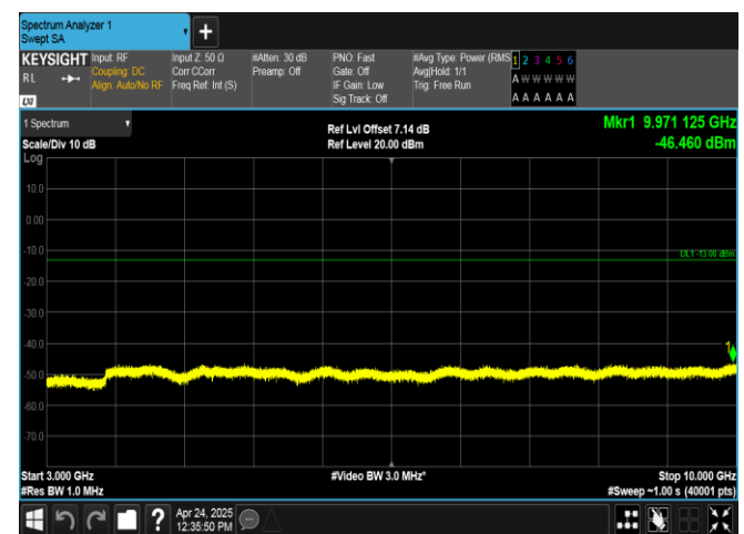
Band26(824-849)-3MHz-QPSK-26915-15RB#0-3000~10000-PASS
