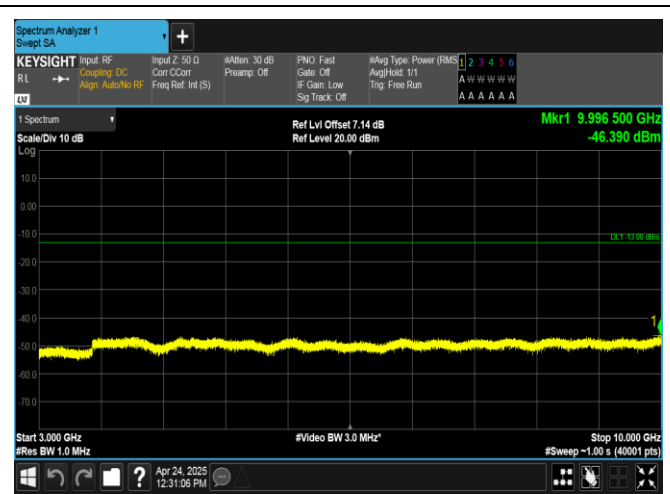
Band26(824-849)-3MHz-QPSK-26915-1RB#0-3000~10000-PASS
