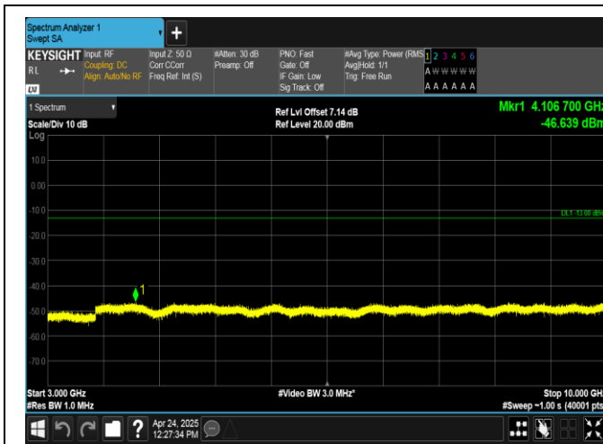
Band26(824-849)-3MHz-16QAM-26805-1RB#14-3000~10000-PASS
