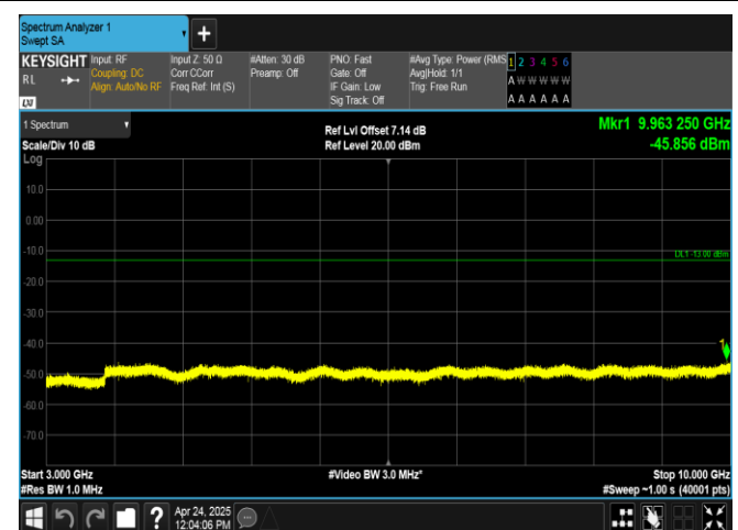
Band26(824-849)-1.4MHz-16QAM-27033-6RB#0-3000~10000-PASS
