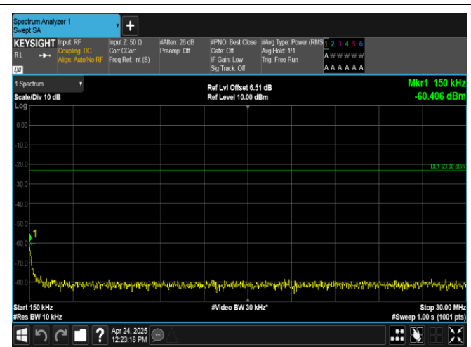
Band26(824-849)-3MHz-QPSK-26805-1RB#0-0.15~30-PASS
