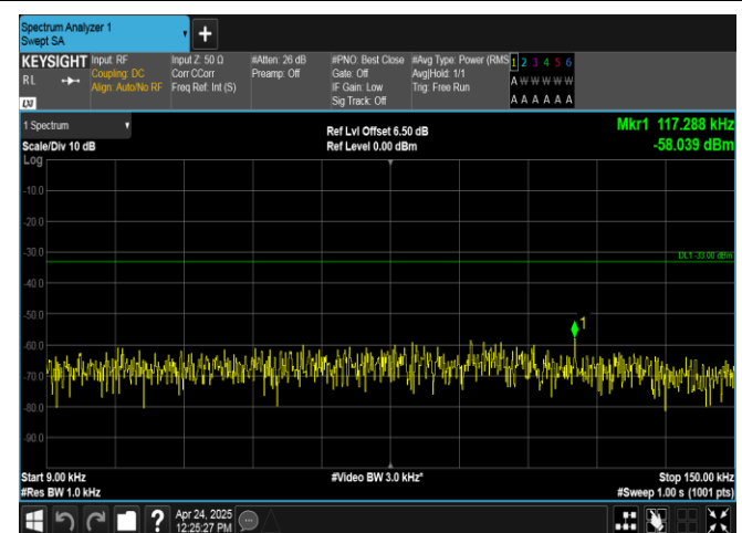
Band26(824-849)-3MHz-QPSK-26805-1RB#14-0.009~0.15-PASS
