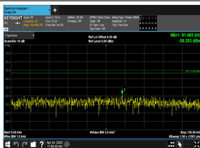
Band26(824-849)-1.4MHz-16OAM-27033-1RB#0-0.009~0.15-PASS
