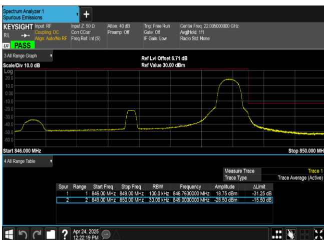
Band26(824-849)-3MHz-16QAM-27025-1RB#14-PASS
