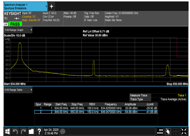
Band26(824-849)-15MHz-QPSK-26965-1RB#0-PASS
