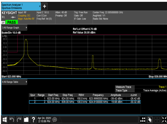
Band26(824-849)-15MHz-QPSK-26865-1RB#0-PASS
