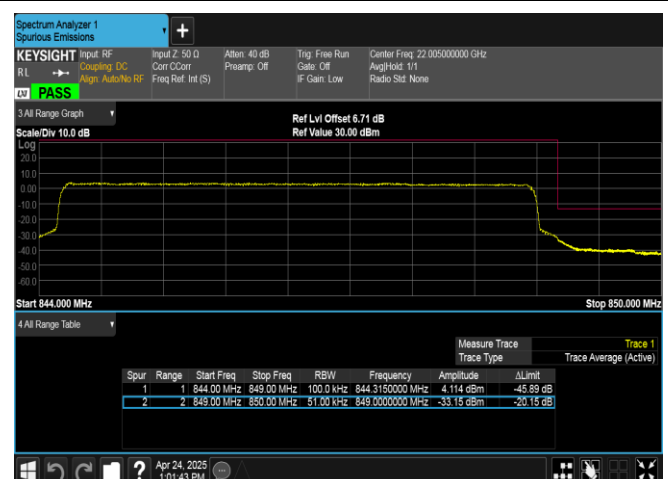
Band26(824-849)-5MHz-QPSK-27015-25RB#0-PASS
