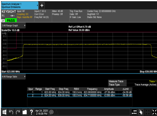
Band26(824-849)-15MHz-QPSK-26865-75RB#0-PASS
