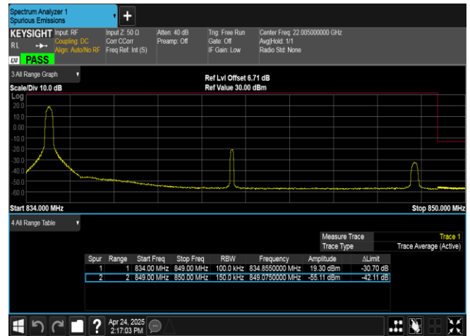
Band26(824-849)-15MHz-16QAM-26965-1RB#0-PASS
