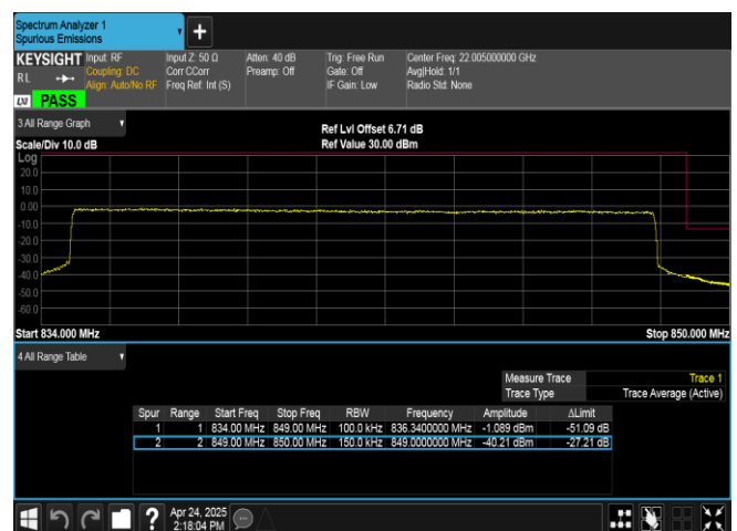
Band26(824-849)-15MHz-16QAM-26965-75RB#0-PASS
