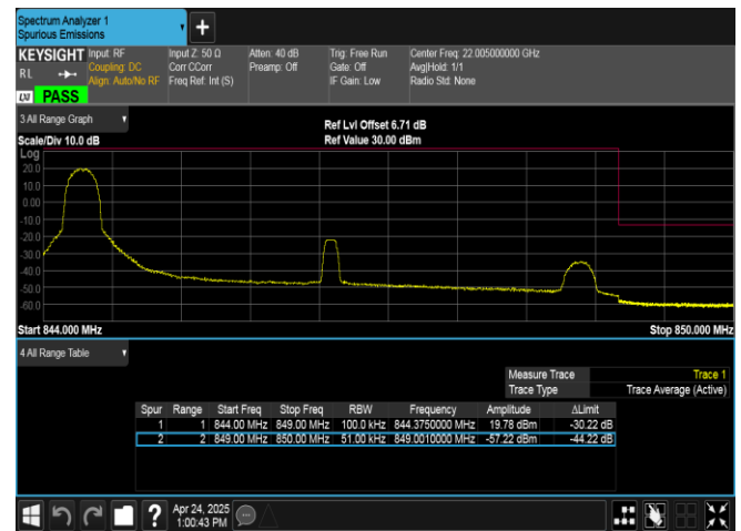
Band26(824-849)-5MHz-QPSK-27015-1RB#0-PASS
