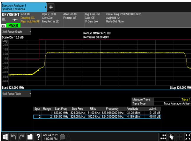
Band26(824-849)-5MHz-QPSK-26815-25RB#0-PASS
