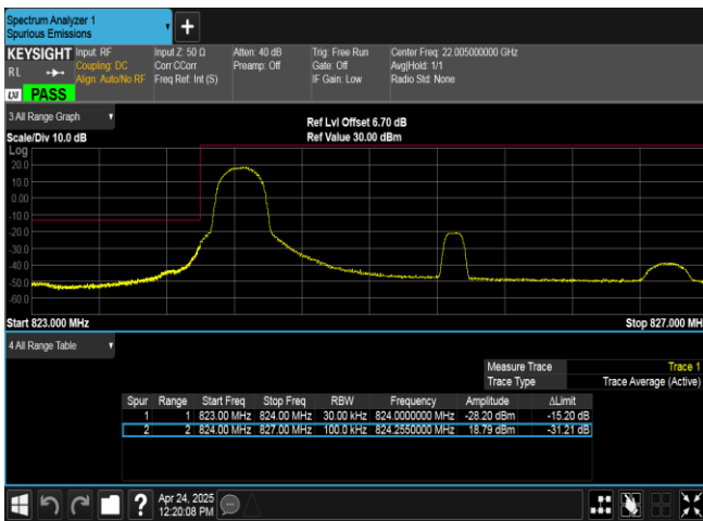
Band26(824-849)-3MHz-16QAM-26805-1RB#0-PASS
