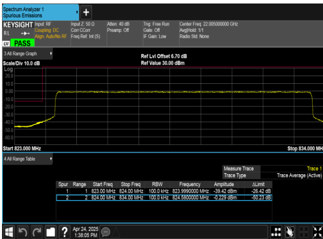
Band26(824-849)-10MHz-16QAM-26840-50RB#0-PASS
