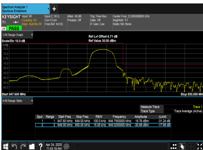
Band26(824-849)-1.4MHz-16QAM-27033-1RB#5-PASS
