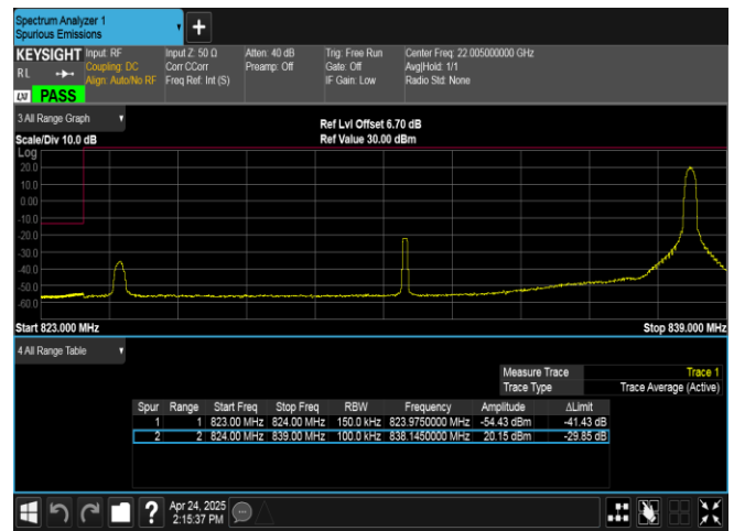
Band26(824-849)-15MHz-QPSK-26865-1RB#74-PASS
