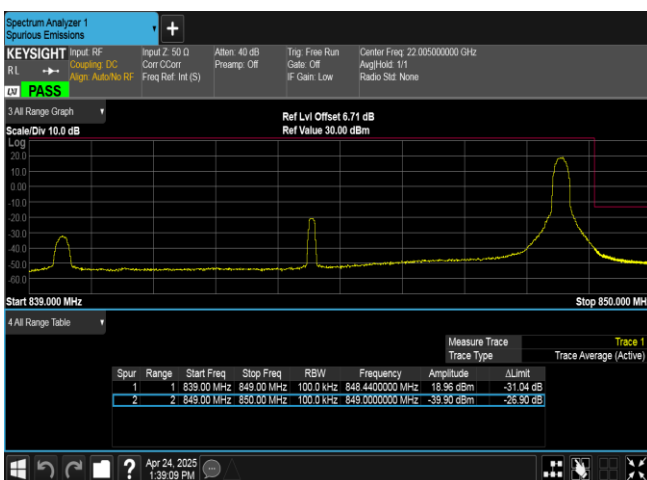
Band26(824-849)-10MHz-16QAM-26990-1RB#49-PASS
