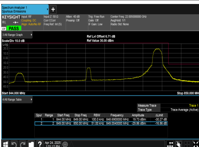
Band26(824-849)-5MHz-QPSK-27015-1RB#24-PASS
