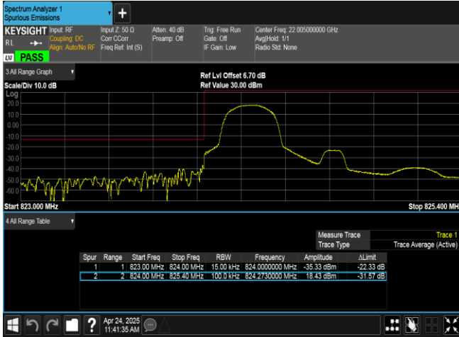
Band26(824-849)-1.4MHz-16QAM-26797-1RB#0-PASS
