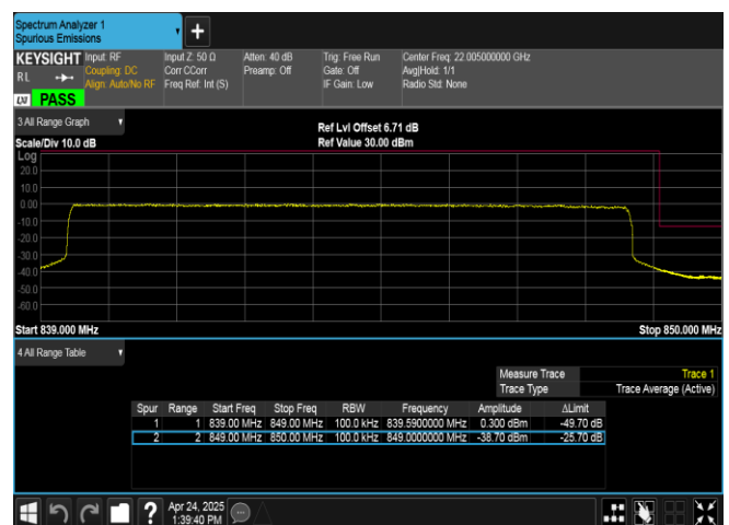
Band26(824-849)-10MHz-16QAM-26990-50RB#0-PASS
