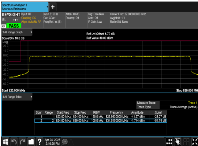
Band26(824-849)-15MHz-16QAM-26865-75RB#0-PASS
