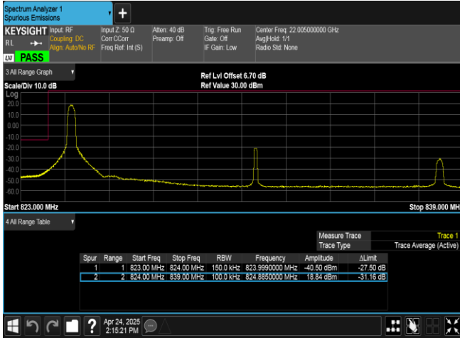
Band26(824-849)-15MHz-16QAM-26865-1RB#0-PASS
