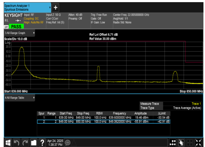
Band26(824-849)-10MHz-16QAM-26990-1RB#0-PASS
