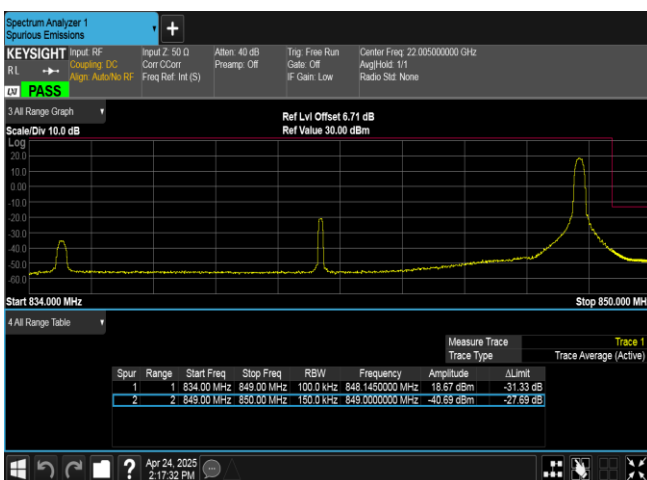
Band26(824-849)-15MHz-16QAM-26965-1RB#74-PASS
