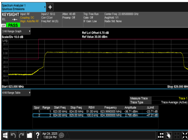
Band26(824-849)-5MHz-16QAM-26815-25RB#0-PASS
