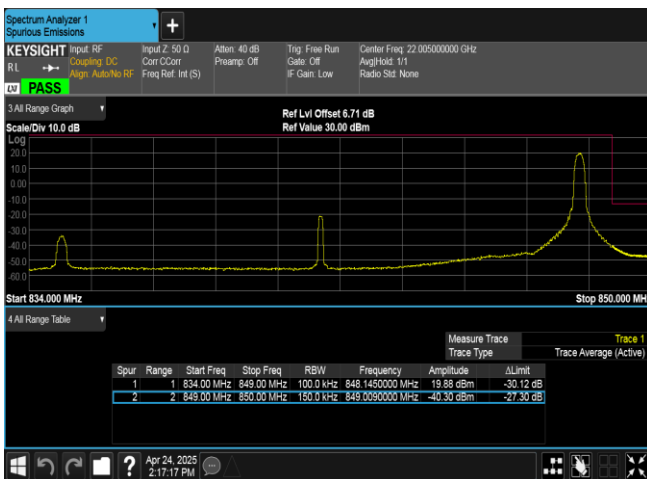
Band26(824-849)-15MHz-QPSK-26965-1RB#74-PASS
