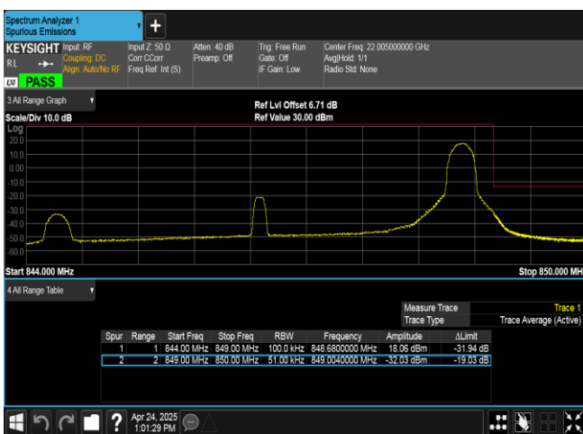
Band26(824-849)-5MHz-16QAM-27015-1RB#24-PASS
