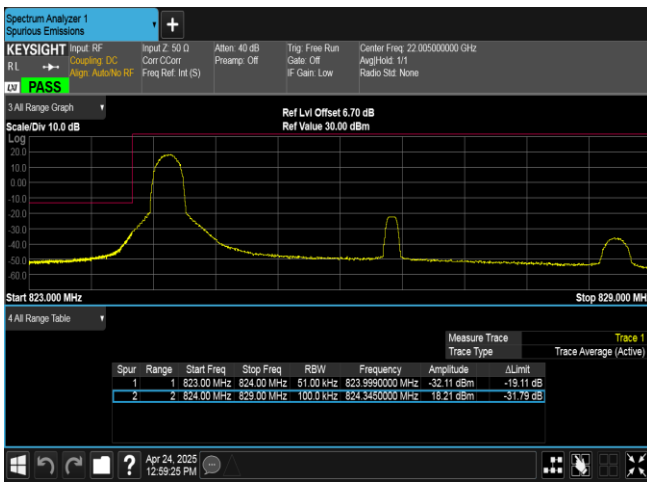
Band26(824-849)-5MHz-16QAM-26815-1RB#0-PASS
