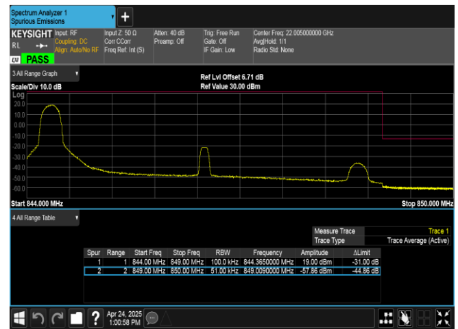
Band26(824-849)-5MHz-16QAM-27015-1RB#0-PASS
