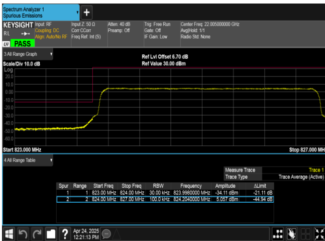
Band26(824-849)-3MHz-16QAM-26805-15RB#0-PASS
