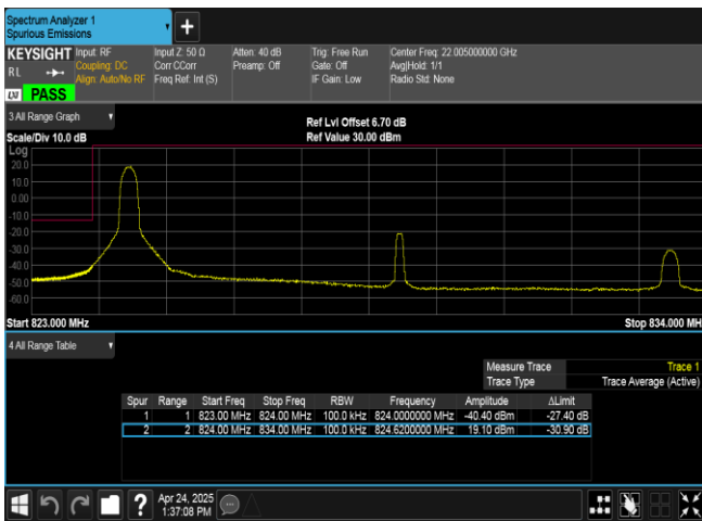
Band26(824-849)-10MHz-16QAM-26840-1RB#0-PASS
