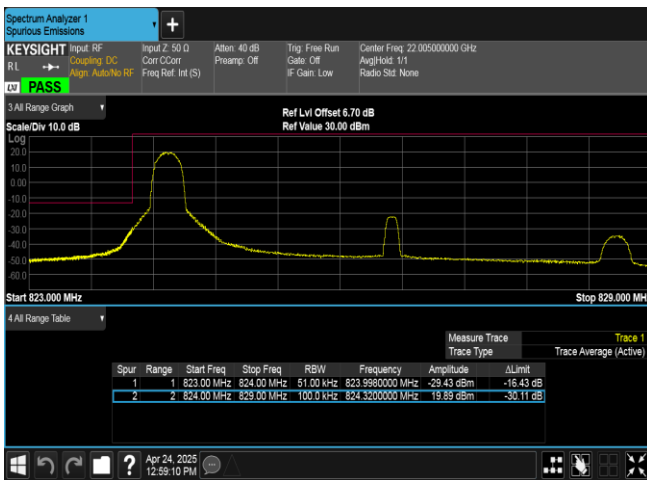
Band26(824-849)-5MHz-QPSK-26815-1RB#0-PASS
