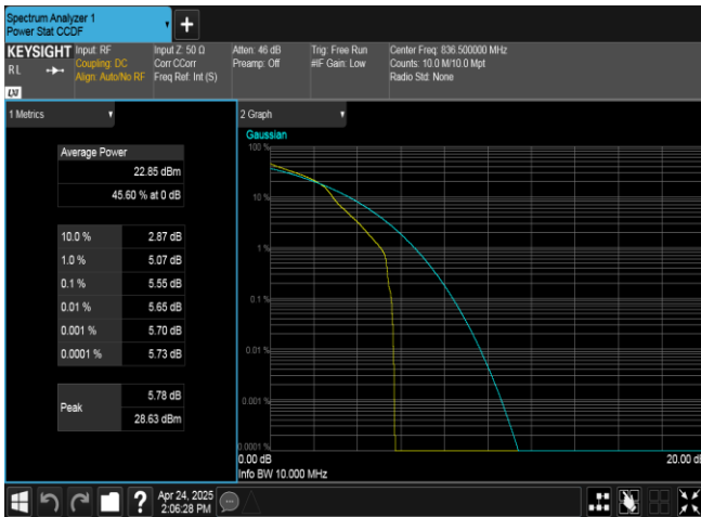
Band26(824-849)-10MHz-16QAM-26915-1RB#0-PASS
