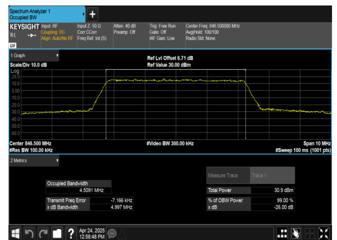
Band26(824-849)-5MHz-16QAM-27015-25RB#0-PASS
