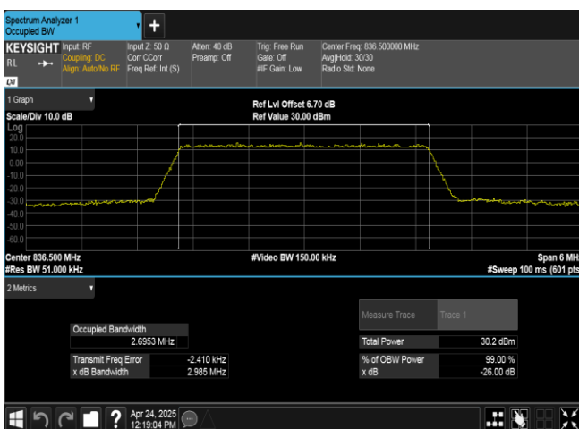
Band26(824-849)-3MHz-16QAM-26915-15RB#0-PASS
