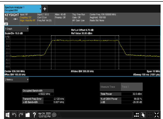
Band26(824-849)-5MHz-QPSK-26915-25RB#0-PASS
