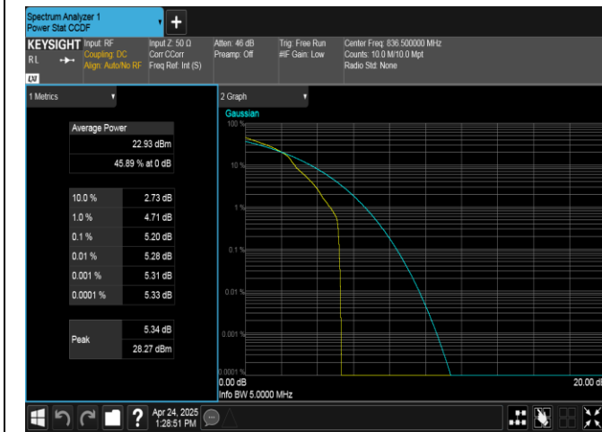
Band26(824-849)-5MHz-16QAM-26915-1RB#0-PASS
