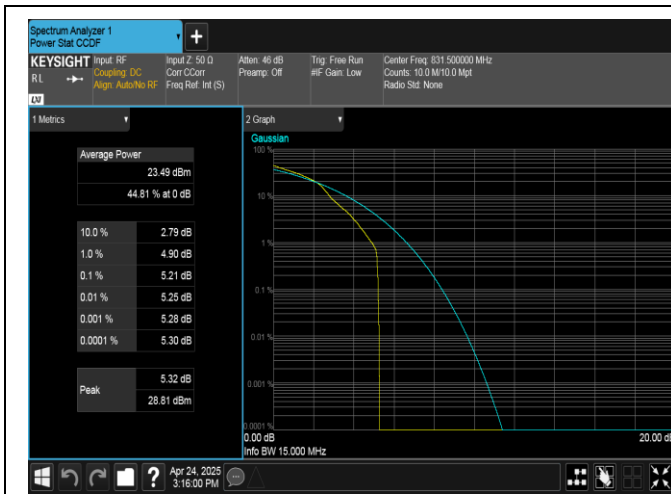
Band26(824-849)-15MHz-16QAM-26865-1RB#0-PASS
