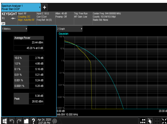
Band26(824-849)-10MHz-16QAM-26990-1RB#0-PASS
