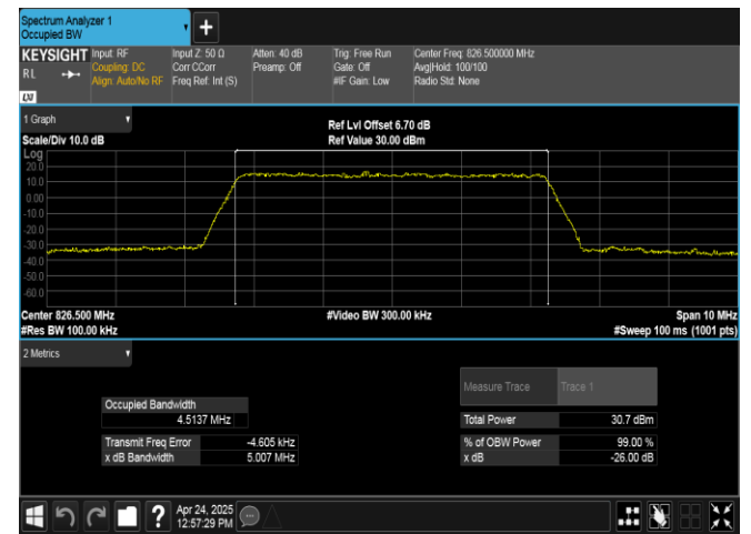
Band26(824-849)-5MHz-16QAM-26815-25RB#0-PASS
