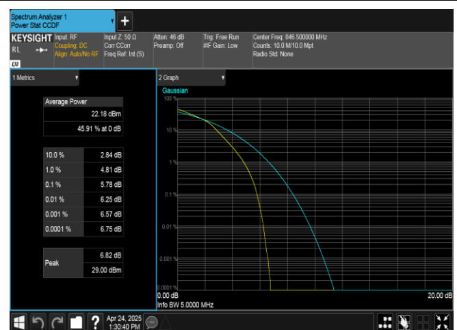
Band26(824-849)-5MHz-16QAM-27015-25RB#0-PASS
