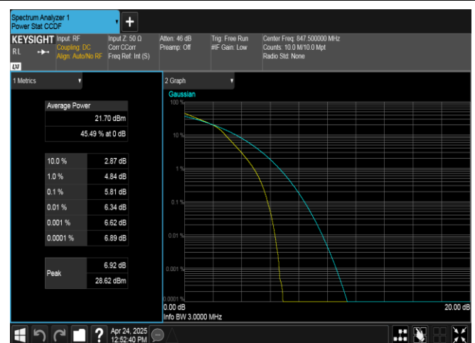
Band26(824-849)-3MHz-16QAM-27025-15RB#0-PASS
