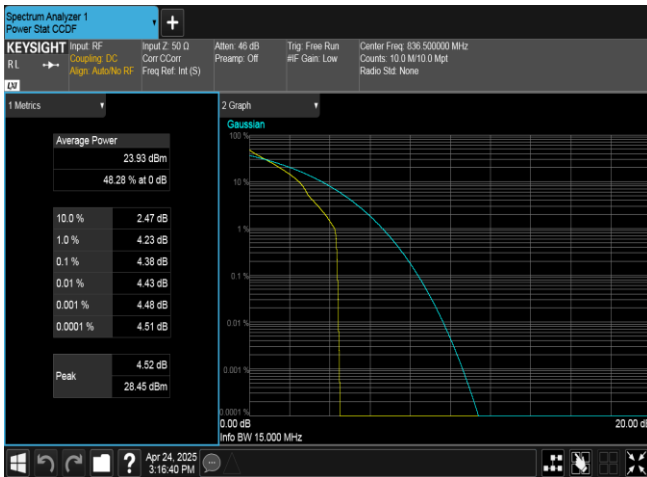
Band26(824-849)-15MHz-QPSK-26915-1RB#0-PASS
