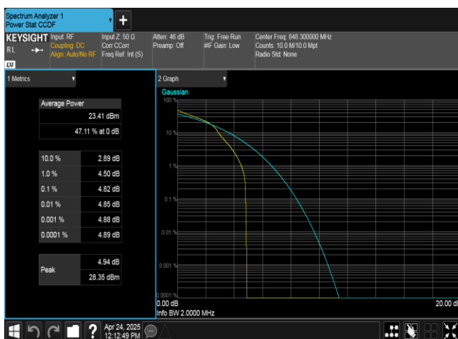
Band26(824-849)-1.4MHz-16QAM-27033-1RB#0-PASS
