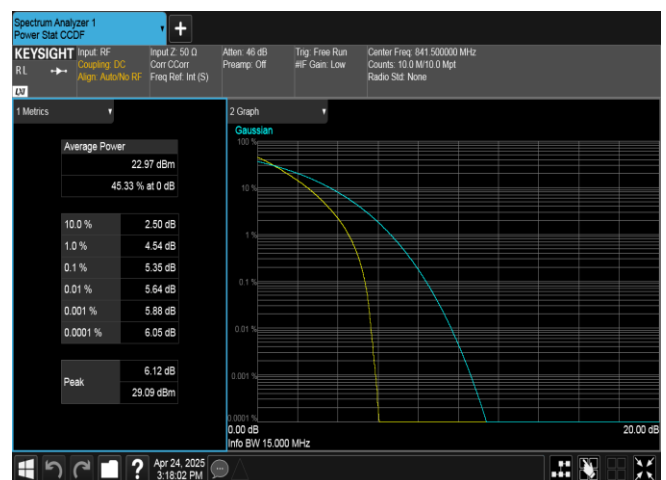
Band26(824-849)-15MHz-QPSK-26965-75RB#0-PASS
