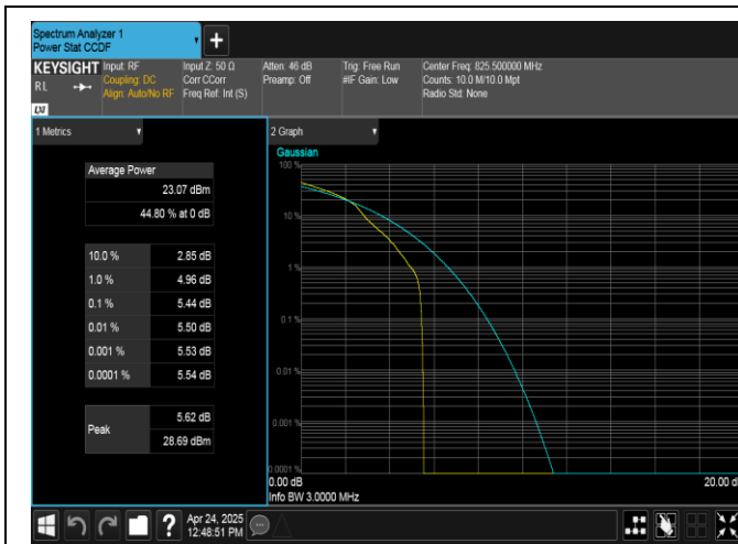
Band26(824-849)-3MHz-16QAM-26805-1RB#0-PASS
