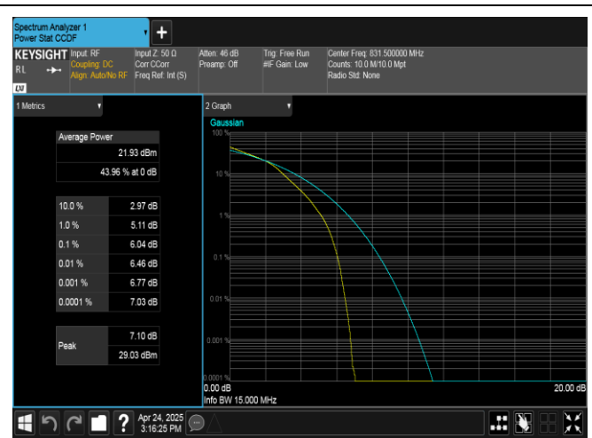
Band26(824-849)-15MHz-16QAM-26865-75RB#0-PASS
