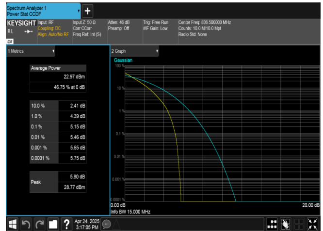
Band26(824-849)-15MHz-QPSK-26915-75RB#0-PASS
