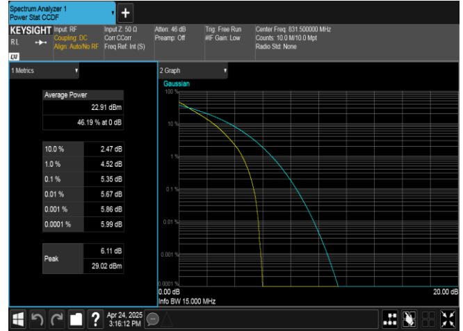
Band26(824-849)-15MHz-QPSK-26865-75RB#0-PASS
