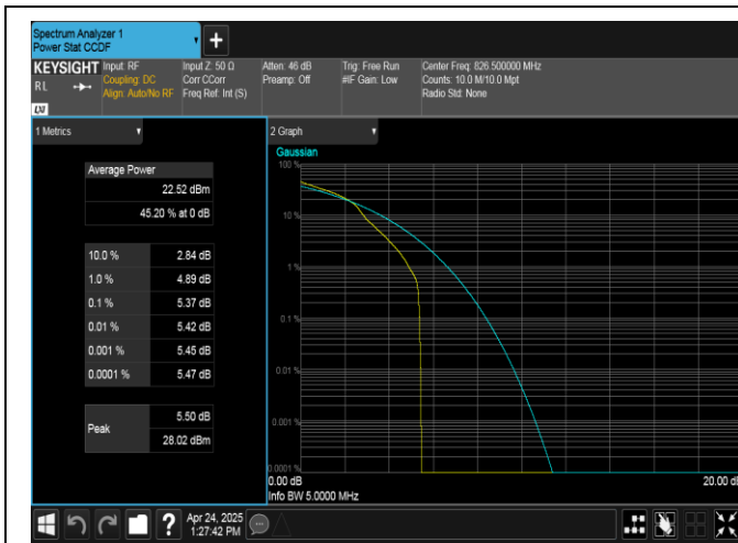
Band26(824-849)-5MHz-16QAM-26815-1RB#0-PASS
