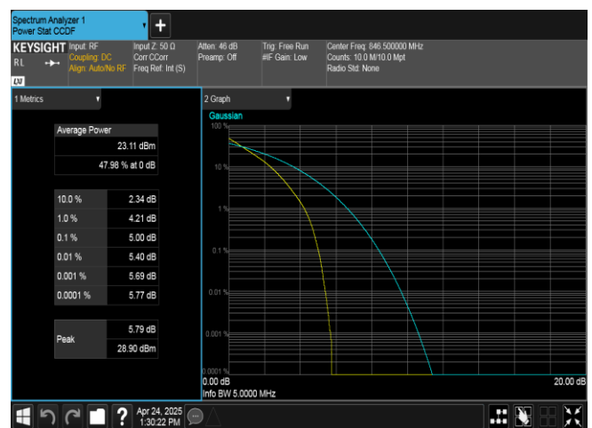
Band26(824-849)-5MHz-QPSK-27015-25RB#0-PASS
