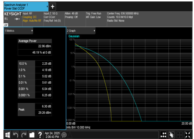
Band26(824-849)-10MHz-QPSK-26915-50RB#0-PASS
