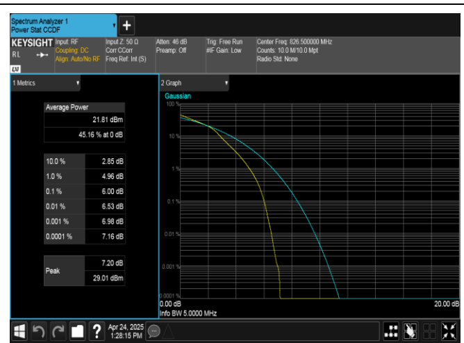
Band26(824-849)-5MHz-16QAM-26815-25RB#0-PASS
