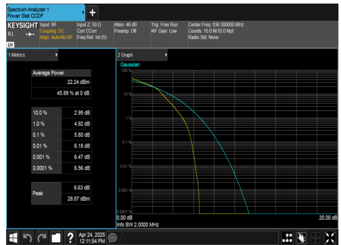
Band26(824-849)-1.4MHz-16QAM-26915-6RB#0-PASS
