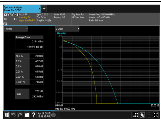
Band26(824-849)-3MHz-16QAM-26805-15RB#0-PASS
