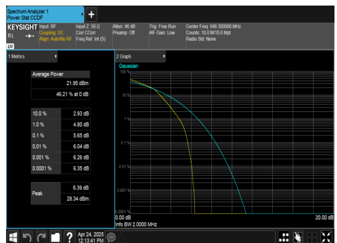
Band26(824-849)-1.4MHz-16QAM-27033-6RB#0-PASS
