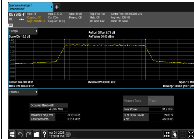
Band26(824-849)-5MHz-QPSK-27015-25RB#0-PASS
