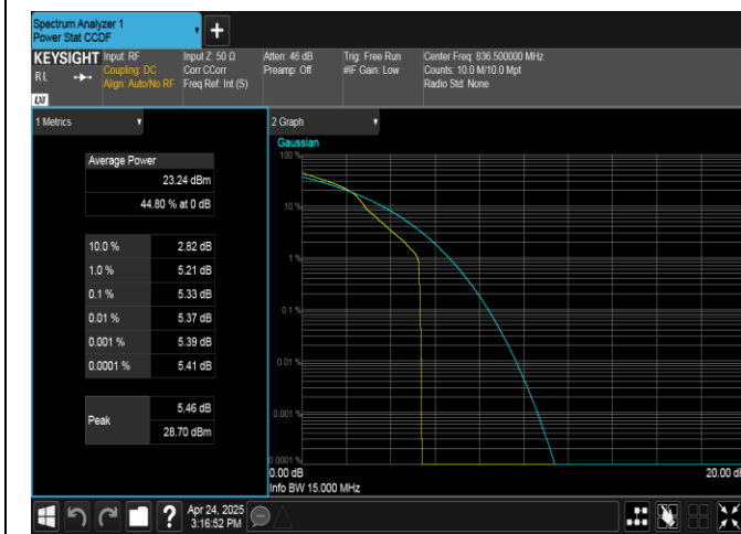
Band26(824-849)-15MHz-16QAM-26915-1RB#0-PASS
