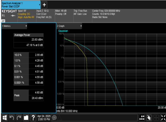
Band26(824-849)-10MHz-QPSK-26840-1RB#0-PASS
