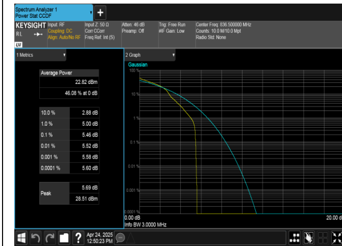
Band26(824-849)-3MHz-16QAM-26915-1RB#0-PASS
