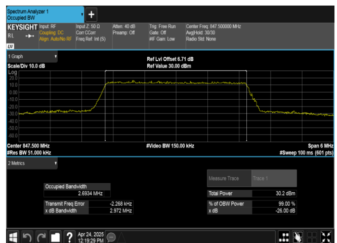
Band26(824-849)-3MHz-16QAM-27025-15RB#0-PASS
