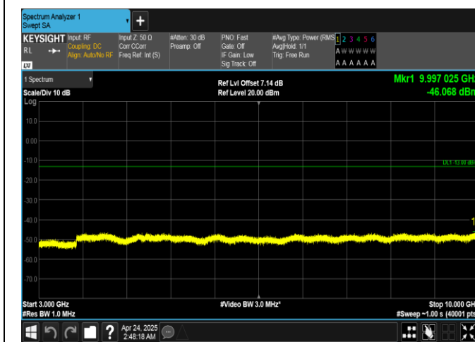
Band26(814-824)-5MHz-16QAM-26740-25RB#0-3000~10000-PASS
