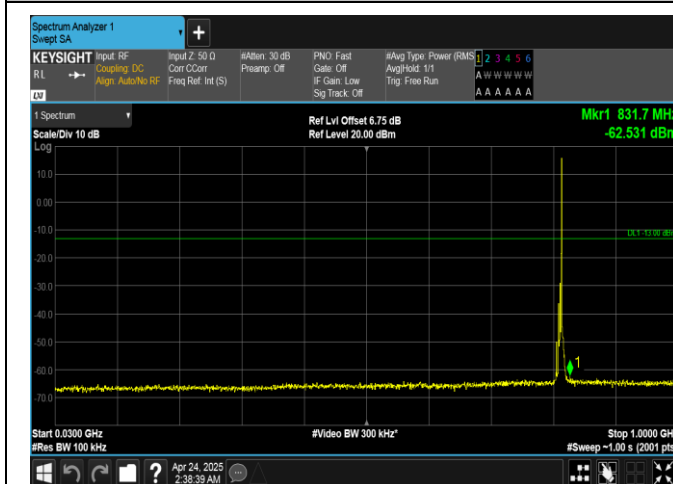
Band26(814-824)-5MHz-16QAM-26715-1RB#24-30~1000-PASS
