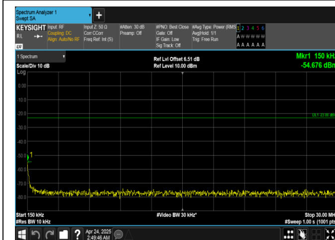
Band26(814-824)-5MHz-16QAM-26765-1RB#0-0.15~30-PASS
