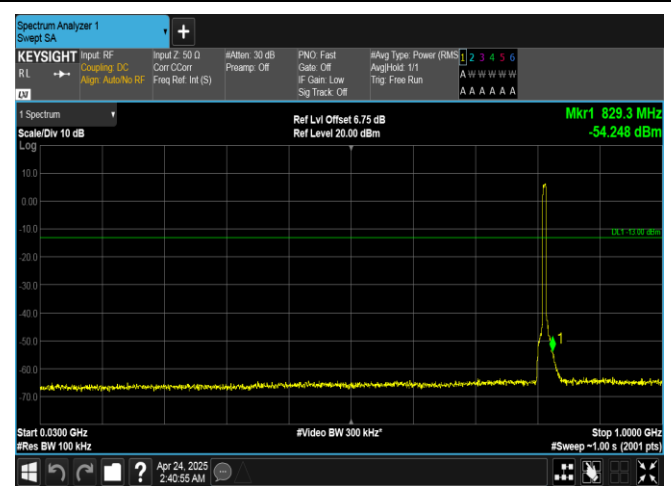
Band26(814-824)-5MHz-16QAM-26715-25RB#0-30~1000-PASS
