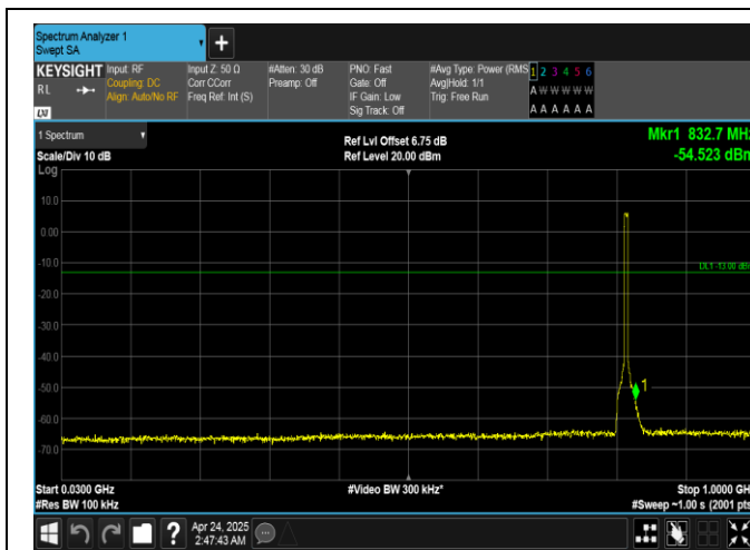
Band26(814-824)-5MHz-16QAM-26740-25RB#0-30~1000-PASS
