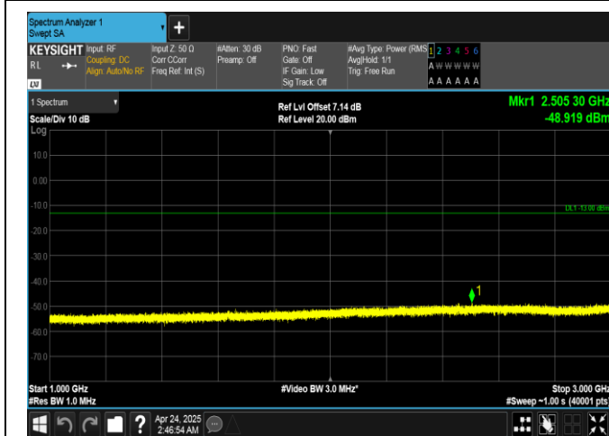
Band26(814-824)-5MHz-QPSK-26740-25RB#0-1000~3000-PASS
