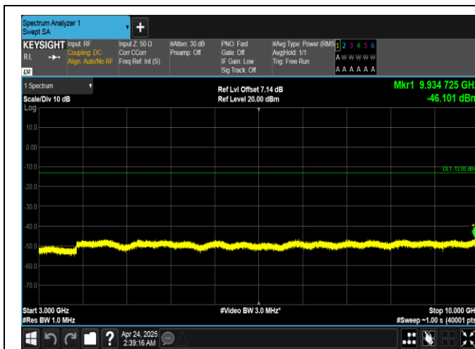
Band26(814-824)-5MHz-16QAM-26715-1RB#24-3000~10000-PASS
