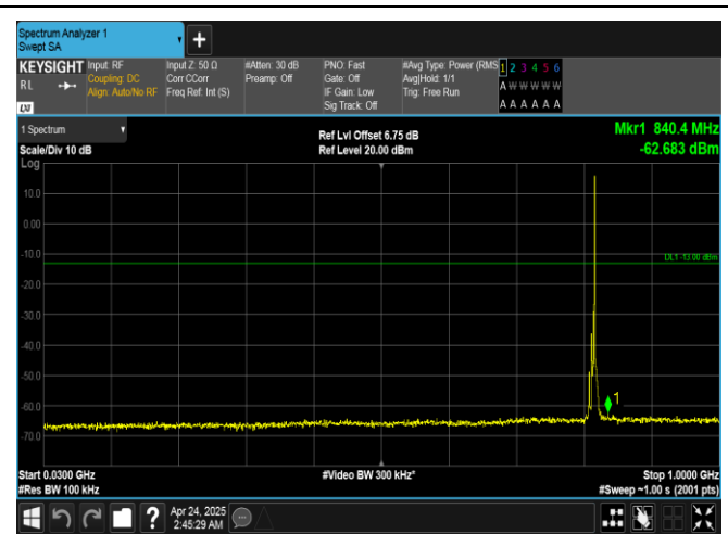
Band26(814-824)-5MHz-16QAM-26740-1RB#24-30~1000-PASS
