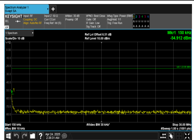
Band26(814-824)-5MHz-16QAM-26715-1RB#24-0.15~30-PASS
