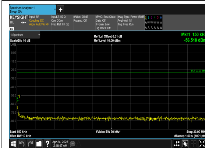
Band26(814-824)-5MHz-16QAM-26715-25RB#0-0.15~30-PASS
