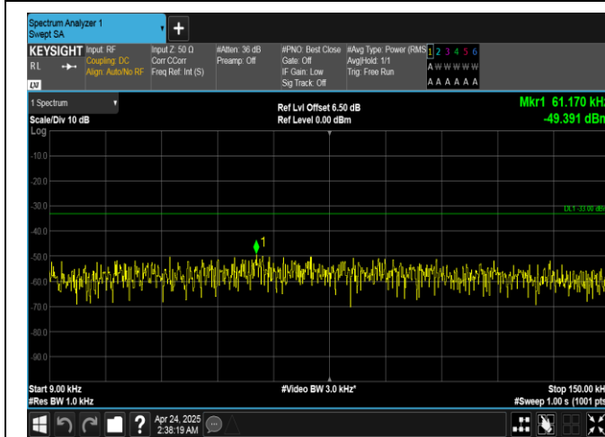
Band26(814-824)-5MHz-16QAM-26715-1RB#24-0.009~0.15-PASS
