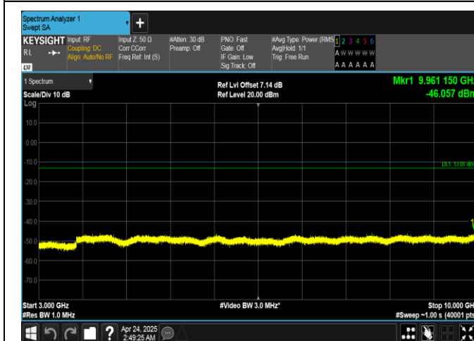
Band26(814-824)-5MHz-QPSK-26765-1RB#0-3000~10000-PASS
