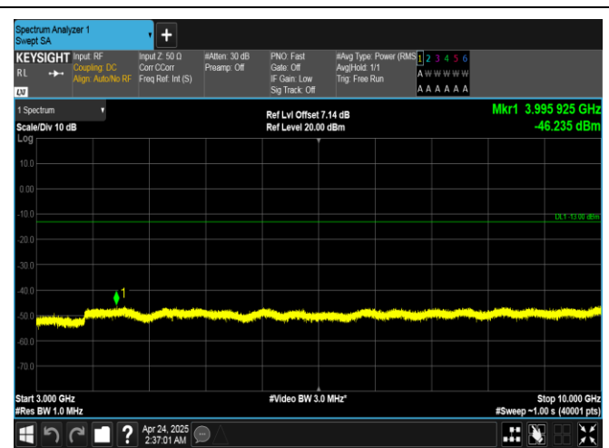
Band26(814-824)-5MHz-16QAM-26715-1RB#0-3000~10000-PASS
