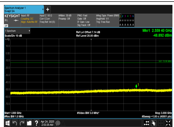
Band26(814-824)-5MHz-QPSK-26765-25RB#0-1000~3000-PASS
