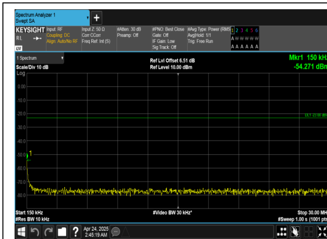
Band26(814-824)-5MHz-16QAM-26740-1RB#24-0.15~30-PASS
