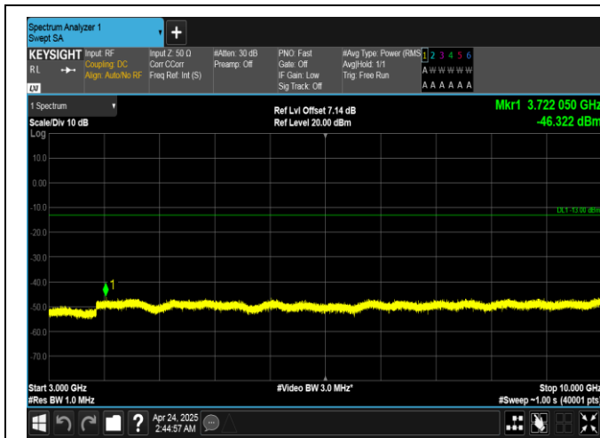
Band26(814-824)-5MHz-QPSK-26740-1RB#24-3000~10000-PASS
