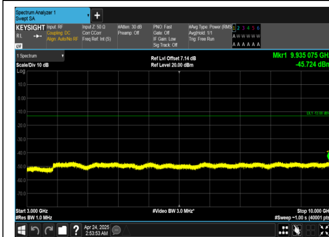
Band26(814-824)-5MHz-QPSK-26765-25RB#0-3000~10000-PASS
