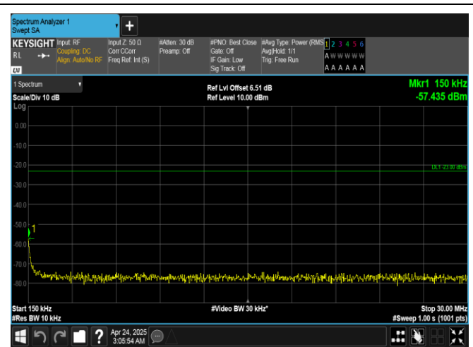
Band26(814-824)-10MHz-QPSK-26740-1RB#0-0.15~30-PASS
