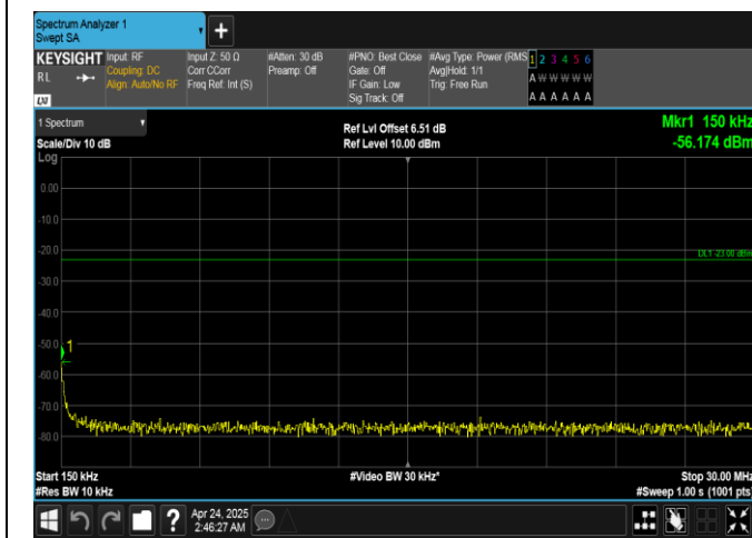
Band26(814-824)-5MHz-QPSK-26740-25RB#0-0.15~30-PASS
