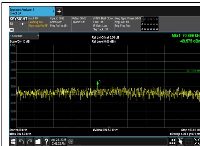
Band26(814-824)-5MHz-QPSK-26765-1RB#0-0.009~0.15-PASS
