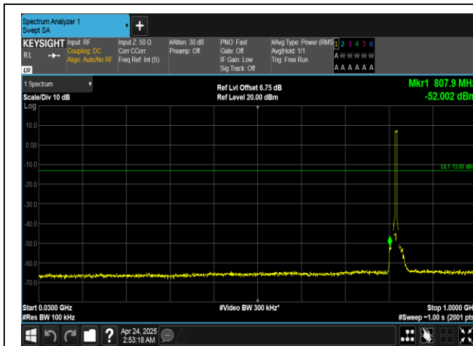
Band26(814-824)-5MHz-QPSK-26765-25RB#0-30~1000-PASS
