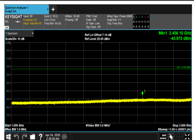
Band26(814-824)-5MHz-16QAM-26715-1RB#24-1000~3000-PASS
