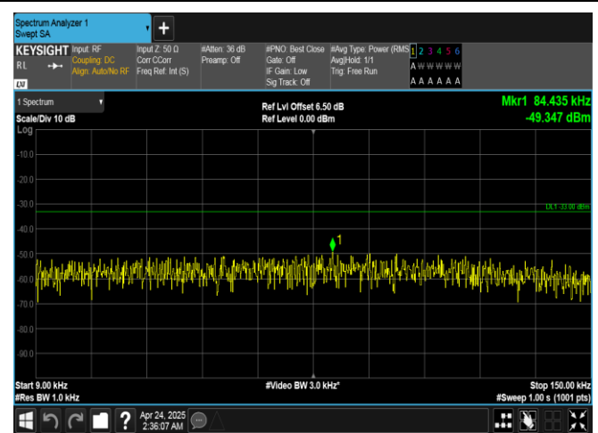
Band26(814-824)-5MHz-16QAM-26715-1RB#0-0.009~0.15-PASS
