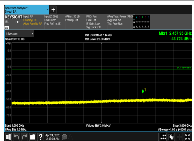
Band26(814-824)-5MHz-QPSK-26765-1RB#0-1000~3000-PASS
