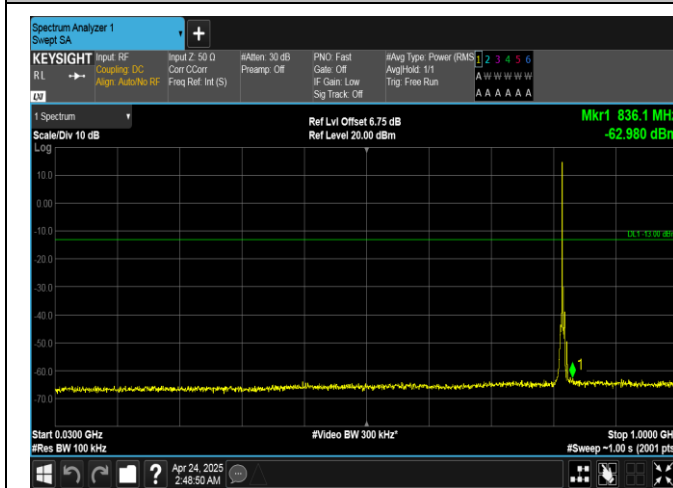
Band26(814-824)-5MHz-QPSK-26765-1RB#0-30~1000-PASS
