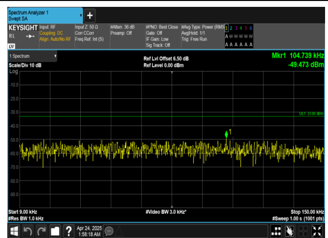
Band26(814-824)-3MHz-16QAM-26705-1RB#0-0.009~0.15-PASS
