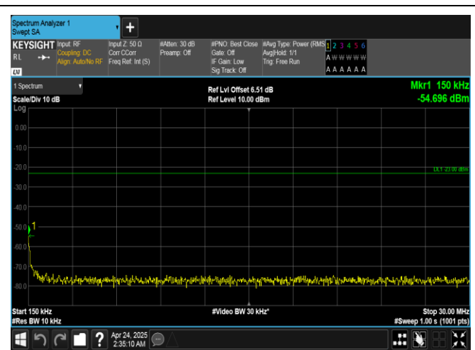
Band26(814-824)-5MHz-QPSK-26715-1RB#0-0.15~30-PASS
