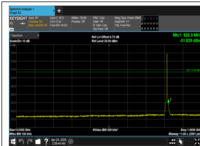
Band26(814-824)-3MHz-16QAM-26740-15RB#0-30~1000-PASS
