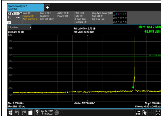
Band26(814-824)-3MHz-QPSK-26775-1RB#0-30~1000-PASS
