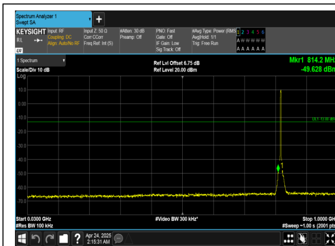
Band26(814-824)-3MHz-QPSK-26775-15RB#0-30~1000-PASS
