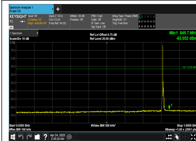
Band26(814-824)-5MHz-QPSK-26715-1RB#0-30~1000-PASS
