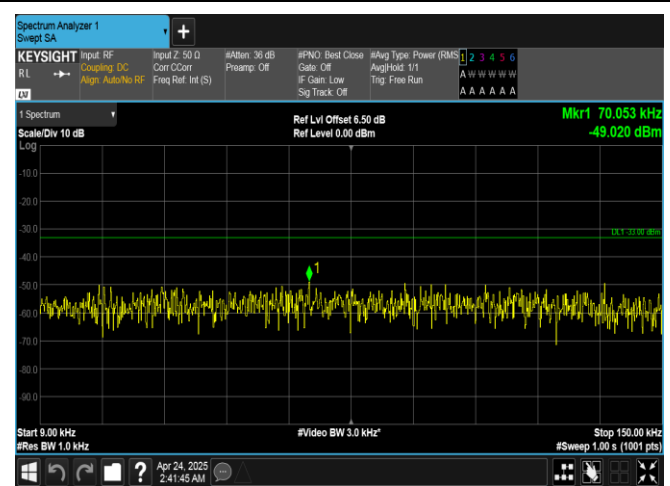
Band26(814-824)-5MHz-QPSK-26740-1RB#0-0.009~0.15-PASS
