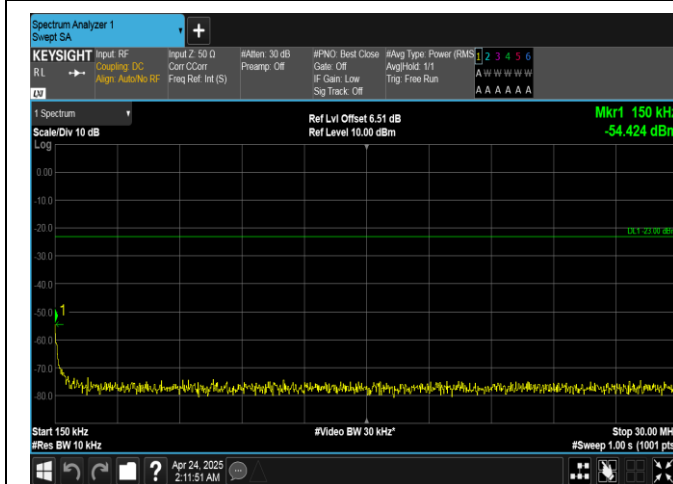
Band26(814-824)-3MHz-16QAM-26775-1RB#0-0.15~30-PASS
