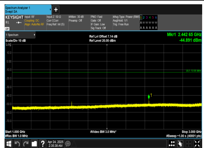
Band26(814-824)-5MHz-QPSK-26715-1RB#0-1000~3000-PASS
