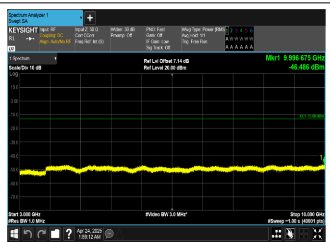
Band26(814-824)-3MHz-16QAM-26705-1RB#0-3000~10000-PASS
