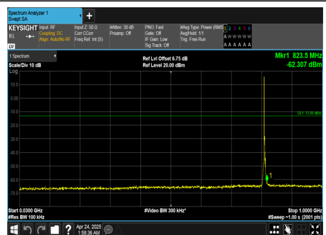
Band26(814-824)-3MHz-16QAM-26705-1RB#0-30~1000-PASS
