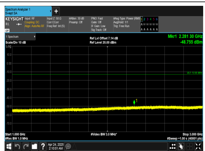
Band26(814-824)-3MHz-16QAM-26740-15RB#0-1000~3000-PASS
