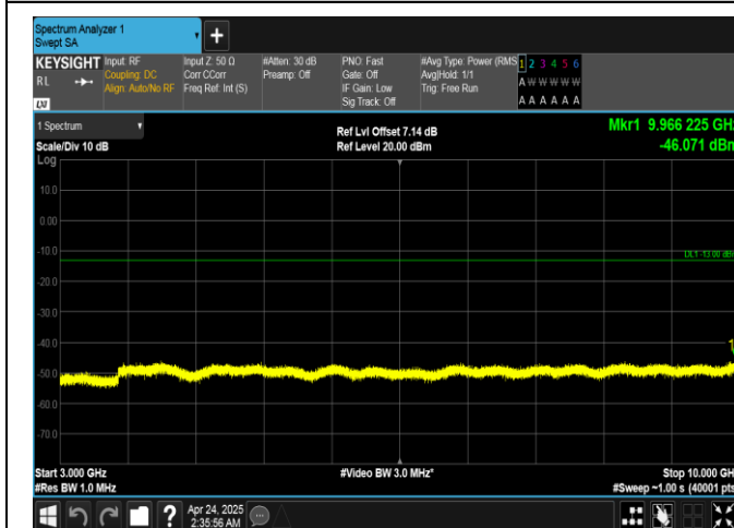
Band26(814-824)-5MHz-QPSK-26715-1RB#0-3000~10000-PASS
