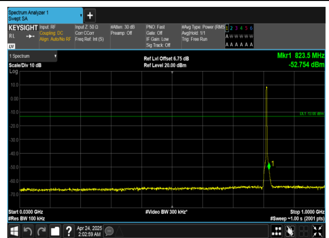
Band26(814-824)-3MHz-16QAM-26705-15RB#0-30~1000-PASS
