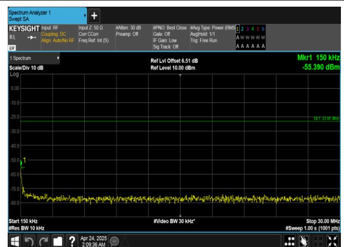
Band26(814-824)-3MHz-16QAM-26740-15RB#0-0.15~30-PASS
