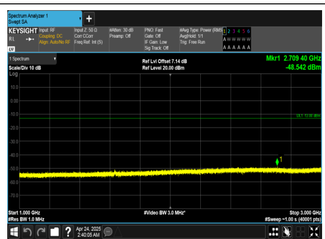
Band26(814-824)-5MHz-QPSK-26715-25RB#0-1000~3000-PASS
