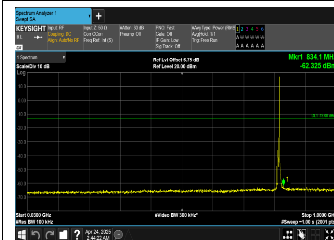
Band26(814-824)-5MHz-QPSK-26740-1RB#24-30~1000-PASS
