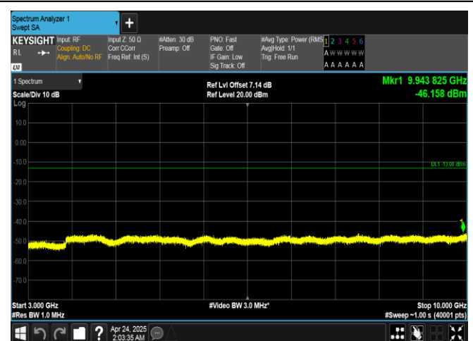
Band26(814-824)-3MHz-16QAM-26705-15RB#0-3000~10000-PASS
