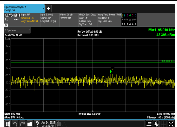
Band26(814-824)-3MHz-QPSK-26775-1RB#14-0.009~0.15-PASS
