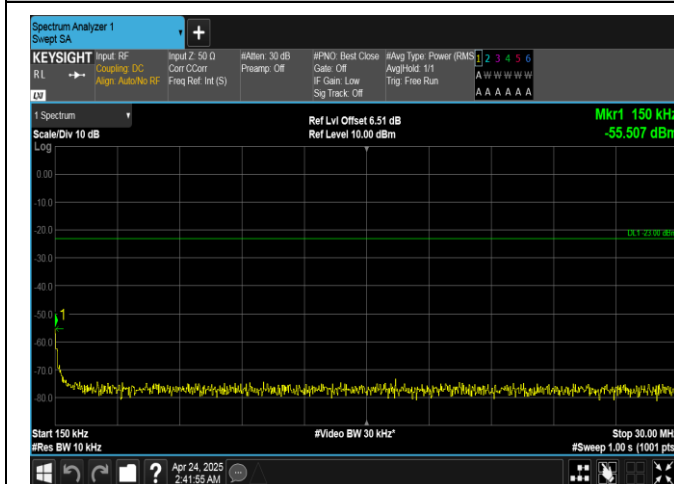
Band26(814-824)-5MHz-QPSK-26740-1RB#0-0.15~30-PASS
