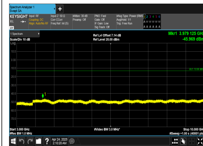
Band26(814-824)-3MHz-16QAM-26740-15RB#0-3000~10000-PASS
