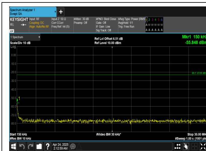
Band26(814-824)-3MHz-QPSK-26775-1RB#14-0.15~30-PASS
