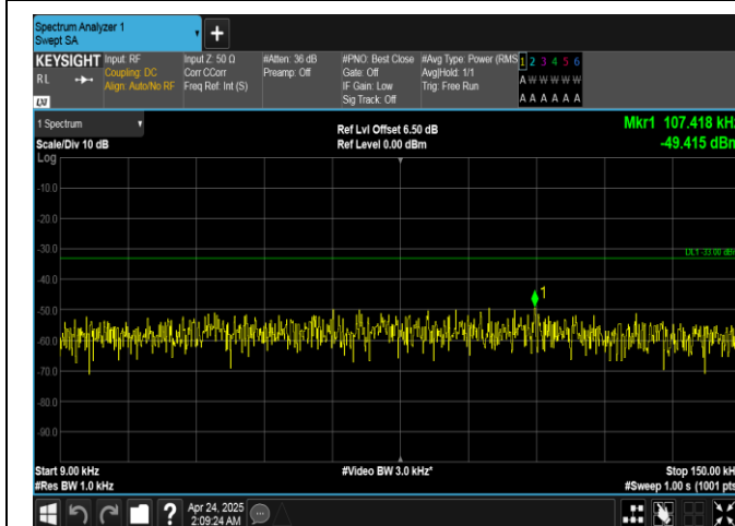
Band26(814-824)-3MHz-16QAM-26740-15RB#0-0.009~0.15-PASS
