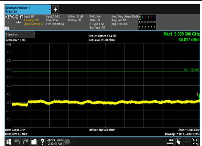
Band26(814-824)-3MHz-QPSK-26775-1RB#14-3000~10000-PASS
