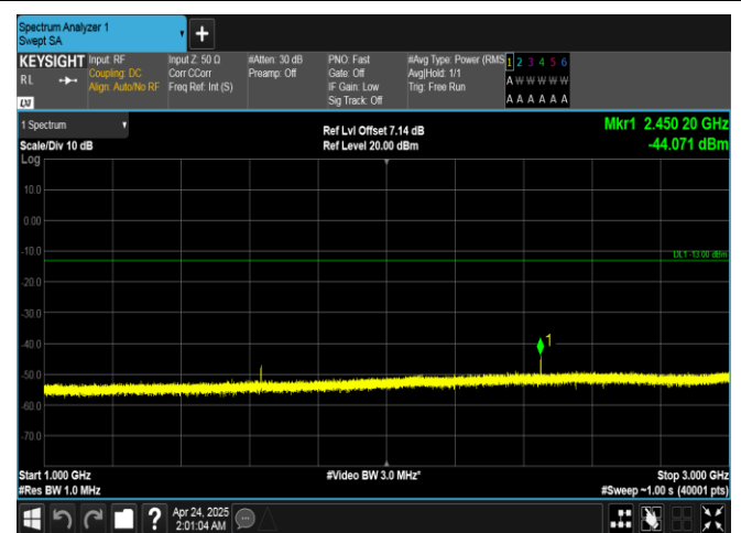
Band26(814-824)-3MHz-16QAM-26705-1RB#14-1000~3000-PASS
