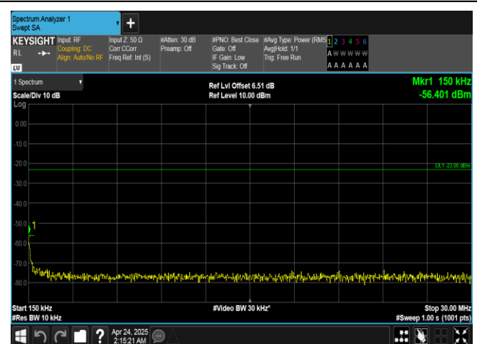
Band26(814-824)-3MHz-QPSK-26775-15RB#0-0.15~30-PASS
