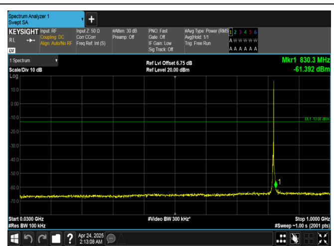
Band26(814-824)-3MHz-QPSK-26775-1RB#14-30~1000-PASS
