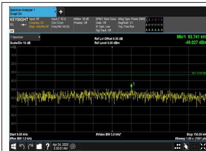
Band26(814-824)-5MHz-QPSK-26715-1RB#0-0.009~0.15-PASS
