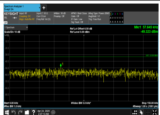
Band26(814-824)-5MHz-QPSK-26715-1RB#24-0.009~0.15-PASS
