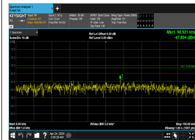
Band26(814-824)-3MHz-16QAM-26705-1RB#14-0.009~0.15-PASS
