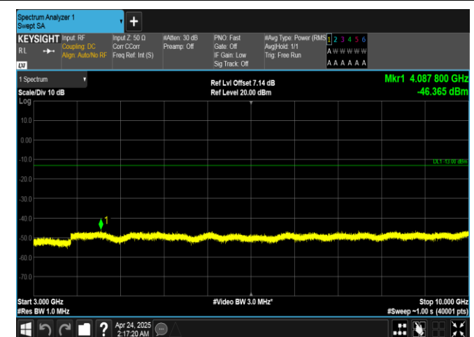
Band26(814-824)-3MHz-16QAM-26775-15RB#0-3000~10000-PASS
