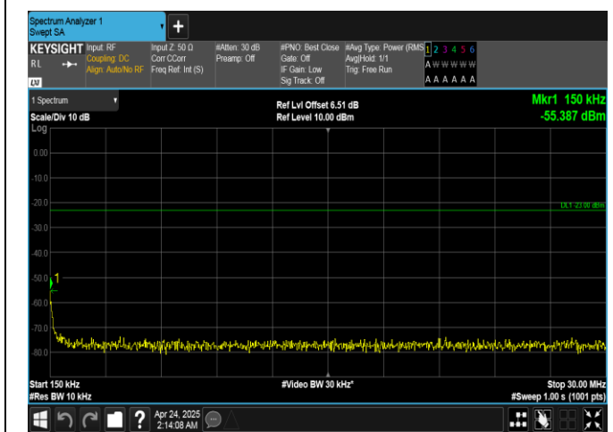
Band26(814-824)-3MHz-16QAM-26775-1RB#14-0.15~30-PASS
