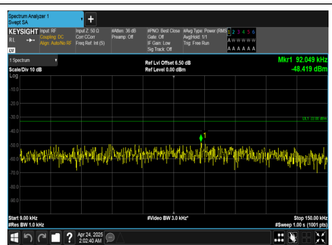
Band26(814-824)-3MHz-16QAM-26705-15RB#0-0.009~0.15-PASS
