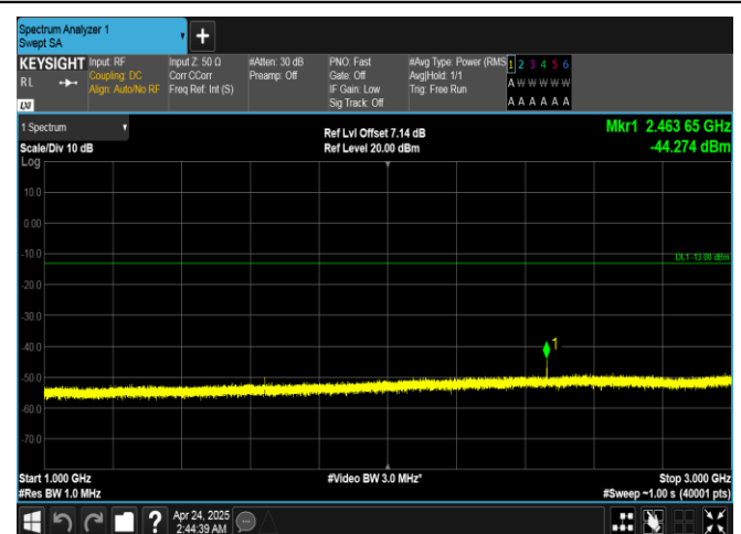
Band26(814-824)-5MHz-QPSK-26740-1RB#24-1000~3000-PASS
