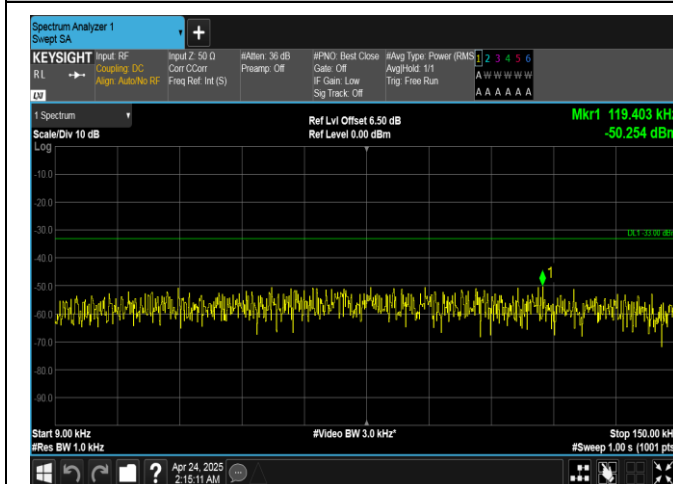
Band26(814-824)-3MHz-QPSK-26775-15RB#0-0.009~0.15-PASS
