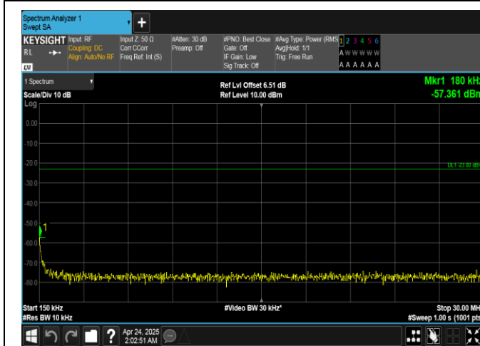
Band26(814-824)-3MHz-16QAM-26705-15RB#0-0.15~30-PASS
