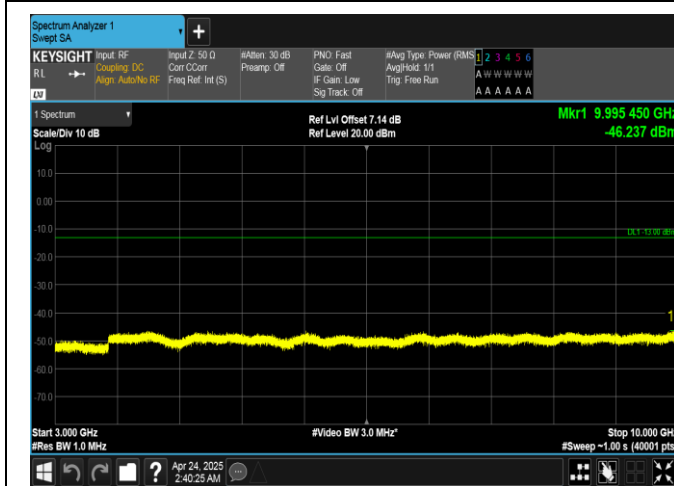
Band26(814-824)-5MHz-QPSK-26715-25RB#0-3000~10000-PASS
