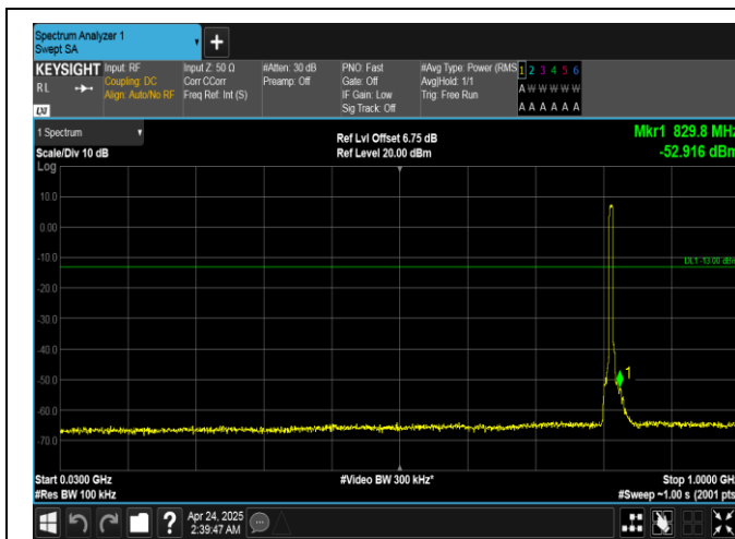
Band26(814-824)-5MHz-QPSK-26715-25RB#0-30~1000-PASS
