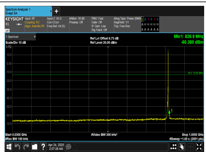
Band26(814-824)-3MHz-16QAM-26740-1RB#14-30~1000-PASS
