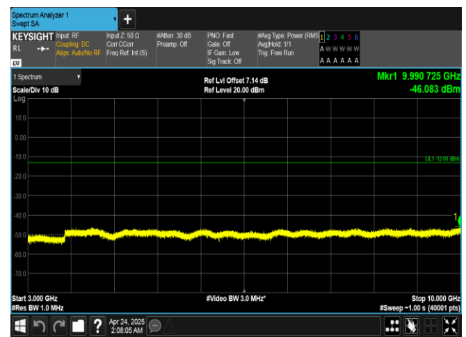
Band26(814-824)-3MHz-16QAM-26740-1RB#14-3000~10000-PASS
