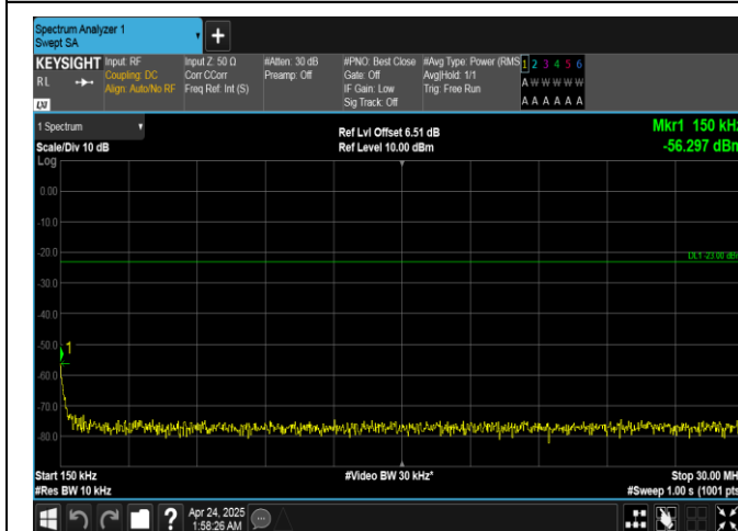
Band26(814-824)-3MHz-16QAM-26705-1RB#0-0.15~30-PASS
