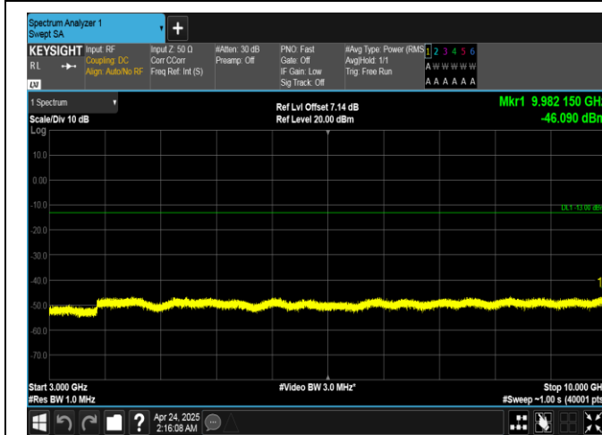
Band26(814-824)-3MHz-QPSK-26775-15RB#0-3000~10000-PASS
