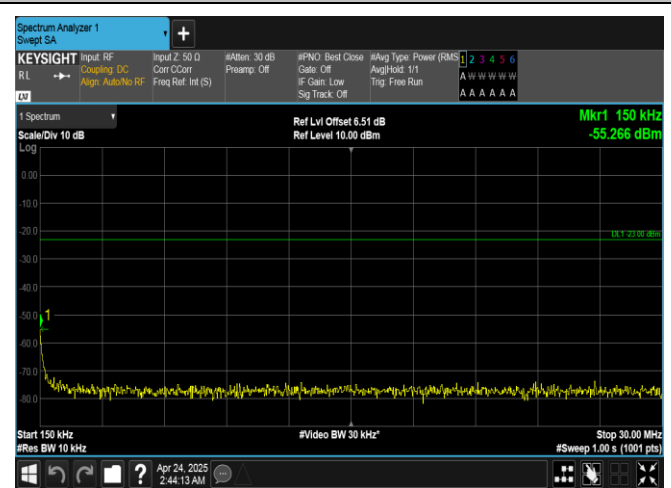
Band26(814-824)-5MHz-QPSK-26740-1RB#24-0.15~30-PASS
