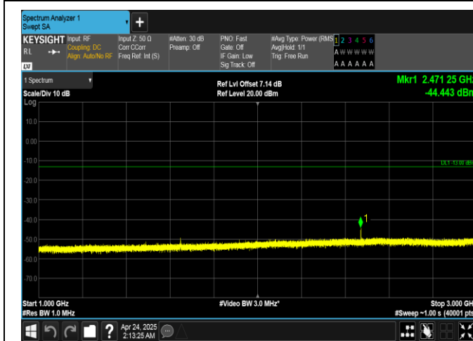
Band26(814-824)-3MHz-QPSK-26775-1RB#14-1000~3000-PASS
