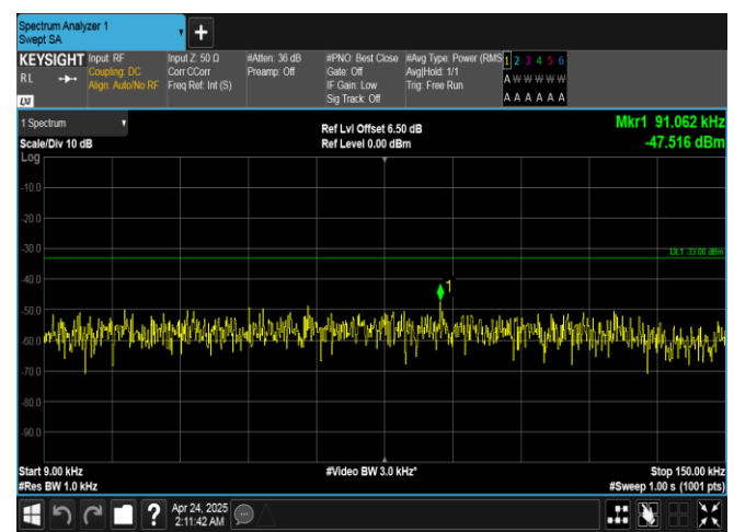
Band26(814-824)-3MHz-16QAM-26775-1RB#0-0.009~0.15-PASS
