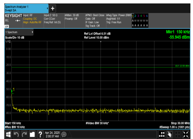
Band26(814-824)-3MHz-16QAM-26705-1RB#14-0.15~30-PASS
