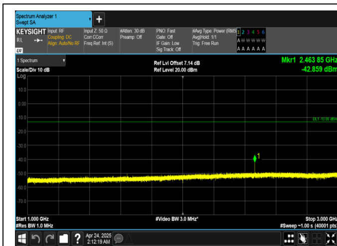
Band26(814-824)-3MHz-16QAM-26775-1RB#0-1000~3000-PASS
