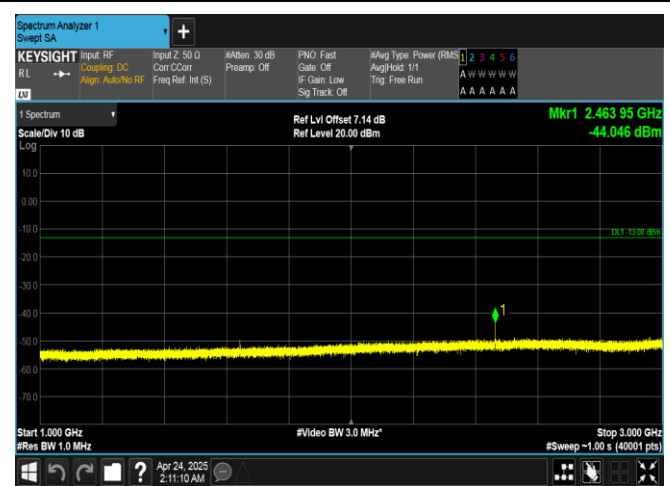
Band26(814-824)-3MHz-QPSK-26775-1RB#0-1000~3000-PASS
