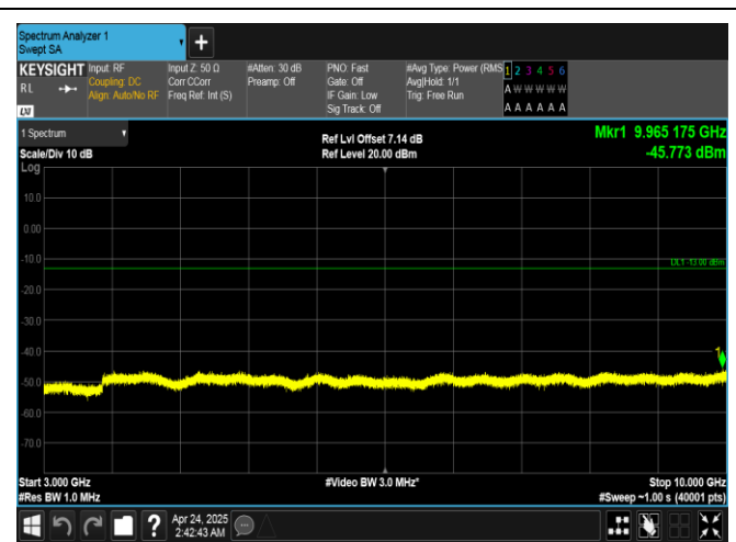
Band26(814-824)-5MHz-QPSK-26740-1RB#0-3000~10000-PASS
