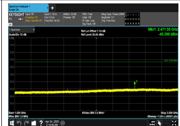
Band26(814-824)-3MHz-16QAM-26775-1RB#14-1000~3000-PASS
