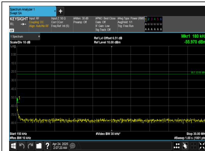
Band26(814-824)-3MHz-16QAM-26740-1RB#14-0.15~30-PASS
