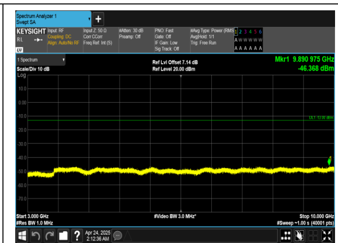
Band26(814-824)-3MHz-16QAM-26775-1RB#0-3000~10000-PASS
