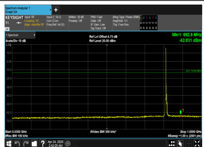
Band26(814-824)-5MHz-QPSK-26740-1RB#0-30~1000-PASS
