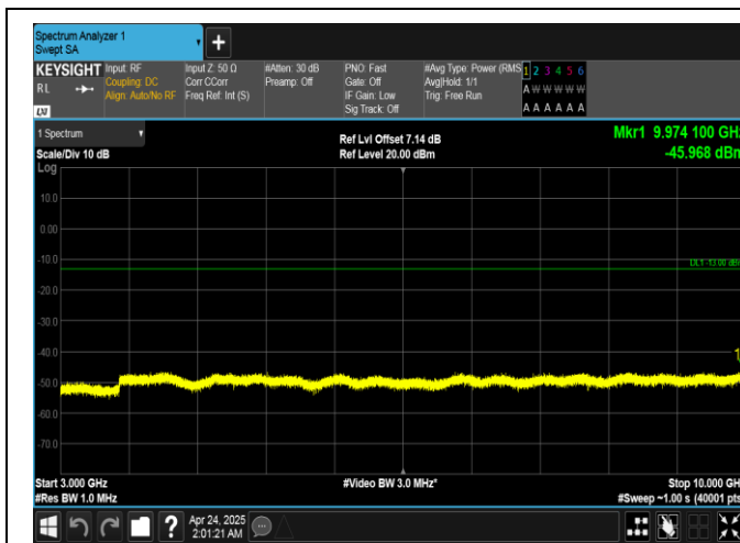
Band26(814-824)-3MHz-16QAM-26705-1RB#14-3000~10000-PASS
