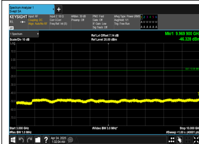
Band26(814-824)-1.4MHz-16QAM-26740-6RB#0-3000~10000-PASS
