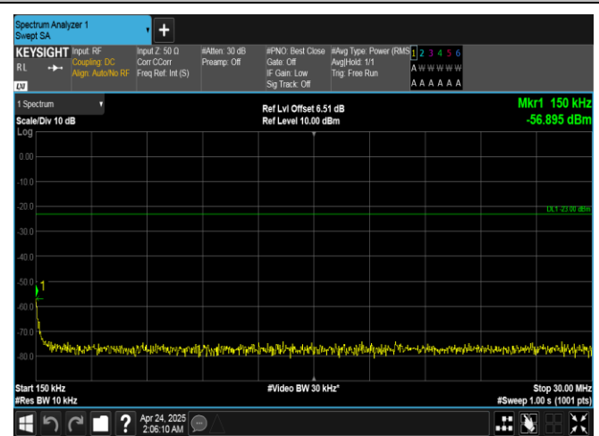
Band26(814-824)-3MHz-QPSK-26740-1RB#14-0.15~30-PASS
