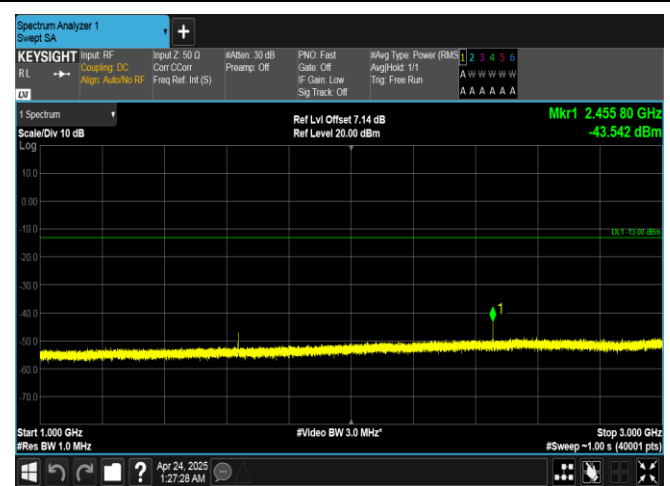
Band26(814-824)-1.4MHz-16QAM-26740-1RB#0-1000~3000-PASS
