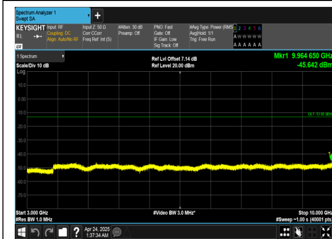
Band26(814-824)-1.4MHz-QPSK-26783-6RB#0-3000~10000-PASS
