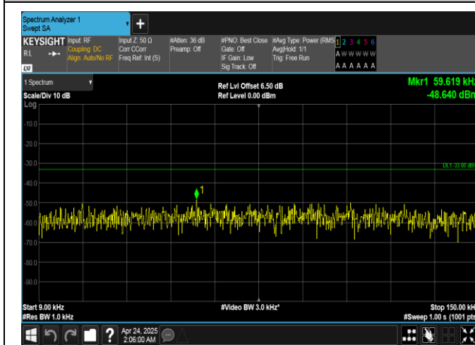
Band26(814-824)-3MHz-QPSK-26740-1RB#14-0.009~0.15-PASS
