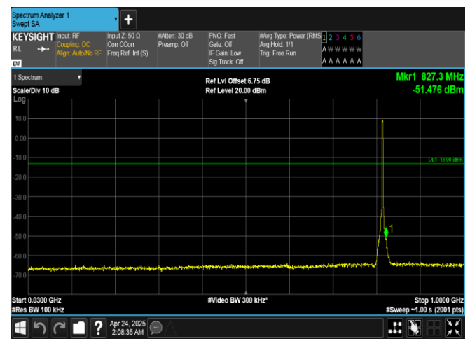
Band26(814-824)-3MHz-QPSK-26740-15RB#0-30~1000-PASS
