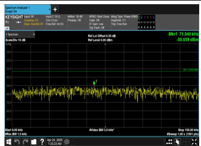
Band26(814-824)-1.4MHz-16QAM-26783-1RB#0-0.009~0.15-PASS
