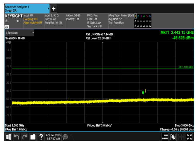
Band26(814-824)-3MHz-QPSK-26705-1RB#0-1000~3000-PASS
