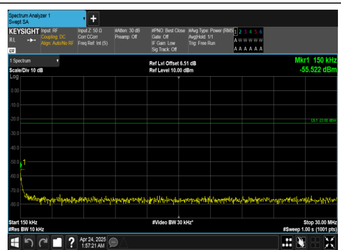
Band26(814-824)-3MHz-QPSK-26705-1RB#0-0.15~30-PASS
