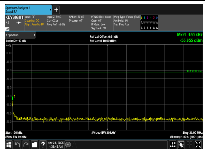
Band26(814-824)-1.4MHz-16QAM-26783-1RB#5-0.15~30-PASS
