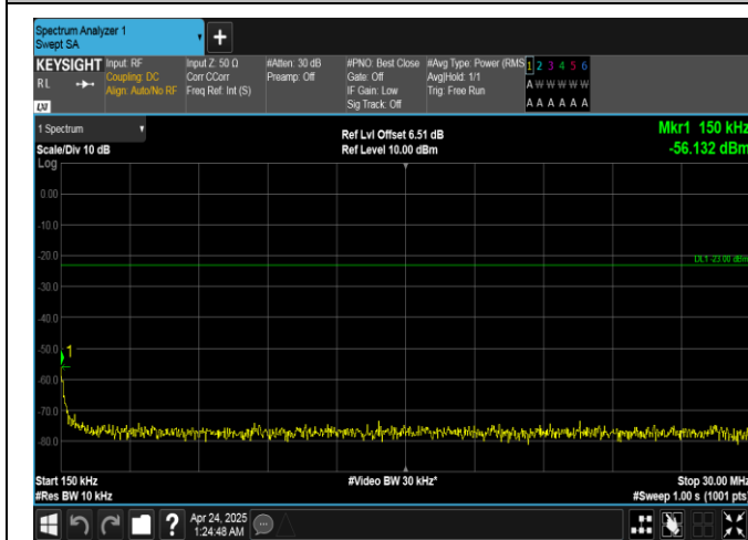
Band26(814-824)-1.4MHz-16QAM-26697-6RB#0-0.15~30-PASS
