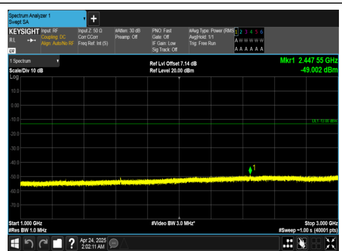
Band26(814-824)-3MHz-QPSK-26705-15RB#0-1000~3000-PASS
