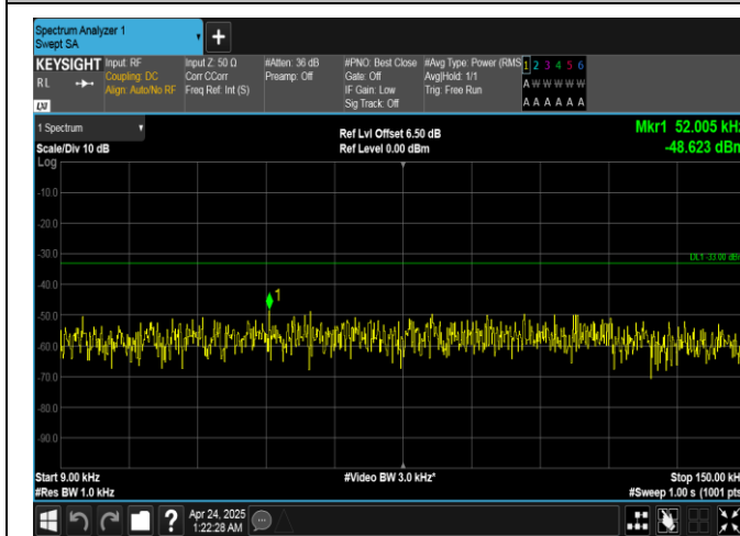
Band26(814-824)-1.4MHz-16QAM-26697-1RB#5-0.009~0.15-PASS
