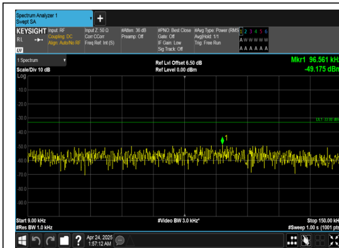
Band26(814-824)-3MHz-QPSK-26705-1RB#0-0.009~0.15-PASS
