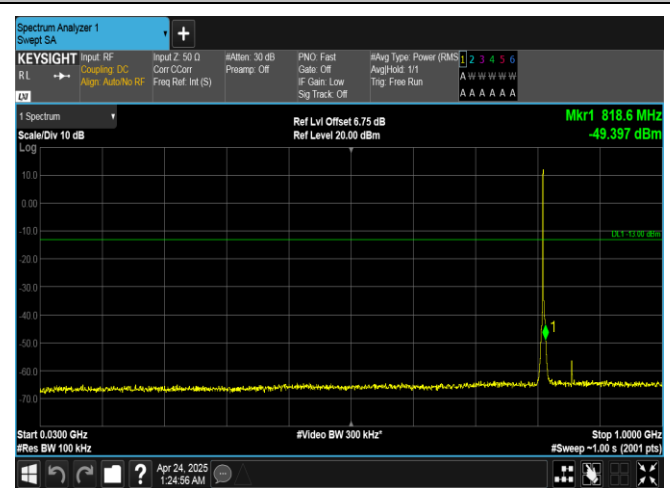
Band26(814-824)-1.4MHz-16QAM-26697-6RB#0-30~1000-PASS
