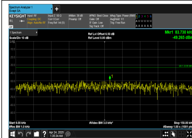
Band26(814-824)-1.4MHz-16QAM-26783-1RB#5-0.009~0.15-PASS
