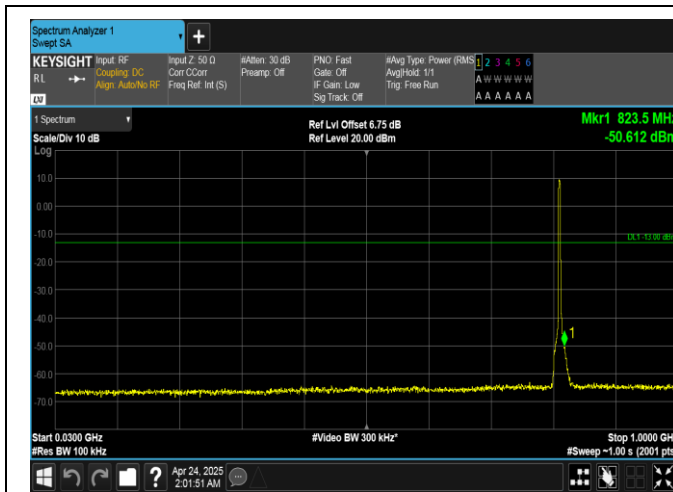
Band26(814-824)-3MHz-QPSK-26705-15RB#0-30~1000-PASS
