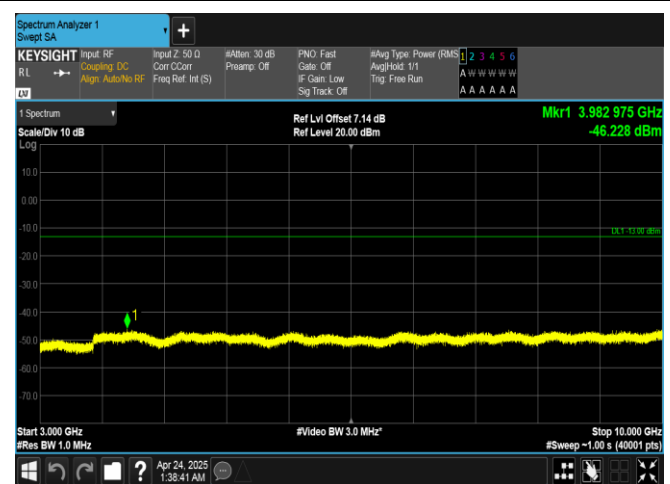
Band26(814-824)-1.4MHz-16QAM-26783-6RB#0-3000~10000-PASS
