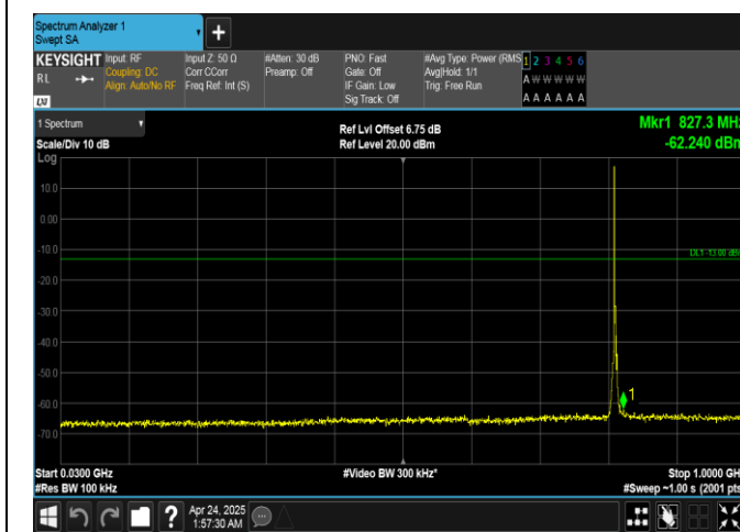
Band26(814-824)-3MHz-QPSK-26705-1RB#0-30~1000-PASS
