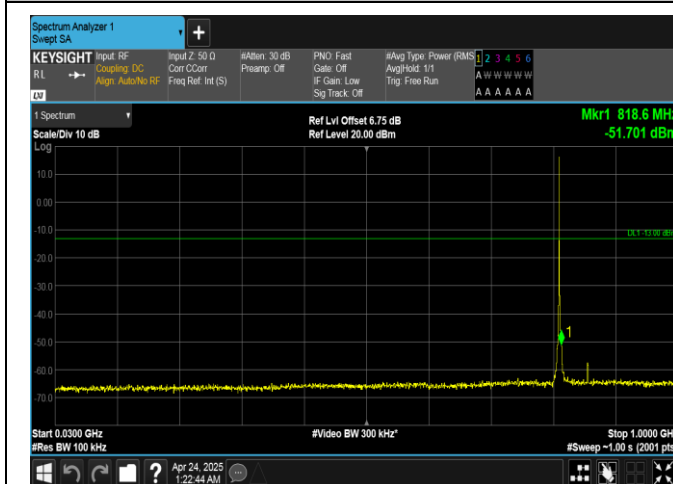
Band26(814-824)-1.4MHz-16QAM-26697-1RB#5-30~1000-PASS
