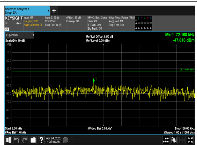
Band26(814-824)-1.4MHz-16QAM-26783-6RB#0-0.009~0.15-PASS
