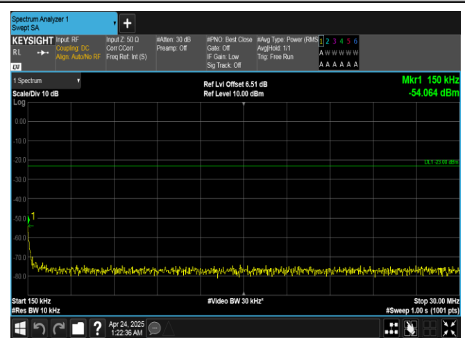
Band26(814-824)-1.4MHz-16QAM-26697-1RB#5-0.15~30-PASS
