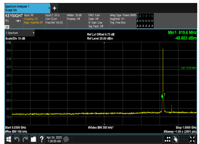
Band26(814-824)-1.4MHz-16QAM-26783-6RB#0-30~1000-PASS
