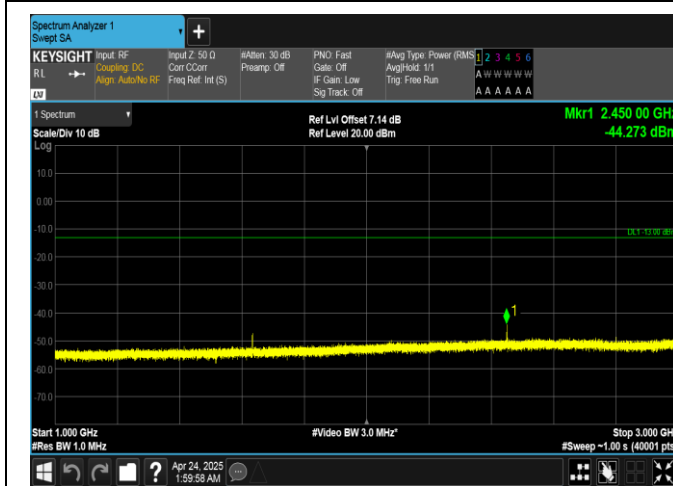
Band26(814-824)-3MHz-QPSK-26705-1RB#14-1000~3000-PASS
