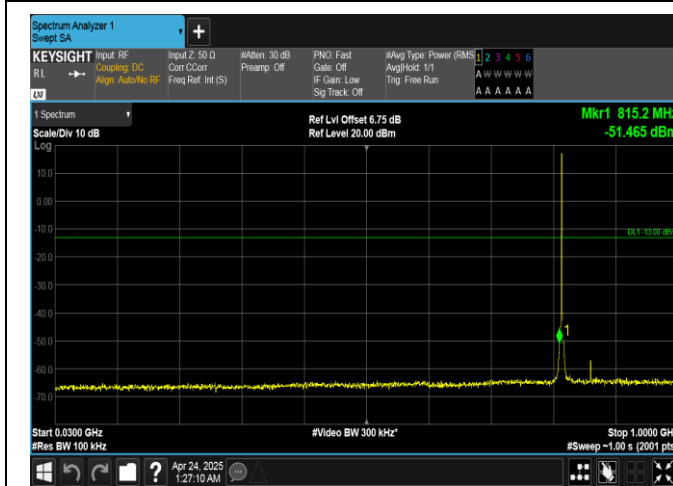
Band26(814-824)-1.4MHz-16QAM-26740-1RB#0-30~1000-PASS
