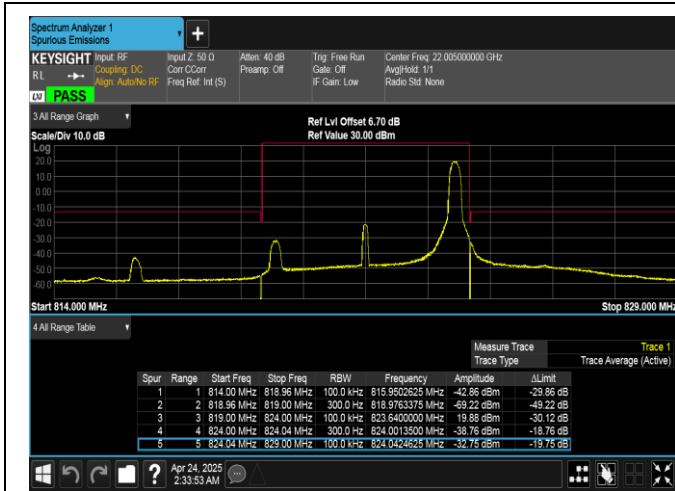
Band26(814-824)-5MHz-QPSK-26765-1RB#24-PASS
