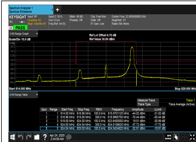
Band26(814-824)-5MHz-16QAM-26765-1RB#24-PASS
