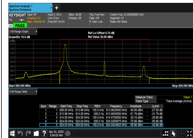
Band26(814-824)-10MHz-QPSK-26740-1RB#0-PASS
