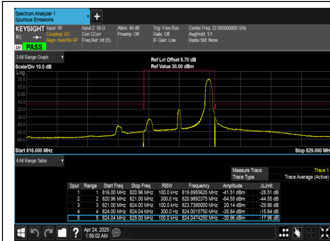
Band26(814-824)-3MHz-QPSK-26775-1RB#14-PASS
