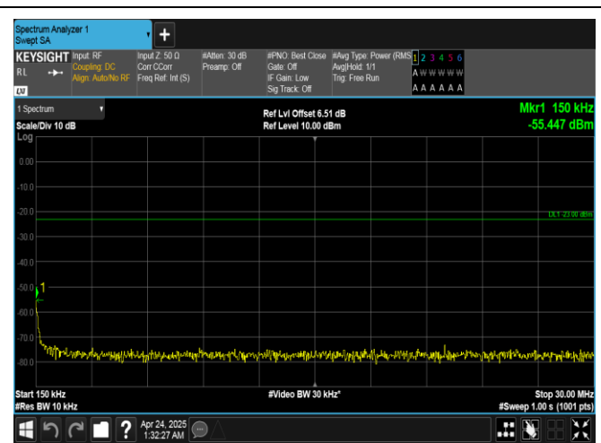
Band26(814-824)-1.4MHz-QPSK-26783-1RB#0-0.15~30-PASS
