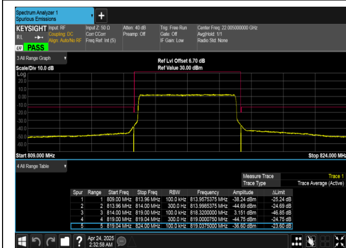
Band26(814-824)-5MHz-16QAM-26715-25RB#0-PASS
