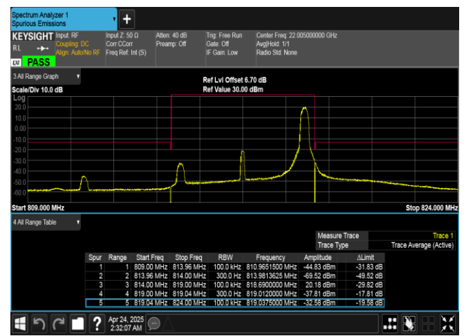
Band26(814-824)-5MHz-QPSK-26715-1RB#24-PASS
