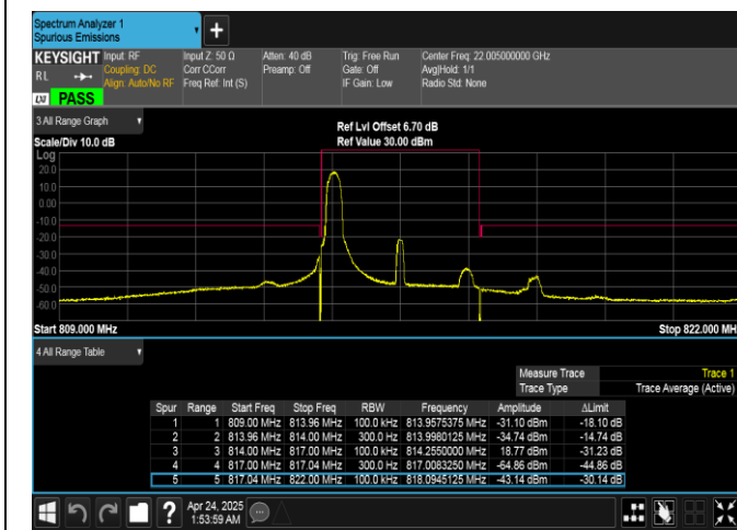
Band26(814-824)-3MHz-16QAM-26705-1RB#0-PASS
