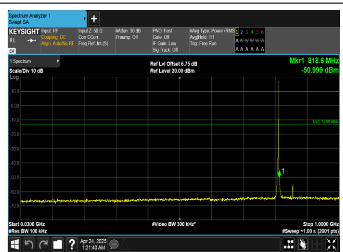
Band26(814-824)-1.4MHz-QPSK-26697-1RB#5-30~1000-PASS
