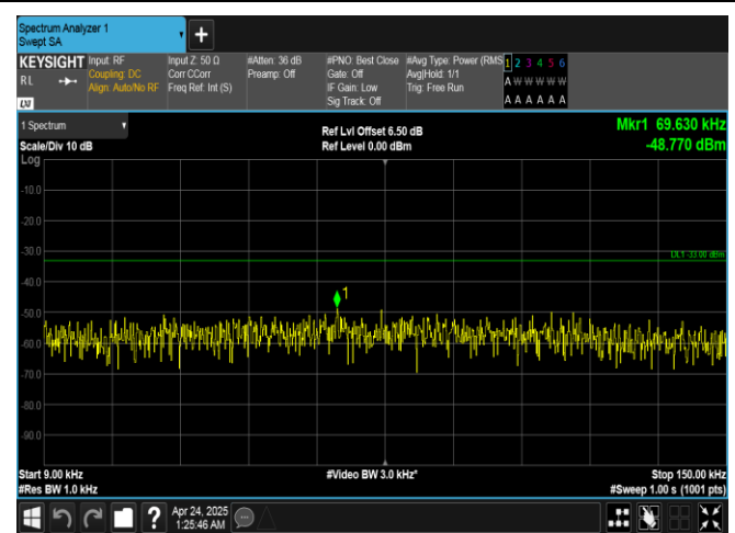
Band26(814-824)-1.4MHz-QPSK-26740-1RB#0-0.009~0.15-PASS
