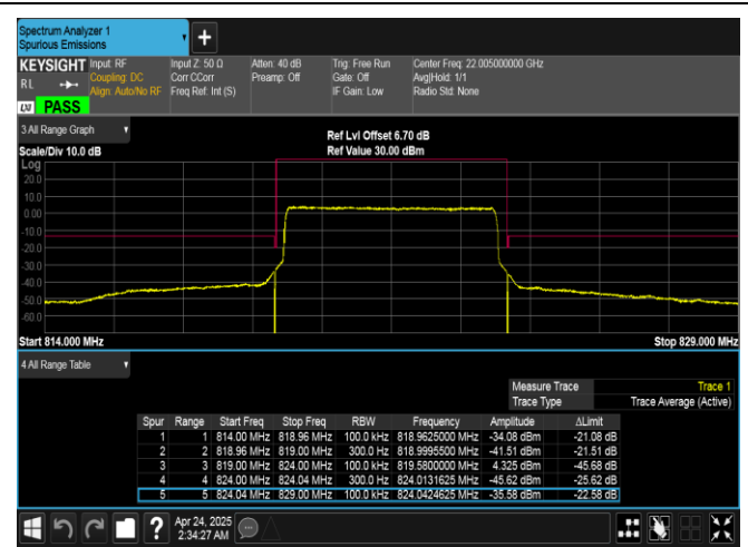
Band26(814-824)-5MHz-QPSK-26765-25RB#0-PASS
