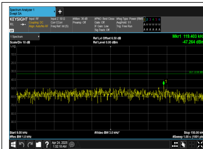
Band26(814-824)-1.4MHz-QPSK-26783-1RB#0-0.009~0.15-PASS
