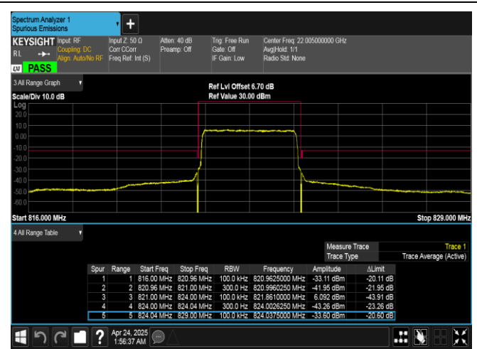
Band26(814-824)-3MHz-QPSK-26775-15RB#0-PASS
