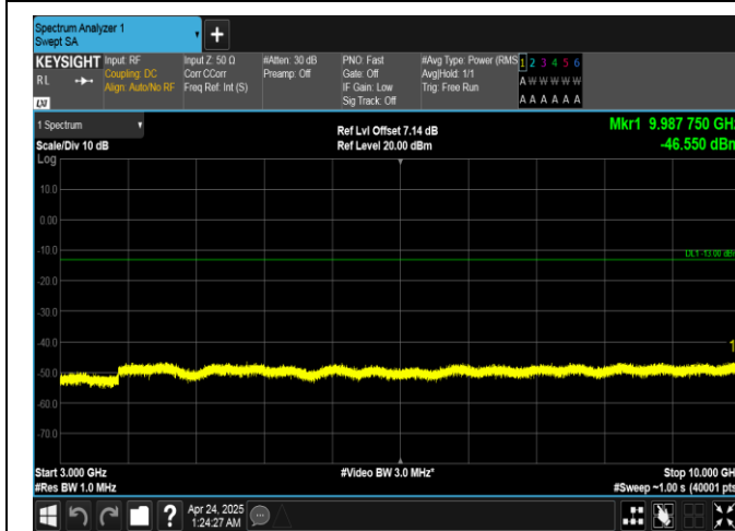
Band26(814-824)-1.4MHz-QPSK-26697-6RB#0-3000~10000-PASS
