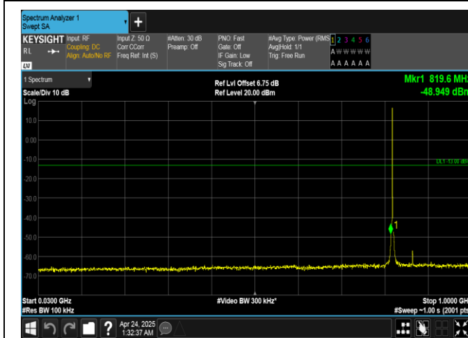
Band26(814-824)-1.4MHz-QPSK-26783-1RB#0-30~1000-PASS
