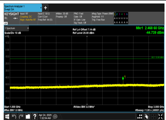
Band26(814-824)-1.4MHz-QPSK-26783-1RB#0-1000~3000-PASS
