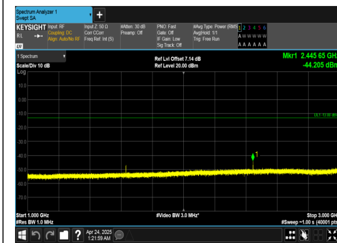
Band26(814-824)-1.4MHz-QPSK-26697-1RB#5-1000~3000-PASS
