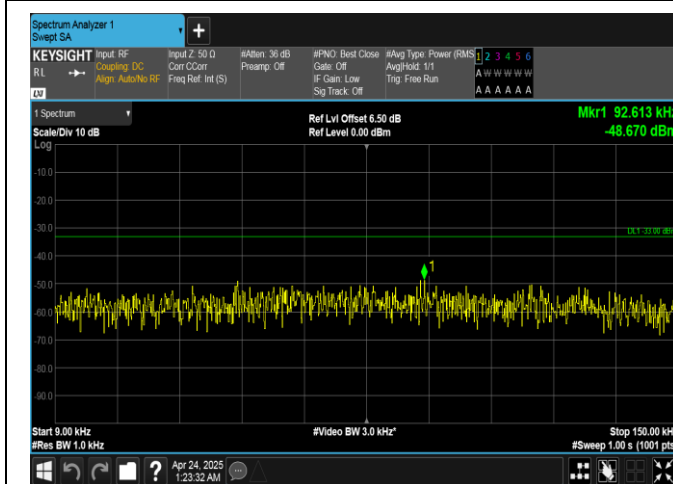
Band26(814-824)-1.4MHz-QPSK-26697-6RB#0-0.009~0.15-PASS
