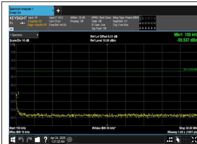
Band26(814-824)-1.4MHz-QPSK-26697-1RB#5-0.15~30-PASS
