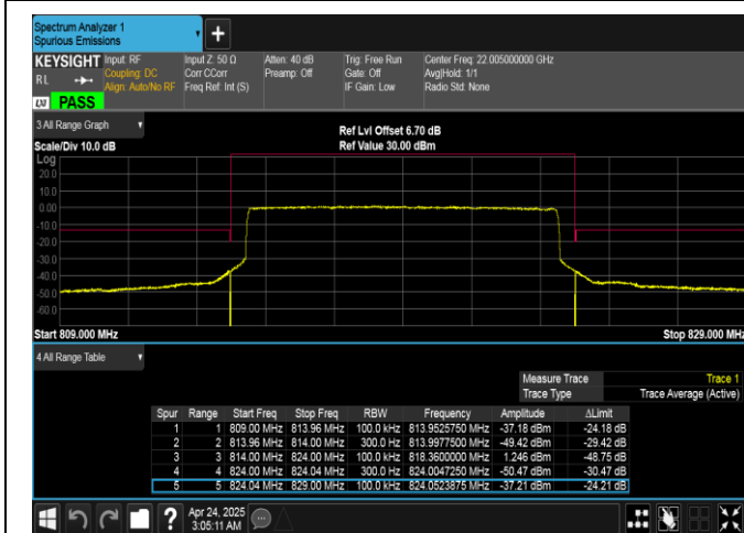
Band26(814-824)-10MHz-QPSK-26740-50RB#0-PASS
