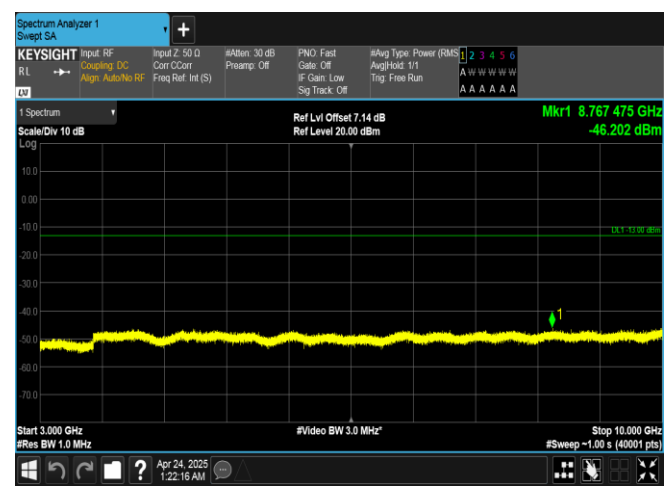
Band26(814-824)-1.4MHz-QPSK-26697-1RB#5-3000~10000-PASS
