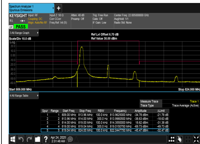
Band26(814-824)-5MHz-16QAM-26715-1RB#0-PASS
