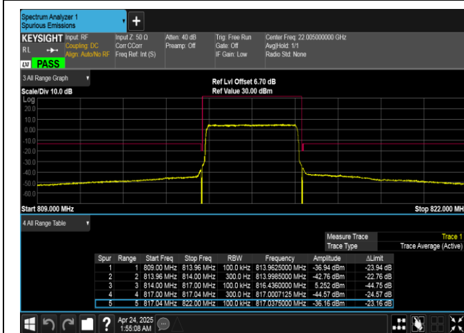
Band26(814-824)-3MHz-16QAM-26705-15RB#0-PASS
