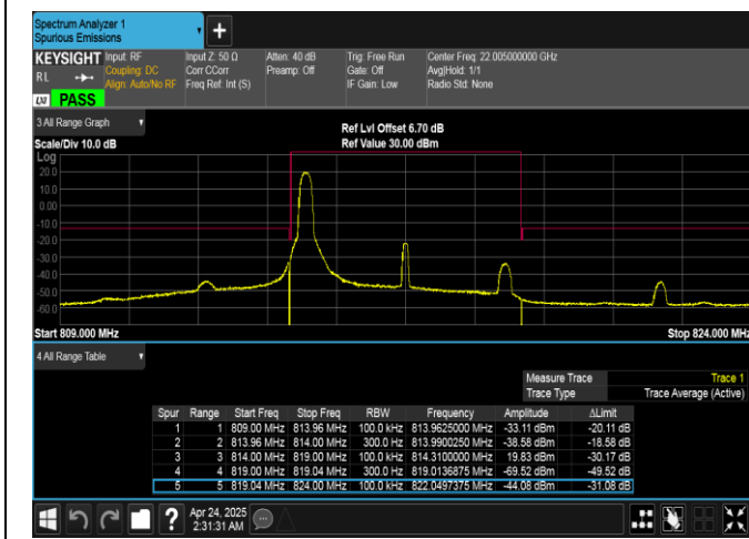
Band26(814-824)-5MHz-QPSK-26715-1RB#0-PASS
