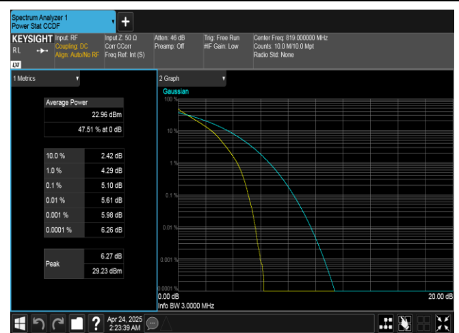
Band26(814-824)-3MHz-QPSK-26740-15RB#0-PASS
