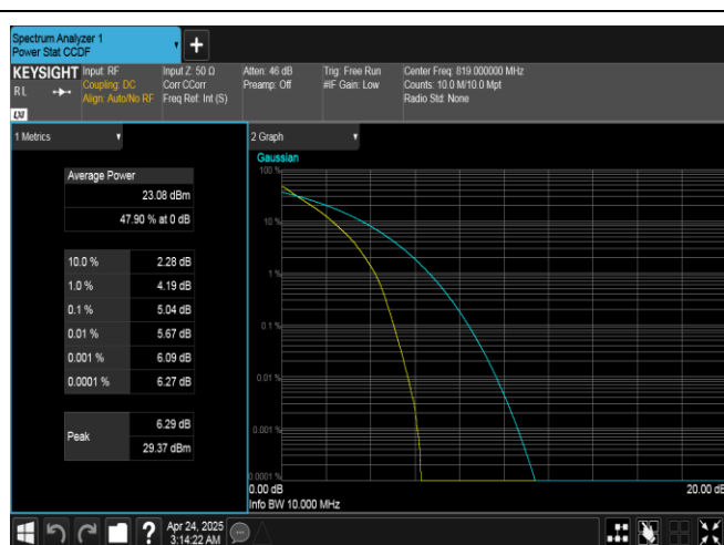
Band26(814-824)-10MHz-QPSK-26740-50RB#0-PASS
