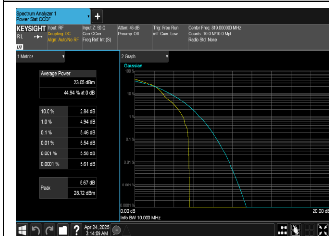
Band26(814-824)-10MHz-16QAM-26740-1RB#0-PASS
