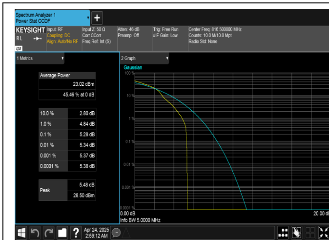
Band26(814-824)-5MHz-16QAM-26715-1RB#0-PASS
