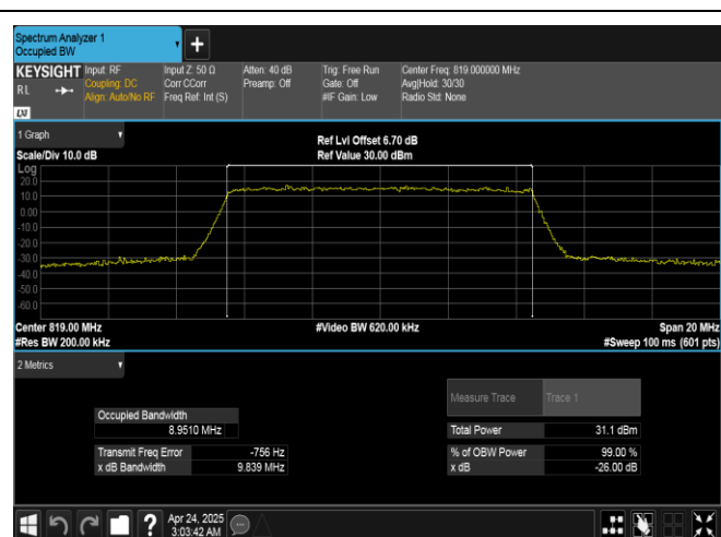
Band26(814-824)-10MHz-16QAM-26740-50RB#0-PASS
