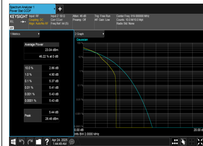
Band26(814-824)-1.4MHz-16QAM-26740-1RB#0-PASS
