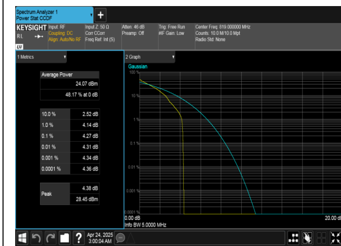
Band26(814-824)-5MHz-QPSK-26740-1RB#0-PASS
