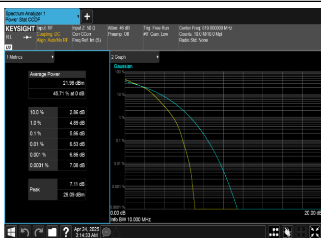
Band26(814-824)-10MHz-16QAM-26740-50RB#0-PASS
