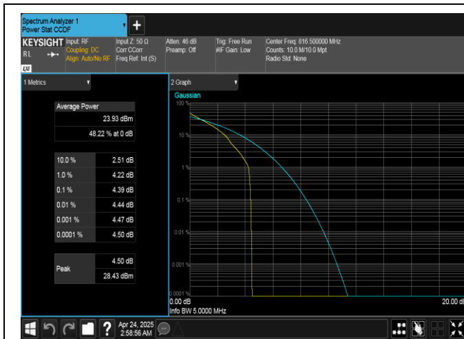
Band26(814-824)-5MHz-QPSK-26715-1RB#0-PASS
