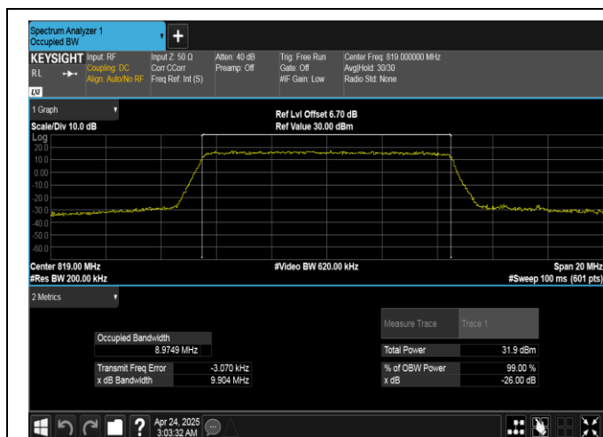
Band26(814-824)-10MHz-QPSK-26740-50RB#0-PASS
