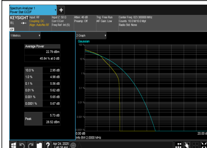
Band26(814-824)-1.4MHz-16QAM-26783-1RB#0-PASS
