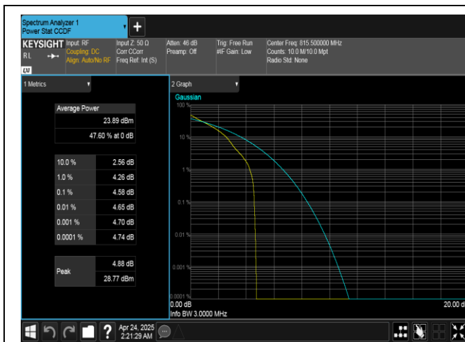
Band26(814-824)-3MHz-QPSK-26705-1RB#0-PASS
