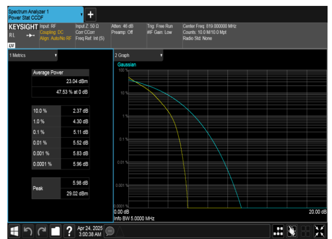
Band26(814-824)-5MHz-QPSK-26740-25RB#0-PASS
