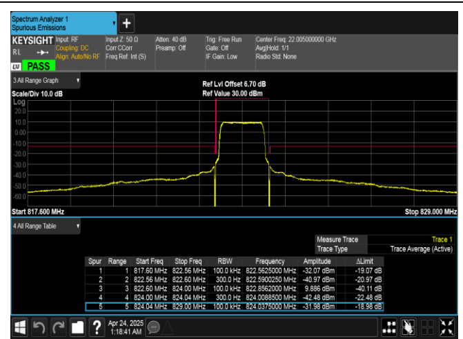
Band26(814-824)-1.4MHz-QPSK-26783-6RB#0-PASS
