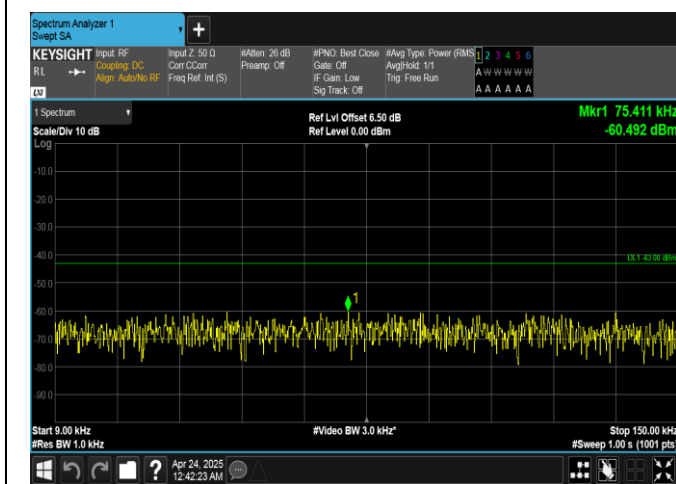
Band25-20MHz-16QAM-26590-1RB#99-0.009~0.15-PASS
