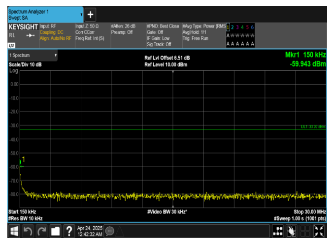
Band25-20MHz-16QAM-26590-1RB#99-0.15~30-PASS
