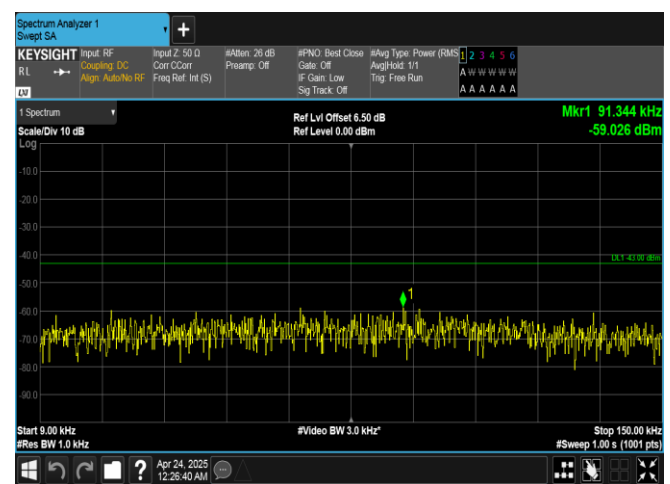
Band25-20MHz-16QAM-26140-1RB#0-0.009~0.15-PASS
