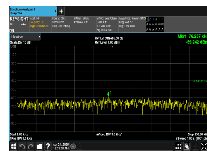
Band25-20MHz-16QAM-26365-1RB#0-0.009~0.15-PASS
