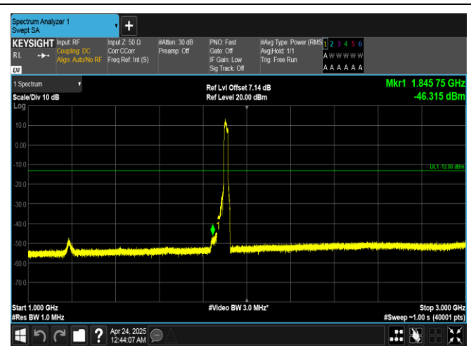
Band25-20MHz-QPSK-26590-100RB#0-1000~3000-PASS
