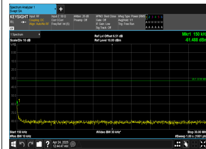
Band25-20MHz-16QAM-26590-100RB#0-0.15~30-PASS
