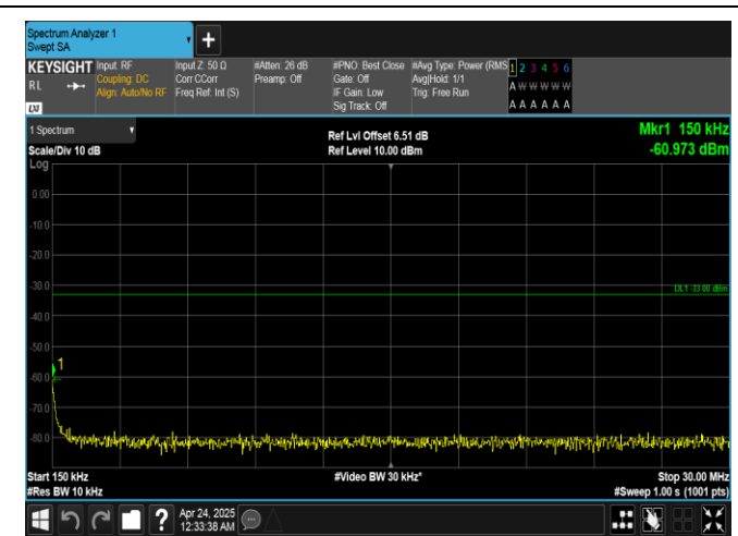
Band25-20MHz-16QAM-26365-1RB#0-0.15~30-PASS
