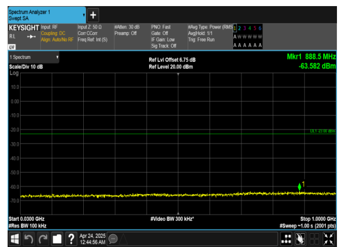
Band25-20MHz-16QAM-26590-100RB#0-30~1000-PASS
