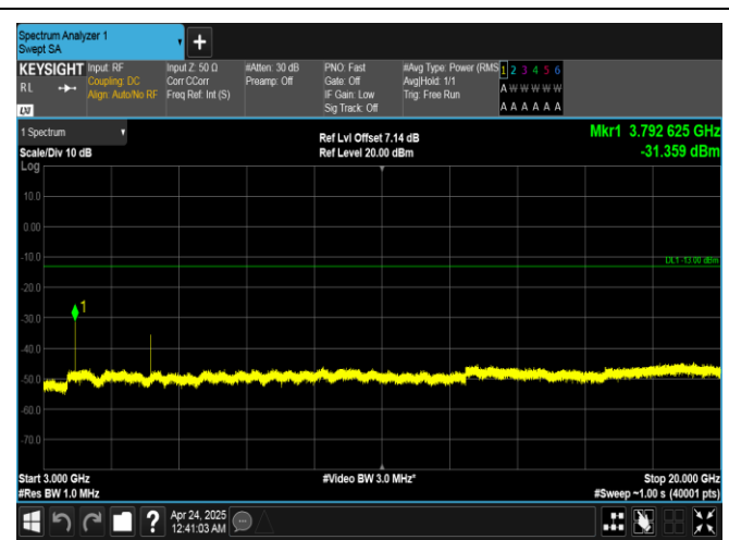
Band25-20MHz-16QAM-26590-1RB#0-3000~20000-PASS
