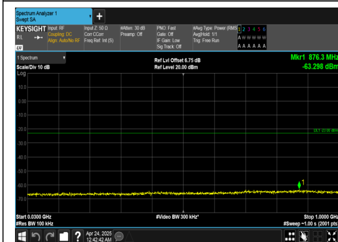
Band25-20MHz-16QAM-26590-1RB#99-30~1000-PASS
