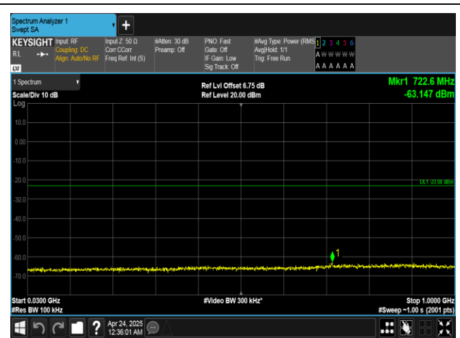
Band25-20MHz-16QAM-26365-1RB#99-30~1000-PASS
