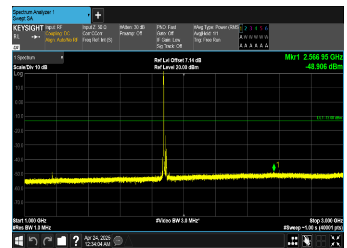
Band25-20MHz-16QAM-26365-1RB#0-1000~3000-PASS
