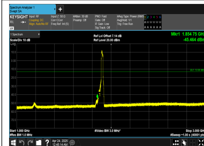
Band25-20MHz-16QAM-26590-100RB#0-1000~3000-PASS
