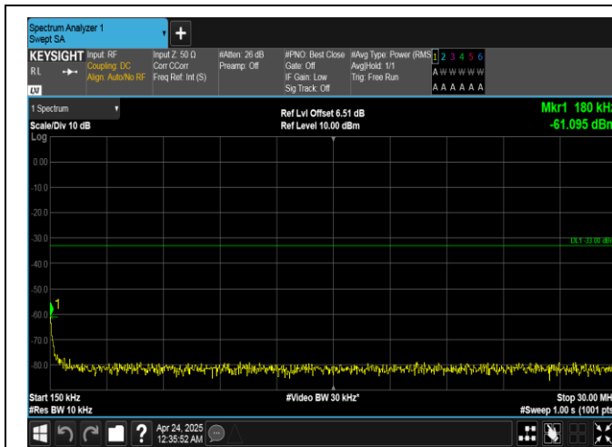
Band25-20MHz-16QAM-26365-1RB#99-0.15~30-PASS
