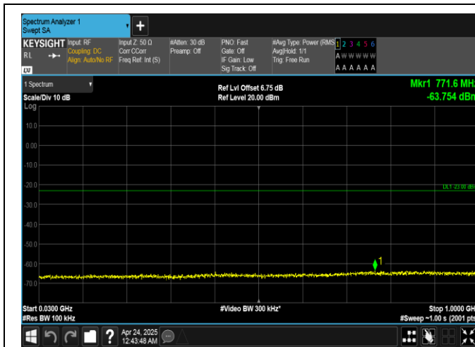
Band25-20MHz-QPSK-26590-100RB#0-30~1000-PASS
