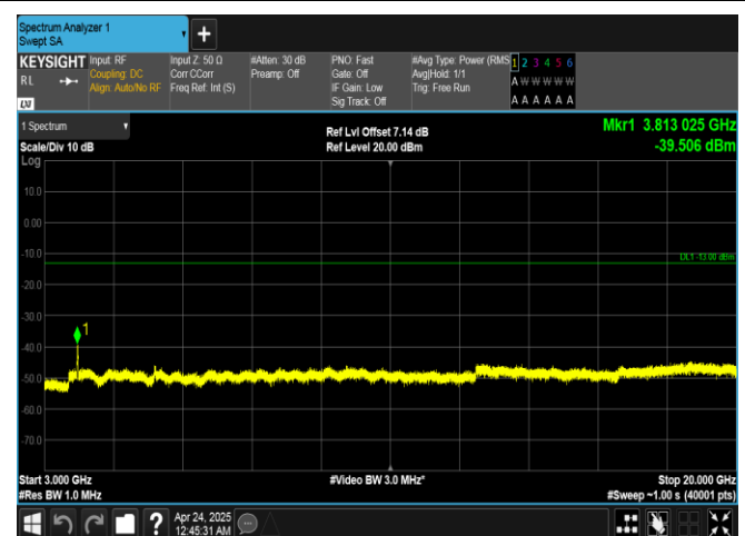
Band25-20MHz-16QAM-26590-100RB#0-3000~20000-PASS
