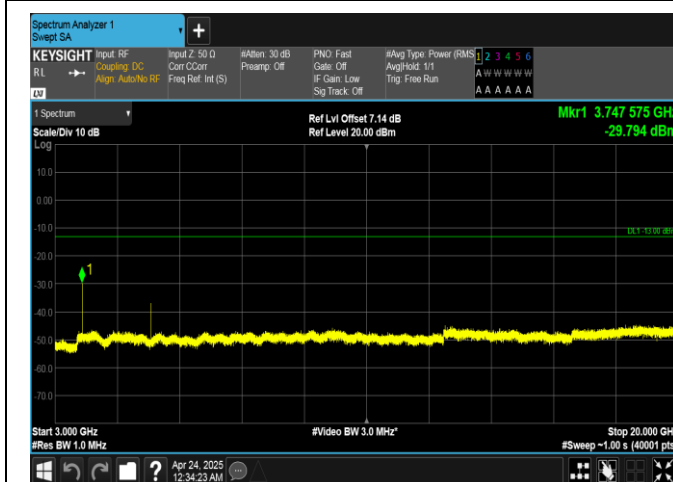
Band25-20MHz-16QAM-26365-1RB#0-3000~20000-PASS
