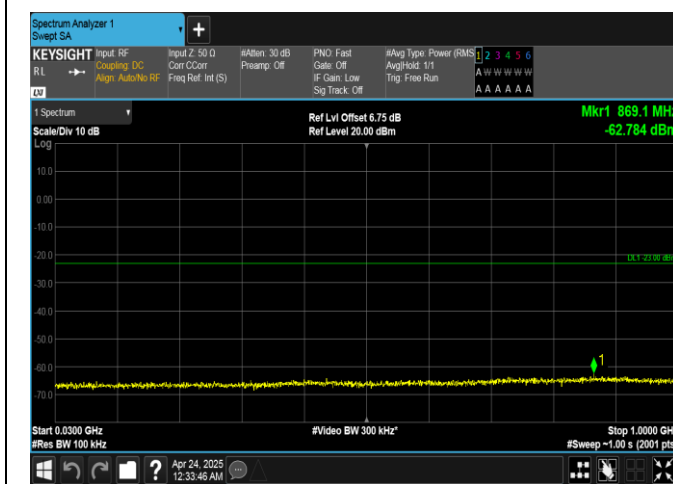
Band25-20MHz-16QAM-26365-1RB#0-30~1000-PASS
