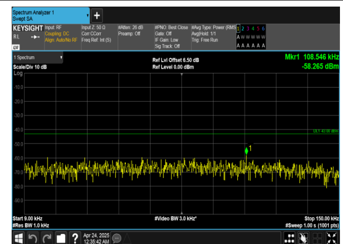
Band25-20MHz-16QAM-26365-1RB#99-0.009~0.15-PASS
