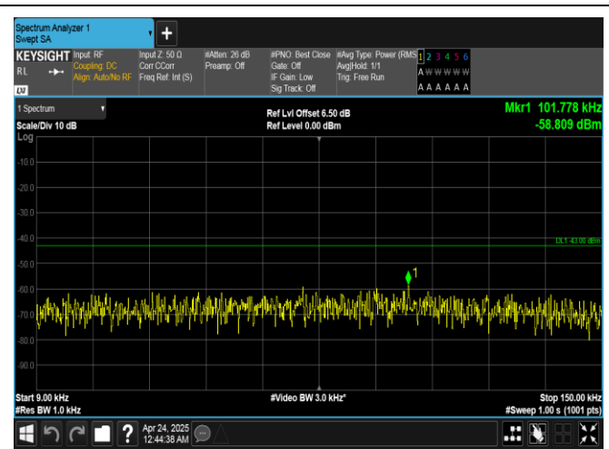
Band25-20MHz-16QAM-26590-100RB#0-0.009~0.15-PASS
