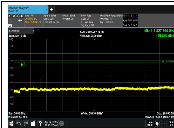
Band25-20MHz-16QAM-26590-1RB#99-3000~20000-PASS
