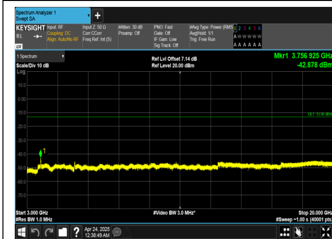
Band25-20MHz-16QAM-26365-100RB#0-3000~20000-PASS
