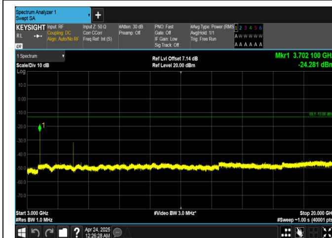
Band25-20MHz-QPSK-26140-1RB#0-3000~20000-PASS
