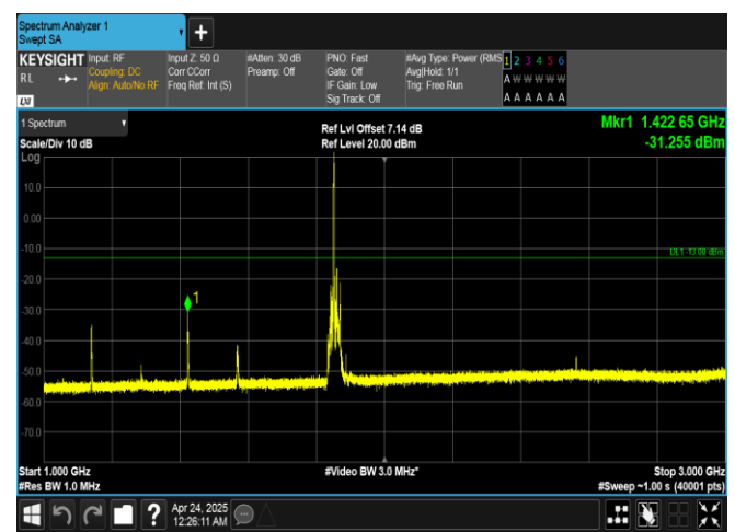
Band25-20MHz-QPSK-26140-1RB#0-1000~3000-PASS
