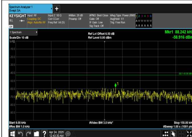
Band25-20MHz-QPSK-26590-100RB#0-0.009~0.15-PASS
