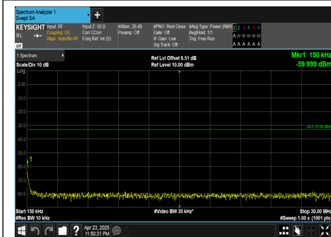
Band25-15MHz-16QAM-26615-1RB#0-0.15~30-PASS
