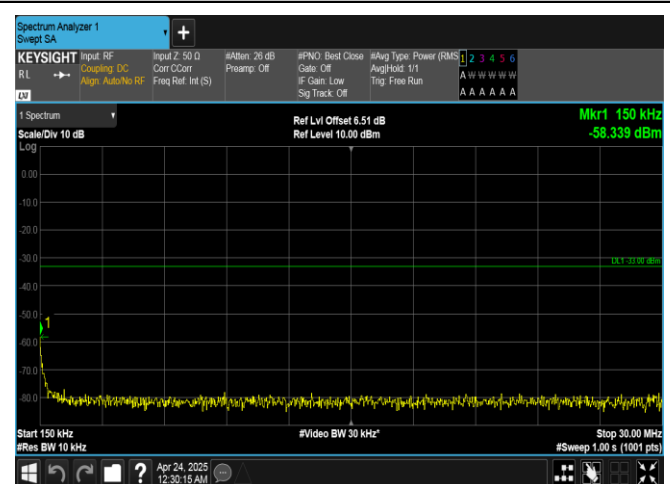
Band25-20MHz-QPSK-26140-100RB#0-0.15~30-PASS
