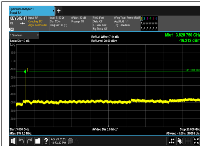
Band25-15MHz-16QAM-26615-1RB#74-3000~20000-PASS
