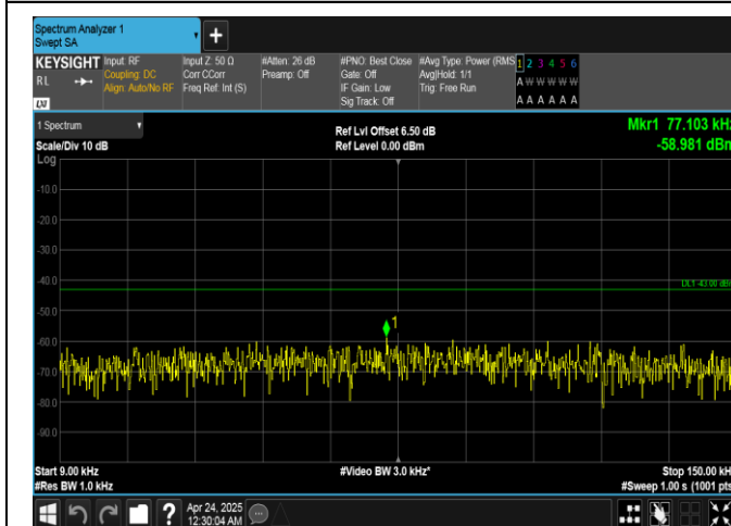
Band25-20MHz-QPSK-26140-100RB#0-0.009~0.15-PASS
