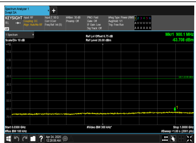
Band25-20MHz-QPSK-26140-1RB#99-30~1000-PASS
