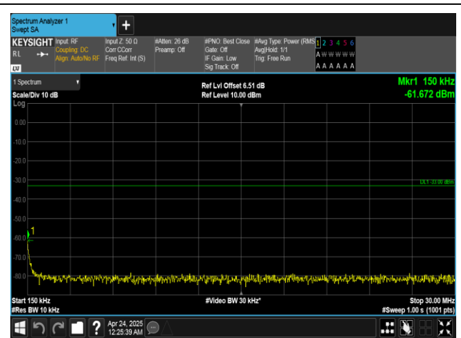
Band25-20MHz-QPSK-26140-1RB#0-0.15~30-PASS
