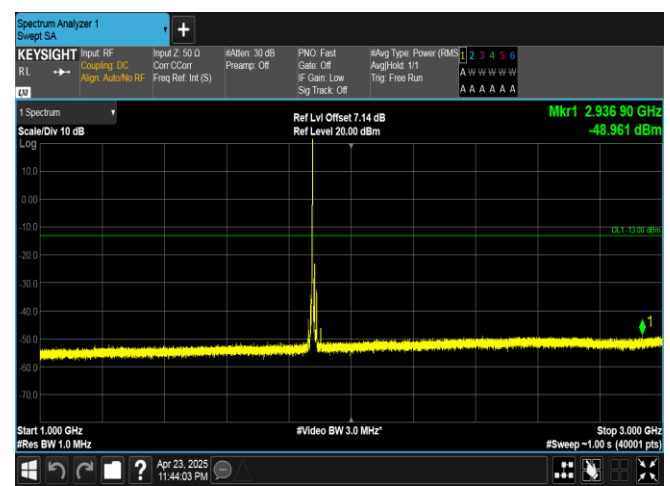
Band25-15MHz-16QAM-26365-1RB#0-1000~3000-PASS
