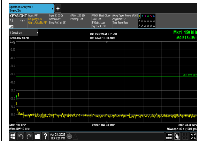
Band25-15MHz-16QAM-26115-75RB#0-0.15~30-PASS
