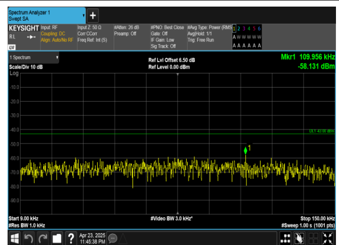
Band25-15MHz-16QAM-26365-1RB#74-0.009~0.15-PASS
