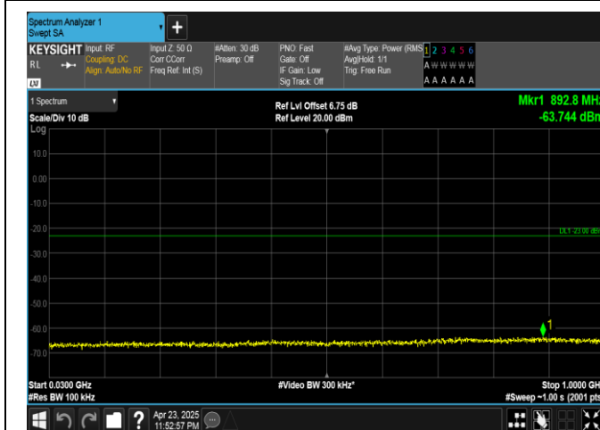
Band25-15MHz-16QAM-26615-1RB#74-30~1000-PASS
