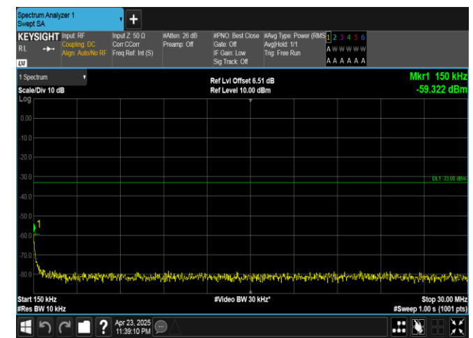
Band25-15MHz-16QAM-26115-1RB#74-0.15~30-PASS
