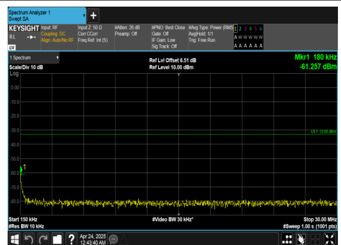
Band25-20MHz-QPSK-26590-100RB#0-0.15~30-PASS
