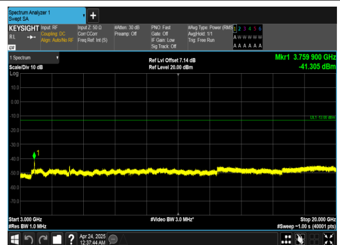
Band25-20MHz-QPSK-26365-100RB#0-3000~20000-PASS
