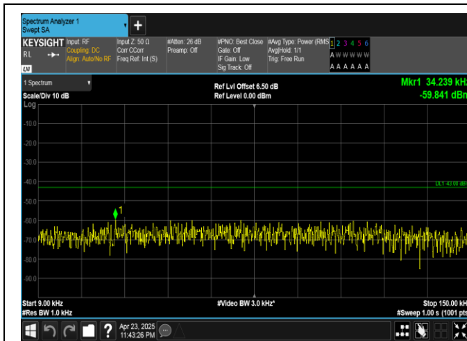
Band25-15MHz-16QAM-26365-1RB#0-0.009~0.15-PASS
