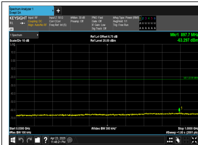
Band25-15MHz-16QAM-26365-75RB#0-30~1000-PASS
