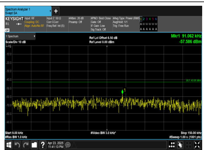
Band25-15MHz-16QAM-26115-75RB#0-0.009~0.15-PASS
