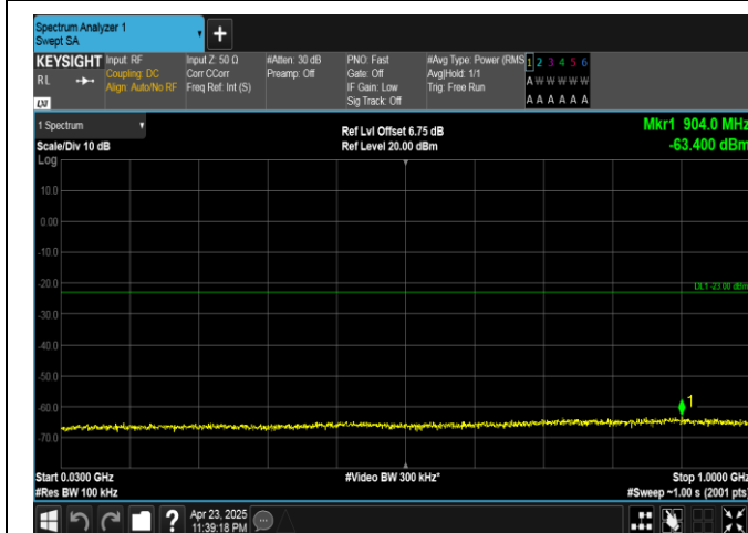
Band25-15MHz-16QAM-26115-1RB#74-30~1000-PASS
