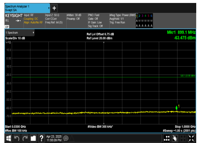
Band25-15MHz-16QAM-26615-75RB#0-30~1000-PASS
