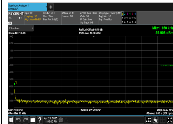
Band25-15MHz-16QAM-26615-75RB#0-0.15~30-PASS
