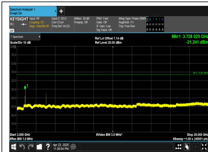
Band25-15MHz-16QAM-26115-1RB#74-3000~20000-PASS
