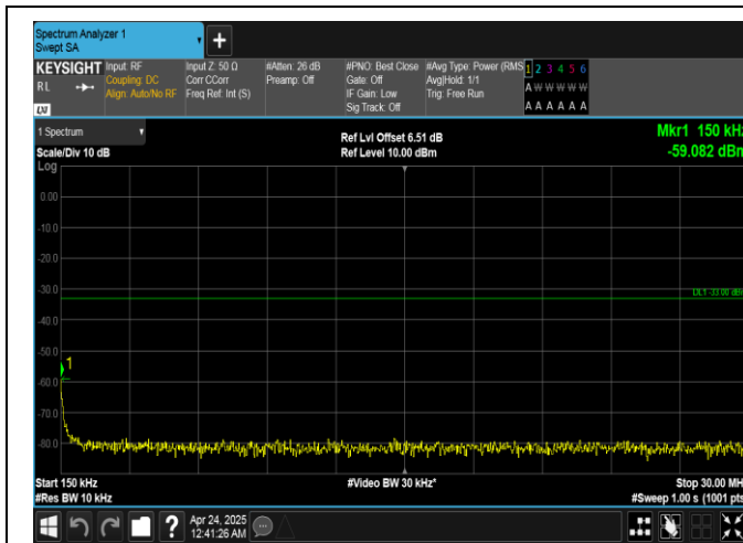
Band25-20MHz-QPSK-26590-1RB#99-0.15~30-PASS
