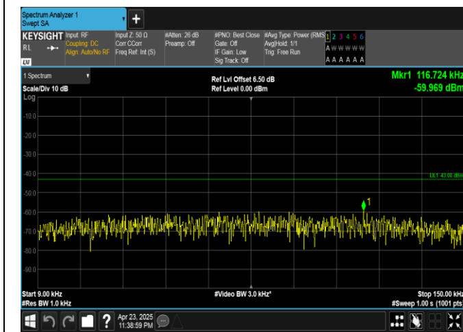
Band25-15MHz-16QAM-26115-1RB#74-0.009~0.15-PASS
