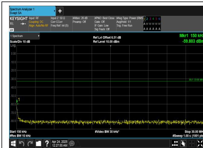
Band25-20MHz-QPSK-26140-1RB#99-0.15~30-PASS
