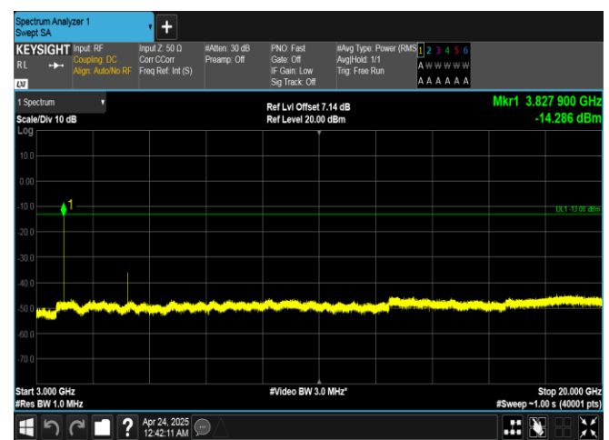
Band25-20MHz-QPSK-26590-1RB#99-3000~20000-PASS
