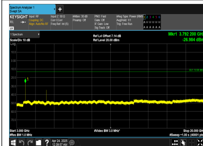
Band25-20MHz-QPSK-26590-1RB#0-3000~20000-PASS
