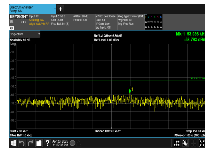
Band25-15MHz-16QAM-26615-1RB#74-0.009~0.15-PASS
