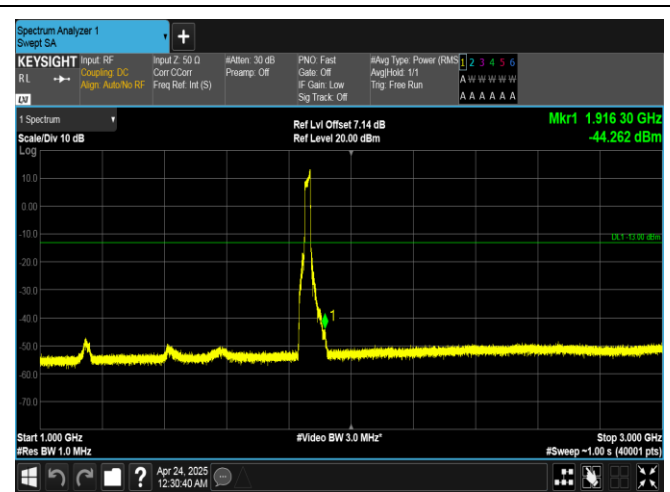
Band25-20MHz-QPSK-26140-100RB#0-1000~3000-PASS
