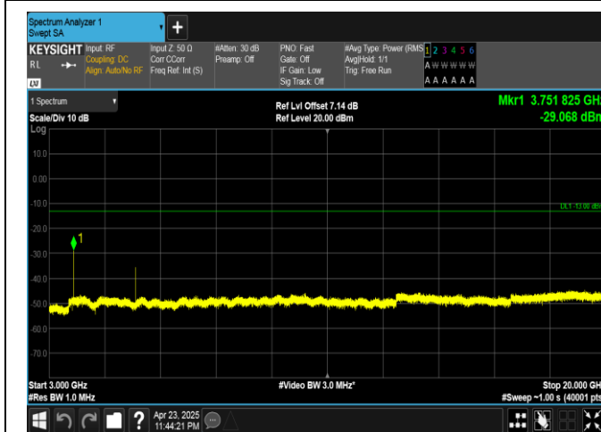
Band25-15MHz-16QAM-26365-1RB#0-3000~20000-PASS
