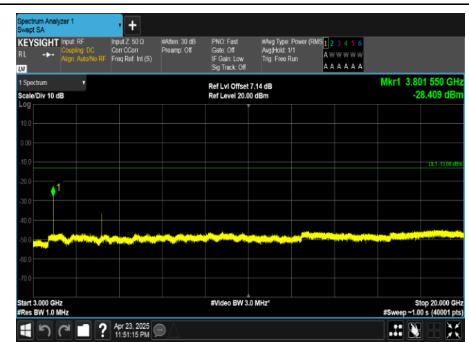
Band25-15MHz-16QAM-26615-1RB#0-3000~20000-PASS
