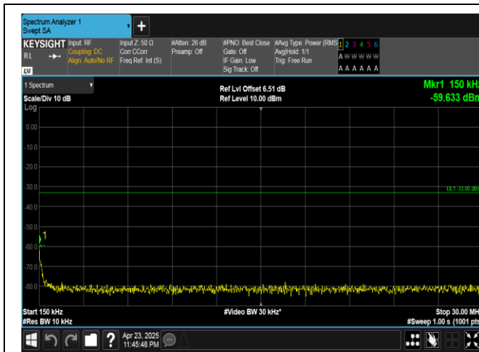
Band25-15MHz-16QAM-26365-1RB#74-0.15~30-PASS
