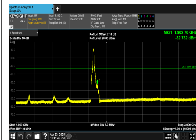
Band25-15MHz-16QAM-26115-75RB#0-1000~3000-PASS
