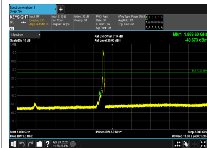
Band25-15MHz-16QAM-26615-75RB#0-1000~3000-PASS
