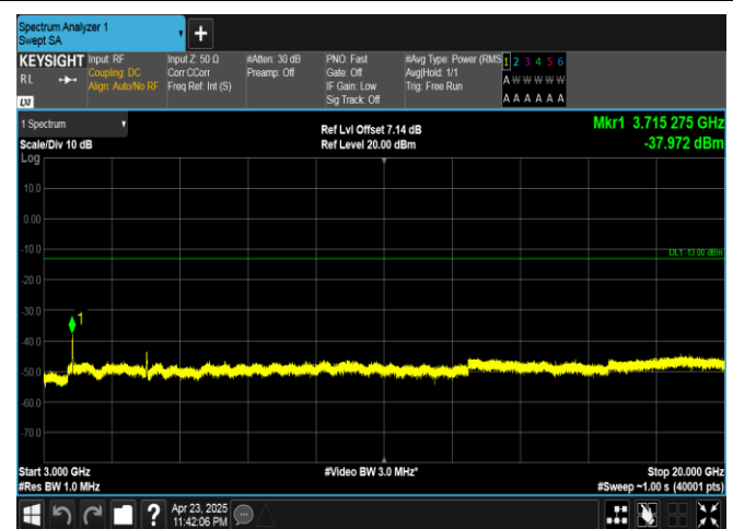
Band25-15MHz-16QAM-26115-75RB#0-3000~20000-PASS
