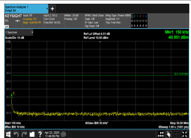
Band25-15MHz-16QAM-26365-75RB#0-0.15~30-PASS
