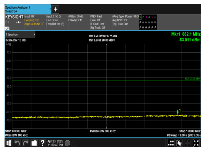
Band25-15MHz-16QAM-26615-1RB#0-30~1000-PASS
