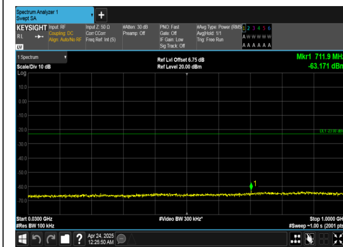
Band25-20MHz-QPSK-26140-1RB#0-30~1000-PASS
