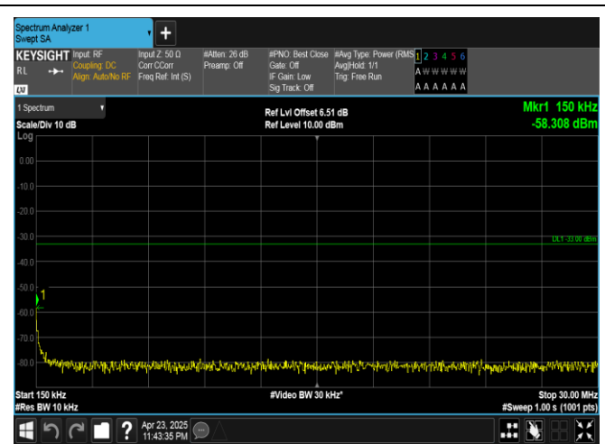
Band25-15MHz-16QAM-26365-1RB#0-0.15~30-PASS
