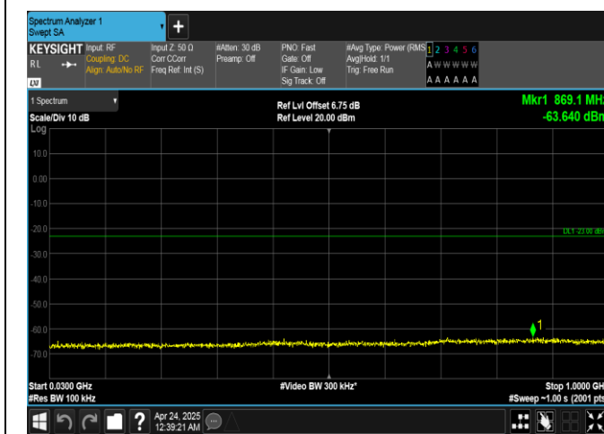
Band25-20MHz-QPSK-26590-1RB#0-30~1000-PASS
