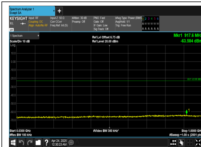
Band25-20MHz-QPSK-26140-100RB#0-30~1000-PASS
