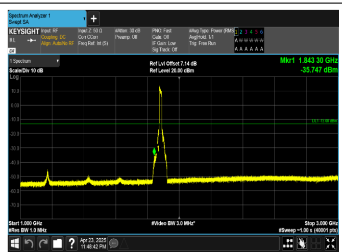
Band25-15MHz-16QAM-26365-75RB#0-1000~3000-PASS
