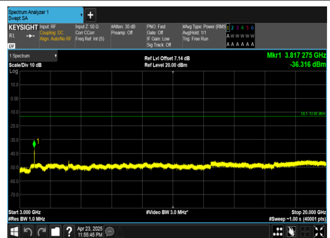
Band25-15MHz-16QAM-26615-75RB#0-3000~20000-PASS
