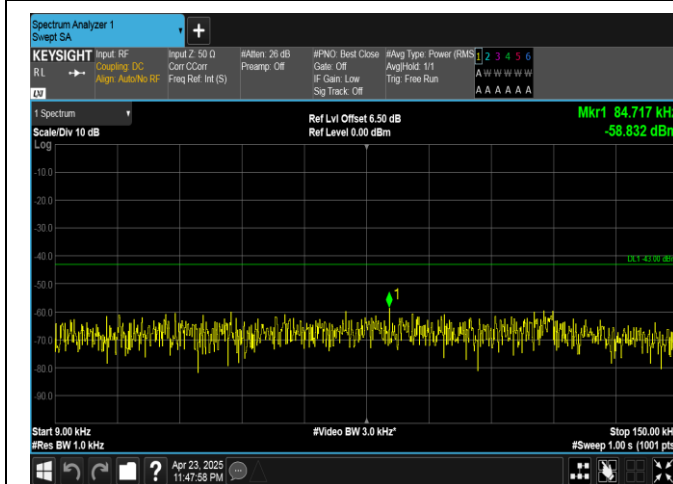
Band25-15MHz-16QAM-26365-75RB#0-0.009~0.15-PASS
