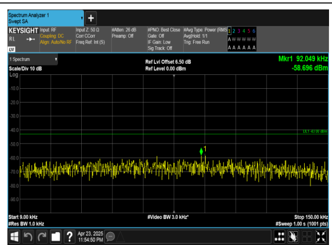
Band25-15MHz-16QAM-26615-75RB#0-0.009~0.15-PASS
