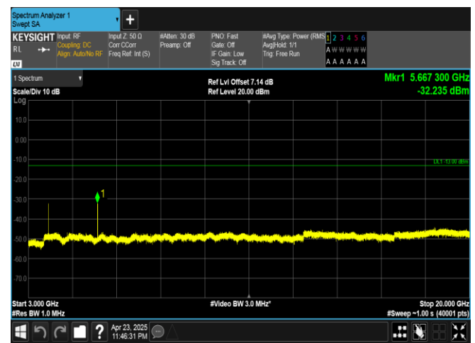
Band25-15MHz-16QAM-26365-1RB#74-3000~20000-PASS
