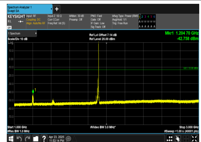
Band25-15MHz-16QAM-26615-1RB#74-1000~3000-PASS
