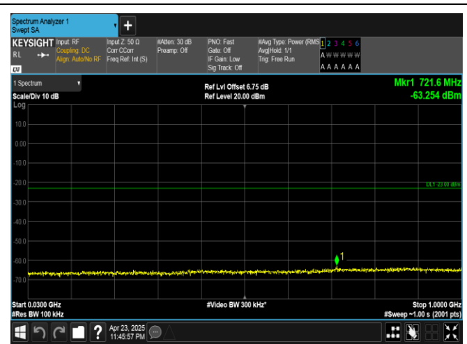
Band25-15MHz-16QAM-26365-1RB#74-30~1000-PASS
