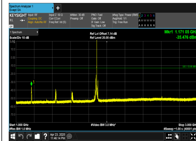
Band25-15MHz-16QAM-26365-1RB#74-1000~3000-PASS
