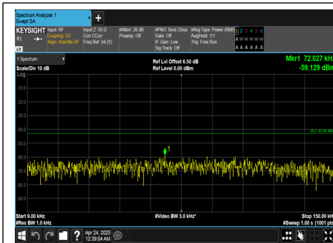
Band25-20MHz-QPSK-26590-1RB#0-0.009~0.15-PASS
