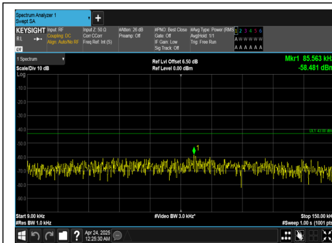
Band25-20MHz-QPSK-26140-1RB#0-0.009~0.15-PASS
