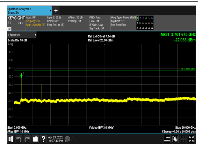
Band25-15MHz-16QAM-26115-1RB#0-3000~20000-PASS
