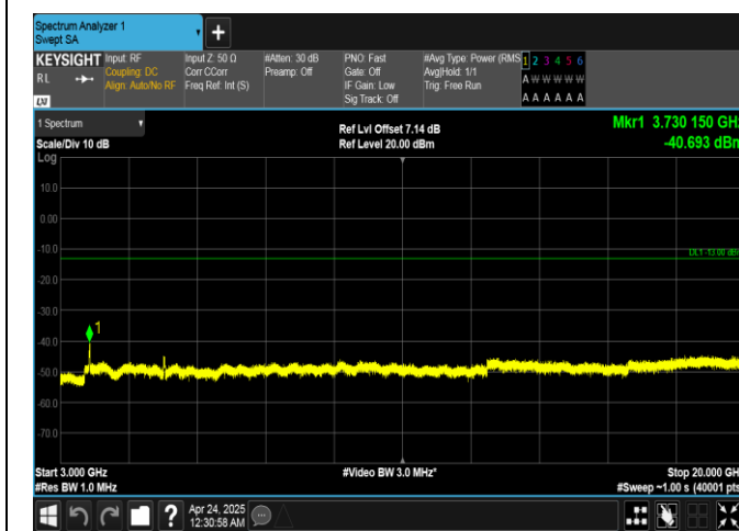
Band25-20MHz-QPSK-26140-100RB#0-3000~20000-PASS
