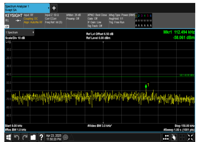
Band25-15MHz-16QAM-26615-1RB#0-0.009~0.15-PASS
