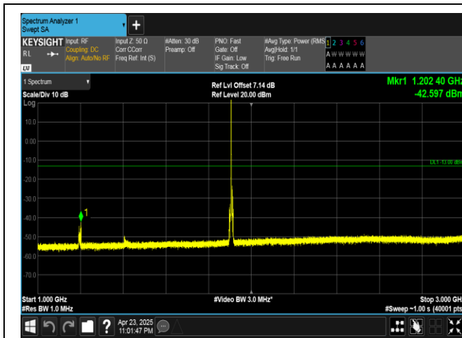
Band25-10MHz-16QAM-26640-1RB#0-1000~3000-PASS
