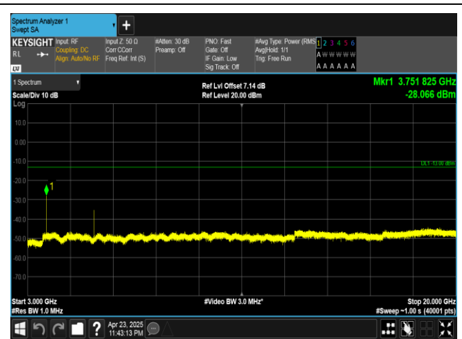
Band25-15MHz-QPSK-26365-1RB#0-3000~20000-PASS
