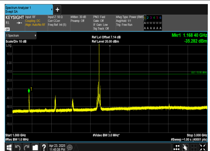
Band25-15MHz-QPSK-26365-1RB#74-1000~3000-PASS
