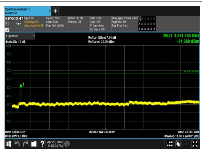
Band25-10MHz-16QAM-26640-1RB#0-3000~20000-PASS
