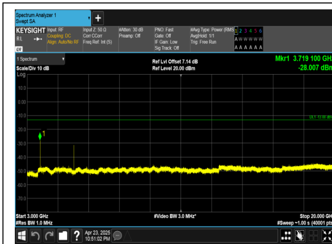
Band25-10MHz-16QAM-26090-1RB#49-3000~20000-PASS
