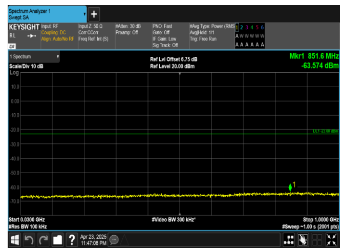
Band25-15MHz-QPSK-26365-75RB#0-30~1000-PASS
