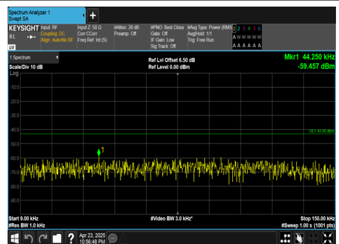
Band25-10MHz-16QAM-26365-1RB#49-0.009~0.15-PASS
