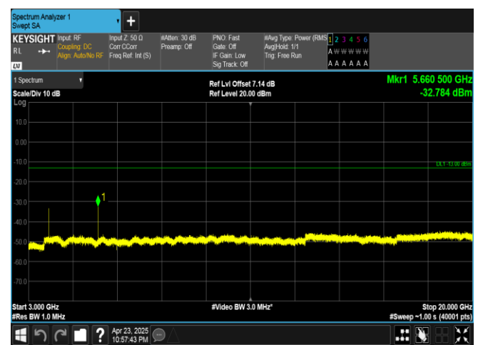
Band25-10MHz-16QAM-26365-1RB#49-3000~20000-PASS
