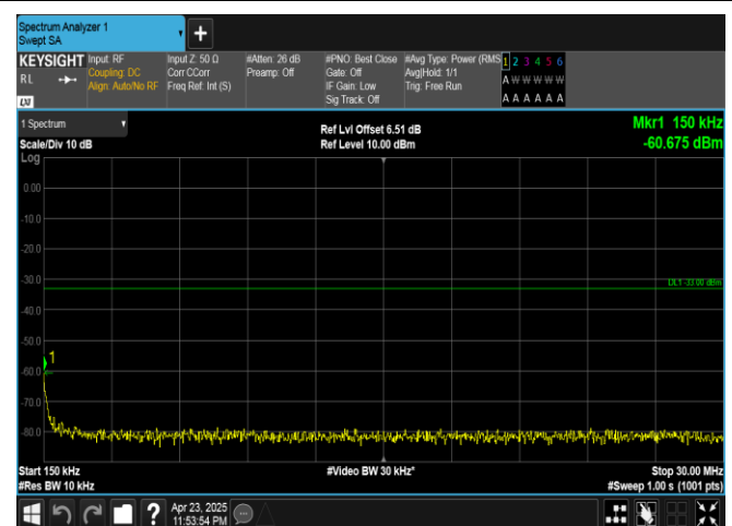
Band25-15MHz-QPSK-26615-75RB#0-0.15~30-PASS
