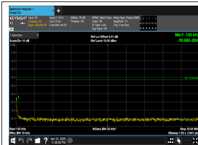
Band25-15MHz-QPSK-26115-1RB#74-0.15~30-PASS
