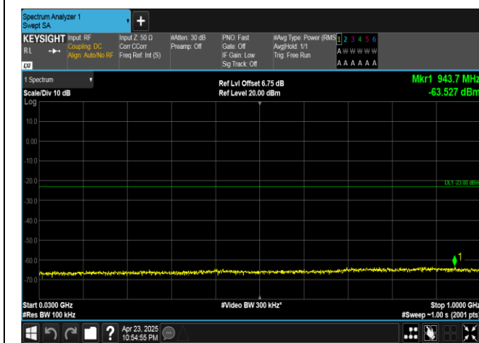
Band25-10MHz-16QAM-26365-1RB#0-30~1000-PASS
