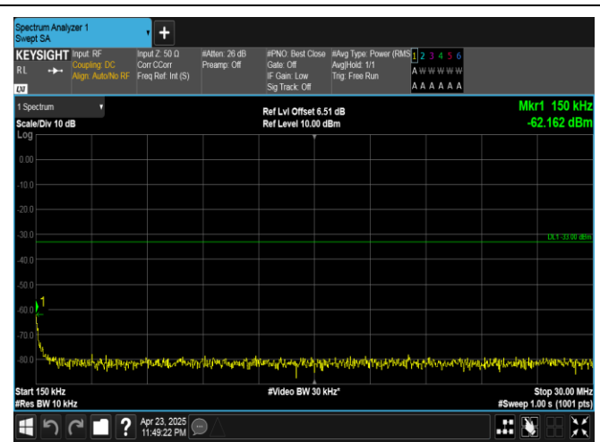
Band25-15MHz-QPSK-26615-1RB#0-0.15~30-PASS
