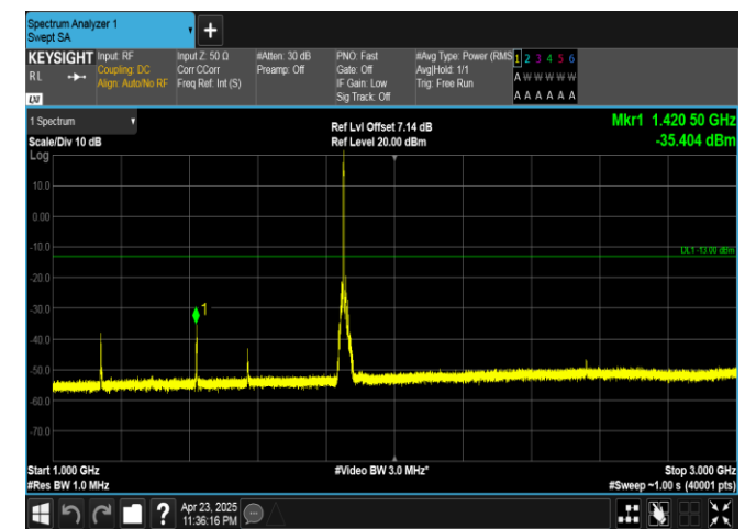
Band25-15MHz-QPSK-26115-1RB#0-1000~3000-PASS
