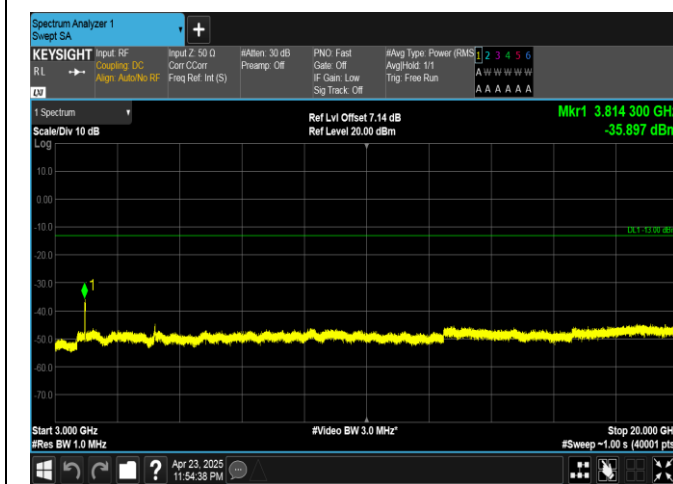
Band25-15MHz-QPSK-26615-75RB#0-3000~20000-PASS
