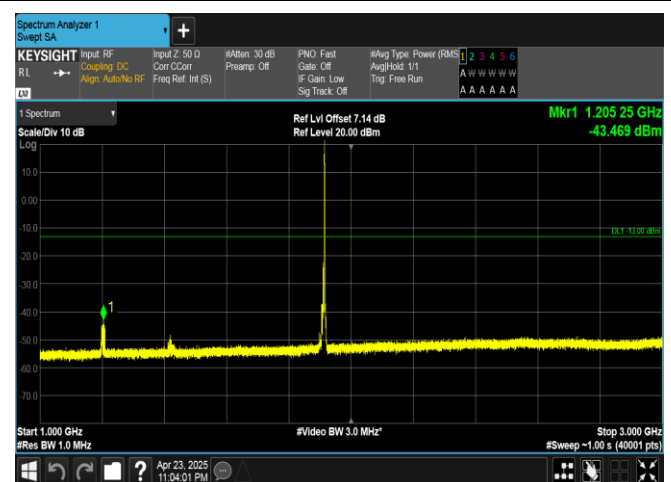
Band25-10MHz-16QAM-26640-1RB#49-1000~3000-PASS
