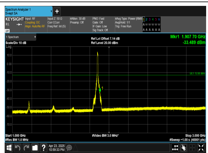
Band25-10MHz-16QAM-26365-50RB#0-1000~3000-PASS
