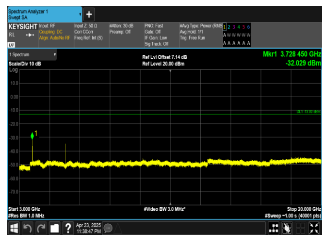
Band25-15MHz-QPSK-26115-1RB#74-3000~20000-PASS
