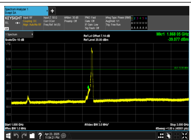
Band25-15MHz-QPSK-26615-75RB#0-1000~3000-PASS
