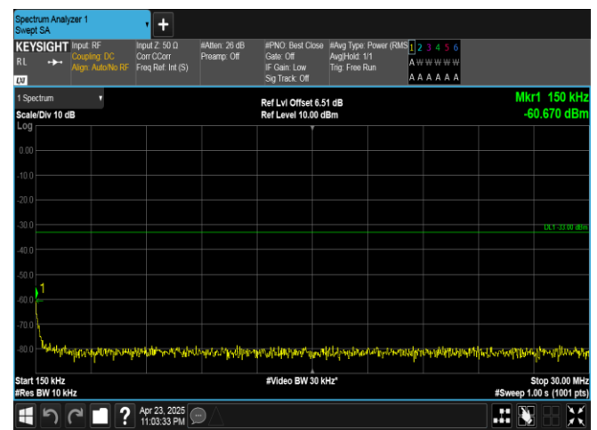
Band25-10MHz-16QAM-26640-1RB#49-0.15~30-PASS
