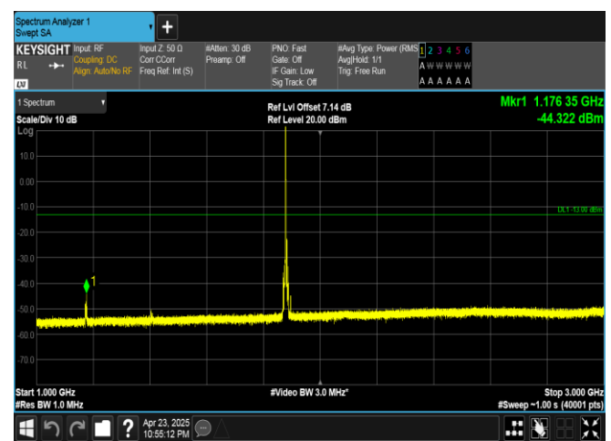
Band25-10MHz-16QAM-26365-1RB#0-1000~3000-PASS
