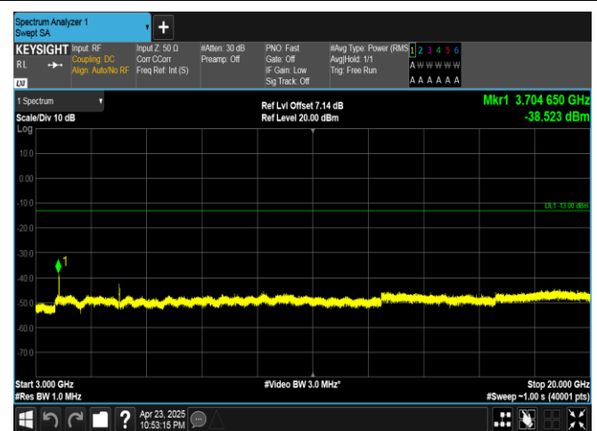
Band25-10MHz-16QAM-26090-50RB#0-3000~20000-PASS
