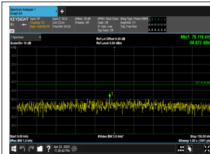
Band25-15MHz-QPSK-26115-1RB#0-0.009~0.15-PASS
