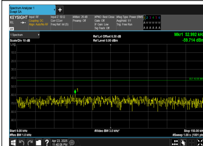
Band25-15MHz-QPSK-26115-75RB#0-0.009~0.15-PASS
