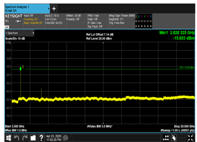
Band25-15MHz-QPSK-26615-1RB#74-3000~20000-PASS
