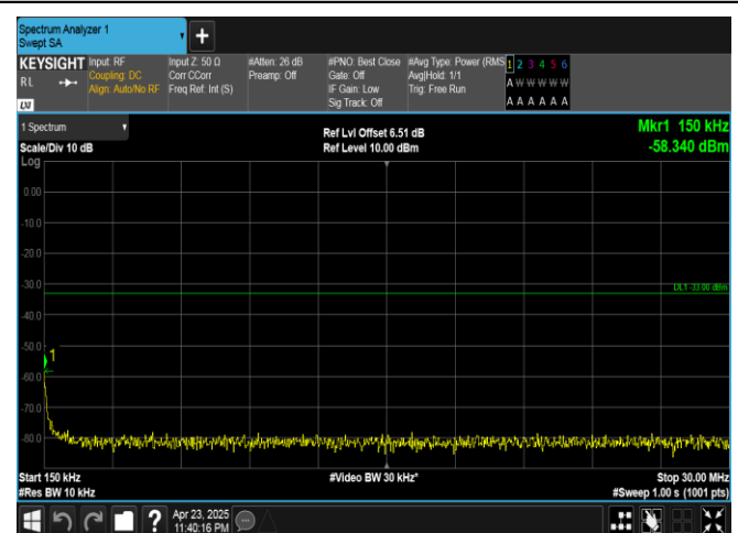
Band25-15MHz-QPSK-26115-75RB#0-0.15~30-PASS
