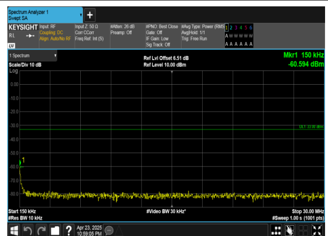
Band25-10MHz-16QAM-26365-50RB#0-0.15~30-PASS
