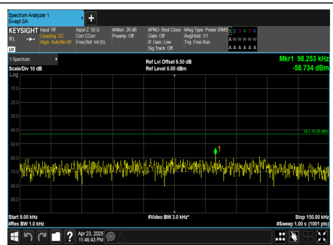
Band25-15MHz-QPSK-26365-75RB#0-0.009~0.15-PASS
