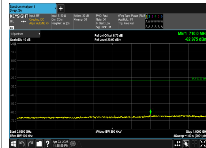
Band25-15MHz-QPSK-26115-1RB#0-30~1000-PASS
