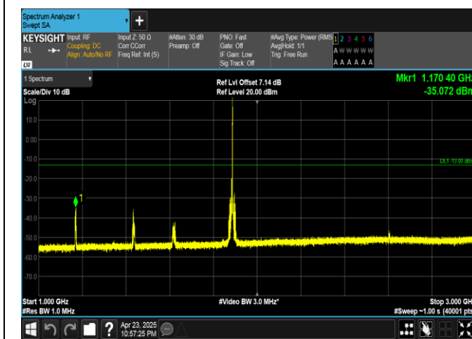
Band25-10MHz-16QAM-26365-1RB#49-1000~3000-PASS
