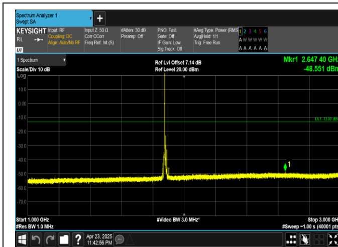
Band25-15MHz-QPSK-26365-1RB#0-1000~3000-PASS
