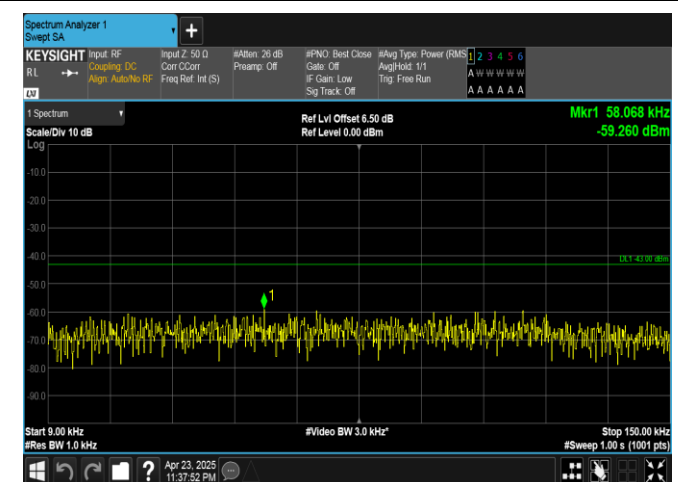
Band25-15MHz-QPSK-26115-1RB#74-0.009~0.15-PASS
