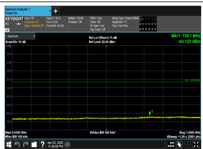
Band25-15MHz-QPSK-26115-1RB#74-30~1000-PASS
