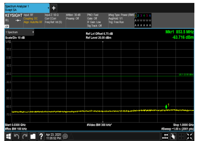
Band25-10MHz-16QAM-26640-50RB#0-30~1000-PASS
