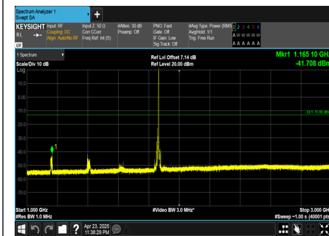
Band25-15MHz-QPSK-26115-1RB#74-1000~3000-PASS
