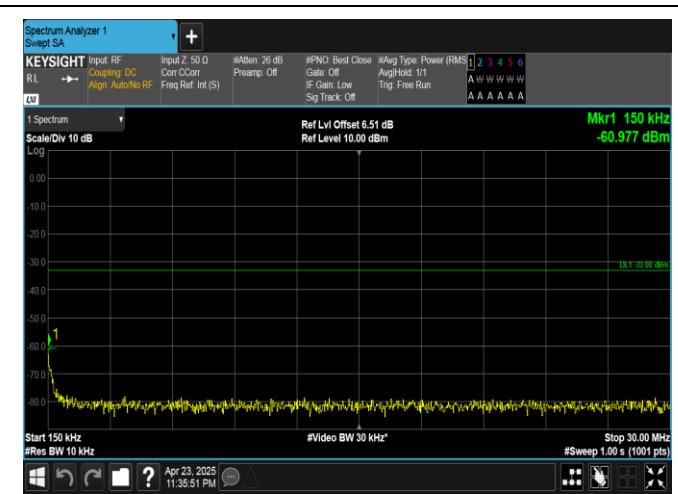
Band25-15MHz-QPSK-26115-1RB#0-0.15~30-PASS
