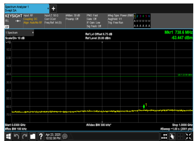
Band25-10MHz-16QAM-26090-50RB#0-30~1000-PASS
