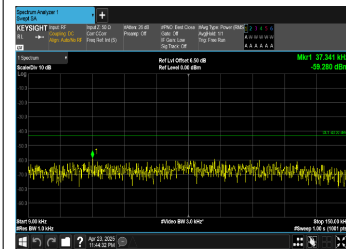
Band25-15MHz-QPSK-26365-1RB#74-0.009~0.15-PASS
