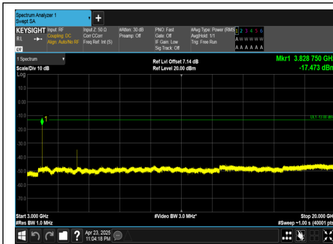
Band25-10MHz-16QAM-26640-1RB#49-3000~20000-PASS
