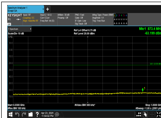
Band25-15MHz-QPSK-26615-75RB#0-30~1000-PASS
