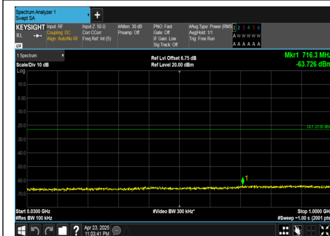
Band25-10MHz-16QAM-26640-1RB#49-30~1000-PASS
