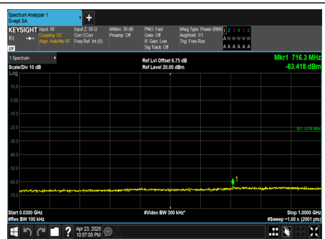
Band25-10MHz-16QAM-26365-1RB#49-30~1000-PASS
