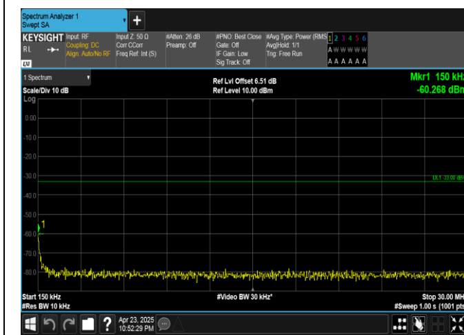
Band25-10MHz-16QAM-26090-50RB#0-0.15~30-PASS
