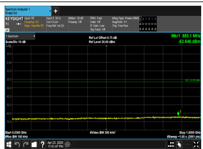
Band25-15MHz-QPSK-26615-1RB#74-30~1000-PASS
