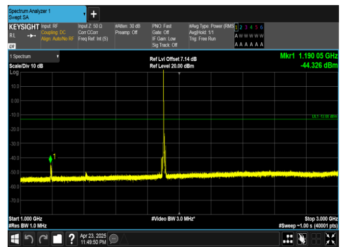
Band25-15MHz-QPSK-26615-1RB#0-1000~3000-PASS
