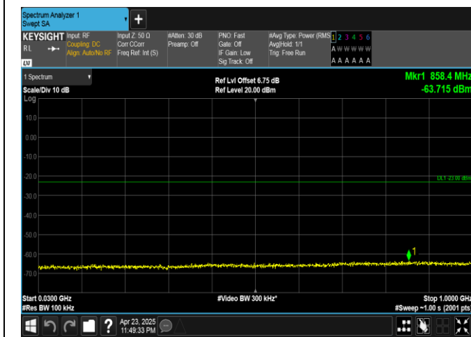
Band25-15MHz-QPSK-26615-1RB#0-30~1000-PASS
