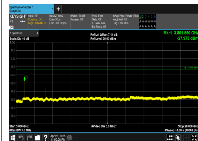
Band25-15MHz-QPSK-26615-1RB#0-3000~20000-PASS
