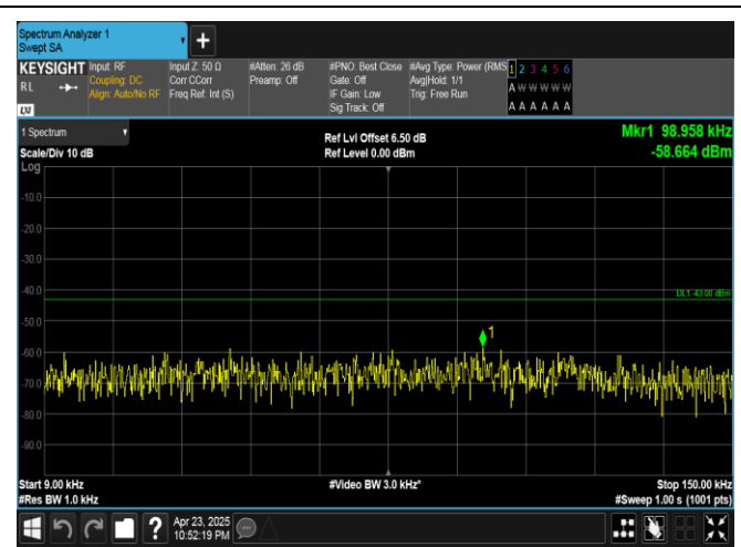
Band25-10MHz-16QAM-26090-50RB#0-0.009~0.15-PASS
