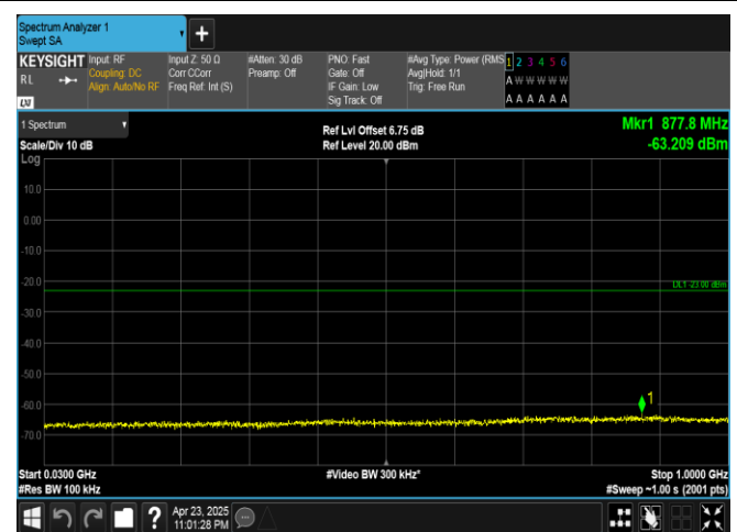
Band25-10MHz-16QAM-26640-1RB#0-30~1000-PASS
