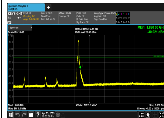
Band25-10MHz-16QAM-26090-50RB#0-1000~3000-PASS
