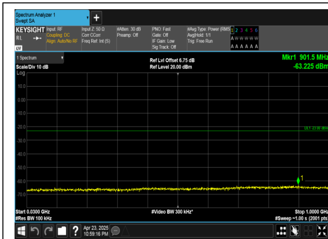
Band25-10MHz-16QAM-26365-50RB#0-30~1000-PASS
