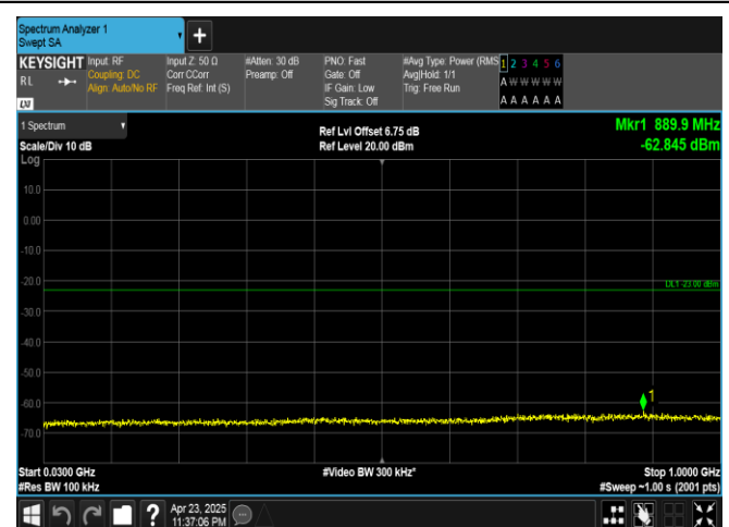
Band25-15MHz-16QAM-26115-1RB#0-30~1000-PASS
