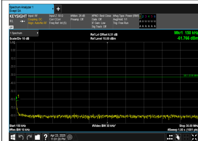
Band25-10MHz-16QAM-26640-1RB#0-0.15~30-PASS
