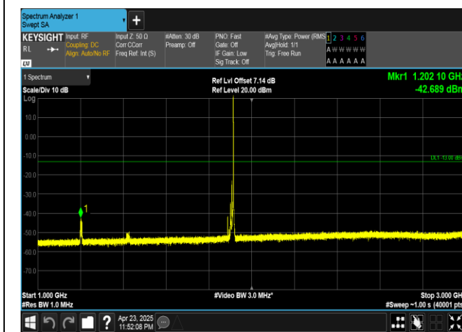
Band25-15MHz-QPSK-26615-1RB#74-1000~3000-PASS
