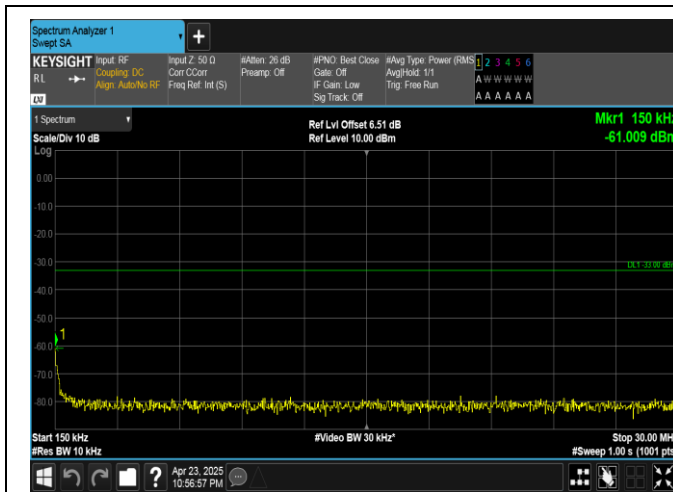
Band25-10MHz-16QAM-26365-1RB#49-0.15~30-PASS
