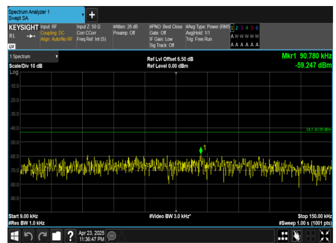
Band25-15MHz-16QAM-26115-1RB#0-0.009~0.15-PASS
