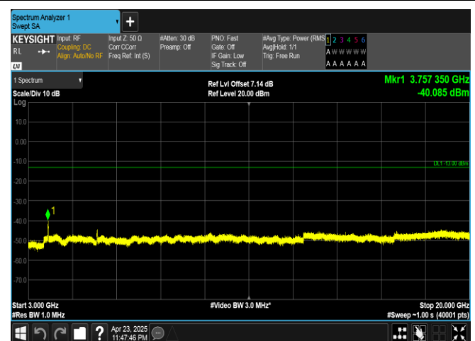
Band25-15MHz-QPSK-26365-75RB#0-3000~20000-PASS
