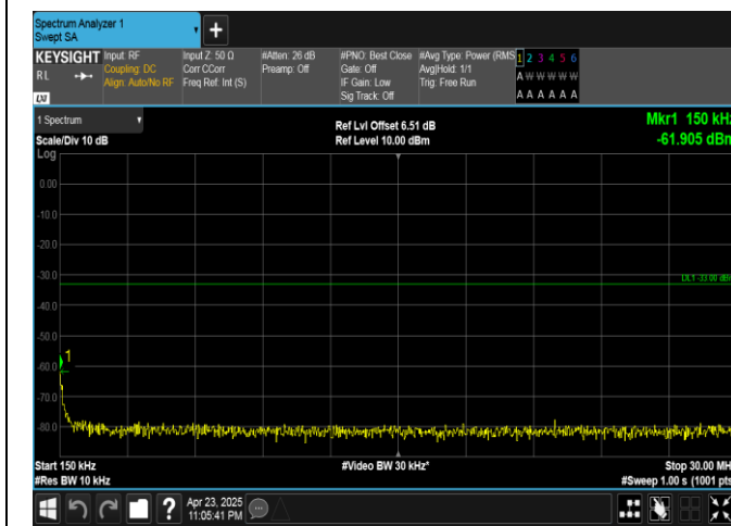
Band25-10MHz-16QAM-26640-50RB#0-0.15~30-PASS
