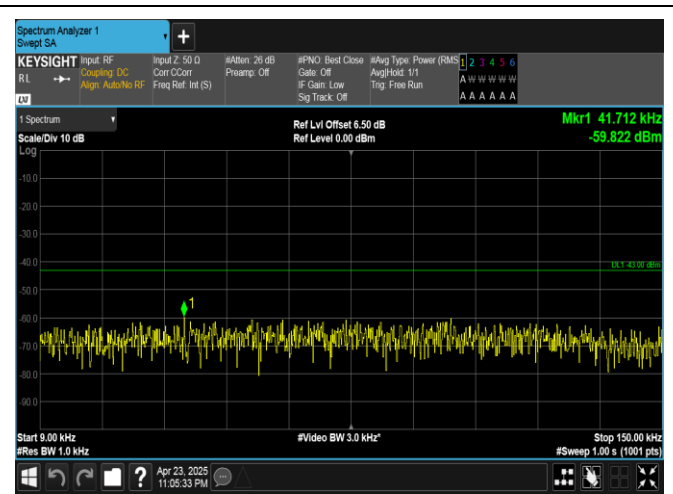
Band25-10MHz-16QAM-26640-50RB#0-0.009~0.15-PASS
