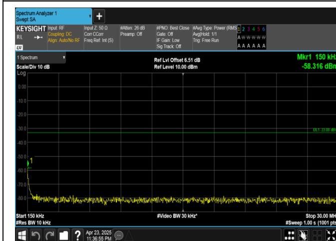
Band25-15MHz-16QAM-26115-1RB#0-0.15~30-PASS
