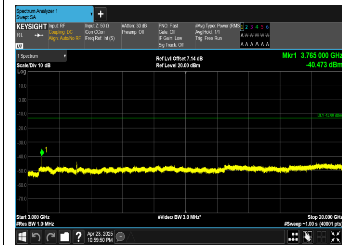
Band25-10MHz-16QAM-26365-50RB#0-3000~20000-PASS
