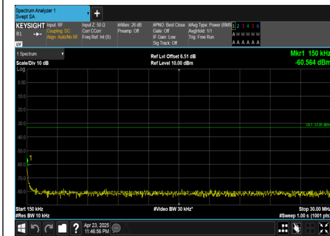
Band25-15MHz-QPSK-26365-75RB#0-0.15~30-PASS
