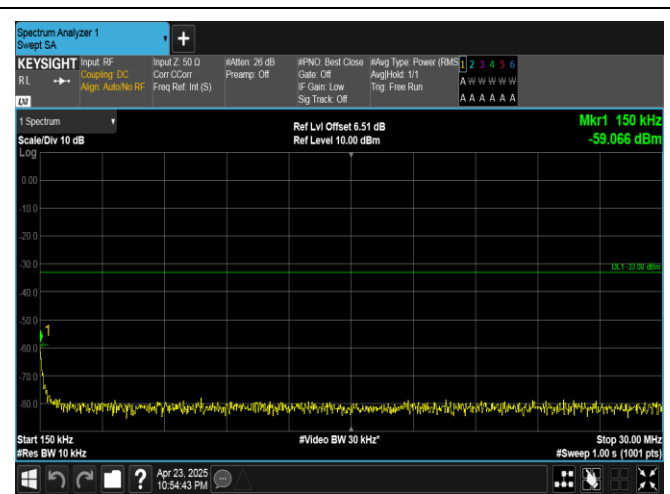
Band25-10MHz-16QAM-26365-1RB#0-0.15~30-PASS
