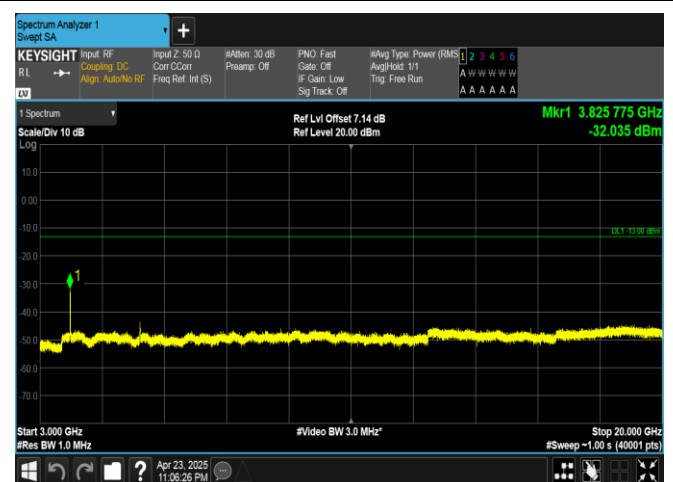
Band25-10MHz-16QAM-26640-50RB#0-3000~20000-PASS
