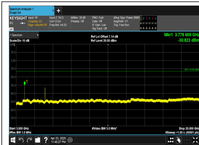
Band25-15MHz-QPSK-26365-1RB#74-3000~20000-PASS
