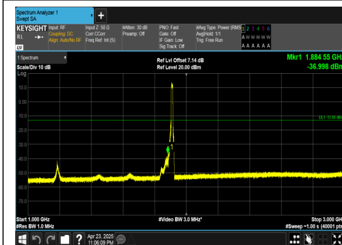
Band25-10MHz-16QAM-26640-50RB#0-1000~3000-PASS
