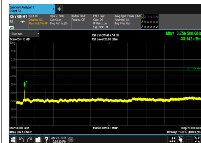
Band25-10MHz-16QAM-26365-1RB#0-3000~20000-PASS
