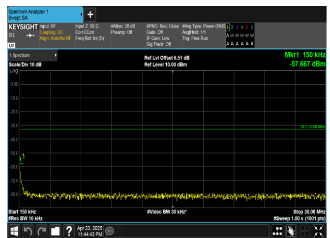
Band25-15MHz-QPSK-26365-1RB#74-0.15~30-PASS
