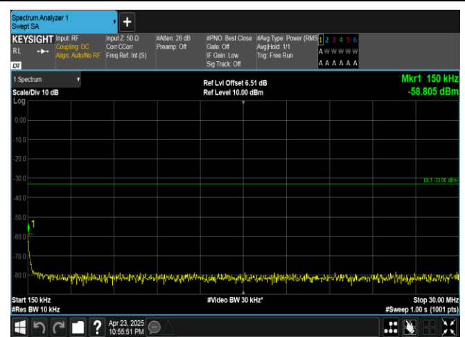
Band25-10MHz-QPSK-26365-1RB#49-0.15~30-PASS
