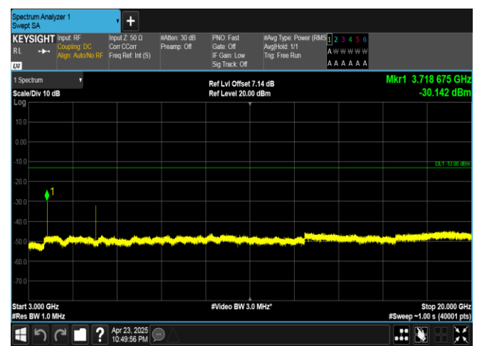
Band25-10MHz-QPSK-26090-1RB#49-3000~20000-PASS
