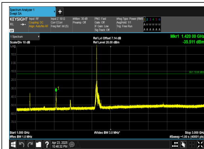
Band25-10MHz-16QAM-26090-1RB#0-1000~3000-PASS
