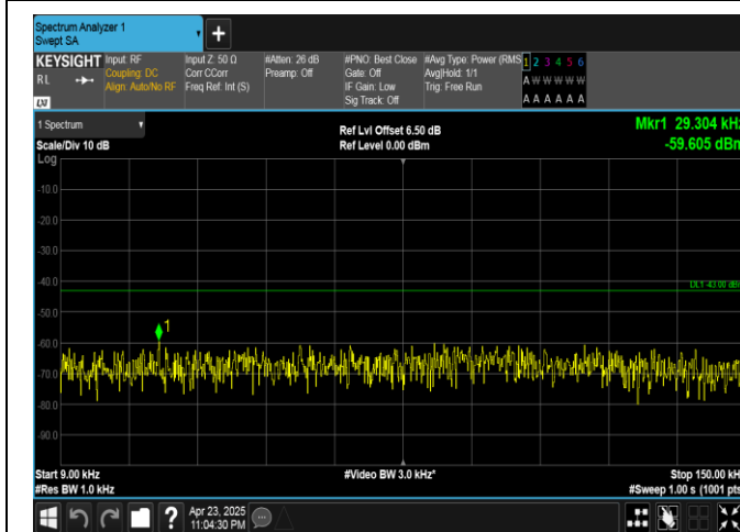
Band25-10MHz-QPSK-26640-50RB#0-0.009~0.15-PASS
