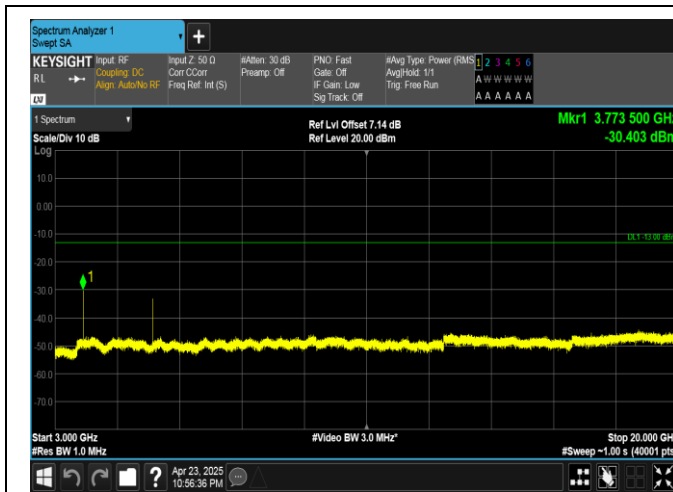
Band25-10MHz-QPSK-26365-1RB#49-3000~20000-PASS
