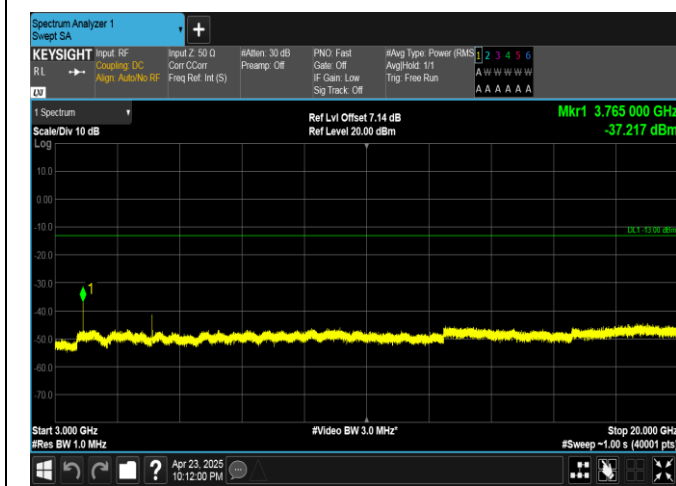
Band25-5MHz-16QAM-26365-25RB#0-3000~20000-PASS
