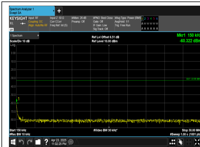
Band25-10MHz-QPSK-26640-1RB#49-0.15~30-PASS
