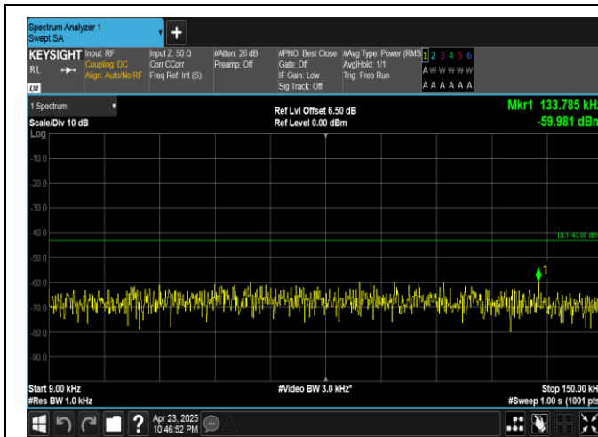
Band25-10MHz-QPSK-26090-1RB#0-0.009~0.15-PASS
