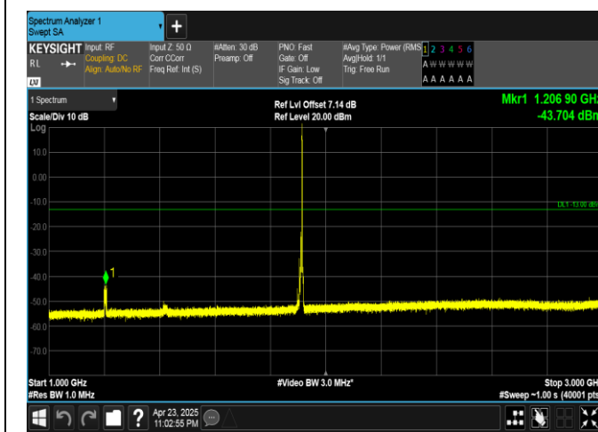
Band25-10MHz-QPSK-26640-1RB#49-1000~3000-PASS
