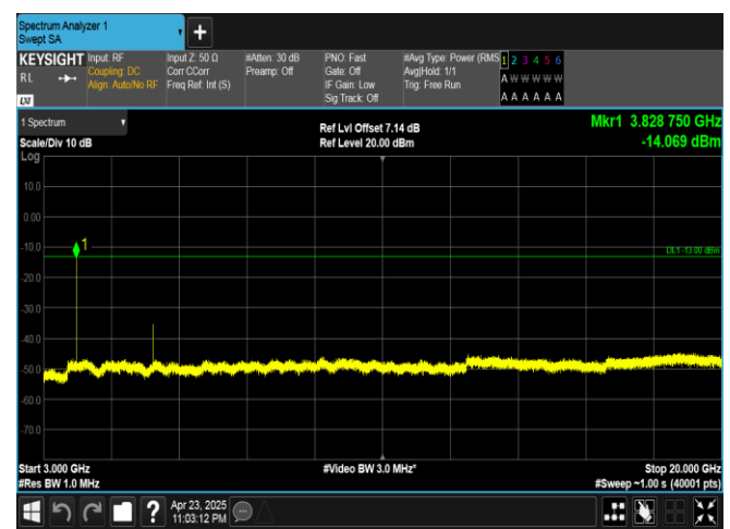
Band25-10MHz-QPSK-26640-1RB#49-3000~20000-PASS
