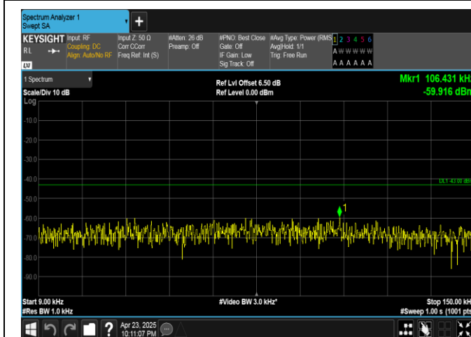
Band25-5MHz-16QAM-26365-25RB#0-0.009~0.15-PASS
