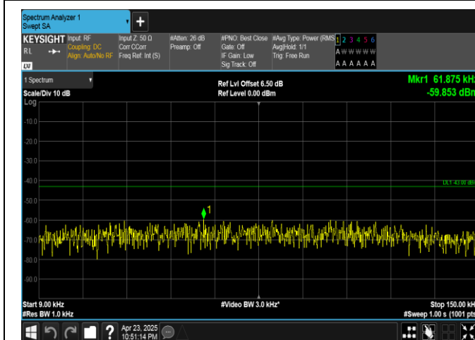
Band25-10MHz-QPSK-26090-50RB#0-0.009~0.15-PASS
