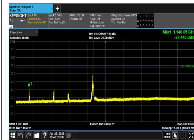
Band25-10MHz-QPSK-26090-1RB#49-1000~3000-PASS
