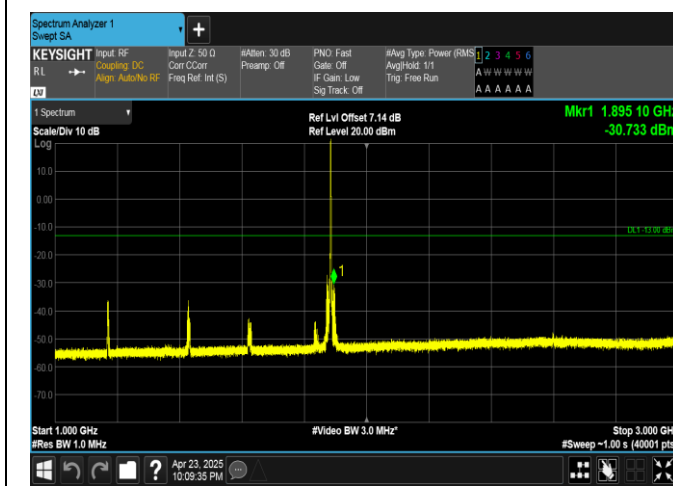
Band25-5MHz-16QAM-26365-1RB#24-1000~3000-PASS
