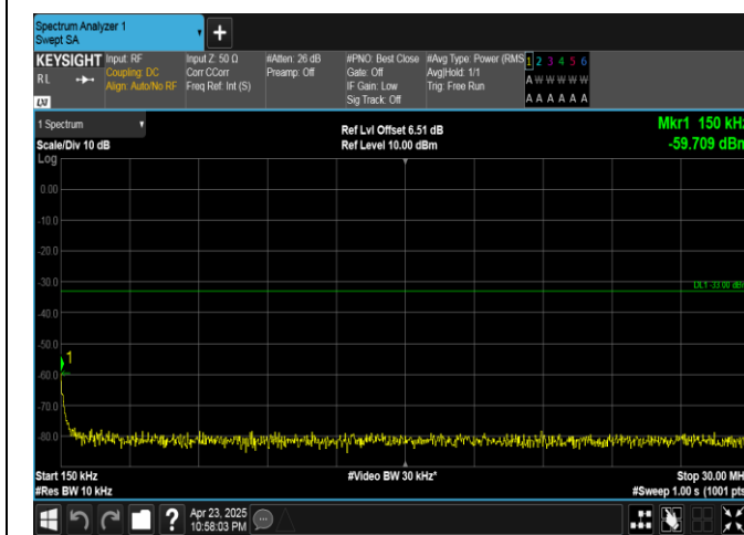
Band25-10MHz-QPSK-26365-50RB#0-0.15~30-PASS
