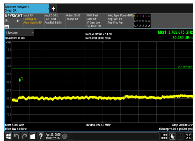
Band25-5MHz-16QAM-26365-1RB#24-3000~20000-PASS
