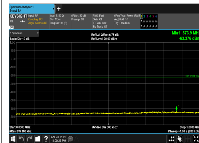
Band25-10MHz-QPSK-26640-1RB#0-30~1000-PASS
