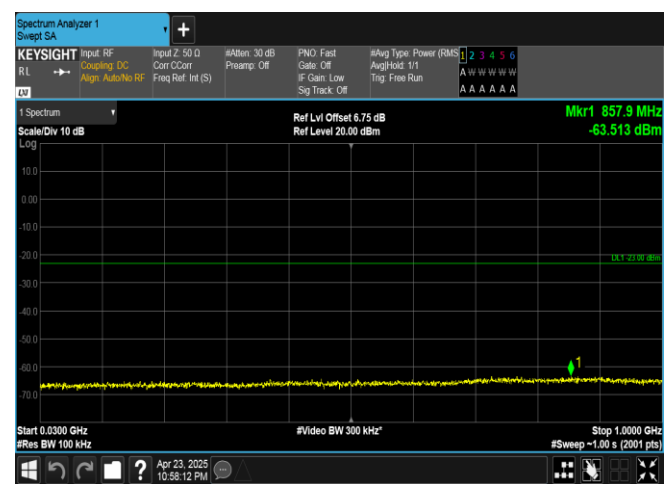
Band25-10MHz-QPSK-26365-50RB#0-30~1000-PASS
