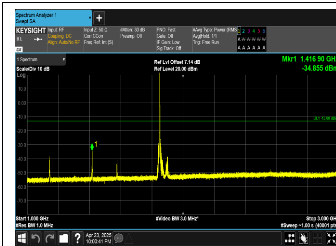
Band25-5MHz-16QAM-26065-1RB#0-1000~3000-PASS
