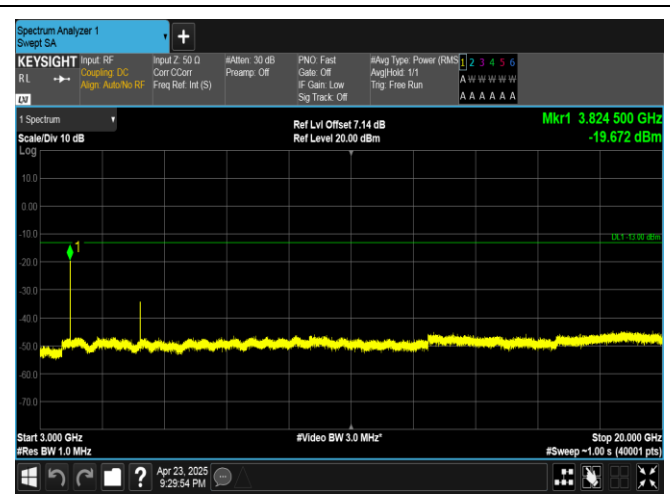
Band25-3MHz-16QAM-26675-1RB#0-3000~20000-PASS
