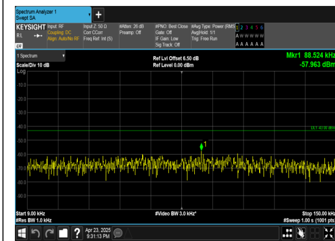
Band25-3MHz-16QAM-26675-1RB#14-0.009~0.15-PASS
