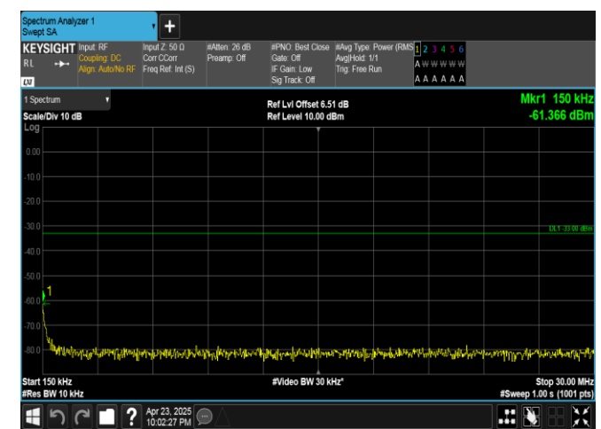
Band25-5MHz-16QAM-26065-1RB#24-0.15~30-PASS
