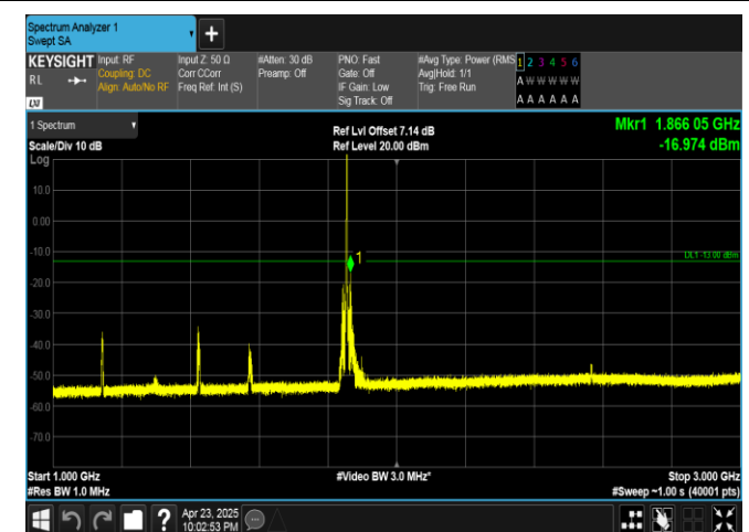
Band25-5MHz-16QAM-26065-1RB#24-1000~3000-PASS
