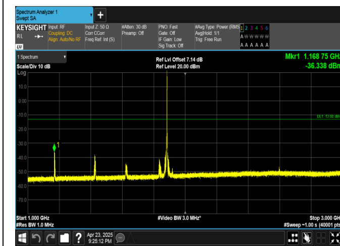
Band25-3MHz-16QAM-26365-1RB#14-1000~3000-PASS
