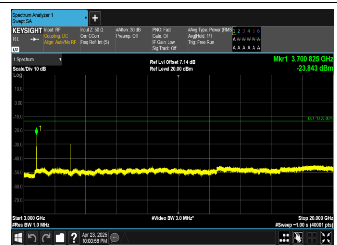
Band25-5MHz-16QAM-26065-1RB#0-3000~20000-PASS
