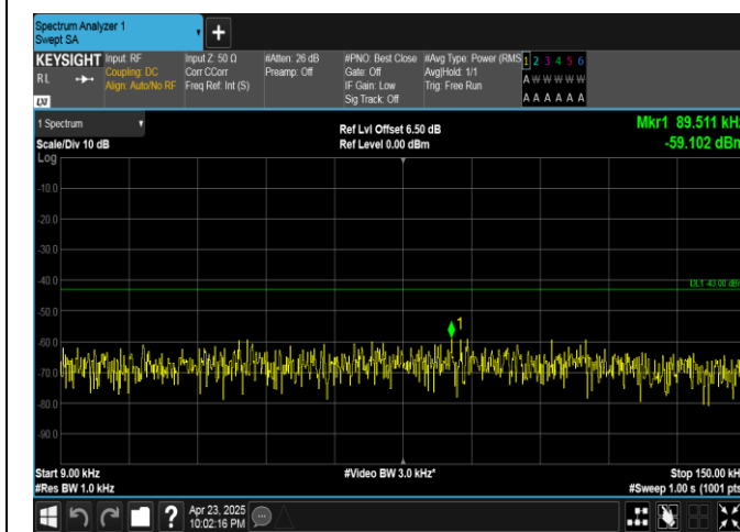
Band25-5MHz-16QAM-26065-1RB#24-0.009~0.15-PASS
