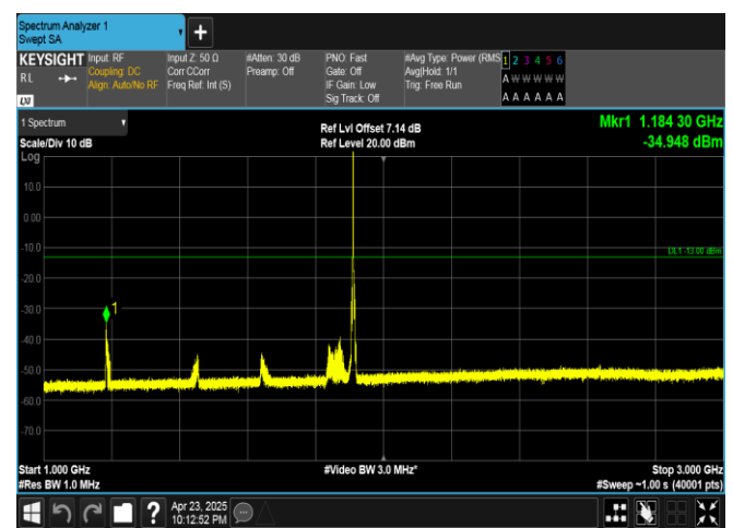
Band25-5MHz-QPSK-26665-1RB#0-1000~3000-PASS
