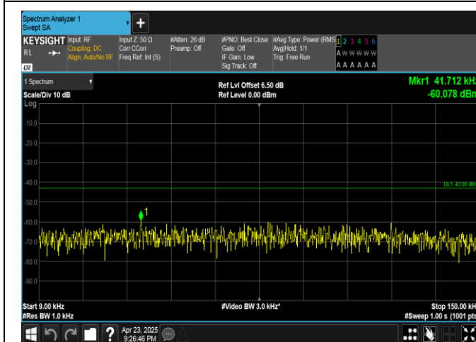
Band25-3MHz-16QAM-26365-15RB#0-0.009~0.15-PASS
