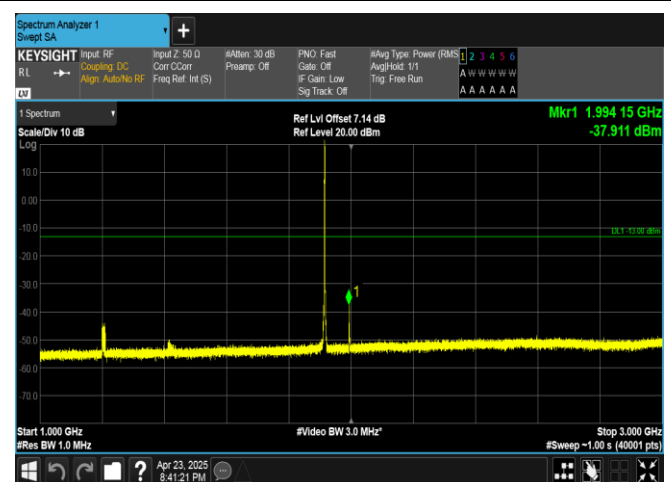
Band25-1.4MHz-16QAM-26683-1RB#5-1000~3000-PASS
