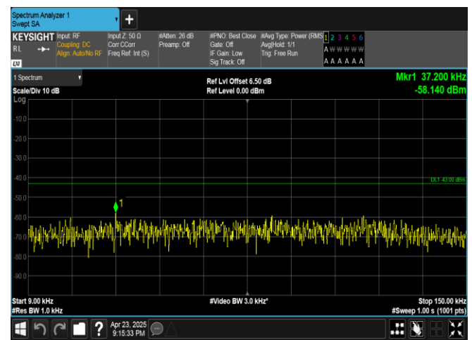
Band25-3MHz-16QAM-26055-1RB#0-0.009~0.15-PASS
