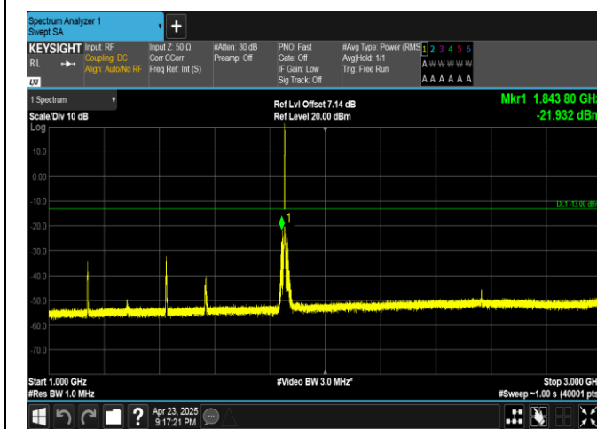
Band25-3MHz-QPSK-26055-1RB#14-1000~3000-PASS
