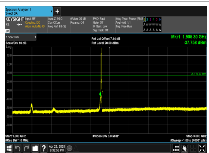
Band25-3MHz-QPSK-26675-15RB#0-1000~3000-PASS
