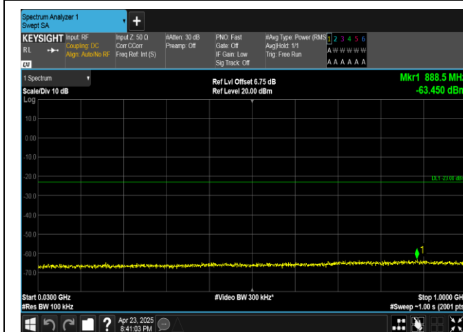
Band25-1.4MHz-16QAM-26683-1RB#5-30~1000-PASS
