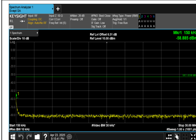
Band25-3MHz-16QAM-26055-1RB#0-0.15~30-PASS
