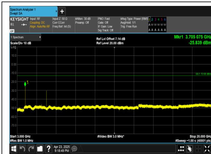
Band25-3MHz-16QAM-26055-1RB#14-3000~20000-PASS
