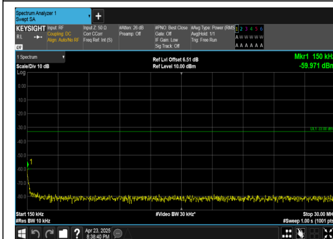
Band25-1.4MHz-16QAM-26683-1RB#0-0.15~30-PASS
