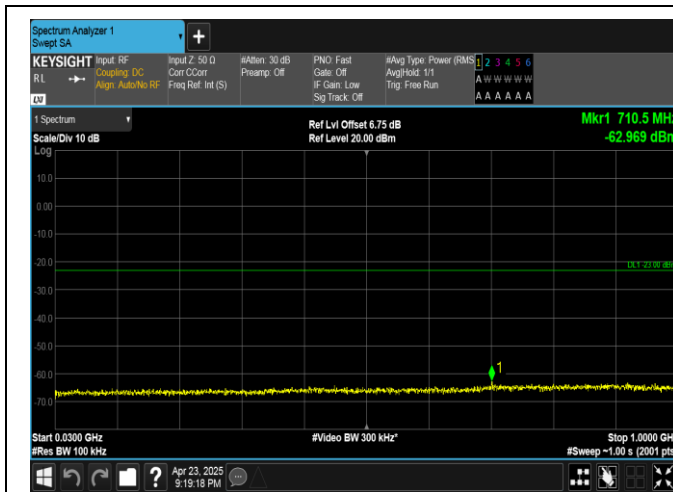
Band25-3MHz-QPSK-26055-15RB#0-30~1000-PASS
