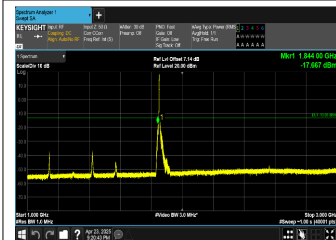
Band25-3MHz-16QAM-26055-15RB#0-1000~3000-PASS
