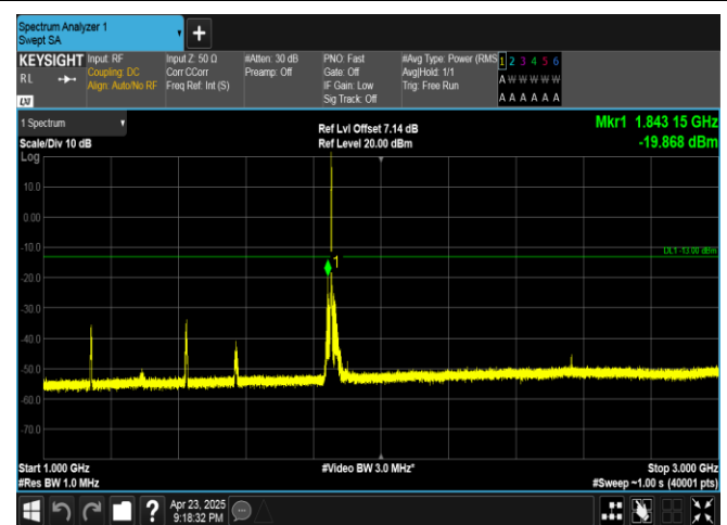
Band25-3MHz-16QAM-26055-1RB#14-1000~3000-PASS
