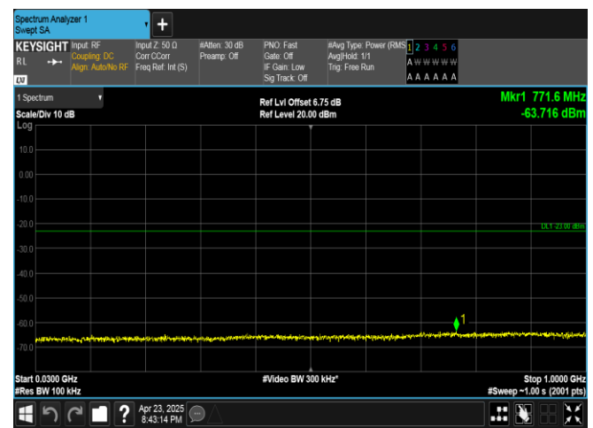
Band25-1.4MHz-16QAM-26683-6RB#0-30~1000-PASS
