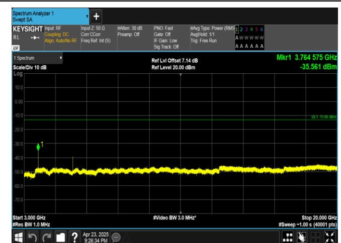
Band25-3MHz-QPSK-26365-15RB#0-3000~20000-PASS
