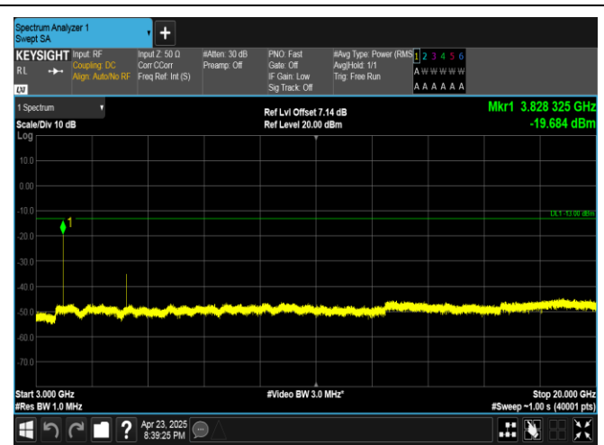
Band25-1.4MHz-16QAM-26683-1RB#0-3000~20000-PASS
