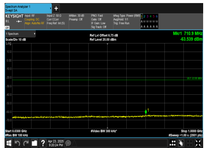
Band25-3MHz-16QAM-26055-15RB#0-30~1000-PASS
