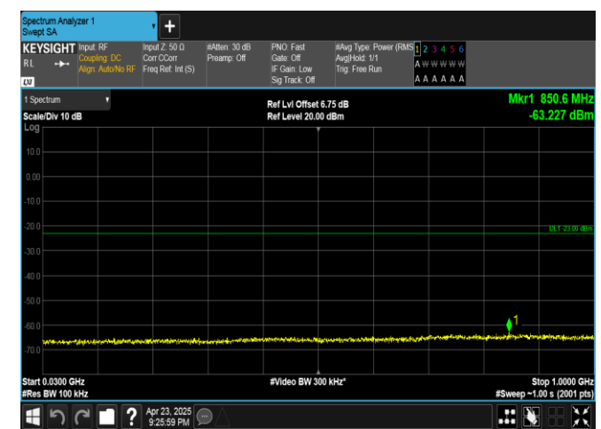
Band25-3MHz-QPSK-26365-15RB#0-30~1000-PASS
