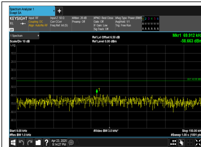
Band25-3MHz-QPSK-26055-1RB#0-0.009~0.15-PASS
