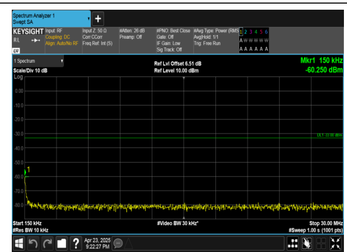
Band25-3MHz-16QAM-26365-1RB#0-0.15~30-PASS
