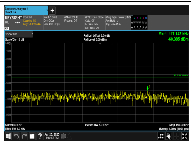
Band25-1.4MHz-16QAM-26683-6RB#0-0.009~0.15-PASS
