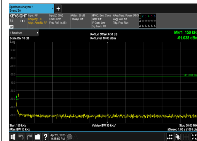
Band25-3MHz-QPSK-26365-15RB#0-0.15~30-PASS
