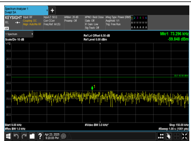
Band25-3MHz-16QAM-26055-15RB#0-0.009~0.15-PASS
