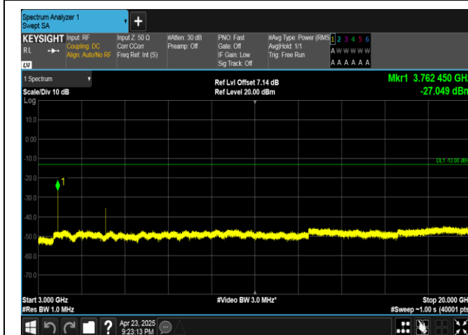
Band25-3MHz-16QAM-26365-1RB#0-3000~20000-PASS
