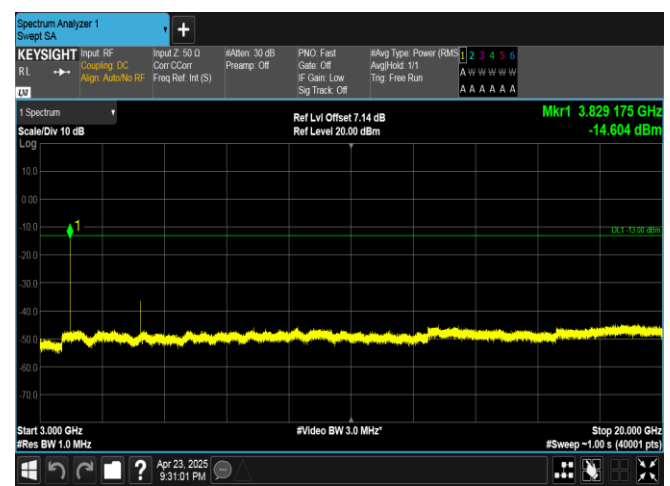
Band25-3MHz-QPSK-26675-1RB#14-3000~20000-PASS
