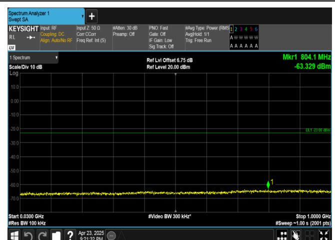
Band25-3MHz-QPSK-26365-1RB#0-30~1000-PASS
