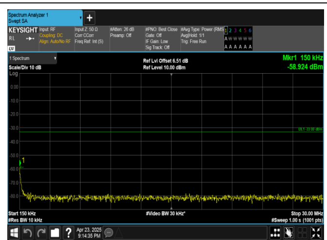
Band25-3MHz-QPSK-26055-1RB#0-0.15~30-PASS
