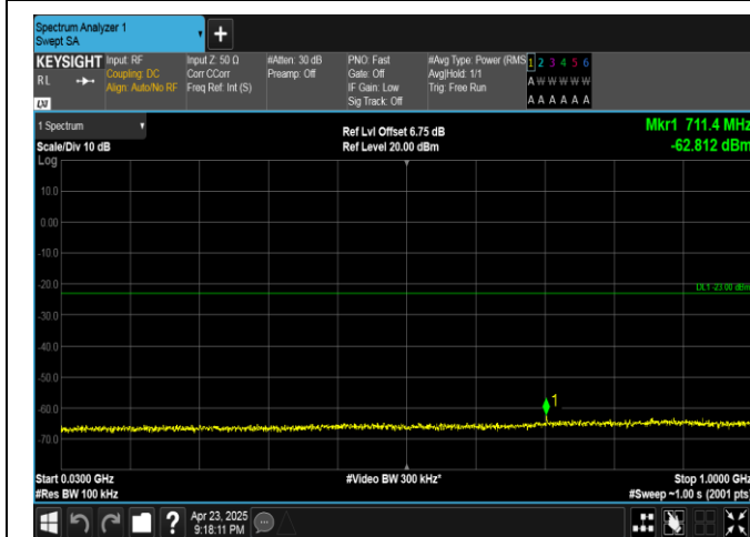
Band25-3MHz-16QAM-26055-1RB#14-30~1000-PASS
