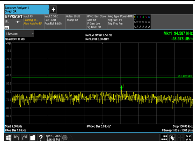
Band25-3MHz-QPSK-26055-1RB#14-0.009~0.15-PASS
