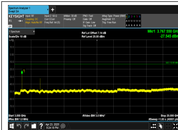
Band25-3MHz-QPSK-26365-1RB#14-3000~20000-PASS
