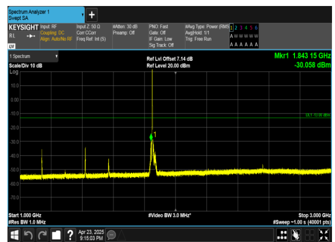
Band25-3MHz-QPSK-26055-1RB#0-1000~3000-PASS
