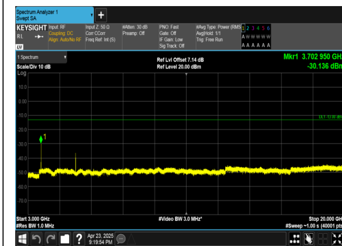
Band25-3MHz-QPSK-26055-15RB#0-3000~20000-PASS
