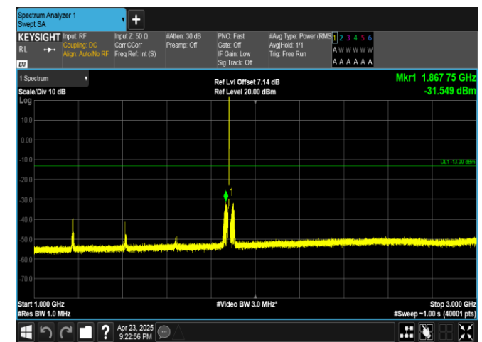
Band25-3MHz-16QAM-26365-1RB#0-1000~3000-PASS
