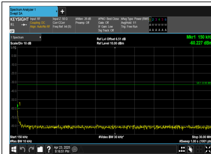
Band25-3MHz-QPSK-26055-1RB#14-0.15~30-PASS
