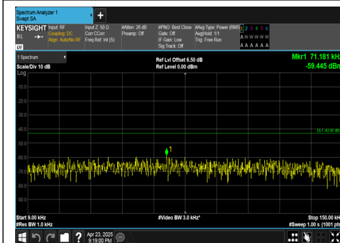
Band25-3MHz-QPSK-26055-15RB#0-0.009~0.15-PASS
