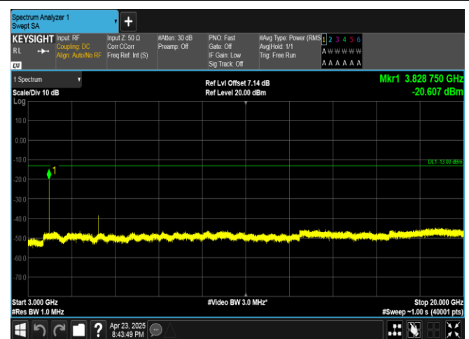
Band25-1.4MHz-16QAM-26683-6RB#0-3000~20000-PASS
