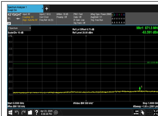
Band25-1.4MHz-16QAM-26365-6RB#0-30~1000-PASS
