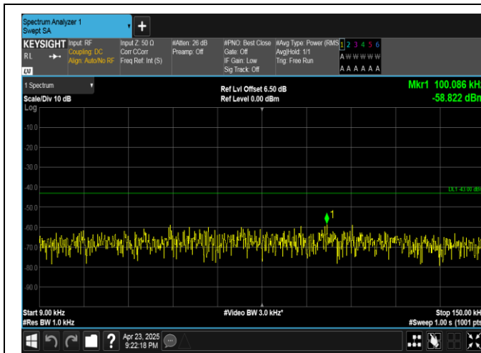
Band25-3MHz-16QAM-26365-1RB#0-0.009~0.15-PASS
