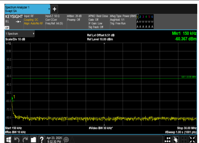
Band25-3MHz-QPSK-26675-15RB#0-0.15~30-PASS
