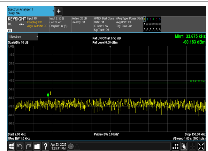
Band25-3MHz-QPSK-26365-15RB#0-0.009~0.15-PASS
