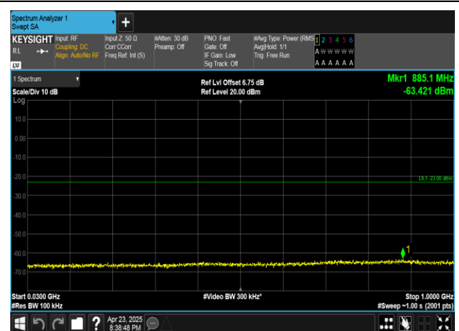
Band25-1.4MHz-16QAM-26683-1RB#0-30~1000-PASS
