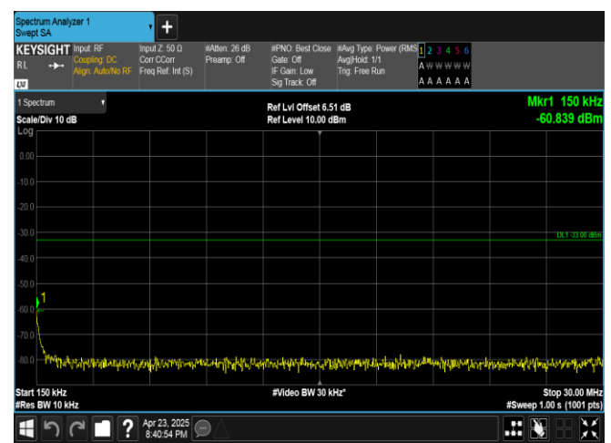
Band25-1.4MHz-16QAM-26683-1RB#5-0.15~30-PASS
