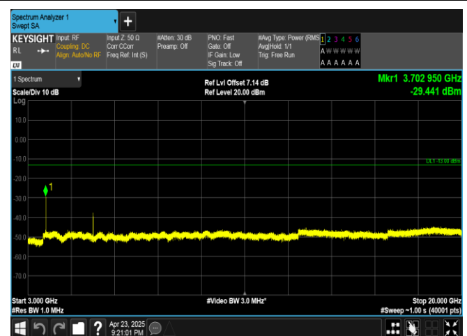
Band25-3MHz-16QAM-26055-15RB#0-3000~20000-PASS
