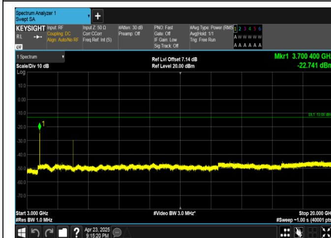
Band25-3MHz-QPSK-26055-1RB#0-3000~20000-PASS
