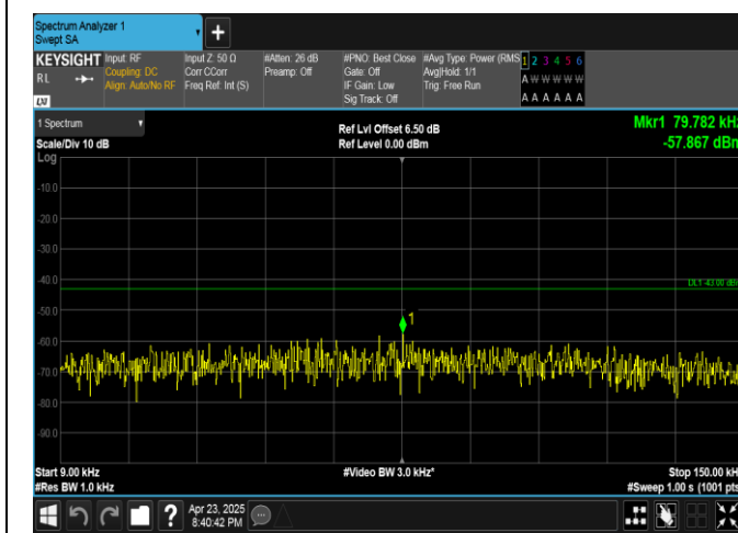
Band25-1.4MHz-16QAM-26683-1RB#5-0.009~0.15-PASS
