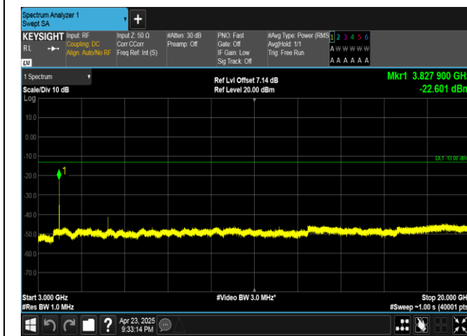
Band25-3MHz-QPSK-26675-15RB#0-3000~20000-PASS
