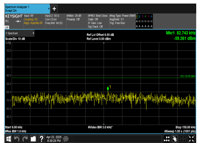
Band25-1.4MHz-16QAM-26683-1RB#0-0.009~0.15-PASS
