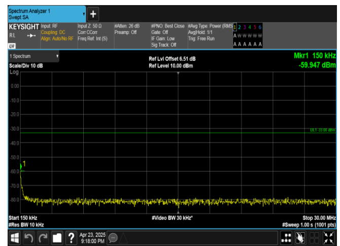
Band25-3MHz-16QAM-26055-1RB#14-0.15~30-PASS
