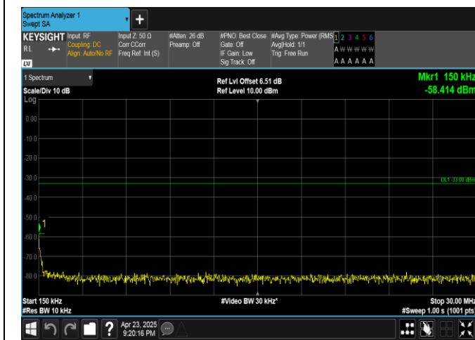
Band25-3MHz-16QAM-26055-15RB#0-0.15~30-PASS
