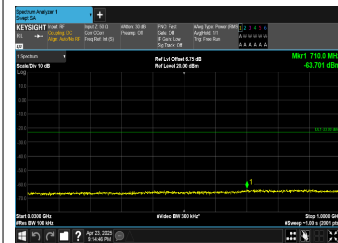
Band25-3MHz-QPSK-26055-1RB#0-30~1000-PASS
