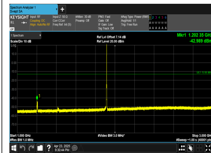
Band25-3MHz-QPSK-26675-1RB#14-1000~3000-PASS
