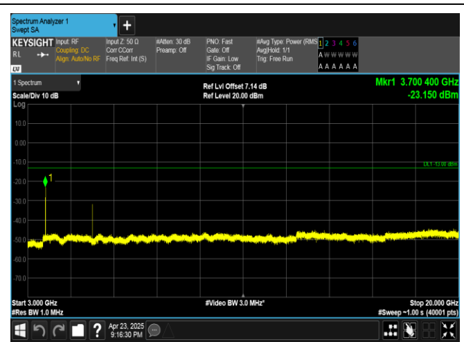
Band25-3MHz-16QAM-26055-1RB#0-3000~20000-PASS
