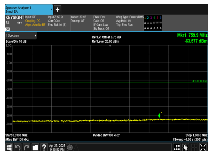
Band25-3MHz-16QAM-26055-1RB#0-30~1000-PASS
