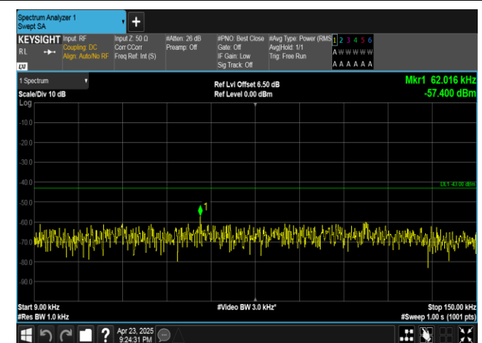
Band25-3MHz-16QAM-26365-1RB#14-0.009~0.15-PASS
