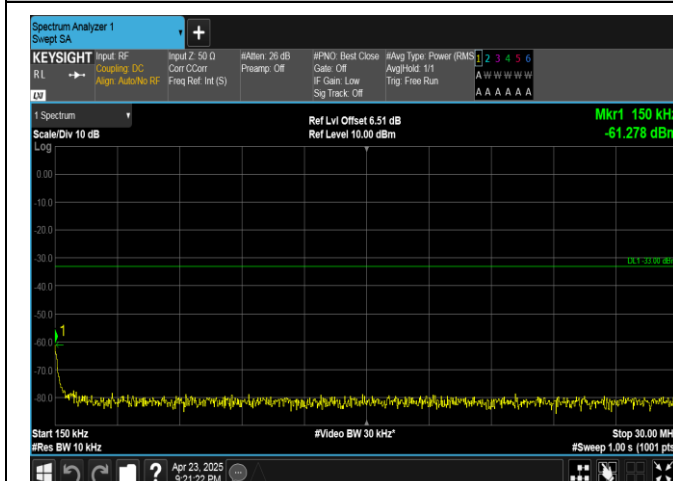
Band25-3MHz-QPSK-26365-1RB#0-0.15~30-PASS
