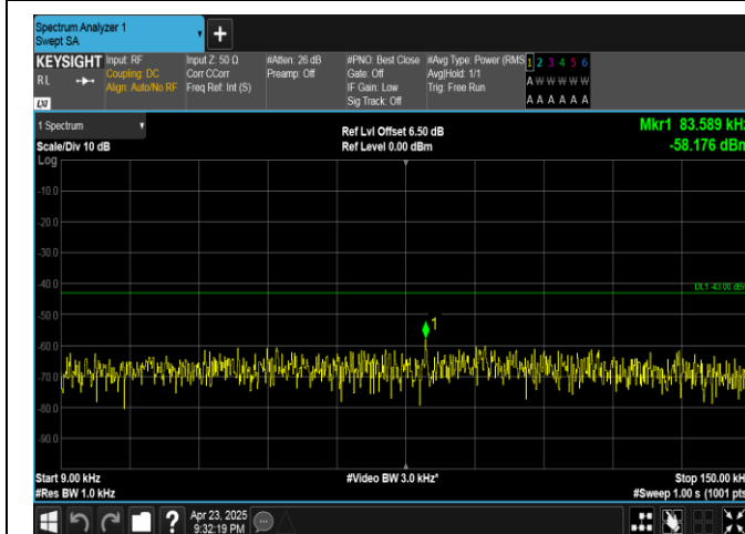
Band25-3MHz-QPSK-26675-15RB#0-0.009~0.15-PASS
