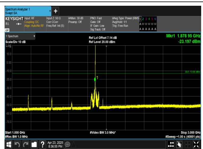
Band25-1.4MHz-16QAM-26365-6RB#0-1000~3000-PASS
