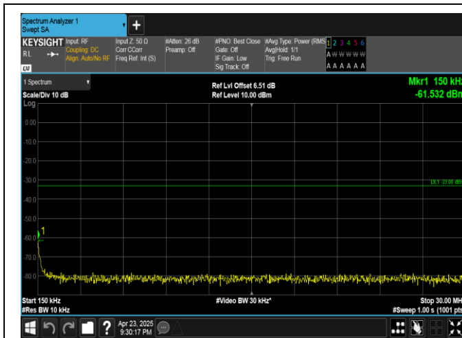
Band25-3MHz-QPSK-26675-1RB#14-0.15~30-PASS
