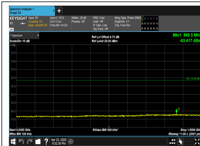
Band25-3MHz-QPSK-26675-15RB#0-30~1000-PASS
