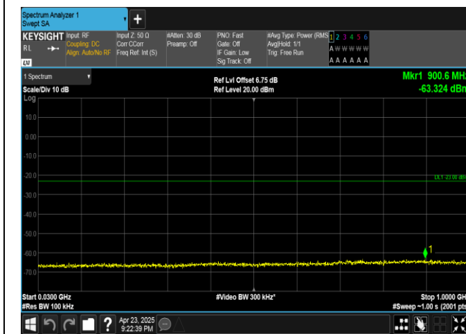
Band25-3MHz-16QAM-26365-1RB#0-30~1000-PASS
