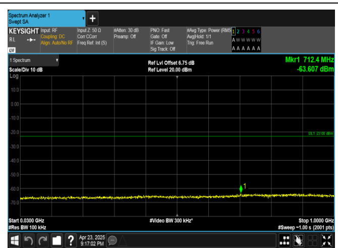
Band25-3MHz-QPSK-26055-1RB#14-30~1000-PASS
