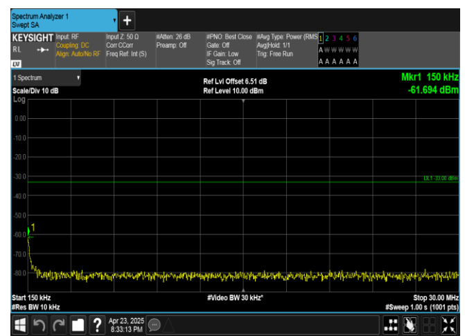
Band25-1.4MHz-QPSK-26365-1RB#5-0.15~30-PASS
