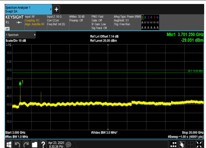
Band25-1.4MHz-16QAM-26047-6RB#0-3000~20000-PASS
