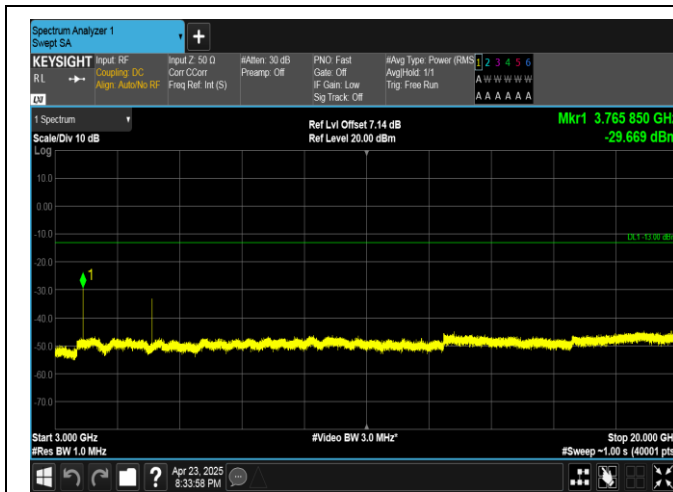
Band25-1.4MHz-QPSK-26365-1RB#5-3000~20000-PASS
