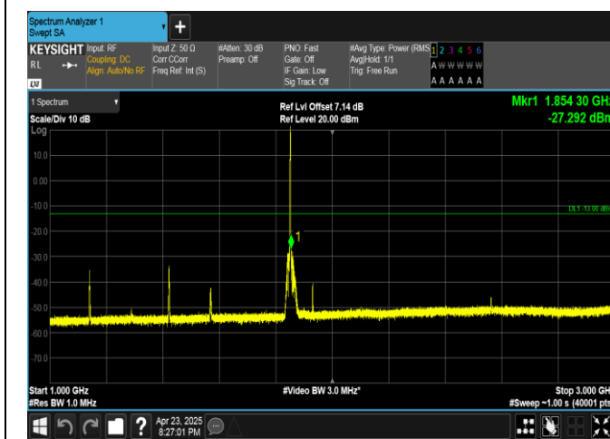
Band25-1.4MHz-QPSK-26047-1RB#5-1000~3000-PASS
