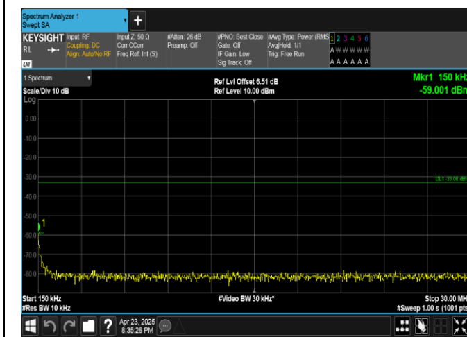
Band25-1.4MHz-QPSK-26365-6RB#0-0.15~30-PASS
