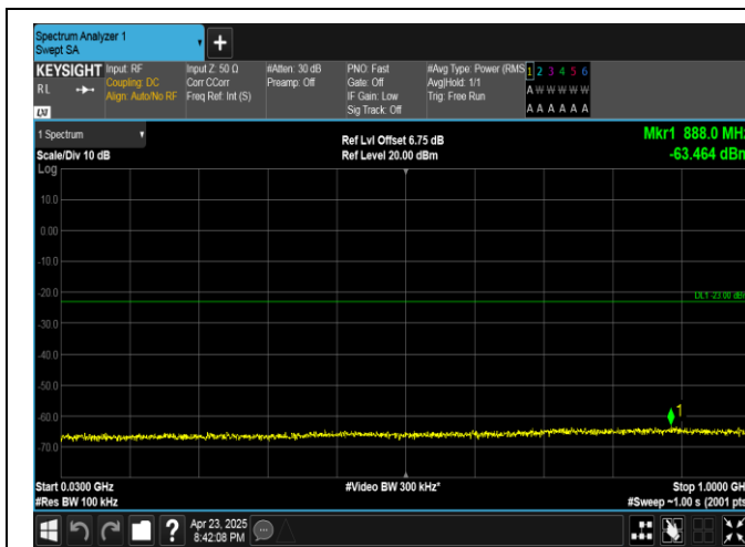
Band25-1.4MHz-QPSK-26683-6RB#0-30~1000-PASS
