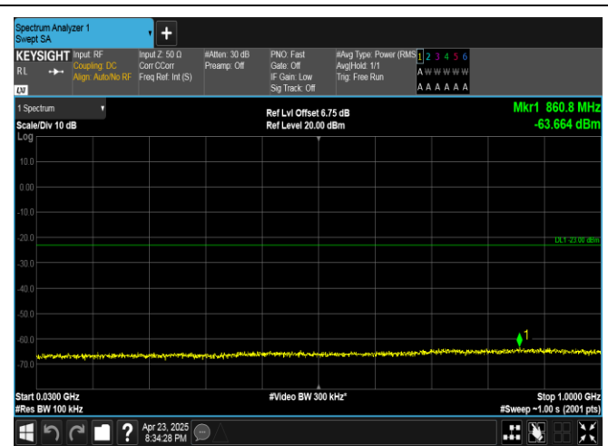
Band25-1.4MHz-16QAM-26365-1RB#5-30~1000-PASS
