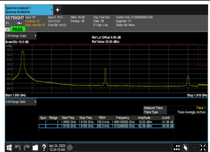
Band25-20MHz-16QAM-26590-1RB#0-PASS
