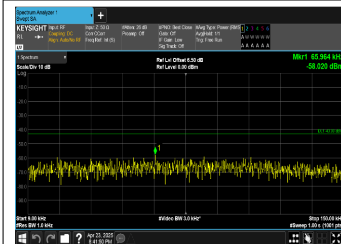
Band25-1.4MHz-QPSK-26683-6RB#0-0.009~0.15-PASS
