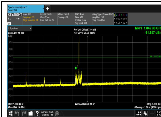
Band25-1.4MHz-QPSK-26365-1RB#0-1000~3000-PASS
