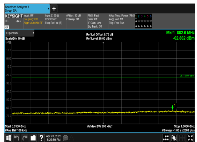
Band25-1.4MHz-16QAM-26047-6RB#0-30~1000-PASS
