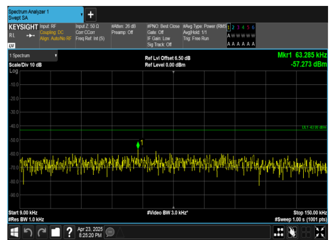
Band25-1.4MHz-16QAM-26047-1RB#0-0.009~0.15-PASS
