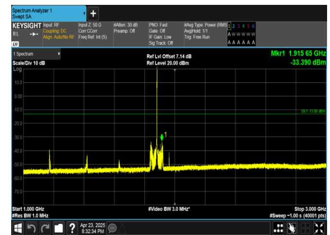
Band25-1.4MHz-16QAM-26365-1RB#0-1000~3000-PASS
