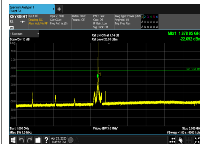
Band25-1.4MHz-QPSK-26365-6RB#0-1000~3000-PASS
