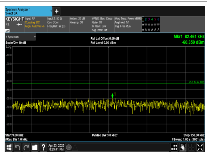
Band25-1.4MHz-16QAM-26047-6RB#0-0.009~0.15-PASS
