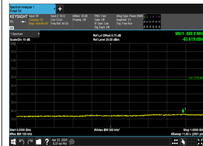
Band25-1.4MHz-QPSK-26683-1RB#0-30~1000-PASS
