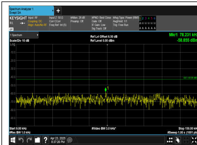
Band25-1.4MHz-QPSK-26683-1RB#0-0.009~0.15-PASS
