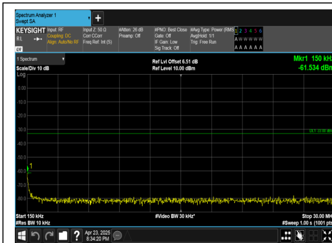
Band25-1.4MHz-16QAM-26365-1RB#5-0.15~30-PASS
