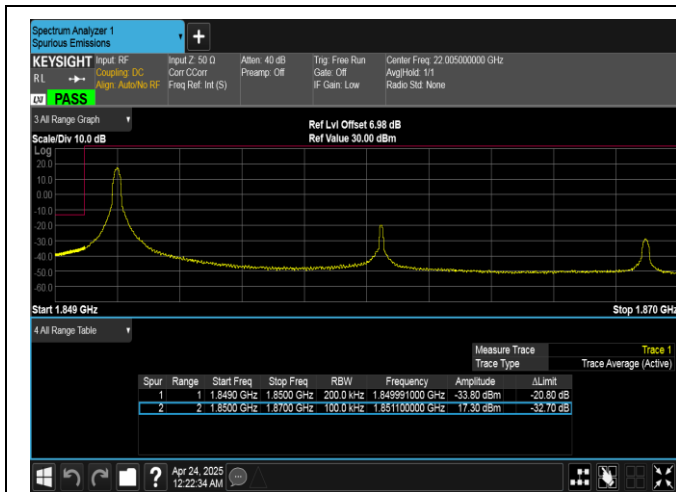
Band25-20MHz-16QAM-26140-1RB#0-PASS
