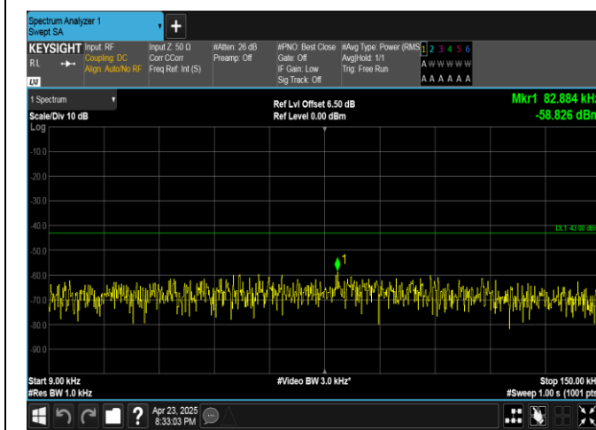
Band25-1.4MHz-QPSK-26365-1RB#5-0.009~0.15-PASS
