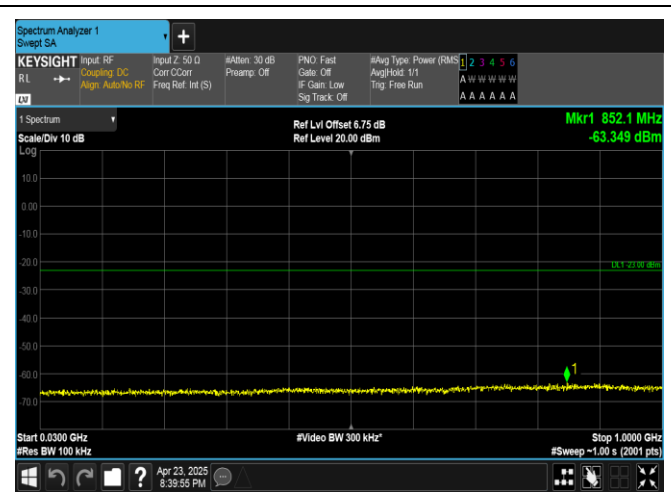
Band25-1.4MHz-QPSK-26683-1RB#5-30~1000-PASS
