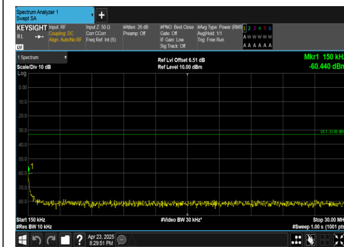
Band25-1.4MHz-16QAM-26047-6RB#0-0.15~30-PASS
