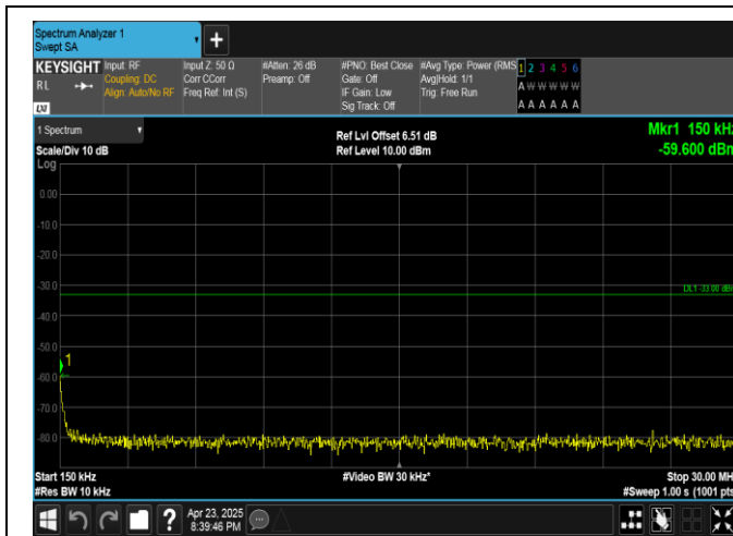
Band25-1.4MHz-QPSK-26683-1RB#5-0.15~30-PASS
