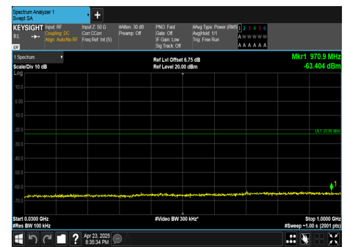
Band25-1.4MHz-QPSK-26365-6RB#0-30~1000-PASS
