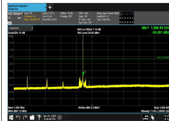
Band25-1.4MHz-16QAM-26365-1RB#5-1000~3000-PASS
