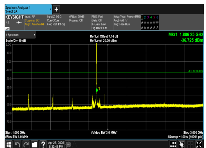
Band25-1.4MHz-QPSK-26365-1RB#5-1000~3000-PASS
