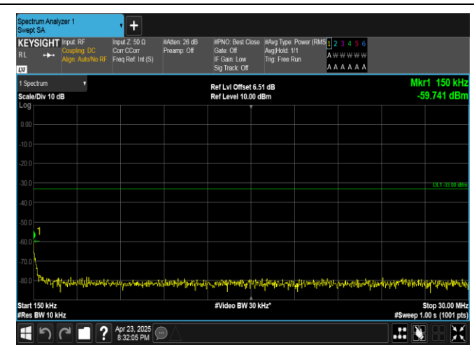
Band25-1.4MHz-16QAM-26365-1RB#0-0.15~30-PASS
