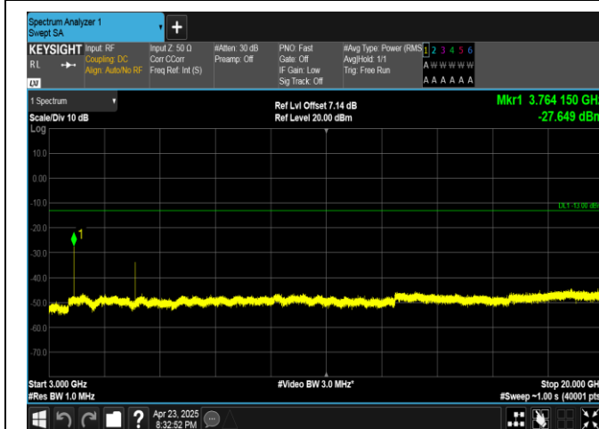
Band25-1.4MHz-16QAM-26365-1RB#0-3000~20000-PASS
