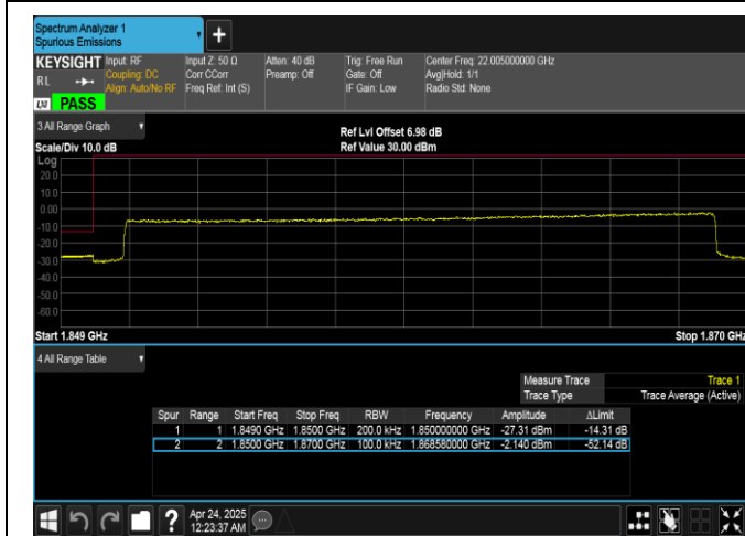
Band25-20MHz-16QAM-26140-100RB#0-PASS
