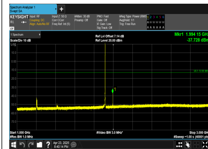
Band25-1.4MHz-QPSK-26683-1RB#5-1000~3000-PASS
