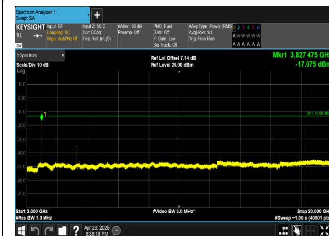
Band25-1.4MHz-QPSK-26683-1RB#0-3000~20000-PASS
