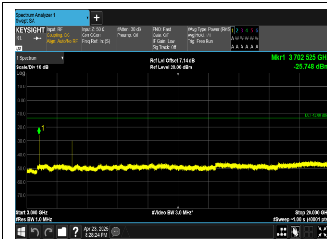
Band25-1.4MHz-16QAM-26047-1RB#5-3000~20000-PASS
