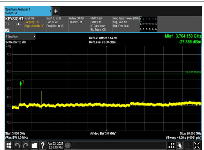
Band25-1.4MHz-QPSK-26365-1RB#0-3000~20000-PASS
