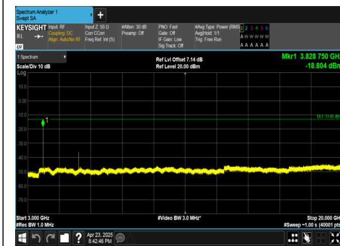
Band25-1.4MHz-QPSK-26683-6RB#0-3000~20000-PASS
