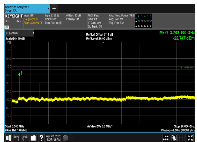
Band25-1.4MHz-QPSK-26047-1RB#5-3000~20000-PASS
