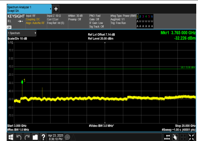
Band25-1.4MHz-QPSK-26365-6RB#0-3000~20000-PASS
