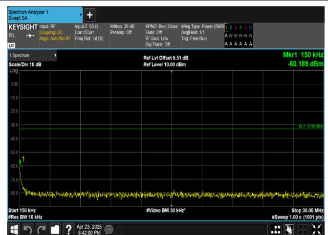
Band25-1.4MHz-QPSK-26683-6RB#0-0.15~30-PASS
