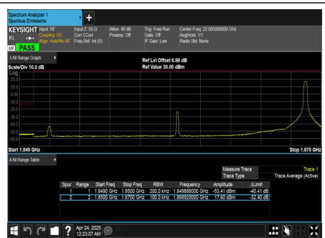
Band25-20MHz-16QAM-26140-1RB#99-PASS
