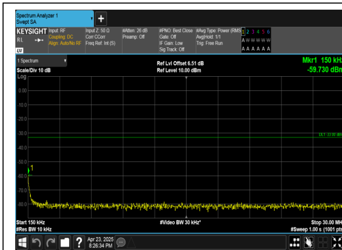
Band25-1.4MHz-QPSK-26047-1RB#5-0.15~30-PASS
