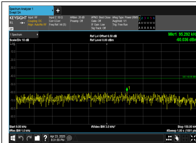
Band25-1.4MHz-16QAM-26365-1RB#0-0.009~0.15-PASS
