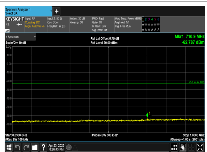
Band25-1.4MHz-QPSK-26047-1RB#5-30~1000-PASS
