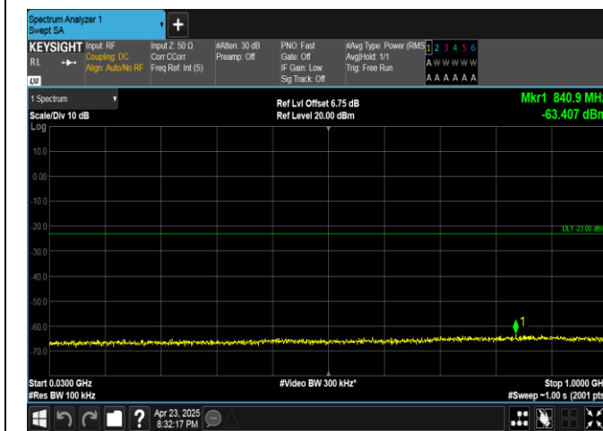
Band25-1.4MHz-16QAM-26365-1RB#0-30~1000-PASS
