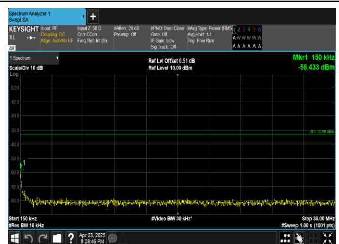
Band25-1.4MHz-QPSK-26047-6RB#0-0.15~30-PASS
