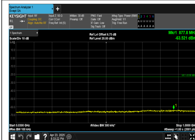
Band25-1.4MHz-QPSK-26365-1RB#5-30~1000-PASS
