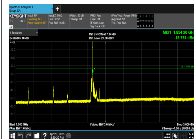
Band25-1.4MHz-16QAM-26047-6RB#0-1000~3000-PASS
