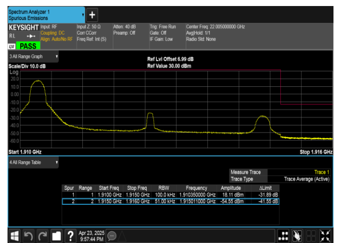
Band25-5MHz-16QAM-26665-1RB#0-PASS
