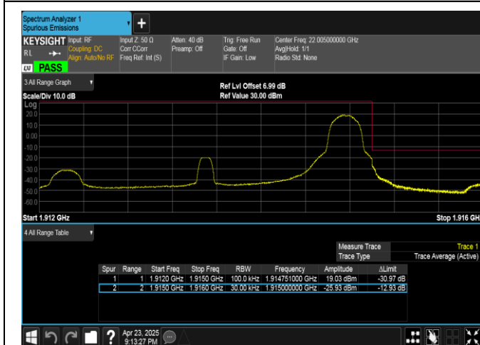
Band25-3MHz-QPSK-26675-1RB#14-PASS
