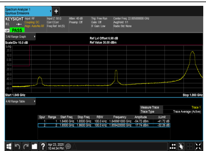
Band25-10MHz-16QAM-26090-1RB#49-PASS
