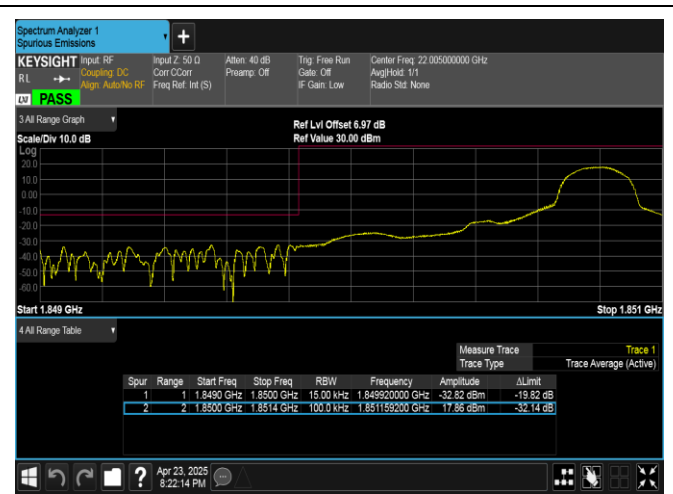
Band25-1.4MHz-16QAM-26047-1RB#5-PASS
