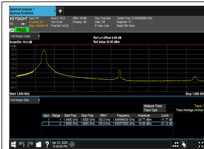
Band25-10MHz-QPSK-26090-1RB#0-PASS
