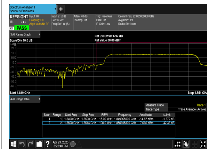
Band25-1.4MHz-16QAM-26047-6RB#0-PASS
