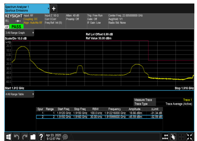
Band25-3MHz-QPSK-26675-1RB#0-PASS
