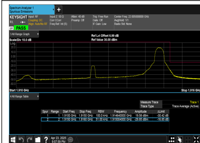
Band25-5MHz-QPSK-26665-1RB#24-PASS
