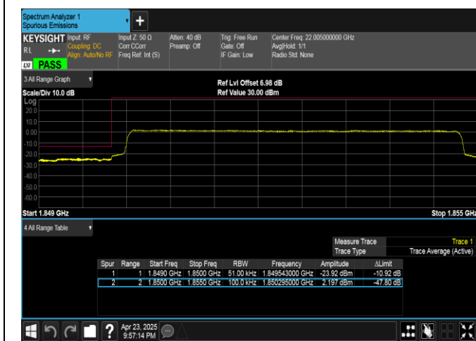
Band25-5MHz-16QAM-26065-25RB#0-PASS
