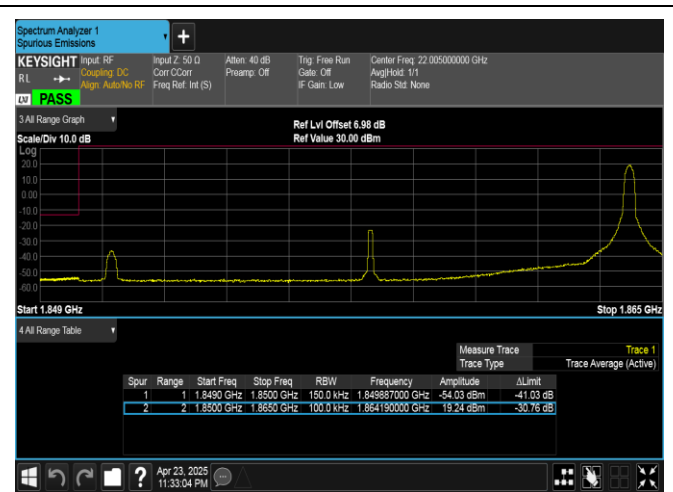
Band25-15MHz-QPSK-26115-1RB#74-PASS
