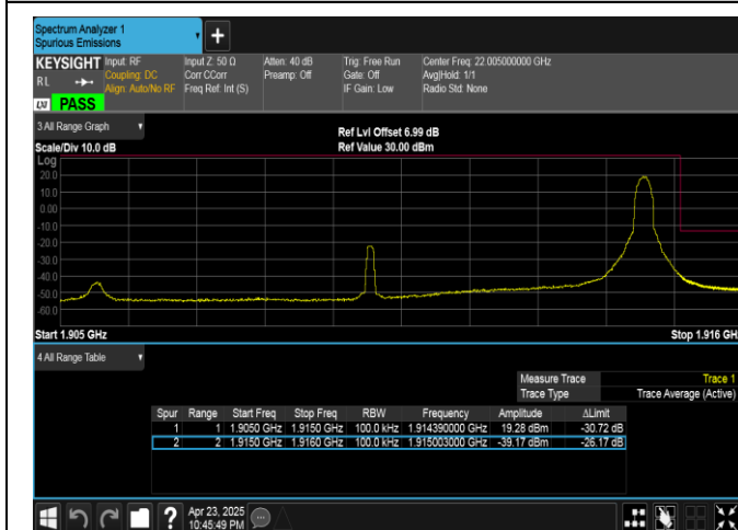
Band25-10MHz-QPSK-26640-1RB#49-PASS
