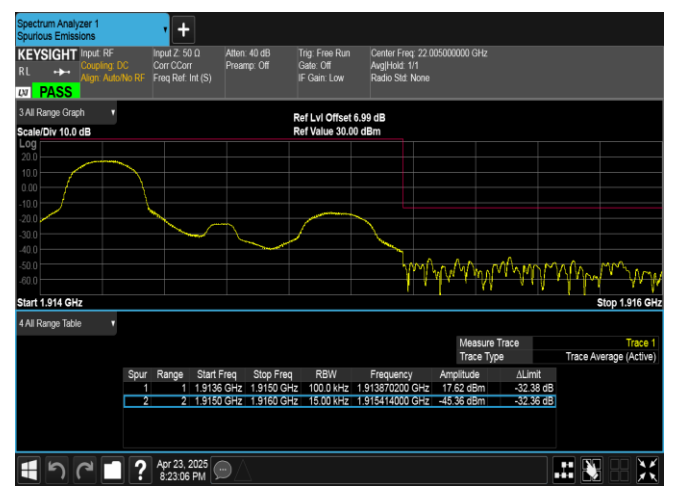
Band25-1.4MHz-16QAM-26683-1RB#0-PASS
