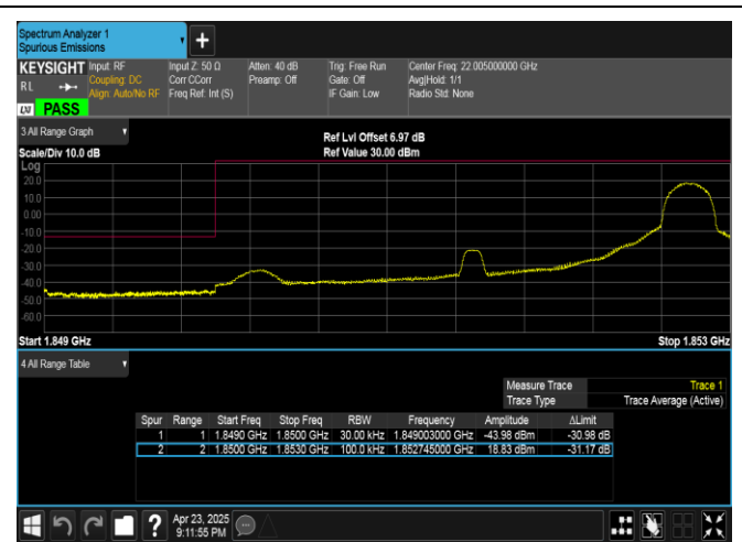
Band25-3MHz-QPSK-26055-1RB#14-PASS
