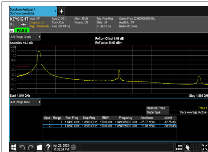
Band25-15MHz-QPSK-26115-1RB#0-PASS
