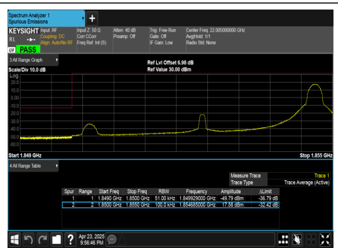
Band25-5MHz-16QAM-26065-1RB#24-PASS
