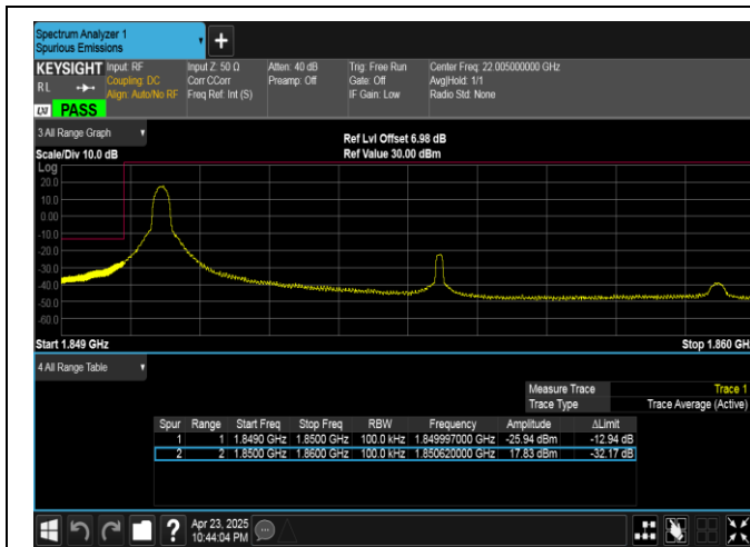
Band25-10MHz-16QAM-26090-1RB#0-PASS
