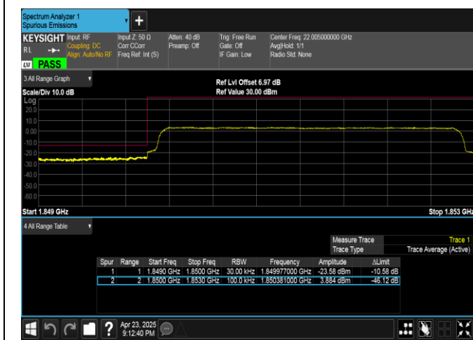
Band25-3MHz-16QAM-26055-15RB#0-PASS
