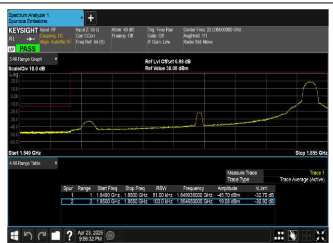
Band25-5MHz-QPSK-26065-1RB#24-PASS
