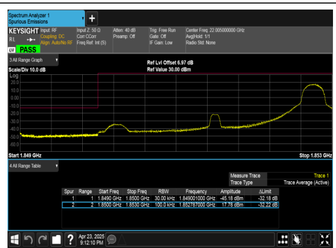
Band25-3MHz-16QAM-26055-1RB#14-PASS
