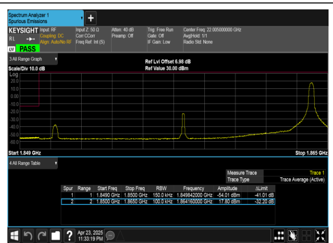
Band25-15MHz-16QAM-26115-1RB#74-PASS
