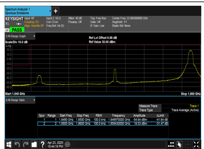
Band25-10MHz-QPSK-26090-1RB#49-PASS
