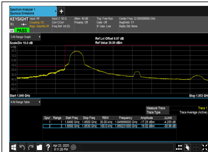
Band25-3MHz-QPSK-26055-1RB#0-PASS
