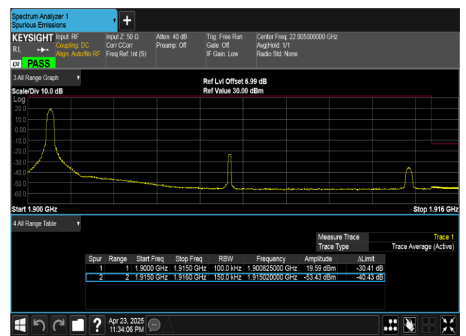
Band25-15MHz-QPSK-26615-1RB#0-PASS
