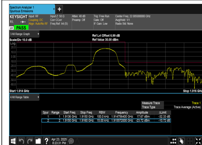
Band25-1.4MHz-16QAM-26683-1RB#5-PASS
