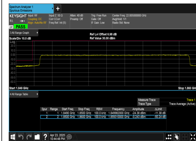
Band25-10MHz-QPSK-26090-50RB#0-PASS
