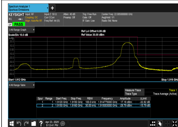
Band25-3MHz-16QAM-26675-1RB#14-PASS
