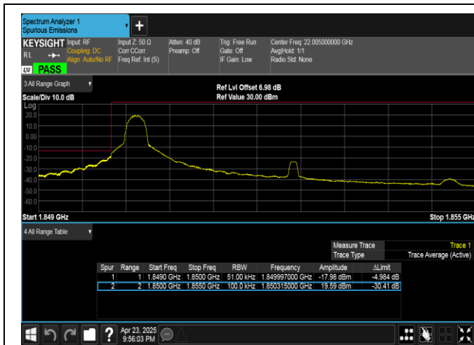
Band25-5MHz-QPSK-26065-1RB#0-PASS
