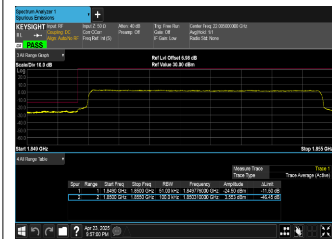
Band25-5MHz-QPSK-26065-25RB#0-PASS
