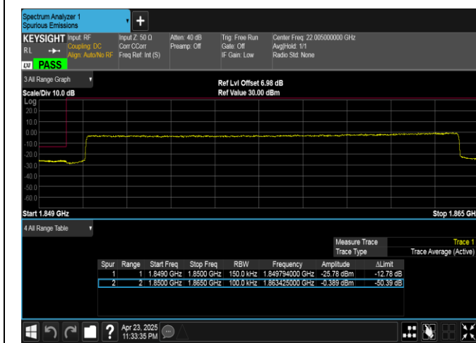
Band25-15MHz-QPSK-26115-75RB#0-PASS
