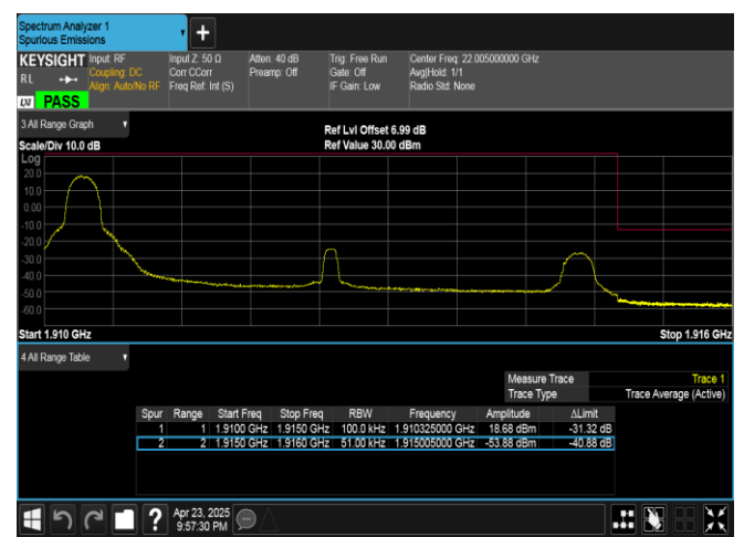
Band25-5MHz-QPSK-26665-1RB#0-PASS
