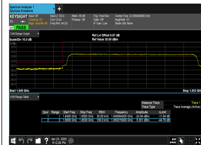
Band25-3MHz-QPSK-26055-15RB#0-PASS
