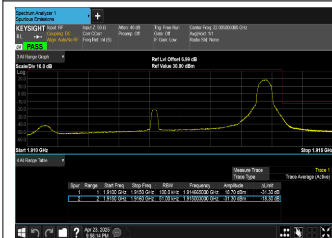
Band25-5MHz-16QAM-26665-1RB#24-PASS
