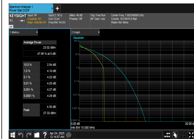
Band25-15MHz-QPSK-26365-1RB#0-PASS
