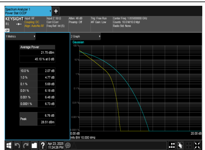
Band25-10MHz-QPSK-26090-50RB#0-PASS
