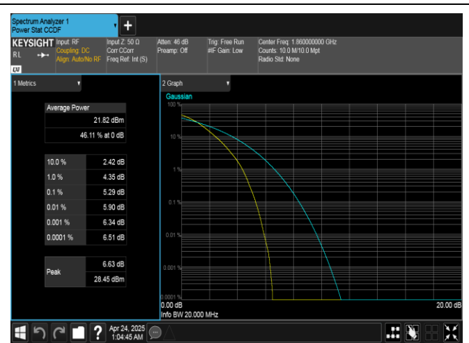
Band25-20MHz-QPSK-26140-100RB#0-PASS
