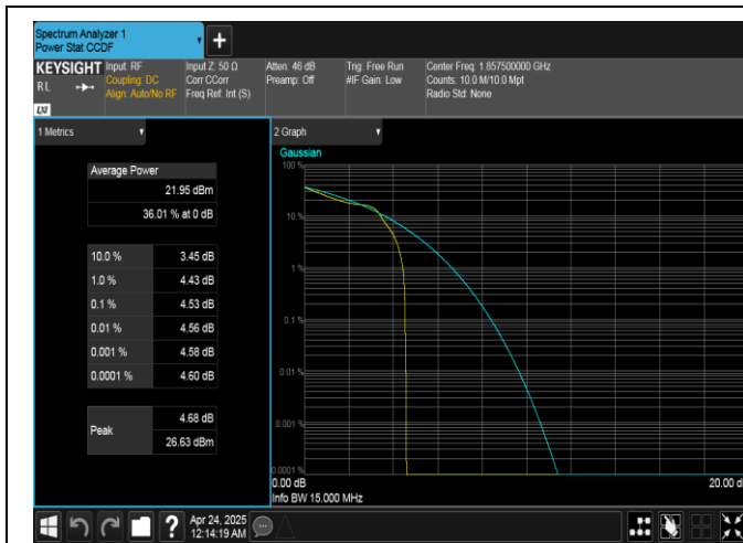
Band25-15MHz-16QAM-26115-1RB#0-PASS
