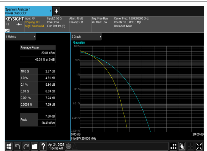
Band25-20MHz-16QAM-26140-100RB#0-PASS
