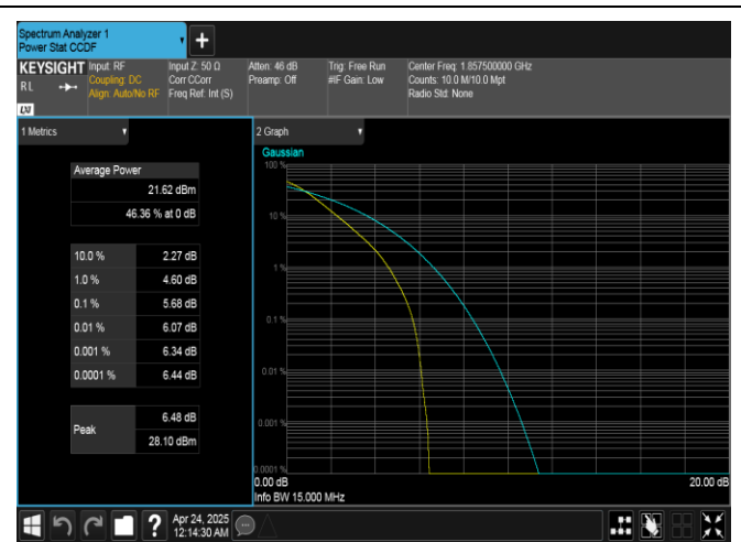
Band25-15MHz-QPSK-26115-75RB#0-PASS
