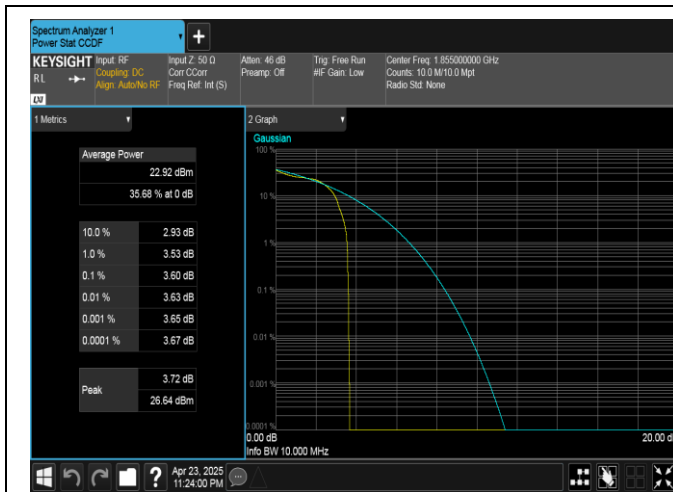
Band25-10MHz-QPSK-26090-1RB#0-PASS
