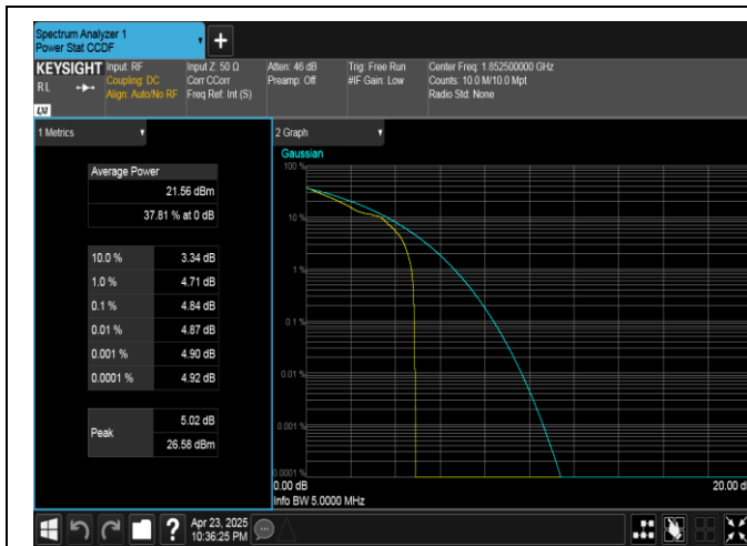
Band25-5MHz-16QAM-26065-1RB#0-PASS
