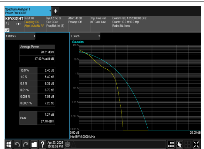
Band25-5MHz-16QAM-26065-25RB#0-PASS
