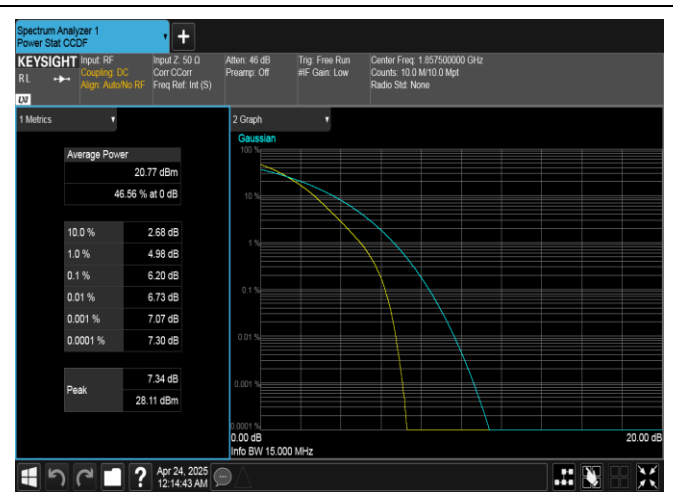
Band25-15MHz-16QAM-26115-75RB#0-PASS
