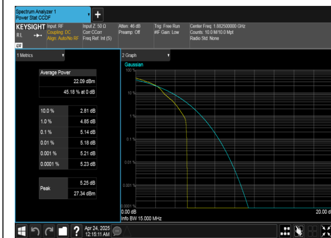
Band25-15MHz-16QAM-26365-1RB#0-PASS
