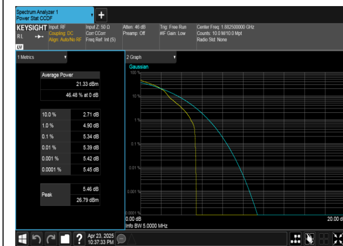
Band25-5MHz-16QAM-26365-1RB#0-PASS
