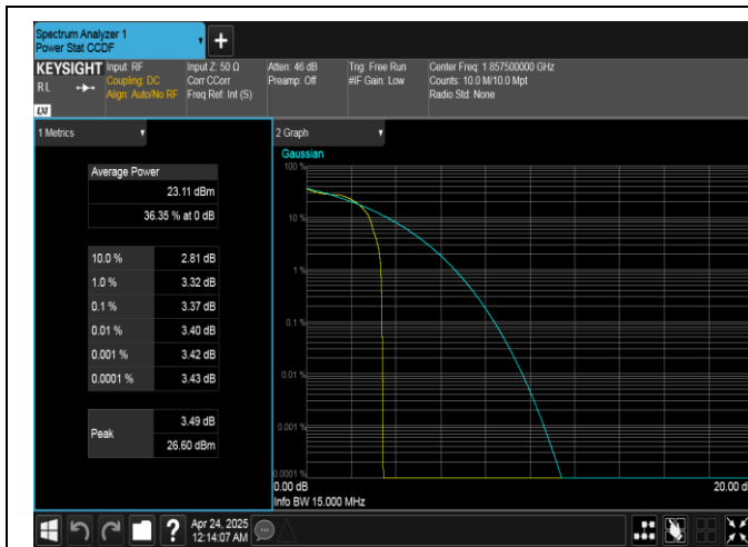
Band25-15MHz-QPSK-26115-1RB#0-PASS
