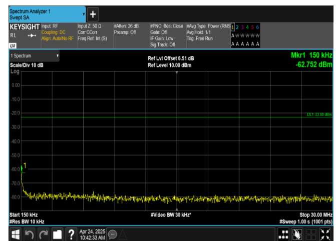
Band17-10MHz-QPSK-23800-50RB#0-0.15~30-PASS
