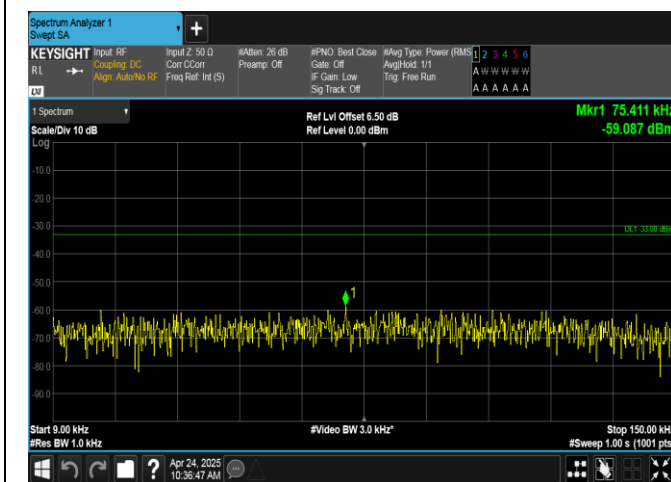
Band17-10MHz-16QAM-23790-50RB#0-0.009~0.15-PASS
