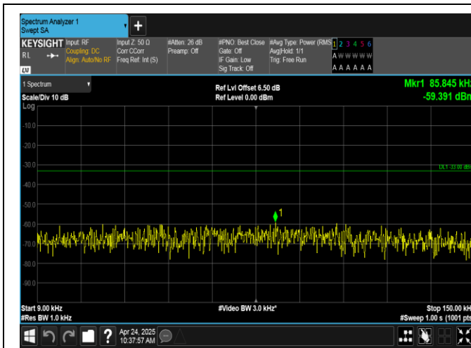
Band17-10MHz-QPSK-23800-1RB#0-0.009~0.15-PASS
