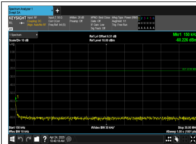
Band17-10MHz-QPSK-23800-1RB#49-0.15~30-PASS
