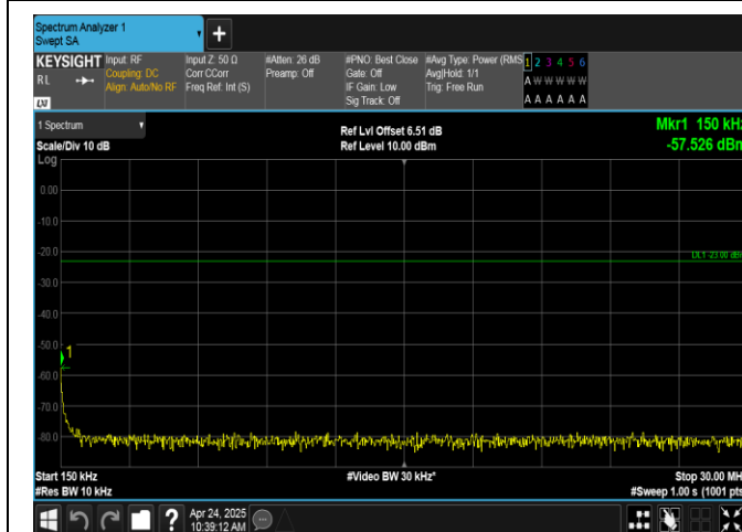
Band17-10MHz-16QAM-23800-1RB#0-0.15~30-PASS
