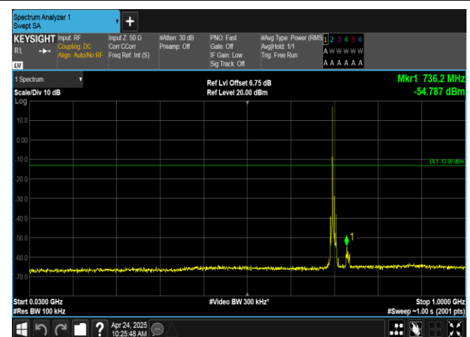
Band17-10MHz-16QAM-23780-1RB#0-30~1000-PASS
