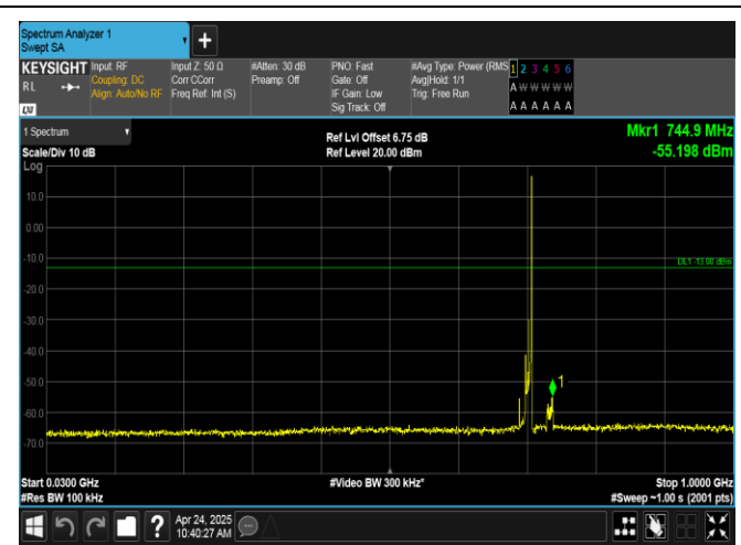
Band17-10MHz-QPSK-23800-1RB#49-30~1000-PASS
