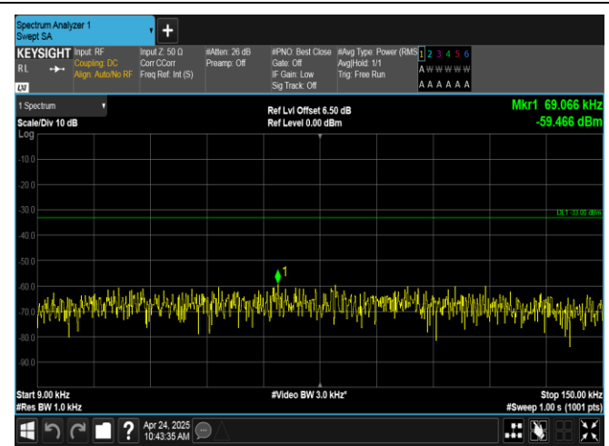
Band17-10MHz-16QAM-23800-50RB#0-0.009~0.15-PASS
