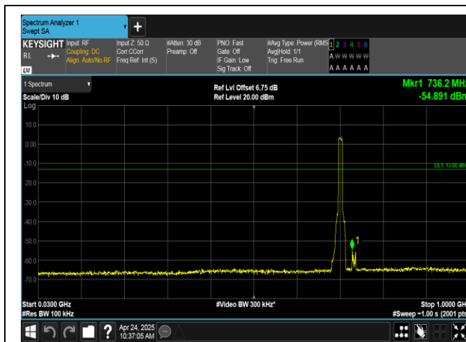
Band17-10MHz-16QAM-23790-50RB#0-30~1000-PASS
