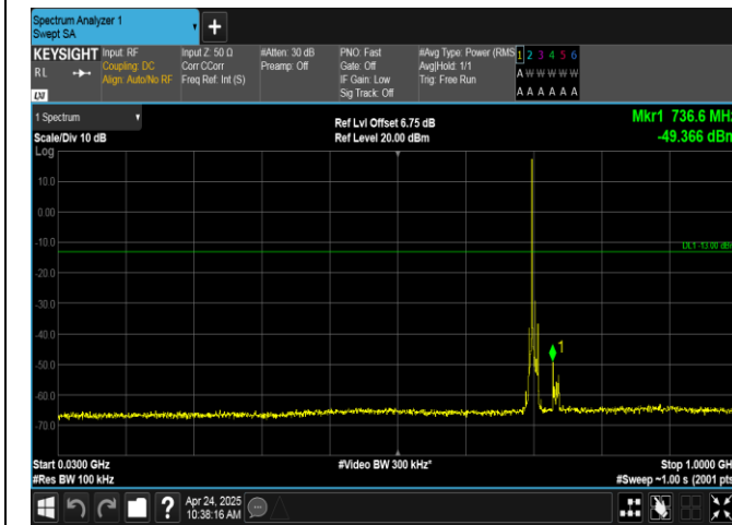
Band17-10MHz-QPSK-23800-1RB#0-30~1000-PASS
