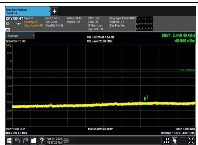
Band17-10MHz-16QAM-23790-50RB#0-1000~3000-PASS
