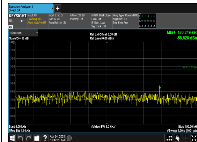
Band17-10MHz-QPSK-23800-50RB#0-0.009~0.15-PASS
