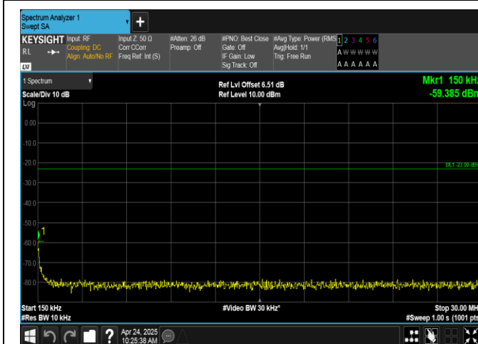
Band17-10MHz-16QAM-23780-1RB#0-0.15~30-PASS
