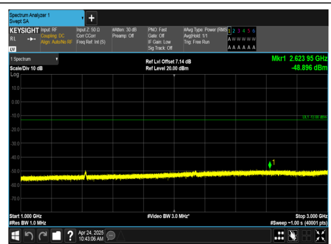
Band17-10MHz-QPSK-23800-50RB#0-1000~3000-PASS
