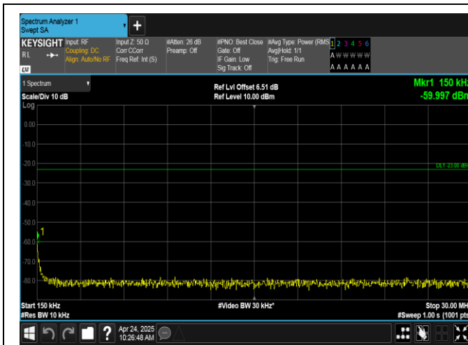
Band17-10MHz-QPSK-23780-1RB#49-0.15~30-PASS
