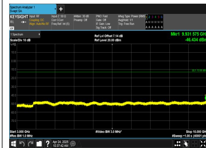
Band17-10MHz-16QAM-23790-50RB#0-3000~10000-PASS
