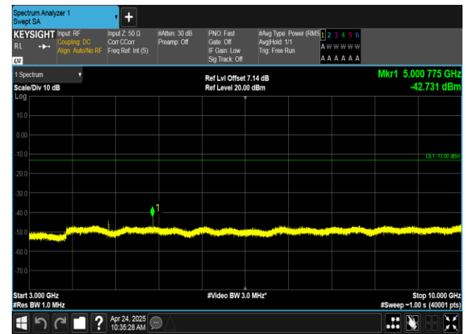
Band17-10MHz-16QAM-23790-1RB#49-3000~10000-PASS
