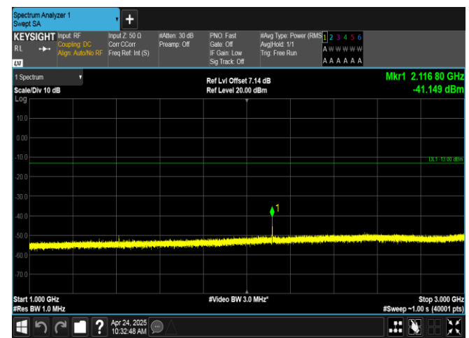
Band17-10MHz-16QAM-23790-1RB#0-1000~3000-PASS
