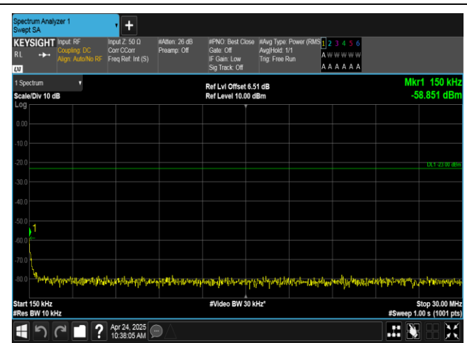
Band17-10MHz-QPSK-23800-1RB#0-0.15~30-PASS
