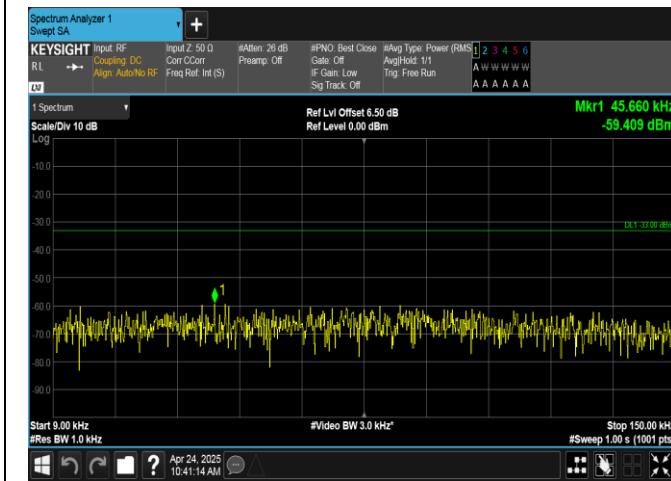
Band17-10MHz-16QAM-23800-1RB#49-0.009~0.15-PASS
