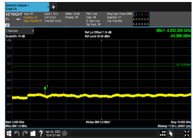
Band17-10MHz-QPSK-23800-1RB#49-3000~10000-PASS
