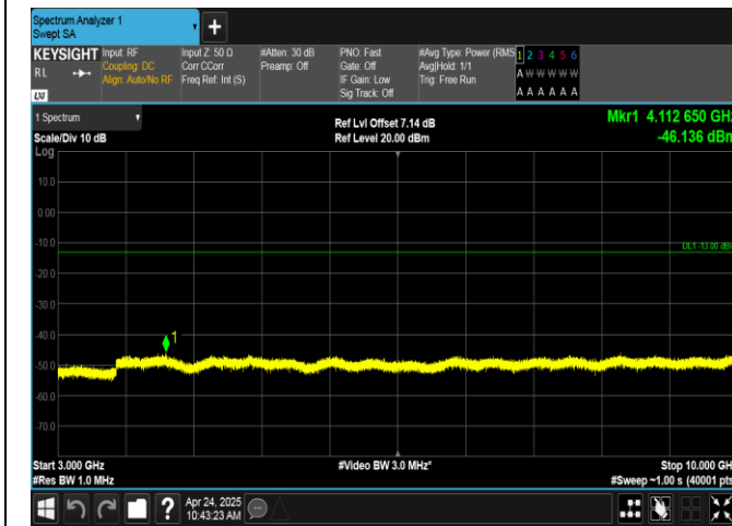
Band17-10MHz-QPSK-23800-50RB#0-3000~10000-PASS
