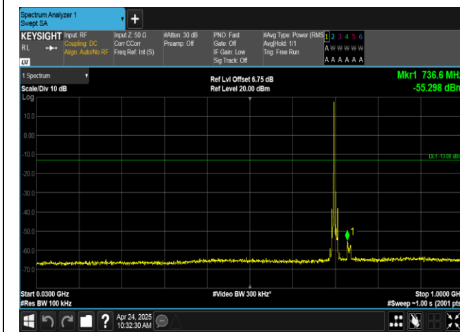
Band17-10MHz-16QAM-23790-1RB#0-30~1000-PASS
