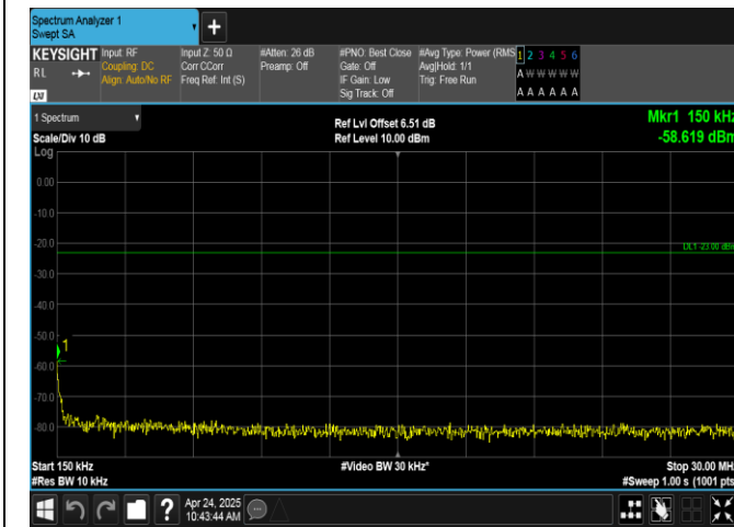
Band17-10MHz-16QAM-23800-50RB#0-0.15~30-PASS
