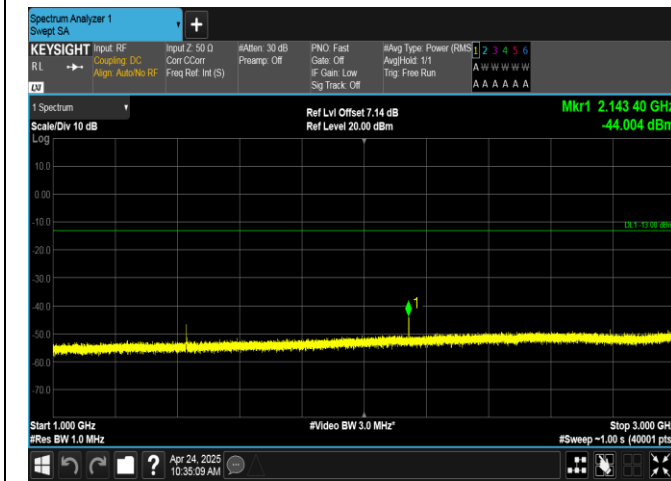
Band17-10MHz-16QAM-23790-1RB#49-1000~3000-PASS
