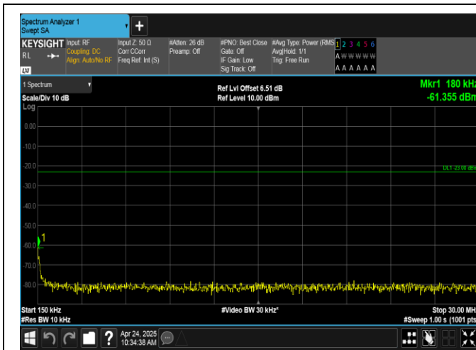
Band17-10MHz-16QAM-23790-1RB#49-0.15~30-PASS
