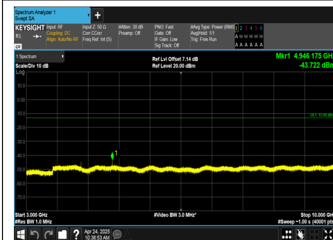
Band17-10MHz-QPSK-23800-1RB#0-3000~10000-PASS
