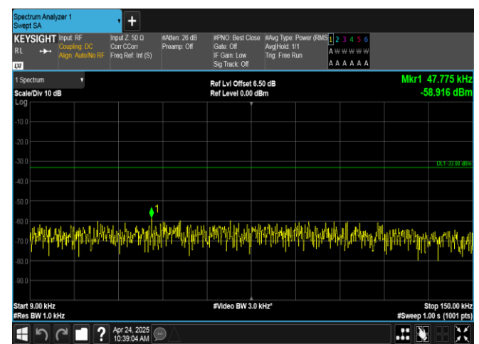
Band17-10MHz-16QAM-23800-1RB#0-0.009~0.15-PASS
