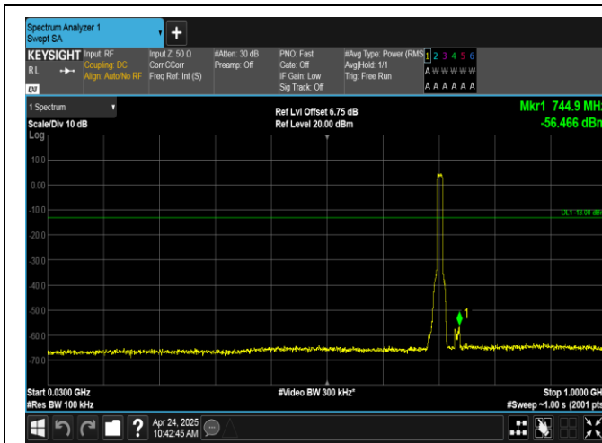
Band17-10MHz-QPSK-23800-50RB#0-30~1000-PASS
