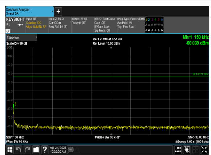
Band17-10MHz-16QAM-23790-1RB#0-0.15~30-PASS
