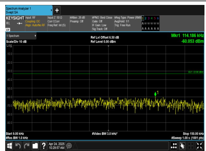
Band17-10MHz-16QAM-23780-50RB#0-0.009~0.15-PASS
