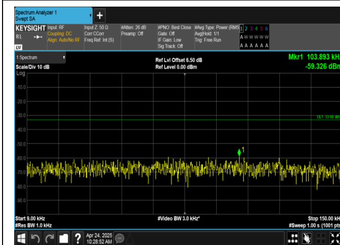
Band17-10MHz-QPSK-23780-50RB#0-0.009~0.15-PASS
