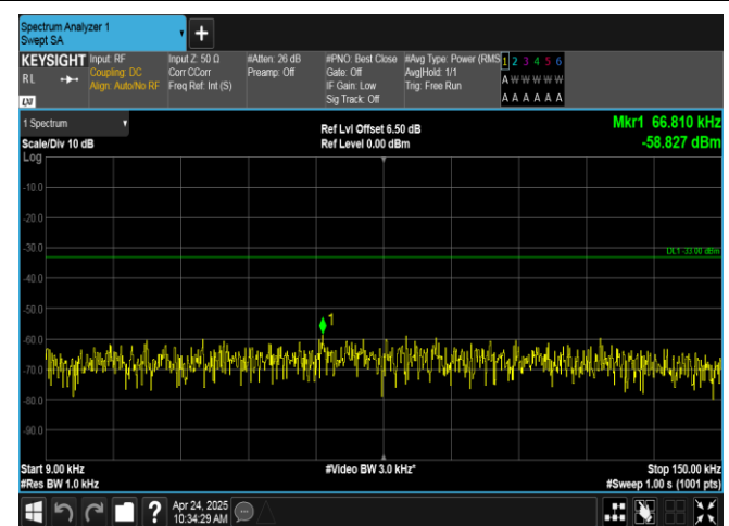
Band17-10MHz-16QAM-23790-1RB#49-0.009~0.15-PASS
