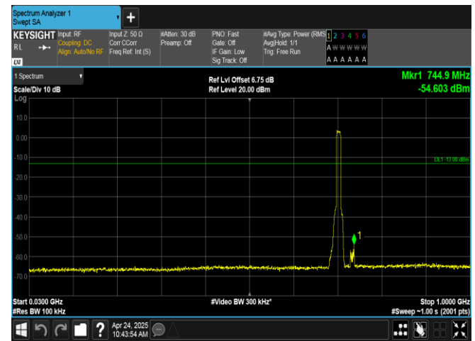
Band17-10MHz-16QAM-23800-50RB#0-30~1000-PASS
