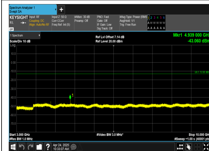
Band17-10MHz-16QAM-23790-1RB#0-3000~10000-PASS
