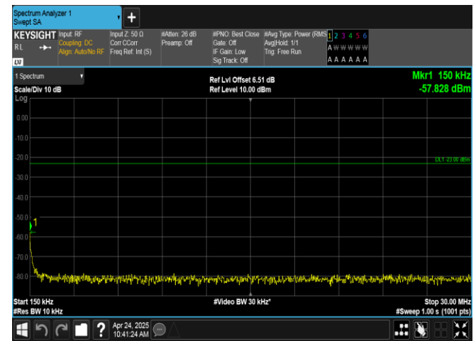
Band17-10MHz-16QAM-23800-1RB#49-0.15~30-PASS
