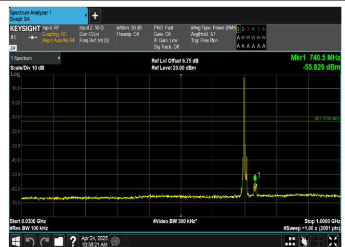
Band17-10MHz-16QAM-23800-1RB#0-30~1000-PASS
