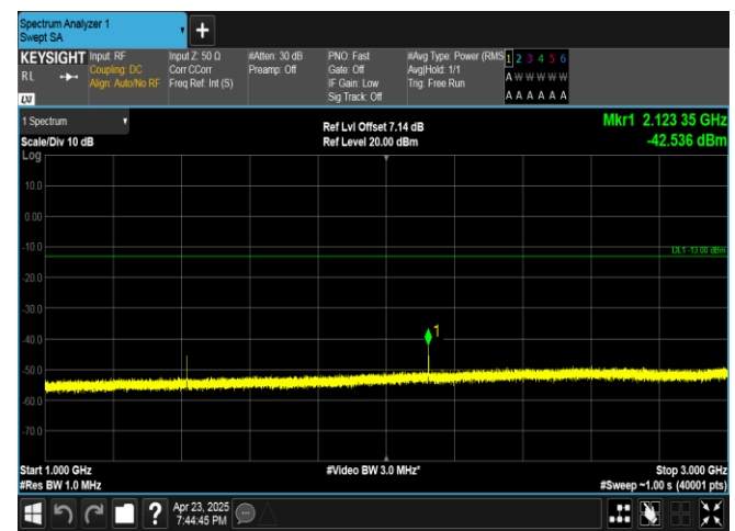
Band17-5MHz-16QAM-23790-1RB#0-1000~3000-PASS
