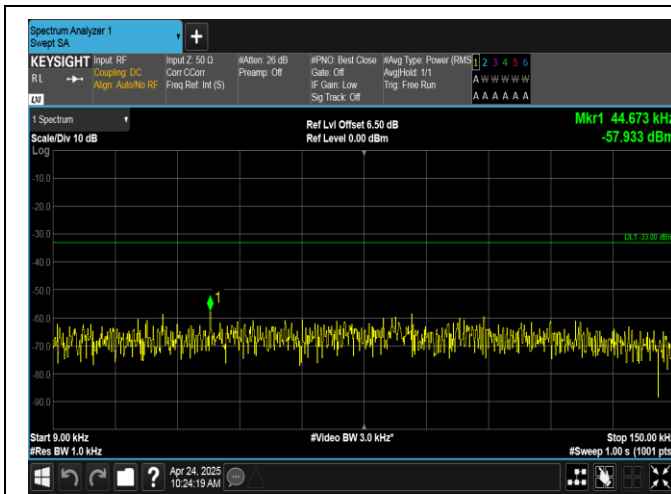
Band17-10MHz-QPSK-23780-1RB#0-0.009~0.15-PASS
