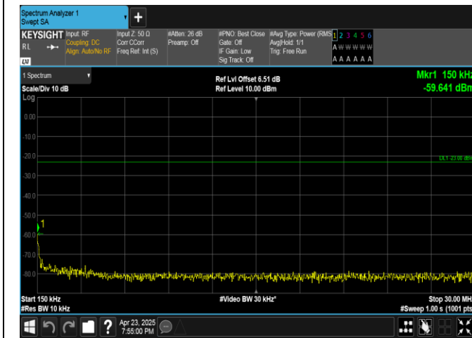
Band17-5MHz-16QAM-23825-25RB#0-0.15~30-PASS
