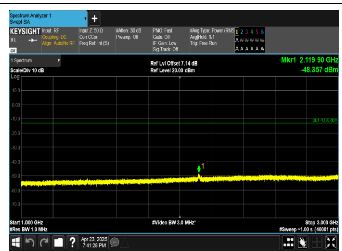
Band17-5MHz-QPSK-23755-25RB#0-1000~3000-PASS
