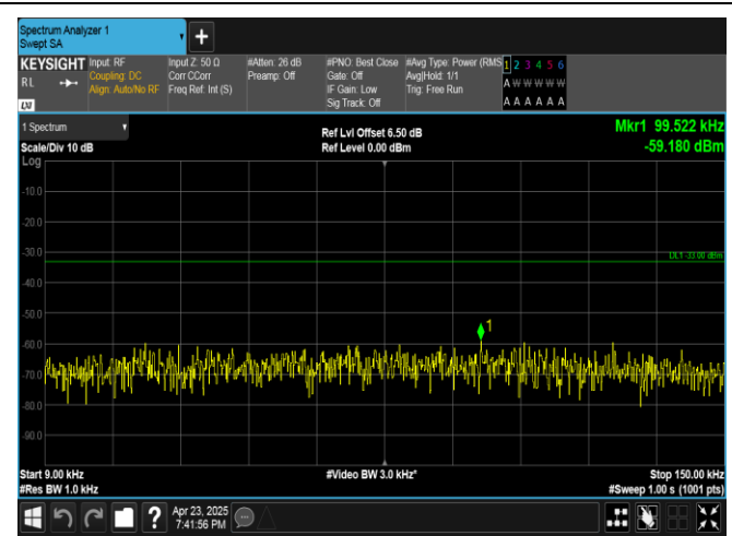
Band17-5MHz-16QAM-23755-25RB#0-0.009~0.15-PASS
