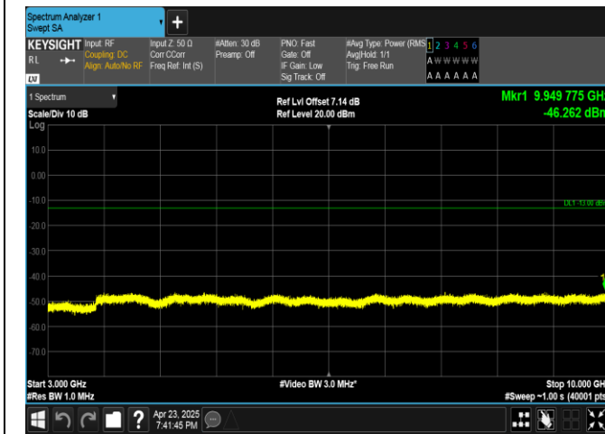
Band17-5MHz-QPSK-23755-25RB#0-3000~10000-PASS
