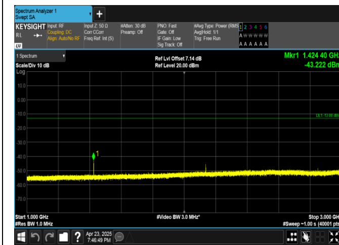
Band17-5MHz-16QAM-23790-1RB#24-1000~3000-PASS
