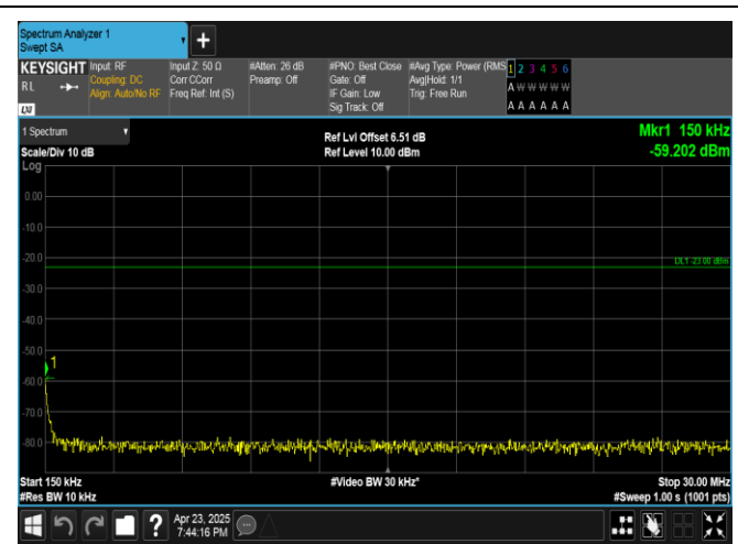
Band17-5MHz-16QAM-23790-1RB#0-0.15~30-PASS
