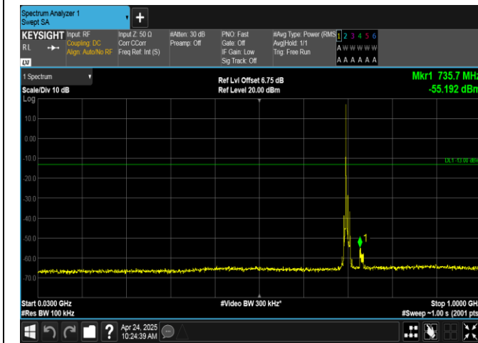
Band17-10MHz-QPSK-23780-1RB#0-30~1000-PASS
