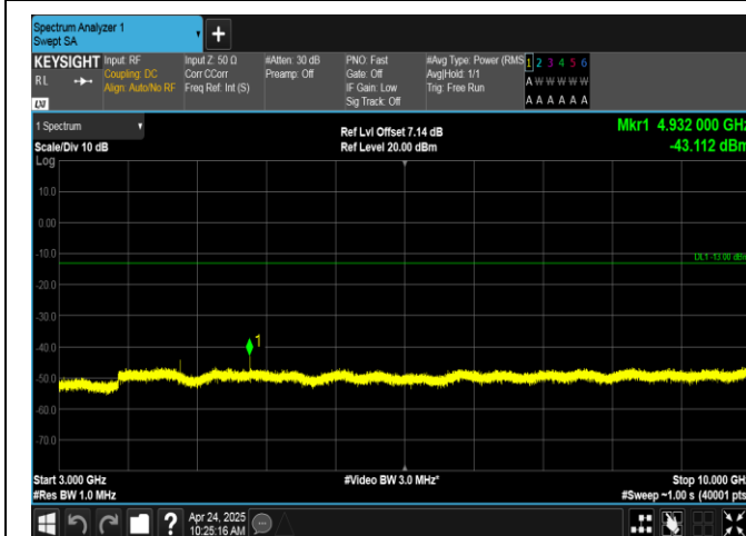
Band17-10MHz-QPSK-23780-1RB#0-3000~10000-PASS
