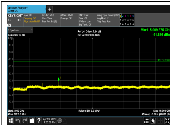
Band17-5MHz-16QAM-23825-1RB#24-3000~10000-PASS
