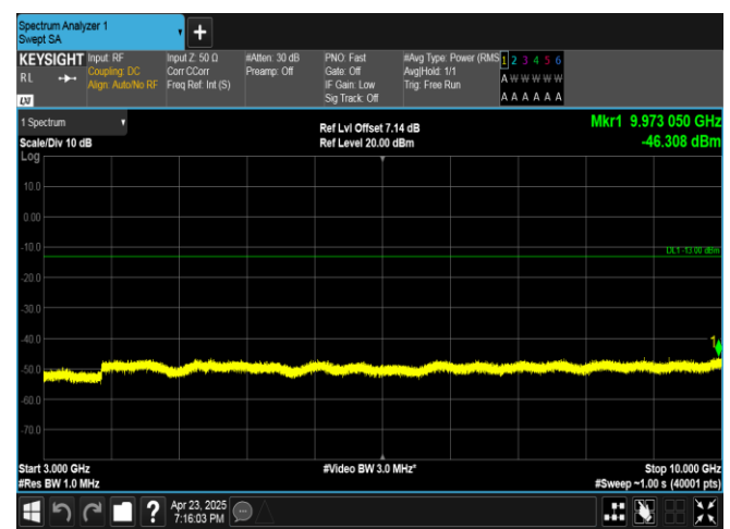
Band13-10MHz-16QAM-23230-1RB#0-3000~10000-PASS
