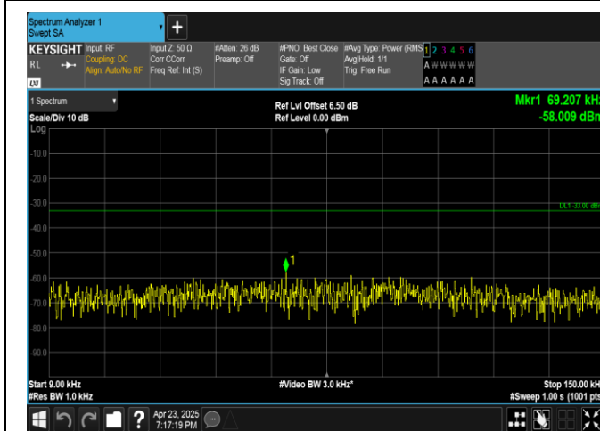
Band13-10MHz-16QAM-23230-1RB#49-0.009~0.15-PASS
