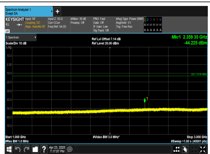
Band13-10MHz-16QAM-23230-1RB#49-1000~3000-PASS
