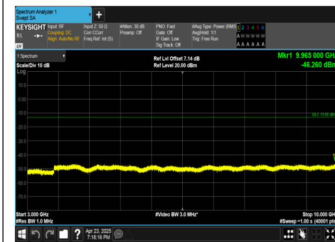
Band13-10MHz-16QAM-23230-1RB#49-3000~10000-PASS
