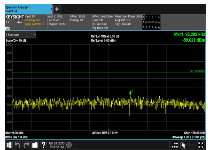
Band13-10MHz-16QAM-23230-50RB#0-0.009~0.15-PASS
