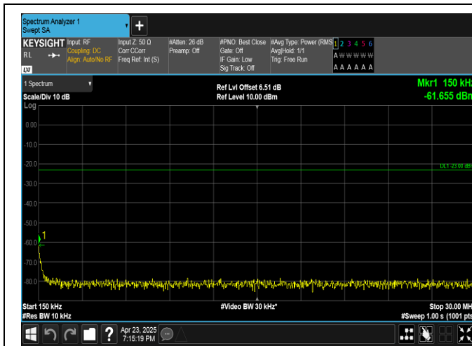
Band13-10MHz-16QAM-23230-1RB#0-0.15~30-PASS
