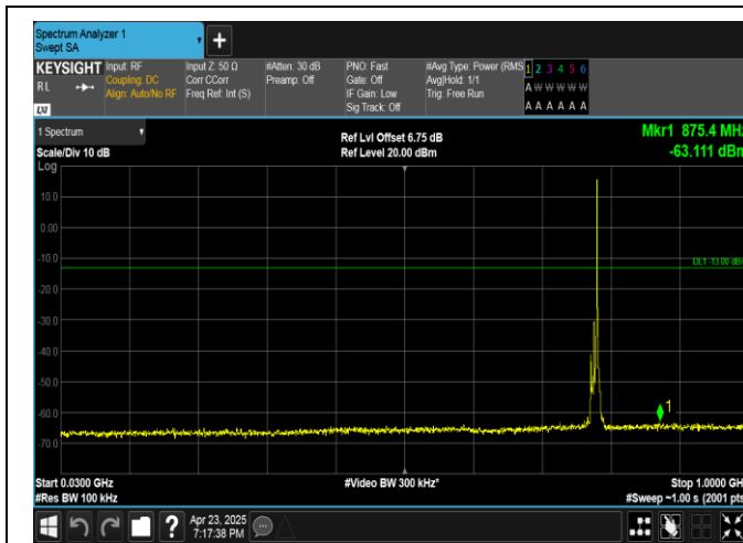
Band13-10MHz-16QAM-23230-1RB#49-30~1000-PASS
