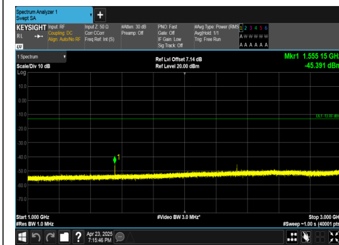
Band13-10MHz-16QAM-23230-1RB#0-1000~3000-PASS
