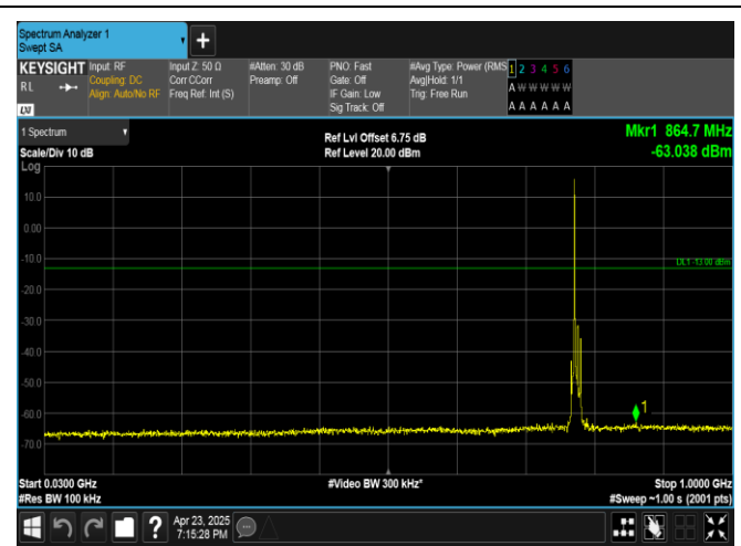
Band13-10MHz-16QAM-23230-1RB#0-30~1000-PASS
