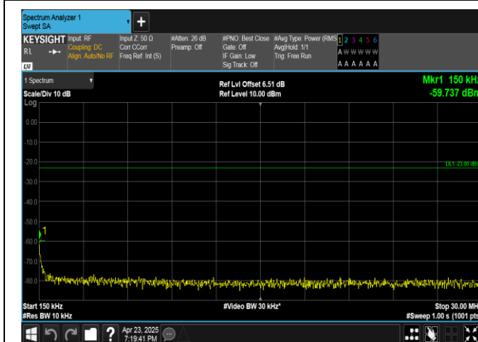
Band13-10MHz-16QAM-23230-50RB#0-0.15~30-PASS
