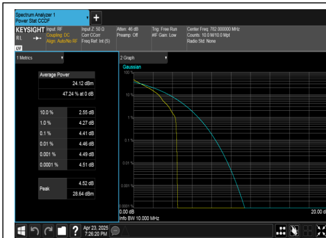
Band13-10MHz-QPSK-23230-1RB#0-PASS
