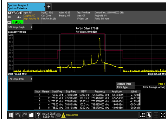
Band13-5MHz-QPSK-23255-1RB#24-PASS
