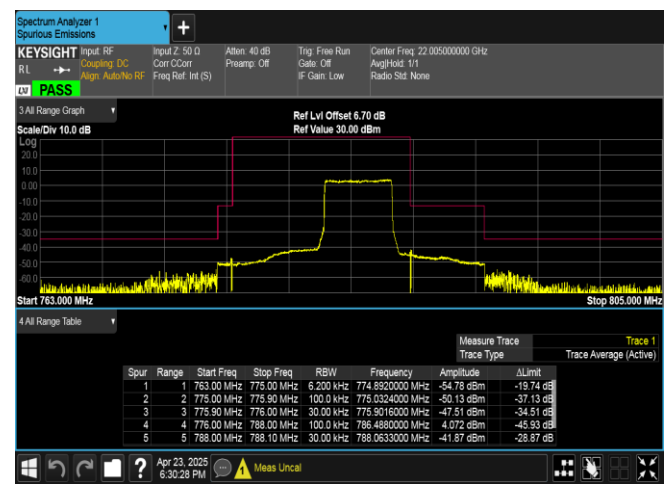
Band13-5MHz-QPSK-23255-25RB#0-PASS
