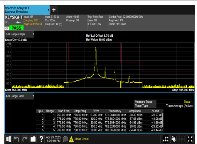
Band13-5MHz-QPSK-23255-1RB#0-PASS
