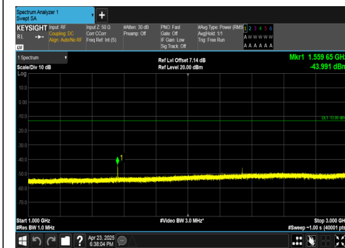
Band13-5MHz-QPSK-23230-1RB#0-1000~3000-PASS
