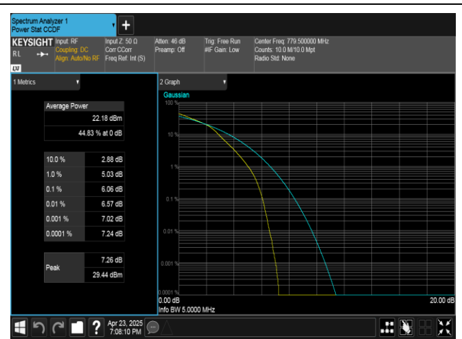
Band13-5MHz-16QAM-23205-25RB#0-PASS
