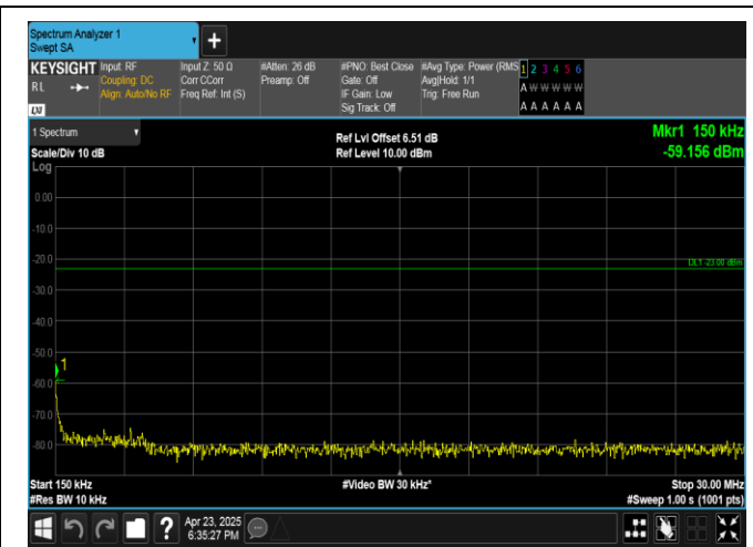
Band13-5MHz-QPSK-23205-25RB#0-0.15~30-PASS
