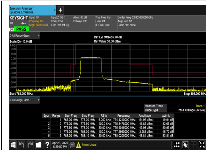
Band13-5MHz-16QAM-23205-25RB#0-PASS
