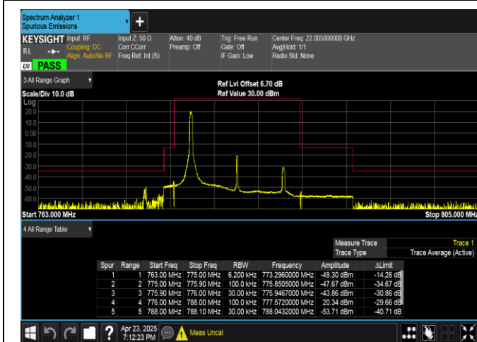
Band13-10MHz-QPSK-23230-1RB#0-PASS
