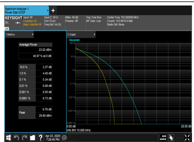
Band13-10MHz-QPSK-23230-50RB#0-PASS
