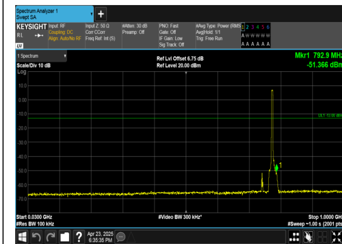
Band13-5MHz-QPSK-23205-25RB#0-30~1000-PASS
