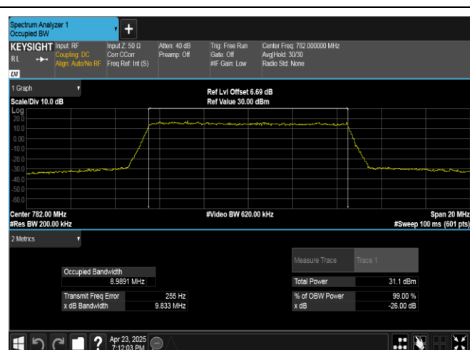
Band13-10MHz-16QAM-23230-50RB#0-PASS
