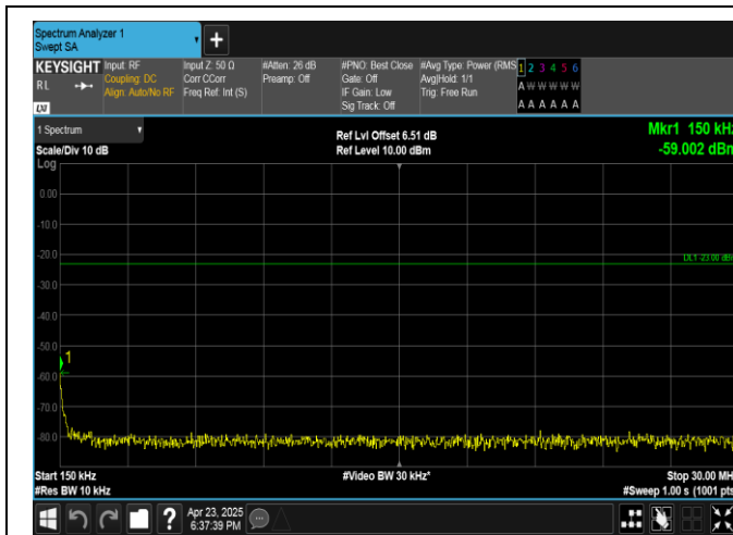
Band13-5MHz-QPSK-23230-1RB#0-0.15~30-PASS
