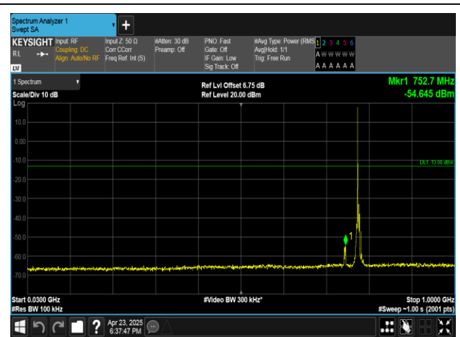
Band13-5MHz-QPSK-23230-1RB#0-30~1000-PASS
