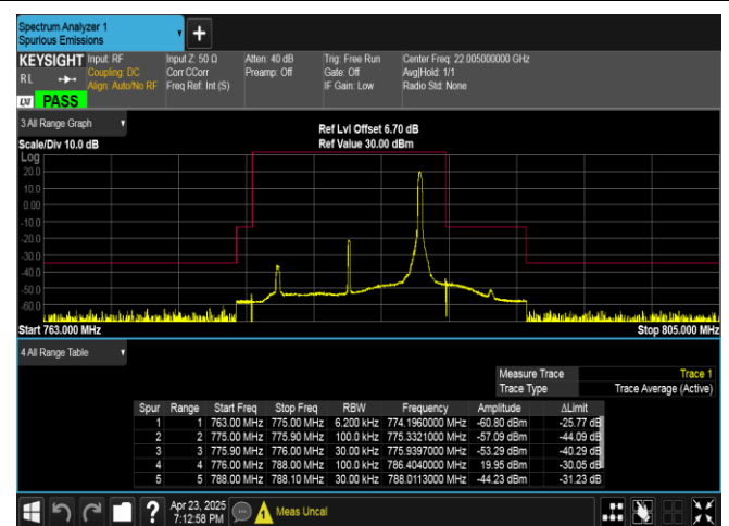
Band13-10MHz-QPSK-23230-1RB#49-PASS
