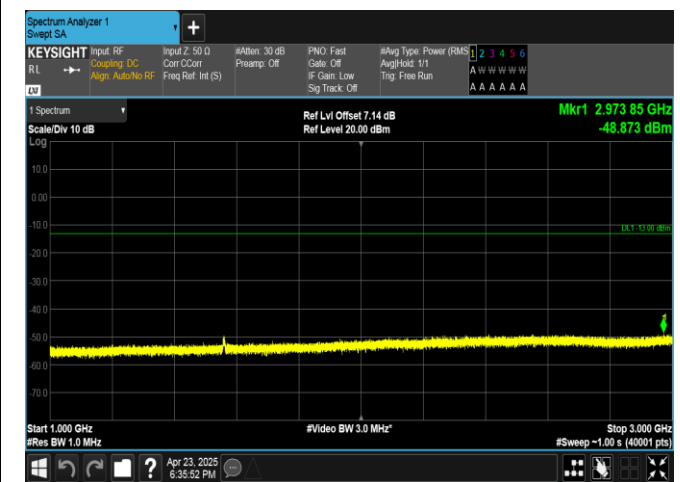
Band13-5MHz-QPSK-23205-25RB#0-1000~3000-PASS
