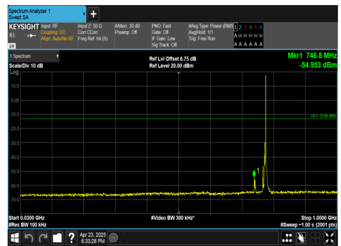
Band13-5MHz-QPSK-23205-1RB#24-30~1000-PASS
