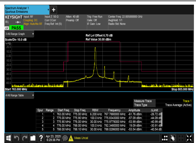
Band13-5MHz-16QAM-23255-1RB#0-PASS
