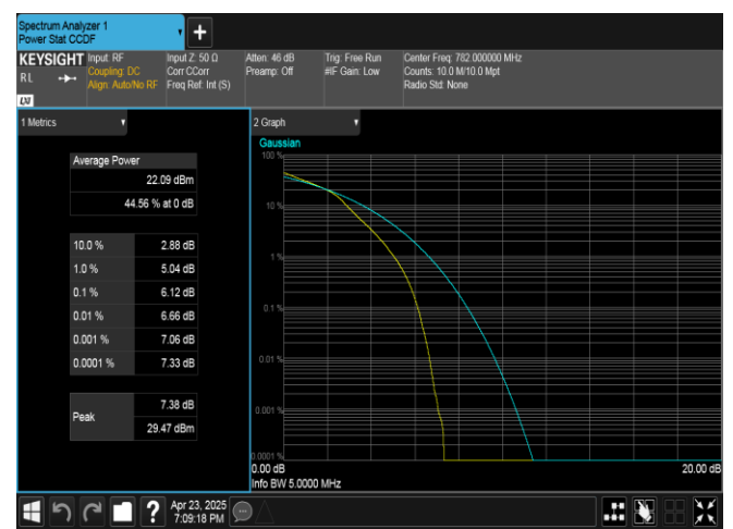
Band13-5MHz-16QAM-23230-25RB#0-PASS
