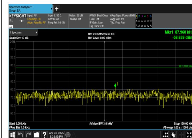
Band13-5MHz-QPSK-23230-1RB#24-0.009~0.15-PASS
