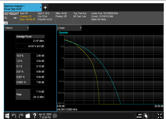
Band13-5MHz-16QAM-23255-25RB#0-PASS
