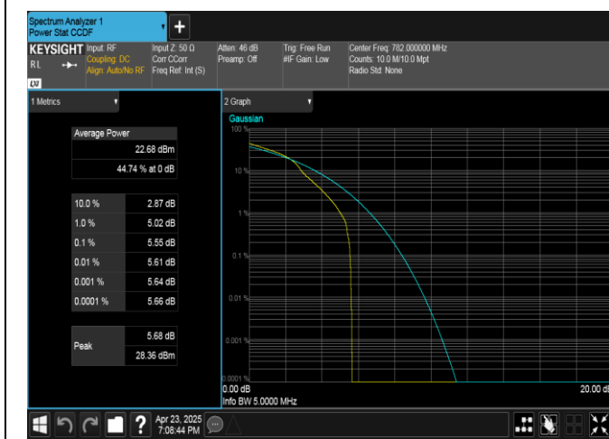
Band13-5MHz-16QAM-23230-1RB#0-PASS
