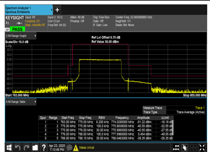
Band13-10MHz-16QAM-23230-50RB#0-PASS
