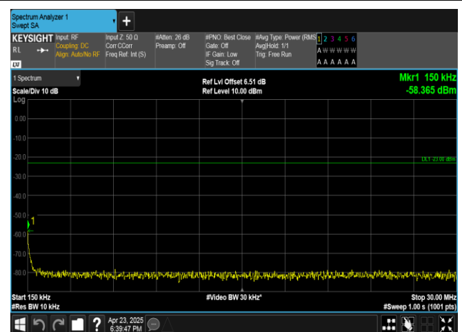
Band13-5MHz-QPSK-23230-1RB#24-0.15~30-PASS
