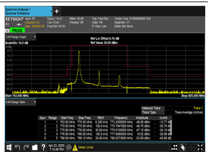
Band13-10MHz-16QAM-23230-1RB#0-PASS
