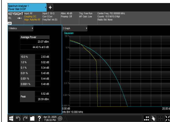
Band13-10MHz-16QAM-23230-1RB#0-PASS
