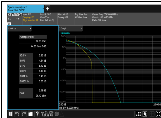
Band13-5MHz-16QAM-23205-1RB#0-PASS
