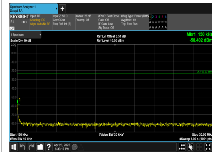
Band13-5MHz-QPSK-23205-1RB#24-0.15~30-PASS
