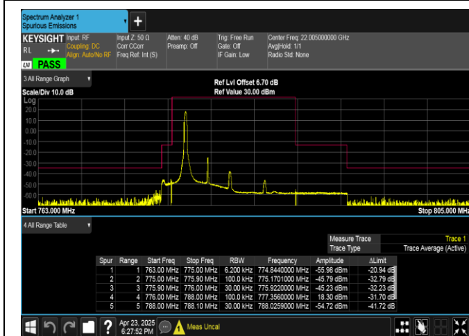
Band13-5MHz-16QAM-23205-1RB#0-PASS
