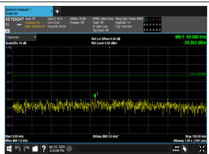
Band13-5MHz-QPSK-23205-1RB#24-0.009~0.15-PASS
