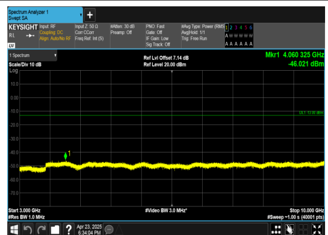
Band13-5MHz-QPSK-23205-1RB#24-3000~10000-PASS
