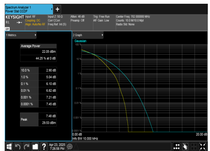
Band13-10MHz-16QAM-23230-50RB#0-PASS
