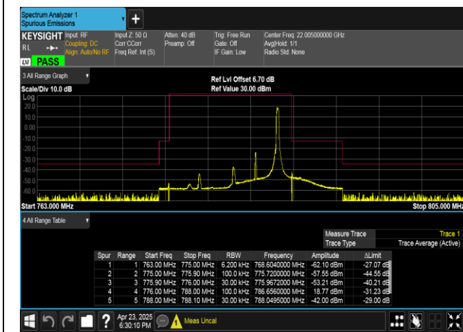
Band13-5MHz-16QAM-23255-1RB#24-PASS
