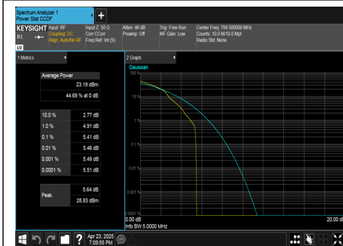
Band13-5MHz-16QAM-23255-1RB#0-PASS
