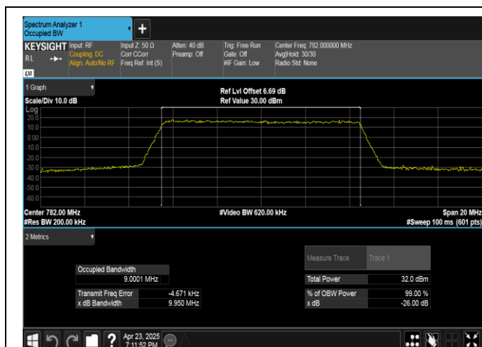
Band13-10MHz-QPSK-23230-50RB#0-PASS
