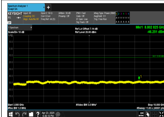
Band13-5MHz-QPSK-23205-25RB#0-3000~10000-PASS
