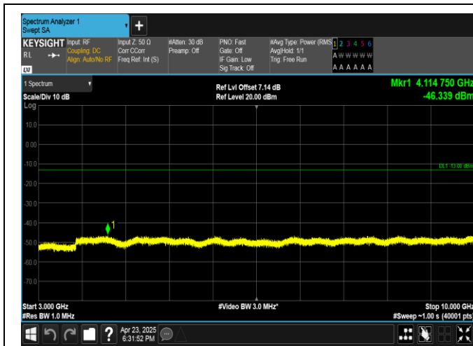
Band13-5MHz-QPSK-23205-1RB#0-3000~10000-PASS
