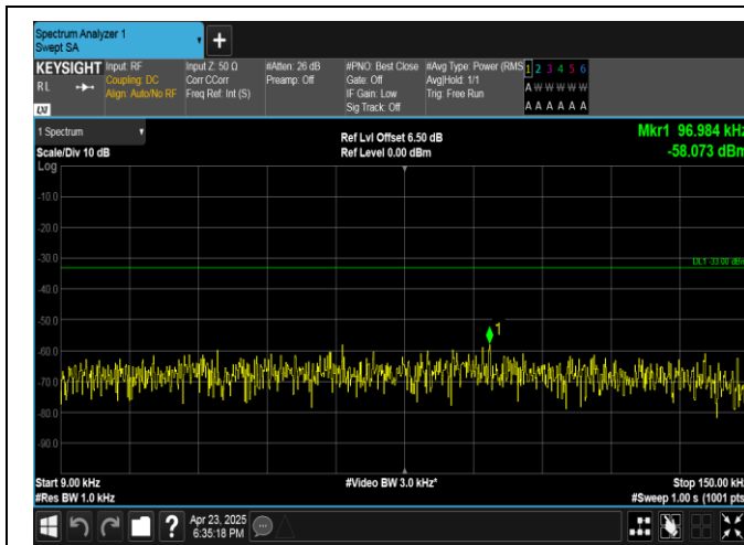
Band13-5MHz-QPSK-23205-25RB#0-0.009~0.15-PASS
