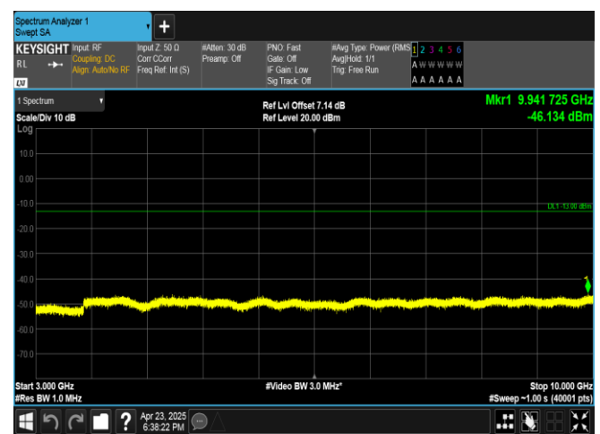
Band13-5MHz-QPSK-23230-1RB#0-3000~10000-PASS
