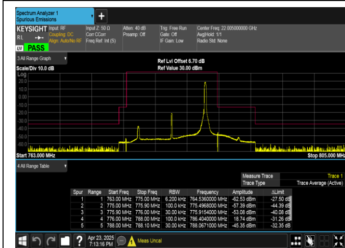
Band13-10MHz-16QAM-23230-1RB#49-PASS
