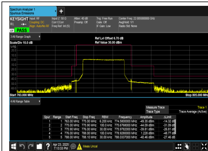
Band13-10MHz-QPSK-23230-50RB#0-PASS
