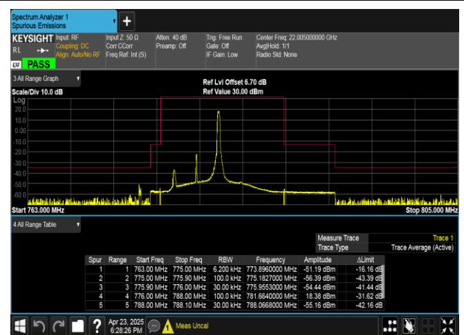
Band13-5MHz-16QAM-23205-1RB#24-PASS
