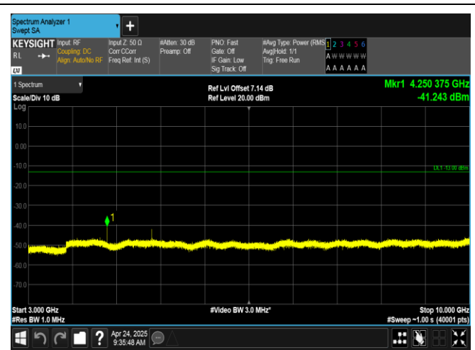
Band12-10MHz-QPSK-23060-1RB#49-3000~10000-PASS
