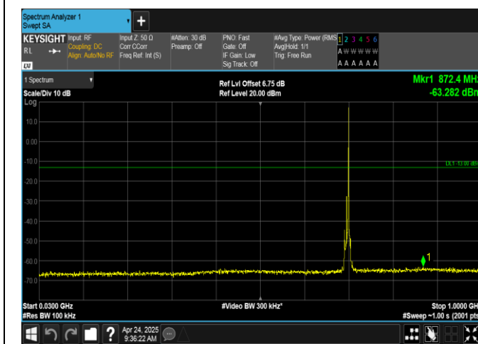
Band12-10MHz-16QAM-23060-1RB#49-30~1000-PASS
