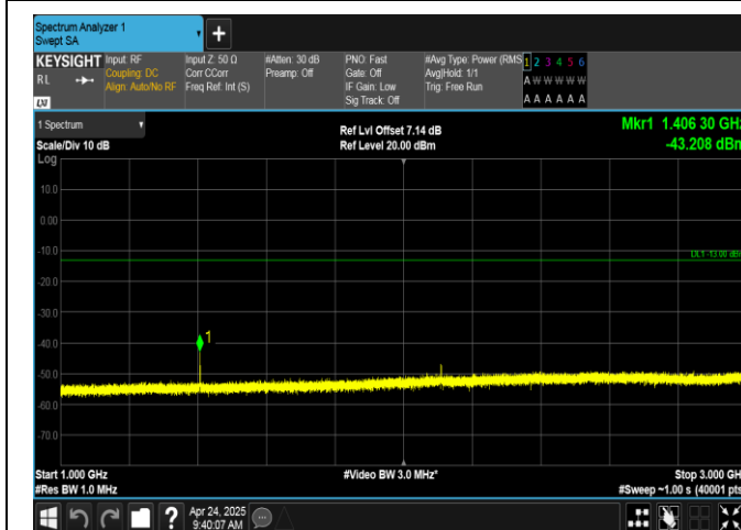
Band12-10MHz-QPSK-23095-1RB#0-1000~3000-PASS
