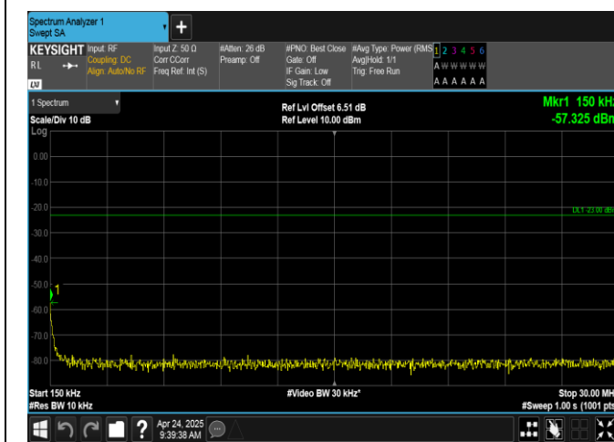
Band12-10MHz-QPSK-23095-1RB#0-0.15~30-PASS
