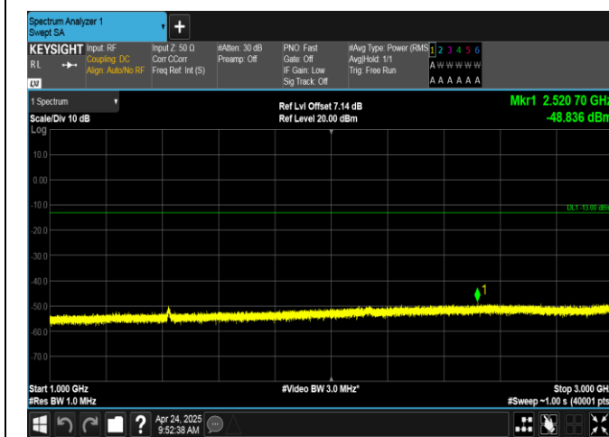
Band12-10MHz-16QAM-23130-50RB#0-1000~3000-PASS
