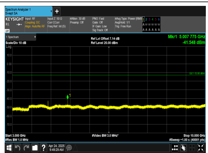
Band12-10MHz-QPSK-23130-1RB#49-3000~10000-PASS
