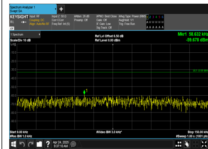
Band12-10MHz-QPSK-23060-50RB#0-0.009~0.15-PASS
