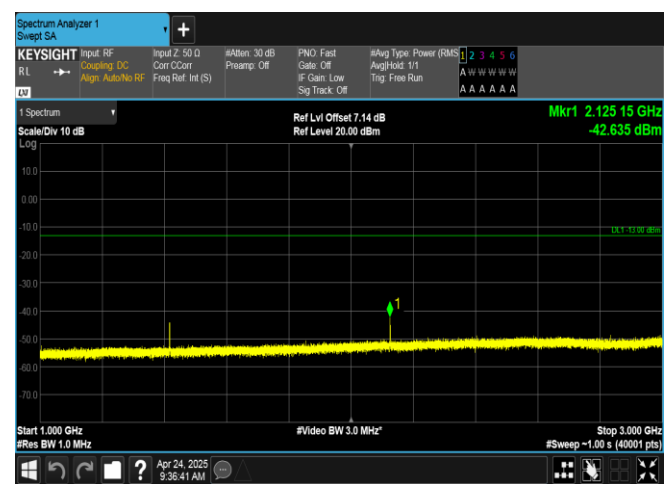
Band12-10MHz-16QAM-23060-1RB#49-1000~3000-PASS
