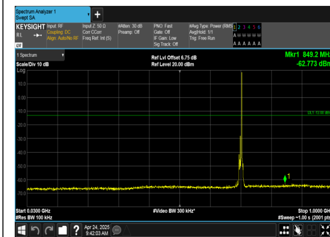
Band12-10MHz-QPSK-23095-1RB#49-30~1000-PASS
