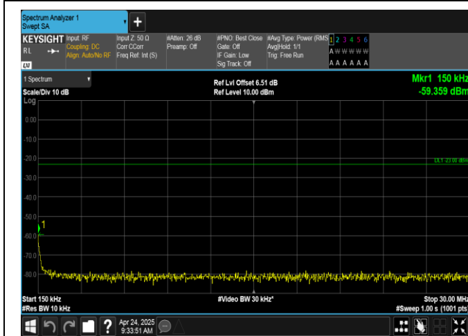
Band12-10MHz-16QAM-23060-1RB#0-0.15~30-PASS
