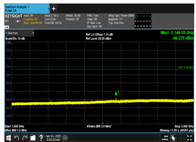
Band12-10MHz-16QAM-23130-1RB#49-1000~3000-PASS
