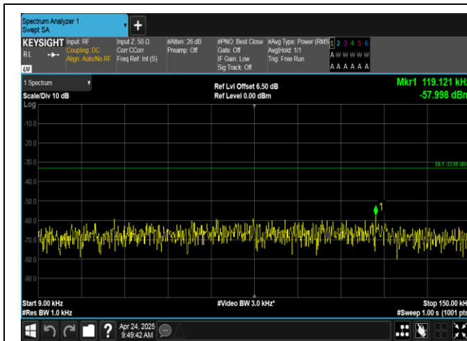
Band12-10MHz-16QAM-23130-1RB#49-0.009~0.15-PASS
