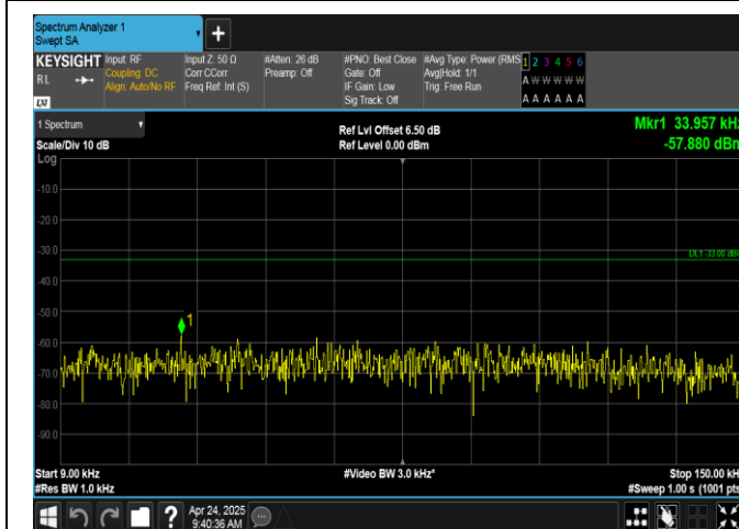
Band12-10MHz-16QAM-23095-1RB#0-0.009~0.15-PASS
