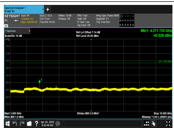
Band12-10MHz-16QAM-23095-1RB#49-3000~10000-PASS
