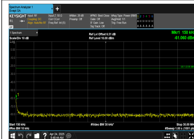
Band12-10MHz-QPSK-23130-1RB#49-0.15~30-PASS
