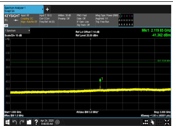
Band12-10MHz-QPSK-23130-1RB#0-1000~3000-PASS
