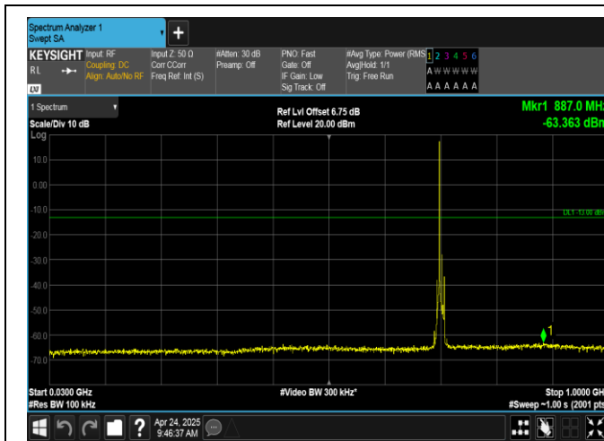
Band12-10MHz-QPSK-23130-1RB#0-30~1000-PASS
