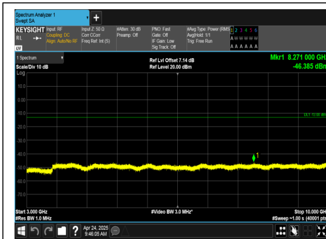
Band12-10MHz-16QAM-23095-50RB#0-3000~10000-PASS
