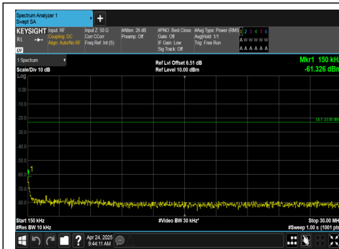
Band12-10MHz-QPSK-23095-50RB#0-0.15~30-PASS
