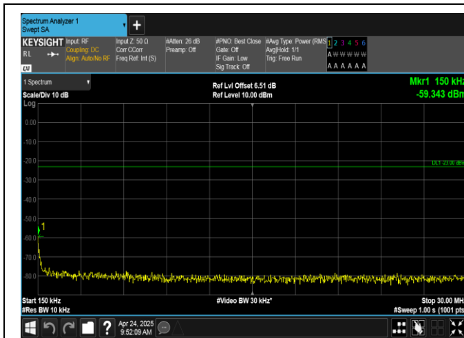
Band12-10MHz-16QAM-23130-50RB#0-0.15~30-PASS
