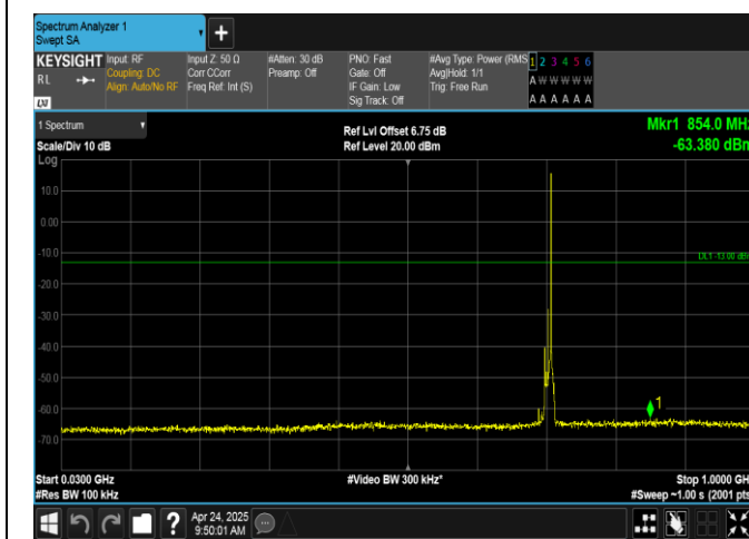
Band12-10MHz-16QAM-23130-1RB#49-30~1000-PASS
