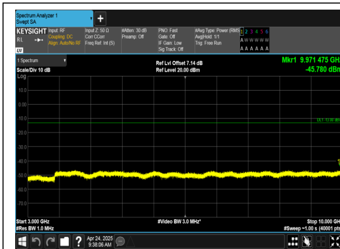
Band12-10MHz-QPSK-23060-50RB#0-3000~10000-PASS
