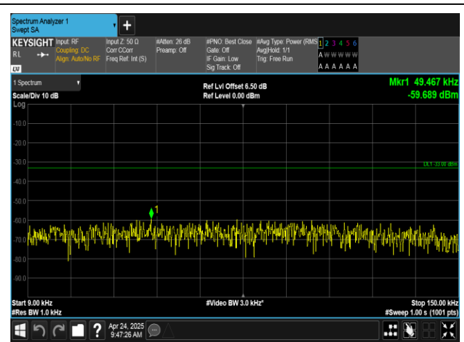
Band12-10MHz-16QAM-23130-1RB#0-0.009~0.15-PASS
