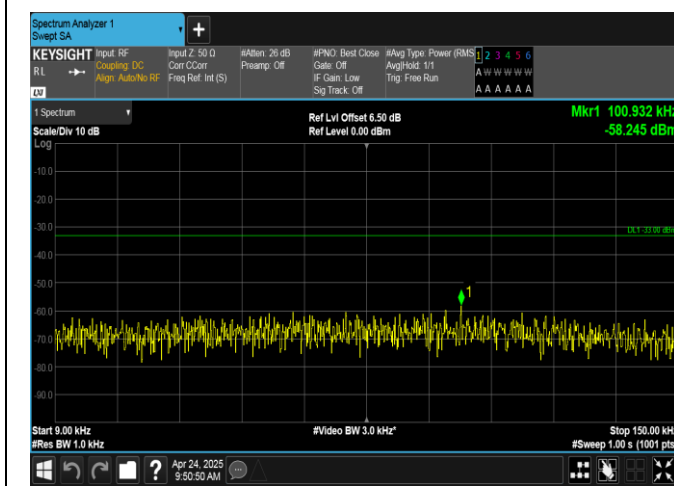
Band12-10MHz-QPSK-23130-50RB#0-0.009~0.15-PASS
