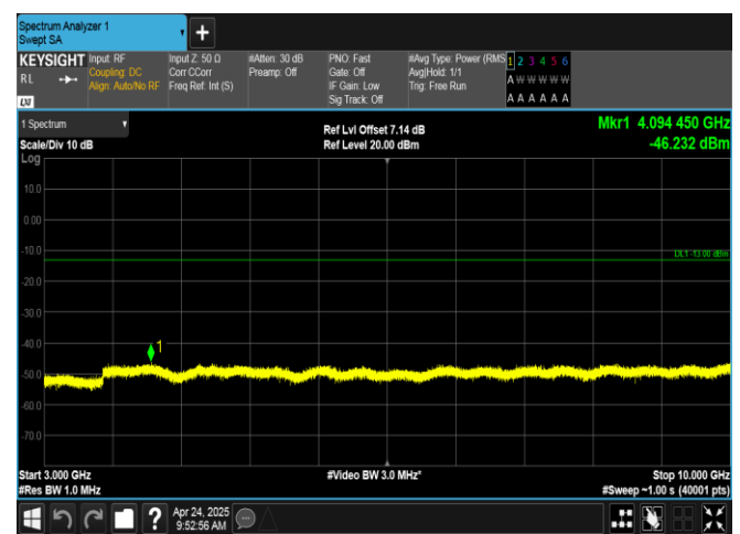
Band12-10MHz-16QAM-23130-50RB#0-3000~10000-PASS
