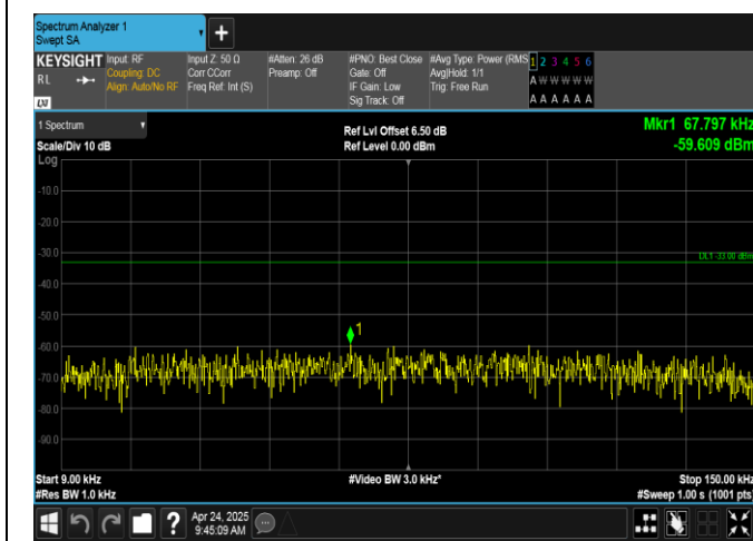
Band12-10MHz-16QAM-23095-50RB#0-0.009~0.15-PASS
