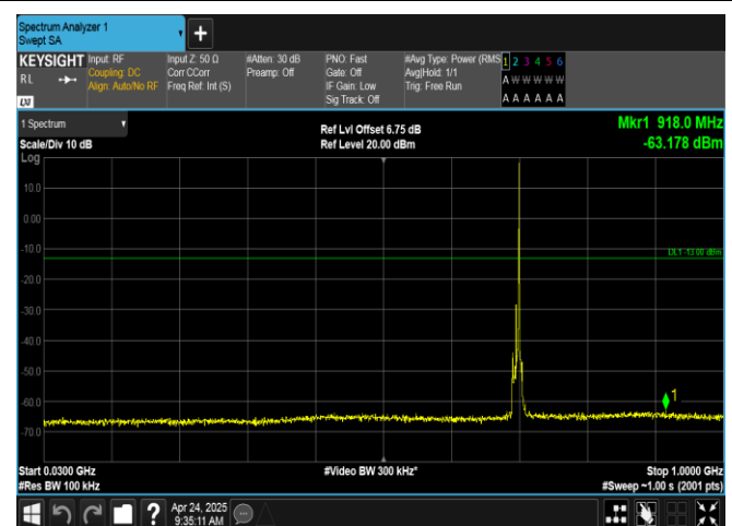
Band12-10MHz-QPSK-23060-1RB#49-30~1000-PASS
