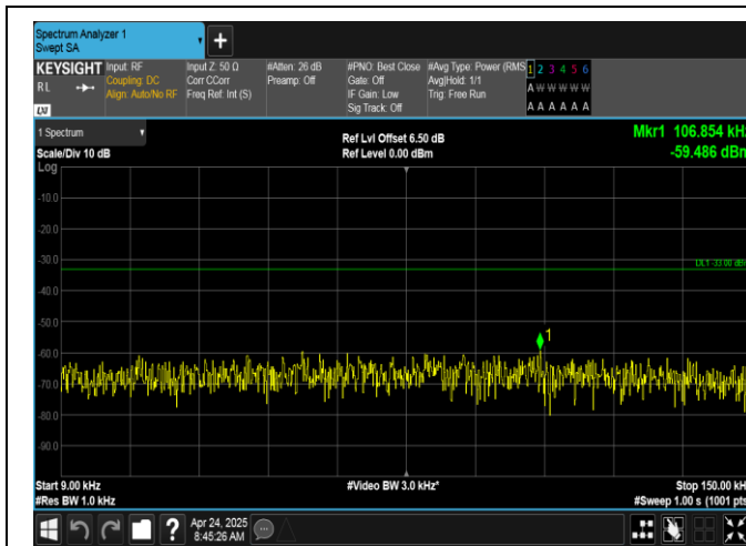
Band12-5MHz-16QAM-23035-1RB#24-0.009~0.15-PASS
