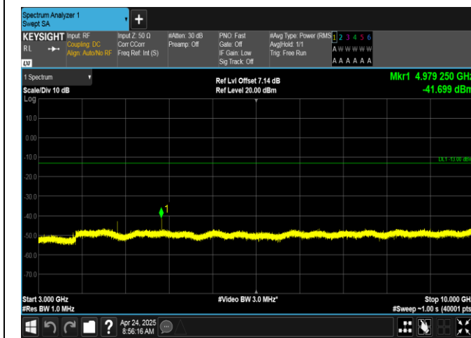
Band12-5MHz-QPSK-23155-1RB#0-3000~10000-PASS
