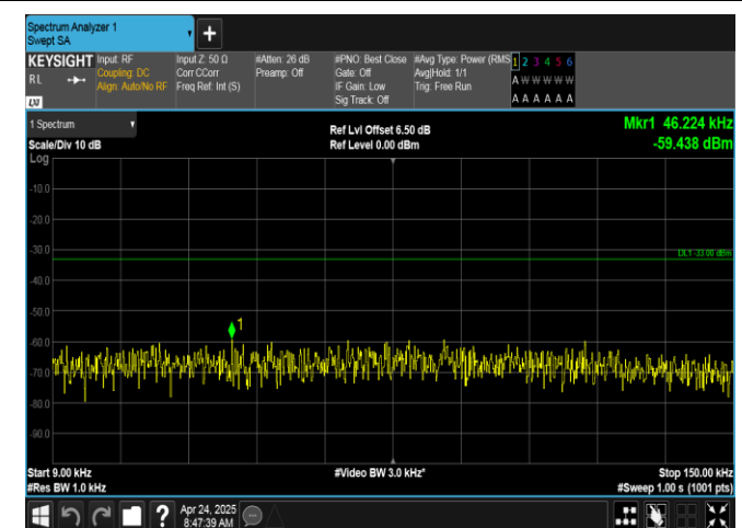
Band12-5MHz-16QAM-23035-25RB#0-0.009~0.15-PASS
