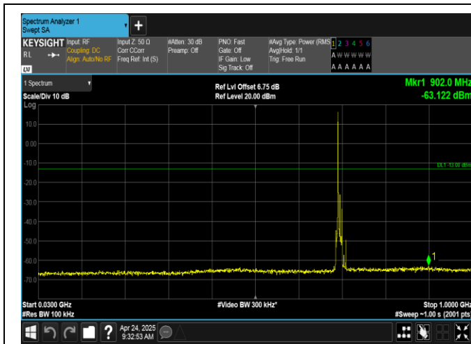
Band12-10MHz-QPSK-23060-1RB#0-30~1000-PASS
