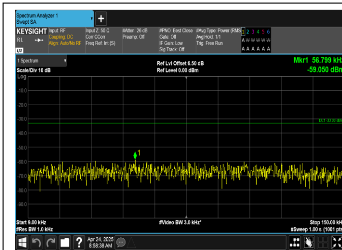
Band12-5MHz-16QAM-23155-1RB#24-0.009~0.15-PASS
