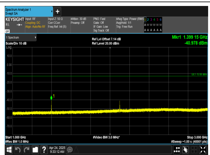
Band12-10MHz-QPSK-23060-1RB#0-1000~3000-PASS
