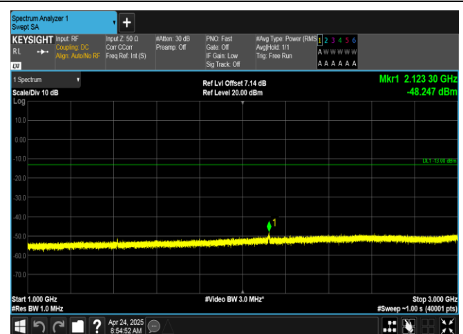
Band12-5MHz-16QAM-23095-25RB#0-1000~3000-PASS
