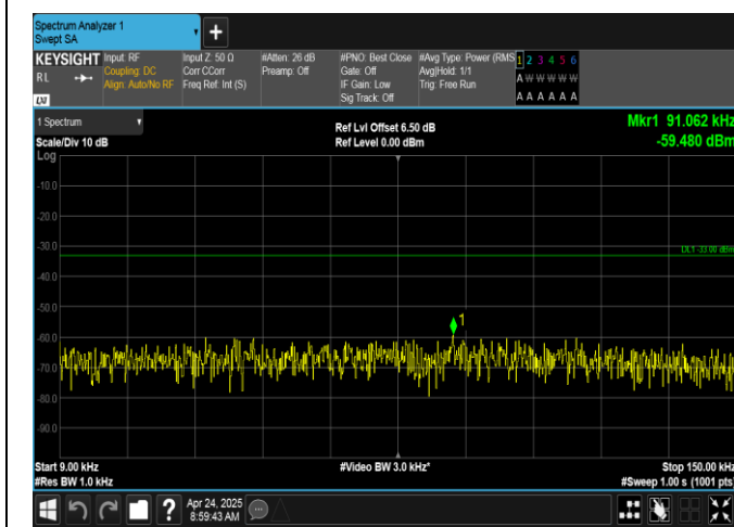
Band12-5MHz-QPSK-23155-25RB#0-0.009~0.15-PASS
