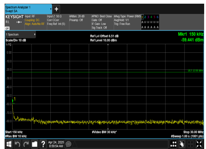
Band12-5MHz-QPSK-23155-25RB#0-0.15~30-PASS
