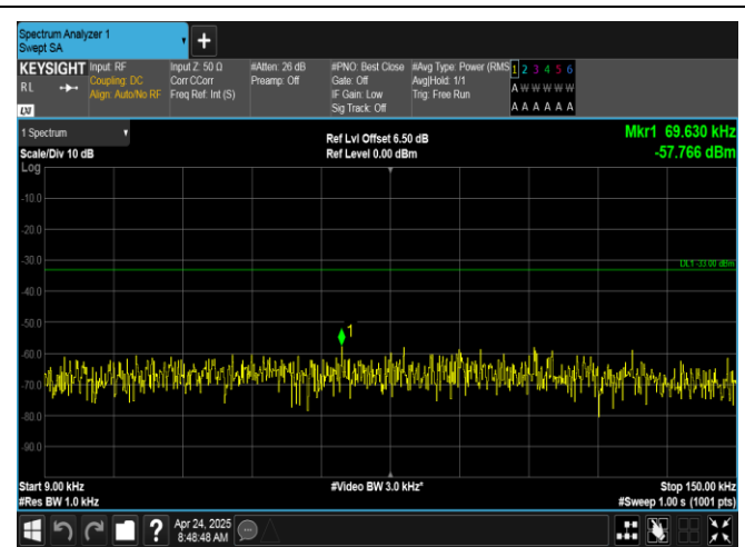
Band12-5MHz-QPSK-23095-1RB#0-0.009~0.15-PASS
