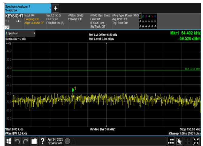
Band12-10MHz-QPSK-23060-1RB#49-0.009~0.15-PASS
