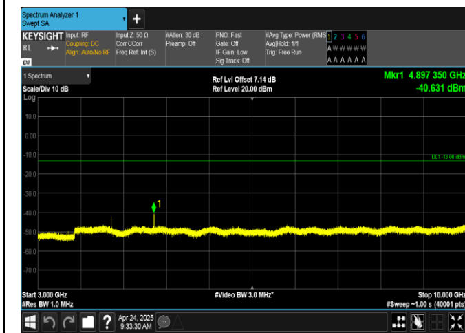
Band12-10MHz-QPSK-23060-1RB#0-3000~10000-PASS
