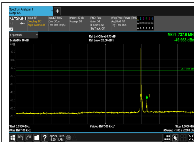
Band12-5MHz-16QAM-23095-1RB#0-30~1000-PASS
