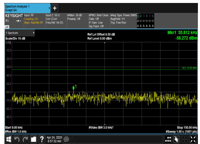
Band12-5MHz-QPSK-23155-1RB#24-0.009~0.15-PASS
