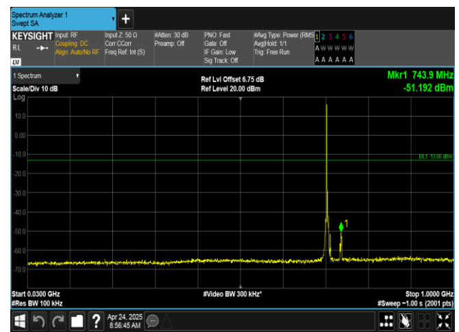
Band12-5MHz-16QAM-23155-1RB#0-30~1000-PASS
