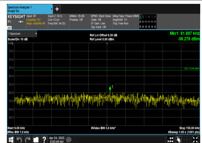
Band12-5MHz-16QAM-23155-25RB#0-0.009~0.15-PASS
