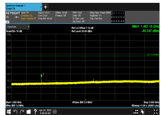
Band12-5MHz-16QAM-23035-1RB#24-1000~3000-PASS
