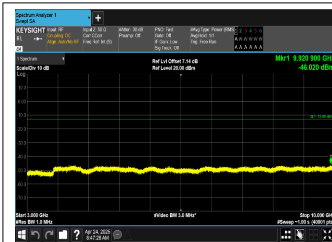
Band12-5MHz-QPSK-23035-25RB#0-3000~10000-PASS
