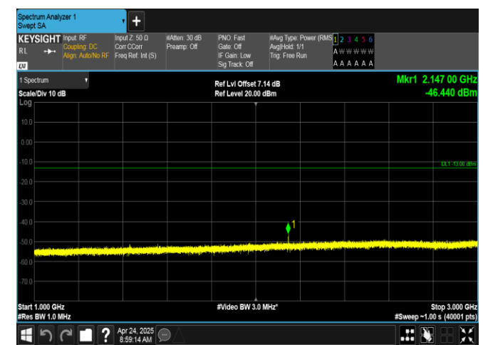
Band12-5MHz-16QAM-23155-1RB#24-1000~3000-PASS
