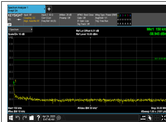
Band12-5MHz-16QAM-23035-25RB#0-0.15~30-PASS
