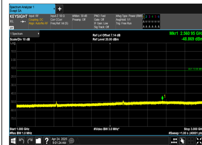
Band12-5MHz-16QAM-23155-25RB#0-1000~3000-PASS
