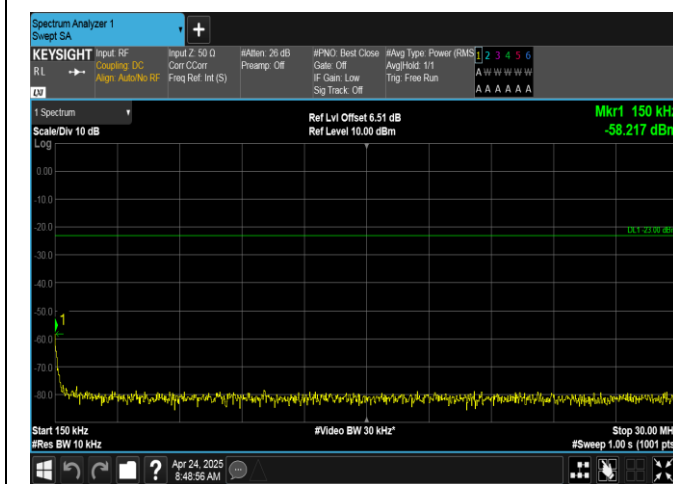
Band12-5MHz-QPSK-23095-1RB#0-0.15~30-PASS
