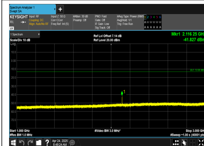
Band12-5MHz-QPSK-23095-1RB#0-1000~3000-PASS
