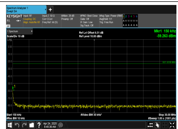
Band12-5MHz-16QAM-23035-1RB#24-0.15~30-PASS
