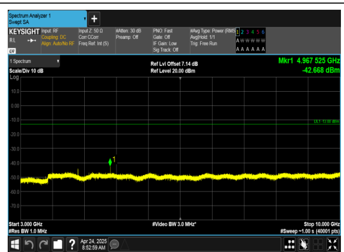
Band12-5MHz-16QAM-23095-1RB#24-3000~10000-PASS
