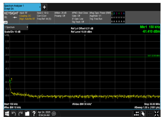
Band12-5MHz-16QAM-23095-25RB#0-0.15~30-PASS
