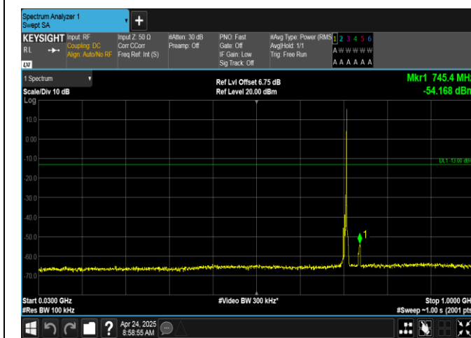
Band12-5MHz-16QAM-23155-1RB#24-30~1000-PASS
