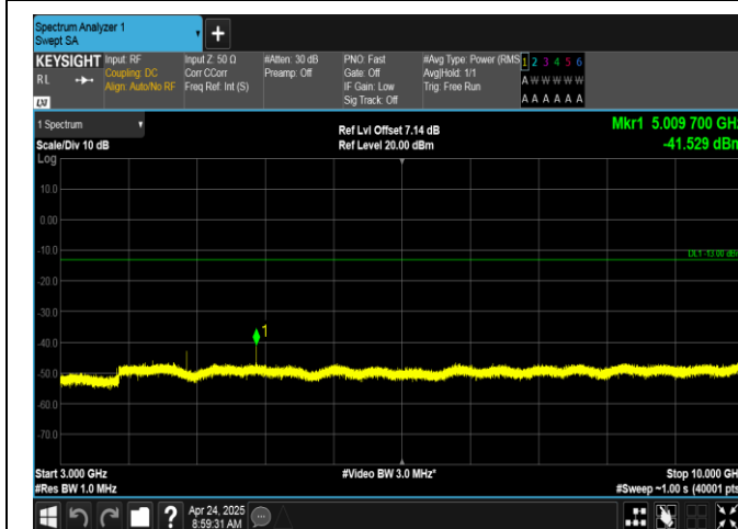
Band12-5MHz-16QAM-23155-1RB#24-3000~10000-PASS
