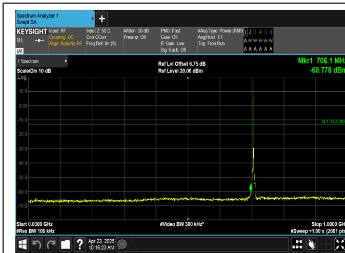
Band12-3MHz-QPSK-23165-1RB#0-30~1000-PASS
