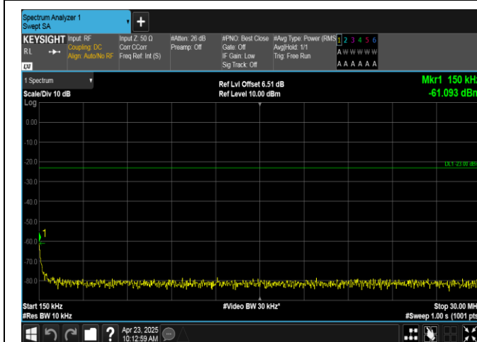
Band12-3MHz-16QAM-23095-1RB#14-0.15~30-PASS
