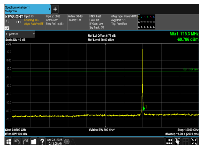
Band12-3MHz-16QAM-23095-1RB#14-30~1000-PASS
