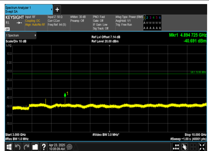
Band12-3MHz-16QAM-23025-1RB#0-3000~10000-PASS
