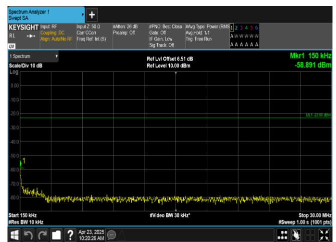
Band12-3MHz-QPSK-23165-15RB#0-0.15~30-PASS
