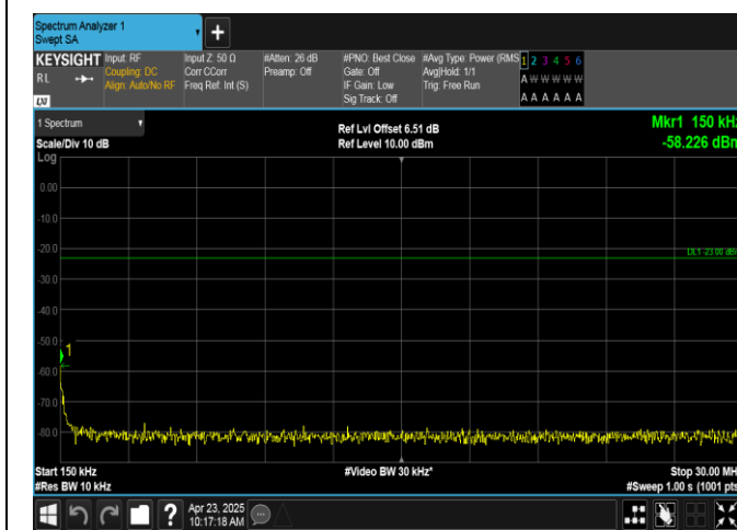
Band12-3MHz-16QAM-23165-1RB#0-0.15~30-PASS
