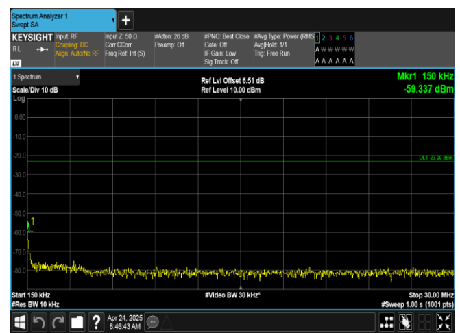
Band12-5MHz-QPSK-23035-25RB#0-0.15~30-PASS
