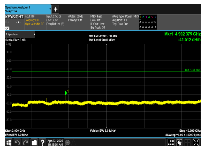
Band12-3MHz-16QAM-23165-1RB#0-3000~10000-PASS
