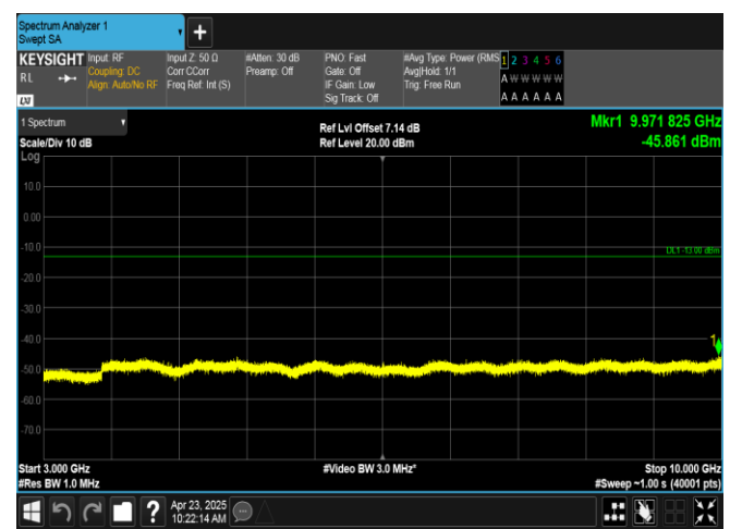
Band12-3MHz-16QAM-23165-15RB#0-3000~10000-PASS
