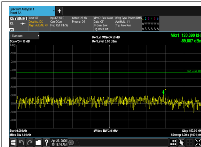
Band12-3MHz-16QAM-23165-1RB#14-0.009~0.15-PASS
