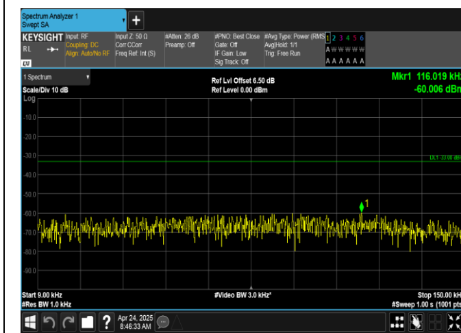
Band12-5MHz-QPSK-23035-25RB#0-0.009~0.15-PASS
