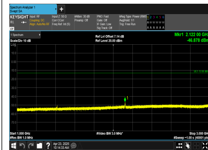
Band12-3MHz-QPSK-23095-15RB#0-1000~3000-PASS
