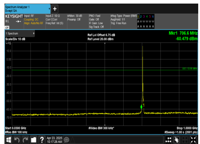
Band12-3MHz-16QAM-23165-1RB#0-30~1000-PASS
