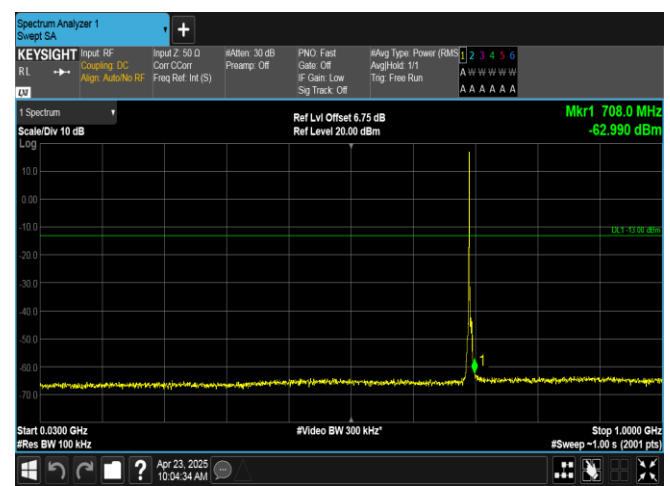
Band12-3MHz-16QAM-23025-1RB#0-30~1000-PASS
