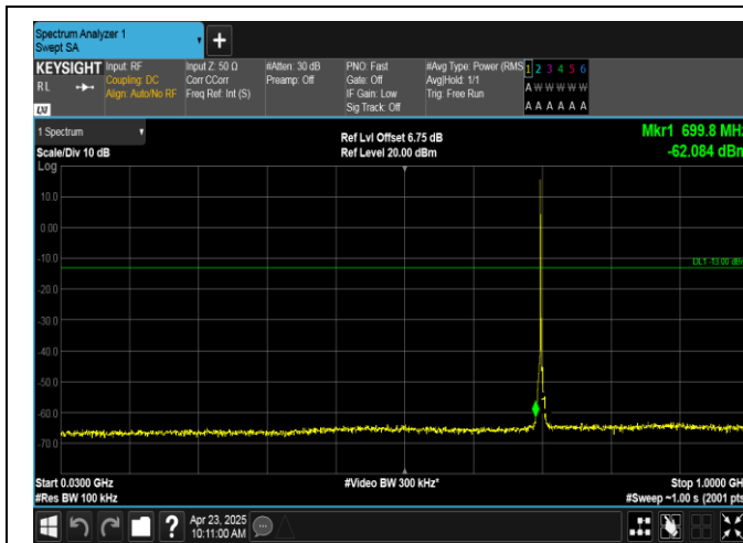
Band12-3MHz-16QAM-23095-1RB#0-30~1000-PASS
