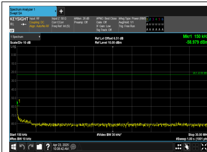
Band12-3MHz-16QAM-23025-15RB#0-0.15~30-PASS
