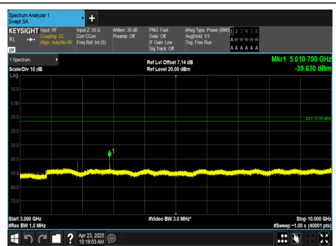
Band12-3MHz-QPSK-23165-1RB#14-3000~10000-PASS
