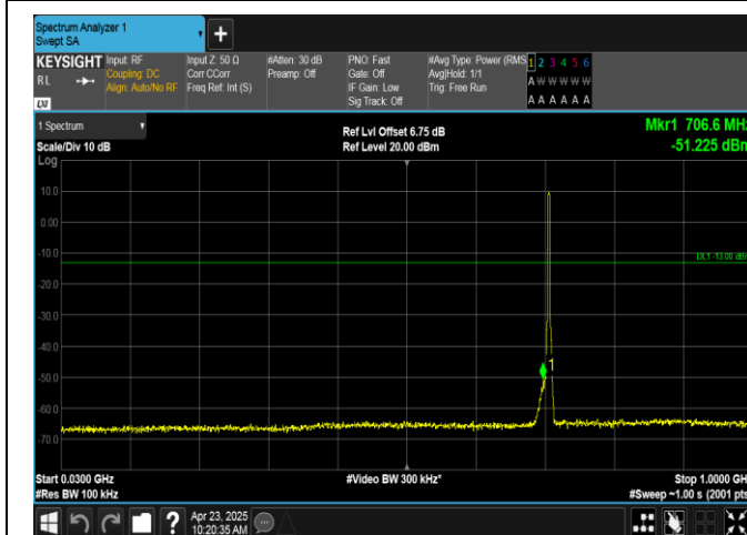
Band12-3MHz-QPSK-23165-15RB#0-30~1000-PASS
