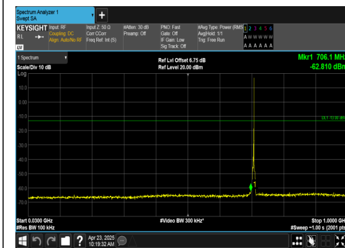
Band12-3MHz-16QAM-23165-1RB#14-30~1000-PASS
