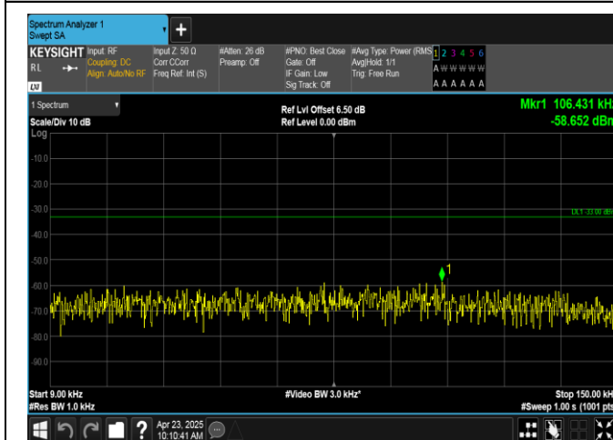
Band12-3MHz-16QAM-23095-1RB#0-0.009~0.15-PASS
