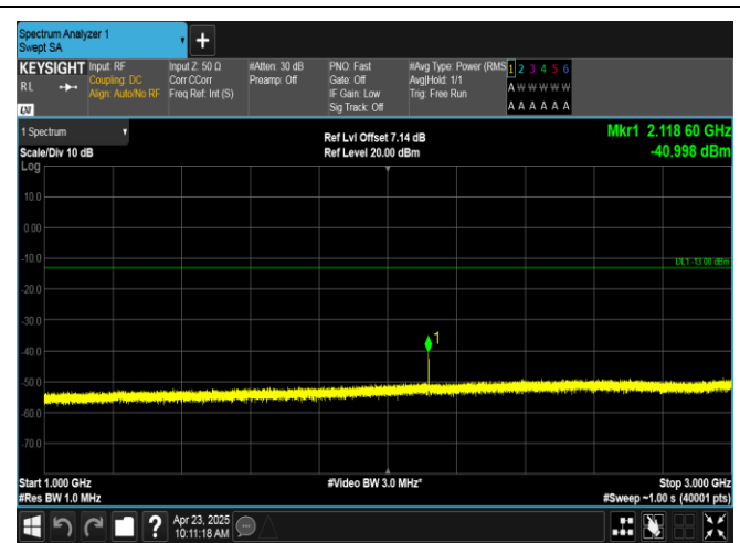
Band12-3MHz-16QAM-23095-1RB#0-1000~3000-PASS
