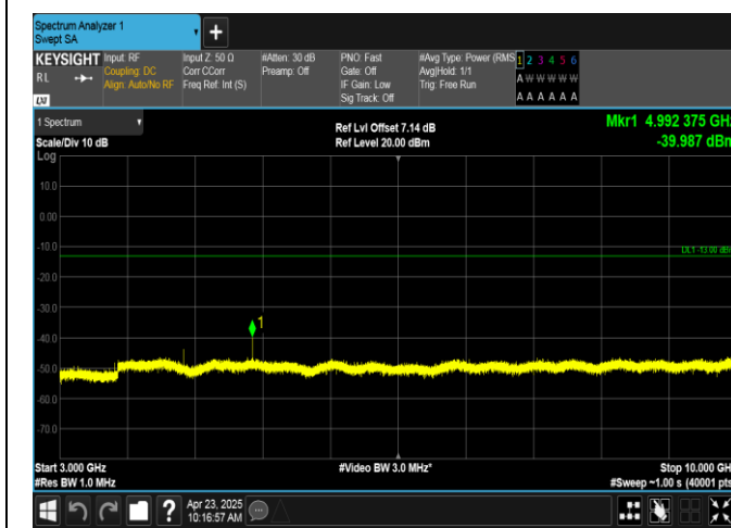
Band12-3MHz-QPSK-23165-1RB#0-3000~10000-PASS
