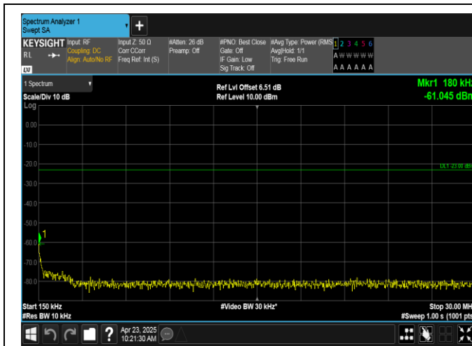
Band12-3MHz-16QAM-23165-15RB#0-0.15~30-PASS
