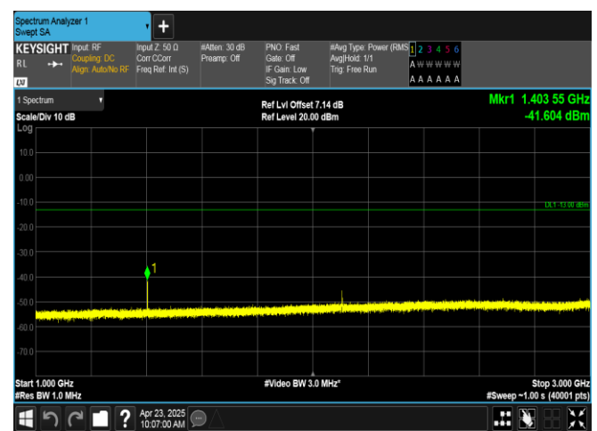
Band12-3MHz-16QAM-23025-1RB#14-1000~3000-PASS
