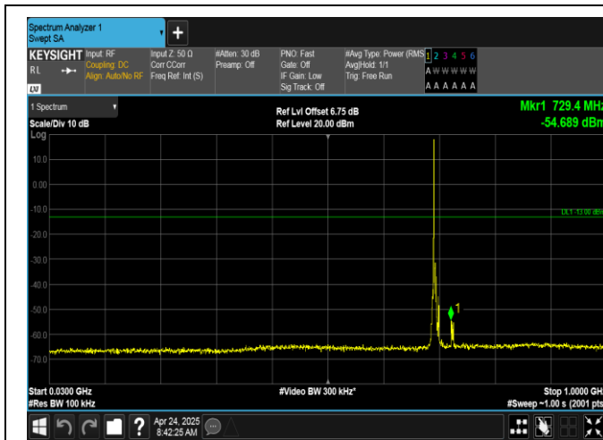
Band12-5MHz-QPSK-23035-1RB#0-30~1000-PASS
