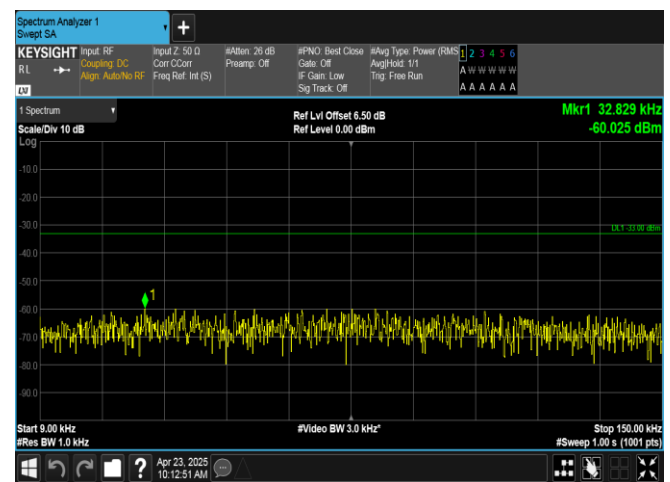
Band12-3MHz-16QAM-23095-1RB#14-0.009~0.15-PASS
