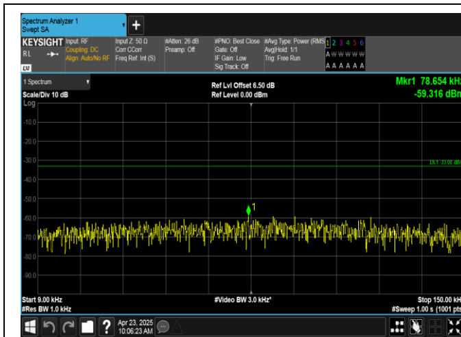
Band12-3MHz-16QAM-23025-1RB#14-0.009~0.15-PASS
