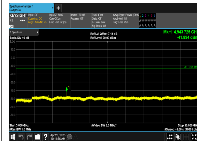
Band12-3MHz-16QAM-23095-1RB#0-3000~10000-PASS
