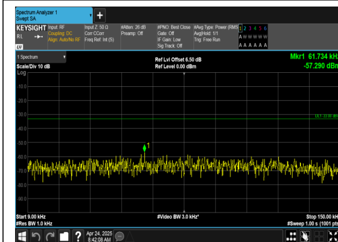
Band12-5MHz-QPSK-23035-1RB#0-0.009~0.15-PASS
