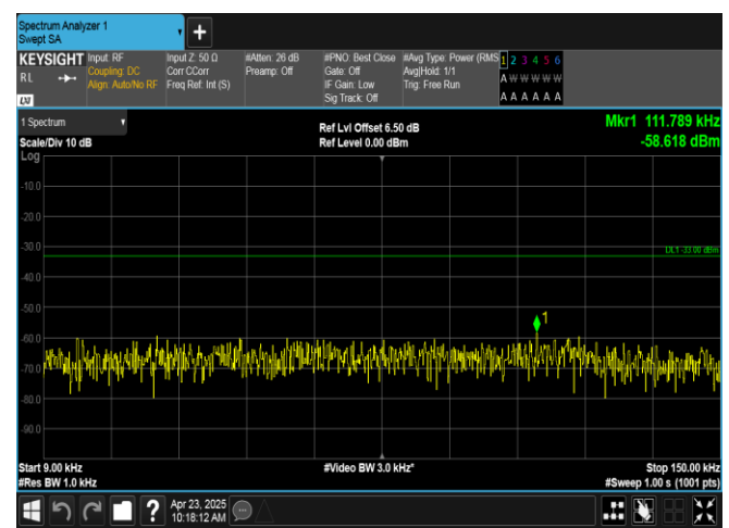
Band12-3MHz-QPSK-23165-1RB#14-0.009~0.15-PASS
