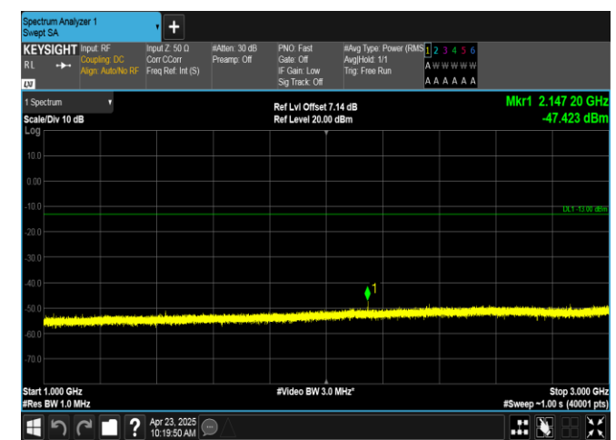
Band12-3MHz-16QAM-23165-1RB#14-1000~3000-PASS
