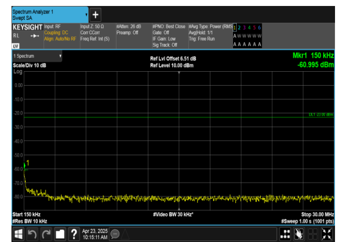
Band12-3MHz-16QAM-23095-15RB#0-0.15~30-PASS
