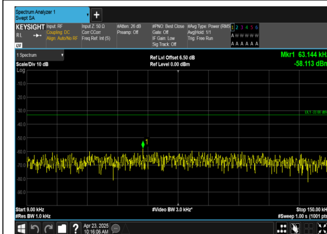
Band12-3MHz-QPSK-23165-1RB#0-0.009~0.15-PASS
