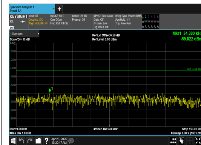
Band12-3MHz-QPSK-23165-15RB#0-0.009~0.15-PASS
