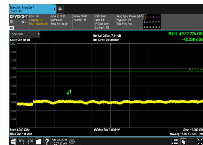
Band12-3MHz-16QAM-23025-1RB#14-3000~10000-PASS
