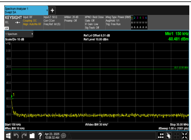
Band12-3MHz-16QAM-23025-1RB#14-0.15~30-PASS
