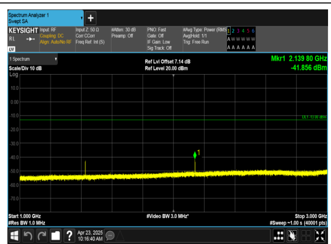
Band12-3MHz-QPSK-23165-1RB#0-1000~3000-PASS
