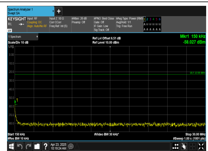
Band12-3MHz-16QAM-23165-1RB#14-0.15~30-PASS
