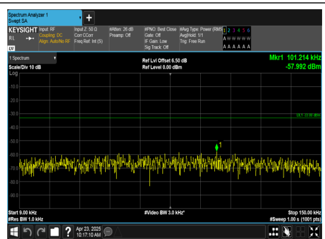
Band12-3MHz-16QAM-23165-1RB#0-0.009~0.15-PASS
