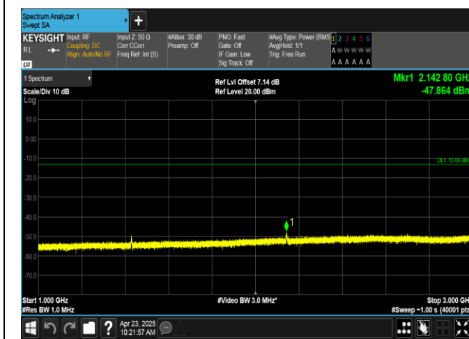
Band12-3MHz-16QAM-23165-15RB#0-1000~3000-PASS
