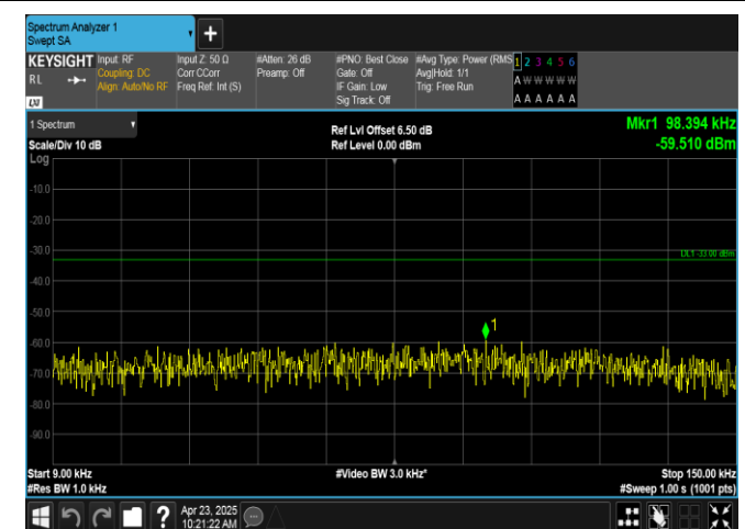
Band12-3MHz-16QAM-23165-15RB#0-0.009~0.15-PASS
