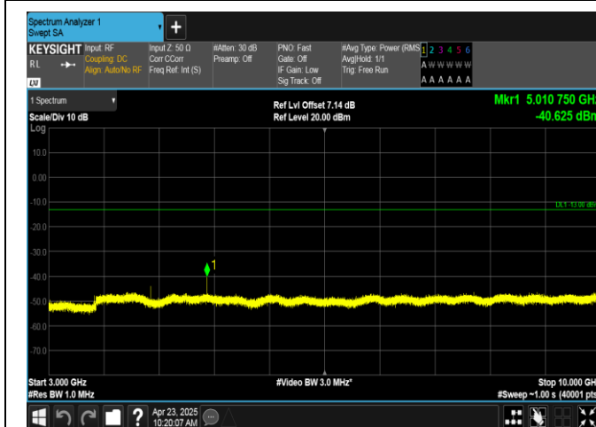
Band12-3MHz-16QAM-23165-1RB#14-3000~10000-PASS
