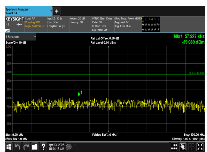
Band12-3MHz-16QAM-23025-1RB#0-0.009~0.15-PASS
