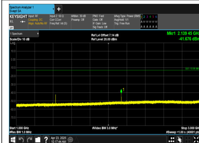
Band12-3MHz-16QAM-23165-1RB#0-1000~3000-PASS
