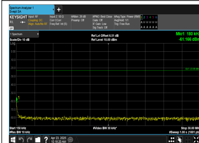
Band12-3MHz-QPSK-23165-1RB#14-0.15~30-PASS
