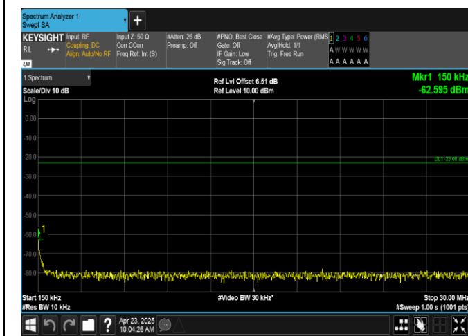
Band12-3MHz-16QAM-23025-1RB#0-0.15~30-PASS
