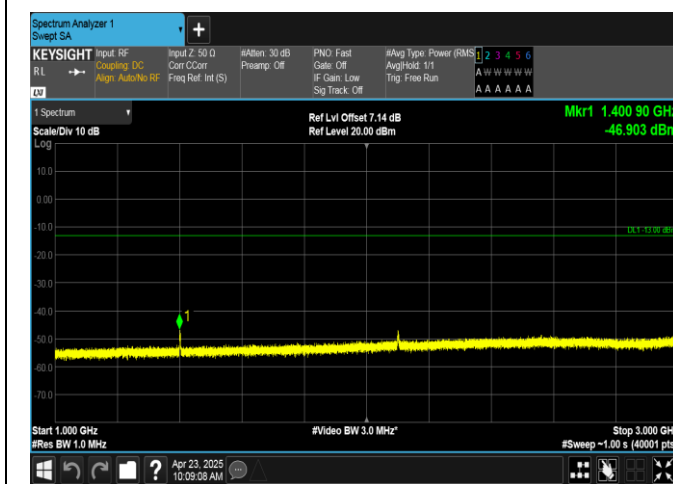
Band12-3MHz-16QAM-23025-15RB#0-1000~3000-PASS
