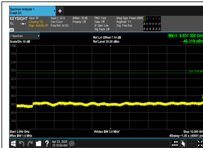
Band12-3MHz-16QAM-23095-15RB#0-3000~10000-PASS
