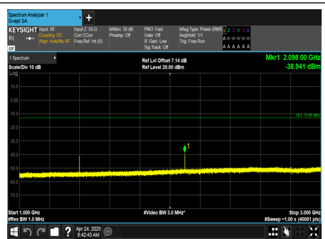
Band12-5MHz-QPSK-23035-1RB#0-1000~3000-PASS
