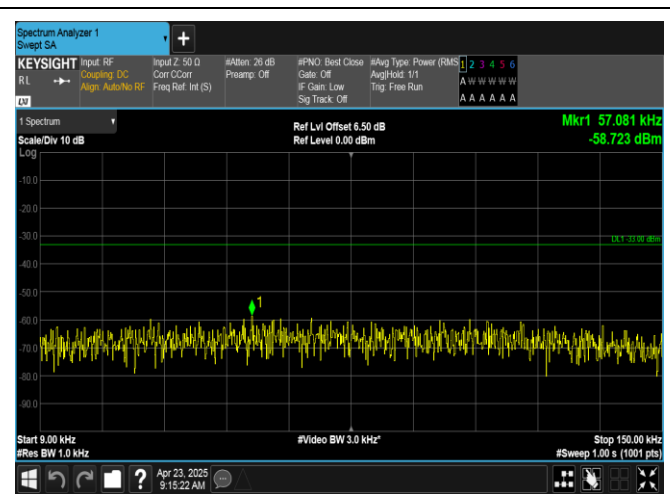
Band12-1.4MHz-16QAM-23017-1RB#0-0.009~0.15-PASS
