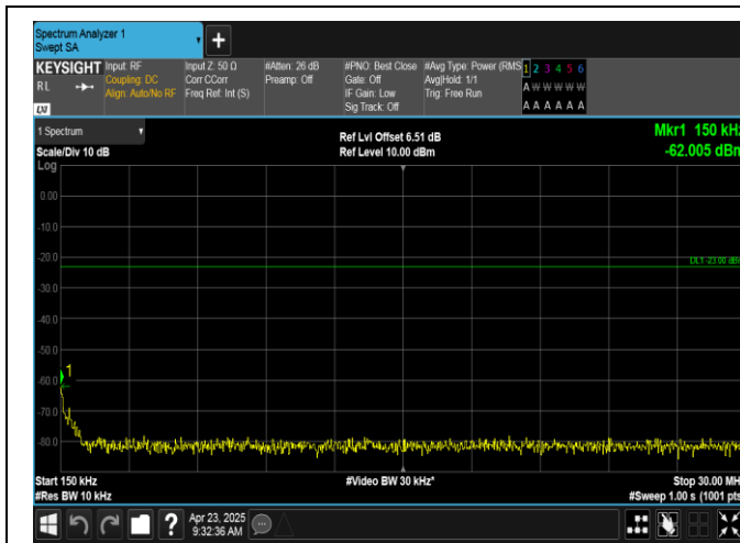
Band12-1.4MHz-16QAM-23173-6RB#0-0.15~30-PASS
