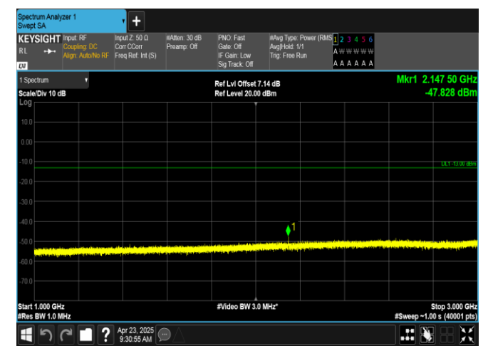
Band12-1.4MHz-16QAM-23173-1RB#5-1000~3000-PASS
