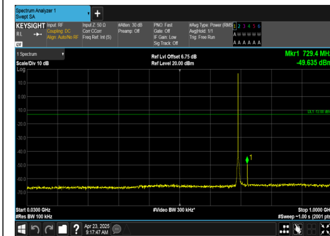
Band12-1.4MHz-16QAM-23017-1RB#5-30~1000-PASS
