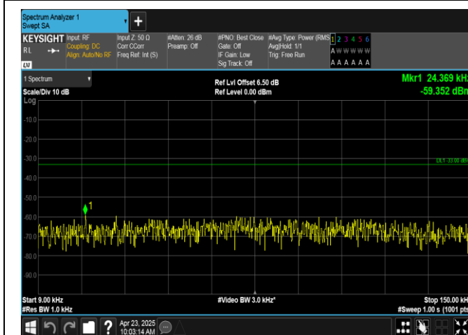
Band12-3MHz-QPSK-23025-1RB#0-0.009~0.15-PASS
