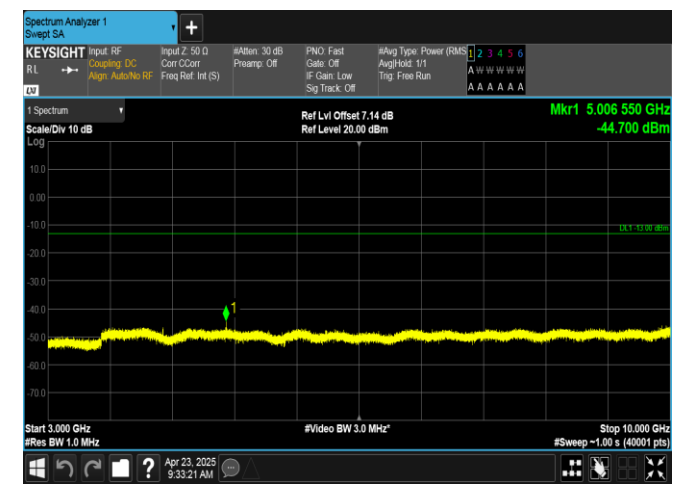
Band12-1.4MHz-16QAM-23173-6RB#0-3000~10000-PASS
