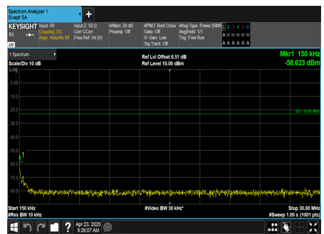
Band12-1.4MHz-16QAM-23095-6RB#0-0.15~30-PASS
