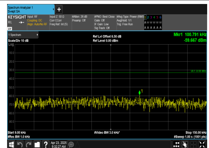
Band12-1.4MHz-16QAM-23173-6RB#0-0.009~0.15-PASS
