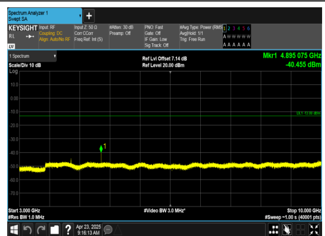
Band12-1.4MHz-16QAM-23017-1RB#0-3000~10000-PASS
