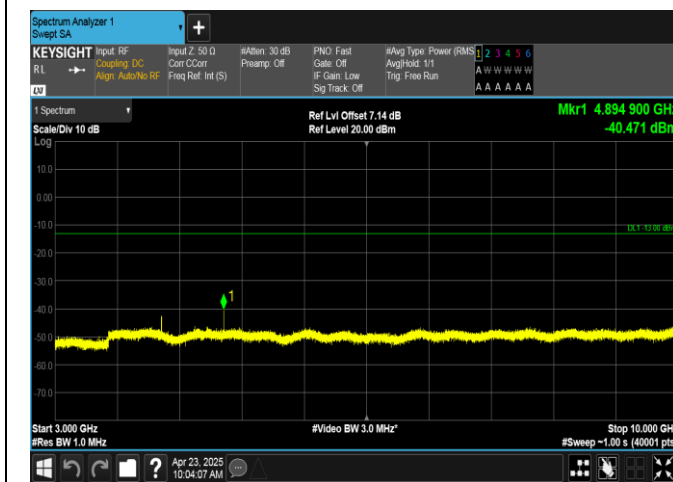
Band12-3MHz-QPSK-23025-1RB#0-3000~10000-PASS
