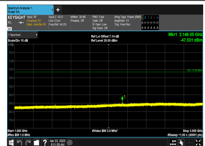
Band12-1.4MHz-QPSK-23173-6RB#0-1000~3000-PASS
