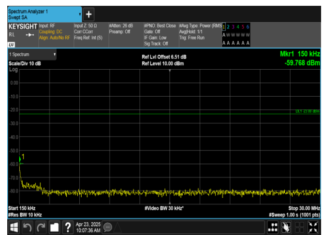
Band12-3MHz-QPSK-23025-15RB#0-0.15~30-PASS
