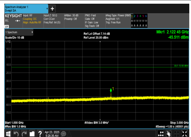
Band12-1.4MHz-16QAM-23095-6RB#0-1000~3000-PASS
