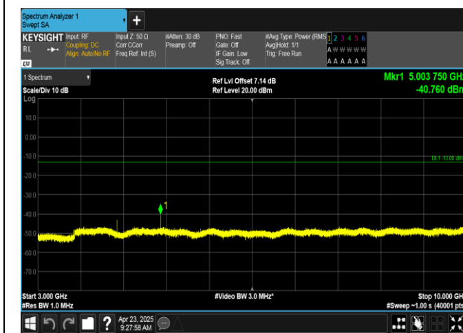
Band12-1.4MHz-QPSK-23173-1RB#0-3000~10000-PASS
