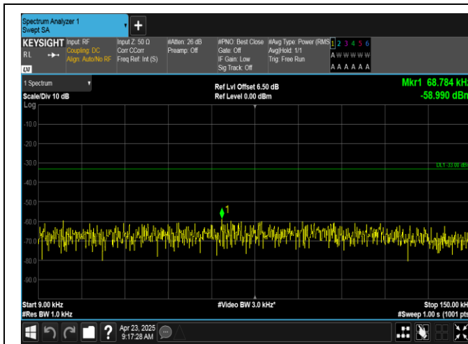
Band12-1.4MHz-16QAM-23017-1RB#5-0.009~0.15-PASS
