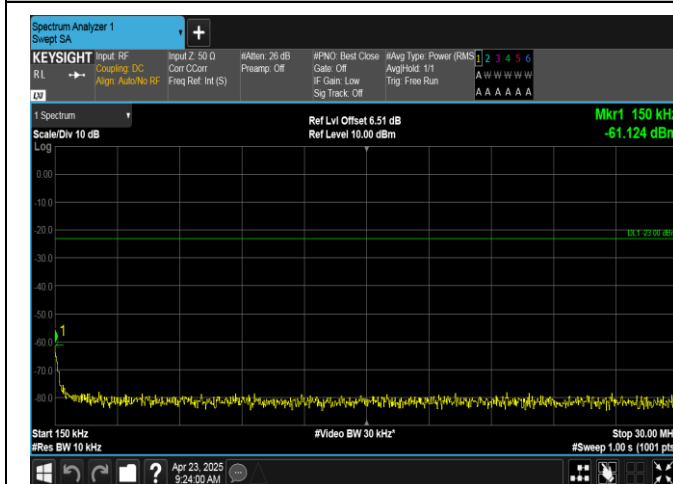
Band12-1.4MHz-16QAM-23095-1RB#5-0.15~30-PASS
