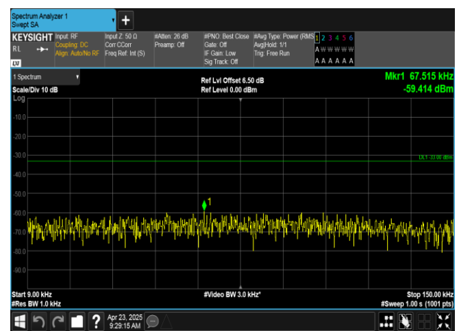
Band12-1.4MHz-QPSK-23173-1RB#5-0.009~0.15-PASS
