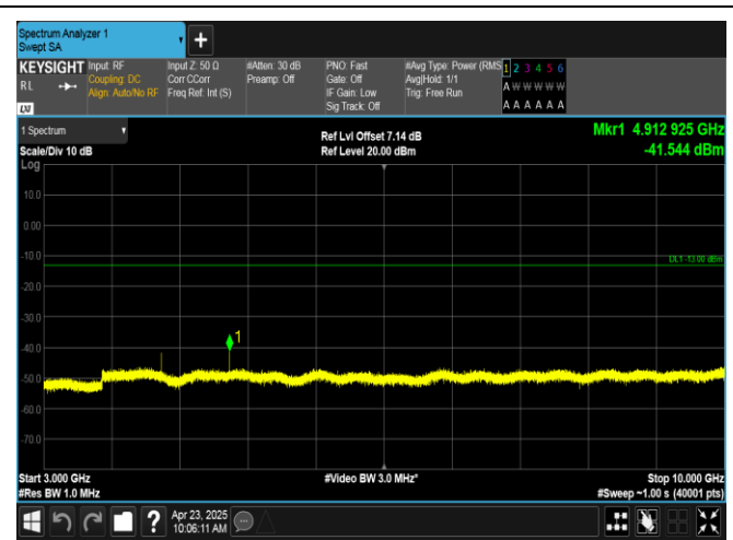
Band12-3MHz-QPSK-23025-1RB#14-3000~10000-PASS
