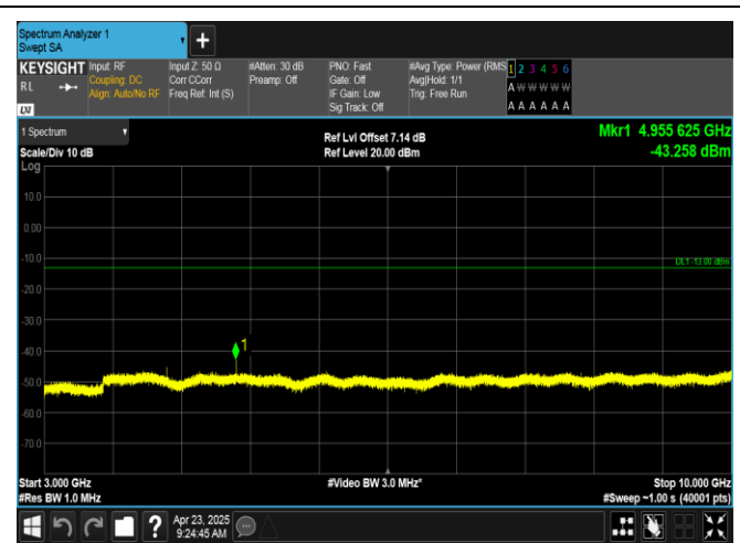
Band12-1.4MHz-16QAM-23095-1RB#5-3000~10000-PASS
