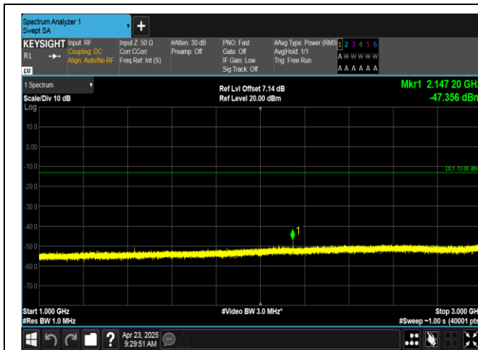
Band12-1.4MHz-QPSK-23173-1RB#5-1000~3000-PASS
