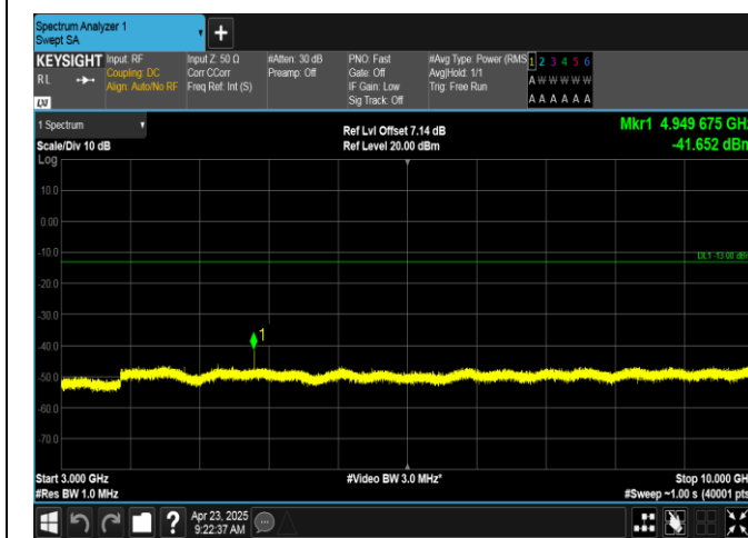
Band12-1.4MHz-16QAM-23095-1RB#0-3000~10000-PASS
