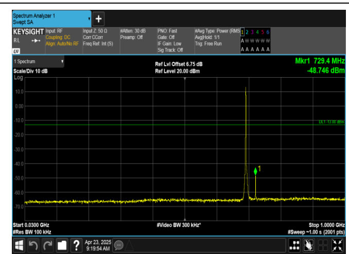
Band12-1.4MHz-16QAM-23017-6RB#0-30~1000-PASS
