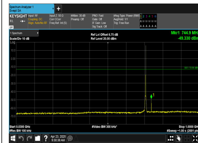
Band12-1.4MHz-16QAM-23173-1RB#5-30~1000-PASS
