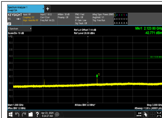
Band12-1.4MHz-16QAM-23095-1RB#5-1000~3000-PASS
