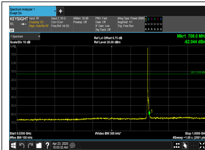
Band12-3MHz-QPSK-23025-1RB#0-30~1000-PASS
