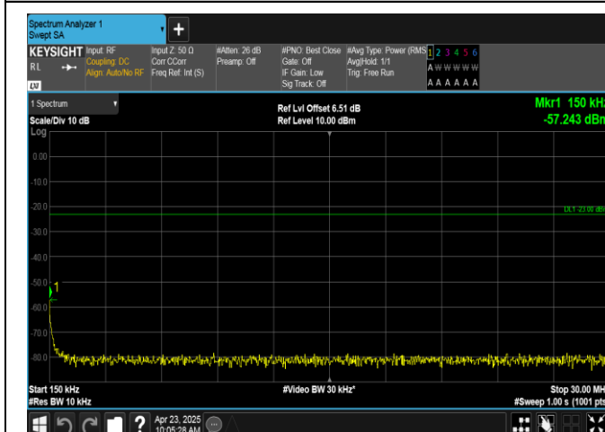
Band12-3MHz-QPSK-23025-1RB#14-0.15~30-PASS
