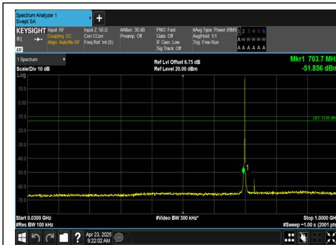
Band12-1.4MHz-16QAM-23095-1RB#0-30~1000-PASS
