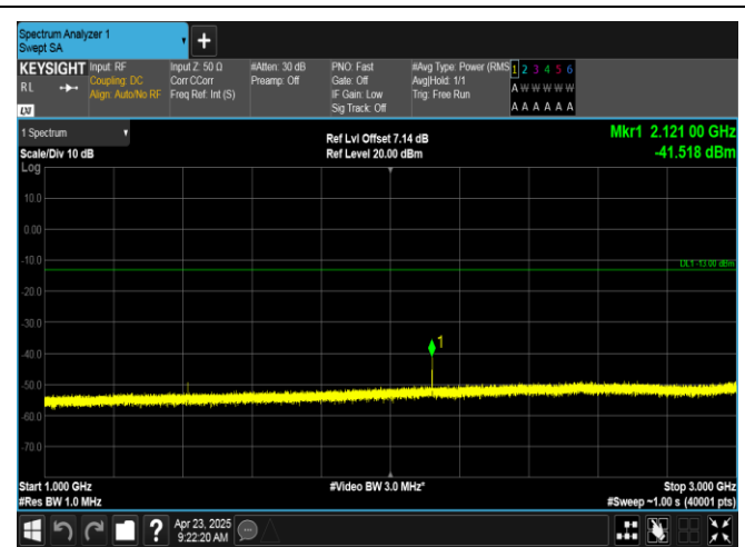
Band12-1.4MHz-16QAM-23095-1RB#0-1000~3000-PASS
