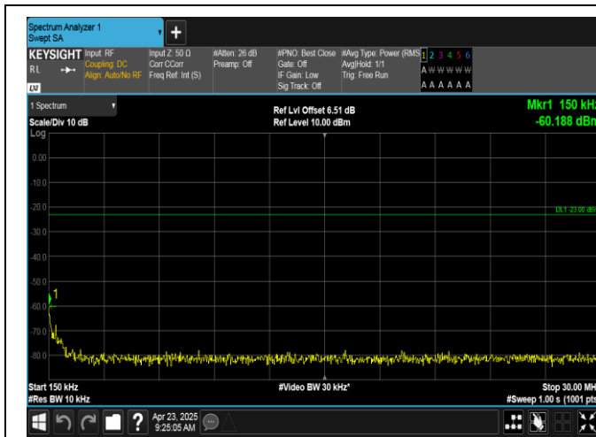
Band12-1.4MHz-QPSK-23095-6RB#0-0.15~30-PASS
