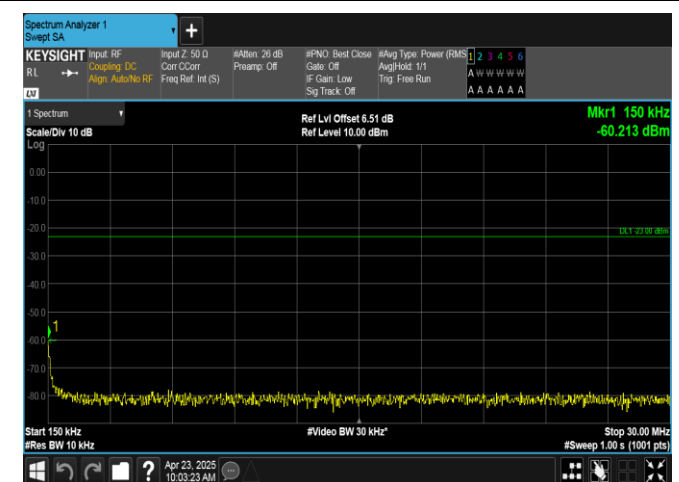
Band12-3MHz-QPSK-23025-1RB#0-0.15~30-PASS
