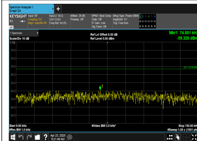
Band12-1.4MHz-16QAM-23095-1RB#0-0.009~0.15-PASS
