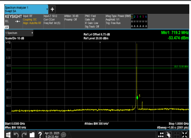
Band12-1.4MHz-QPSK-23173-1RB#5-30~1000-PASS
