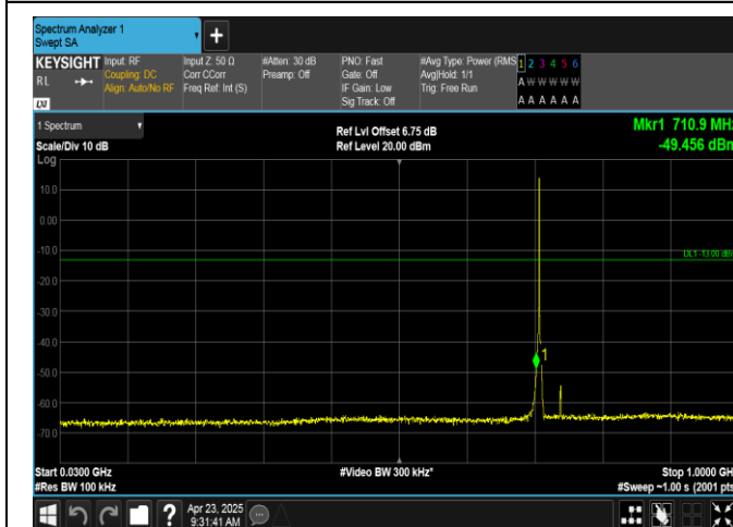
Band12-1.4MHz-QPSK-23173-6RB#0-30~1000-PASS
