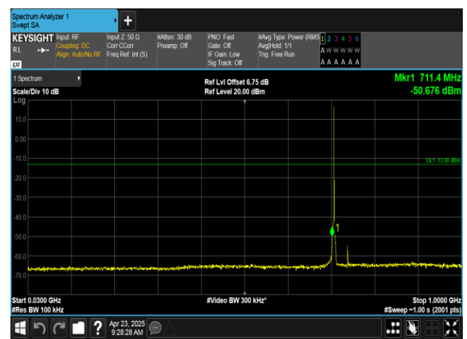
Band12-1.4MHz-16QAM-23173-1RB#0-30~1000-PASS
