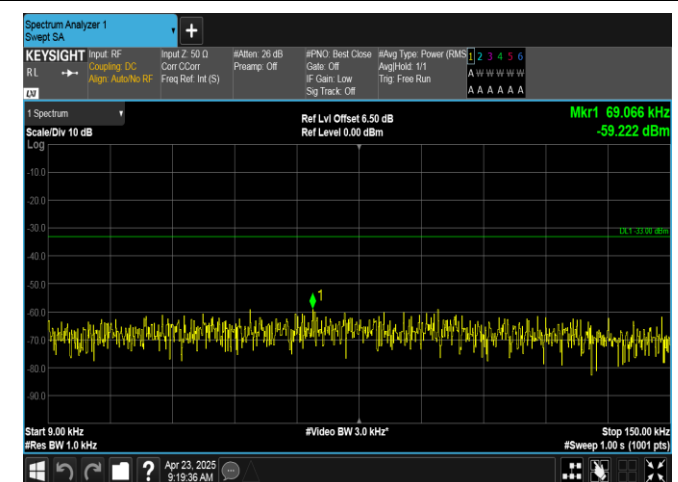
Band12-1.4MHz-16QAM-23017-6RB#0-0.009~0.15-PASS
