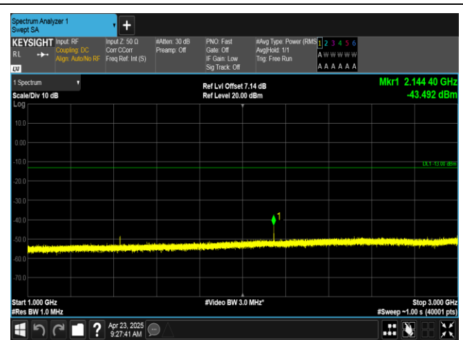
Band12-1.4MHz-QPSK-23173-1RB#0-1000~3000-PASS
