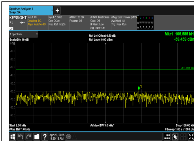
Band12-1.4MHz-16QAM-23173-1RB#5-0.009~0.15-PASS
