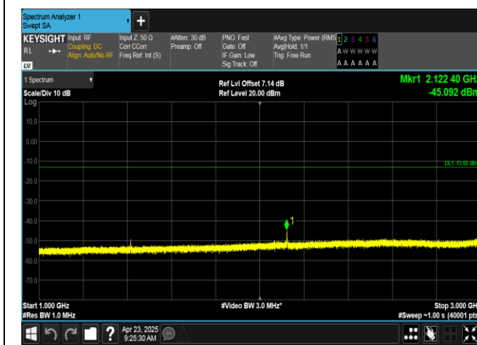
Band12-1.4MHz-QPSK-23095-6RB#0-1000~3000-PASS
