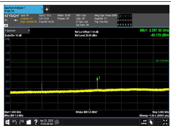
Band12-3MHz-QPSK-23025-1RB#0-1000~3000-PASS
