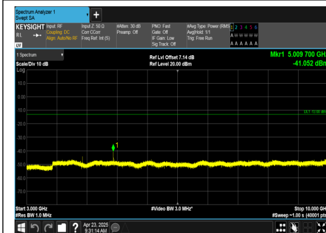
Band12-1.4MHz-16QAM-23173-1RB#5-3000~10000-PASS
