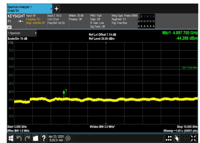
Band12-1.4MHz-16QAM-23017-6RB#0-3000~10000-PASS
