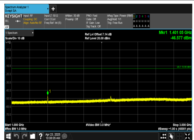
Band12-3MHz-QPSK-23025-15RB#0-1000~3000-PASS
