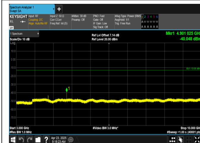
Band12-1.4MHz-16QAM-23017-1RB#5-3000~10000-PASS
