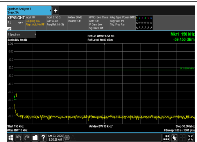
Band12-1.4MHz-16QAM-23173-1RB#5-0.15~30-PASS
