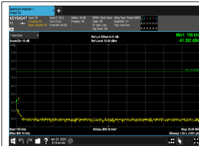
Band12-1.4MHz-16QAM-23017-6RB#0-0.15~30-PASS
