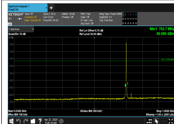
Band12-1.4MHz-16QAM-23095-6RB#0-0.30~1000-PASS
