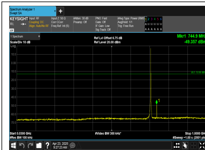
Band12-1.4MHz-QPSK-23173-1RB#0-30~1000-PASS
