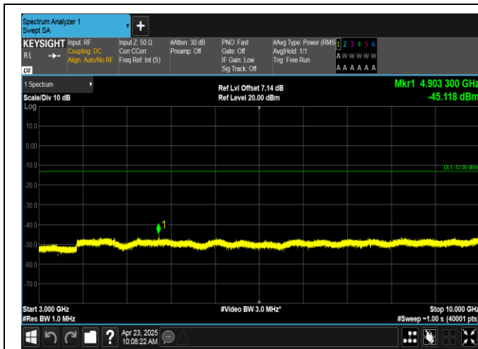
Band12-3MHz-QPSK-23025-15RB#0-3000~10000-PASS
