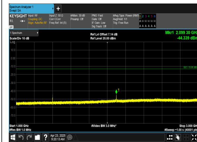
Band12-1.4MHz-16QAM-23017-6RB#0-1000~3000-PASS
