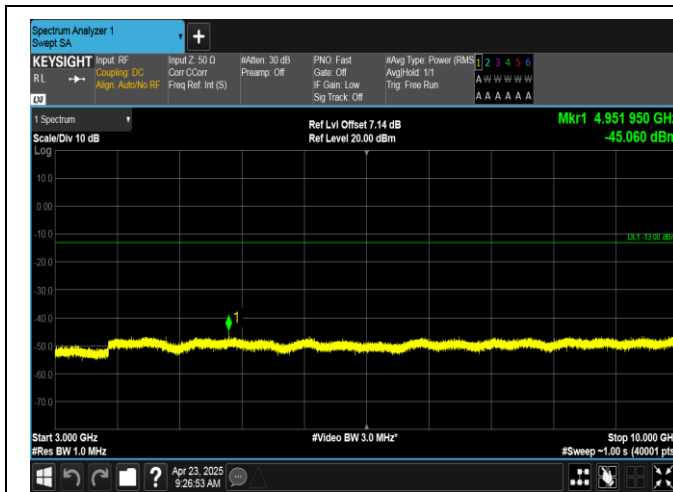
Band12-1.4MHz-16QAM-23095-6RB#0-3000~10000-PASS
