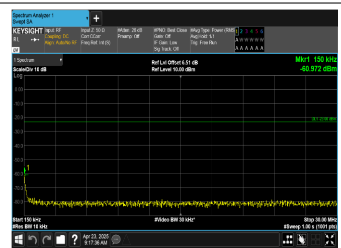
Band12-1.4MHz-16QAM-23017-1RB#5-0.15~30-PASS
