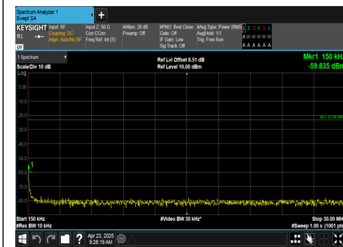
Band12-1.4MHz-16QAM-23173-1RB#0-0.15~30-PASS
