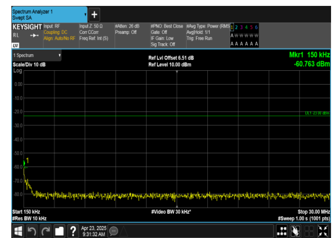
Band12-1.4MHz-QPSK-23173-6RB#0-0.15~30-PASS
