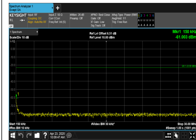
Band12-3MHz-QPSK-23095-1RB#0-0.15~30-PASS
