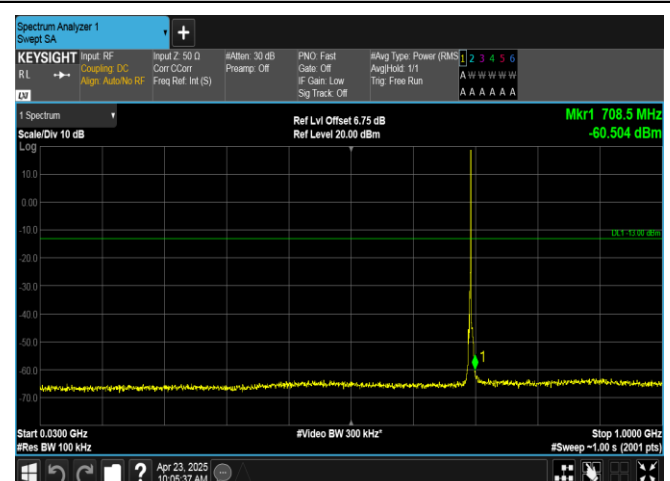
Band12-3MHz-QPSK-23025-1RB#14-30~1000-PASS
