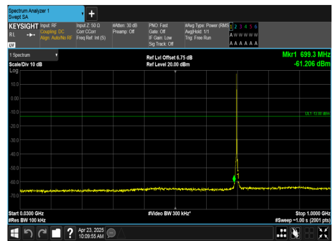
Band12-3MHz-QPSK-23095-1RB#0-30~1000-PASS
