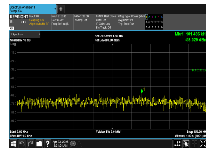
Band12-1.4MHz-QPSK-23173-6RB#0-0.009~0.15-PASS
