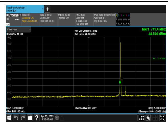
Band12-1.4MHz-16QAM-23173-6RB#0-30~1000-PASS
