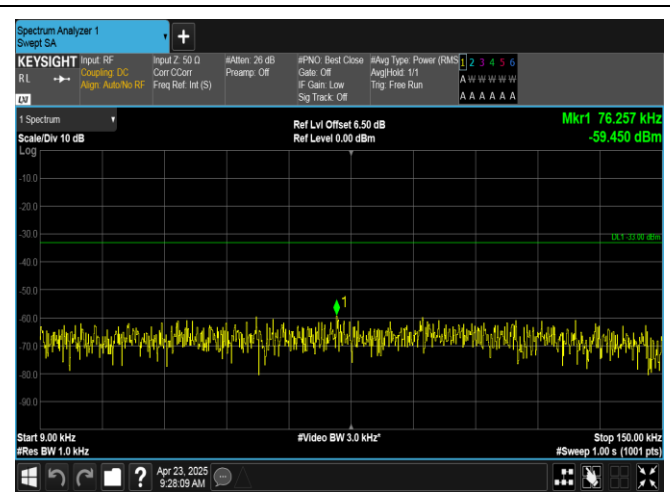
Band12-1.4MHz-16QAM-23173-1RB#0-0.009~0.15-PASS
