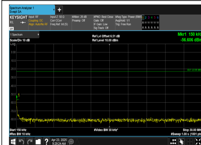
Band12-1.4MHz-QPSK-23173-1RB#5-0.15~30-PASS
