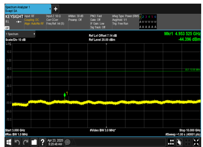
Band12-1.4MHz-QPSK-23095-6RB#0-3000~10000-PASS
