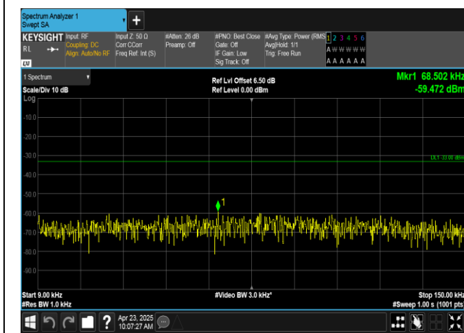
Band12-3MHz-QPSK-23025-15RB#0-0.009~0.15-PASS
