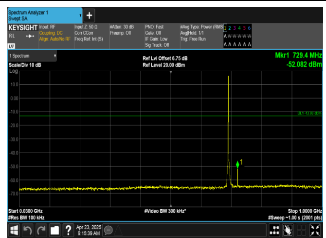
Band12-1.4MHz-16QAM-23017-1RB#0-30~1000-PASS
