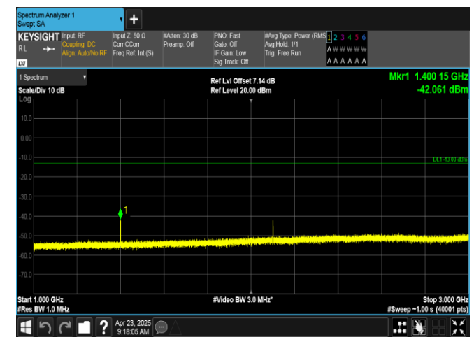
Band12-1.4MHz-16QAM-23017-1RB#5-1000~3000-PASS
