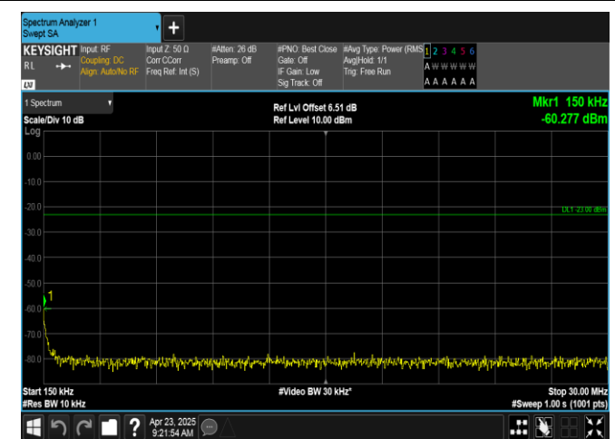
Band12-1.4MHz-16QAM-23095-1RB#0-0.15~30-PASS
