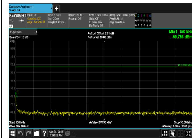
Band12-1.4MHz-QPSK-23095-1RB#0-0.15~30-PASS
