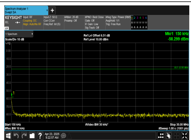
Band12-1.4MHz-QPSK-23095-1RB#5-0.15~30-PASS
