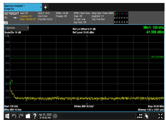
Band12-1.4MHz-QPSK-23017-6RB#0-0.15~30-PASS
