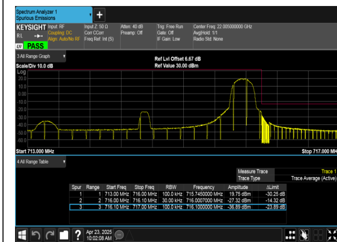
Band12-3MHz-QPSK-23165-1RB#14-PASS
