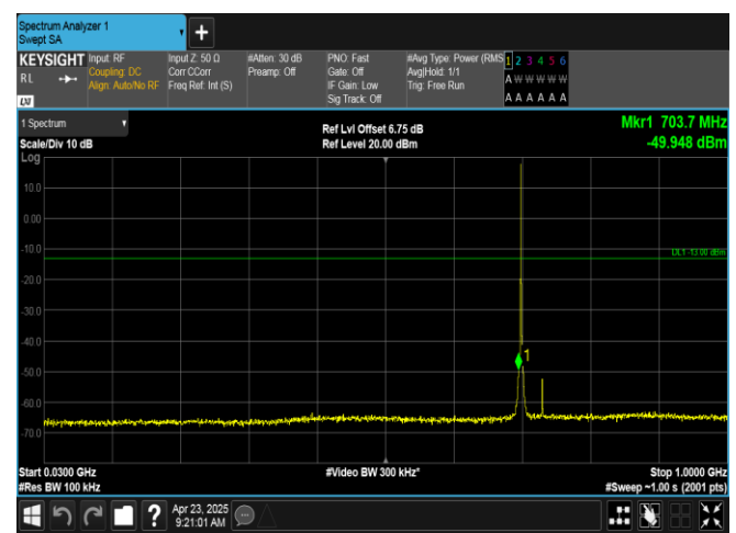
Band12-1.4MHz-QPSK-23095-1RB#0-30~1000-PASS
