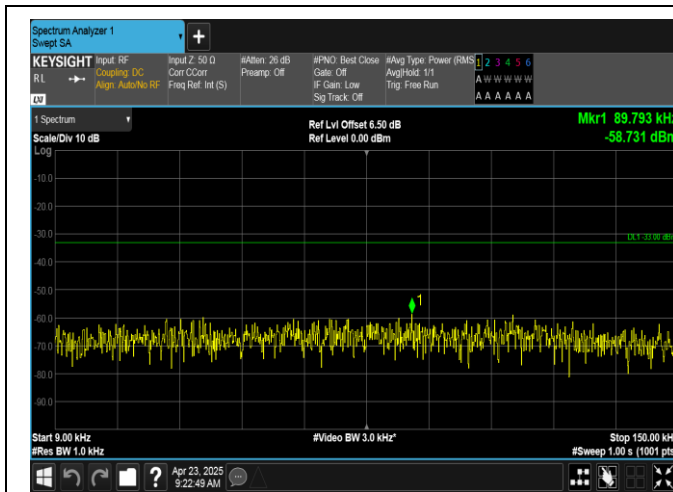
Band12-1.4MHz-QPSK-23095-1RB#5-0.009~0.15-PASS
