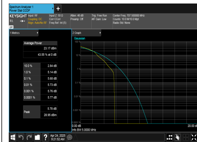
Band12-5MHz-16QAM-23095-1RB#0-PASS
