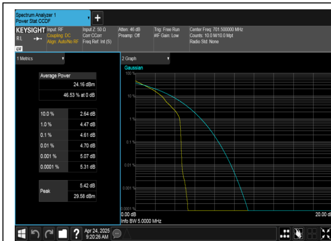
Band12-5MHz-QPSK-23035-1RB#0-PASS
