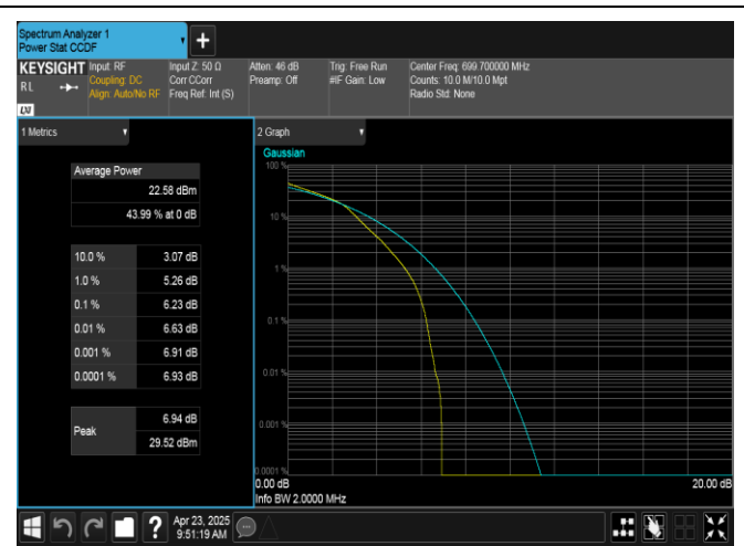
Band12-1.4MHz-16QAM-23017-6RB#0-PASS
