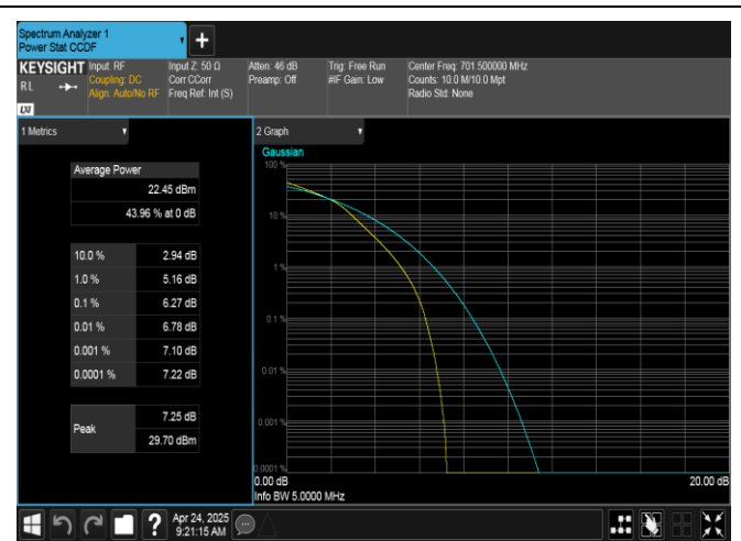
Band12-5MHz-16QAM-23035-25RB#0-PASS
