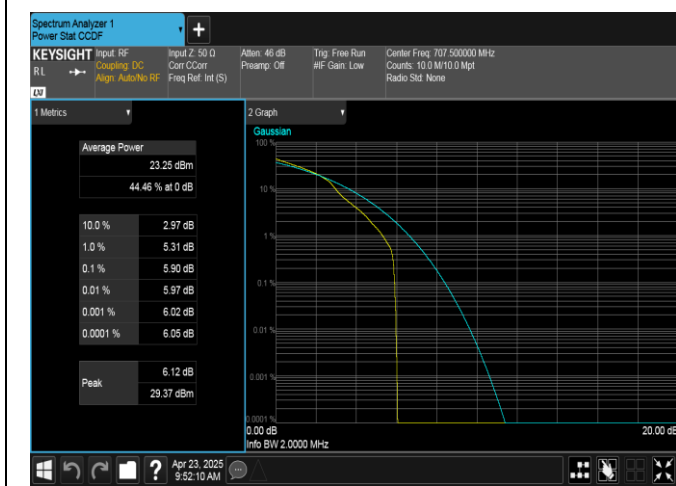
Band12-1.4MHz-16QAM-23095-1RB#0-PASS
