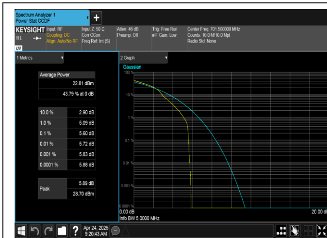
Band12-5MHz-16QAM-23035-1RB#0-PASS
