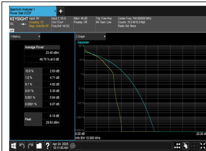
Band12-10MHz-QPSK-23060-1RB#0-PASS
