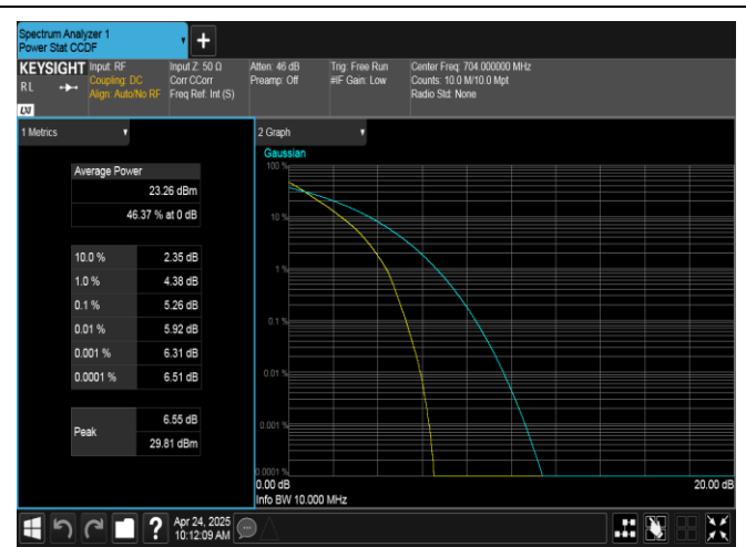
Band12-10MHz-QPSK-23060-50RB#0-PASS
