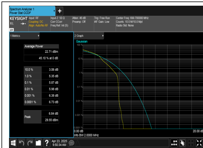
Band12-1.4MHz-16QAM-23017-1RB#0-PASS
