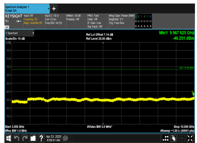
Band5-10MHz-16QAM-20600-50RB#0-3000~10000-PASS
