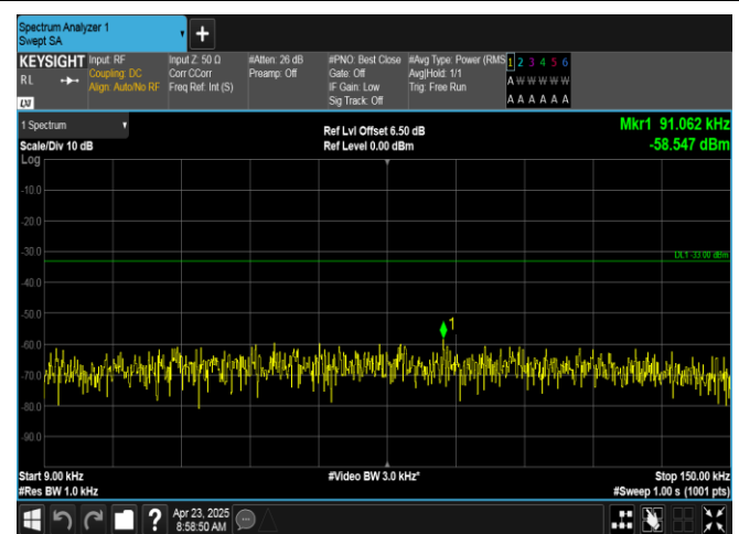
Band5-10MHz-16QAM-20600-50RB#0-0.009~0.15-PASS
