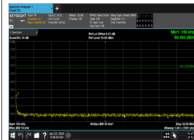
Band5-10MHz-QPSK-20525-1RB#0-0.15~30-PASS
