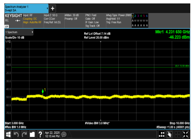
Band5-5MHz-16QAM-20625-25RB#0-3000~10000-PASS
