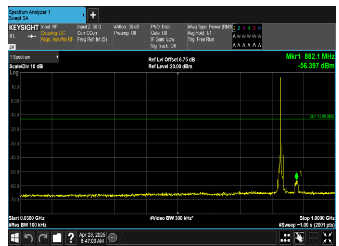
Band5-10MHz-QPSK-20525-1RB#0-30~1000-PASS
