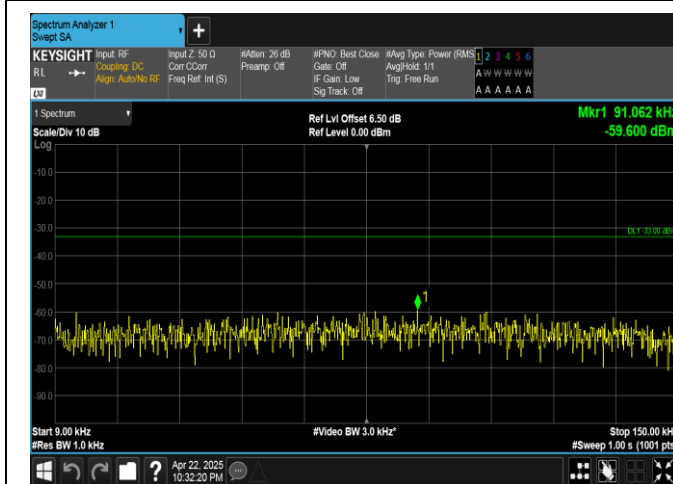
Band5-10MHz-QPSK-20450-1RB#0-0.009~0.15-PASS
