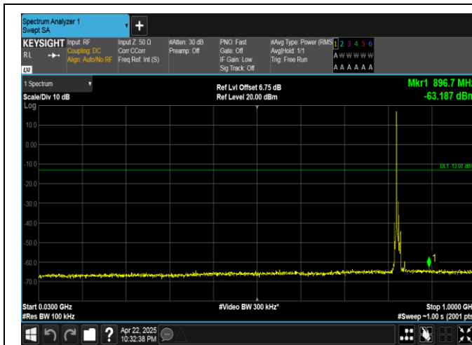
Band5-10MHz-QPSK-20450-1RB#0-30~1000-PASS
