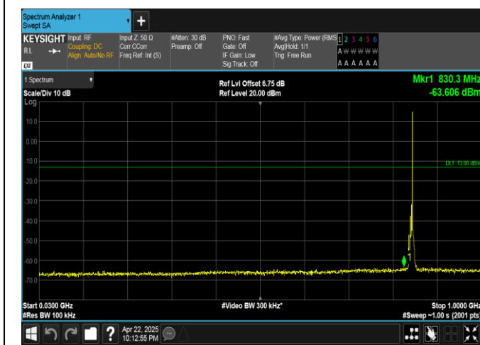
Band5-5MHz-16QAM-20625-1RB#24-30~1000-PASS
