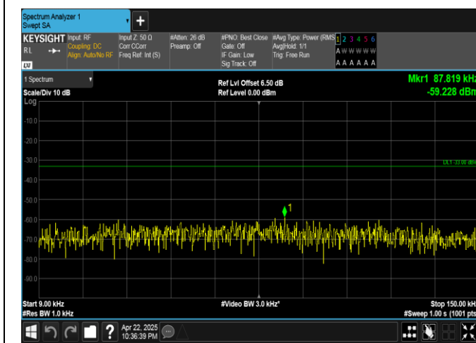
Band5-10MHz-QPSK-20450-50RB#0-0.009~0.15-PASS
