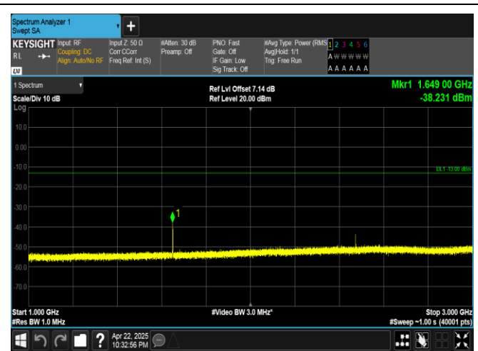
Band5-10MHz-QPSK-20450-1RB#0-1000~3000-PASS
