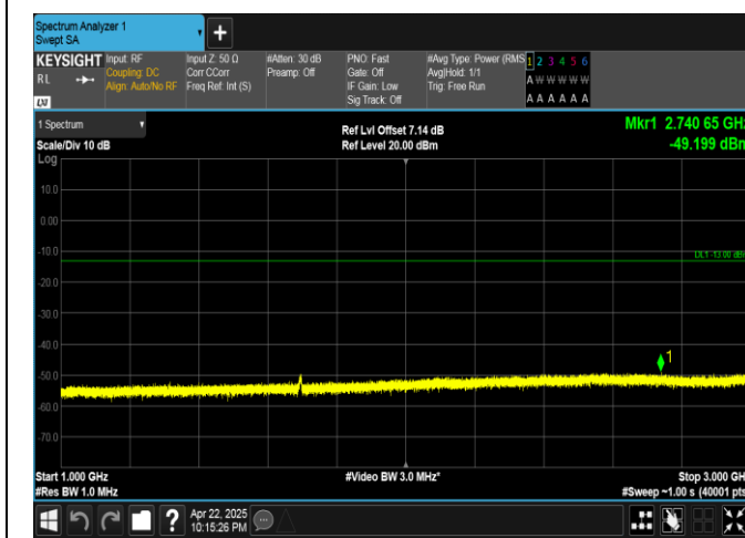
Band5-5MHz-16QAM-20625-25RB#0-1000~3000-PASS
