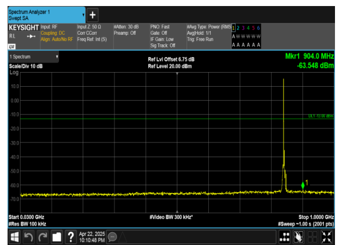
Band5-5MHz-16QAM-20625-1RB#0-30~1000-PASS
