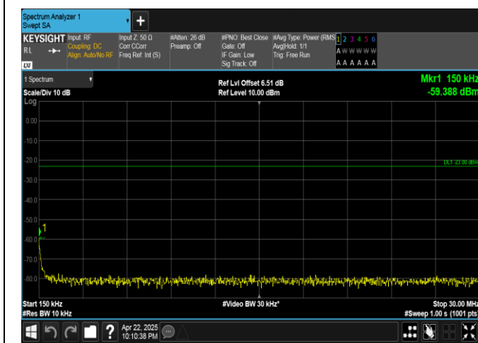
Band5-5MHz-16QAM-20625-1RB#0-0.15~30-PASS
