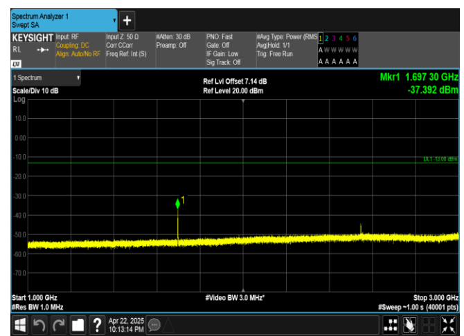
Band5-5MHz-16QAM-20625-1RB#24-1000~3000-PASS
