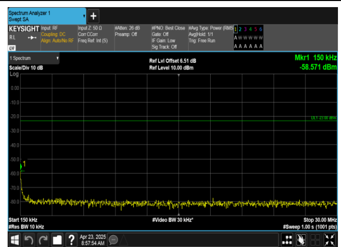
Band5-10MHz-QPSK-20600-50RB#0-0.15~30-PASS
