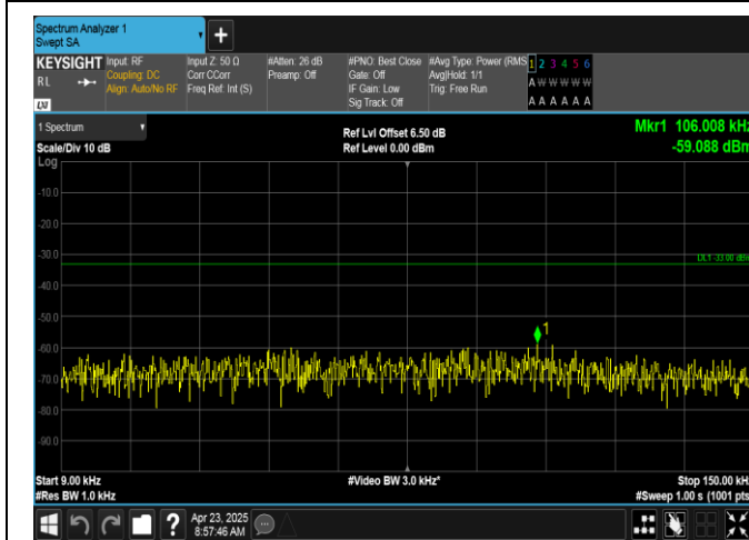
Band5-10MHz-QPSK-20600-50RB#0-0.009~0.15-PASS
