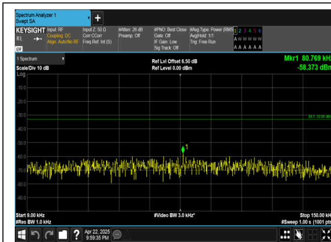
Band5-5MHz-16QAM-20425-1RB#24-0.009~0.15-PASS
