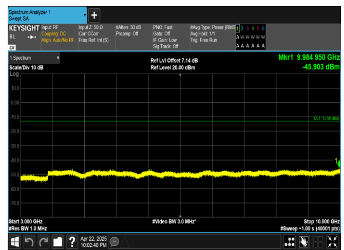
Band5-5MHz-16QAM-20425-25RB#0-3000~10000-PASS
