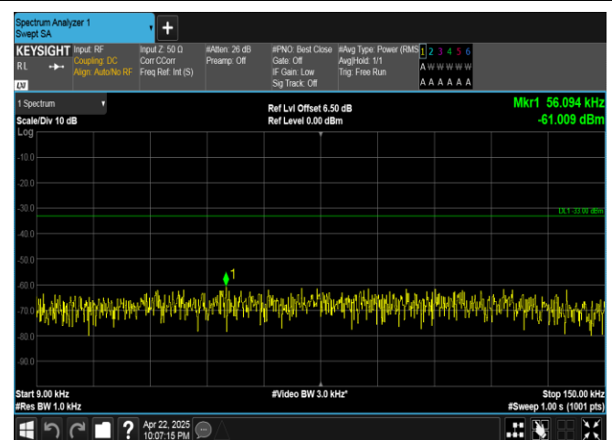
Band5-5MHz-QPSK-20525-25RB#0-0.009~0.15-PASS
