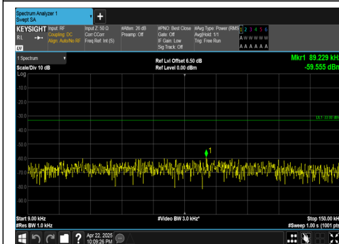
Band5-5MHz-QPSK-20625-1RB#0-0.009~0.15-PASS
