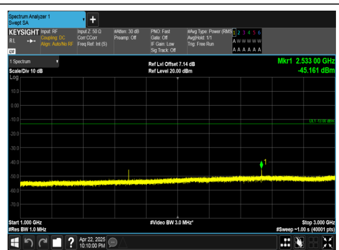
Band5-5MHz-QPSK-20625-1RB#0-1000~3000-PASS
