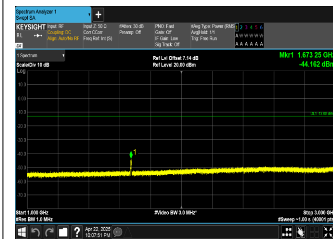
Band5-5MHz-QPSK-20525-25RB#0-1000~3000-PASS
