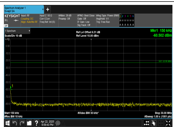
Band5-5MHz-16QAM-20425-1RB#24-0.15~30-PASS
