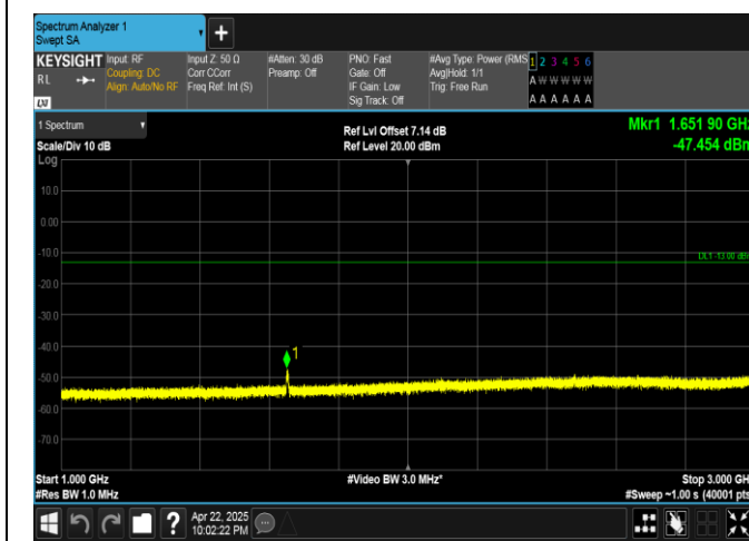
Band5-5MHz-16QAM-20425-25RB#0-1000~3000-PASS
