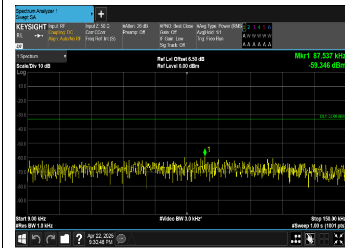
Band5-3MHz-16QAM-20525-15RB#0-0.009~0.15-PASS
