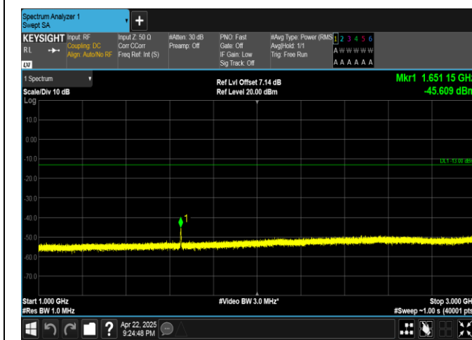
Band5-3MHz-16QAM-20415-15RB#0-1000~3000-PASS
