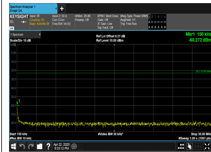
Band5-3MHz-16QAM-20635-1RB#0-0.15~30-PASS
