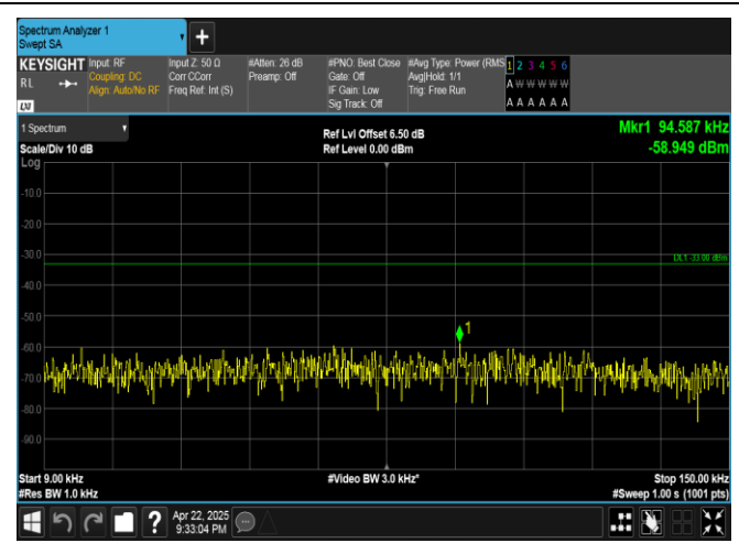
Band5-3MHz-16QAM-20635-1RB#0-0.009~0.15-PASS
