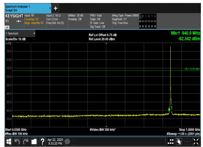
Band5-3MHz-16QAM-20635-1RB#0-30~1000-PASS
