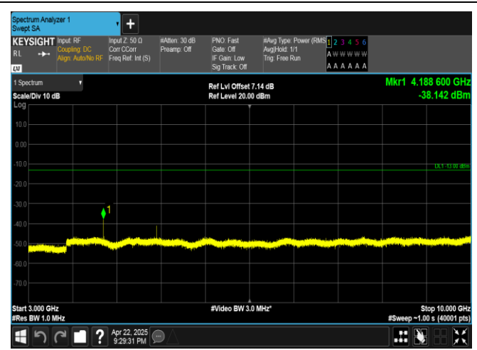
Band5-3MHz-16QAM-20525-1RB#14-3000~10000-PASS
