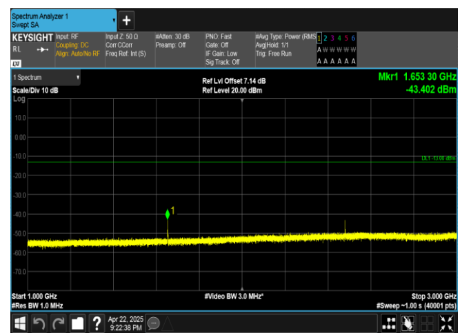
Band5-3MHz-16QAM-20415-1RB#14-1000~3000-PASS
