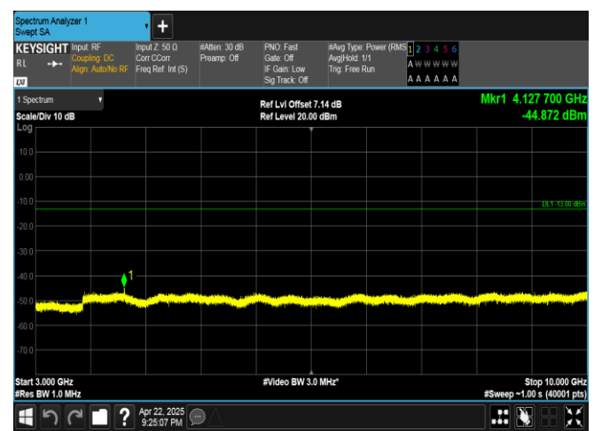
Band5-3MHz-16QAM-20415-15RB#0-3000~10000-PASS
