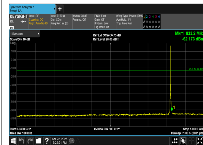
Band5-3MHz-16QAM-20415-1RB#14-30~1000-PASS
