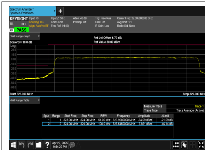
Band5-5MHz-QPSK-20425-25RB#0-PASS
