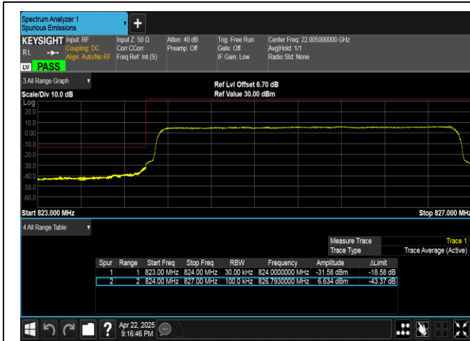
Band5-3MHz-QPSK-20415-15RB#0-PASS
