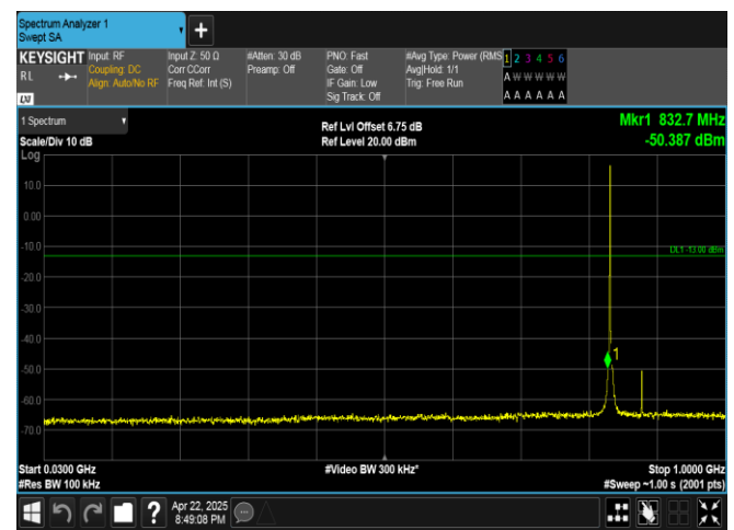
Band5-1.4MHz-QPSK-20525-1RB#0-30~1000-PASS
