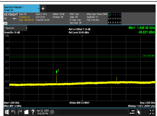
Band5-1.4MHz-QPSK-20407-1RB#0-1000~3000-PASS
