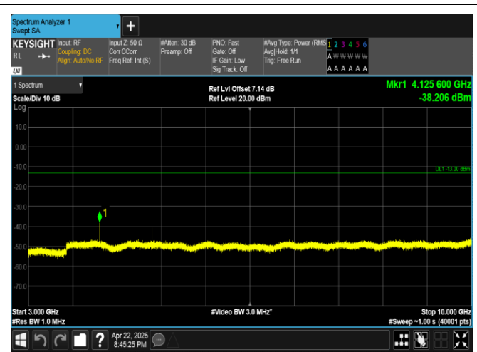
Band5-1.4MHz-QPSK-20407-1RB#5-3000~10000-PASS
