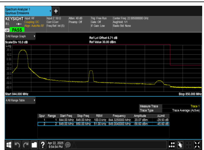
Band5-5MHz-QPSK-20625-1RB#0-PASS
