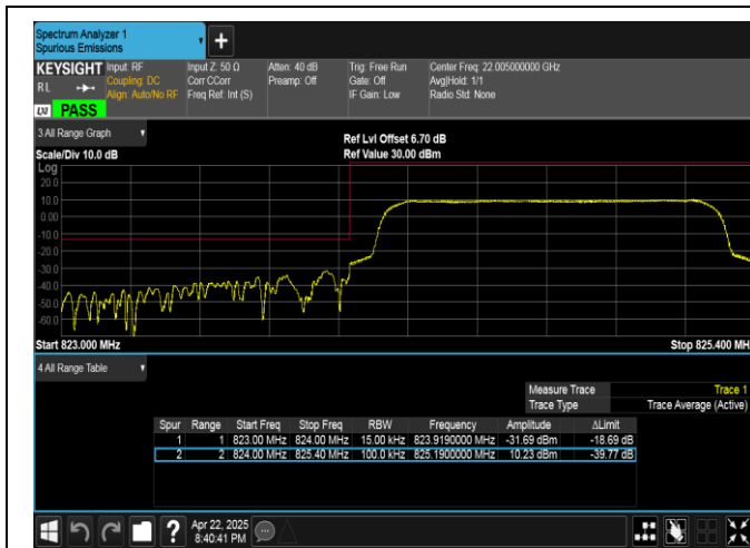
Band5-1.4MHz-QPSK-20407-6RB#0-PASS
