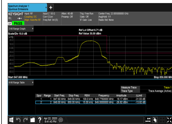
Band5-1.4MHz-16QAM-20643-1RB#5-PASS
