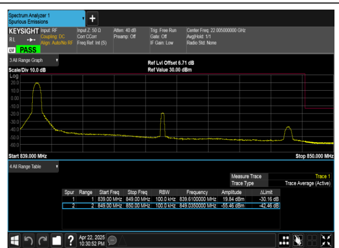
Band5-10MHz-QPSK-20600-1RB#0-PASS
