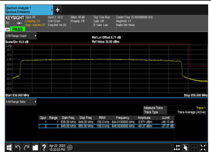
Band5-10MHz-16QAM-20600-50RB#0-PASS
