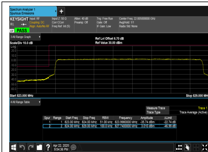
Band5-5MHz-16QAM-20425-25RB#0-PASS
