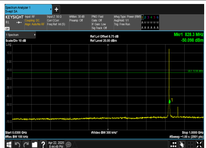
Band5-1.4MHz-QPSK-20407-1RB#5-30~1000-PASS
