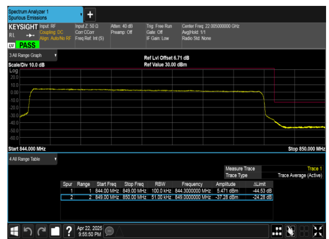
Band5-5MHz-QPSK-20625-25RB#0-PASS
