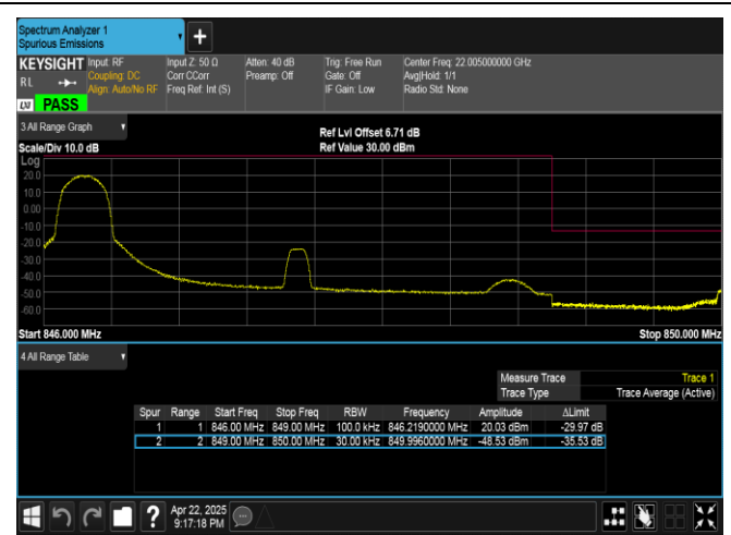
Band5-3MHz-QPSK-20635-1RB#0-PASS
