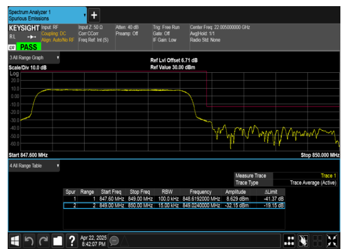
Band5-1.4MHz-16QAM-20643-6RB#0-PASS
