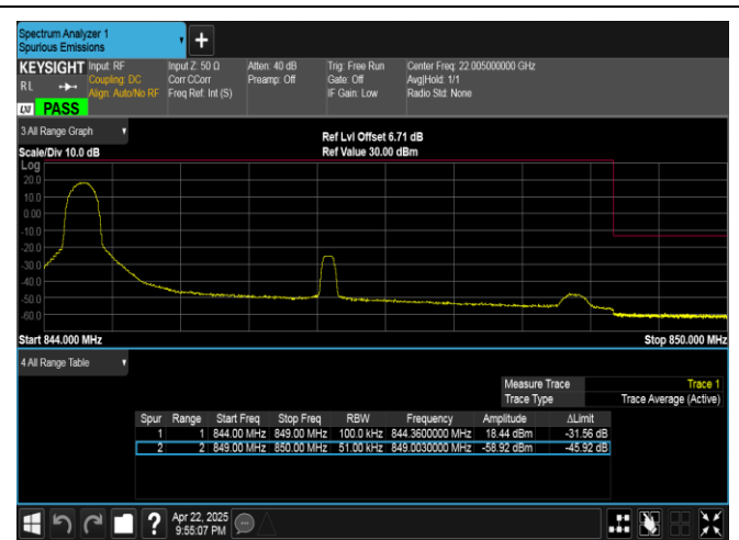
Band5-5MHz-16QAM-20625-1RB#0-PASS
