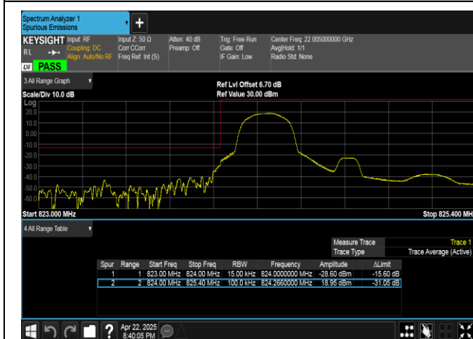
Band5-1.4MHz-16QAM-20407-1RB#0-PASS
