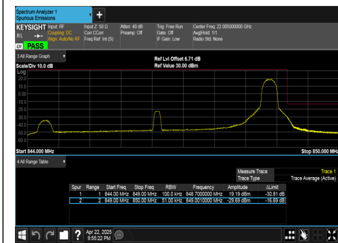
Band5-5MHz-QPSK-20625-1RB#24-PASS
