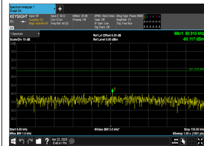
Band5-1.4MHz-QPSK-20407-6RB#0-0.009~0.15-PASS
