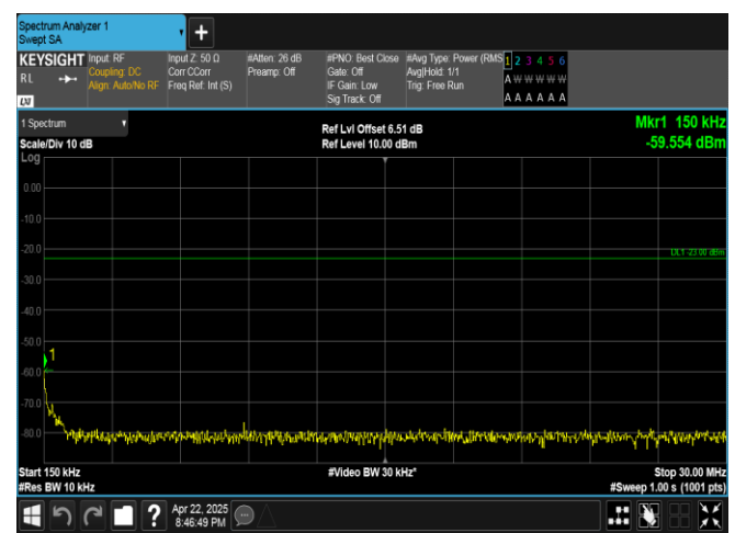
Band5-1.4MHz-QPSK-20407-6RB#0-0.15~30-PASS
