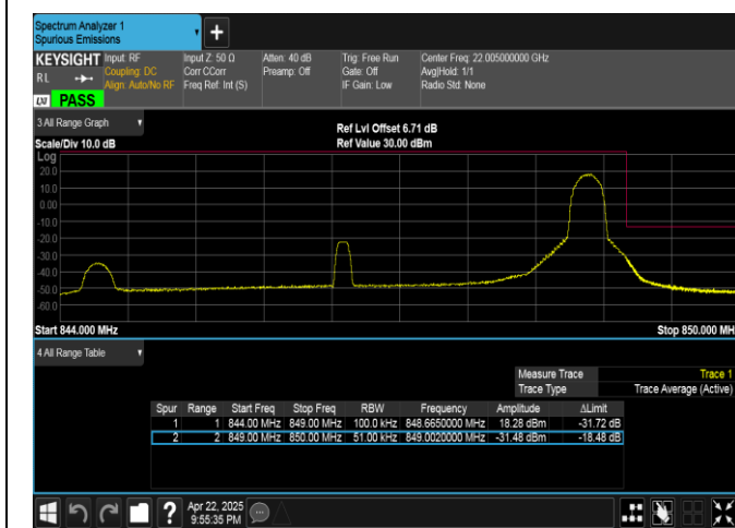
Band5-5MHz-16QAM-20625-1RB#24-PASS
