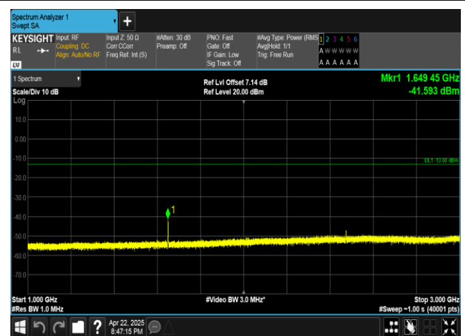
Band5-1.4MHz-QPSK-20407-6RB#0-1000~3000-PASS
