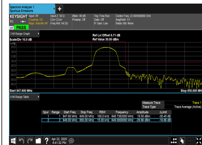
Band5-1.4MHz-QPSK-20643-1RB#5-PASS
