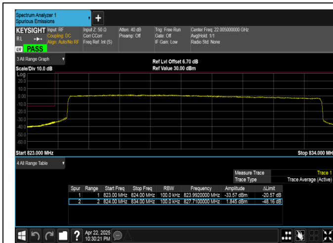
Band5-10MHz-QPSK-20450-50RB#0-PASS
