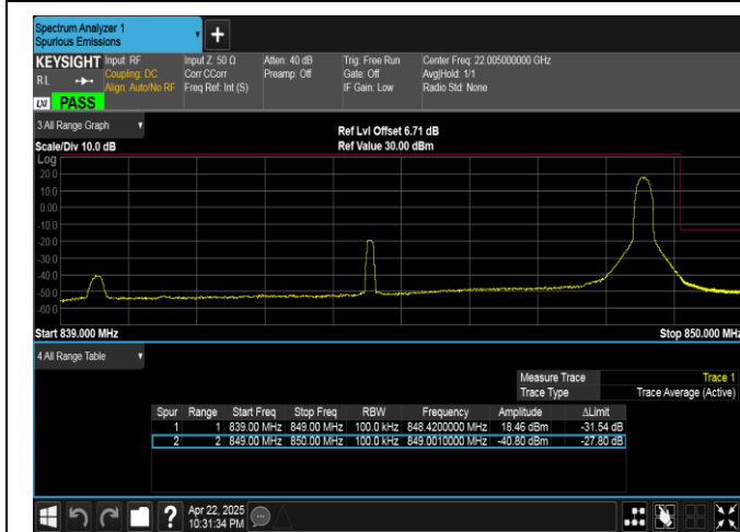
Band5-10MHz-16QAM-20600-1RB#49-PASS
