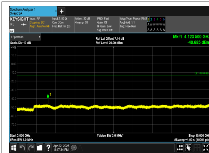
Band5-1.4MHz-QPSK-20407-6RB#0-3000~10000-PASS
