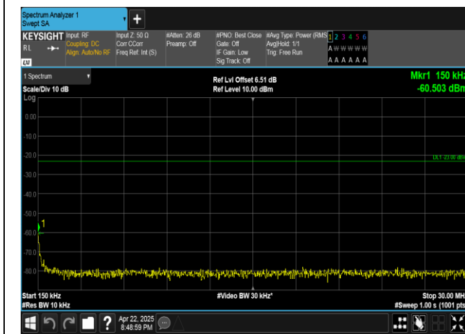
Band5-1.4MHz-QPSK-20525-1RB#0-0.15~30-PASS
