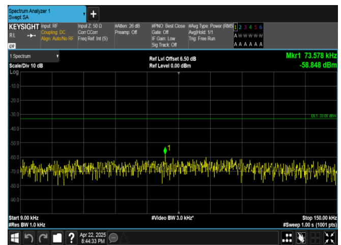
Band5-1.4MHz-QPSK-20407-1RB#5-0.009~0.15-PASS
