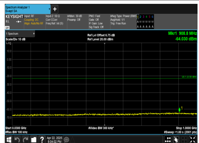
Band4-20MHz-16QAM-20175-1RB#99-30~1000-PASS
