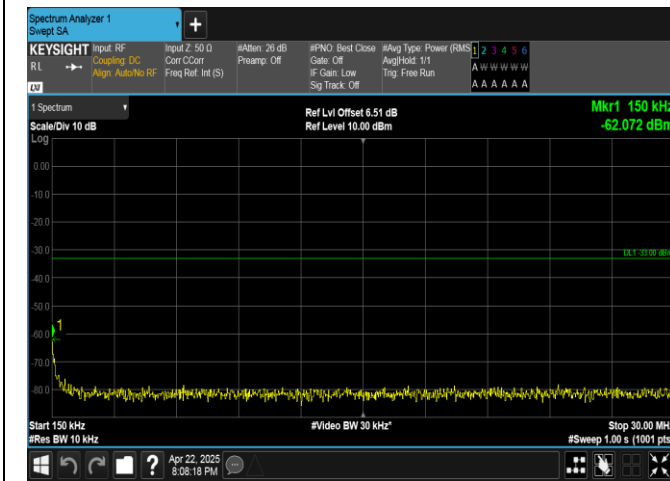
Band4-20MHz-16QAM-20300-1RB#0-0.15~30-PASS
