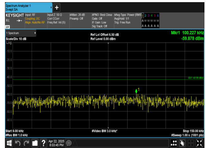
Band4-20MHz-16QAM-20175-1RB#99-0.009~0.15-PASS
