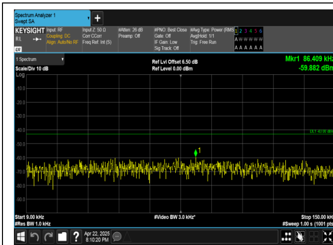
Band4-20MHz-16QAM-20300-1RB#99-0.009~0.15-PASS
