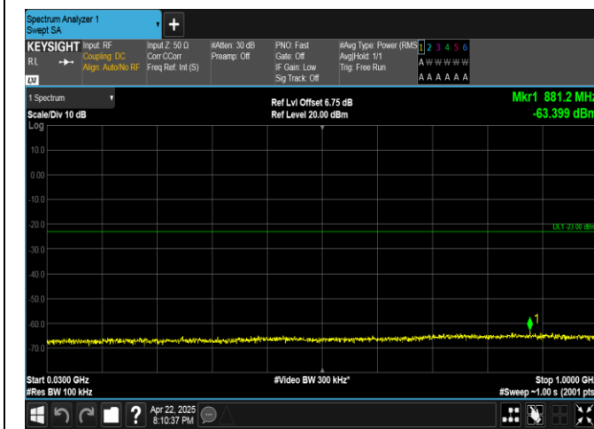
Band4-20MHz-16QAM-20300-1RB#99-30~1000-PASS
