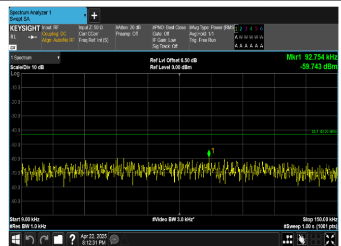
Band4-20MHz-16QAM-20300-100RB#0-0.009~0.15-PASS
