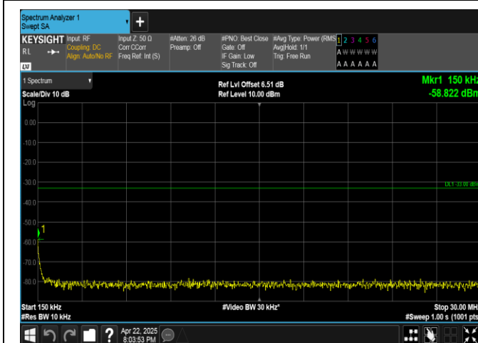
Band4-20MHz-16QAM-20175-1RB#99-0.15~30-PASS
