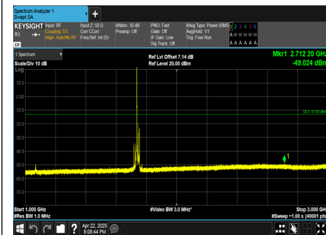
Band4-20MHz-16QAM-20300-1RB#0-1000~3000-PASS
