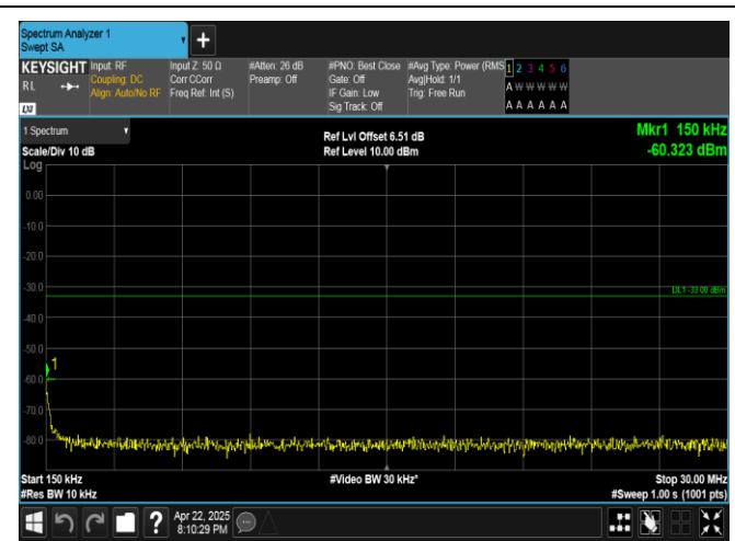
Band4-20MHz-16QAM-20300-1RB#99-0.15~30-PASS
