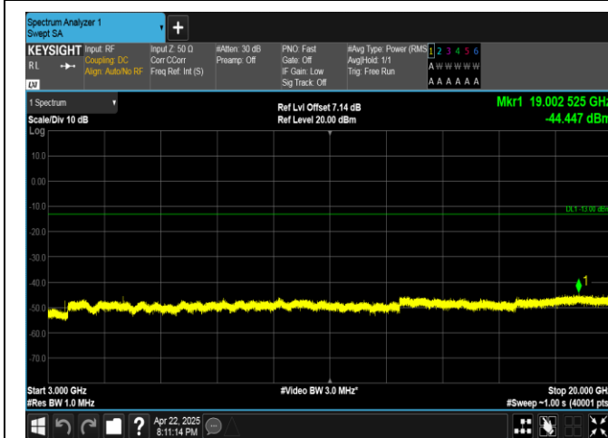
Band4-20MHz-16QAM-20300-1RB#99-3000~20000-PASS
