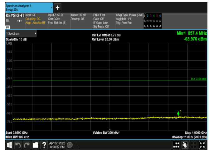
Band4-20MHz-16QAM-20300-1RB#0-30~1000-PASS
