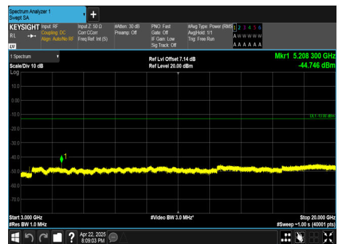
Band4-20MHz-16QAM-20300-1RB#0-3000~20000-PASS
