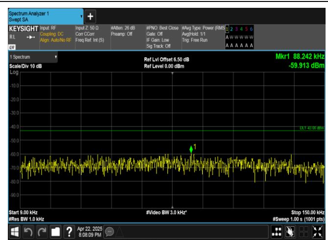
Band4-20MHz-16QAM-20300-1RB#0-0.009~0.15-PASS
