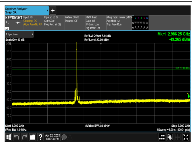
Band4-20MHz-16QAM-20175-1RB#0-1000~3000-PASS
