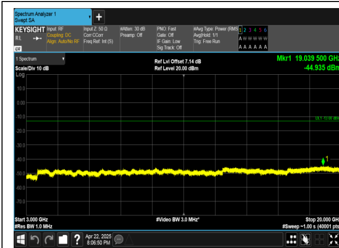
Band4-20MHz-16QAM-20175-100RB#0-3000~20000-PASS
