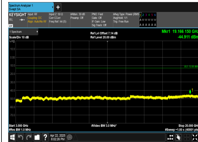
Band4-20MHz-16QAM-20175-1RB#0-3000~20000-PASS
