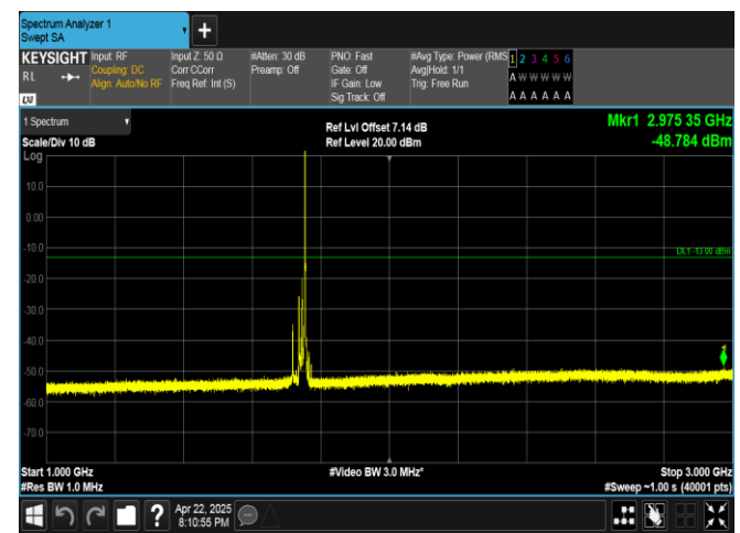
Band4-20MHz-16QAM-20300-1RB#99-1000~3000-PASS
