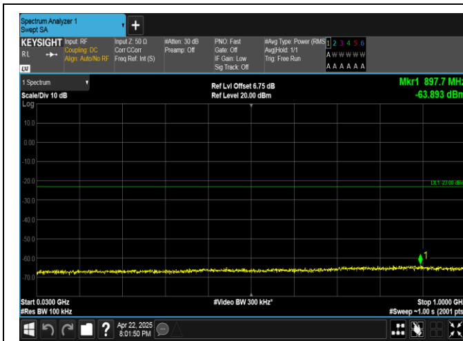
Band4-20MHz-16QAM-20175-1RB#0-30~1000-PASS
