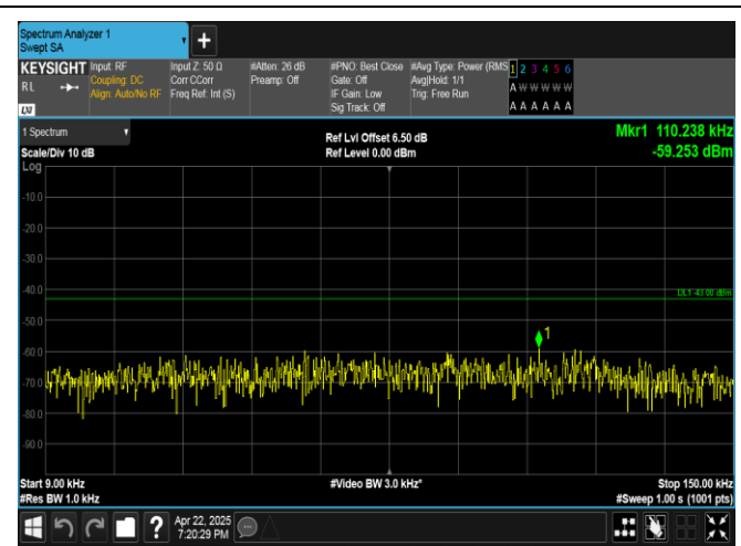
Band4-15MHz-16QAM-20325-1RB#0-0.009~0.15-PASS
