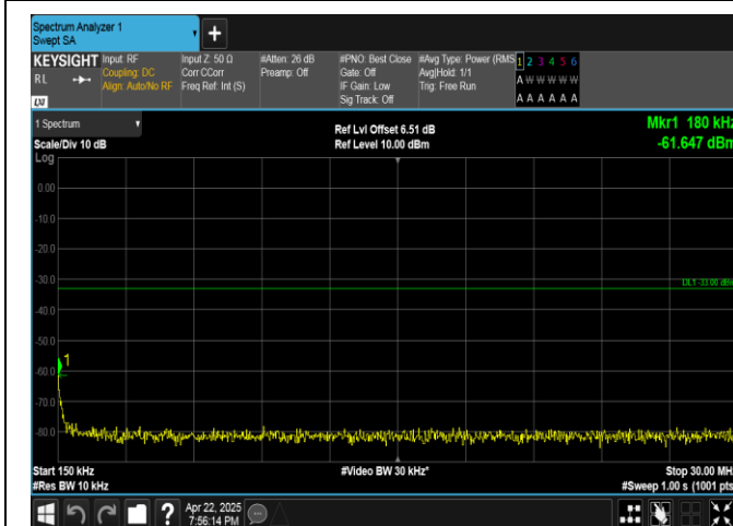
Band4-20MHz-QPSK-20050-1RB#99-0.15~30-PASS
