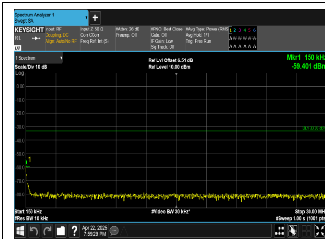
Band4-20MHz-16QAM-20050-100RB#0-0.15~30-PASS
