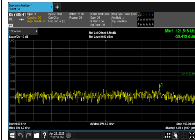
Band4-20MHz-QPSK-20050-100RB#0-0.009~0.15-PASS
