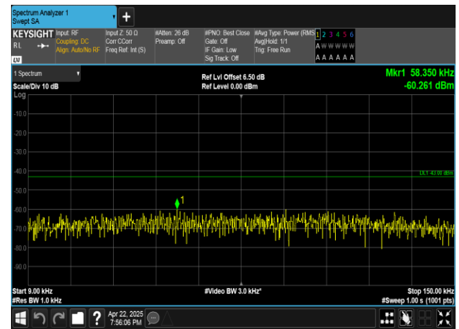
Band4-20MHz-QPSK-20050-1RB#99-0.009~0.15-PASS
