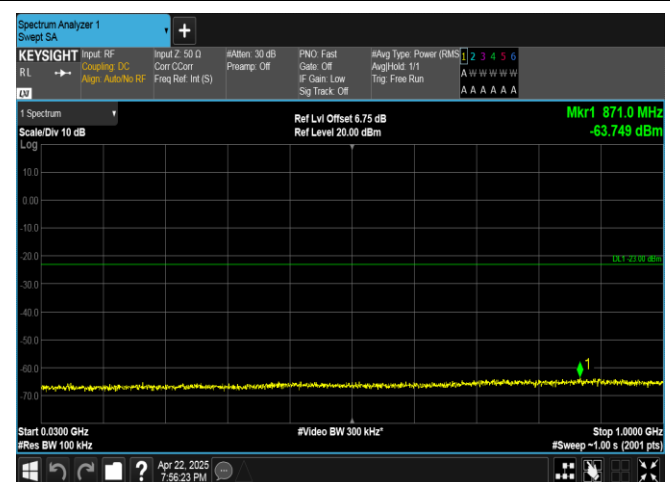
Band4-20MHz-QPSK-20050-1RB#99-30~1000-PASS
