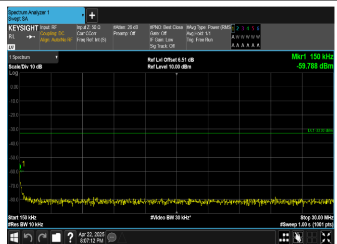
Band4-20MHz-QPSK-20300-1RB#0-0.15~30-PASS
