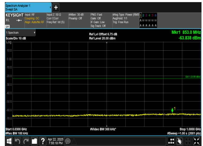
Band4-20MHz-16QAM-20050-1RB#0-30~1000-PASS
