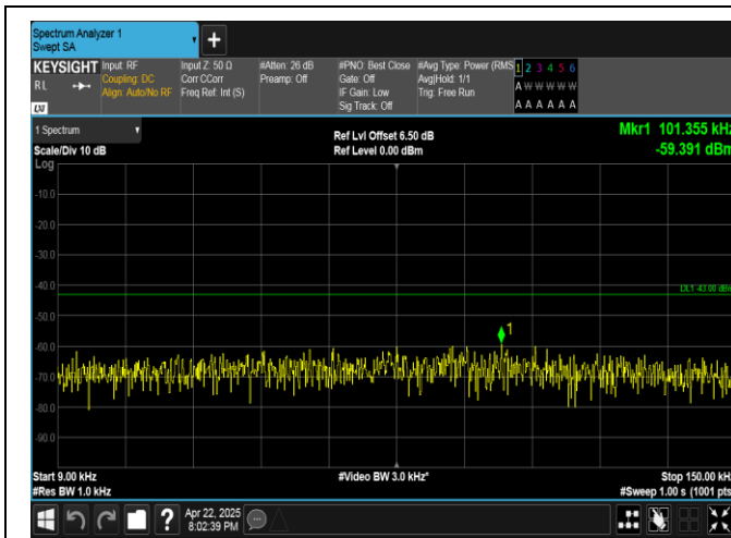
Band4-20MHz-QPSK-20175-1RB#99-0.009~0.15-PASS
