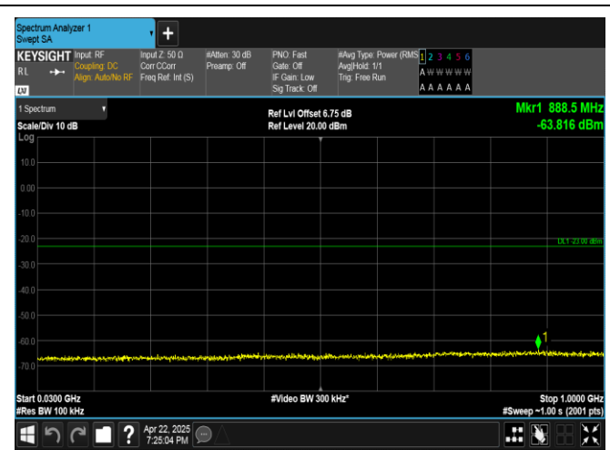
Band4-15MHz-16QAM-20325-75RB#0-30~1000-PASS
