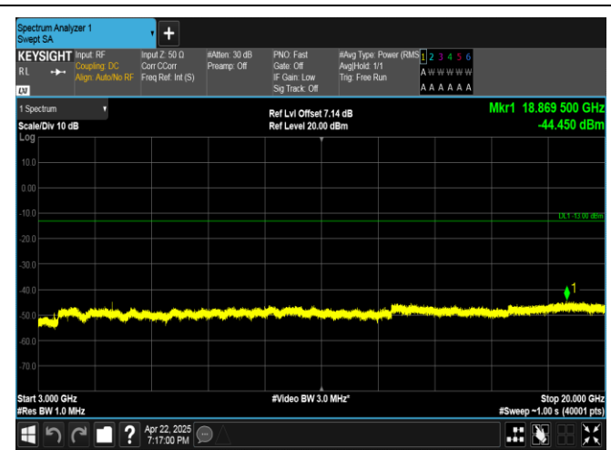
Band4-15MHz-16QAM-20175-1RB#74-3000~20000-PASS
