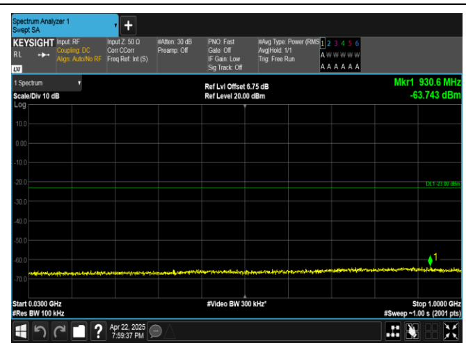
Band4-20MHz-16QAM-20050-100RB#0-30~1000-PASS
