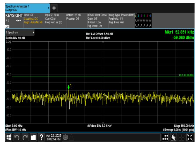
Band4-20MHz-QPSK-20300-1RB#99-0.009~0.15-PASS
