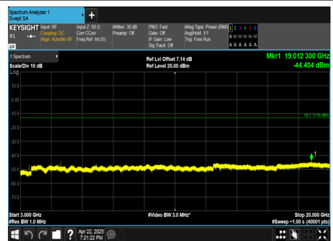
Band4-15MHz-16QAM-20325-1RB#0-3000~20000-PASS
