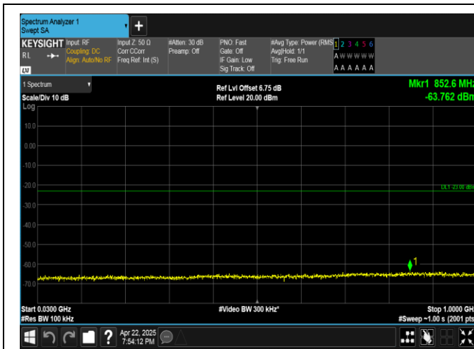
Band4-20MHz-QPSK-20050-1RB#0-30~1000-PASS
