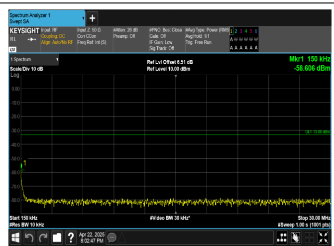
Band4-20MHz-QPSK-20175-1RB#99-0.15~30-PASS
