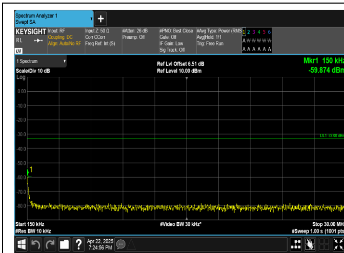
Band4-15MHz-16QAM-20325-75RB#0-0.15~30-PASS
