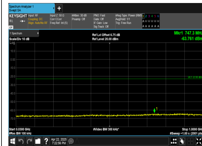
Band4-15MHz-16QAM-20325-1RB#74-30~1000-PASS
