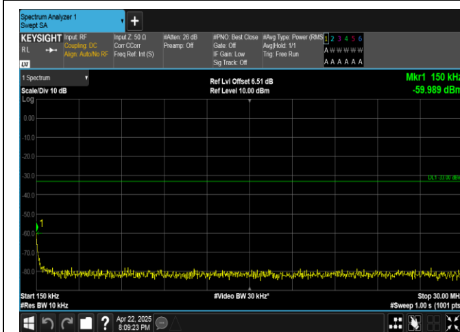
Band4-20MHz-QPSK-20300-1RB#99-0.15~30-PASS
