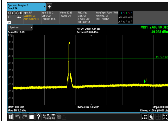
Band4-20MHz-16QAM-20050-100RB#0-1000~3000-PASS
