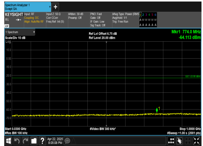
Band4-20MHz-QPSK-20175-100RB#0-30~1000-PASS
