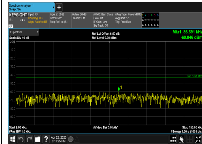
Band4-20MHz-QPSK-20300-100RB#0-0.009~0.15-PASS
