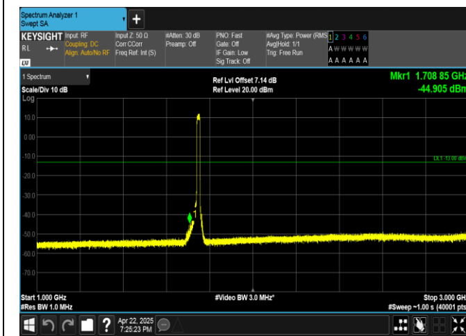
Band4-15MHz-16QAM-20325-75RB#0-1000~3000-PASS
