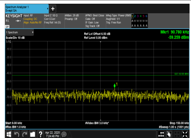
Band4-15MHz-16QAM-20325-75RB#0-0.009~0.15-PASS
