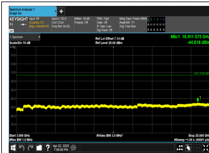
Band4-20MHz-QPSK-20050-100RB#0-3000~20000-PASS
