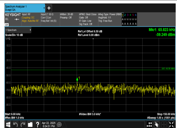
Band4-20MHz-QPSK-20175-100RB#0-0.009~0.15-PASS
