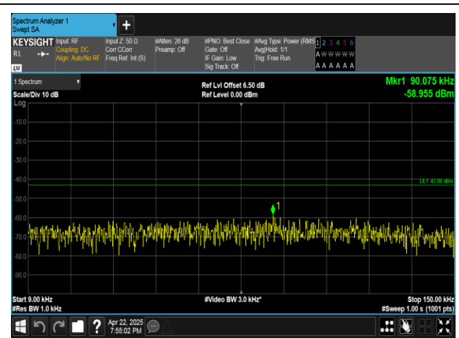
Band4-20MHz-16QAM-20050-1RB#0-0.009~0.15-PASS
