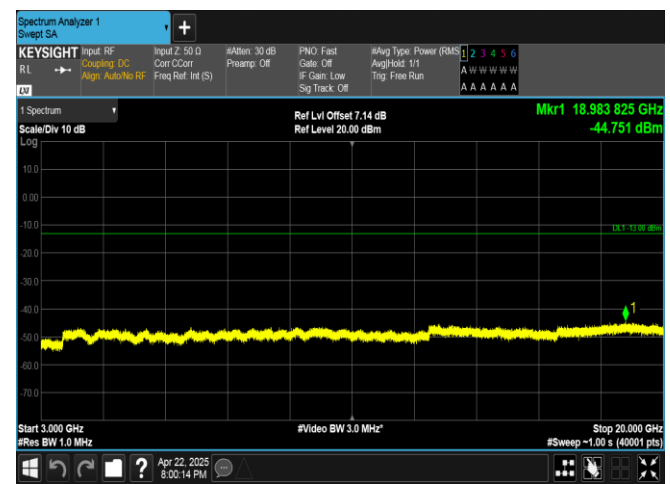
Band4-20MHz-16QAM-20050-100RB#0-3000~20000-PASS
