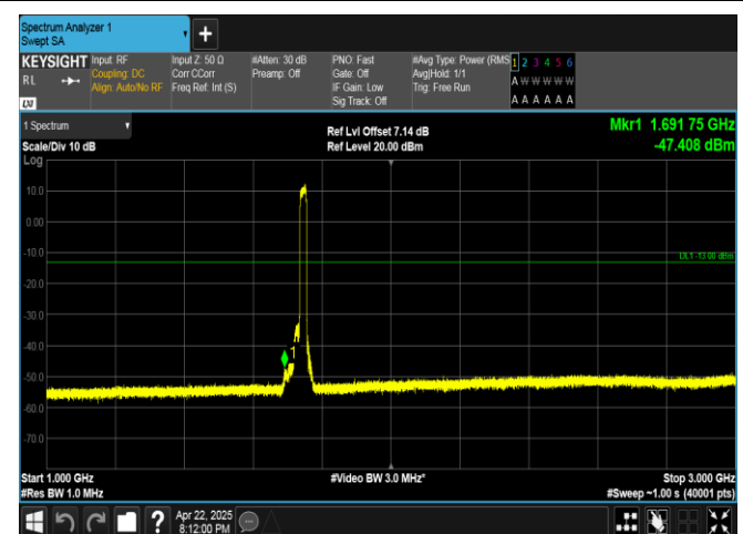
Band4-20MHz-QPSK-20300-100RB#0-1000~3000-PASS
