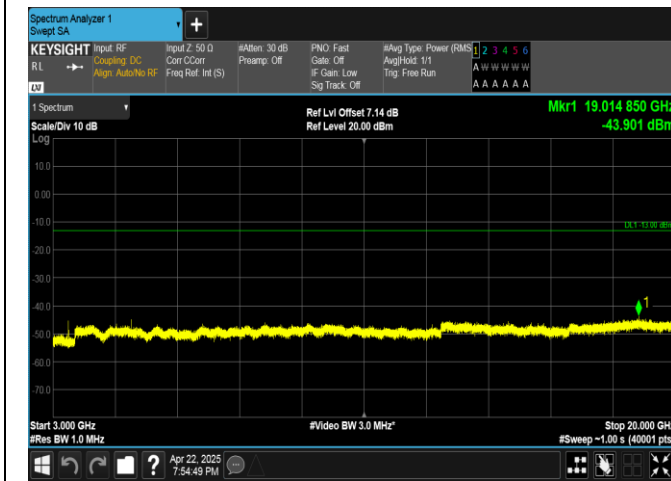
Band4-20MHz-QPSK-20050-1RB#0-3000~20000-PASS
