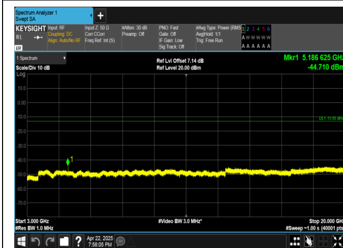
Band4-20MHz-16QAM-20050-1RB#99-3000~20000-PASS
