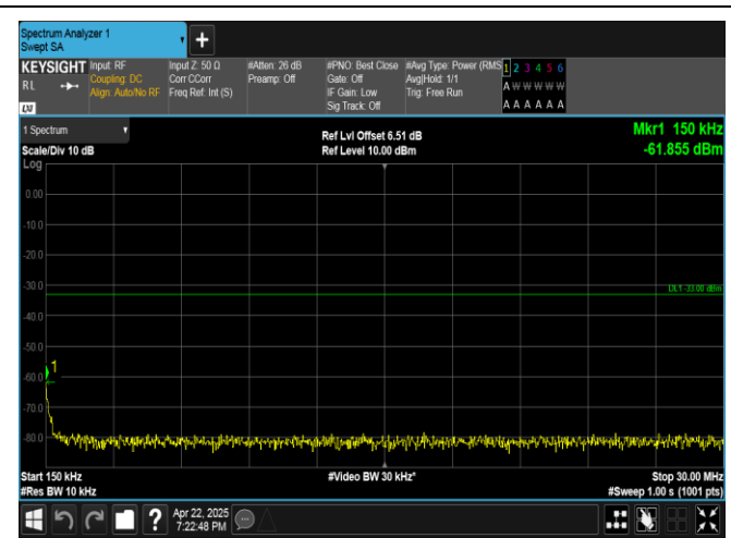
Band4-15MHz-16QAM-20325-1RB#74-0.15~30-PASS
