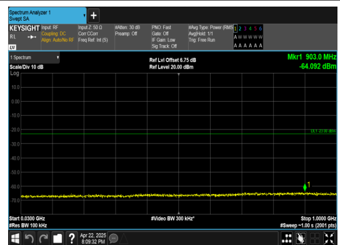
Band4-20MHz-QPSK-20300-1RB#99-30~1000-PASS
