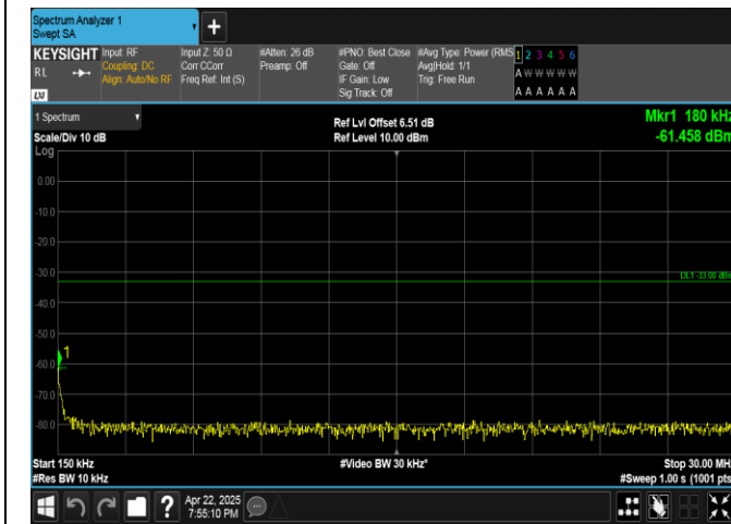
Band4-20MHz-16QAM-20050-1RB#0-0.15~30-PASS
