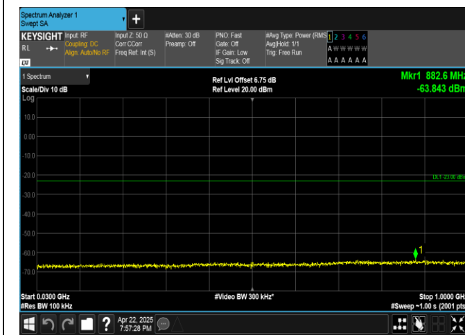
Band4-20MHz-16QAM-20050-1RB#99-30~1000-PASS
