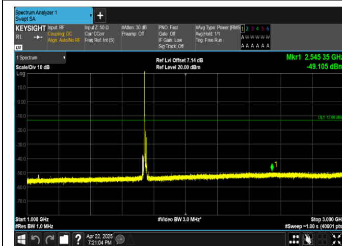
Band4-15MHz-16QAM-20325-1RB#0-1000~3000-PASS
