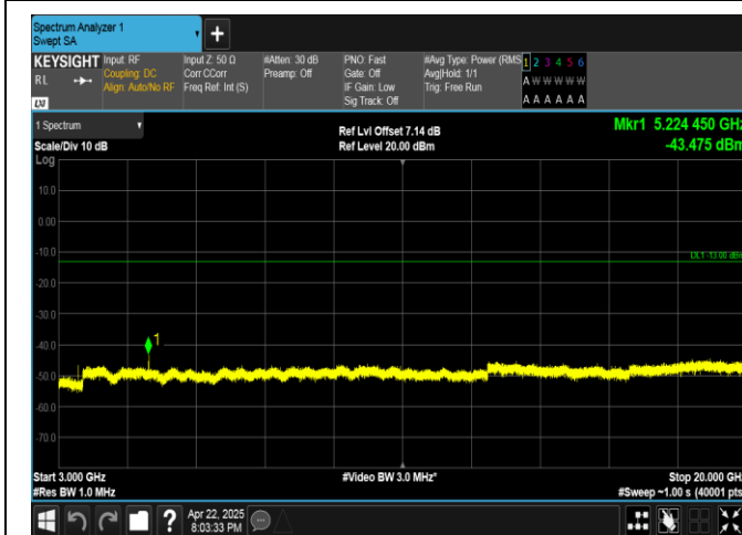
Band4-20MHz-QPSK-20175-1RB#99-3000~20000-PASS
