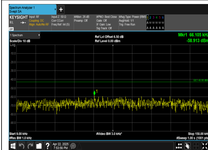
Band4-20MHz-QPSK-20050-1RB#0-0.009~0.15-PASS
