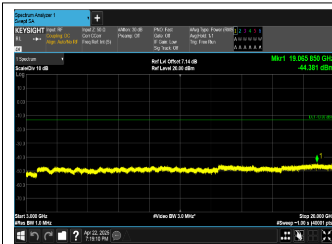
Band4-15MHz-16QAM-20175-75RB#0-3000~20000-PASS
