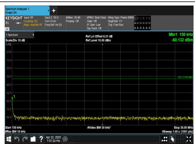
Band4-20MHz-16QAM-20050-1RB#99-0.15~30-PASS
