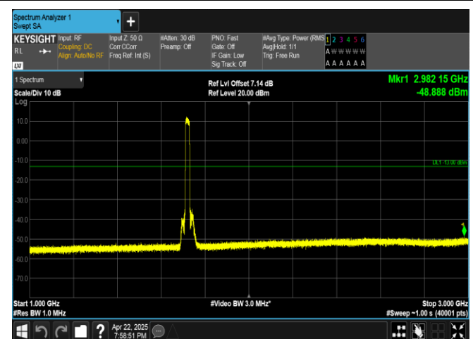
Band4-20MHz-QPSK-20050-100RB#0-1000~3000-PASS
