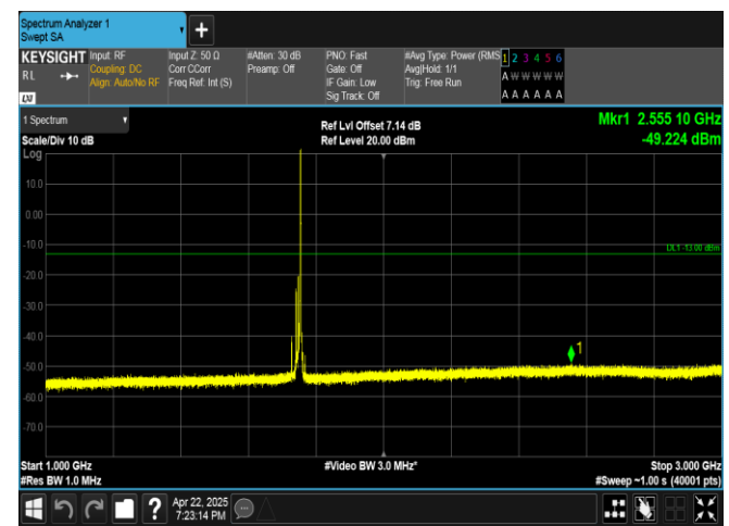
Band4-15MHz-16QAM-20325-1RB#74-1000~3000-PASS
