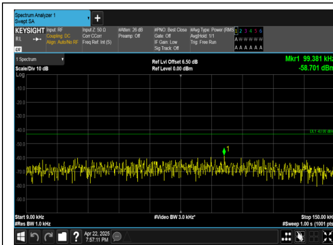
Band4-20MHz-16QAM-20050-1RB#99-0.009~0.15-PASS
