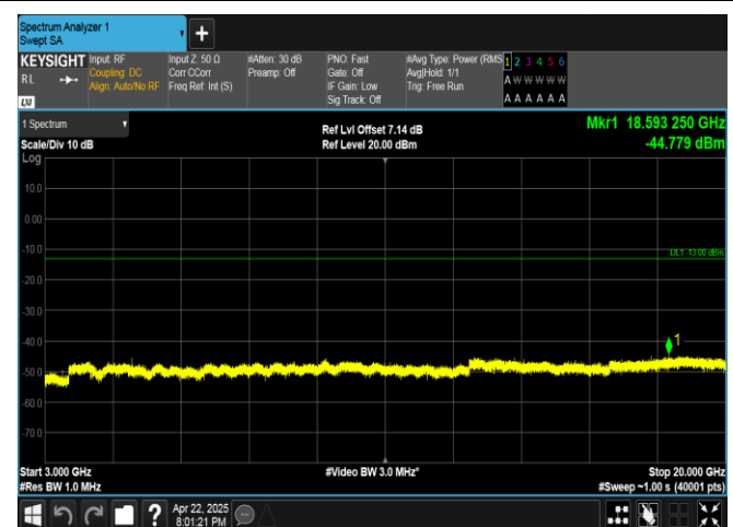
Band4-20MHz-QPSK-20175-1RB#0-3000~20000-PASS
