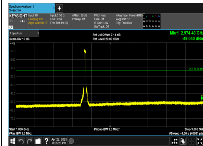
Band4-20MHz-QPSK-20175-100RB#0-1000~3000-PASS
