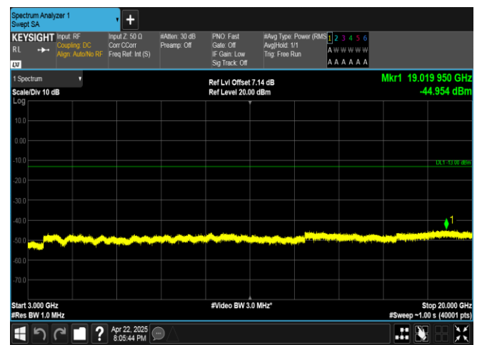
Band4-20MHz-QPSK-20175-100RB#0-3000~20000-PASS
