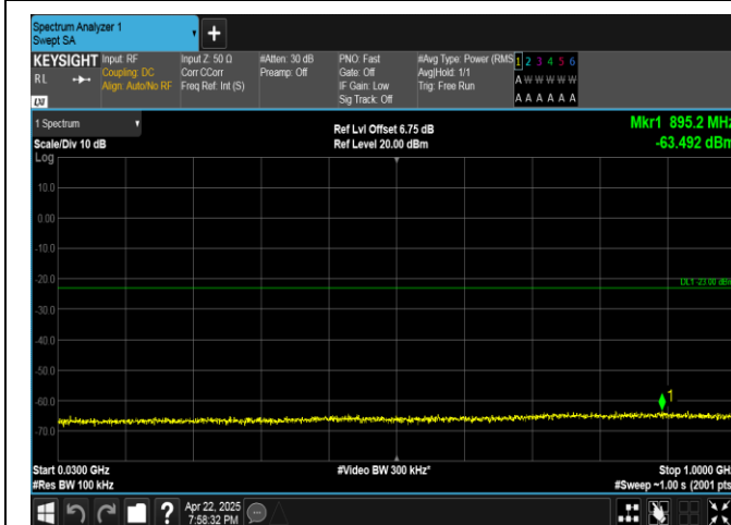
Band4-20MHz-QPSK-20050-100RB#0-30~1000-PASS
