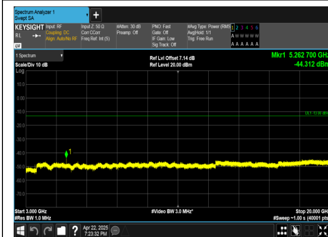
Band4-15MHz-16QAM-20325-1RB#74-3000~20000-PASS
