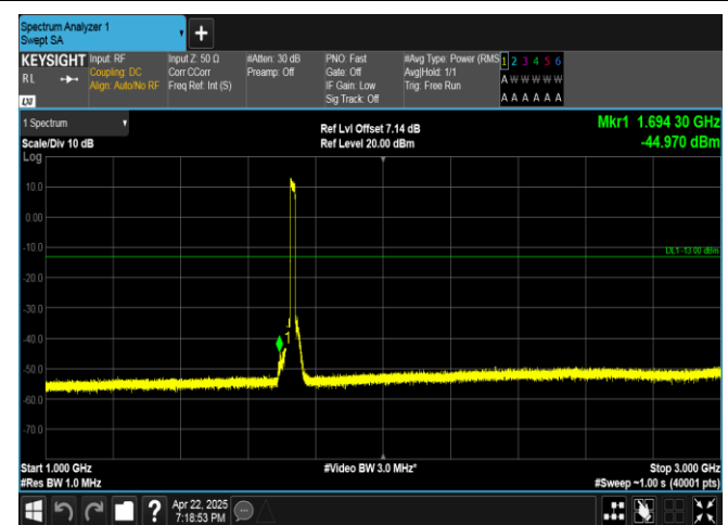
Band4-15MHz-16QAM-20175-75RB#0-1000~3000-PASS
