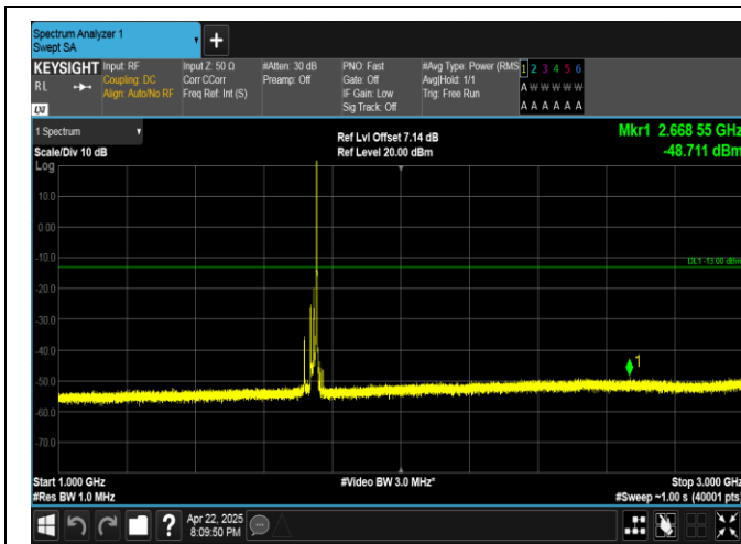
Band4-20MHz-QPSK-20300-1RB#99-1000~3000-PASS
