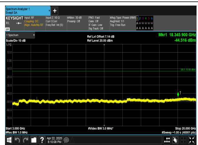
Band4-20MHz-QPSK-20300-1RB#99-3000~20000-PASS
