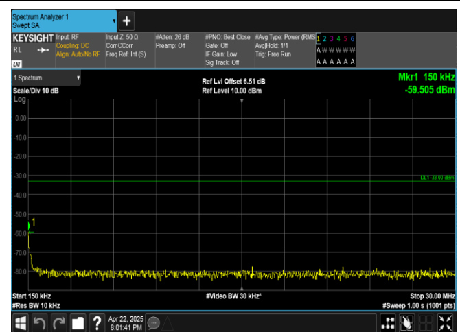
Band4-20MHz-16QAM-20175-1RB#0-0.15~30-PASS
