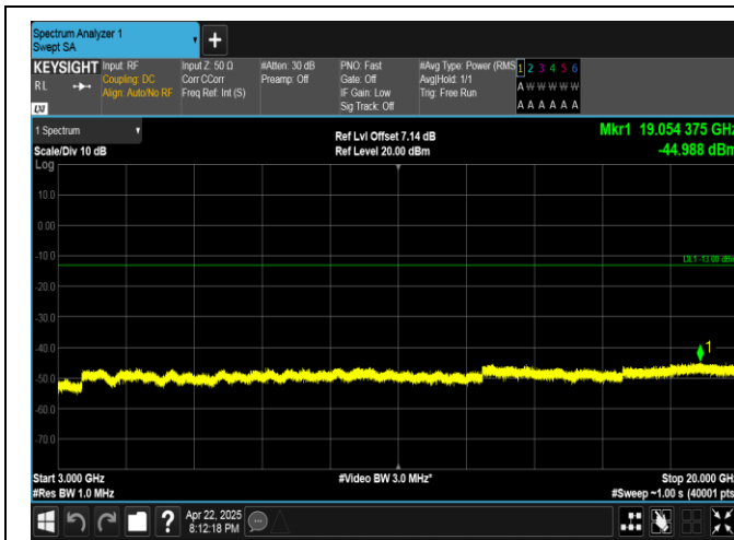
Band4-20MHz-QPSK-20300-100RB#0-3000~20000-PASS
