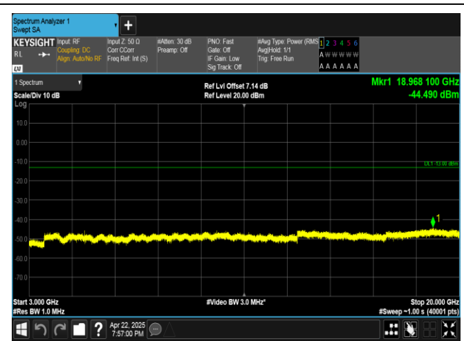
Band4-20MHz-QPSK-20050-1RB#99-3000~20000-PASS
