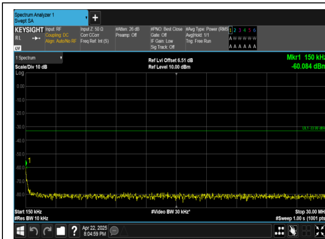
Band4-20MHz-QPSK-20175-100RB#0-0.15~30-PASS
