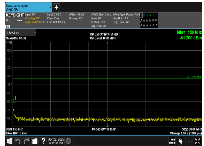
Band4-20MHz-QPSK-20300-100RB#0-0.15~30-PASS
