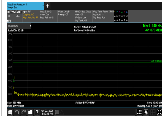
Band4-20MHz-QPSK-20175-1RB#0-0.15~30-PASS
