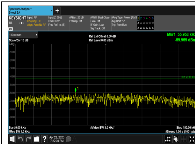
Band4-15MHz-16QAM-20325-1RB#74-0.009~0.15-PASS
