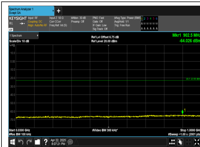
Band4-20MHz-QPSK-20300-1RB#0-30~1000-PASS
