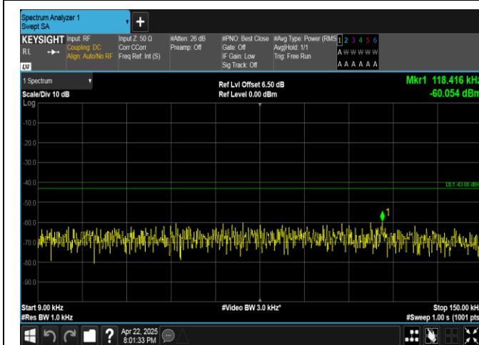
Band4-20MHz-16QAM-20175-1RB#0-0.009~0.15-PASS
