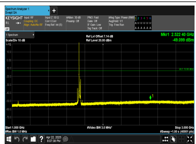
Band4-20MHz-QPSK-20300-1RB#0-1000~3000-PASS
