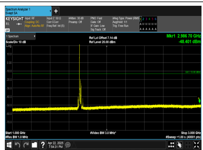
Band4-20MHz-QPSK-20050-1RB#0-1000~3000-PASS
