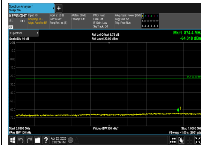
Band4-20MHz-QPSK-20175-1RB#99-30~1000-PASS
