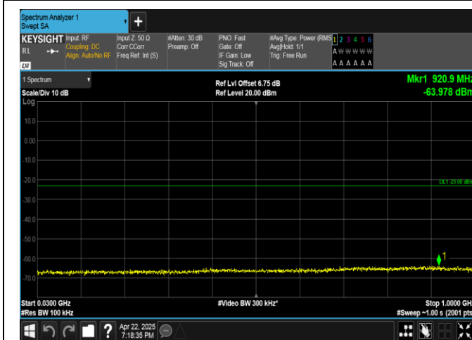
Band4-15MHz-16QAM-20175-75RB#0-30~1000-PASS
