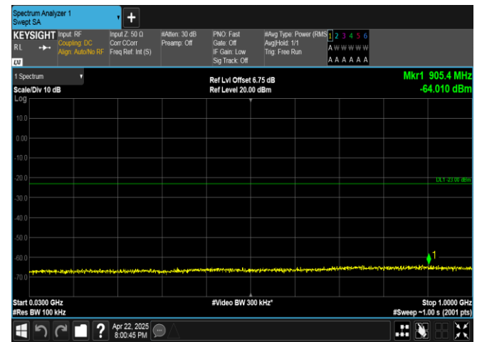
Band4-20MHz-QPSK-20175-1RB#0-30~1000-PASS
