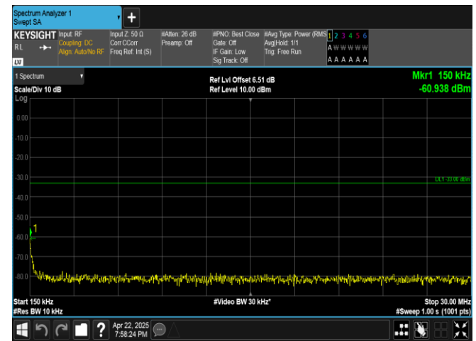
Band4-20MHz-QPSK-20050-100RB#0-0.15~30-PASS
