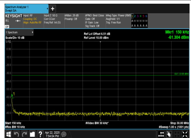
Band4-20MHz-QPSK-20050-1RB#0-0.15~30-PASS
