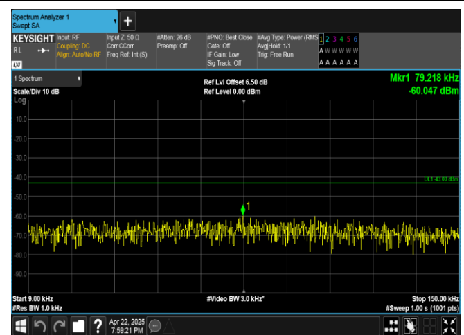
Band4-20MHz-16QAM-20050-100RB#0-0.009~0.15-PASS
