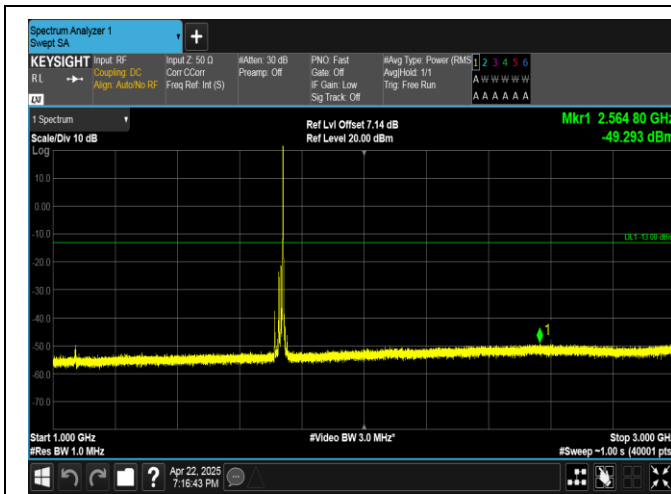
Band4-15MHz-16QAM-20175-1RB#74-1000~3000-PASS
