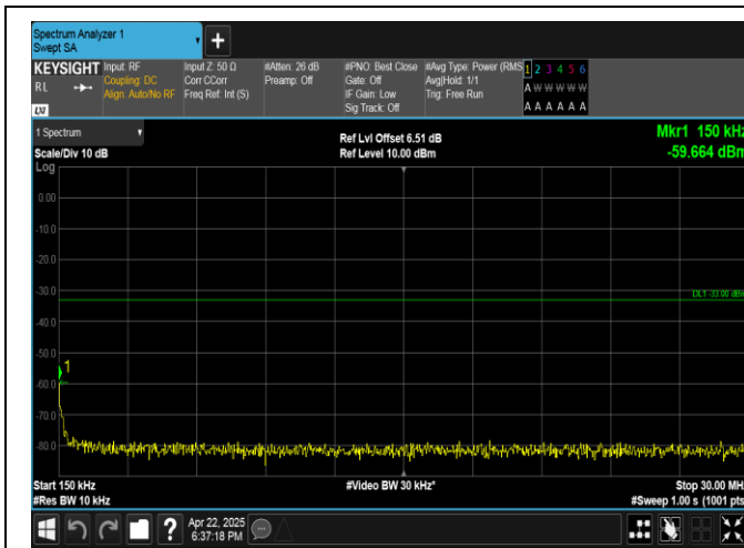
Band4-10MHz-16QAM-20350-50RB#0-0.15~30-PASS
