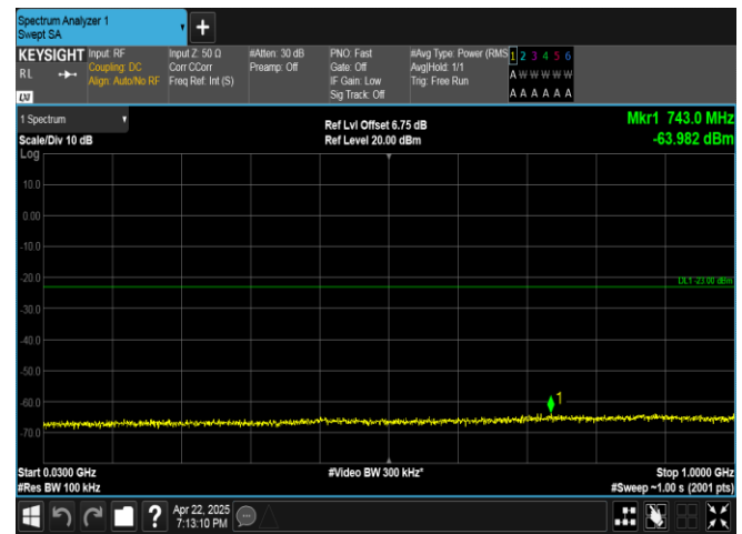
Band4-15MHz-QPSK-20175-1RB#0-30~1000-PASS
