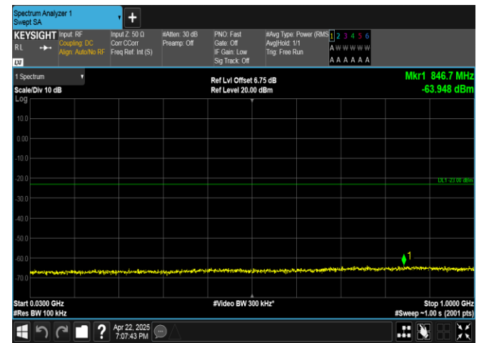
Band4-15MHz-16QAM-20025-1RB#0-30~1000-PASS
