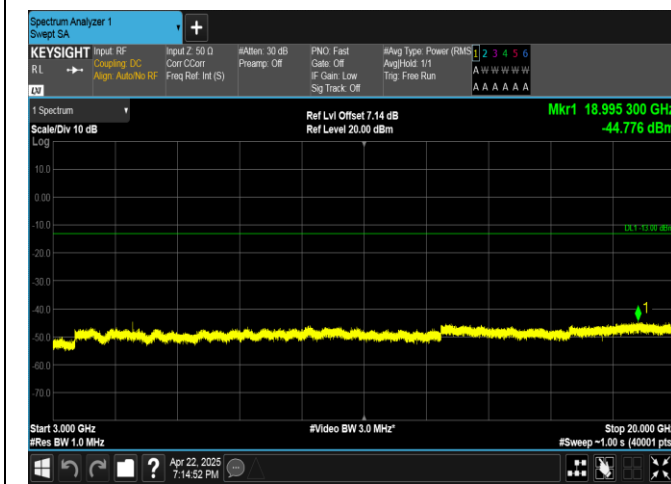
Band4-15MHz-16QAM-20175-1RB#0-3000~20000-PASS
