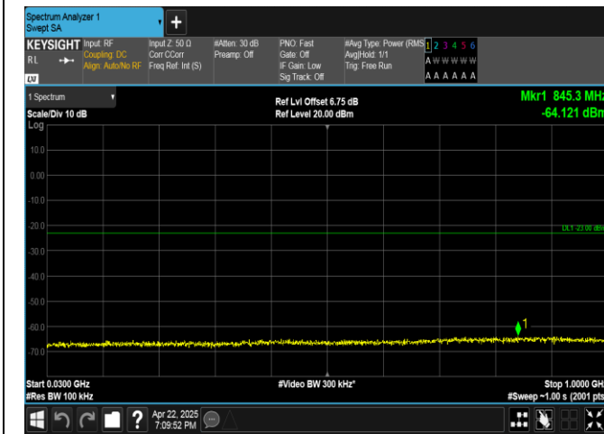
Band4-15MHz-16QAM-20025-1RB#74-30~1000-PASS
