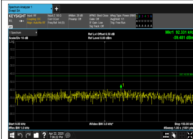
Band4-15MHz-QPSK-20025-1RB#0-0.009~0.15-PASS
