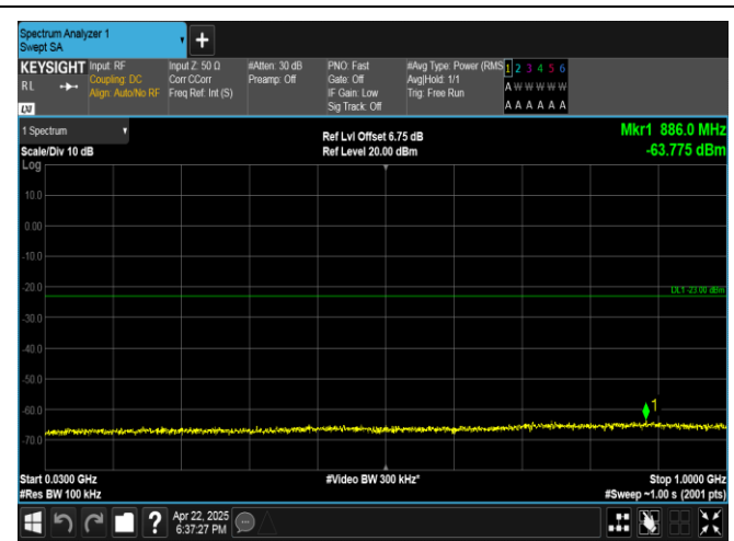
Band4-10MHz-16QAM-20350-50RB#0-30~1000-PASS
