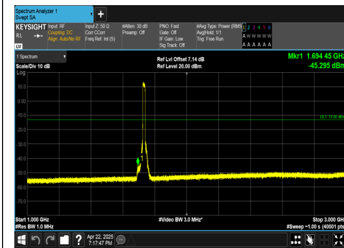
Band4-15MHz-QPSK-20175-75RB#0-1000~3000-PASS
