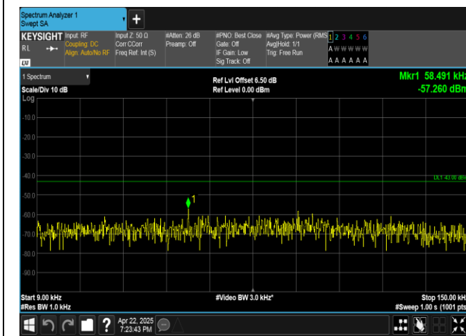
Band4-15MHz-QPSK-20325-75RB#0-0.009~0.15-PASS
