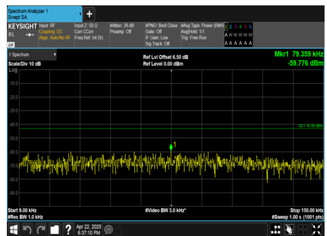
Band4-10MHz-16QAM-20350-50RB#0-0.009~0.15-PASS
