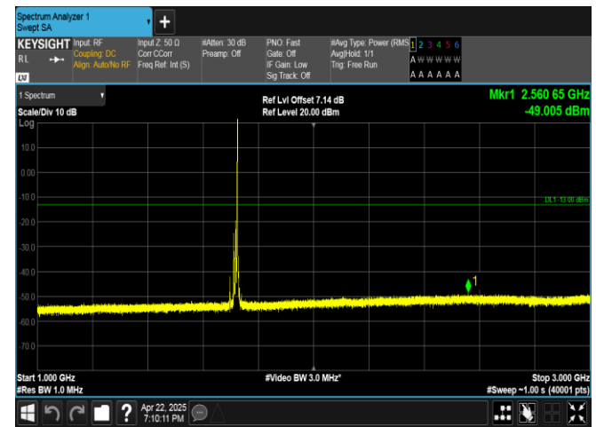
Band4-15MHz-16QAM-20025-1RB#74-1000~3000-PASS
