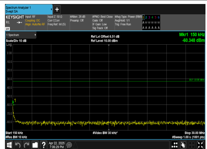
Band4-15MHz-QPSK-20025-1RB#0-0.15~30-PASS
