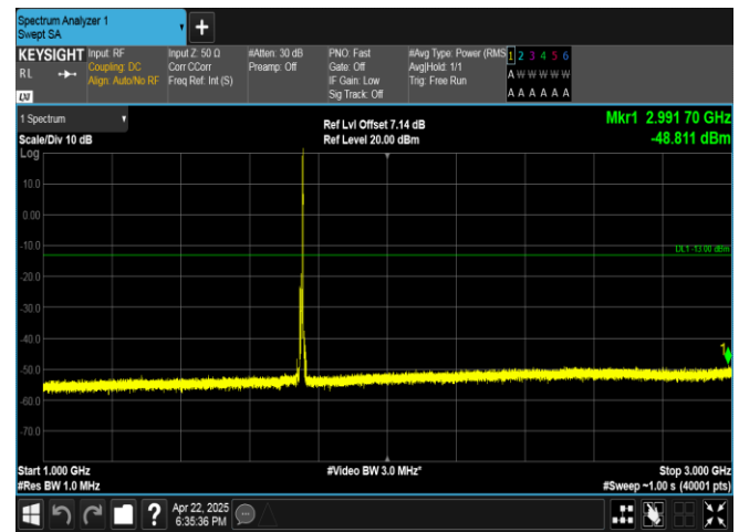
Band4-10MHz-16QAM-20350-1RB#49-1000~3000-PASS
