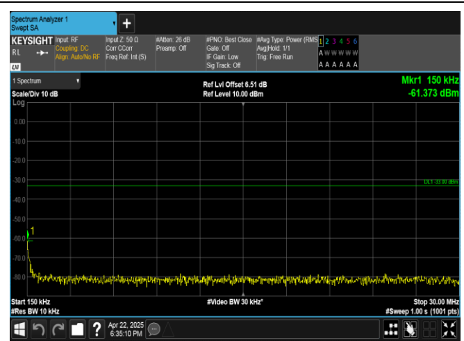
Band4-10MHz-16QAM-20350-1RB#49-0.15~30-PASS
