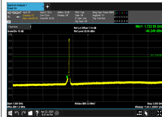
Band4-10MHz-16QAM-20350-50RB#0-1000~3000-PASS
