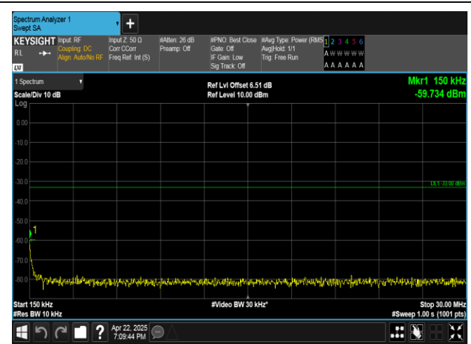
Band4-15MHz-16QAM-20025-1RB#74-0.15~30-PASS
