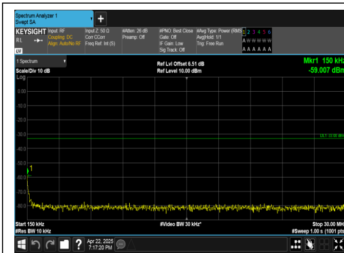
Band4-15MHz-QPSK-20175-75RB#0-0.15~30-PASS
