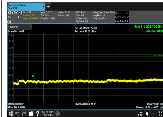
Band4-15MHz-QPSK-20325-1RB#0-3000~20000-PASS
