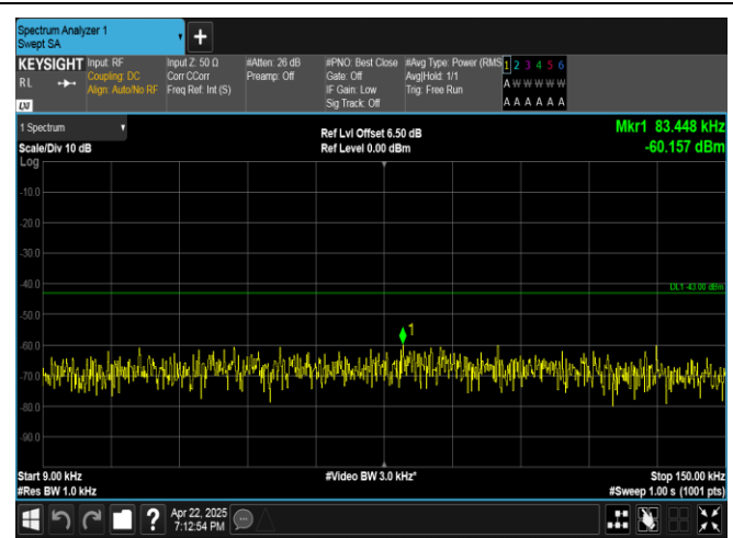
Band4-15MHz-QPSK-20175-1RB#0-0.009~0.15-PASS
