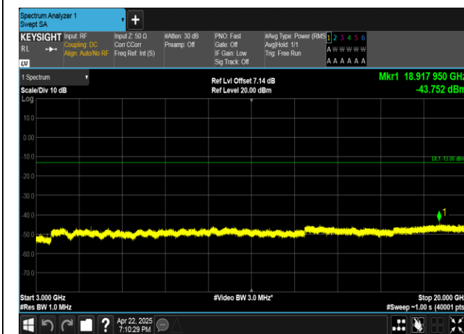
Band4-15MHz-16QAM-20025-1RB#74-3000~20000-PASS
