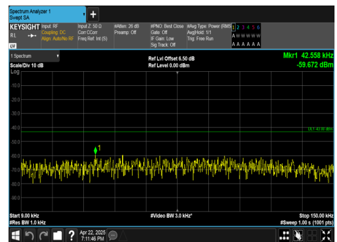
Band4-15MHz-16QAM-20025-75RB#0-0.009~0.15-PASS
