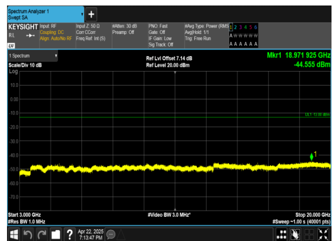
Band4-15MHz-QPSK-20175-1RB#0-3000~20000-PASS
