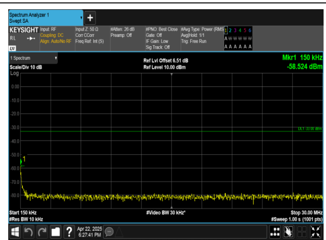
Band4-10MHz-QPSK-20175-1RB#49-0.15~30-PASS
