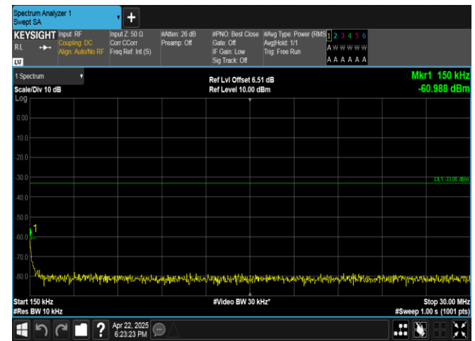
Band4-10MHz-QPSK-20000-50RB#0-0.15~30-PASS
