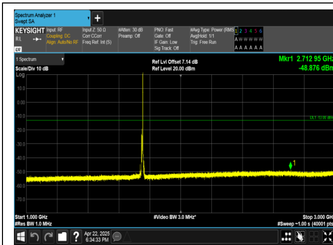
Band4-10MHz-QPSK-20350-1RB#49-1000~3000-PASS
