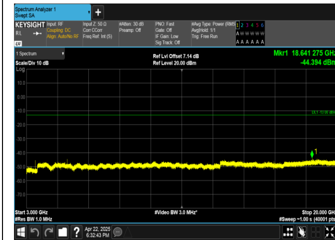
Band4-10MHz-QPSK-20350-1RB#0-3000~20000-PASS
