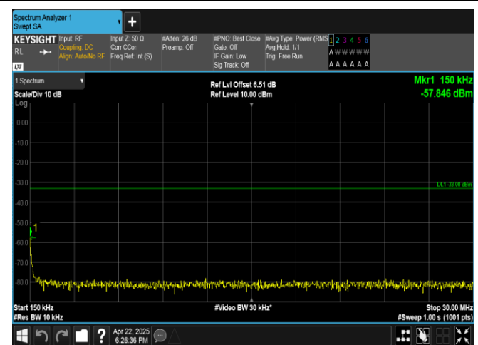
Band4-10MHz-16QAM-20175-1RB#0-0.15~30-PASS
