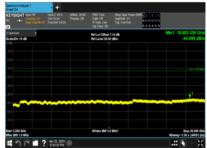
Band4-10MHz-QPSK-20175-50RB#0-3000~20000-PASS
