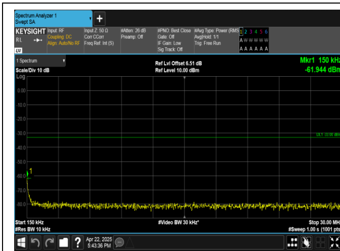
Band4-5MHz-16QAM-20375-25RB#0-0.15~30-PASS
