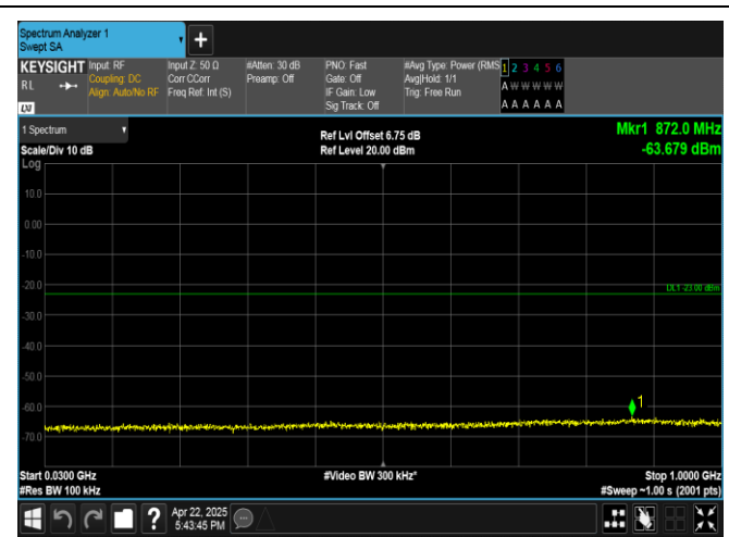
Band4-5MHz-16QAM-20375-25RB#0-30~1000-PASS
