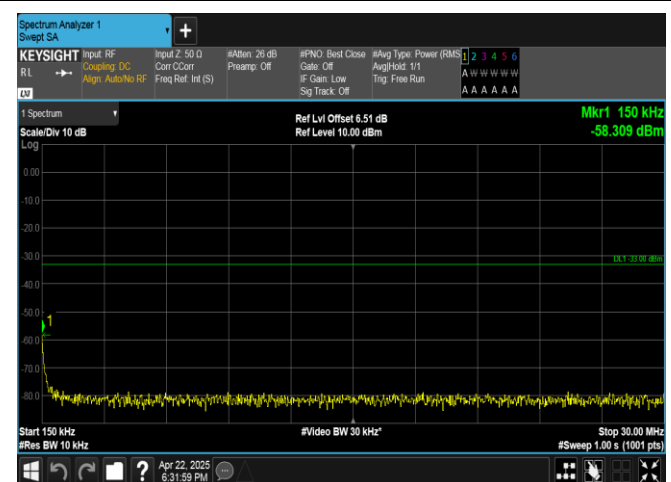
Band4-10MHz-QPSK-20350-1RB#0-0.15~30-PASS
