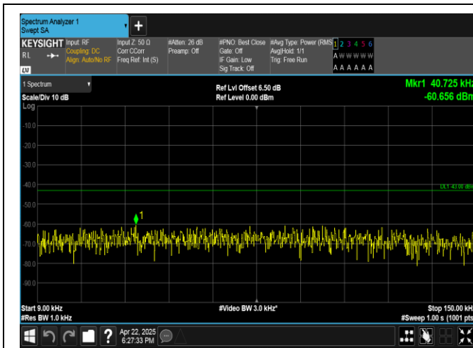
Band4-10MHz-QPSK-20175-1RB#49-0.009~0.15-PASS
