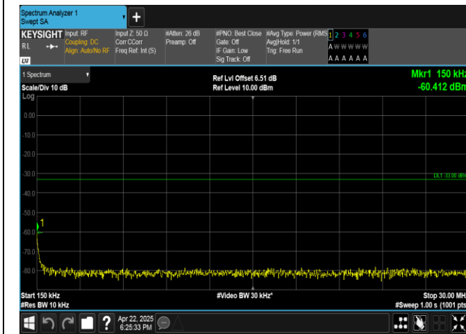
Band4-10MHz-QPSK-20175-1RB#0-0.15~30-PASS
