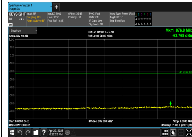
Band4-10MHz-16QAM-20000-1RB#49-30~1000-PASS
