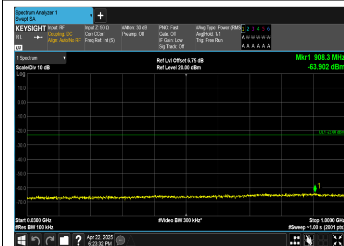
Band4-10MHz-QPSK-20000-50RB#0-30~1000-PASS
