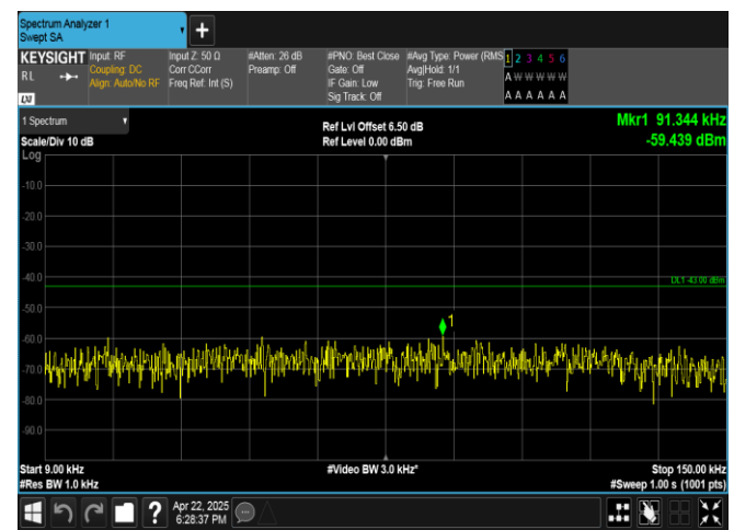
Band4-10MHz-16QAM-20175-1RB#49-0.009~0.15-PASS
