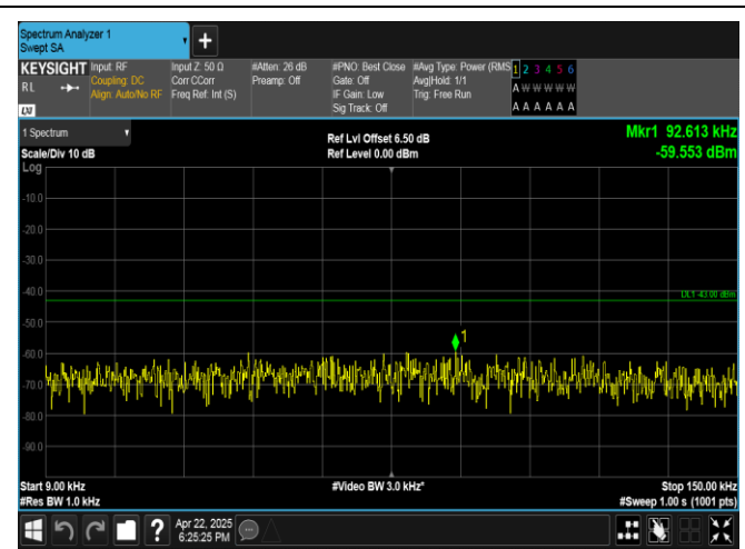
Band4-10MHz-QPSK-20175-1RB#0-0.009~0.15-PASS
