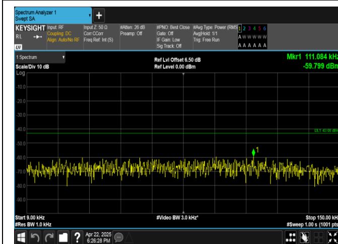
Band4-10MHz-16QAM-20175-1RB#0-0.009~0.15-PASS
