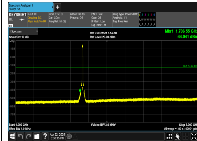
Band4-10MHz-QPSK-20175-50RB#0-1000~3000-PASS
