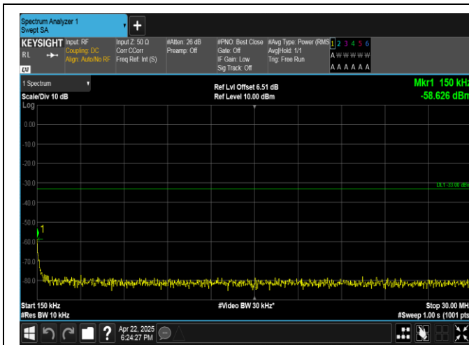
Band4-10MHz-16QAM-20000-50RB#0-0.15~30-PASS
