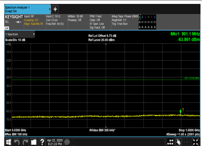
Band4-10MHz-QPSK-20000-1RB#49-30~1000-PASS
