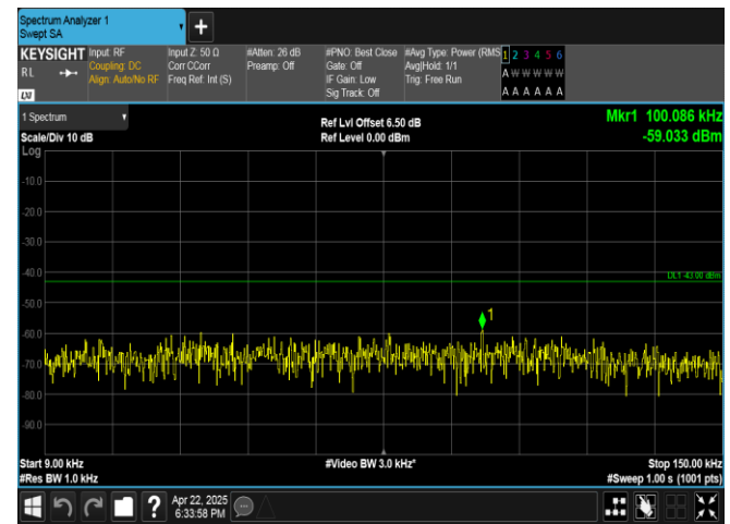
Band4-10MHz-QPSK-20350-1RB#49-0.009~0.15-PASS
