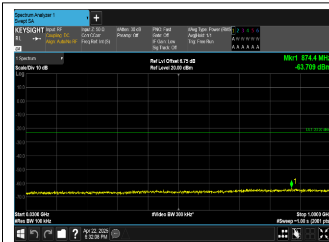
Band4-10MHz-QPSK-20350-1RB#0-30~1000-PASS
