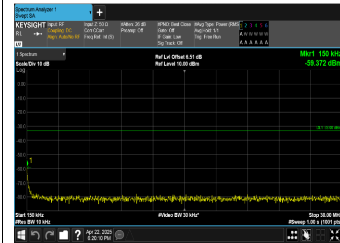
Band4-10MHz-16QAM-20000-1RB#0-0.15~30-PASS
