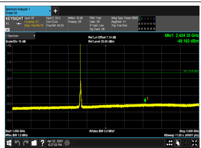
Band4-10MHz-16QAM-20175-1RB#0-1000~3000-PASS
