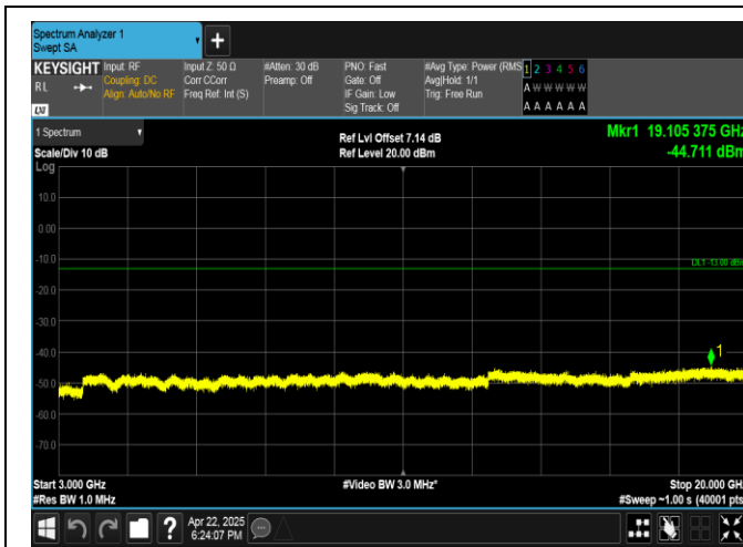
Band4-10MHz-QPSK-20000-50RB#0-3000~20000-PASS
