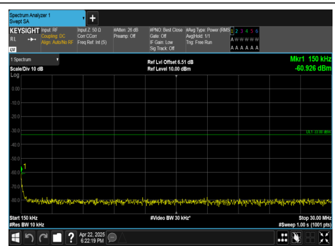
Band4-10MHz-16QAM-20000-1RB#49-0.15~30-PASS
