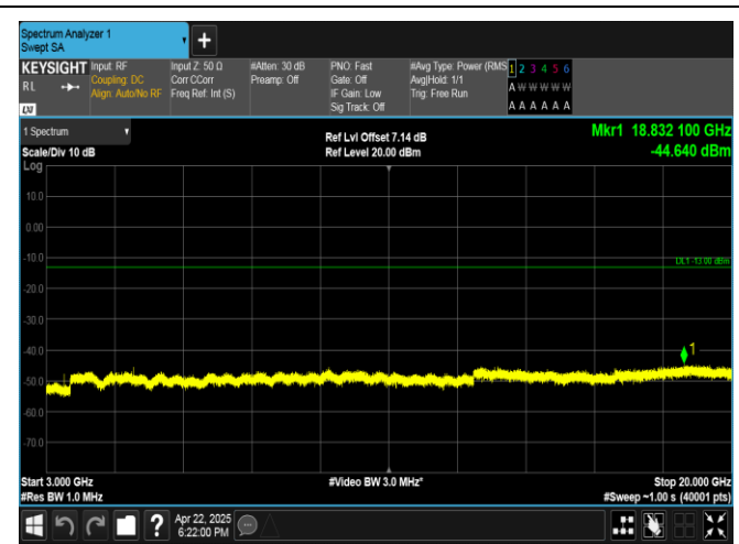
Band4-10MHz-QPSK-20000-1RB#49-3000~20000-PASS
