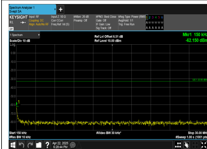
Band4-10MHz-16QAM-20175-1RB#49-0.15~30-PASS
