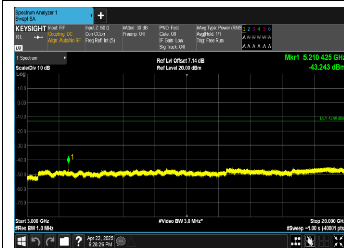
Band4-10MHz-QPSK-20175-1RB#49-3000~20000-PASS
