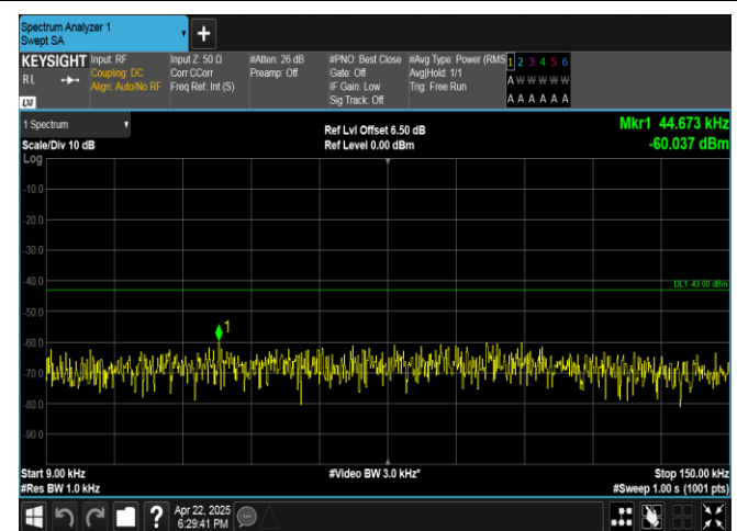
Band4-10MHz-QPSK-20175-50RB#0-0.009~0.15-PASS
