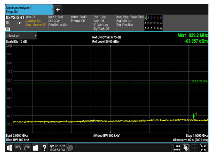
Band4-10MHz-16QAM-20175-1RB#49-30~1000-PASS
