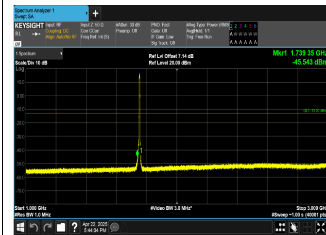
Band4-5MHz-16QAM-20375-25RB#0-1000~3000-PASS
