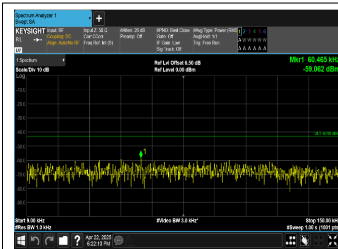
Band4-10MHz-16QAM-20000-1RB#49-0.009~0.15-PASS
