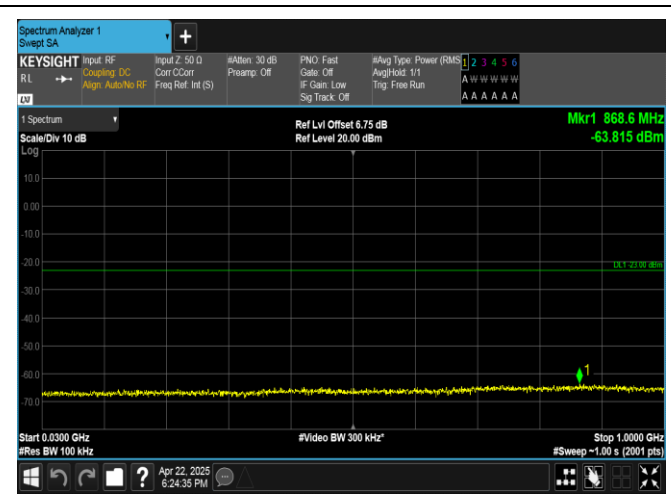
Band4-10MHz-16QAM-20000-50RB#0-30~1000-PASS
