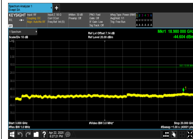
Band4-10MHz-16QAM-20175-1RB#0-3000~20000-PASS
