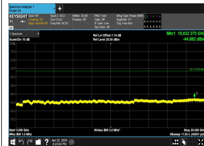
Band4-10MHz-16QAM-20000-1RB#49-3000~20000-PASS
