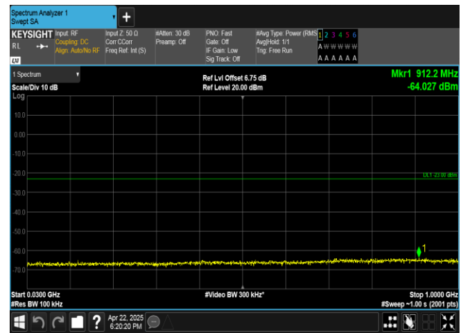
Band4-10MHz-16QAM-20000-1RB#0-30~1000-PASS
