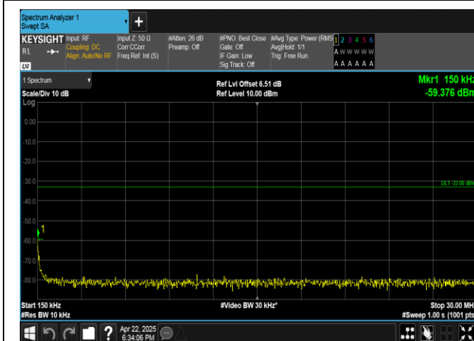
Band4-10MHz-QPSK-20350-1RB#49-0.15~30-PASS
