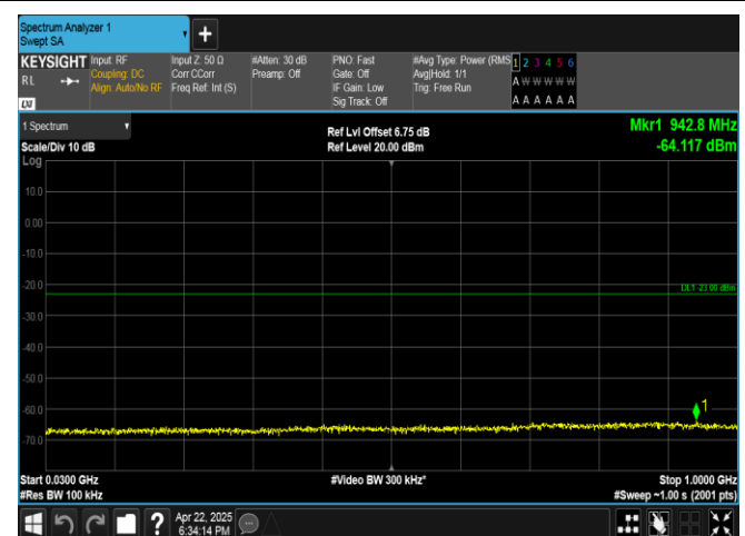
Band4-10MHz-QPSK-20350-1RB#49-30~1000-PASS
