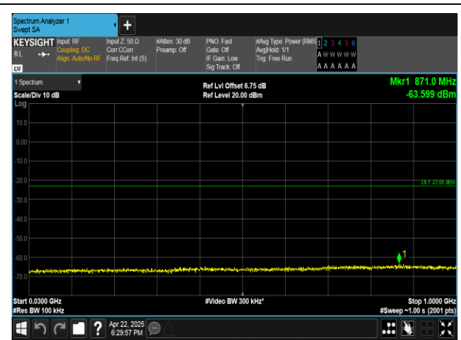
Band4-10MHz-QPSK-20175-50RB#0-30~1000-PASS
