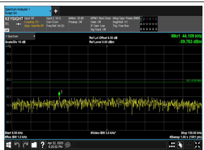
Band4-10MHz-16QAM-20000-1RB#0-0.009~0.15-PASS
