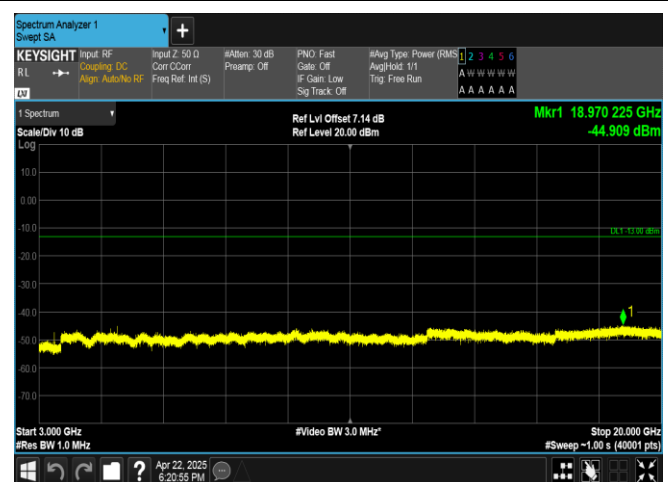
Band4-10MHz-16QAM-20000-1RB#0-3000~20000-PASS
