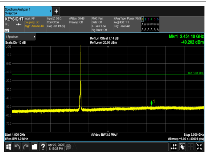
Band4-10MHz-QPSK-20000-1RB#0-1000~3000-PASS
