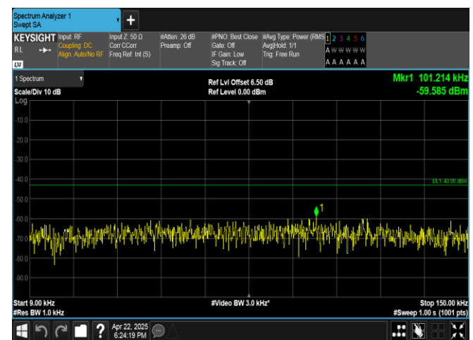
Band4-10MHz-16QAM-20000-50RB#0-0.009~0.15-PASS
