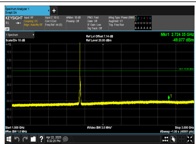
Band4-10MHz-QPSK-20350-1RB#0-1000~3000-PASS
