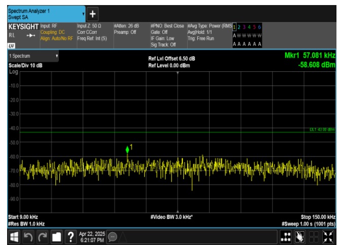
Band4-10MHz-QPSK-20000-1RB#49-0.009~0.15-PASS
