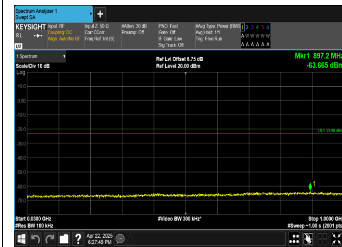
Band4-10MHz-QPSK-20175-1RB#49-30~1000-PASS
