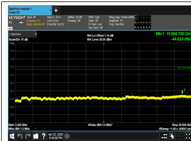
Band4-10MHz-QPSK-20350-50RB#0-3000~20000-PASS
