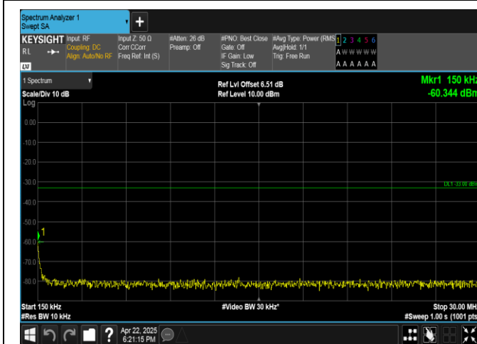
Band4-10MHz-QPSK-20000-1RB#49-0.15~30-PASS
