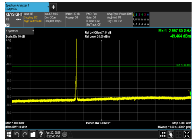
Band4-10MHz-16QAM-20000-1RB#49-1000~3000-PASS
