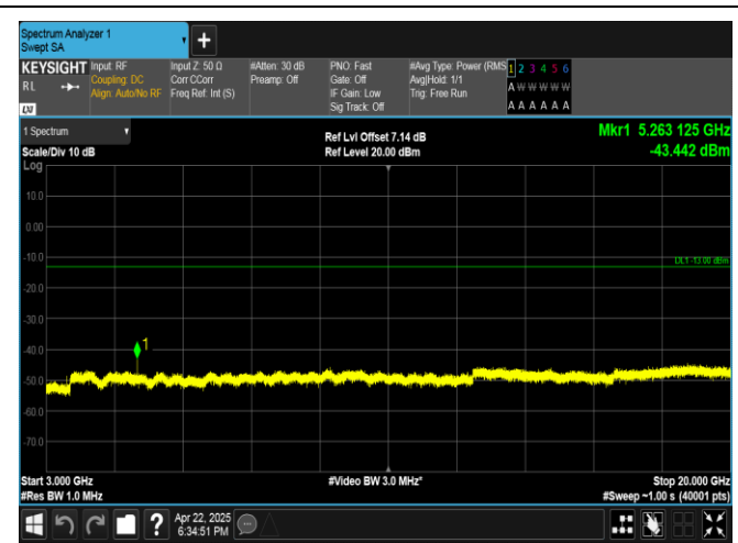
Band4-10MHz-QPSK-20350-1RB#49-3000~20000-PASS
