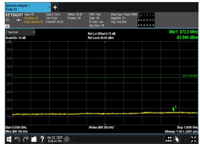
Band4-10MHz-QPSK-20175-1RB#0-30~1000-PASS
