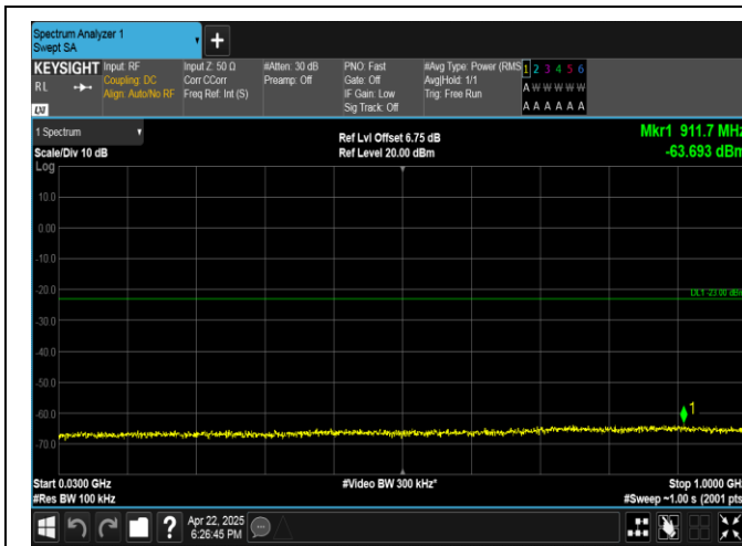
Band4-10MHz-16QAM-20175-1RB#0-30~1000-PASS
