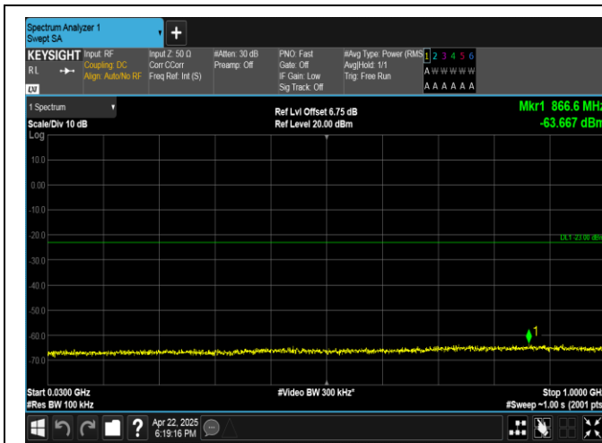
Band4-10MHz-QPSK-20000-1RB#0-30~1000-PASS
