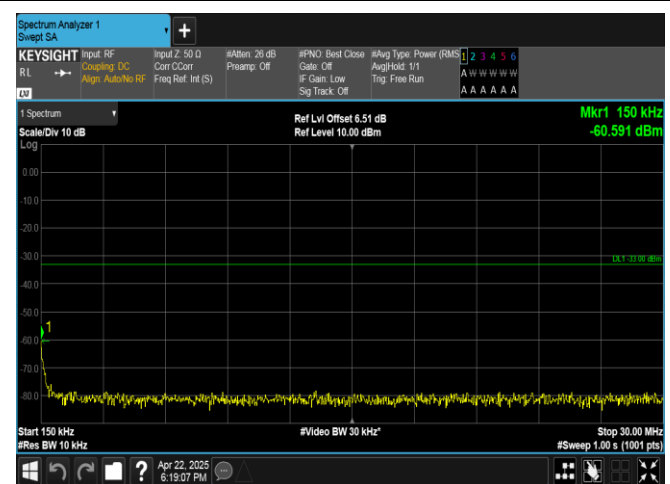
Band4-10MHz-QPSK-20000-1RB#0-0.15~30-PASS
