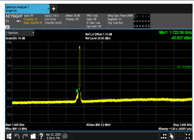
Band4-10MHz-QPSK-20350-50RB#0-1000~3000-PASS
