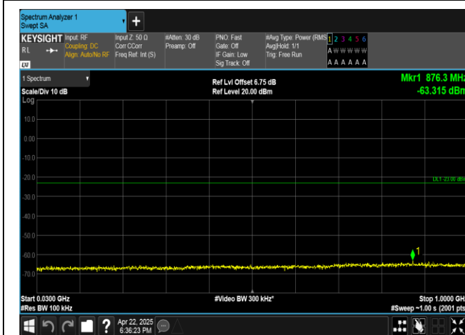
Band4-10MHz-QPSK-20350-50RB#0-30~1000-PASS
