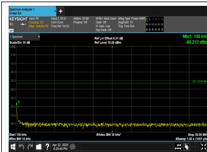
Band4-10MHz-QPSK-20175-50RB#0-0.15~30-PASS
