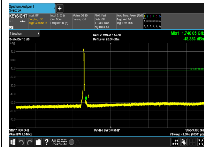
Band4-10MHz-16QAM-20000-50RB#0-1000~3000-PASS
