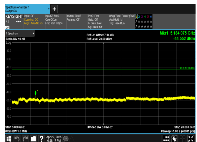
Band4-10MHz-QPSK-20175-1RB#0-3000~20000-PASS
