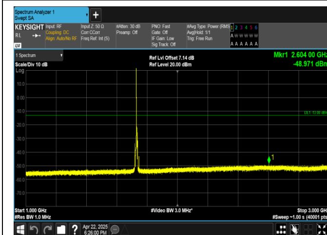
Band4-10MHz-QPSK-20175-1RB#0-1000~3000-PASS
