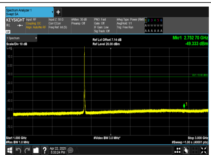
Band4-5MHz-16QAM-20175-1RB#0-1000~3000-PASS
