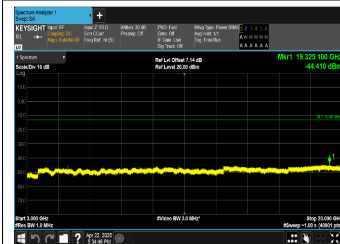
Band4-5MHz-QPSK-20175-1RB#24-3000~20000-PASS
