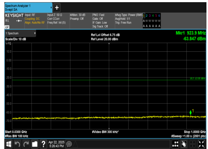
Band4-5MHz-16QAM-19975-1RB#0-30~1000-PASS
