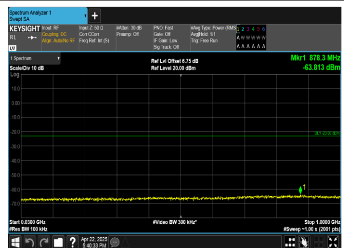
Band4-5MHz-QPSK-20375-1RB#24-30~1000-PASS
