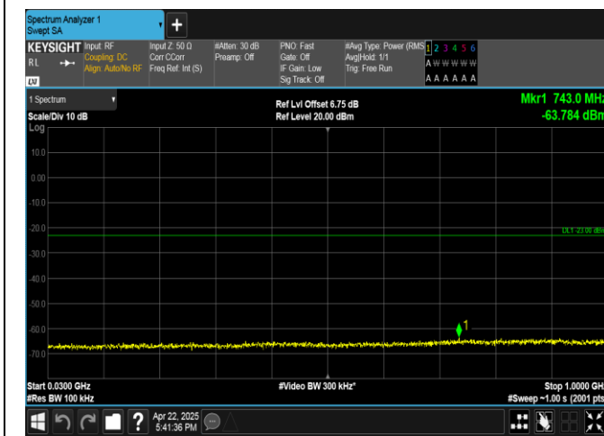
Band4-5MHz-16QAM-20375-1RB#24-30~1000-PASS
