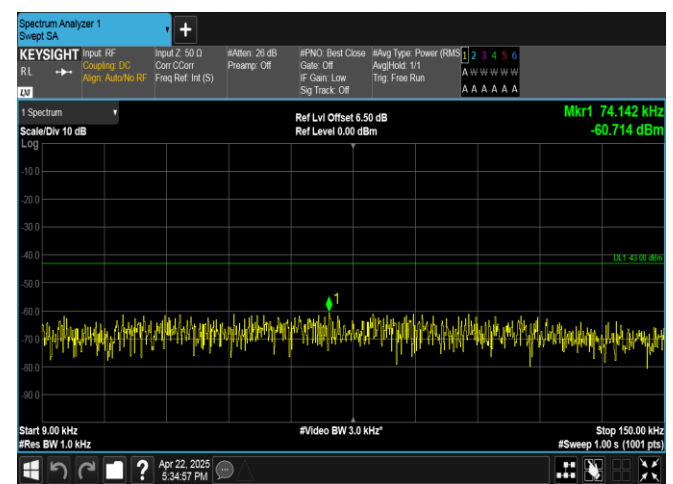
Band4-5MHz-16QAM-20175-1RB#24-0.009~0.15-PASS
