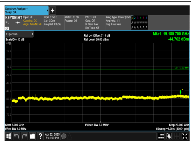
Band4-5MHz-QPSK-20375-1RB#24-3000~20000-PASS
