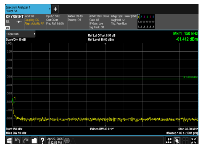
Band4-5MHz-16QAM-20175-1RB#0-0.15~30-PASS
