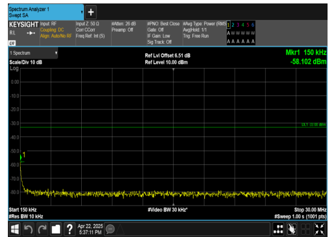
Band4-5MHz-16QAM-20175-25RB#0-0.15~30-PASS
