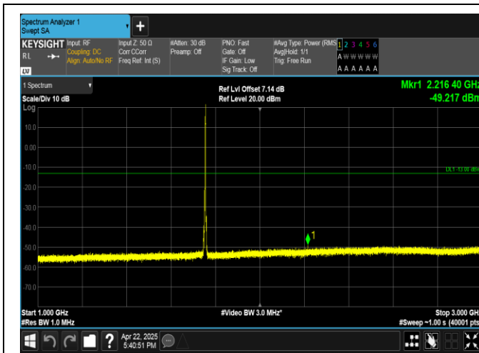
Band4-5MHz-QPSK-20375-1RB#24-1000~3000-PASS
