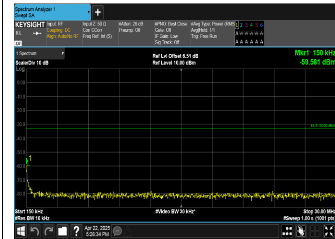
Band4-5MHz-16QAM-19975-1RB#0-0.15~30-PASS
