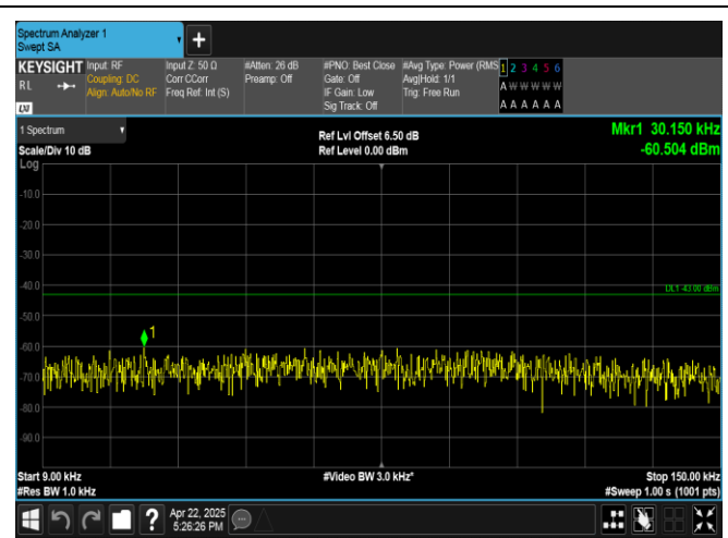
Band4-5MHz-16QAM-19975-1RB#0-0.009~0.15-PASS
