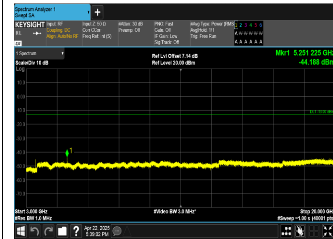
Band4-5MHz-QPSK-20375-1RB#0-3000~20000-PASS
