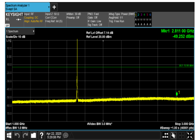
Band4-5MHz-16QAM-19975-1RB#24-1000~3000-PASS
