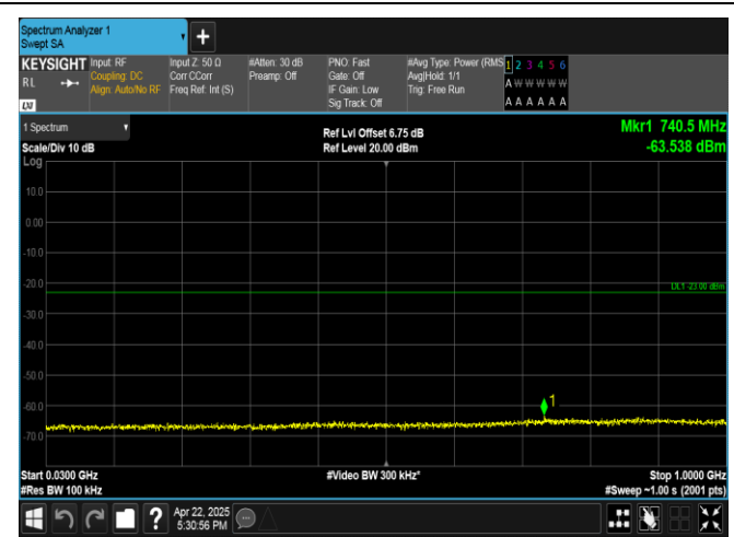
Band4-5MHz-16QAM-19975-25RB#0-30~1000-PASS
