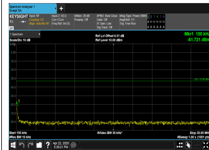
Band4-5MHz-16QAM-20375-1RB#0-0.15~30-PASS
