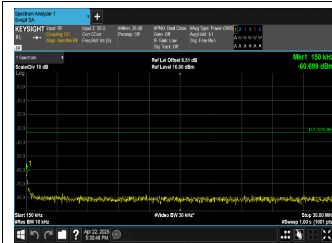
Band4-5MHz-16QAM-19975-25RB#0-0.15~30-PASS
