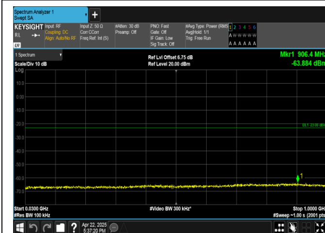
Band4-5MHz-16QAM-20175-25RB#0-30~1000-PASS
