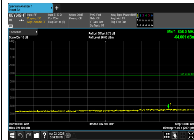
Band4-5MHz-QPSK-20175-1RB#24-30~1000-PASS
