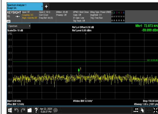
Band4-5MHz-QPSK-19975-25RB#0-0.009~0.15-PASS
