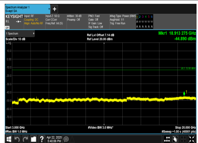
Band4-5MHz-16QAM-20375-1RB#0-3000~20000-PASS
