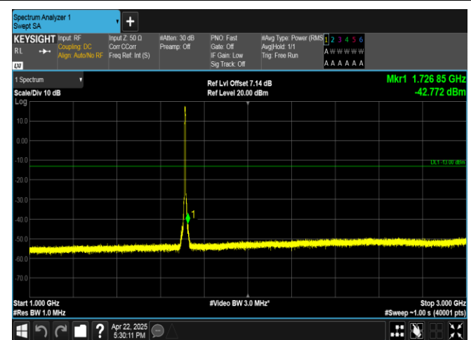
Band4-5MHz-QPSK-19975-25RB#0-1000~3000-PASS
