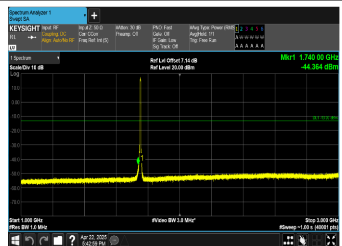
Band4-5MHz-QPSK-20375-25RB#0-1000~3000-PASS
