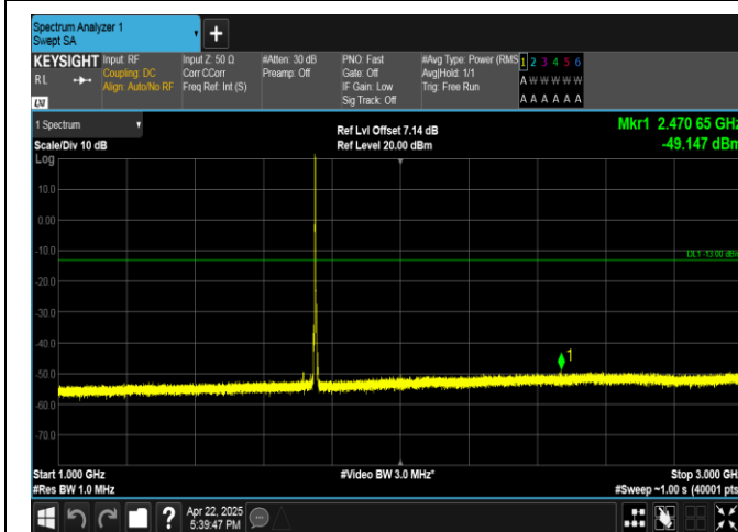
Band4-5MHz-16QAM-20375-1RB#0-1000~3000-PASS
