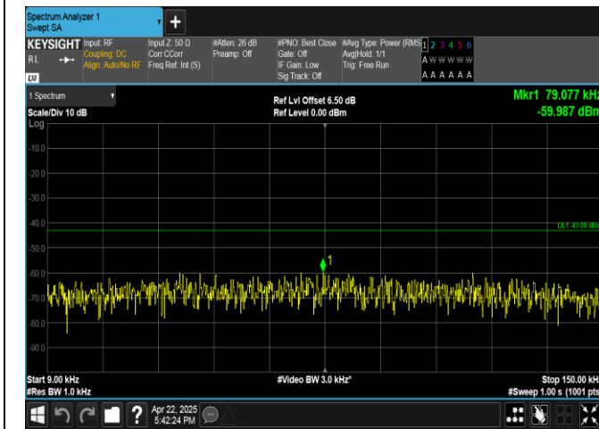
Band4-5MHz-QPSK-20375-25RB#0-0.009~0.15-PASS
