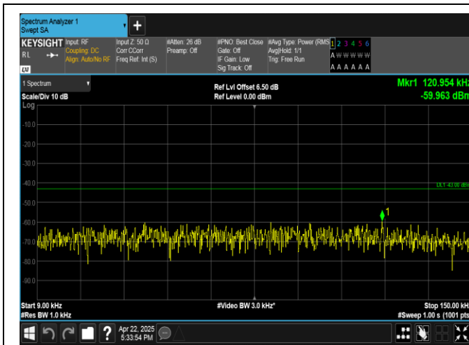
Band4-5MHz-QPSK-20175-1RB#24-0.009~0.15-PASS
