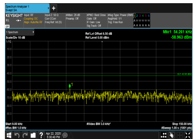
Band4-5MHz-16QAM-19975-25RB#0-0.009~0.15-PASS
