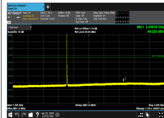
Band4-5MHz-16QAM-19975-1RB#0-1000~3000-PASS
