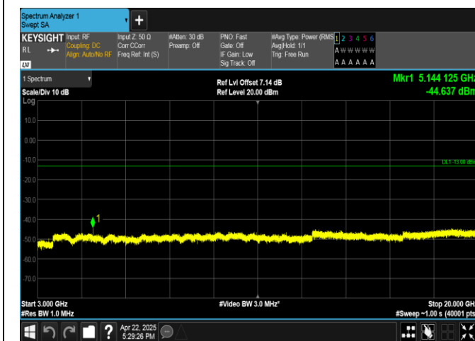
Band4-5MHz-16QAM-19975-1RB#24-3000~20000-PASS
