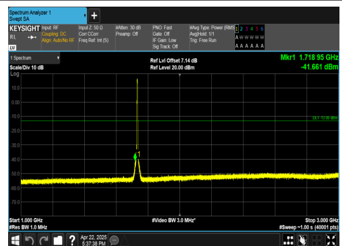
Band4-5MHz-16QAM-20175-25RB#0-1000~3000-PASS
