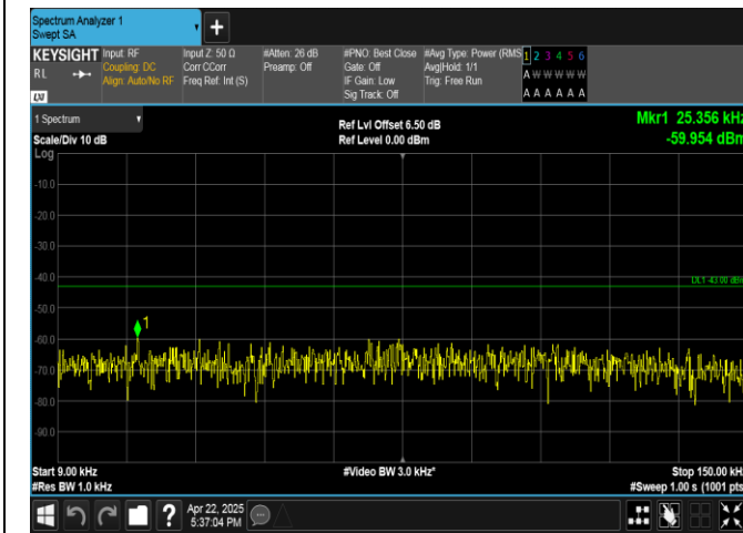
Band4-5MHz-16QAM-20175-25RB#0-0.009~0.15-PASS
