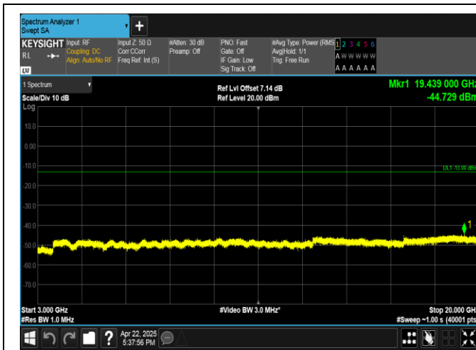
Band4-5MHz-16QAM-20175-25RB#0-3000~20000-PASS
