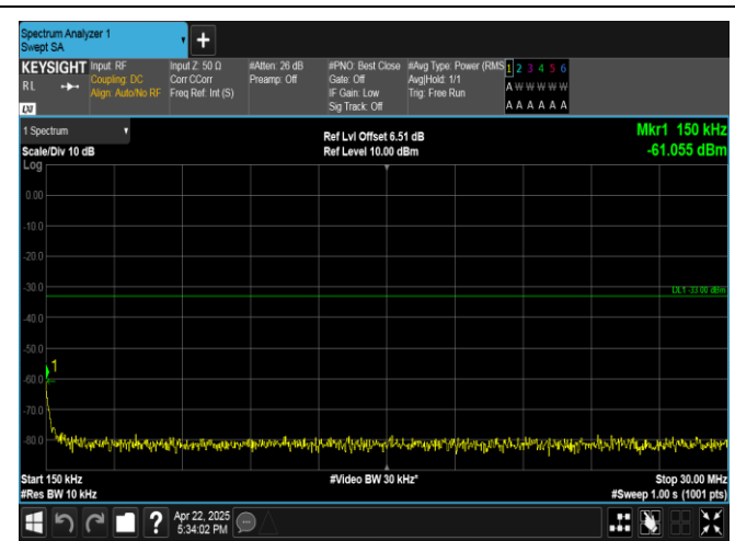
Band4-5MHz-QPSK-20175-1RB#24-0.15~30-PASS
