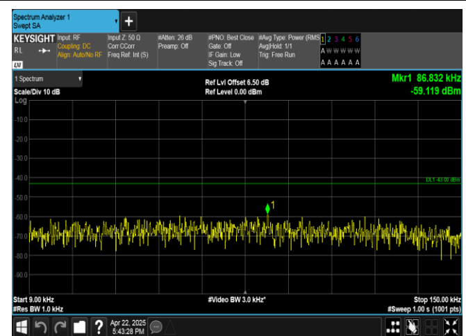
Band4-5MHz-16QAM-20375-25RB#0-0.009~0.15-PASS
