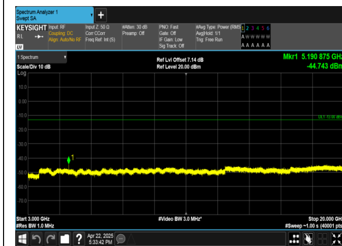
Band4-5MHz-16QAM-20175-1RB#0-3000~20000-PASS
