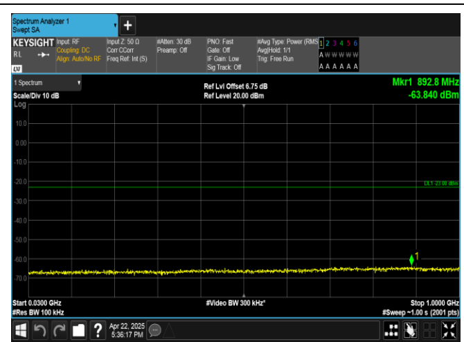
Band4-5MHz-QPSK-20175-25RB#0-30~1000-PASS
