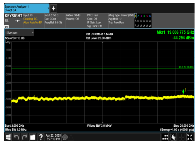
Band4-5MHz-16QAM-19975-1RB#0-3000~20000-PASS
