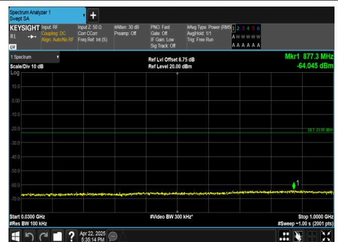
Band4-5MHz-16QAM-20175-1RB#24-30~1000-PASS
