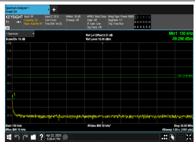
Band4-5MHz-16QAM-19975-1RB#24-0.15~30-PASS
