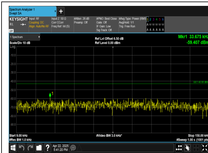
Band4-5MHz-16QAM-20375-1RB#24-0.009~0.15-PASS
