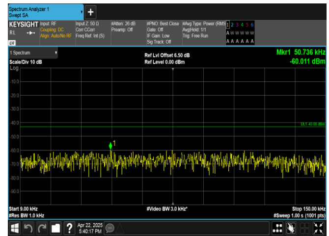
Band4-5MHz-QPSK-20375-1RB#24-0.009~0.15-PASS
