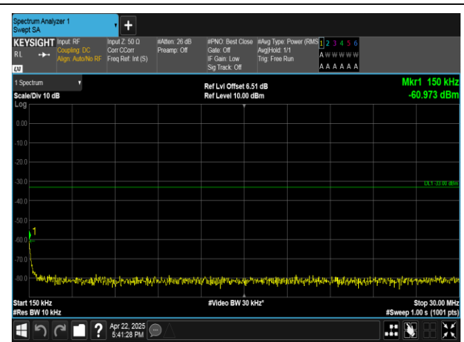
Band4-5MHz-16QAM-20375-1RB#24-0.15~30-PASS
