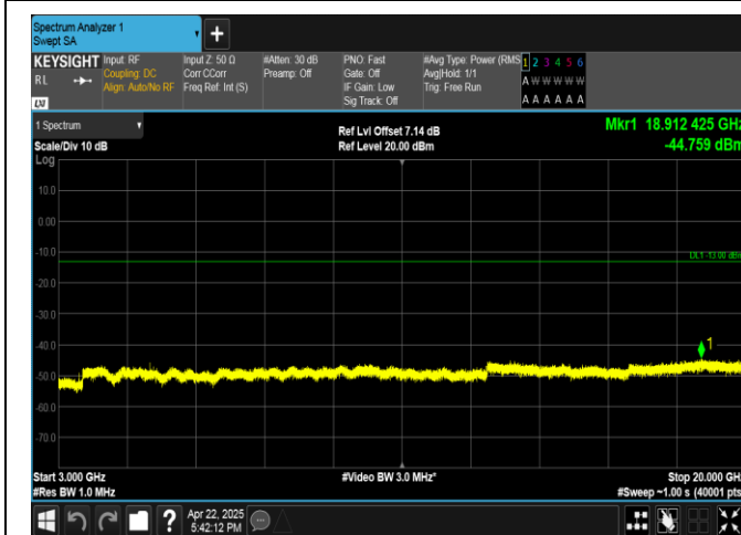
Band4-5MHz-16QAM-20375-1RB#24-3000~20000-PASS
