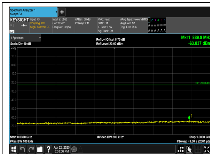
Band4-5MHz-16QAM-20175-1RB#0-30~1000-PASS
