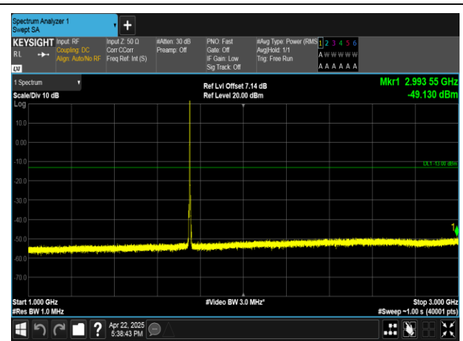
Band4-5MHz-QPSK-20375-1RB#0-1000~3000-PASS
