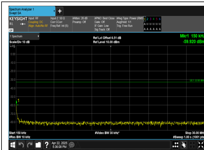
Band4-5MHz-QPSK-20175-25RB#0-0.15~30-PASS
