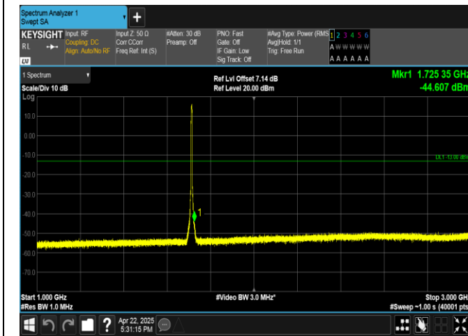
Band4-5MHz-16QAM-19975-25RB#0-1000~3000-PASS
