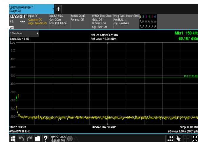
Band4-5MHz-16QAM-20175-1RB#24-0.15~30-PASS
