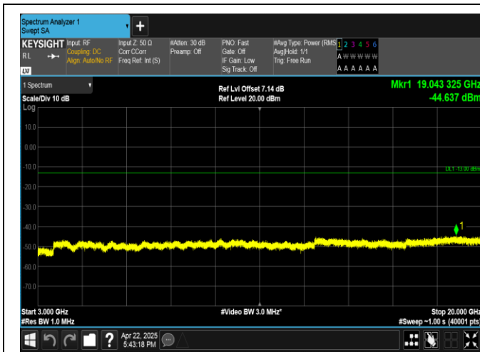
Band4-5MHz-QPSK-20375-25RB#0-3000~20000-PASS
