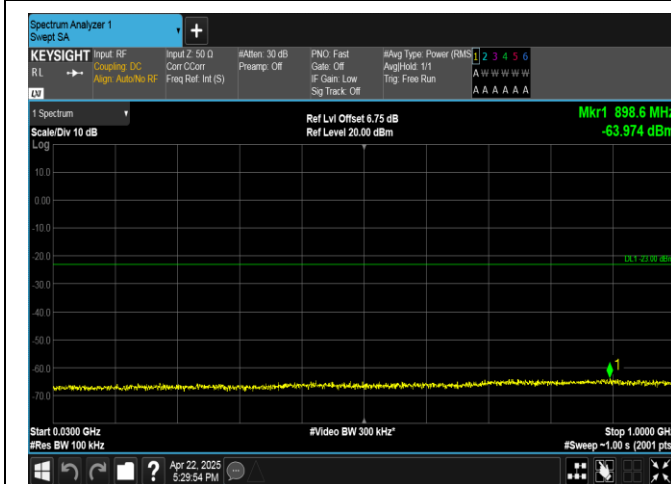
Band4-5MHz-QPSK-19975-25RB#0-30~1000-PASS
