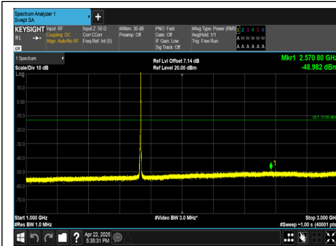
Band4-5MHz-16QAM-20175-1RB#24-1000~3000-PASS
