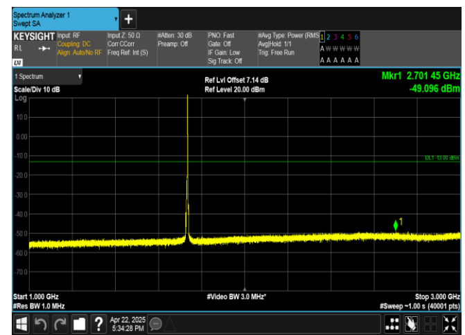
Band4-5MHz-QPSK-20175-1RB#24-1000~3000-PASS
