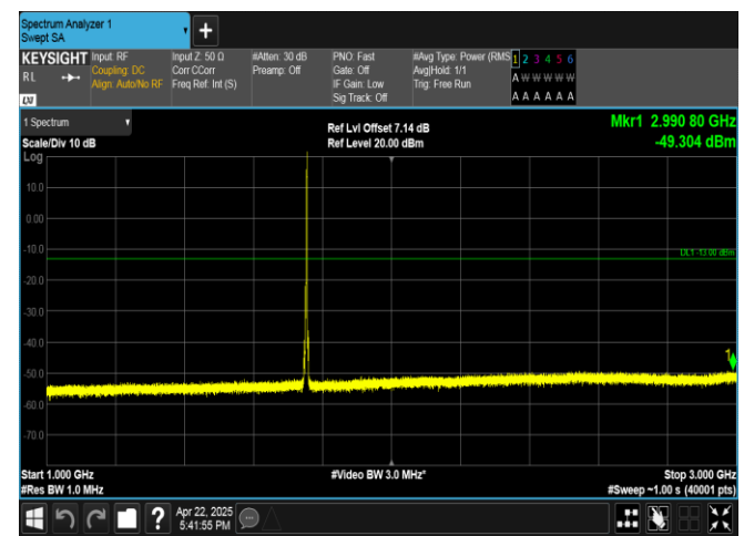
Band4-5MHz-16QAM-20375-1RB#24-1000~3000-PASS
