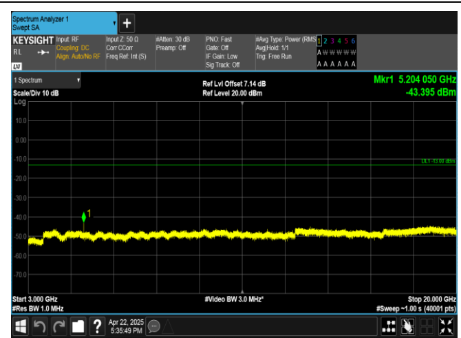
Band4-5MHz-16QAM-20175-1RB#24-3000~20000-PASS
