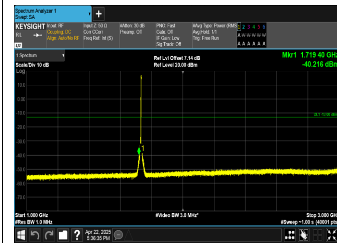
Band4-5MHz-QPSK-20175-25RB#0-1000~3000-PASS
