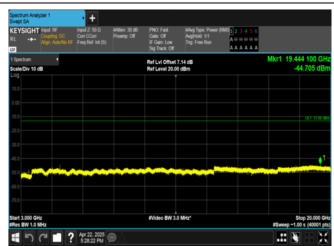
Band4-5MHz-QPSK-19975-1RB#24-3000~20000-PASS
