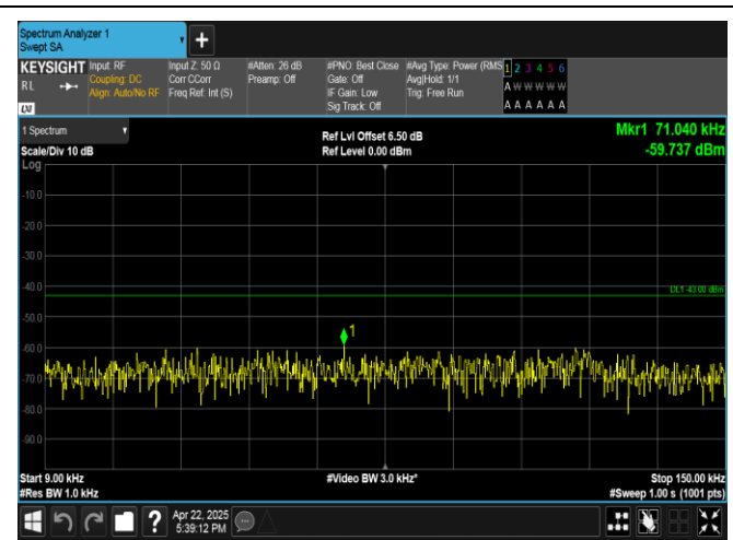
Band4-5MHz-16QAM-20375-1RB#0-0.009~0.15-PASS
