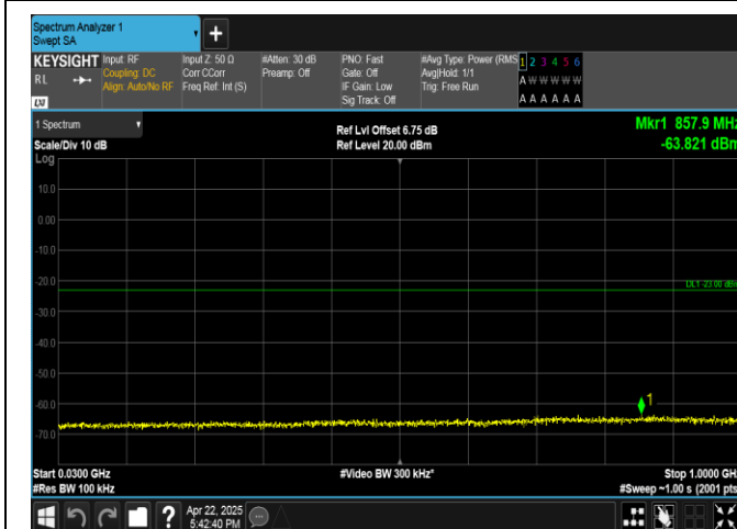
Band4-5MHz-QPSK-20375-25RB#0-30~1000-PASS
