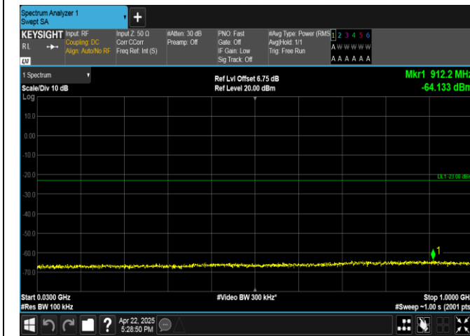
Band4-5MHz-16QAM-19975-1RB#24-30~1000-PASS
