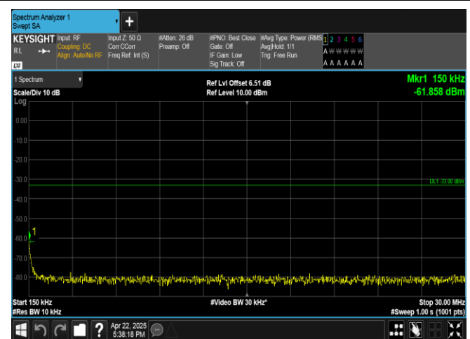
Band4-5MHz-QPSK-20375-1RB#0-0.15~30-PASS
