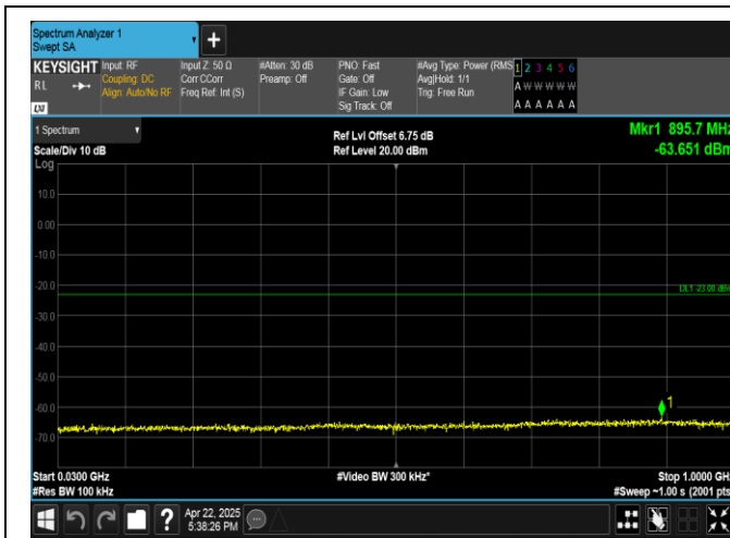
Band4-5MHz-QPSK-20375-1RB#0-30~1000-PASS
