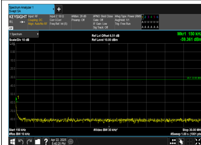
Band4-5MHz-QPSK-20375-1RB#24-0.15~30-PASS
