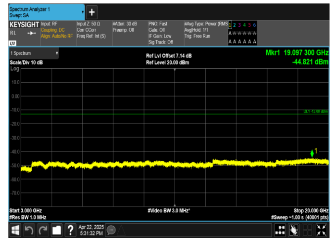
Band4-5MHz-16QAM-19975-25RB#0-3000~20000-PASS
