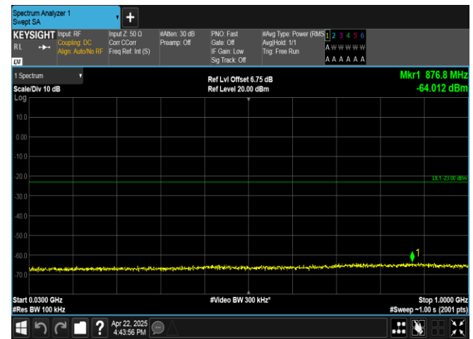
Band4-3MHz-QPSK-20175-1RB#0-30~1000-PASS
