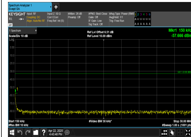
Band4-3MHz-QPSK-20175-1RB#0-0.15~30-PASS
