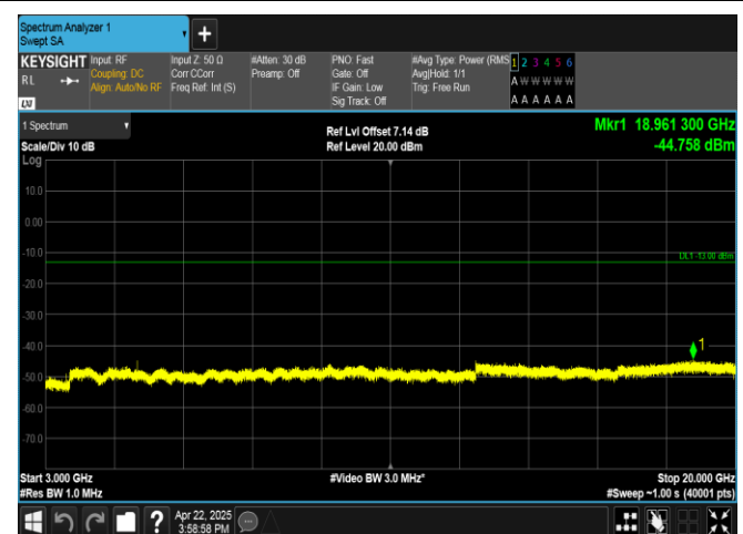
Band4-1.4MHz-16QAM-20393-1RB#0-3000~20000-PASS
