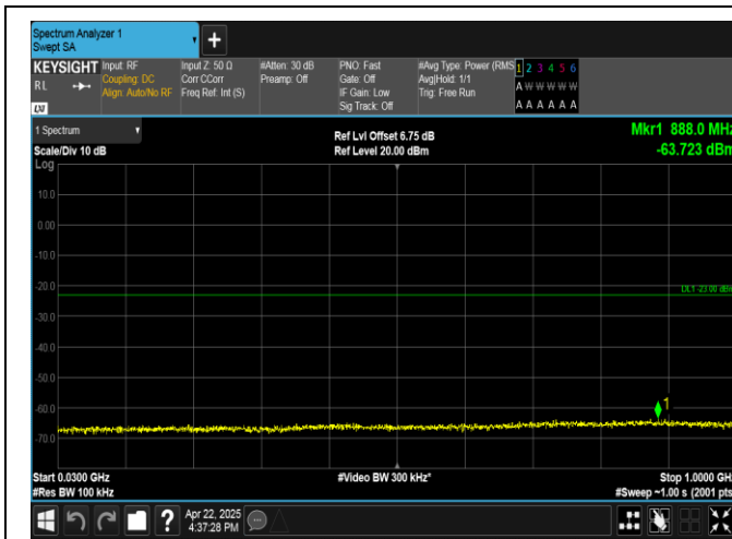
Band4-3MHz-QPSK-19965-1RB#0-30~1000-PASS
