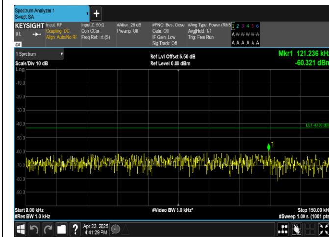
Band4-3MHz-QPSK-19965-15RB#0-0.009~0.15-PASS
