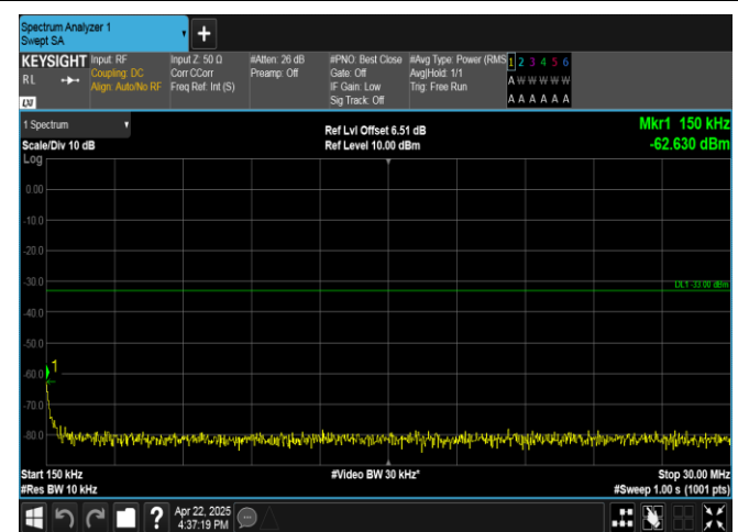
Band4-3MHz-QPSK-19965-1RB#0-0.15~30-PASS
