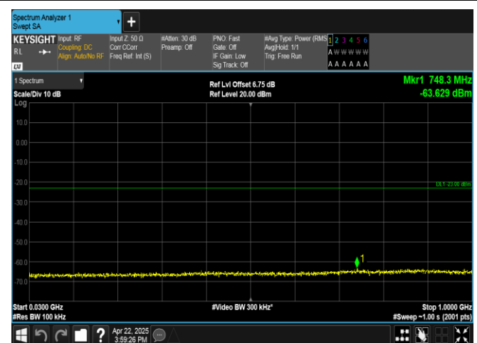
Band4-1.4MHz-QPSK-20393-1RB#5-30~1000-PASS
