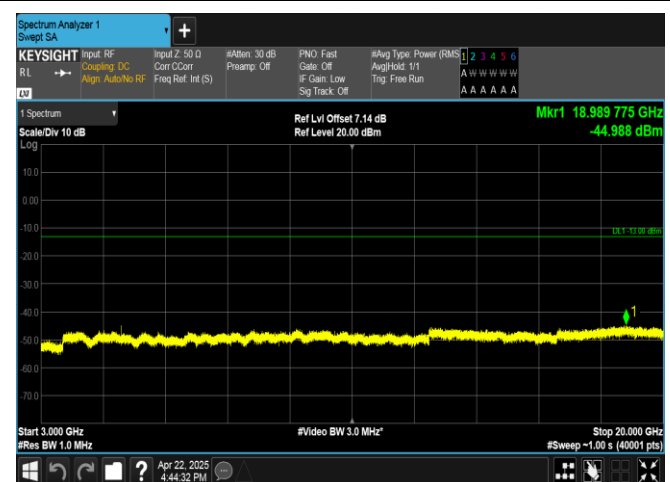
Band4-3MHz-QPSK-20175-1RB#0-3000~20000-PASS
