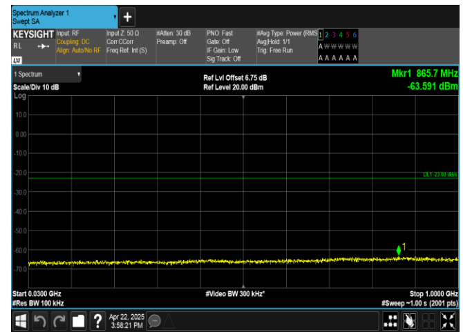
Band4-1.4MHz-16QAM-20393-1RB#0-30~1000-PASS
