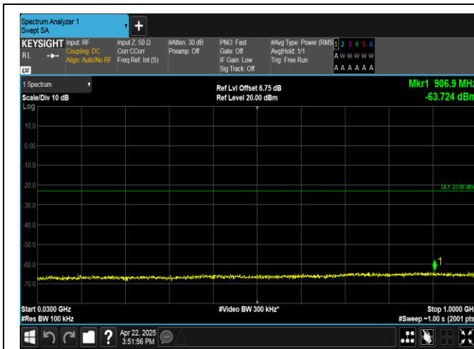
Band4-1.4MHz-16QAM-20175-1RB#0-30~1000-PASS
