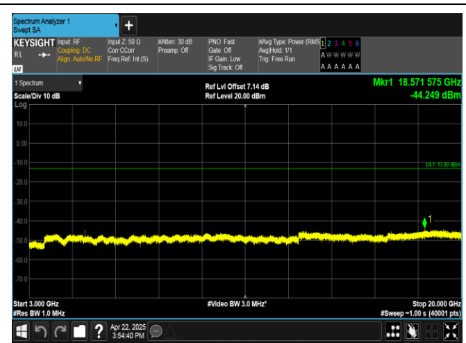
Band4-1.4MHz-16QAM-20175-1RB#5-3000~20000-PASS
