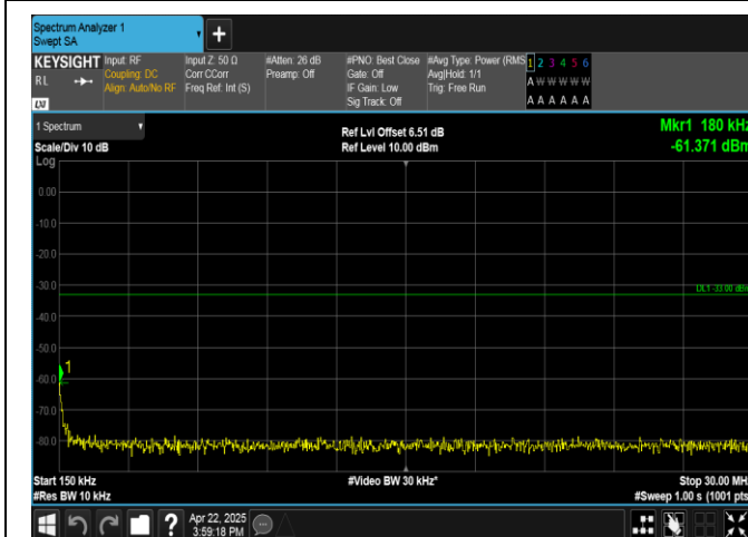
Band4-1.4MHz-QPSK-20393-1RB#5-0.15~30-PASS
