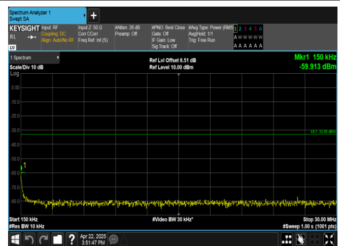
Band4-1.4MHz-16QAM-20175-1RB#0-0.15~30-PASS
