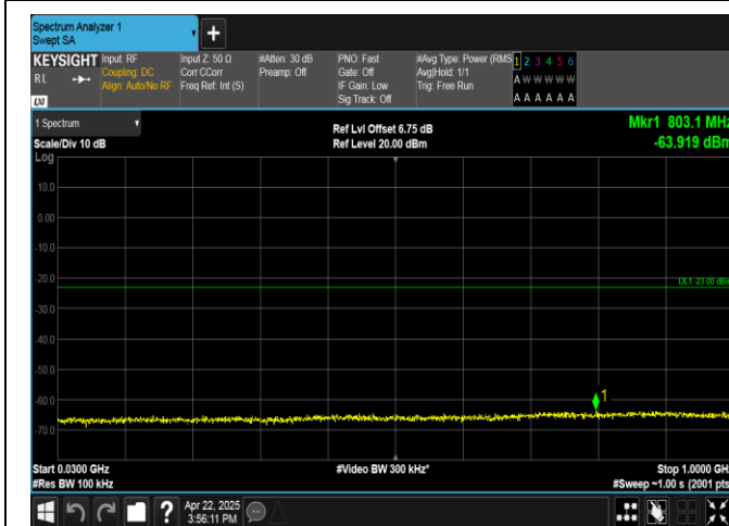
Band4-1.4MHz-16QAM-20175-6RB#0-30~1000-PASS
