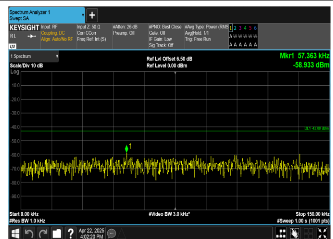
Band4-1.4MHz-16QAM-20393-6RB#0-0.009~0.15-PASS
