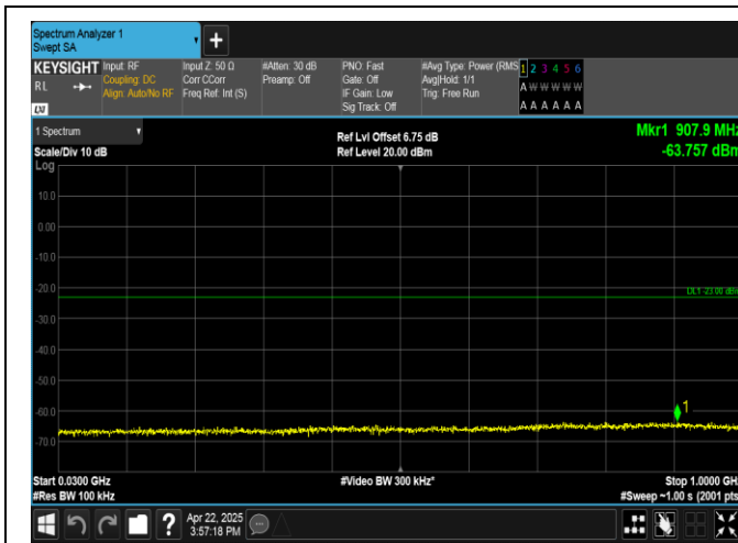
Band4-1.4MHz-QPSK-20393-1RB#0-30~1000-PASS
