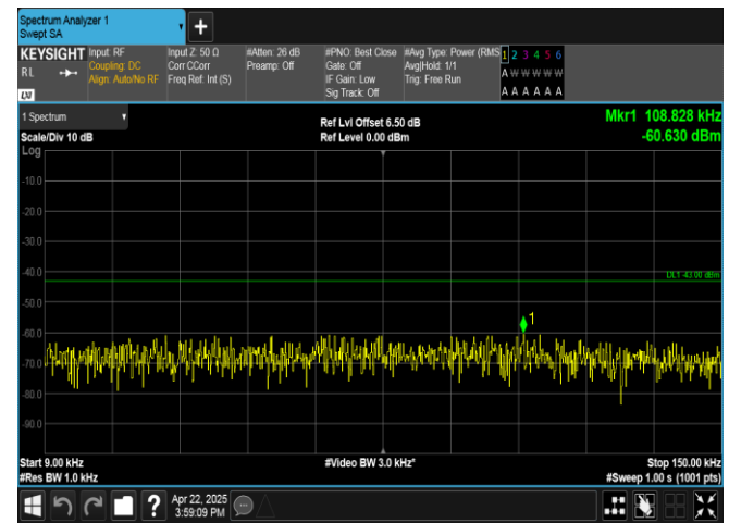
Band4-1.4MHz-QPSK-20393-1RB#5-0.009~0.15-PASS
