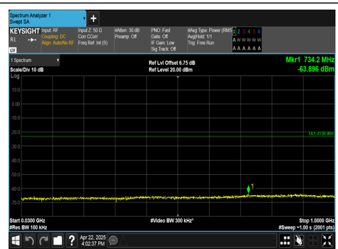
Band4-1.4MHz-16QAM-20393-6RB#0-30~1000-PASS
