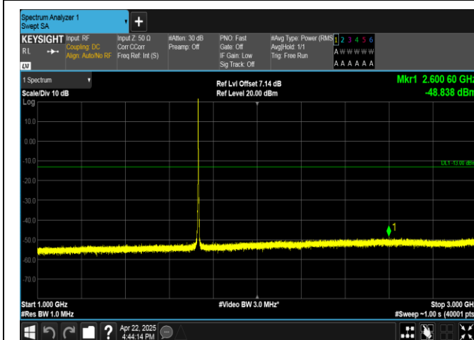
Band4-3MHz-QPSK-20175-1RB#0-1000~3000-PASS
