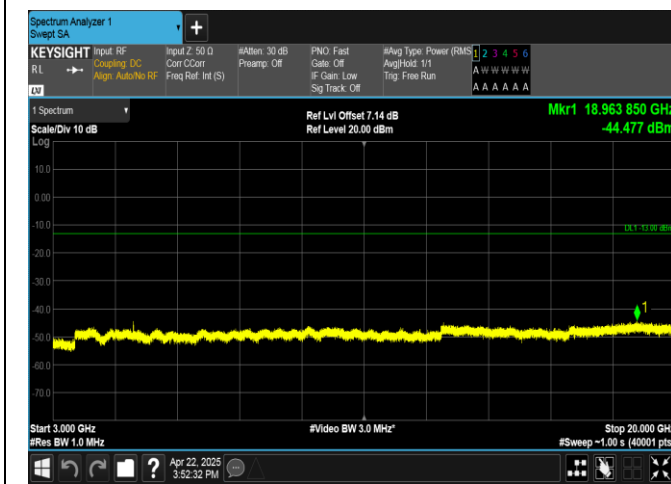
Band4-1.4MHz-16QAM-20175-1RB#0-3000~20000-PASS
