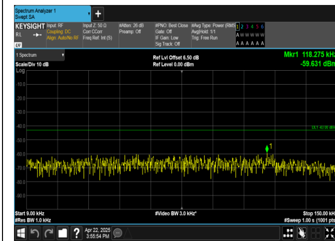
Band4-1.4MHz-16QAM-20175-6RB#0-0.009~0.15-PASS
