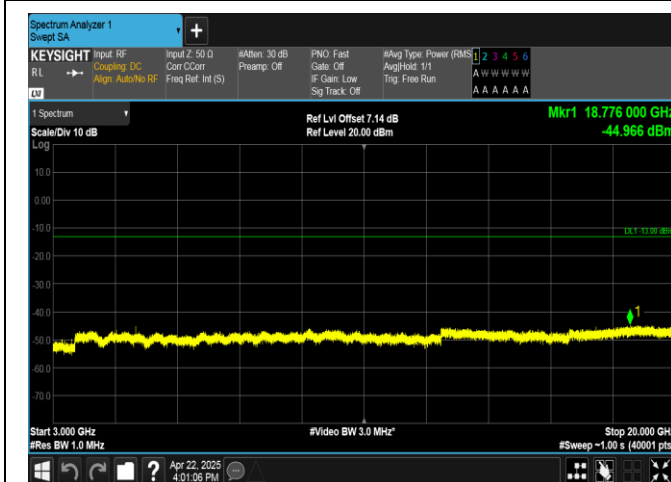
Band4-1.4MHz-16QAM-20393-1RB#5-3000~20000-PASS
