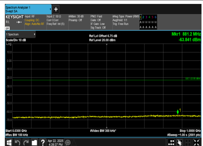
Band4-3MHz-QPSK-19965-1RB#14-30~1000-PASS
