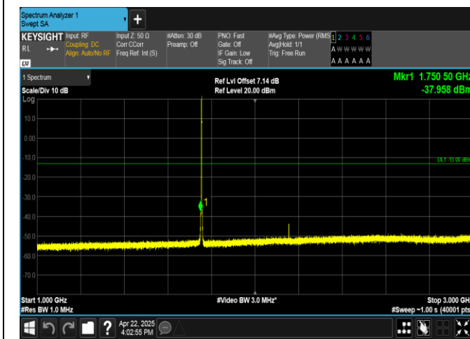
Band4-1.4MHz-16QAM-20393-6RB#0-1000~3000-PASS
