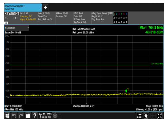
Band4-1.4MHz-16QAM-20175-1RB#5-30~1000-PASS
