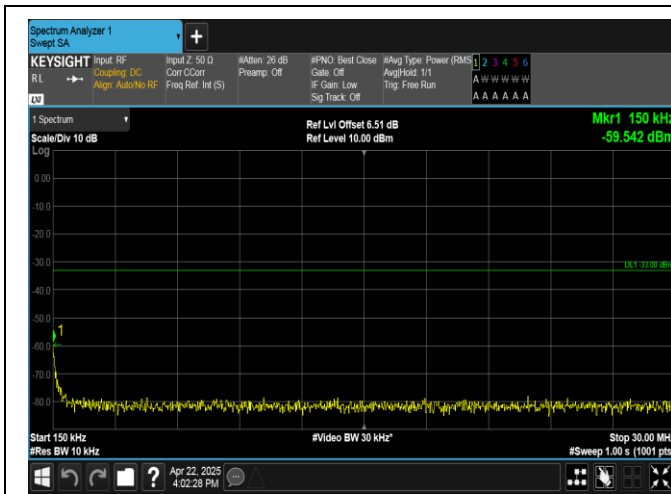
Band4-1.4MHz-16QAM-20393-6RB#0-0.15~30-PASS
