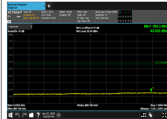
Band4-1.4MHz-16QAM-20393-1RB#5-30~1000-PASS
