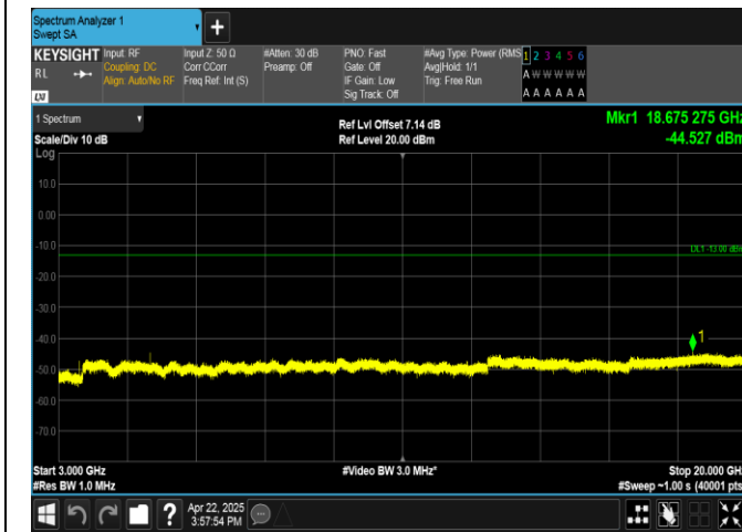
Band4-1.4MHz-QPSK-20393-1RB#0-3000~20000-PASS
