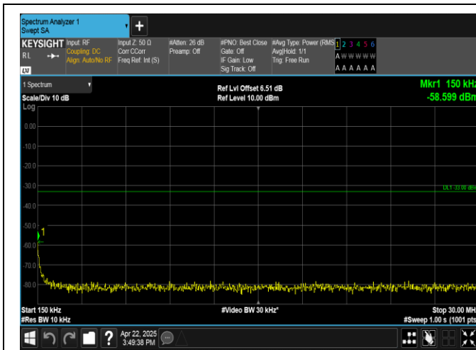
Band4-1.4MHz-16QAM-19957-6RB#0-0.15~30-PASS
