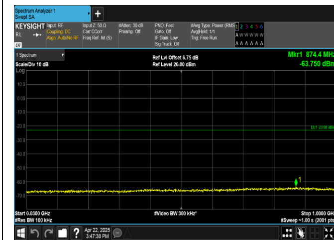
Band4-1.4MHz-16QAM-19957-1RB#5-30~1000-PASS
