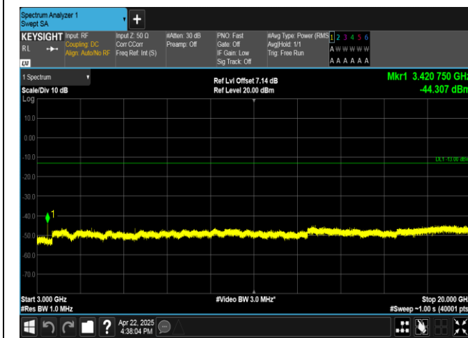
Band4-3MHz-QPSK-19965-1RB#0-3000~20000-PASS
