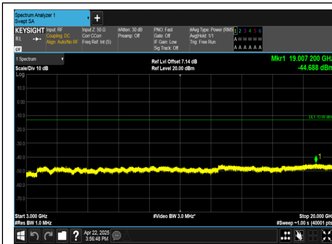
Band4-1.4MHz-16QAM-20175-6RB#0-3000~20000-PASS
