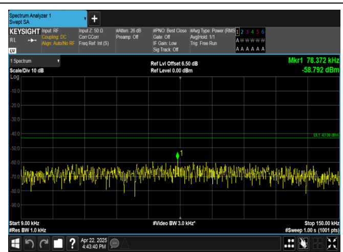
Band4-3MHz-QPSK-20175-1RB#0-0.009~0.15-PASS
