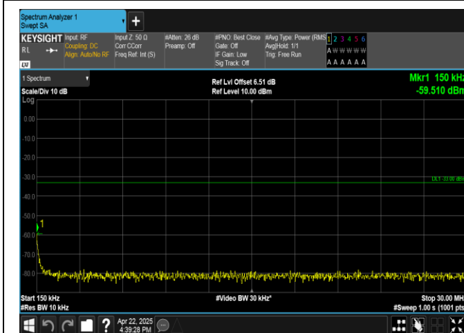
Band4-3MHz-QPSK-19965-1RB#14-0.15~30-PASS
