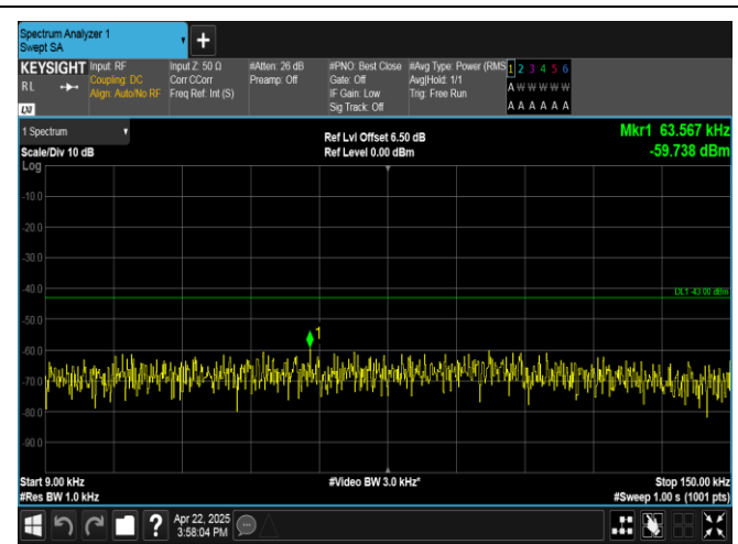
Band4-1.4MHz-16QAM-20393-1RB#0-0.009~0.15-PASS
