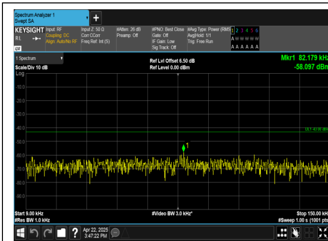
Band4-1.4MHz-16QAM-19957-1RB#5-0.009~0.15-PASS
