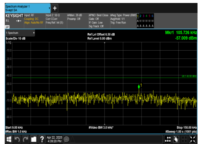
Band4-3MHz-QPSK-19965-1RB#14-0.009~0.15-PASS
