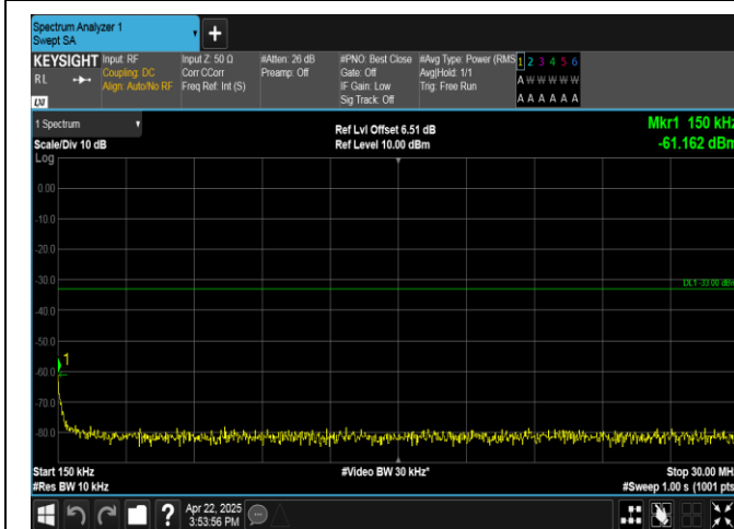
Band4-1.4MHz-16QAM-20175-1RB#5-0.15~30-PASS
