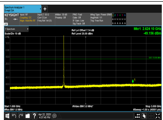
Band4-3MHz-QPSK-19965-1RB#0-1000~3000-PASS
