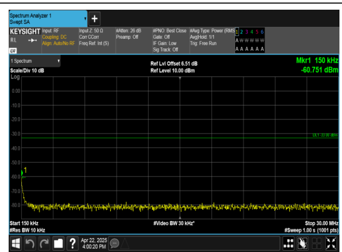
Band4-1.4MHz-16QAM-20393-1RB#5-0.15~30-PASS
