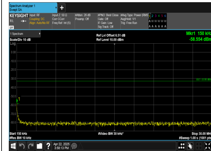
Band4-1.4MHz-16QAM-20393-1RB#0-0.15~30-PASS
