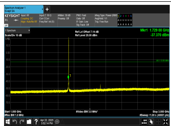
Band4-1.4MHz-16QAM-20175-1RB#0-1000~3000-PASS
