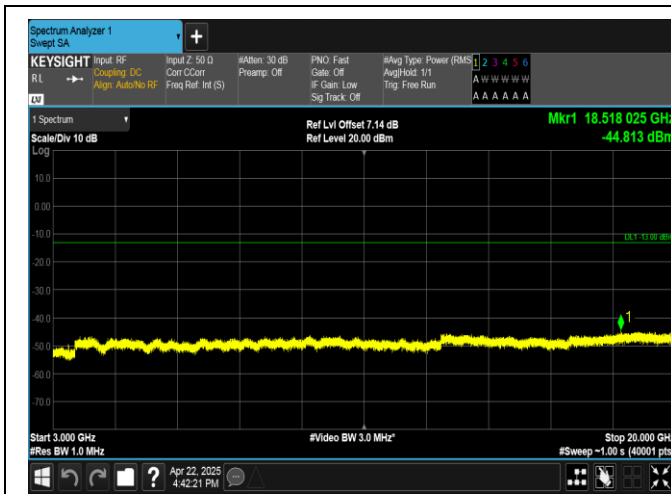
Band4-3MHz-QPSK-19965-15RB#0-3000~20000-PASS
