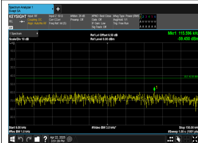
Band4-1.4MHz-16QAM-20175-1RB#0-0.009~0.15-PASS
