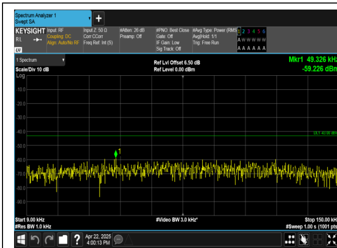
Band4-1.4MHz-16QAM-20393-1RB#5-0.009~0.15-PASS
