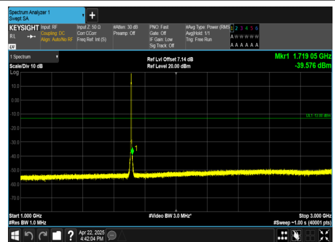
Band4-3MHz-QPSK-19965-15RB#0-1000~3000-PASS
