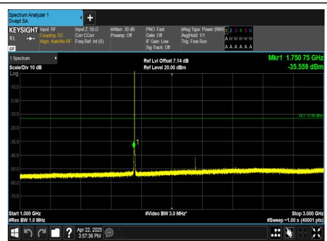
Band4-1.4MHz-QPSK-20393-1RB#0-1000~3000-PASS
