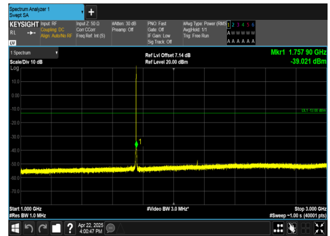
Band4-1.4MHz-16QAM-20393-1RB#5-1000~3000-PASS
