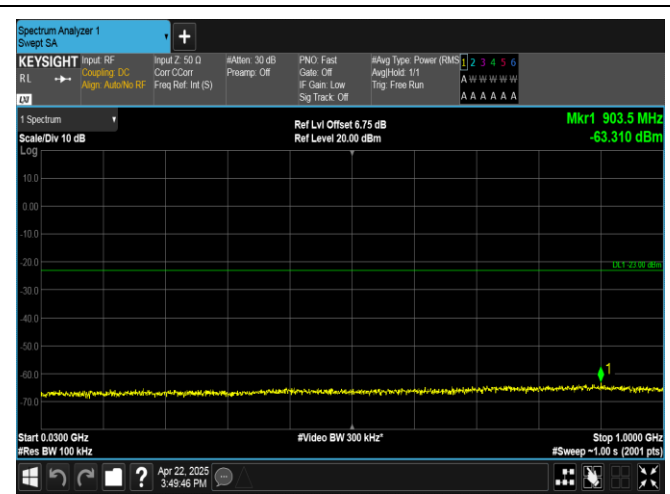
Band4-1.4MHz-16QAM-19957-6RB#0-30~1000-PASS
