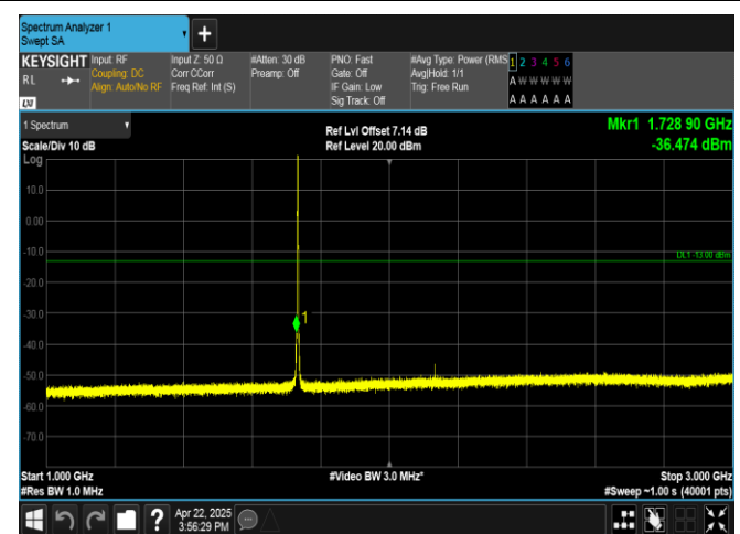
Band4-1.4MHz-16QAM-20175-6RB#0-1000~3000-PASS
