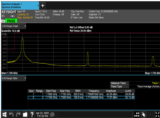
Band4-20MHz-16QAM-20050-1RB#0-PASS
