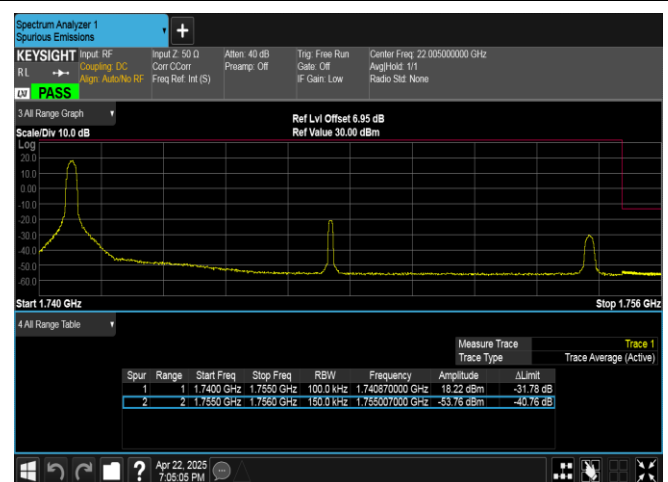
Band4-15MHz-16QAM-20325-1RB#0-PASS
