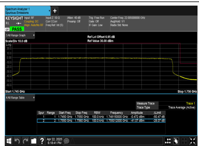
Band4-10MHz-16QAM-20350-50RB#0-PASS
