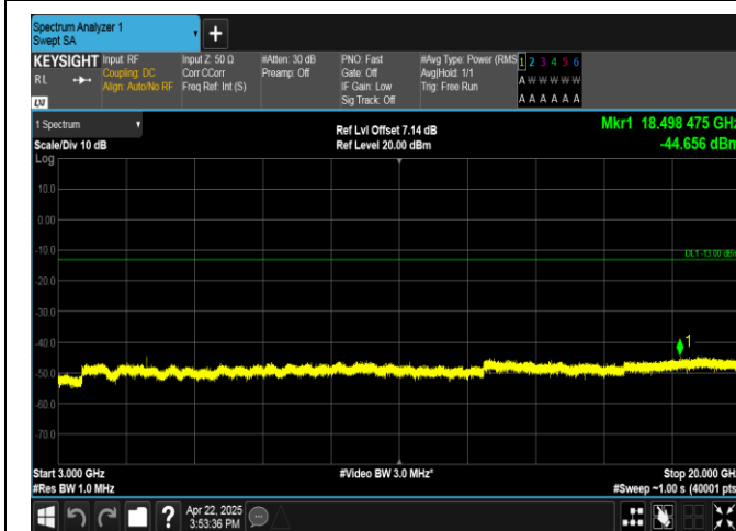
Band4-1.4MHz-QPSK-20175-1RB#5-3000~20000-PASS
