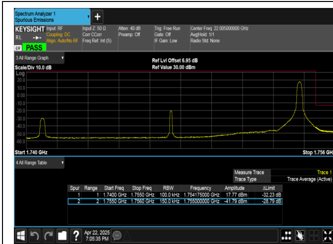
Band4-15MHz-16QAM-20325-1RB#74-PASS
