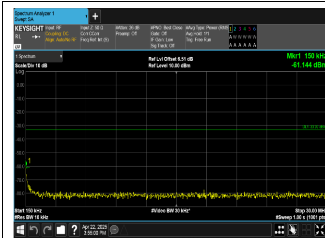
Band4-1.4MHz-QPSK-20175-6RB#0-0.15~30-PASS
