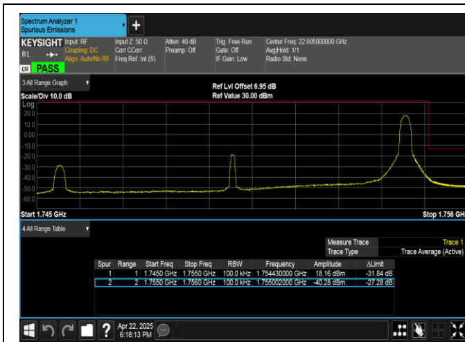
Band4-10MHz-16QAM-20350-1RB#49-PASS
