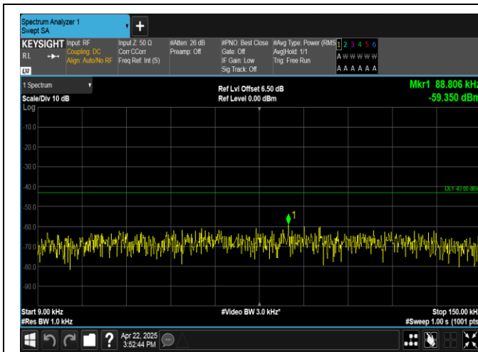
Band4-1.4MHz-QPSK-20175-1RB#5-0.009~0.15-PASS
