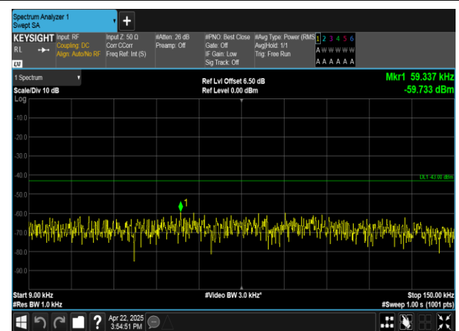
Band4-1.4MHz-QPSK-20175-6RB#0-0.009~0.15-PASS
