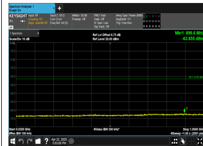
Band4-1.4MHz-QPSK-20175-1RB#5-30~1000-PASS
