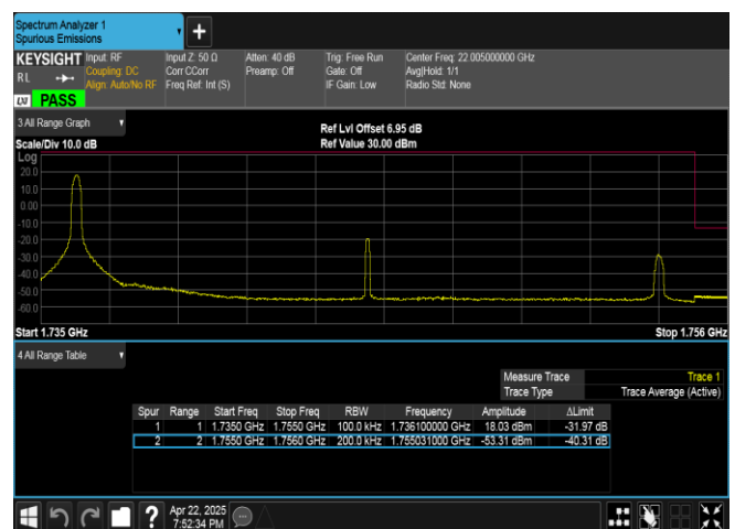
Band4-20MHz-16QAM-20300-1RB#0-PASS
