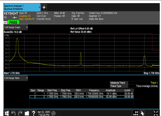
Band4-20MHz-QPSK-20300-1RB#0-PASS
