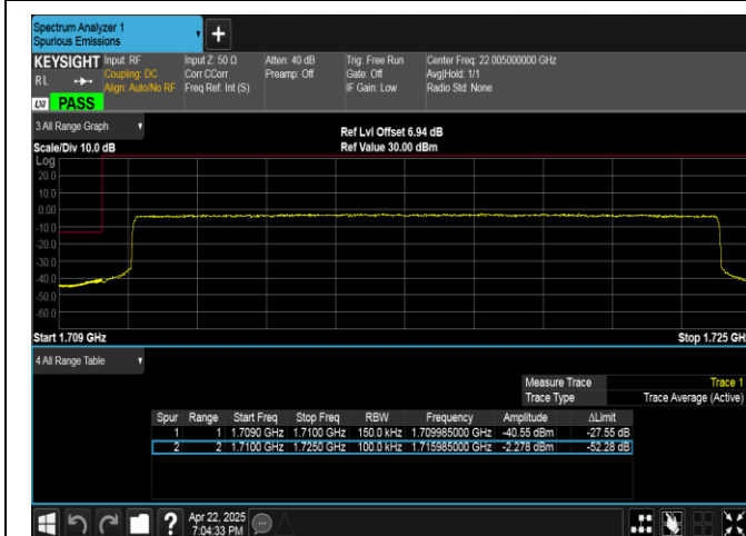
Band4-15MHz-16QAM-20025-75RB#0-PASS
