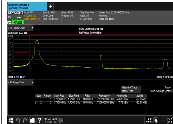
Band4-10MHz-16QAM-20000-1RB#0-PASS
