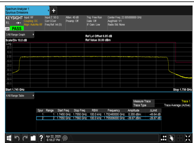
Band4-10MHz-QPSK-20350-50RB#0-PASS
