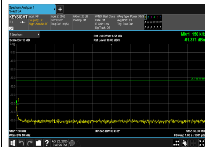
Band4-1.4MHz-QPSK-19957-1RB#5-0.15~30-PASS
