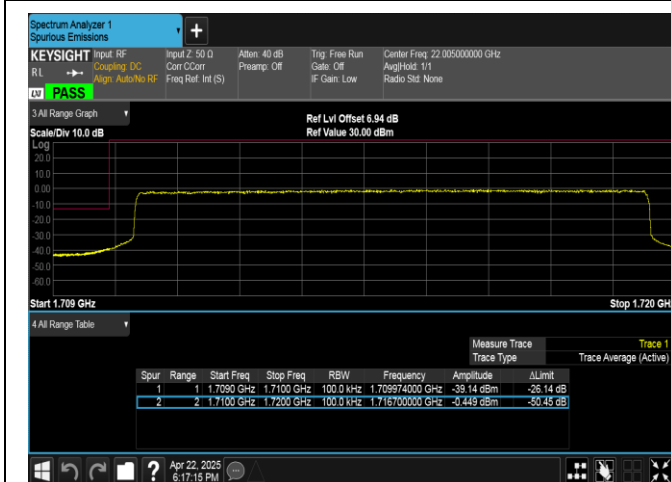
Band4-10MHz-16QAM-20000-50RB#0-PASS
