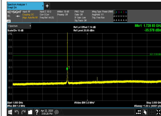
Band4-1.4MHz-QPSK-20175-6RB#0-1000~3000-PASS
