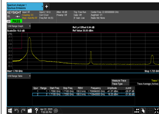
Band4-15MHz-16QAM-20025-1RB#0-PASS
