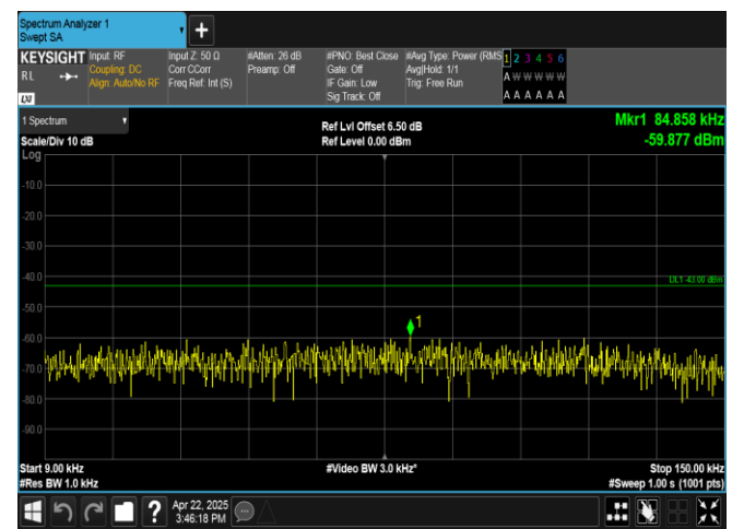
Band4-1.4MHz-QPSK-19957-1RB#5-0.009~0.15-PASS
