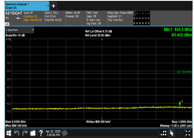
Band4-1.4MHz-QPSK-20175-6RB#0-30~1000-PASS
