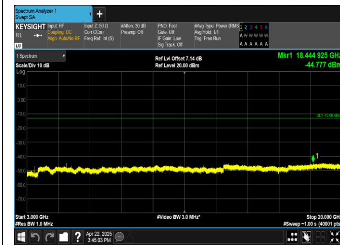
Band4-1.4MHz-QPSK-19957-1RB#0-3000~20000-PASS
