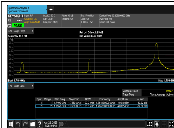
Band4-15MHz-QPSK-20325-1RB#74-PASS
