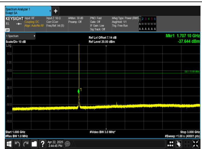
Band4-1.4MHz-QPSK-19957-1RB#0-1000~3000-PASS
