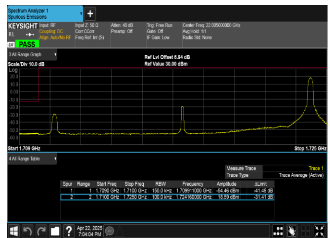
Band4-15MHz-16QAM-20025-1RB#74-PASS
