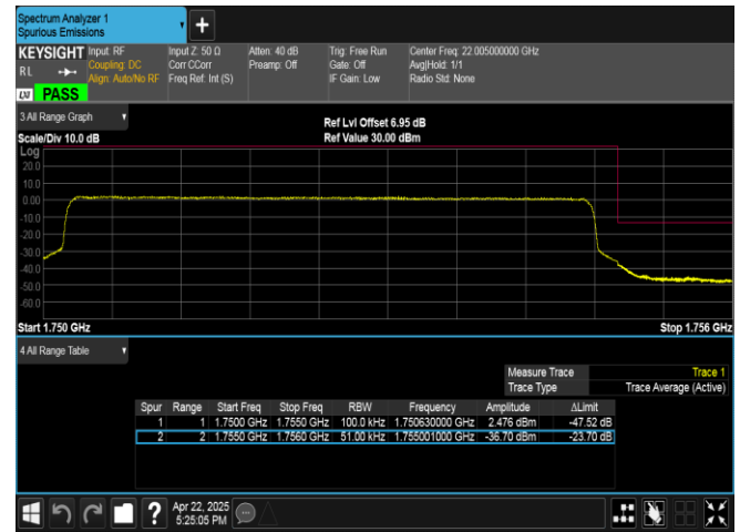
Band4-5MHz-16QAM-20375-25RB#0-PASS
