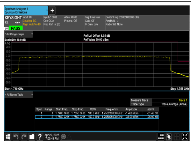
Band4-15MHz-QPSK-20325-75RB#0-PASS
