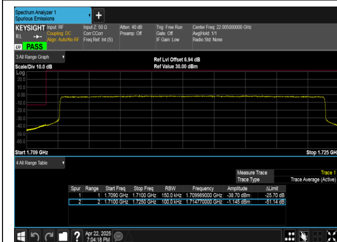
Band4-15MHz-QPSK-20025-75RB#0-PASS
