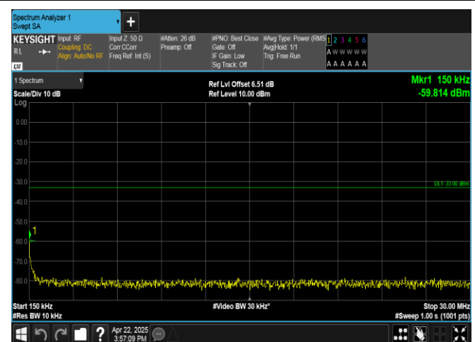
Band4-1.4MHz-QPSK-20393-1RB#0-0.15~30-PASS
