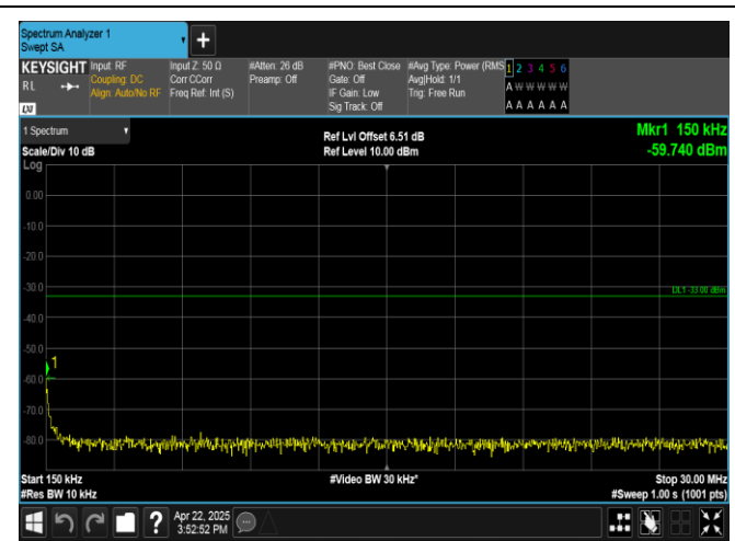
Band4-1.4MHz-QPSK-20175-1RB#5-0.15~30-PASS
