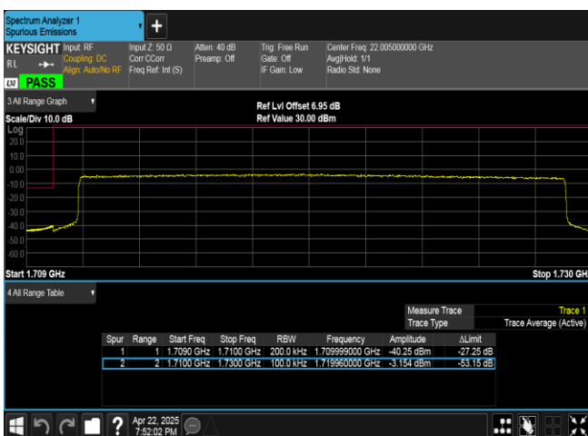
Band4-20MHz-16QAM-20050-100RB#0-PASS
