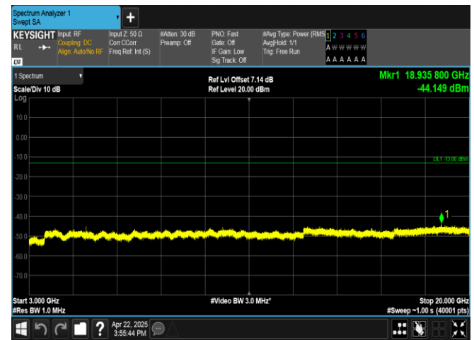
Band4-1.4MHz-QPSK-20175-6RB#0-3000~20000-PASS
