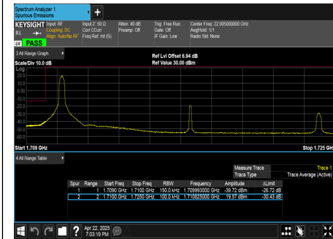
Band4-15MHz-QPSK-20025-1RB#0-PASS
