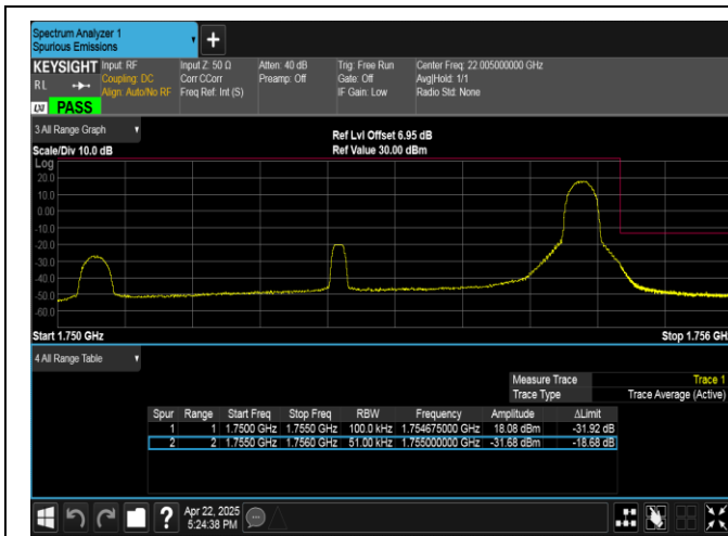
Band4-5MHz-16QAM-20375-1RB#24-PASS
