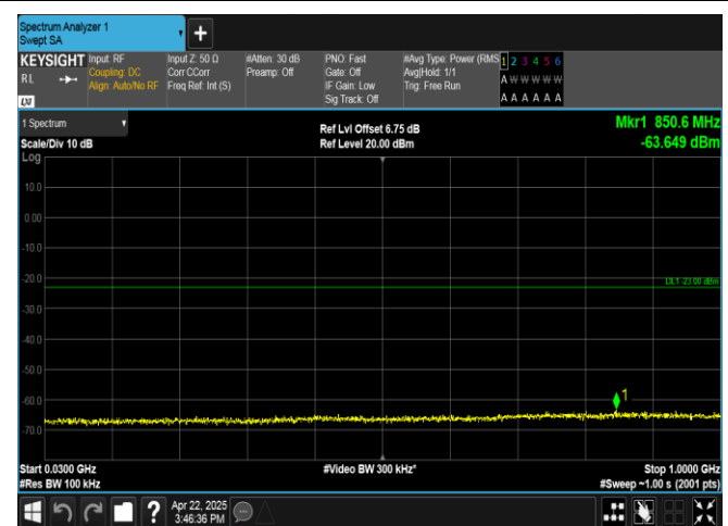
Band4-1.4MHz-QPSK-19957-1RB#5-30~1000-PASS
