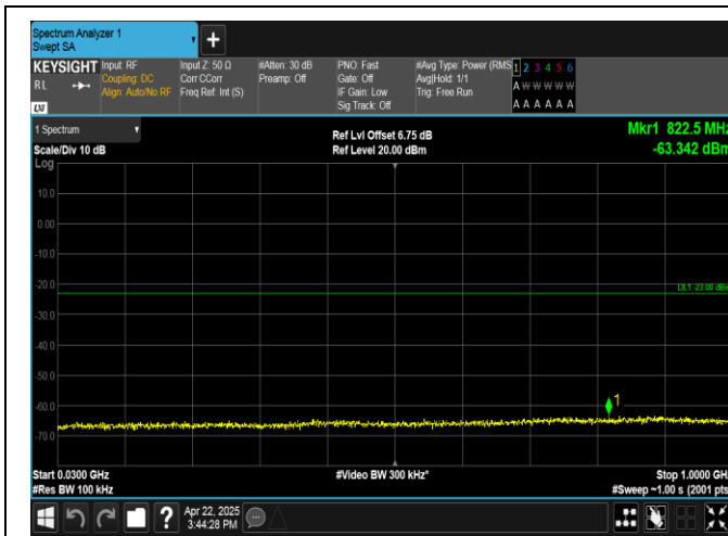
Band4-1.4MHz-QPSK-19957-1RB#0-30~1000-PASS
