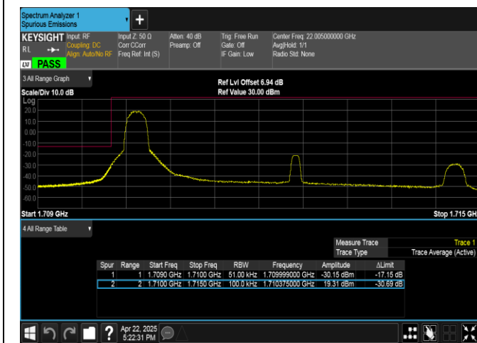
Band4-5MHz-QPSK-19975-1RB#0-PASS
