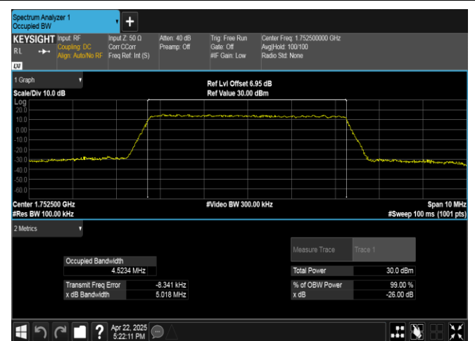
Band4-5MHz-16QAM-20375-25RB#0-PASS
