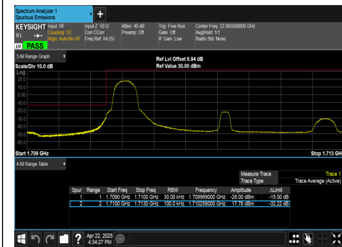
Band4-3MHz-16QAM-19965-1RB#0-PASS
