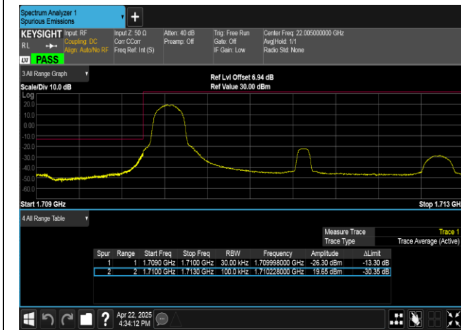
Band4-3MHz-QPSK-19965-1RB#0-PASS
