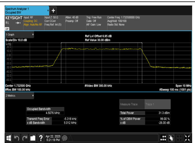
Band4-5MHz-QPSK-20175-25RB#0-PASS
