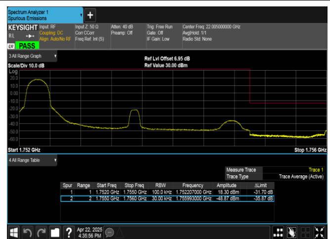
Band4-3MHz-16QAM-20385-1RB#0-PASS
