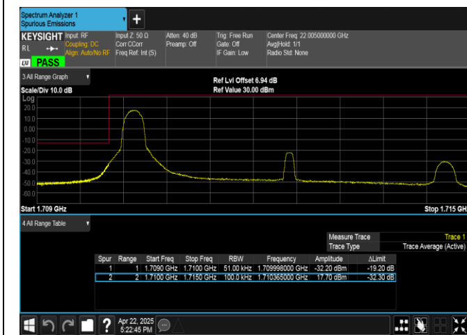
Band4-5MHz-16QAM-19975-1RB#0-PASS
