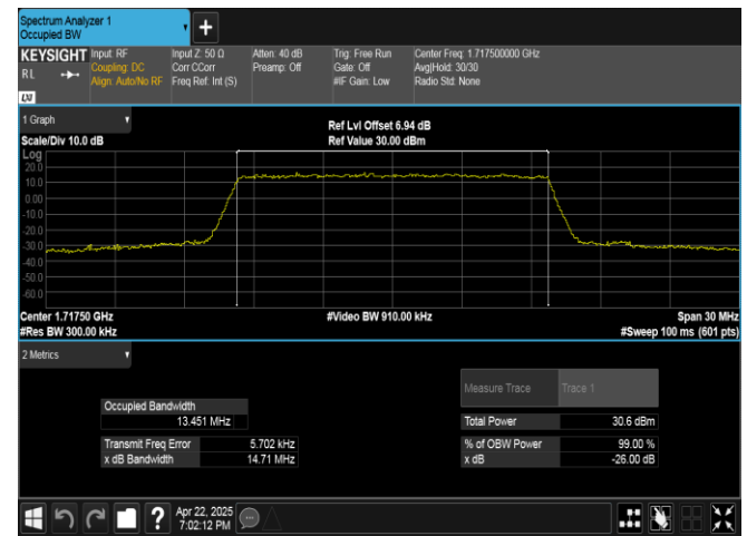
Band4-15MHz-16QAM-20025-75RB#0-PASS
