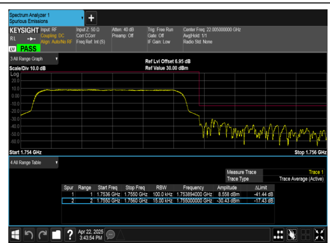
Band4-1.4MHz-16QAM-20393-6RB#0-PASS
