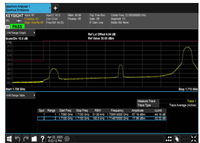
Band4-5MHz-16QAM-19975-1RB#24-PASS
