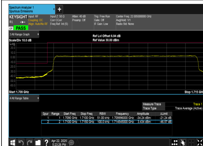
Band4-5MHz-QPSK-19975-25RB#0-PASS
