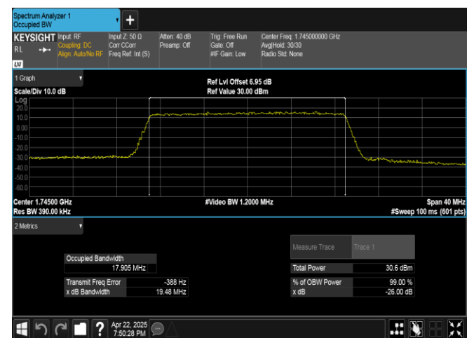
Band4-20MHz-16QAM-20300-100RB#0-PASS
