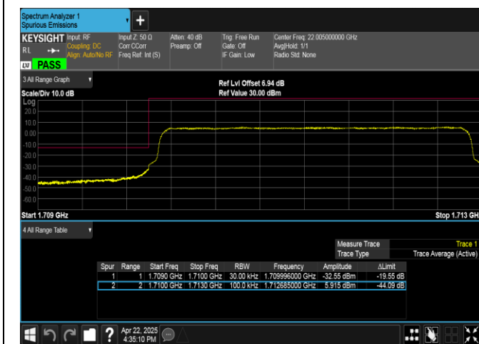
Band4-3MHz-QPSK-19965-15RB#0-PASS
