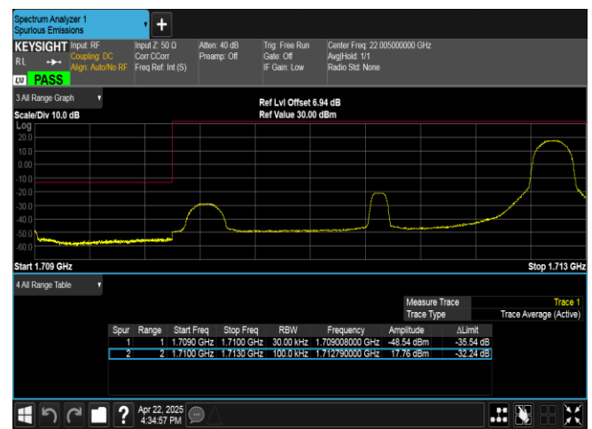
Band4-3MHz-16QAM-19965-1RB#14-PASS
