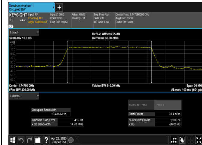
Band4-15MHz-QPSK-20325-75RB#0-PASS
