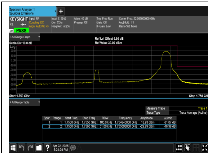
Band4-5MHz-QPSK-20375-1RB#24-PASS
