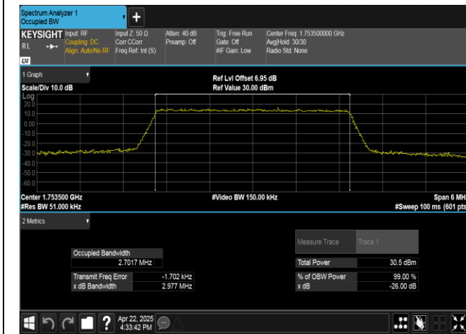
Band4-3MHz-QPSK-20385-15RB#0-PASS
