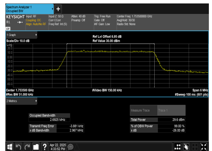
Band4-3MHz-16QAM-20385-15RB#0-PASS
