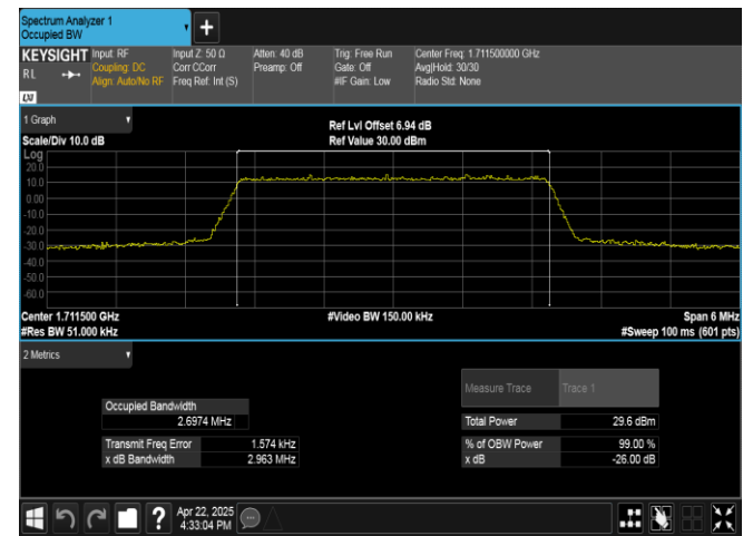
Band4-3MHz-16QAM-19965-15RB#0-PASS
