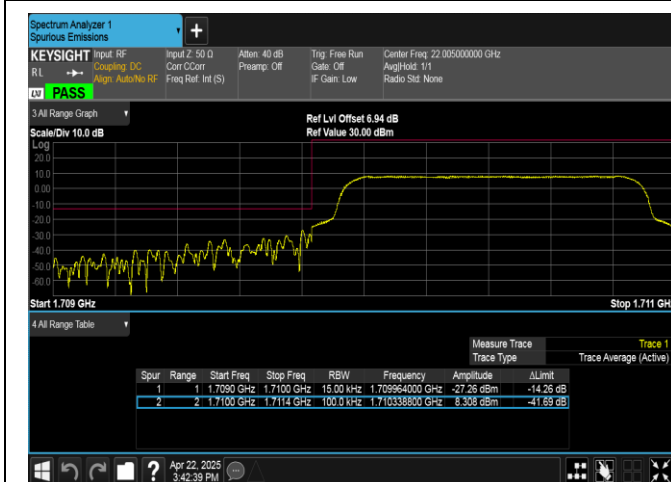
Band4-1.4MHz-16QAM-19957-6RB#0-PASS
