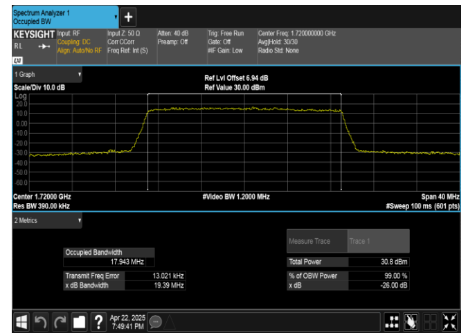
Band4-20MHz-16QAM-20050-100RB#0-PASS
