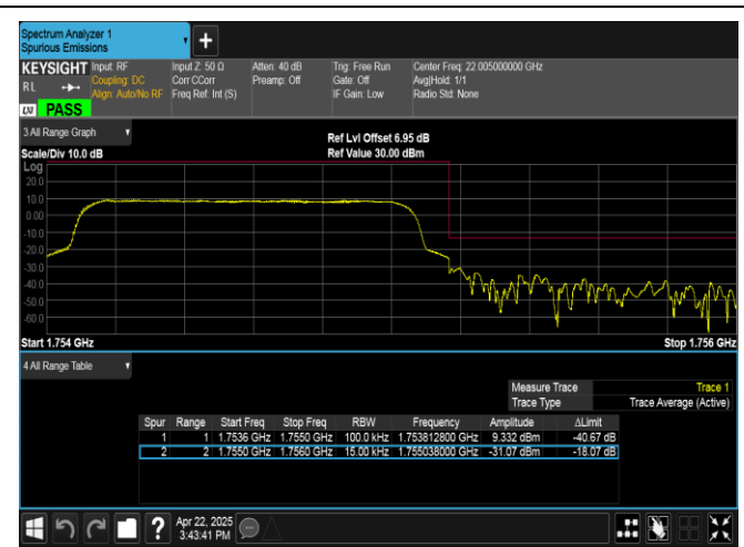
Band4-1.4MHz-QPSK-20393-6RB#0-PASS
