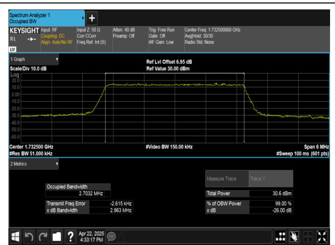
Band4-3MHz-QPSK-20175-15RB#0-PASS
