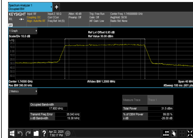
Band4-20MHz-QPSK-20300-100RB#0-PASS
