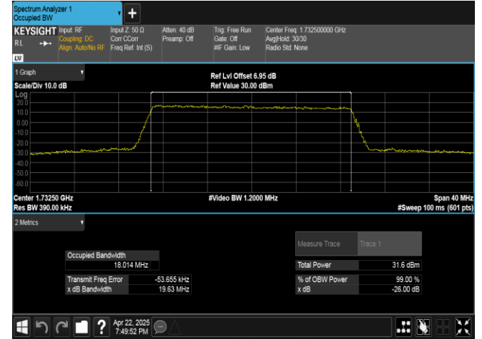
Band4-20MHz-QPSK-20175-100RB#0-PASS
