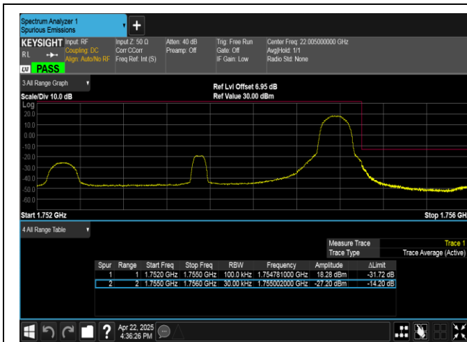
Band4-3MHz-16QAM-20385-1RB#14-PASS
