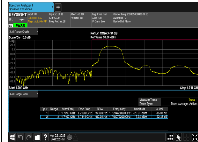
Band4-1.4MHz-16QAM-19957-1RB#0-PASS
