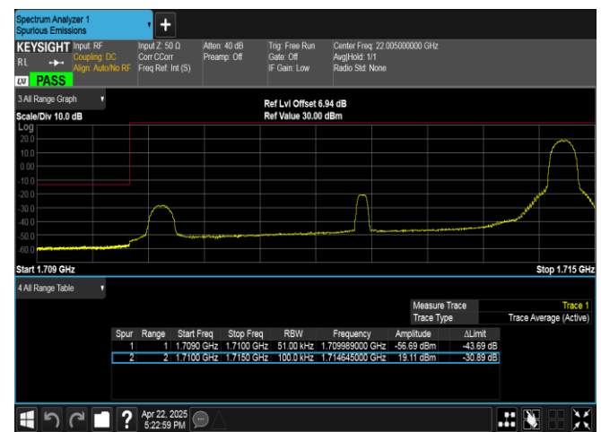
Band4-5MHz-QPSK-19975-1RB#24-PASS
