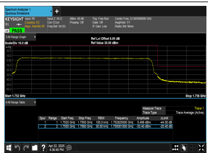
Band4-3MHz-QPSK-20385-15RB#0-PASS
