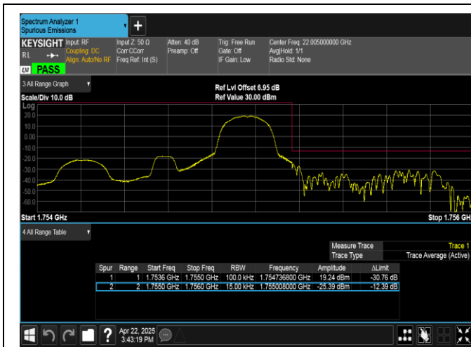
Band4-1.4MHz-QPSK-20393-1RB#5-PASS
