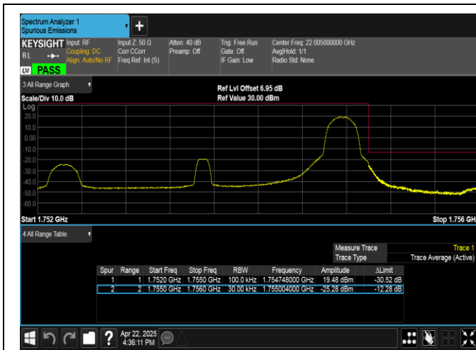
Band4-3MHz-QPSK-20385-1RB#14-PASS
