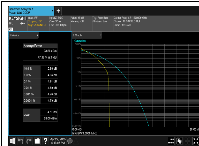
Band4-3MHz-QPSK-19965-1RB#0-PASS
