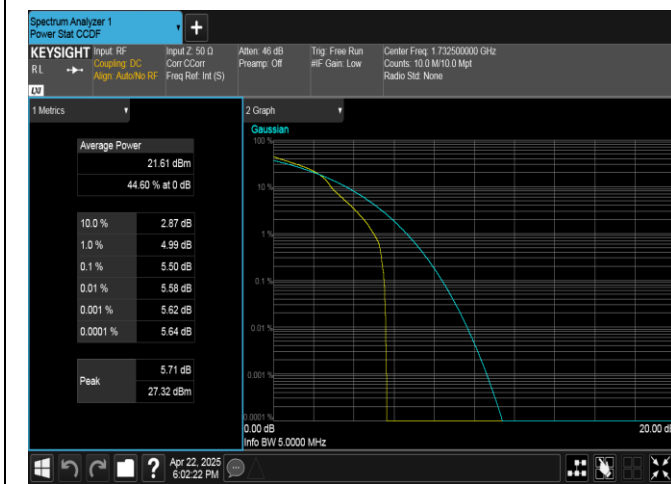
Band4-5MHz-16QAM-20175-1RB#0-PASS
