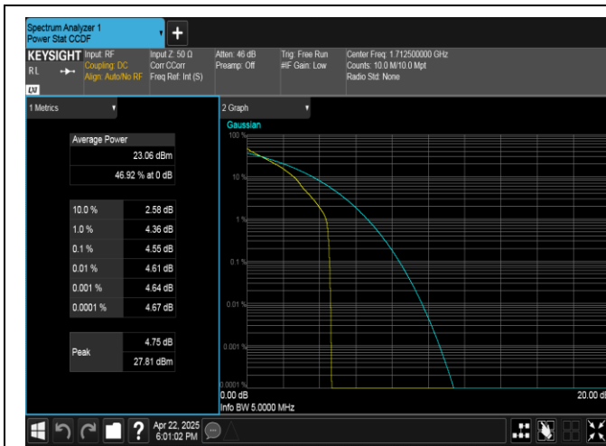
Band4-5MHz-QPSK-19975-1RB#0-PASS
