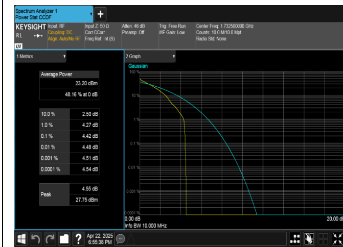
Band4-10MHz-QPSK-20175-1RB#0-PASS
