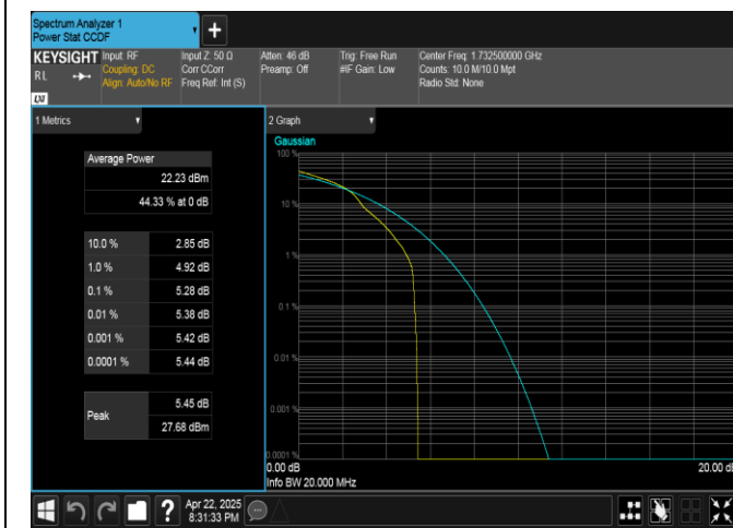
Band4-20MHz-16QAM-20175-1RB#0-PASS
