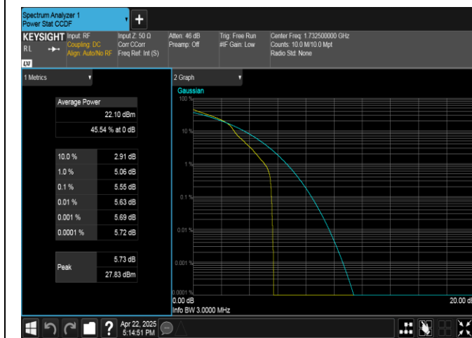
Band4-3MHz-16QAM-20175-1RB#0-PASS
