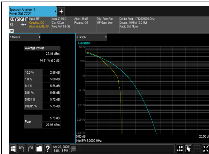
Band4-5MHz-16QAM-19975-1RB#0-PASS
