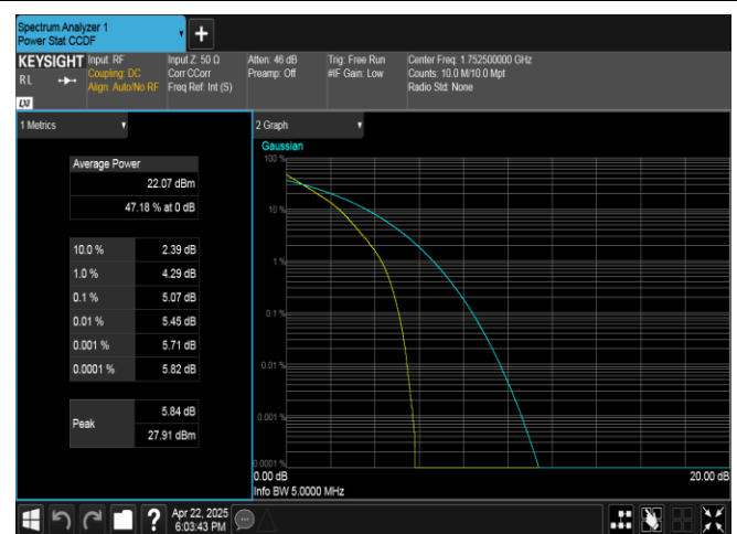
Band4-5MHz-QPSK-20375-25RB#0-PASS
