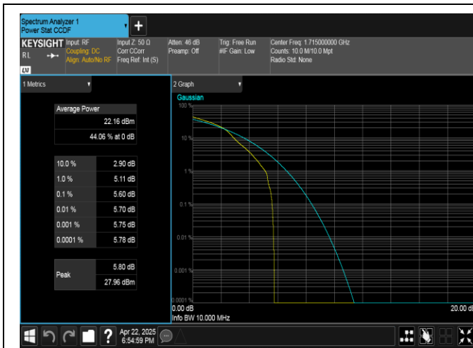
Band4-10MHz-16QAM-20000-1RB#0-PASS
