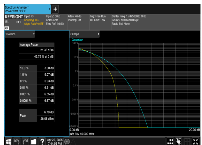
Band4-15MHz-16QAM-20325-75RB#0-PASS
