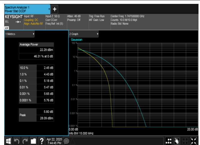
Band4-15MHz-QPSK-20325-75RB#0-PASS
