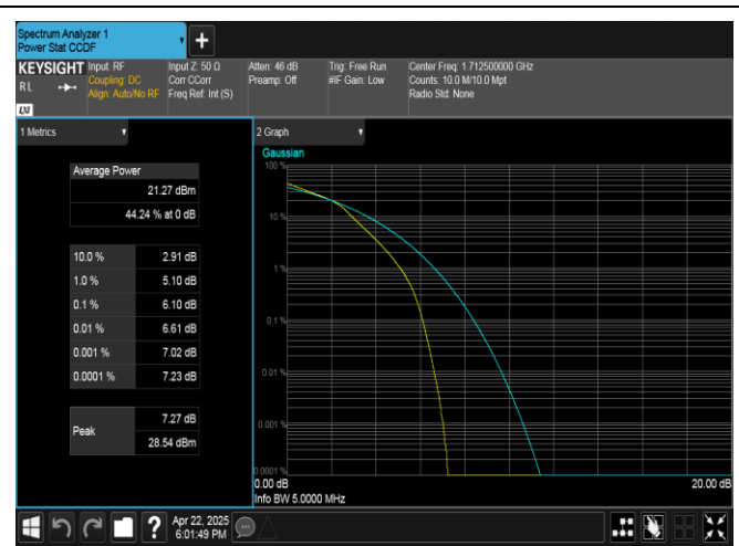
Band4-5MHz-16QAM-19975-25RB#0-PASS
