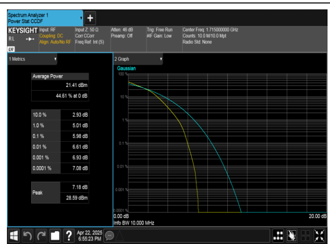
Band4-10MHz-16QAM-20000-50RB#0-PASS
