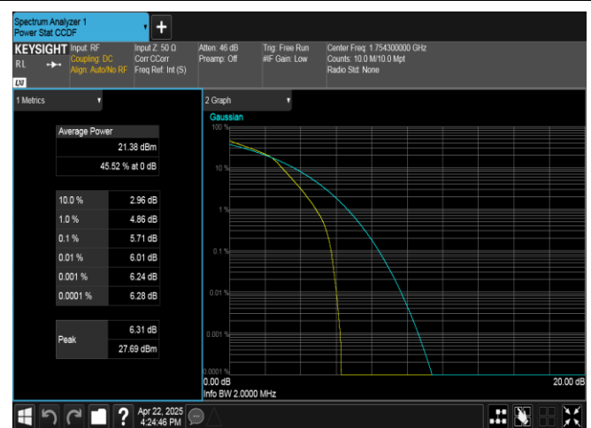
Band4-1.4MHz-16QAM-20393-6RB#0-PASS
