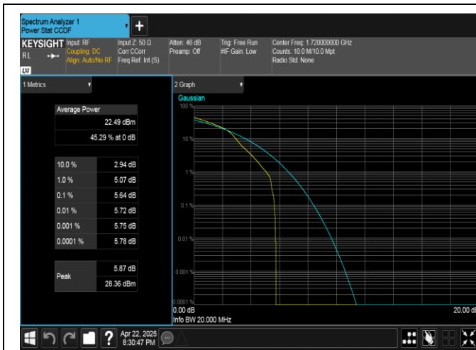
Band4-20MHz-16QAM-20050-1RB#0-PASS
