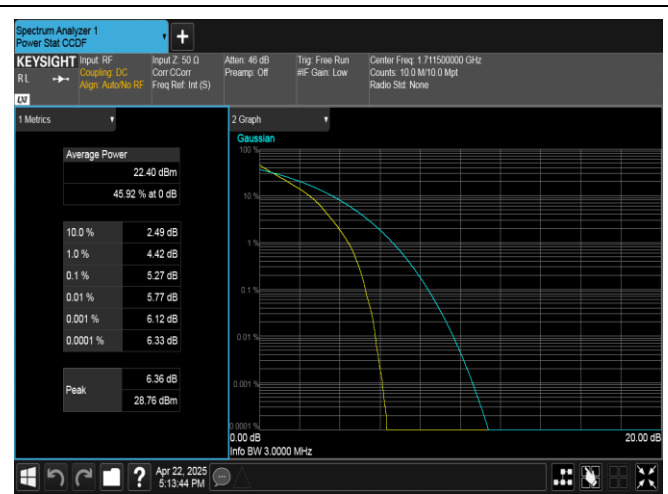
Band4-3MHz-QPSK-19965-15RB#0-PASS
