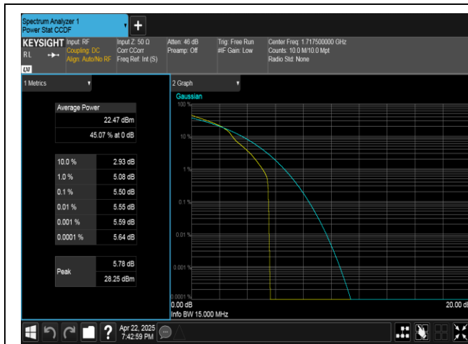
Band4-15MHz-16QAM-20025-1RB#0-PASS
