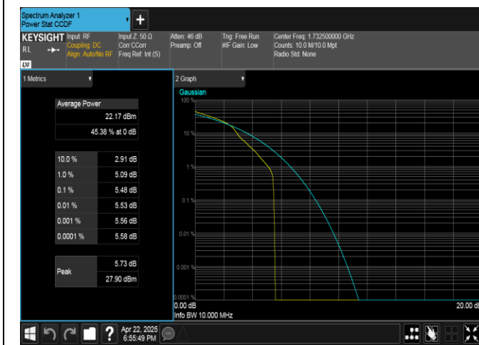
Band4-10MHz-16QAM-20175-1RB#0-PASS
