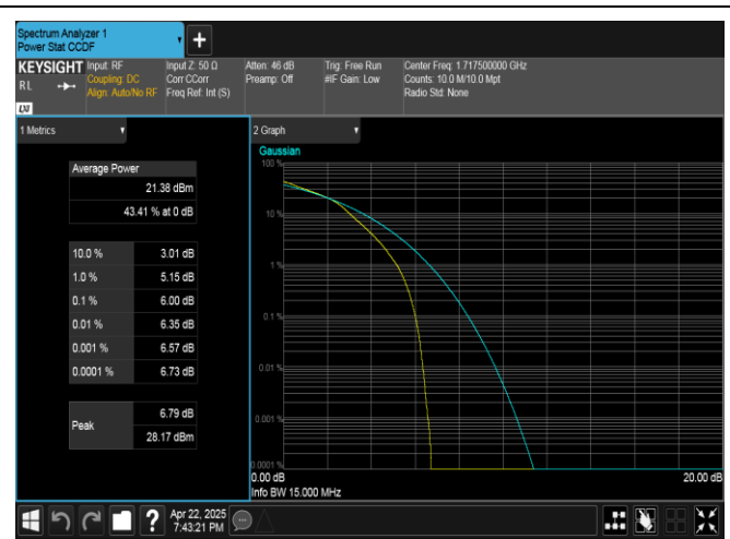
Band4-15MHz-16QAM-20025-75RB#0-PASS
