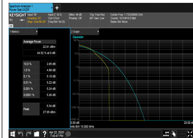
Band4-15MHz-16QAM-20175-1RB#0-PASS
