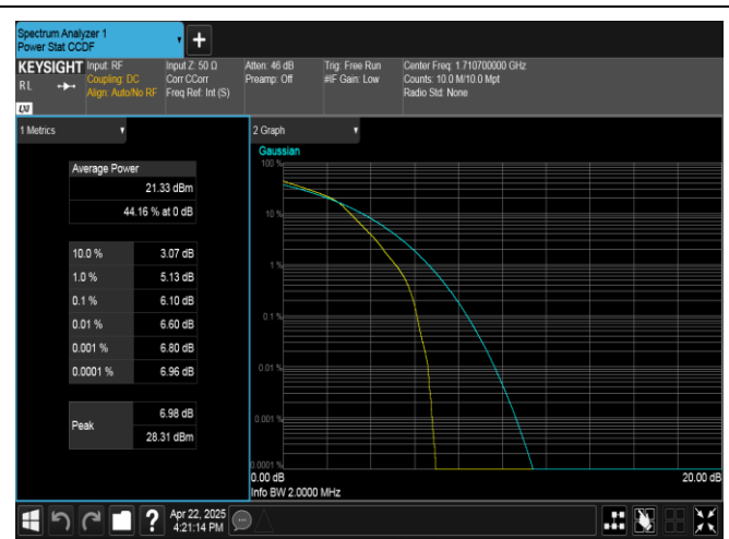
Band4-1.4MHz-16QAM-19957-6RB#0-PASS
