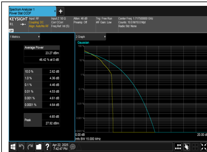
Band4-15MHz-QPSK-20025-1RB#0-PASS
