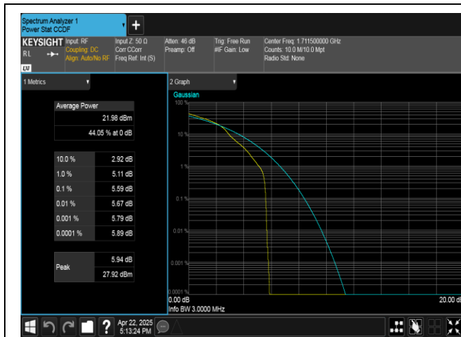
Band4-3MHz-16QAM-19965-1RB#0-PASS
