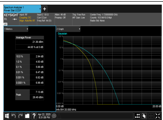
Band4-20MHz-16QAM-20050-100RB#0-PASS
