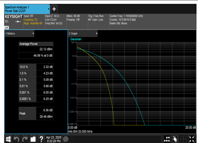
Band4-20MHz-QPSK-20300-100RB#0-PASS
