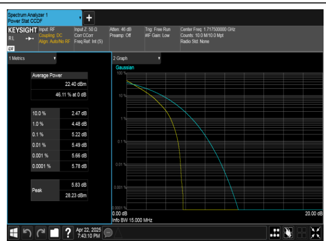
Band4-15MHz-QPSK-20025-75RB#0-PASS
