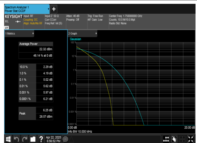
Band4-10MHz-QPSK-20350-50RB#0-PASS
