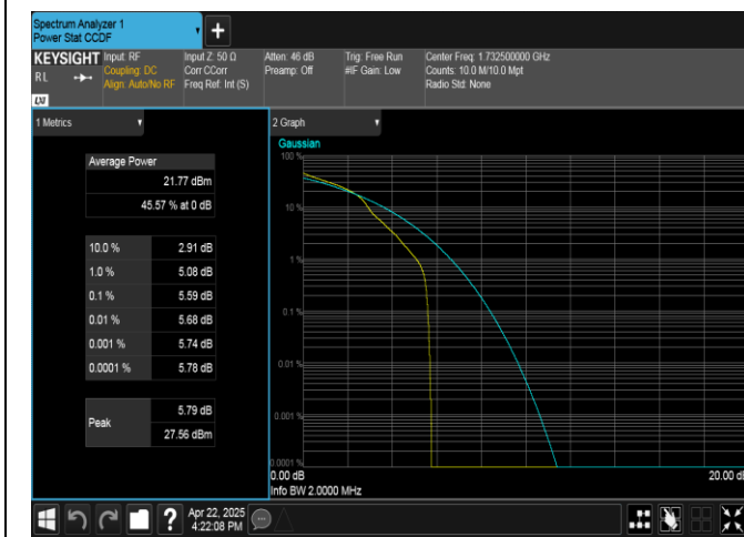
Band4-1.4MHz-16QAM-20175-1RB#0-PASS
