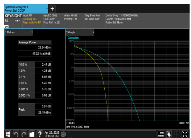
Band4-3MHz-QPSK-20385-15RB#0-PASS
