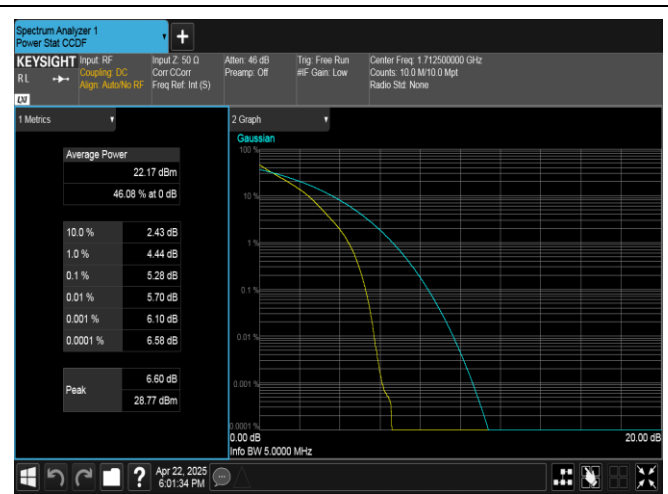
Band4-5MHz-QPSK-19975-25RB#0-PASS
