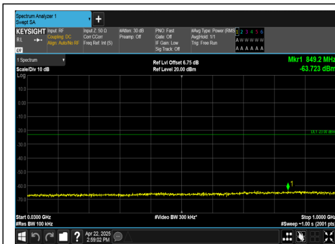
Band2-20MHz-16QAM-18900-100RB#0-30~1000-PASS
