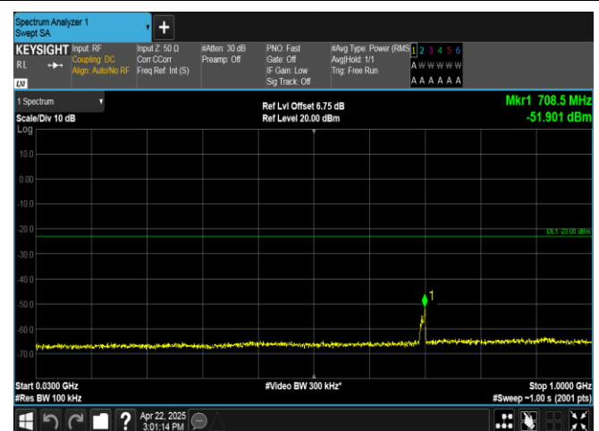
Band2-20MHz-16QAM-19100-1RB#0-30~1000-PASS
