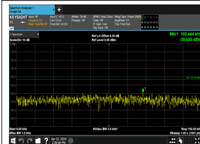
Band2-20MHz-16QAM-18900-100RB#0-0.009~0.15-PASS
