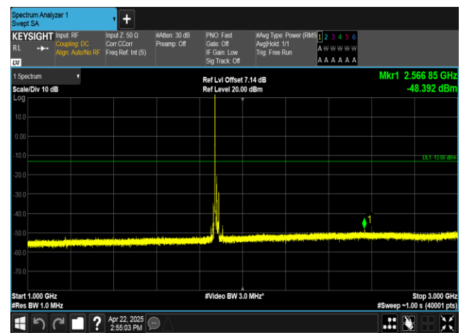
Band2-20MHz-16QAM-18900-1RB#0-1000~3000-PASS
