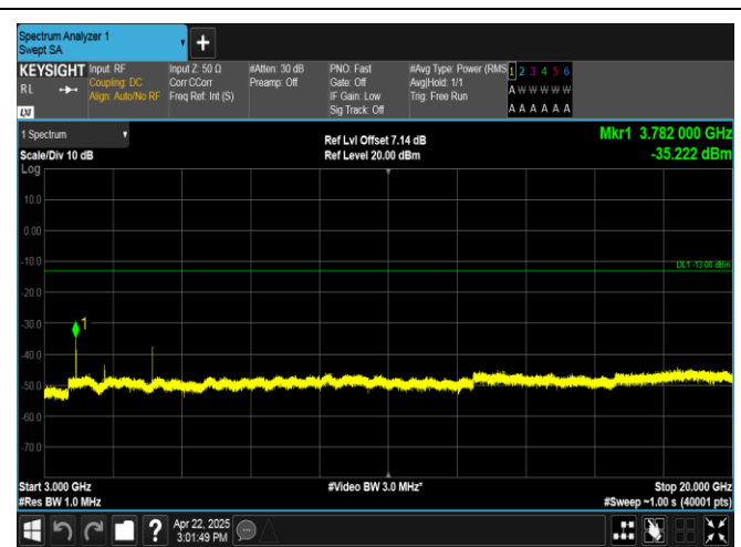
Band2-20MHz-16QAM-19100-1RB#0-3000~20000-PASS
