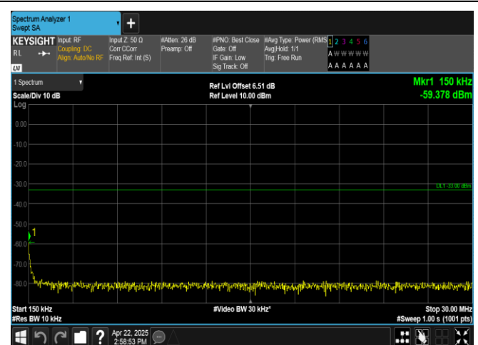
Band2-20MHz-16QAM-18900-100RB#0-0.15~30-PASS
