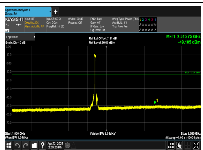
Band2-20MHz-16QAM-18900-100RB#0-1000~3000-PASS
