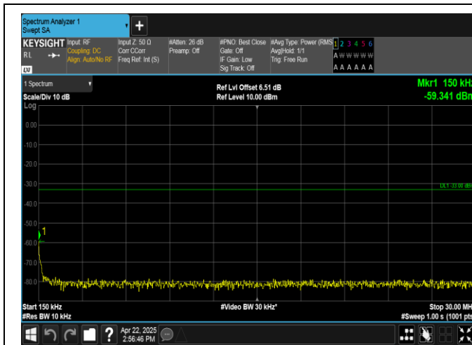
Band2-20MHz-16QAM-18900-1RB#99-0.15~30-PASS
