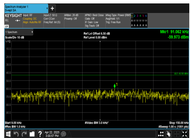
Band2-20MHz-16QAM-19100-1RB#0-0.009~0.15-PASS
