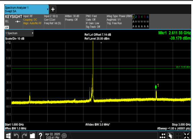
Band2-20MHz-16QAM-19100-1RB#99-1000~3000-PASS
