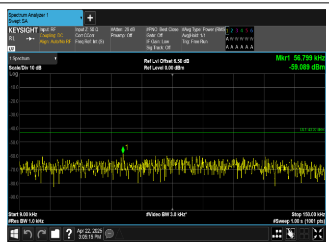
Band2-20MHz-16QAM-19100-100RB#0-0.009~0.15-PASS
