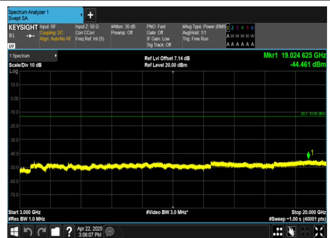
Band2-20MHz-16QAM-19100-100RB#0-3000~20000-PASS
