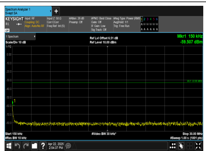
Band2-20MHz-16QAM-18900-1RB#0-0.15~30-PASS
