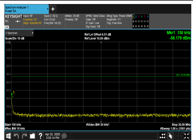
Band2-20MHz-16QAM-19100-1RB#99-0.15~30-PASS
