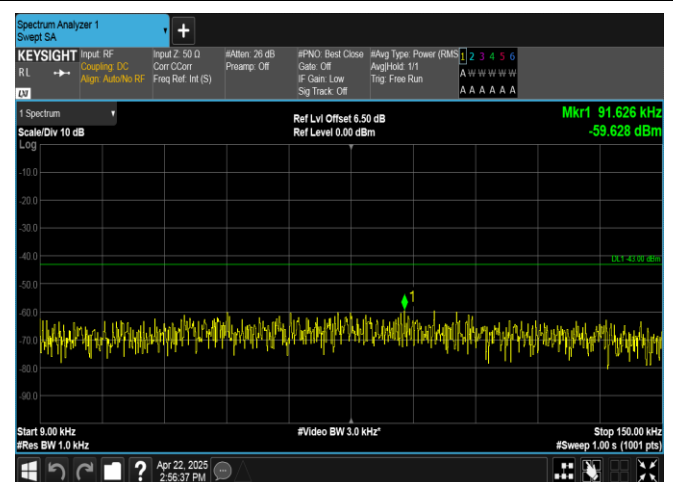
Band2-20MHz-16QAM-18900-1RB#99-0.009~0.15-PASS
