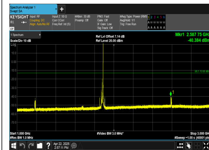
Band2-20MHz-16QAM-18900-1RB#99-1000~3000-PASS
