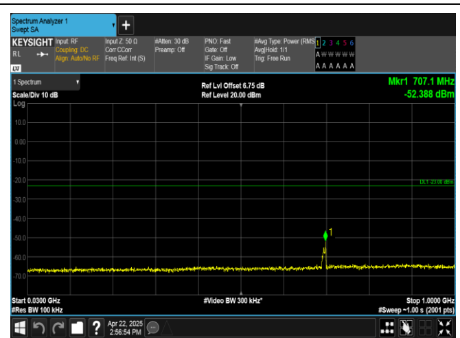
Band2-20MHz-16QAM-18900-1RB#99-30~1000-PASS
