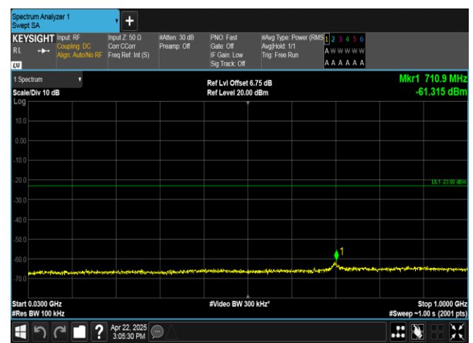
Band2-20MHz-16QAM-19100-100RB#0-30~1000-PASS
