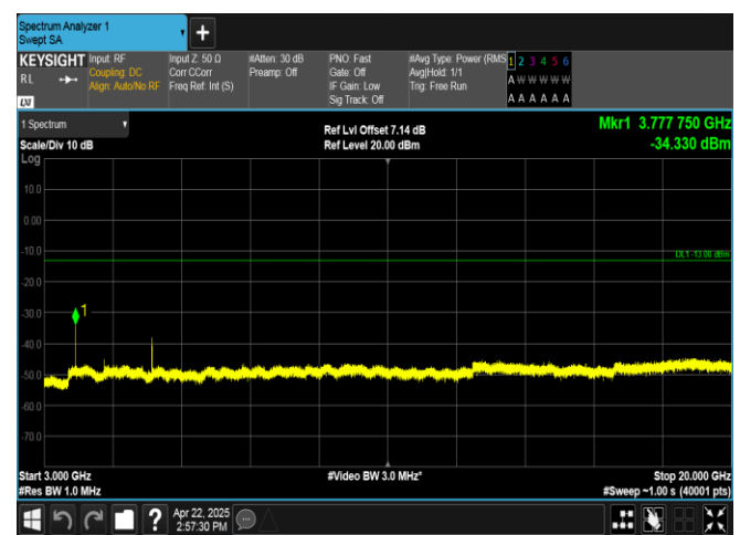
Band2-20MHz-16QAM-18900-1RB#99-3000~20000-PASS
