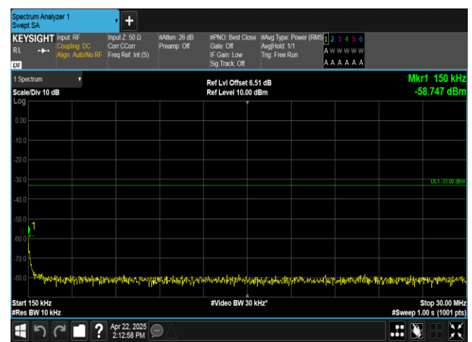
Band2-15MHz-16QAM-19125-1RB#74-0.15~30-PASS
