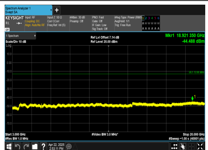
Band2-20MHz-16QAM-18700-100RB#0-3000~20000-PASS
