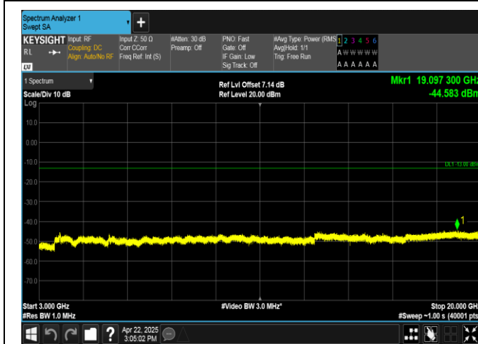
Band2-20MHz-QPSK-19100-100RB#0-3000~20000-PASS
