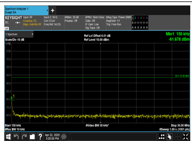
Band2-20MHz-QPSK-19100-1RB#0-0.15~30-PASS
