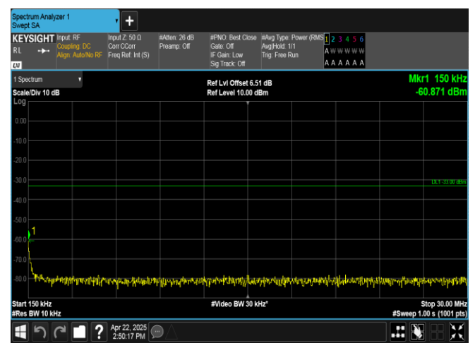
Band2-20MHz-16QAM-18700-1RB#99-0.15~30-PASS
