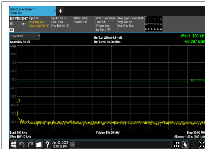
Band2-20MHz-QPSK-18700-1RB#99-0.15~30-PASS
