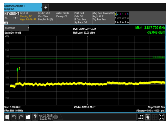
Band2-20MHz-QPSK-19100-1RB#99-3000~20000-PASS
