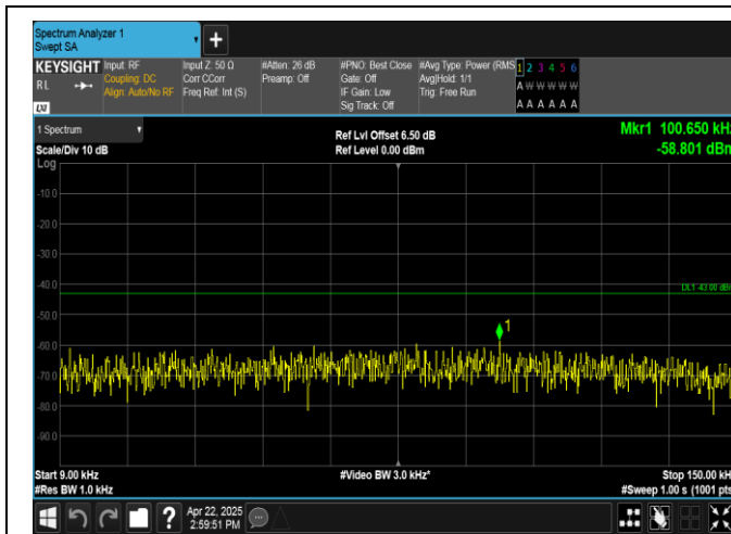
Band2-20MHz-QPSK-19100-1RB#0-0.009~0.15-PASS
