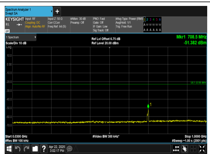
Band2-20MHz-QPSK-19100-1RB#99-30~1000-PASS
