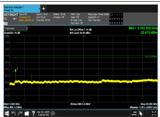
Band2-20MHz-16QAM-18700-1RB#0-3000~20000-PASS
