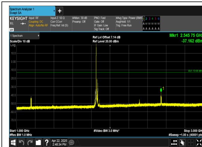
Band2-20MHz-16QAM-18700-1RB#0-1000~3000-PASS
