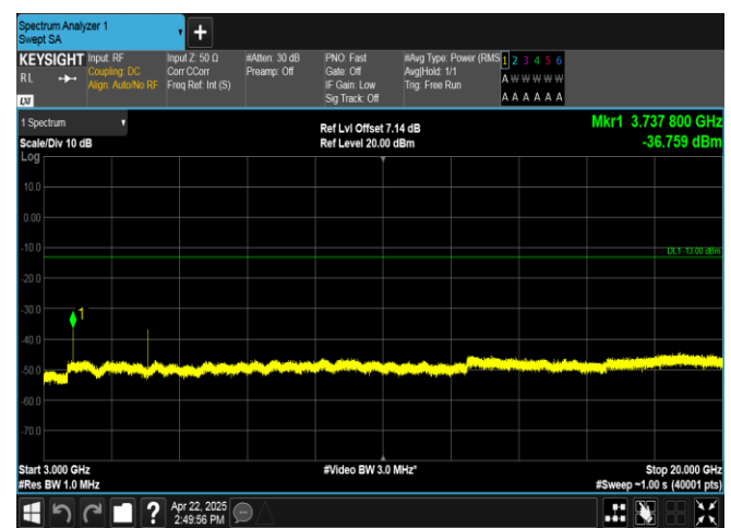
Band2-20MHz-QPSK-18700-1RB#99-3000~20000-PASS
