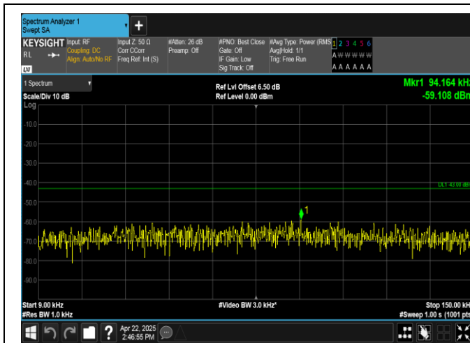
Band2-20MHz-QPSK-18700-1RB#0-0.009~0.15-PASS
