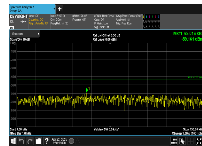
Band2-20MHz-16QAM-18700-1RB#99-0.009~0.15-PASS
