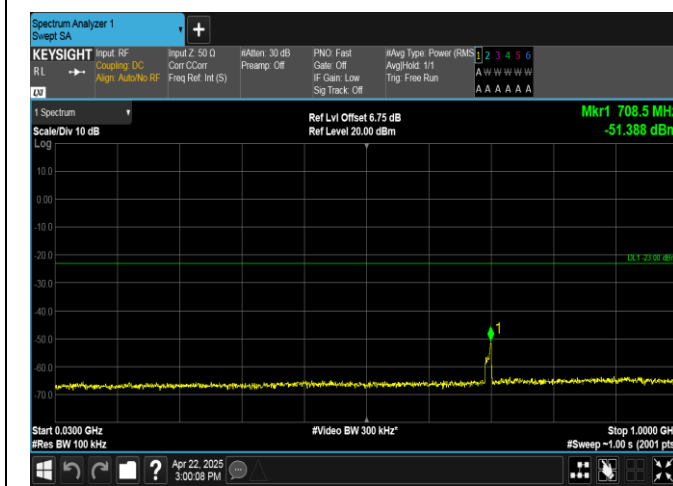
Band2-20MHz-QPSK-19100-1RB#0-30~1000-PASS
