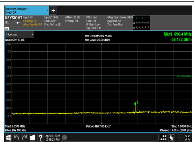
Band2-20MHz-QPSK-18700-1RB#99-30~1000-PASS
