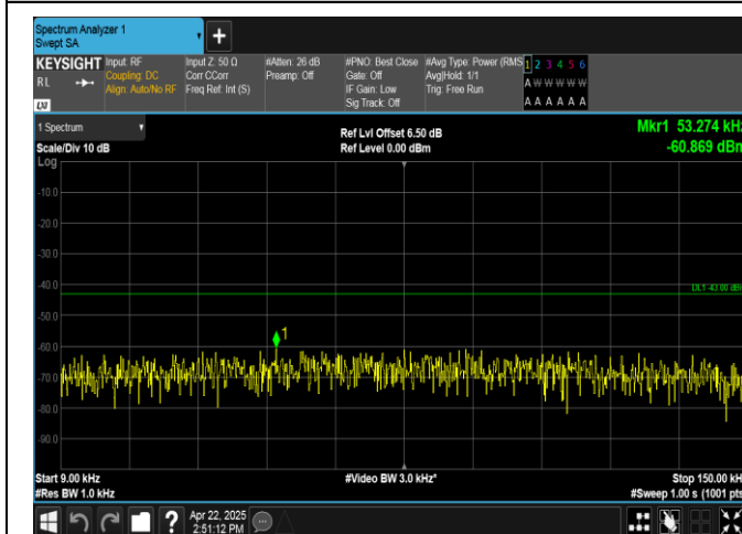
Band2-20MHz-QPSK-18700-100RB#0-0.009~0.15-PASS
