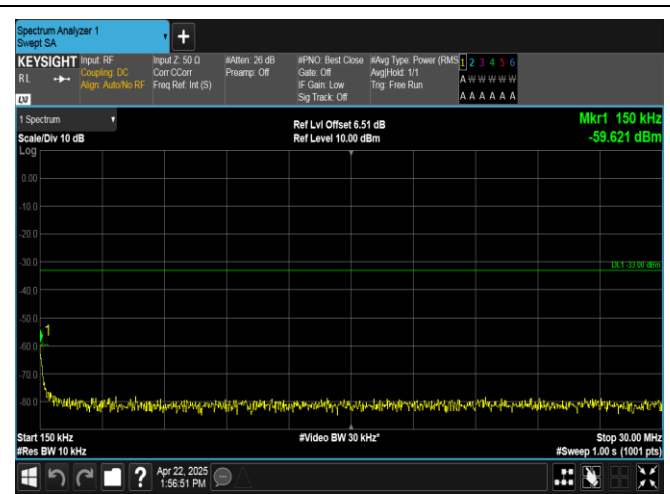
Band2-15MHz-QPSK-18675-1RB#0-0.15~30-PASS
