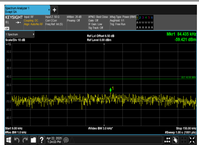
Band2-10MHz-16QAM-19150-50RB#0-0.009~0.15-PASS
