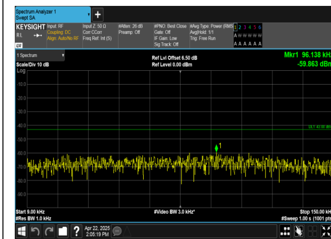
Band2-15MHz-QPSK-18900-1RB#74-0.009~0.15-PASS
