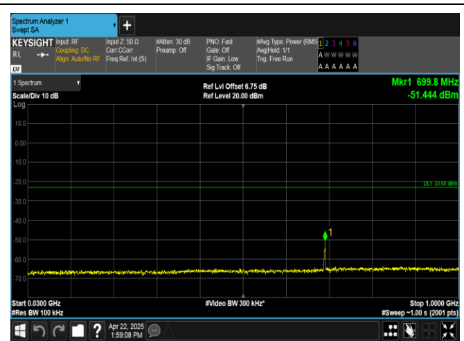
Band2-15MHz-QPSK-18675-1RB#74-30~1000-PASS
