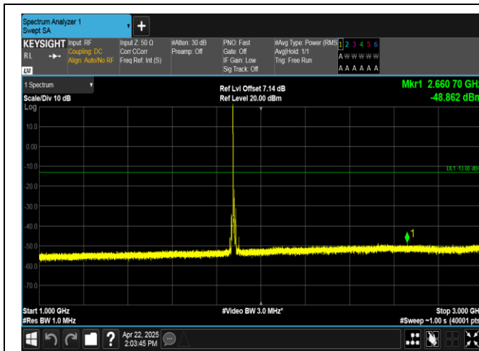
Band2-15MHz-QPSK-18900-1RB#0-1000~3000-PASS
