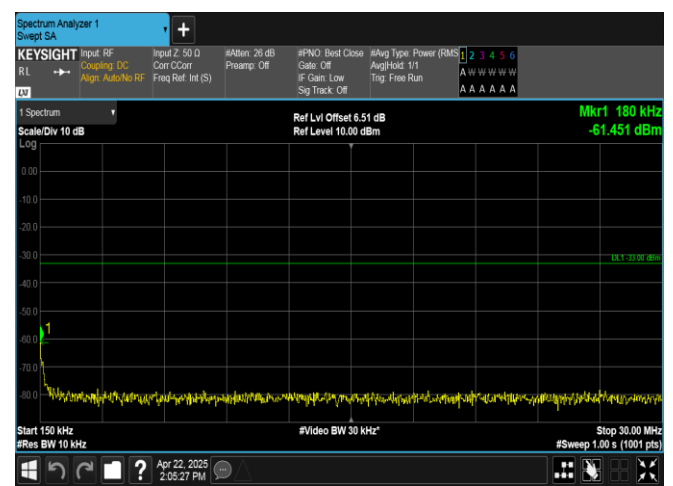
Band2-15MHz-QPSK-18900-1RB#74-0.15~30-PASS
