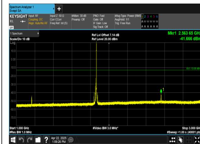
Band2-15MHz-QPSK-18675-1RB#74-1000~3000-PASS
