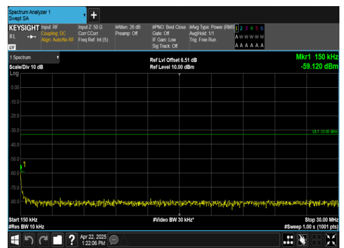
Band2-10MHz-16QAM-19150-1RB#49-0.15~30-PASS
