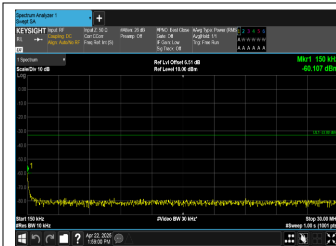
Band2-15MHz-QPSK-18675-1RB#74-0.15~30-PASS
