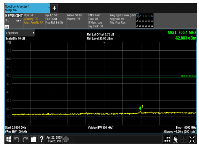
Band2-10MHz-16QAM-19150-50RB#0-30~1000-PASS
