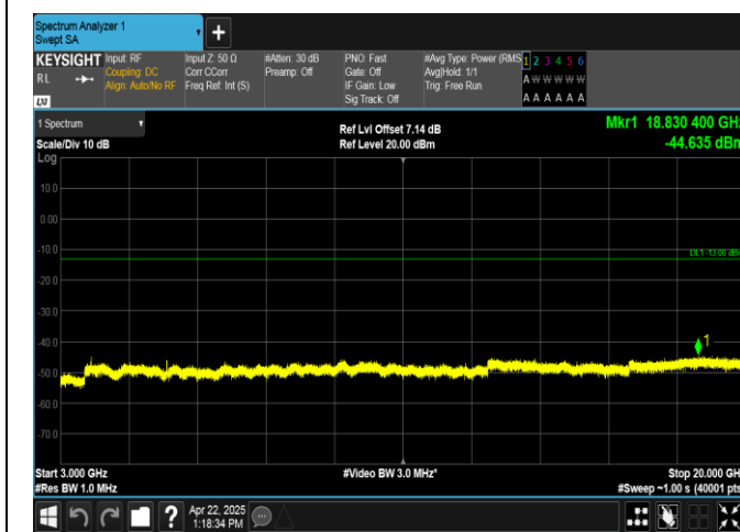
Band2-10MHz-16QAM-18900-50RB#0-3000~20000-PASS
