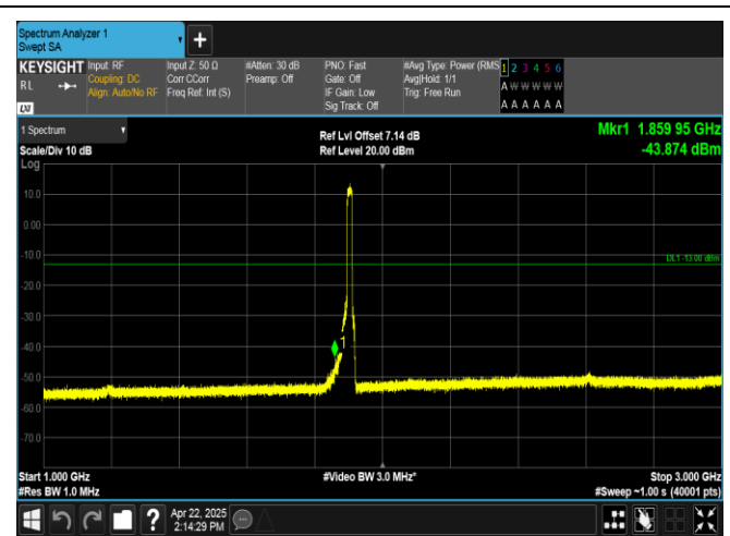
Band2-15MHz-QPSK-19125-75RB#0-1000~3000-PASS
