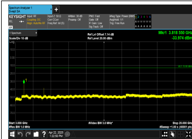
Band2-10MHz-16QAM-19150-1RB#49-3000~20000-PASS
