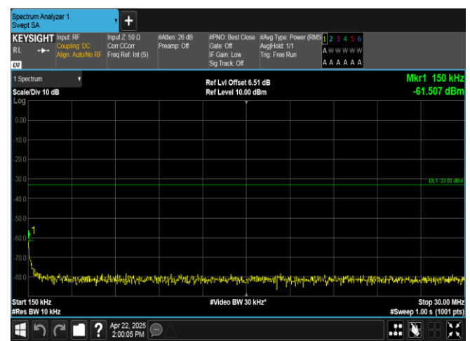
Band2-15MHz-16QAM-18675-1RB#74-0.15~30-PASS
