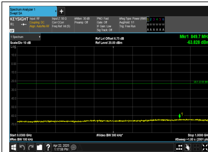
Band2-10MHz-16QAM-18900-50RB#0-30~1000-PASS
