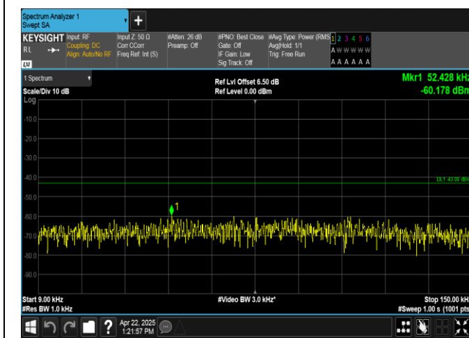
Band2-10MHz-16QAM-19150-1RB#49-0.009~0.15-PASS
