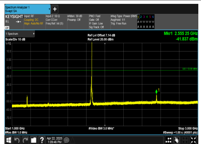
Band2-10MHz-16QAM-18650-1RB#49-1000~3000-PASS
