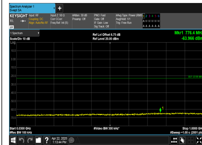
Band2-10MHz-16QAM-18900-1RB#0-30~1000-PASS
