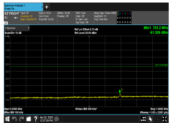
Band2-5MHz-16QAM-19175-25RB#0-30~1000-PASS
