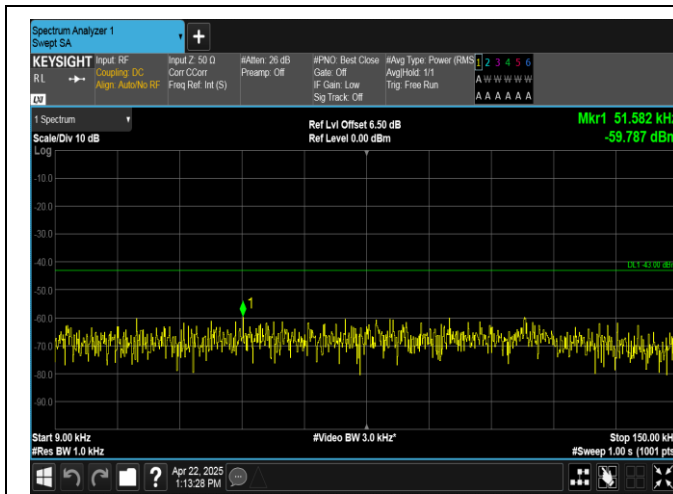
Band2-10MHz-16QAM-18900-1RB#0-0.009~0.15-PASS
