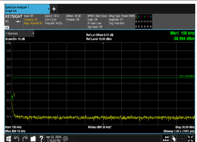
Band2-10MHz-QPSK-18650-50RB#0-0.15~30-PASS
