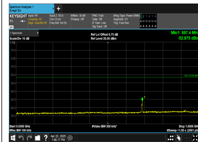
Band2-10MHz-QPSK-18650-1RB#0-30~1000-PASS
