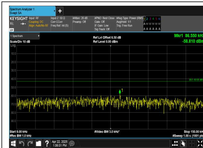
Band2-10MHz-QPSK-18650-1RB#0-0.009~0.15-PASS
