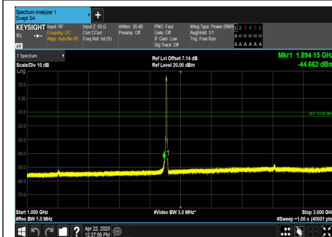
Band2-5MHz-16QAM-19175-25RB#0-1000~3000-PASS
