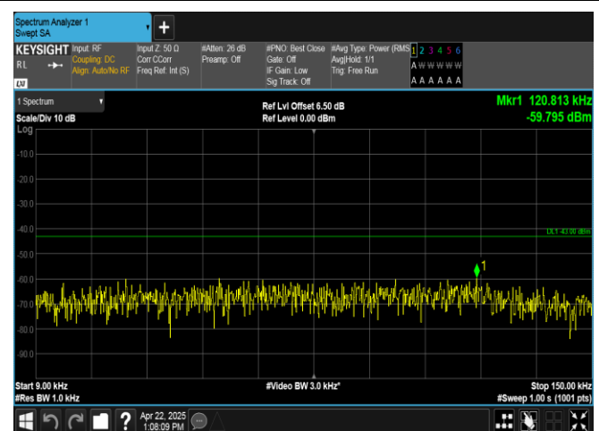
Band2-10MHz-QPSK-18650-1RB#49-0.009~0.15-PASS
