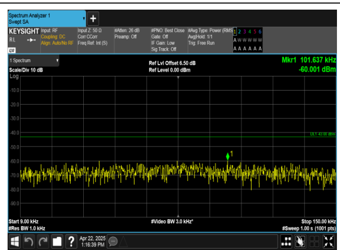
Band2-10MHz-QPSK-18900-50RB#0-0.009~0.15-PASS
