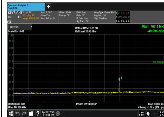
Band2-10MHz-QPSK-19150-1RB#0-30~1000-PASS
