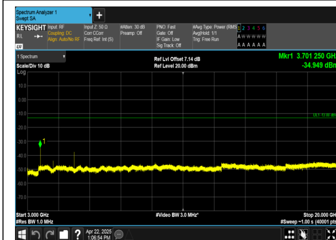
Band2-10MHz-QPSK-18650-1RB#0-3000~20000-PASS
