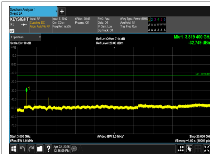
Band2-5MHz-16QAM-19175-1RB#24-3000~20000-PASS
