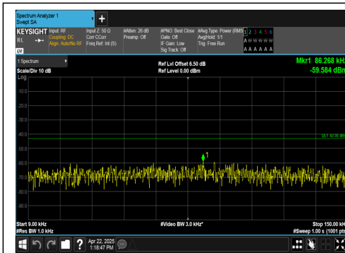
Band2-10MHz-QPSK-19150-1RB#0-0.009~0.15-PASS
