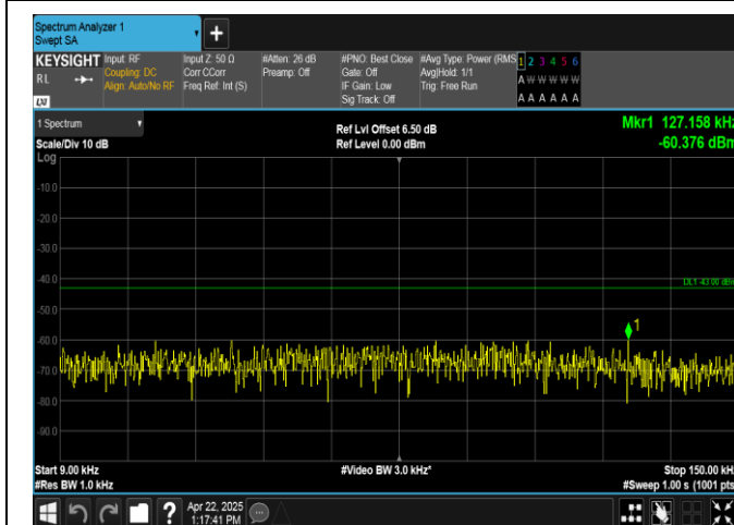
Band2-10MHz-16QAM-18900-50RB#0-0.009~0.15-PASS
