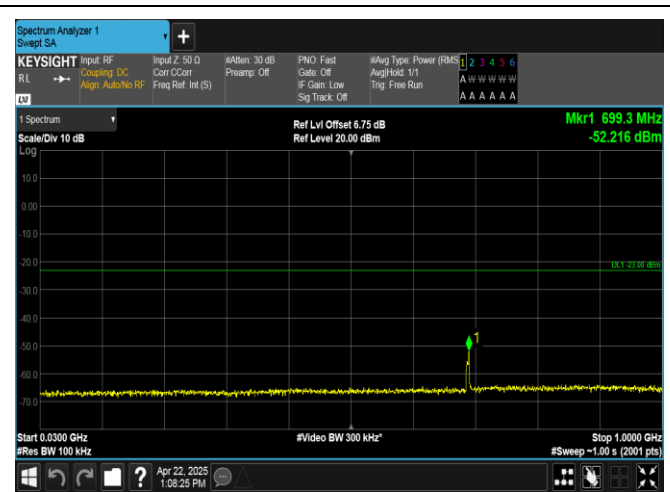
Band2-10MHz-QPSK-18650-1RB#49-30~1000-PASS
