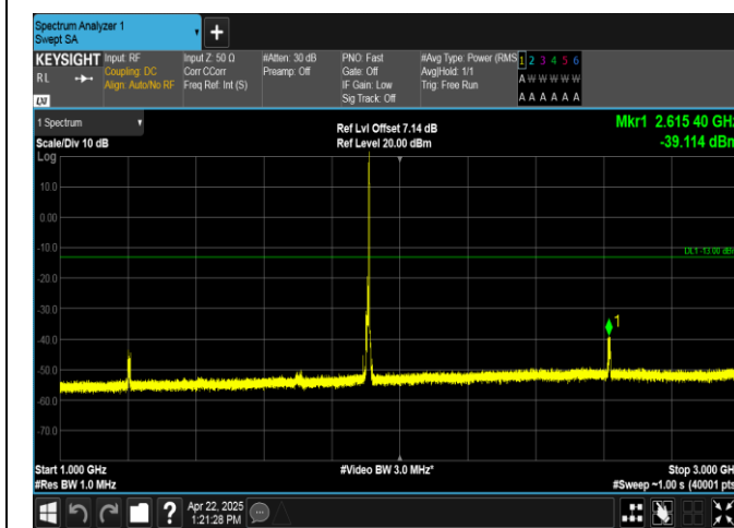
Band2-10MHz-QPSK-19150-1RB#49-1000~3000-PASS
