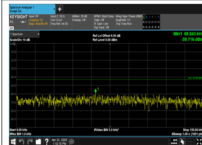
Band2-10MHz-QPSK-18650-50RB#0-0.009~0.15-PASS
