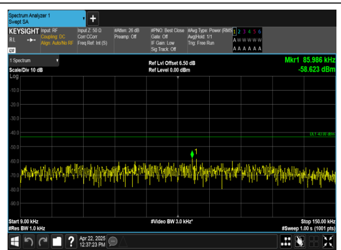
Band2-5MHz-16QAM-19175-25RB#0-0.009~0.15-PASS
