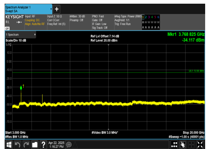
Band2-10MHz-16QAM-18900-1RB#49-3000~20000-PASS
