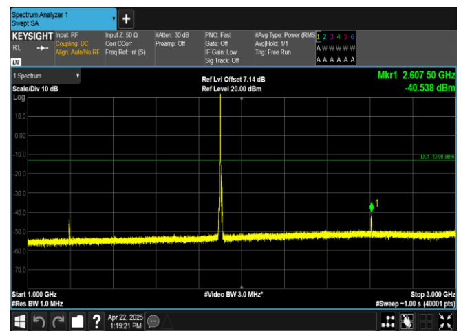
Band2-10MHz-QPSK-19150-1RB#0-1000~3000-PASS
