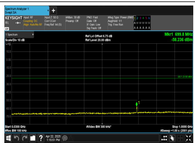
Band2-10MHz-16QAM-18900-1RB#49-30~1000-PASS
