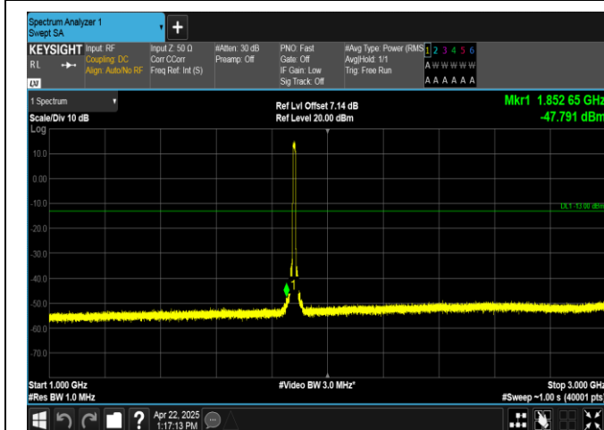
Band2-10MHz-QPSK-18900-50RB#0-1000~3000-PASS
