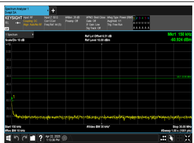
Band2-10MHz-16QAM-18900-1RB#0-0.15~30-PASS
