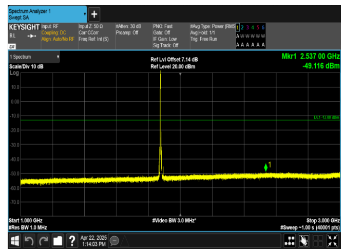
Band2-10MHz-16QAM-18900-1RB#0-1000~3000-PASS
