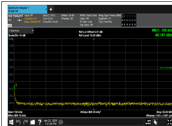
Band2-10MHz-QPSK-19150-1RB#49-0.15~30-PASS
