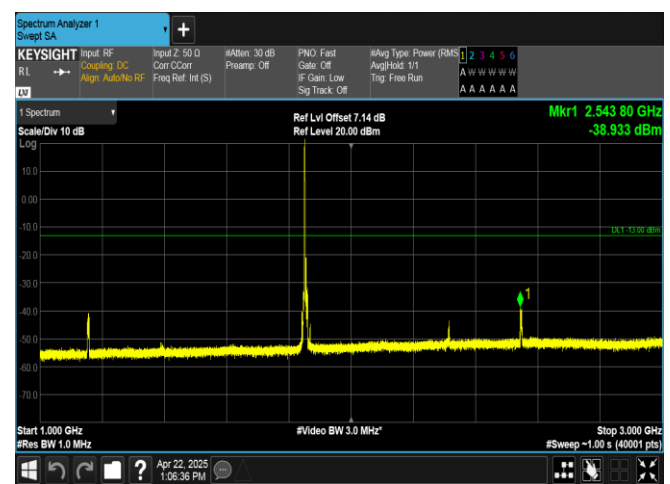
Band2-10MHz-QPSK-18650-1RB#0-1000~3000-PASS
