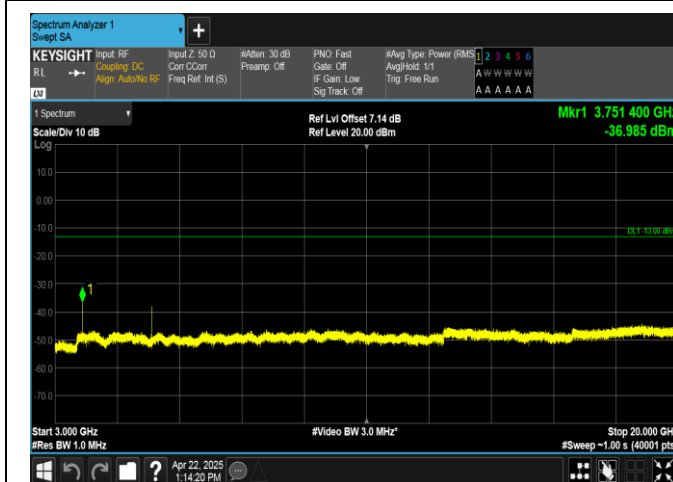
Band2-10MHz-16QAM-18900-1RB#0-3000~20000-PASS
