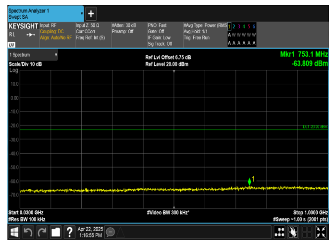
Band2-10MHz-QPSK-18900-50RB#0-30~1000-PASS
