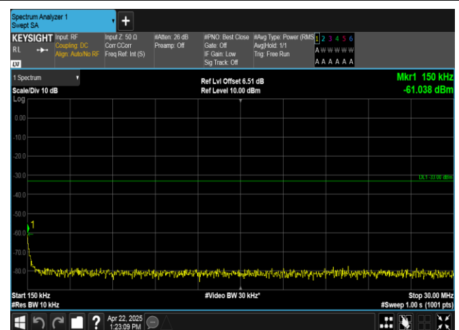
Band2-10MHz-QPSK-19150-50RB#0-0.15~30-PASS
