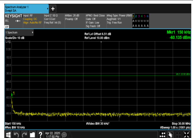
Band2-10MHz-16QAM-18900-50RB#0-0.15~30-PASS
