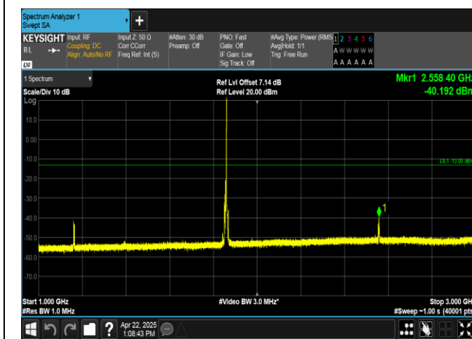
Band2-10MHz-QPSK-18650-1RB#49-1000~3000-PASS
