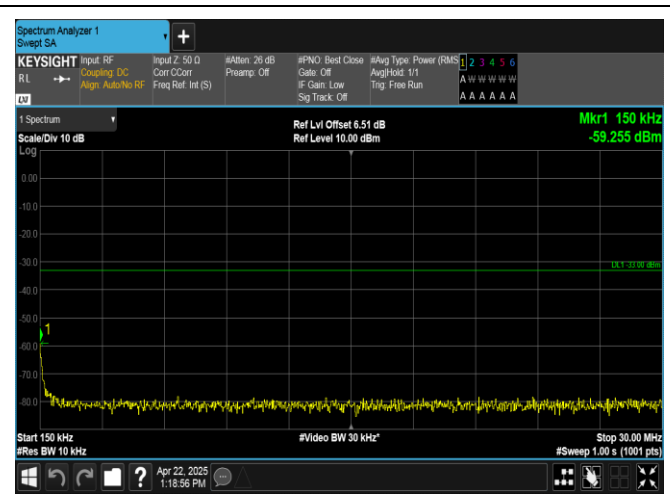
Band2-10MHz-QPSK-19150-1RB#0-0.15~30-PASS
