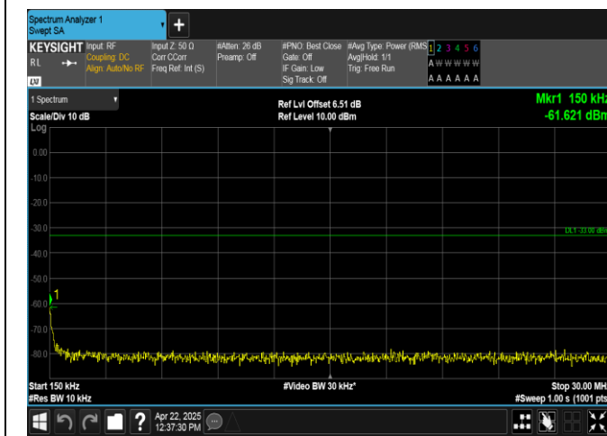
Band2-5MHz-16QAM-19175-25RB#0-0.15~30-PASS
