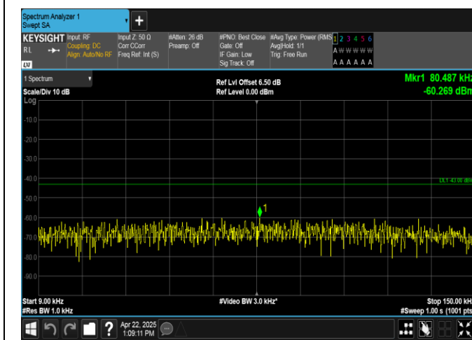
Band2-10MHz-16QAM-18650-1RB#49-0.009~0.15-PASS
