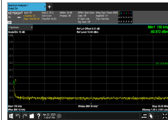
Band2-10MHz-QPSK-18900-50RB#0-0.15~30-PASS
