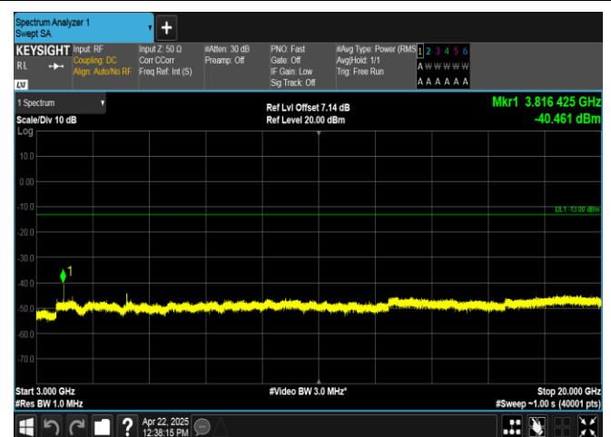
Band2-5MHz-16QAM-19175-25RB#0-3000~20000-PASS
