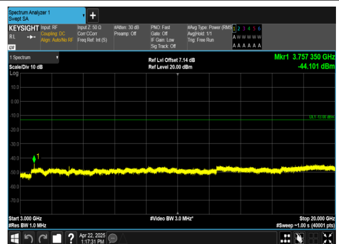
Band2-10MHz-QPSK-18900-50RB#0-3000~20000-PASS
