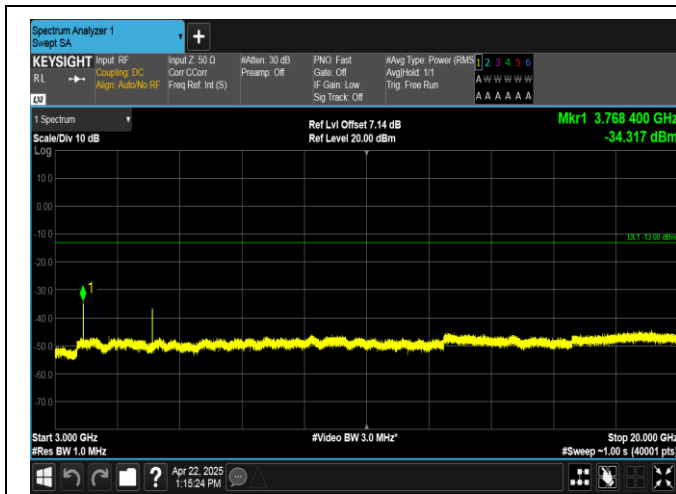
Band2-10MHz-QPSK-18900-1RB#49-3000~20000-PASS
