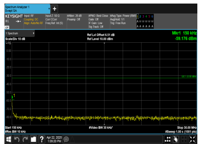
Band2-10MHz-16QAM-18650-1RB#49-0.15~30-PASS
