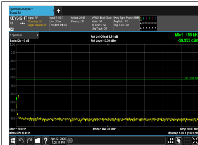
Band2-10MHz-QPSK-18650-1RB#49-0.15~30-PASS
