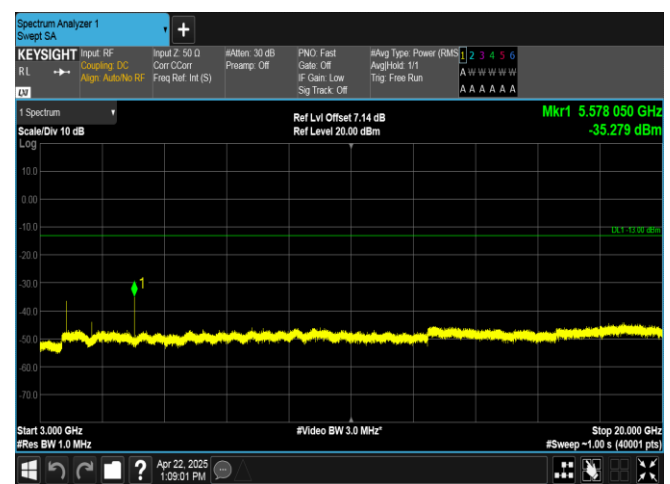
Band2-10MHz-QPSK-18650-1RB#49-3000~20000-PASS
