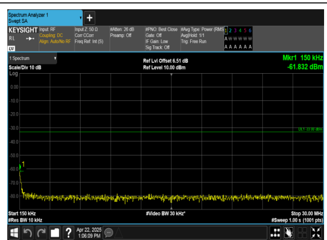
Band2-10MHz-QPSK-18650-1RB#0-0.15~30-PASS
