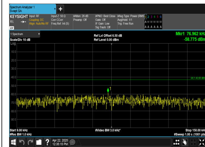
Band2-5MHz-16QAM-19175-1RB#24-0.009~0.15-PASS
