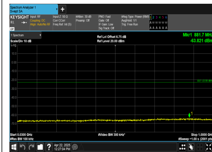
Band2-5MHz-16QAM-18900-1RB#0-30~1000-PASS
