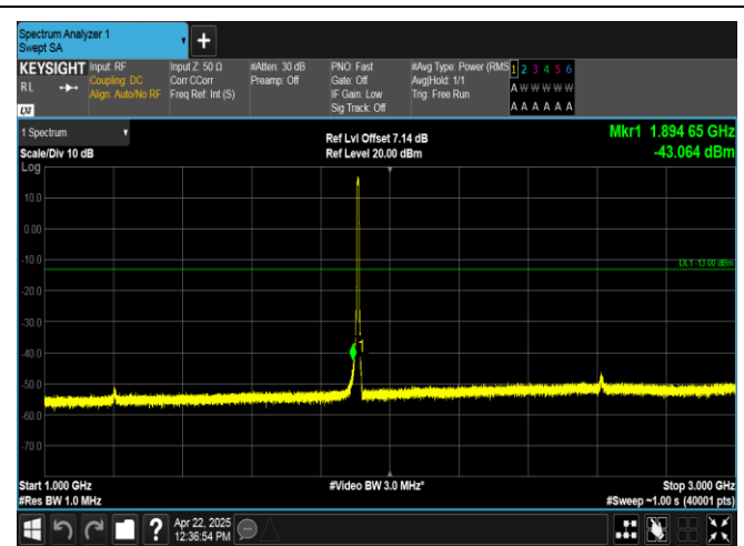
Band2-5MHz-QPSK-19175-25RB#0-1000~3000-PASS
