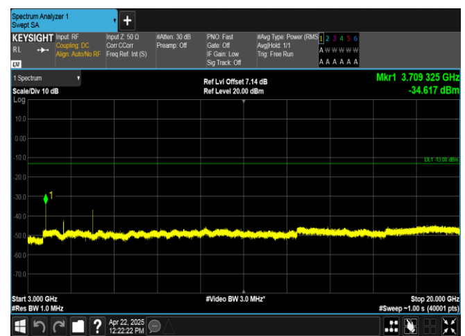
Band2-5MHz-QPSK-18625-1RB#24-3000~20000-PASS
