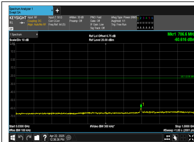
Band2-5MHz-QPSK-19175-25RB#0-30~1000-PASS
