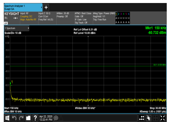
Band2-5MHz-16QAM-18625-1RB#24-0.15~30-PASS
