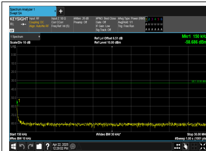
Band2-5MHz-16QAM-18900-1RB#24-0.15~30-PASS
