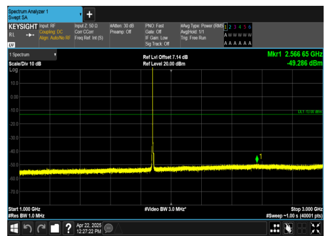
Band2-5MHz-16QAM-18900-1RB#0-1000~3000-PASS
