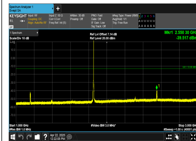
Band2-5MHz-QPSK-18625-1RB#24-1000~3000-PASS
