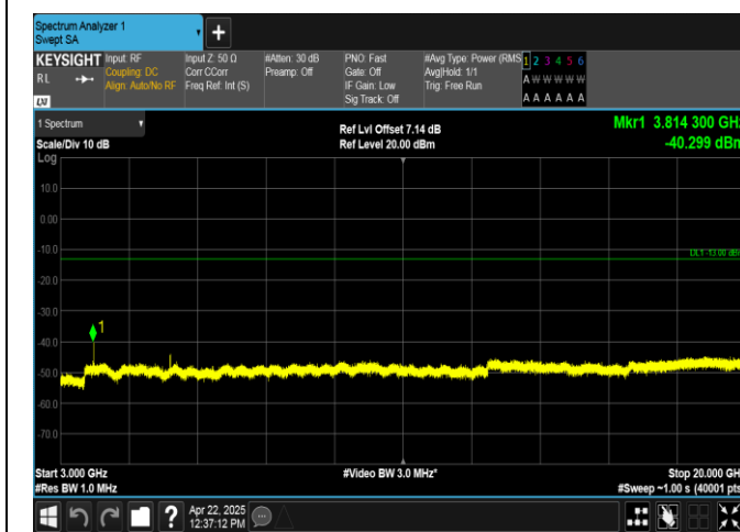
Band2-5MHz-QPSK-19175-25RB#0-3000~20000-PASS
