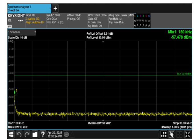
Band2-5MHz-16QAM-19175-1RB#24-0.15~30-PASS
