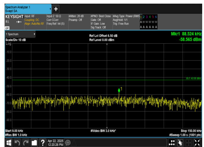
Band2-5MHz-16QAM-18625-1RB#0-0.009~0.15-PASS
